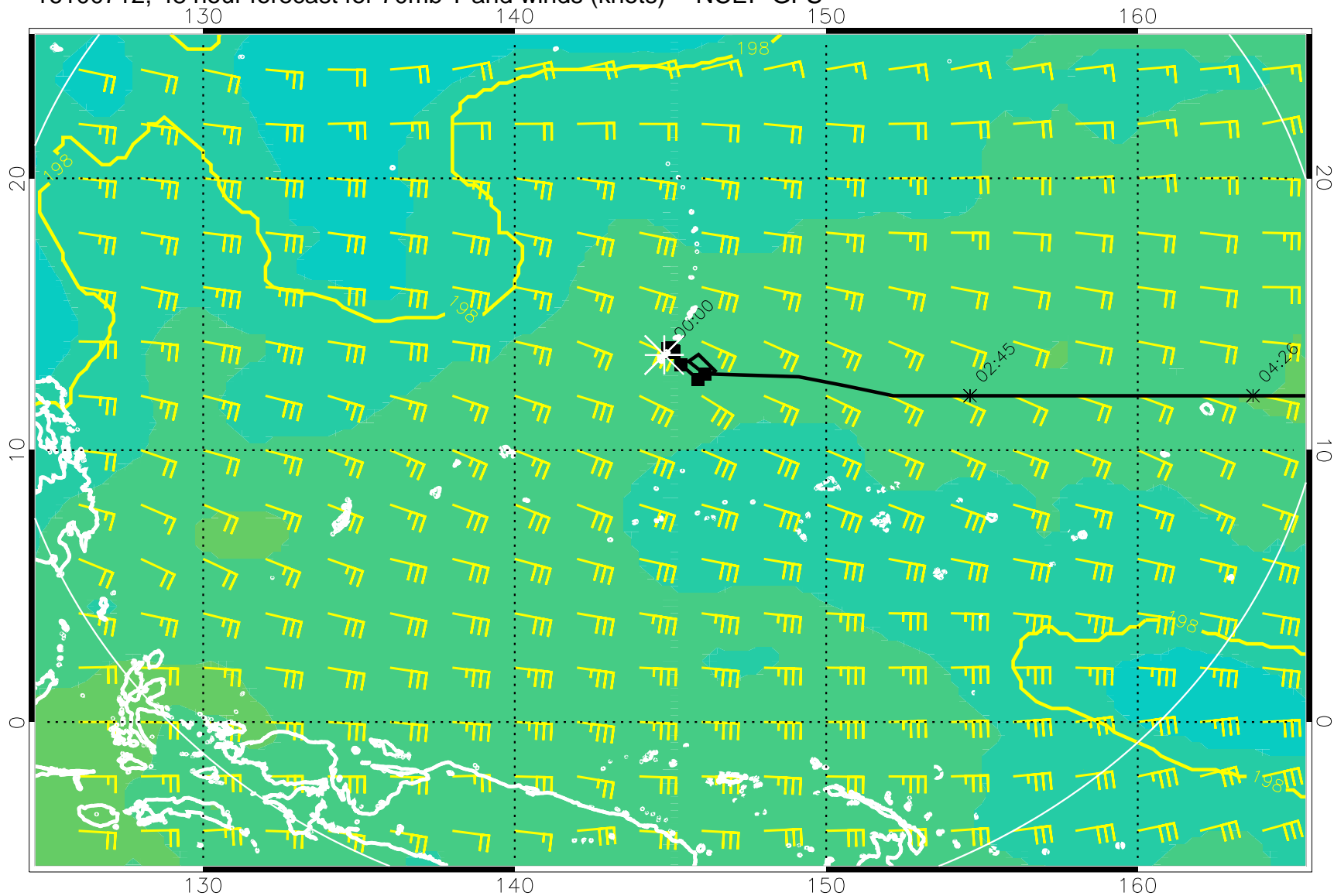
16100712, 48 hour forecast for 70mb T and winds (knots) -- NCEP GFS
