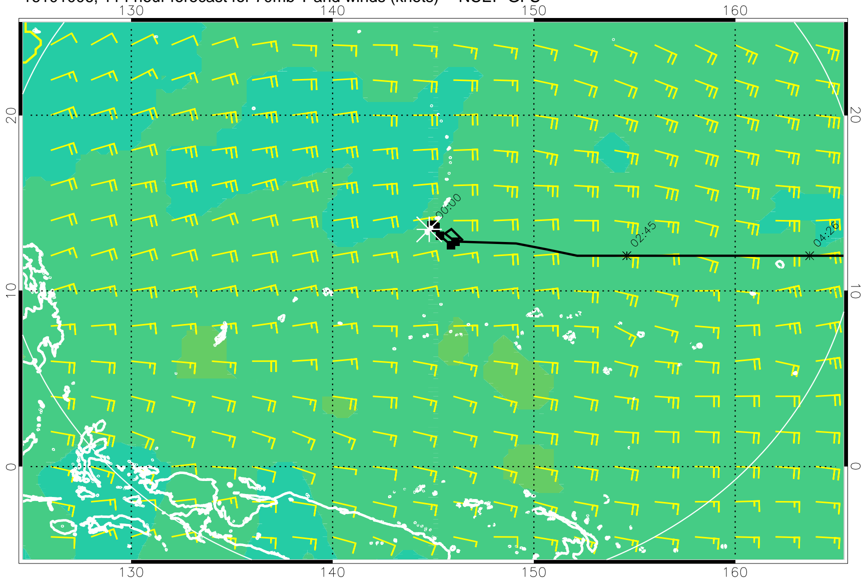
16101006, 114 hour forecast for 70mb T and winds (knots) -- NCEP GFS
