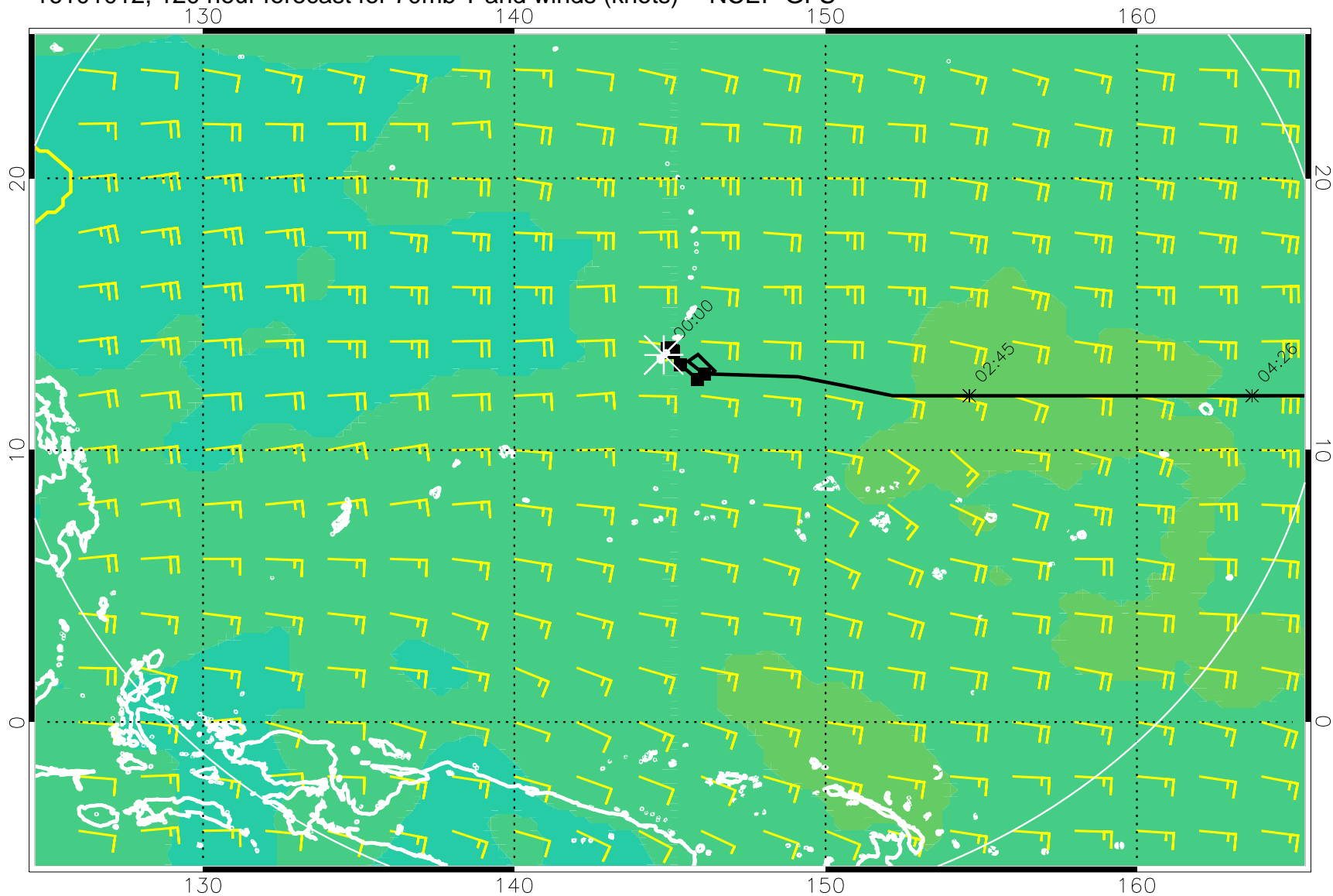
16101012, 120 hour forecast for 70mb T and winds (knots) -- NCEP GFS
