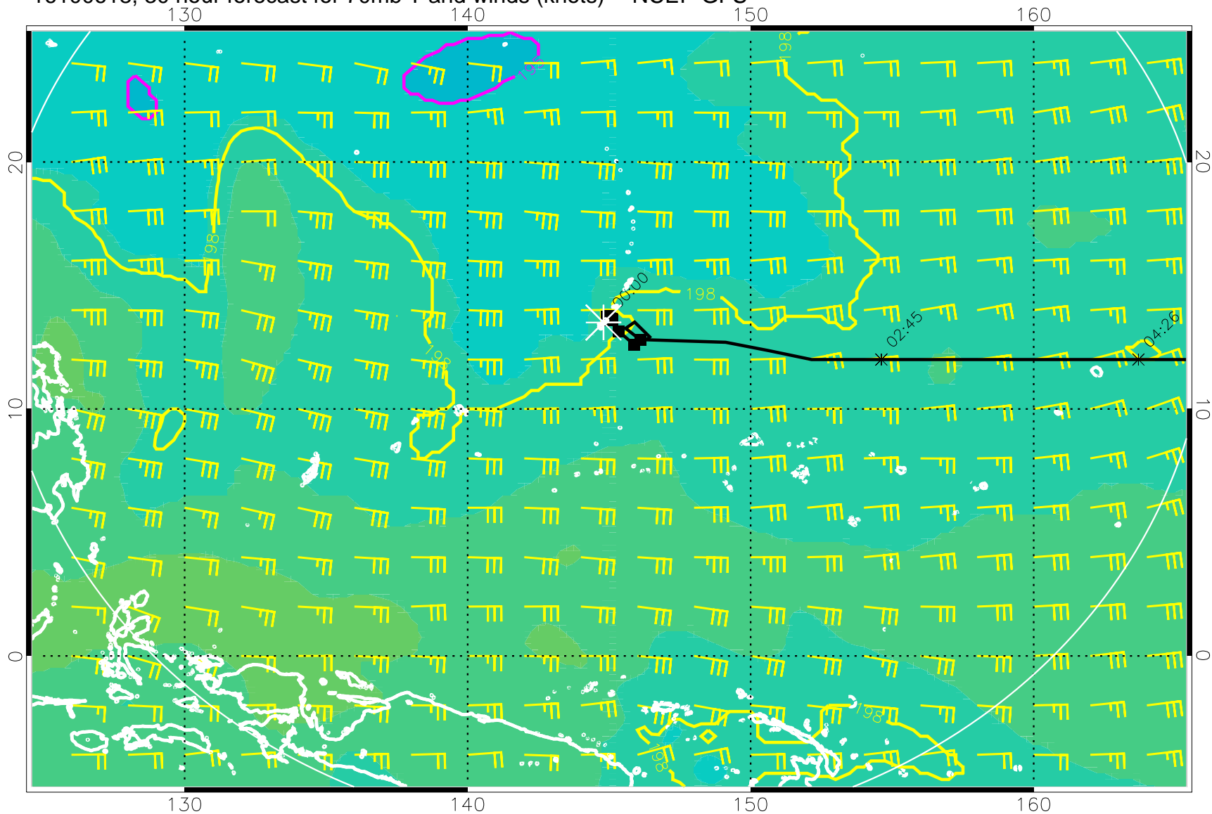
16100618, 30 hour forecast for 70mb T and winds (knots) -- NCEP GFS
