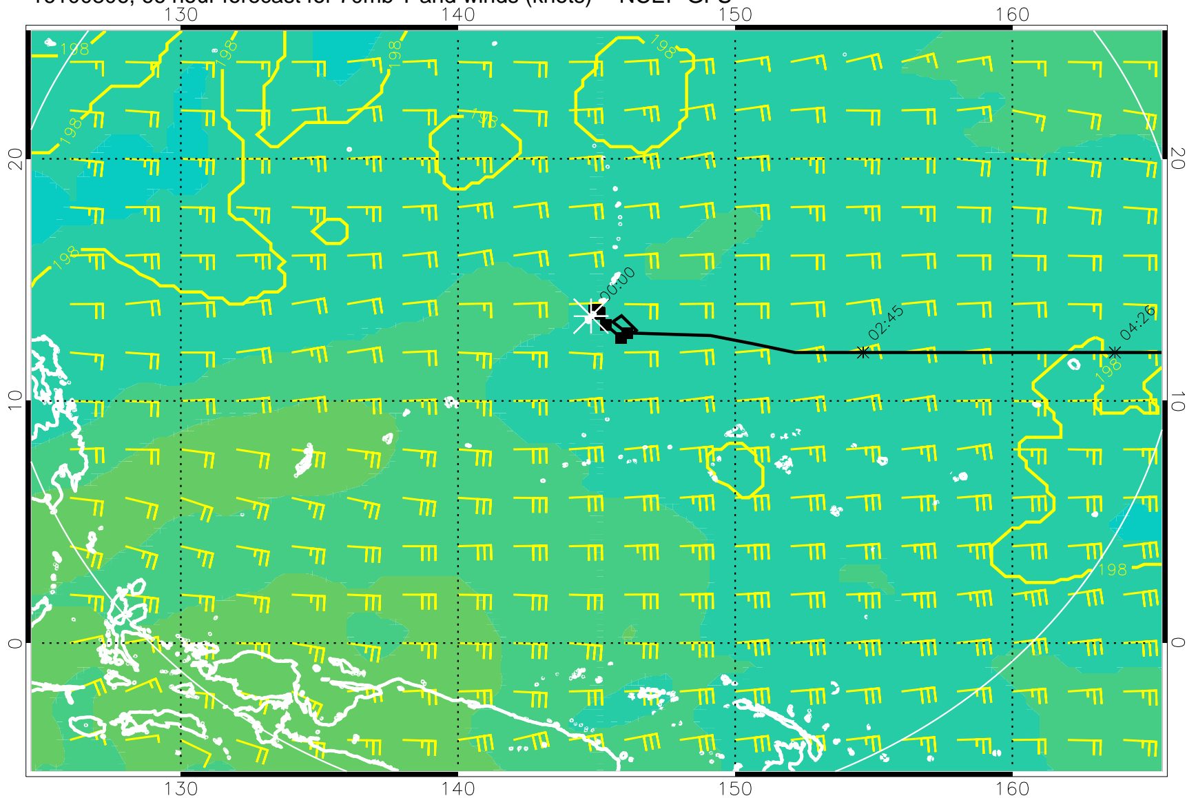
16100806, 66 hour forecast for 70mb T and winds (knots) -- NCEP GFS
