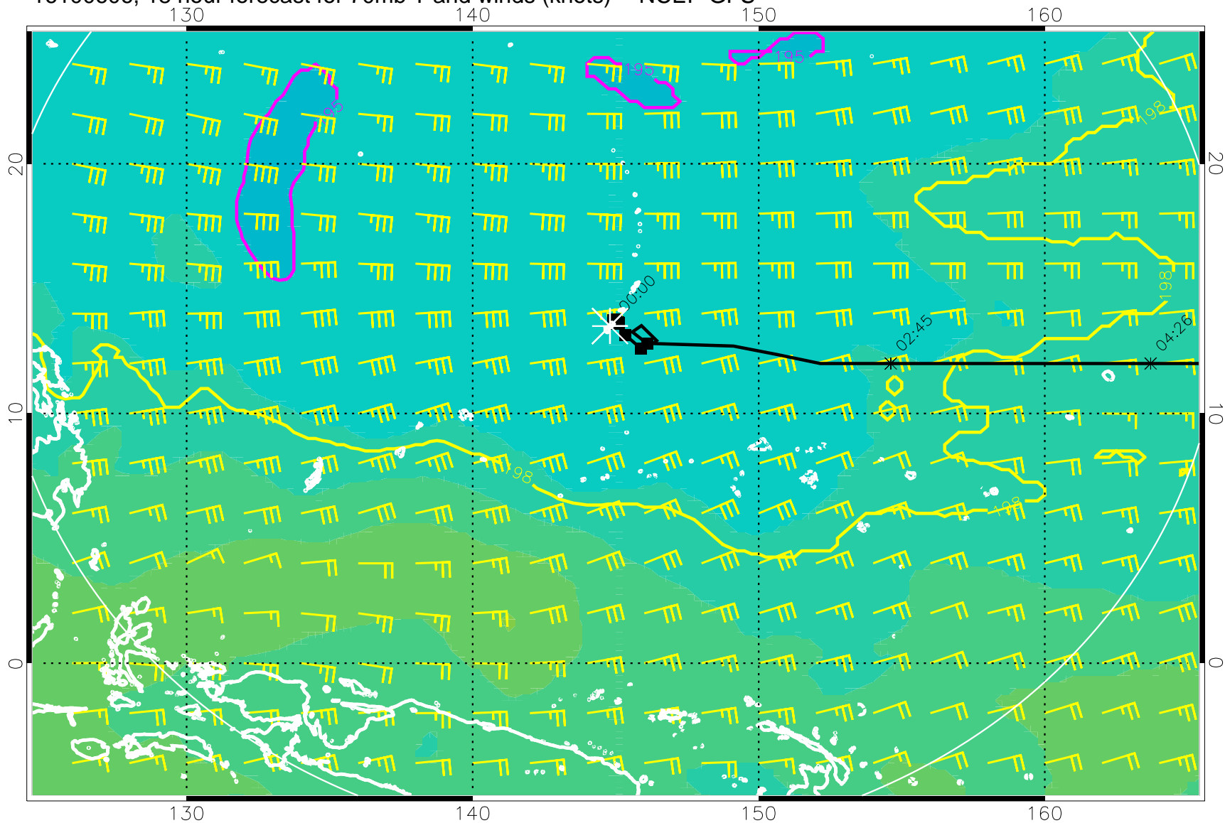
16100606, 18 hour forecast for 70mb T and winds (knots) -- NCEP GFS
