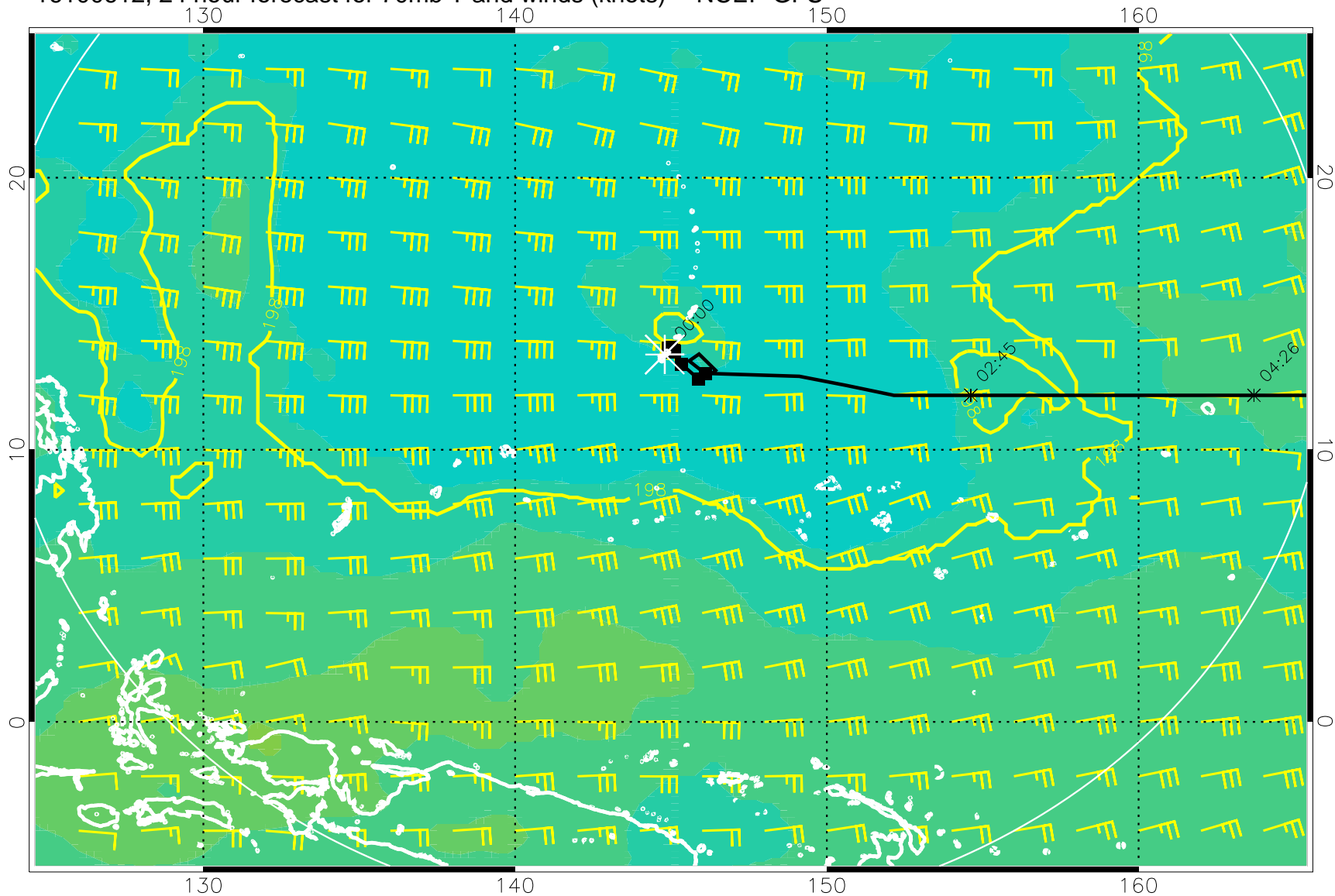
16100612, 24 hour forecast for 70mb T and winds (knots) -- NCEP GFS
