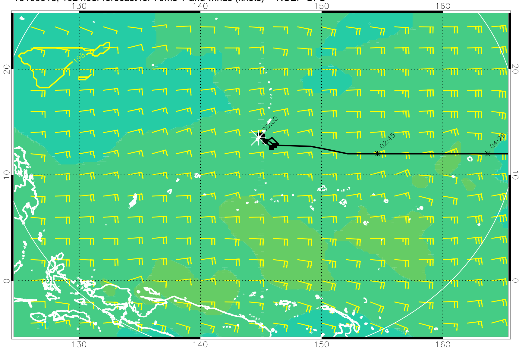
16100918, 102 hour forecast for 70mb T and winds (knots) -- NCEP GFS
