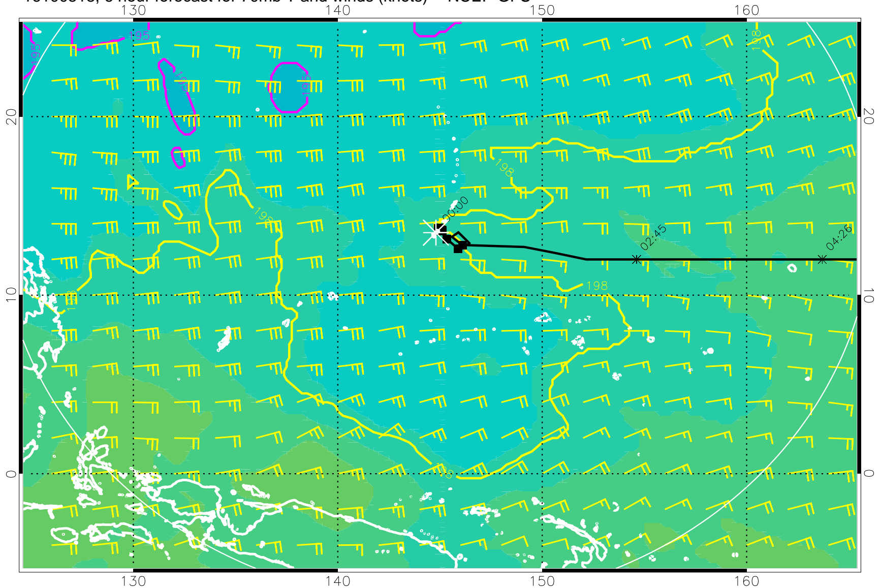
16100518, 6 hour forecast for 70mb T and winds (knots) -- NCEP GFS
