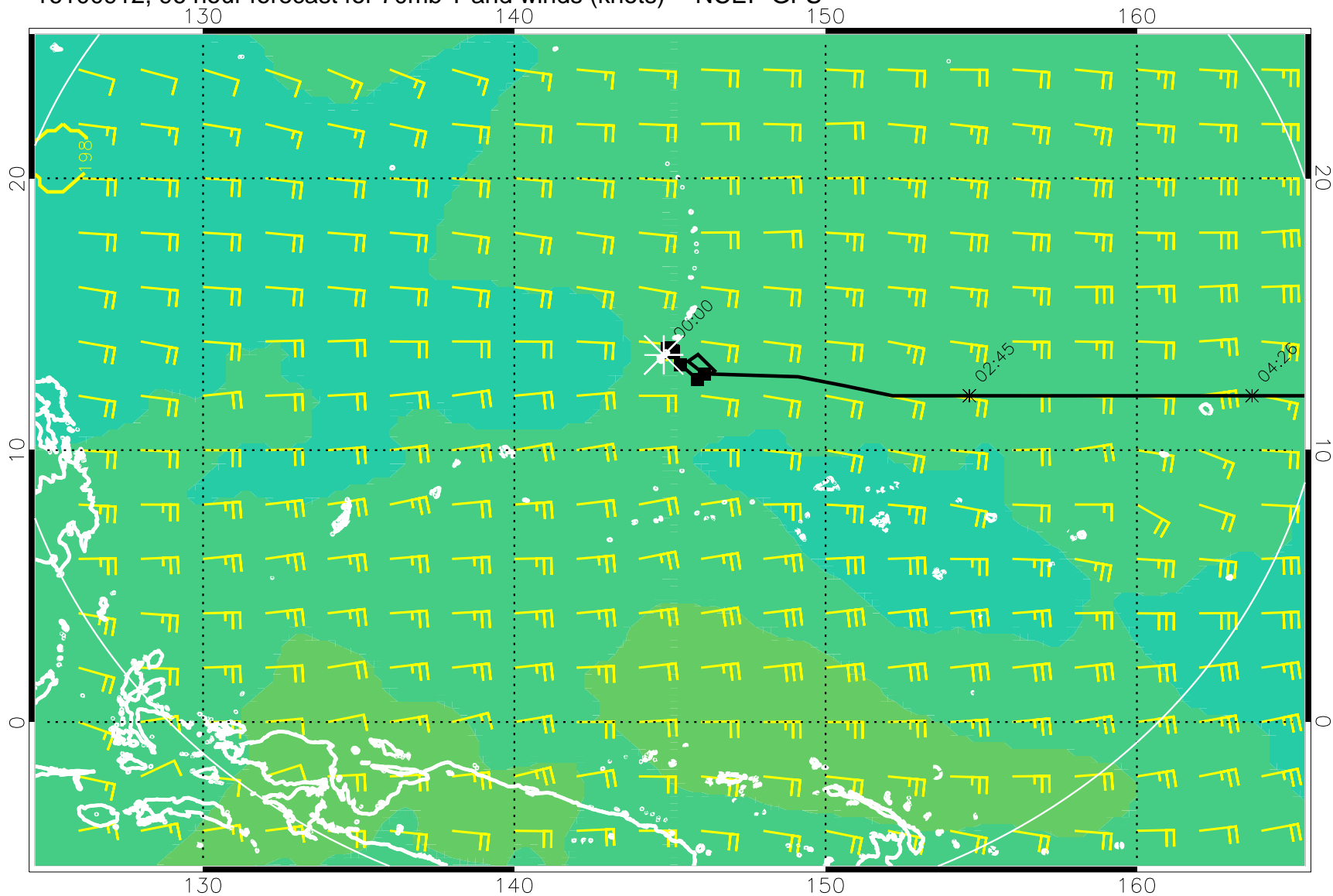
16100912, 96 hour forecast for 70mb T and winds (knots) -- NCEP GFS
