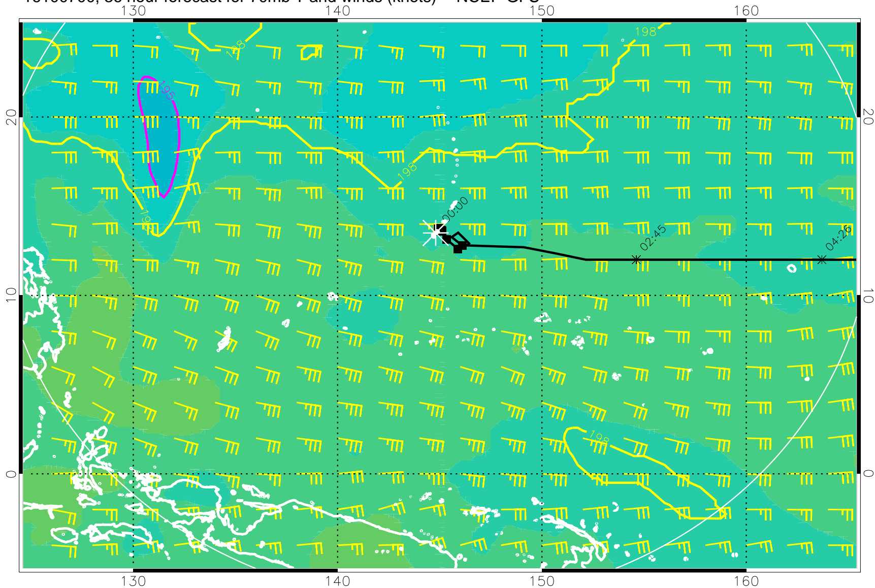
16100700, 36 hour forecast for 70mb T and winds (knots) -- NCEP GFS
