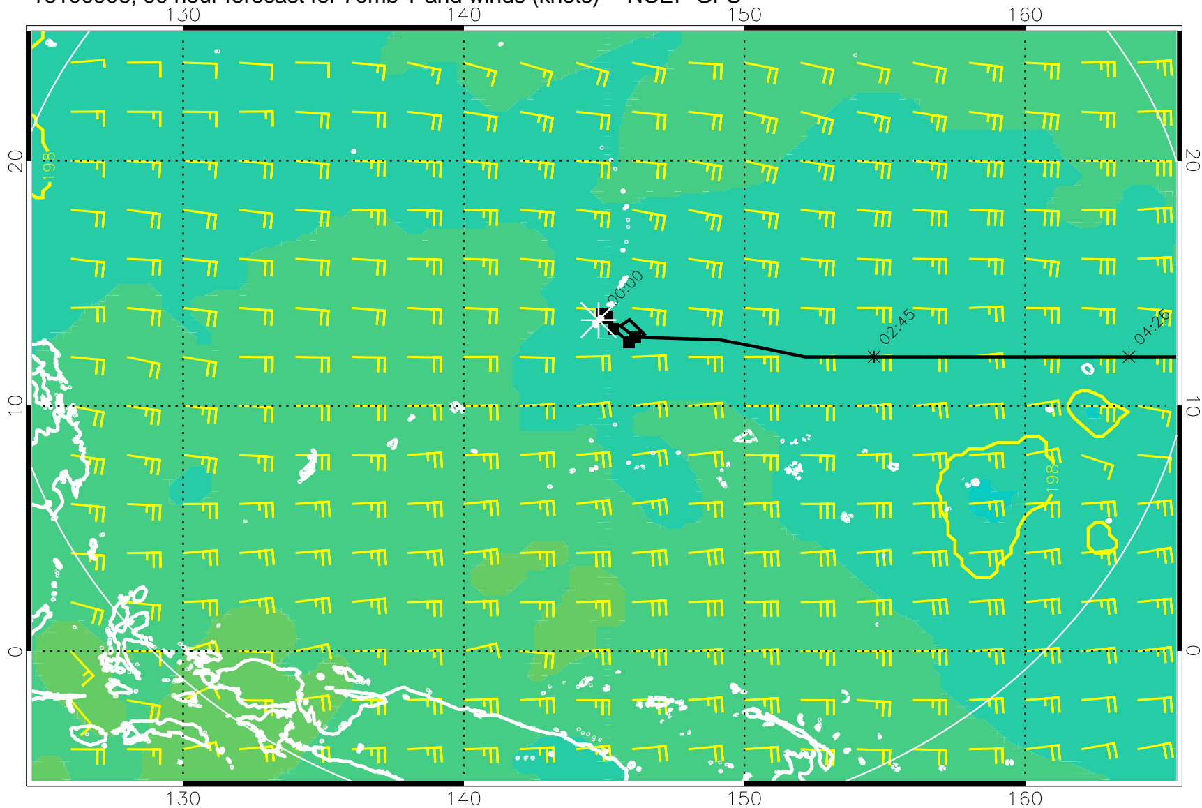
16100906, 90 hour forecast for 70mb T and winds (knots) -- NCEP GFS
