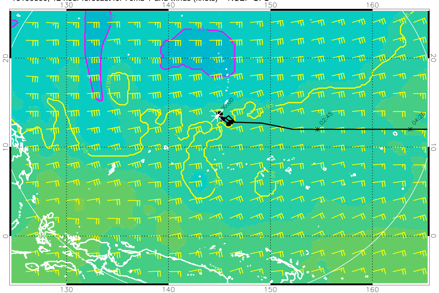
16100600, 12 hour forecast for 70mb T and winds (knots) -- NCEP GFS
