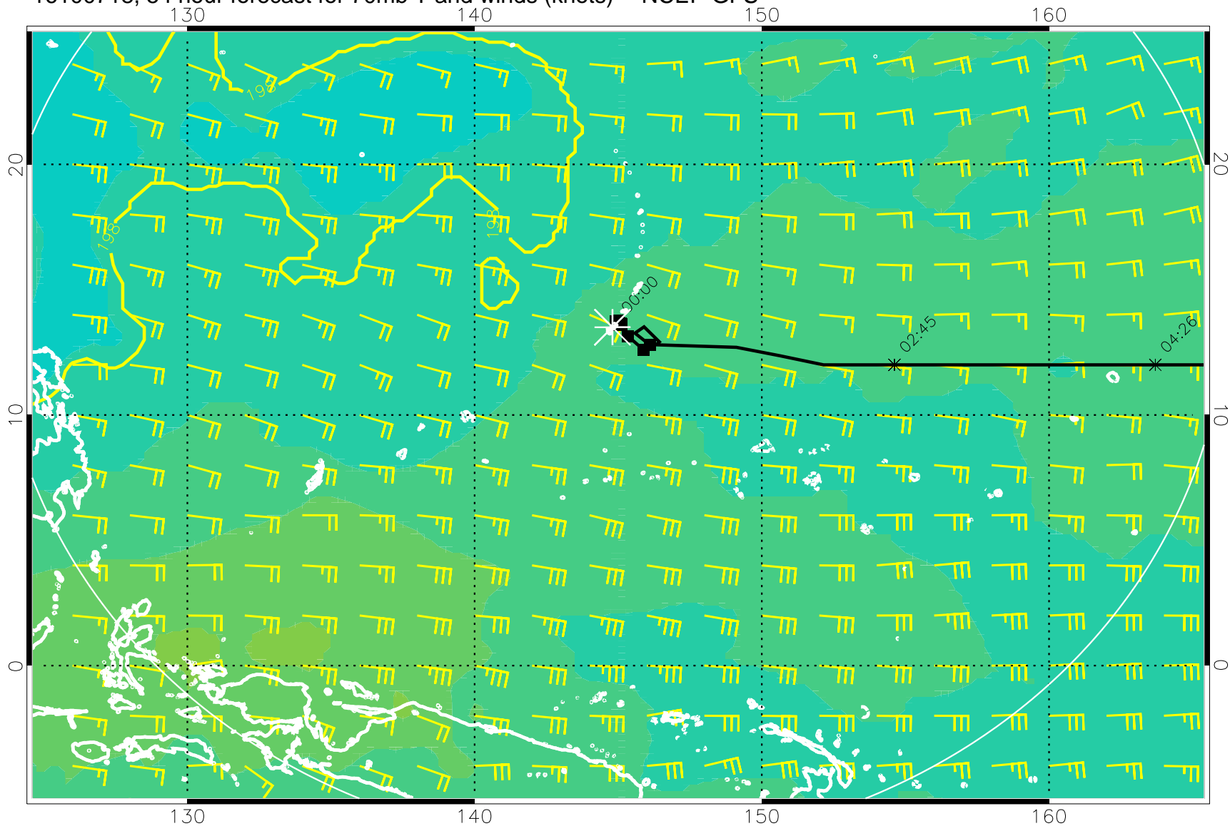
16100718, 54 hour forecast for 70mb T and winds (knots) -- NCEP GFS
