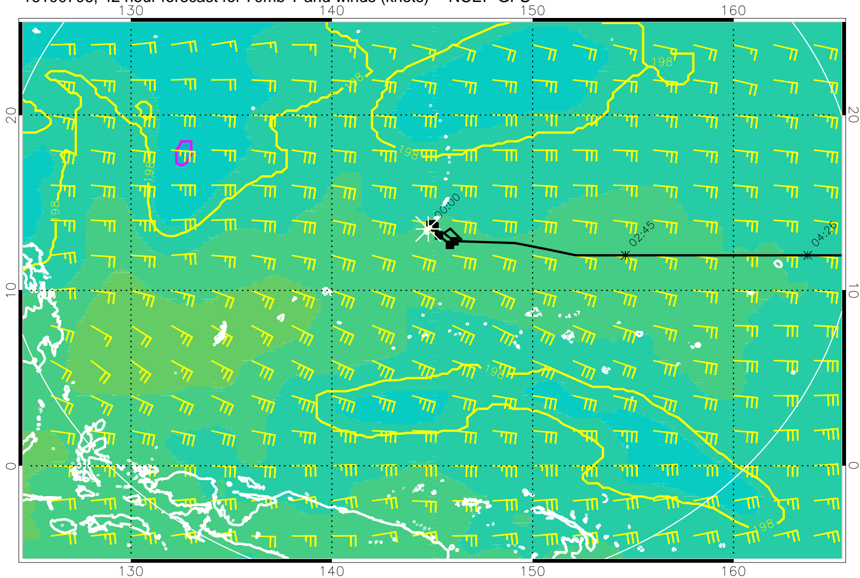
16100706, 42 hour forecast for 70mb T and winds (knots) -- NCEP GFS
