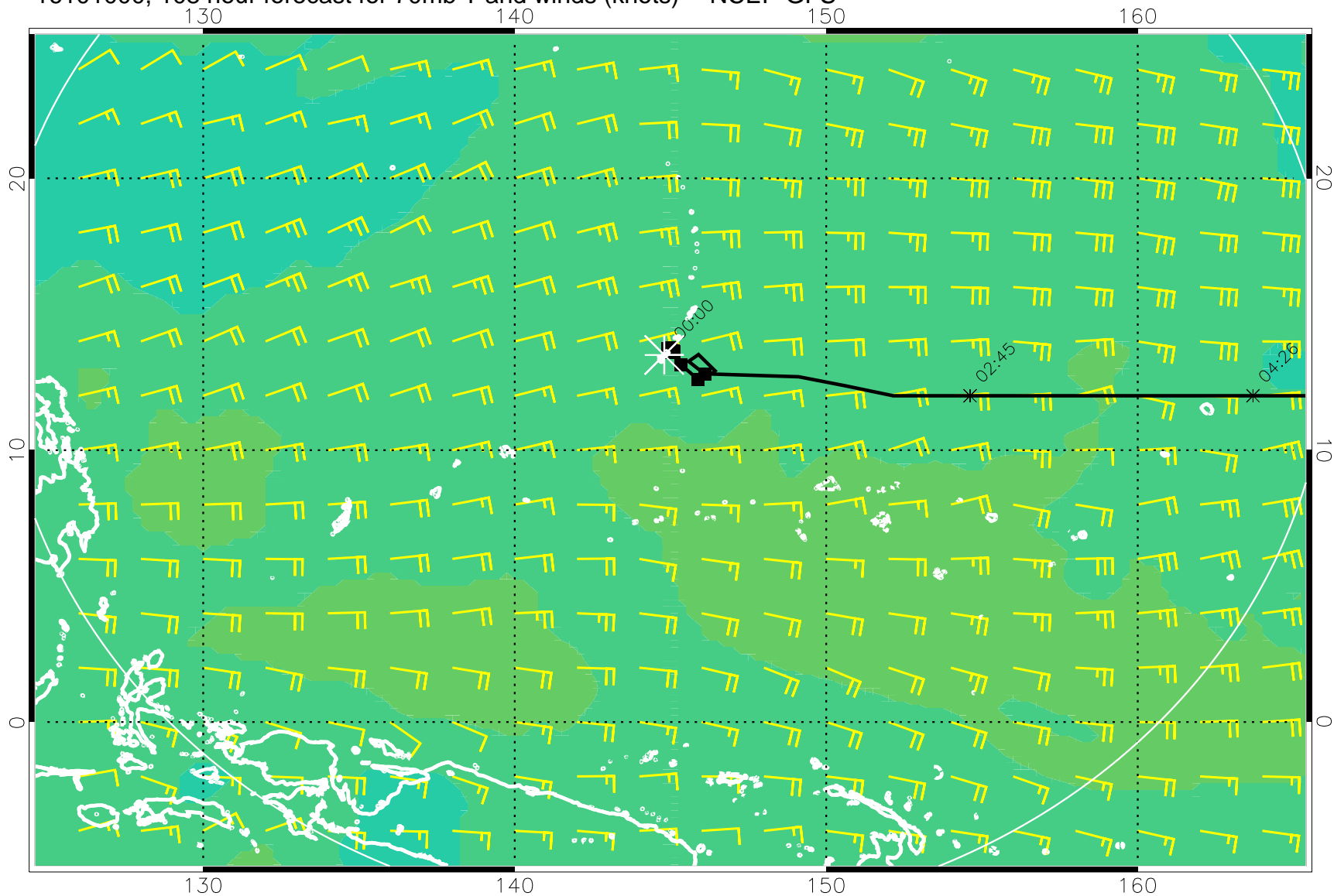
16101000, 108 hour forecast for 70mb T and winds (knots) -- NCEP GFS
