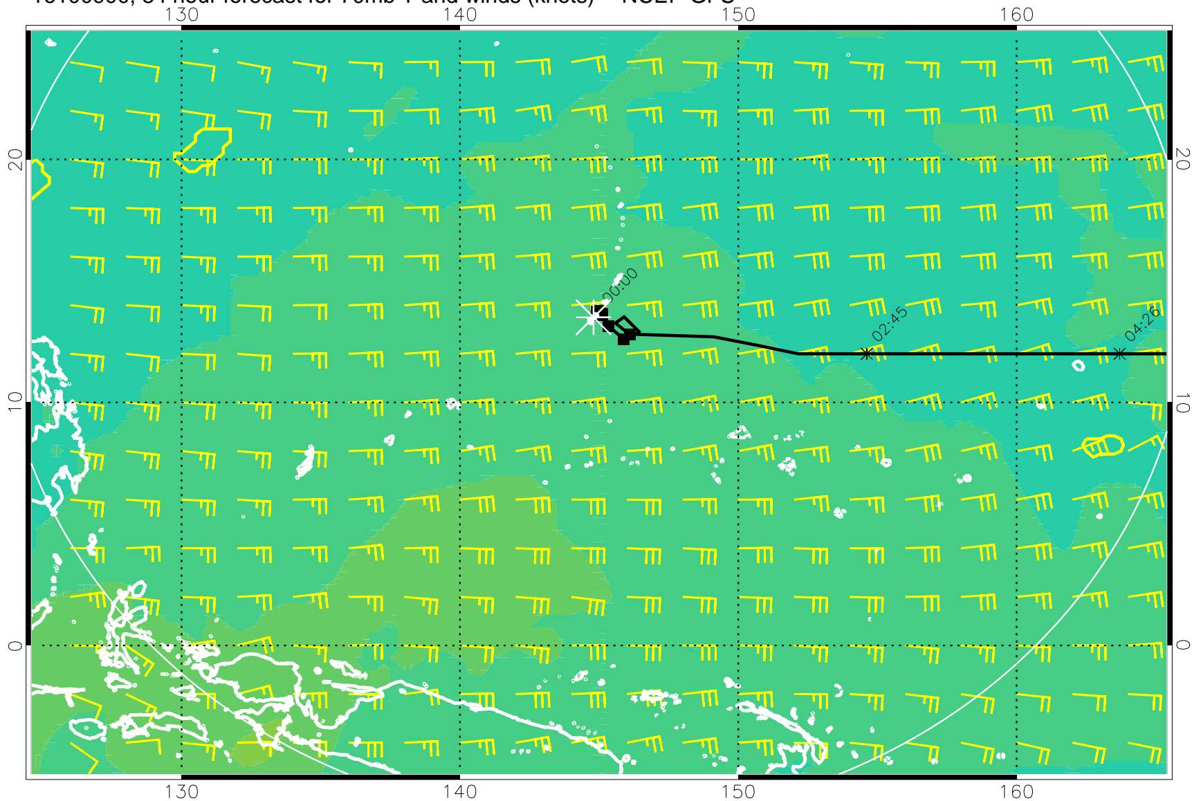
16100900, 84 hour forecast for 70mb T and winds (knots) -- NCEP GFS
