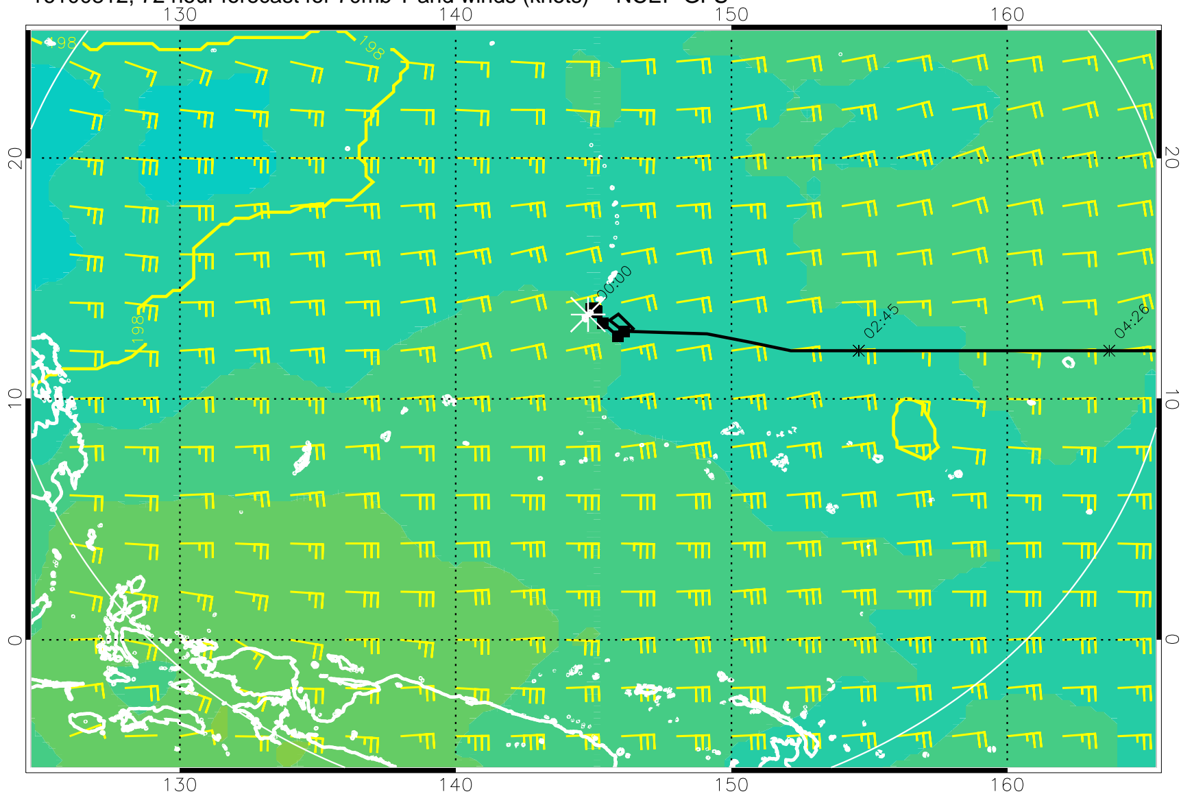
16100812, 72 hour forecast for 70mb T and winds (knots) -- NCEP GFS
