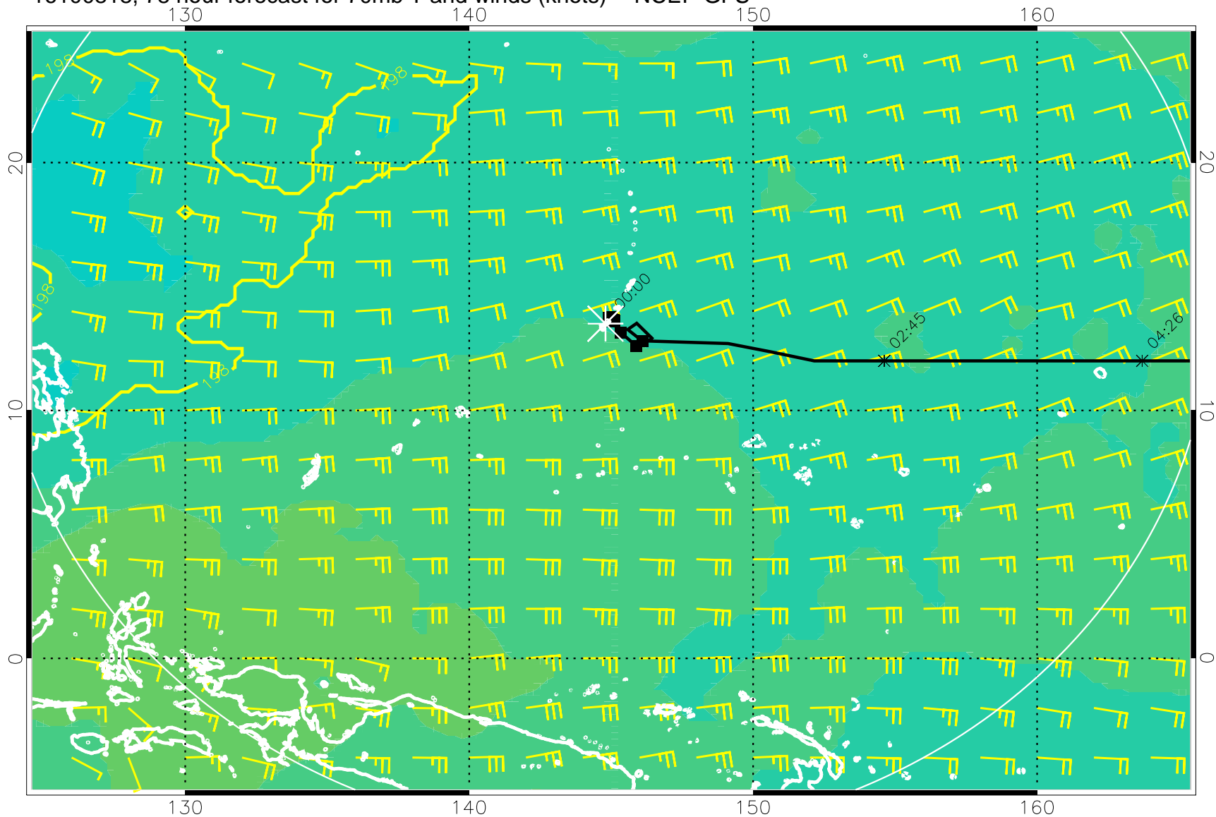
16100818, 78 hour forecast for 70mb T and winds (knots) -- NCEP GFS
