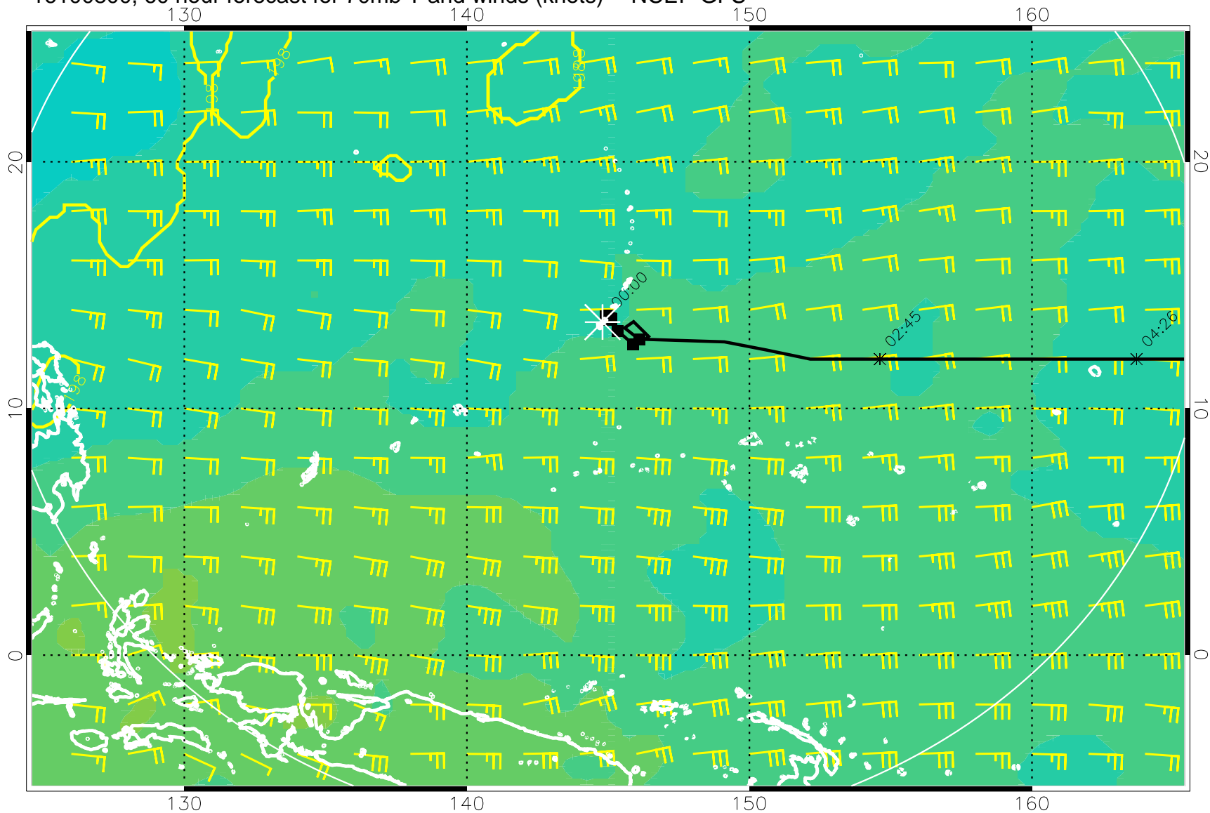
16100800, 60 hour forecast for 70mb T and winds (knots) -- NCEP GFS
