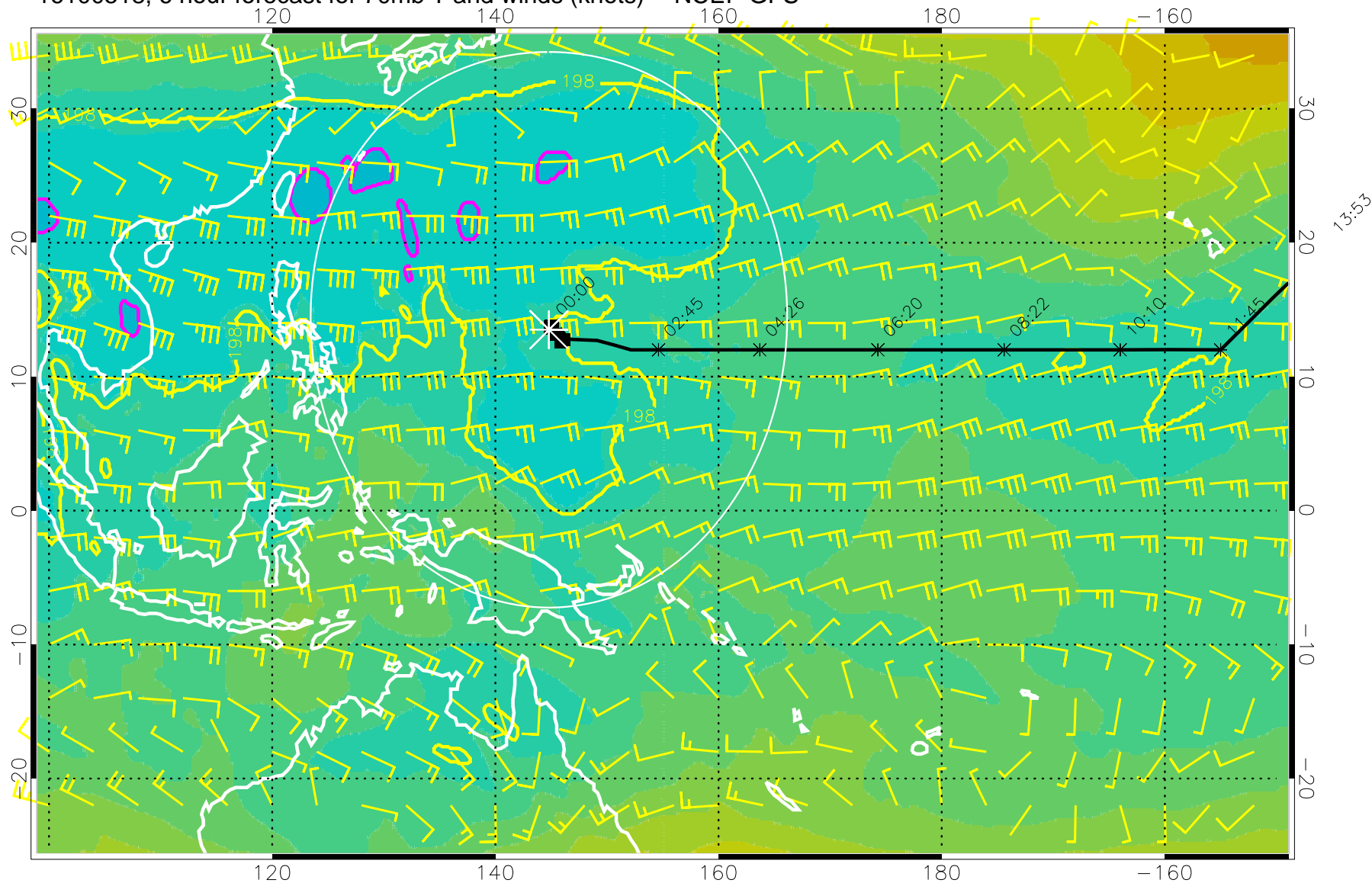
16100518, 6 hour forecast for 70mb T and winds (knots) -- NCEP GFS
