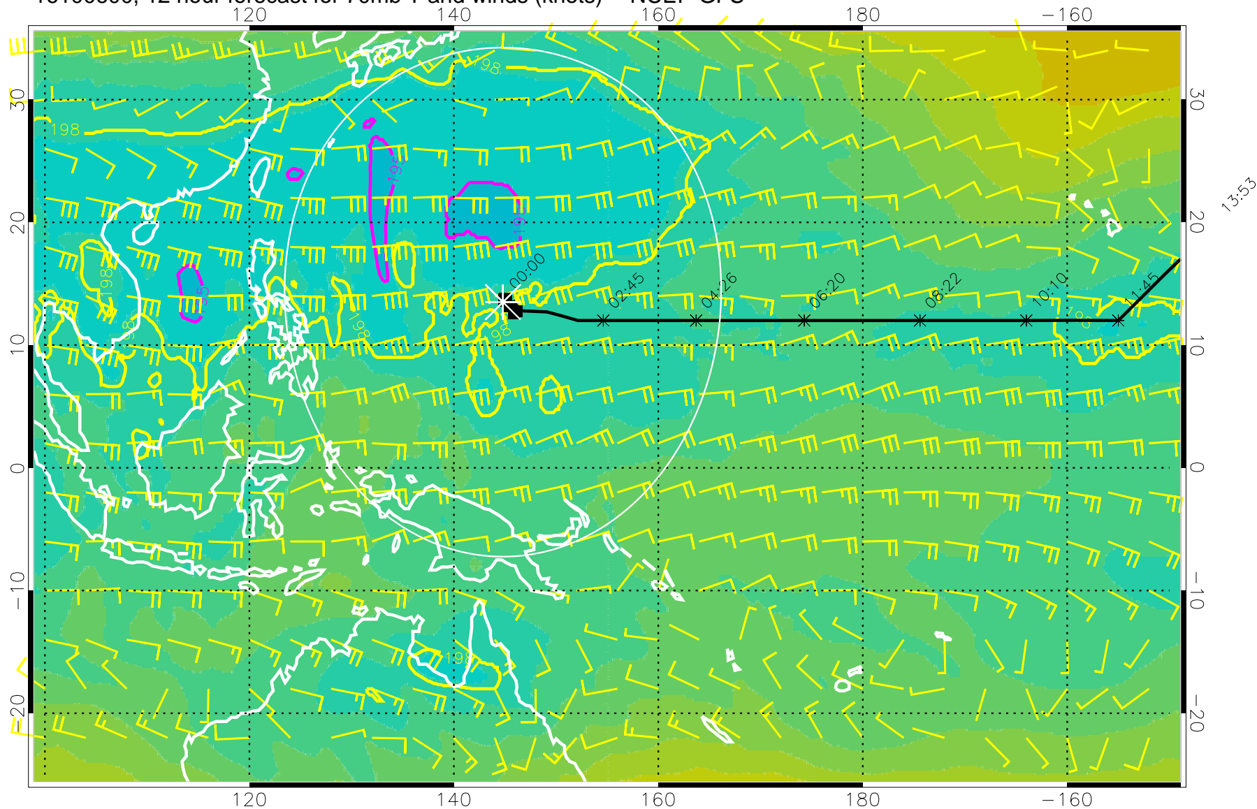
16100600, 12 hour forecast for 70mb T and winds (knots) -- NCEP GFS
