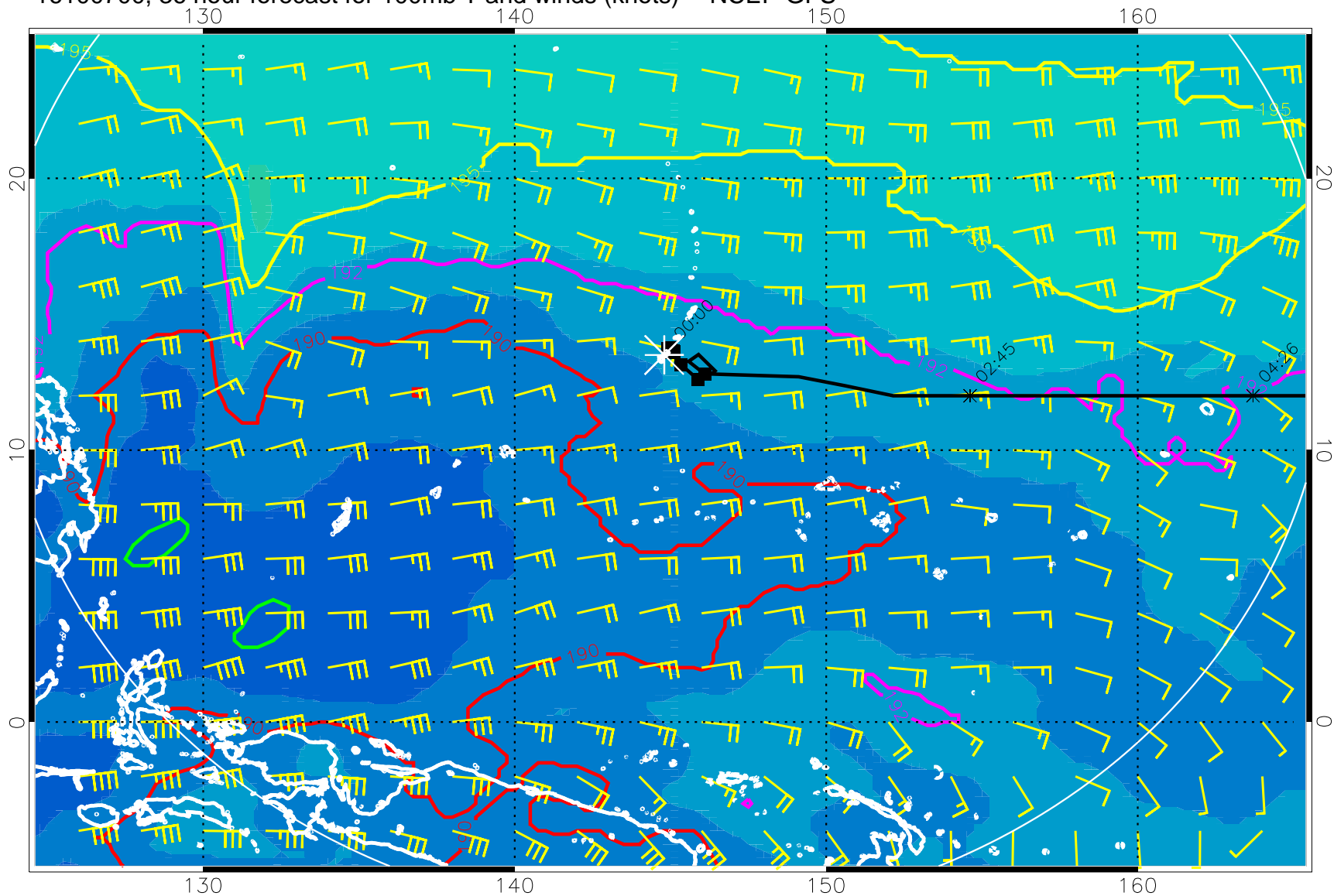
16100700, 36 hour forecast for 100mb T and winds (knots) -- NCEP GFS
