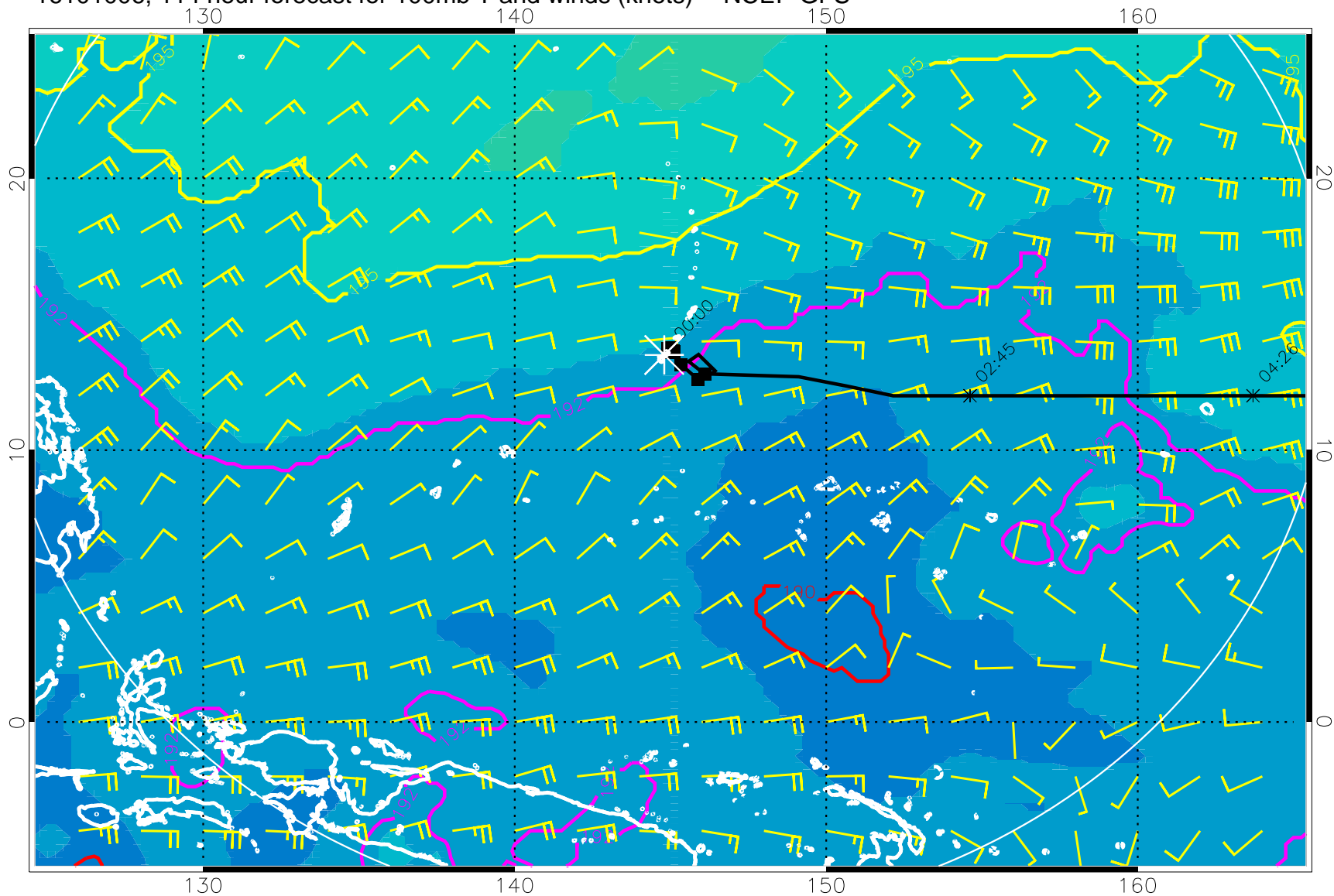
16101006, 114 hour forecast for 100mb T and winds (knots) -- NCEP GFS
