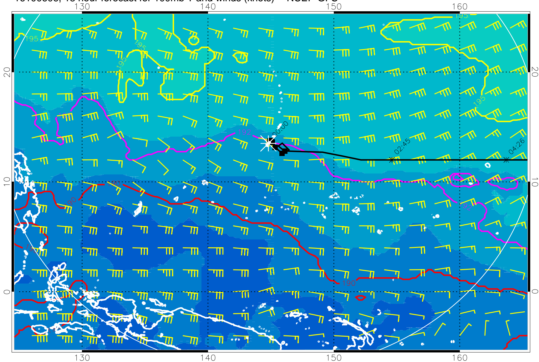
16100606, 18 hour forecast for 100mb T and winds (knots) -- NCEP GFS
