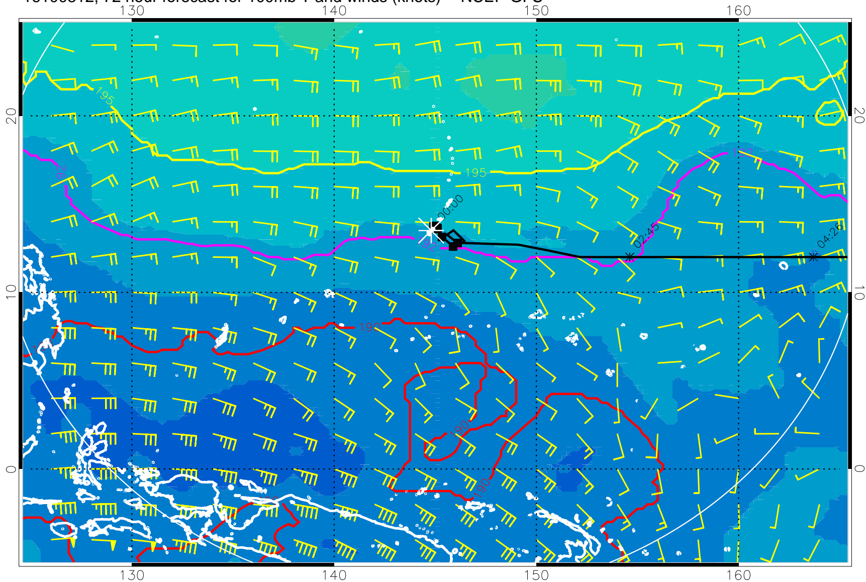
16100812, 72 hour forecast for 100mb T and winds (knots) -- NCEP GFS
