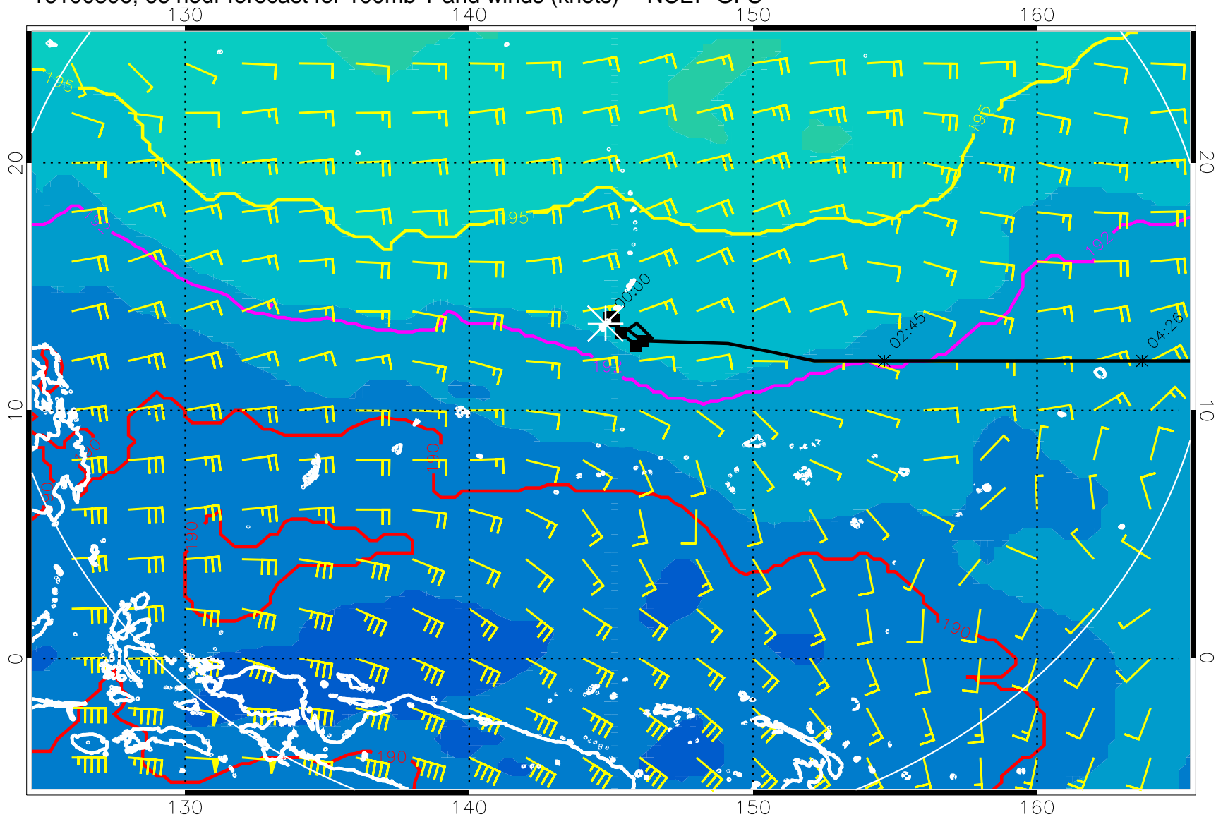
16100806, 66 hour forecast for 100mb T and winds (knots) -- NCEP GFS
