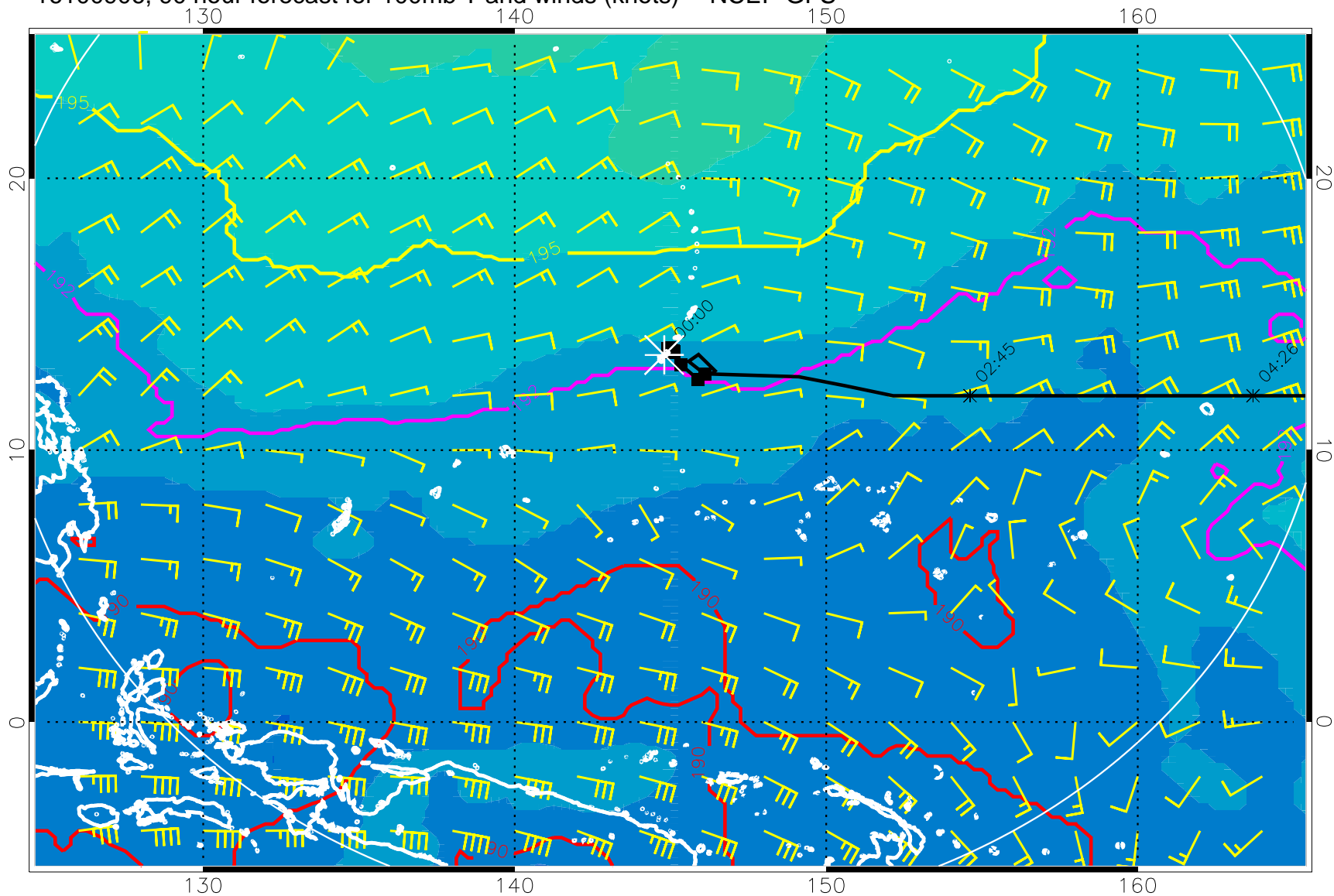
16100906, 90 hour forecast for 100mb T and winds (knots) -- NCEP GFS
