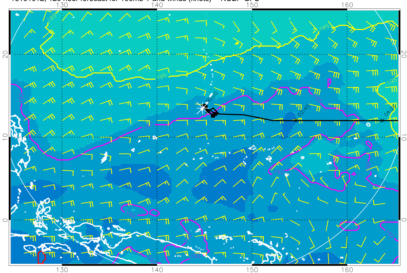
16101012, 120 hour forecast for 100mb T and winds (knots) -- NCEP GFS
