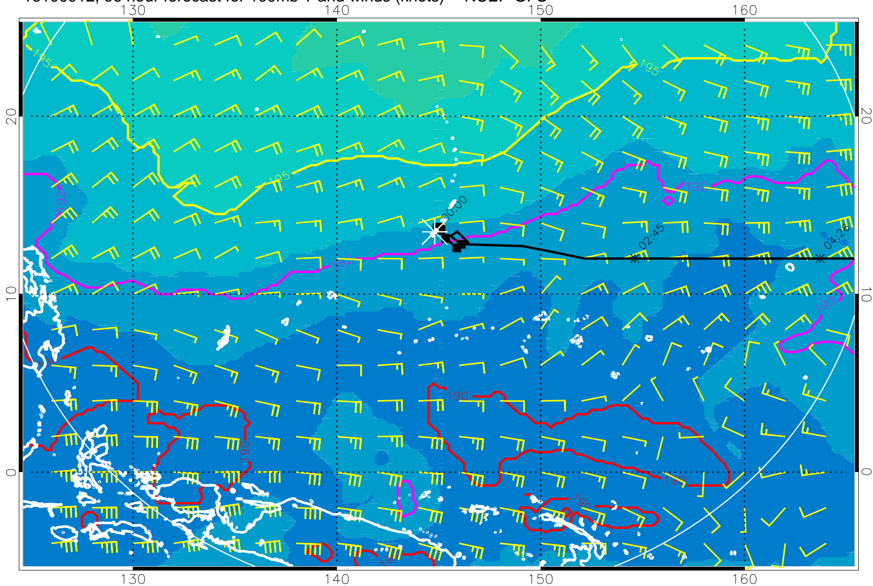
16100912, 96 hour forecast for 100mb T and winds (knots) -- NCEP GFS
