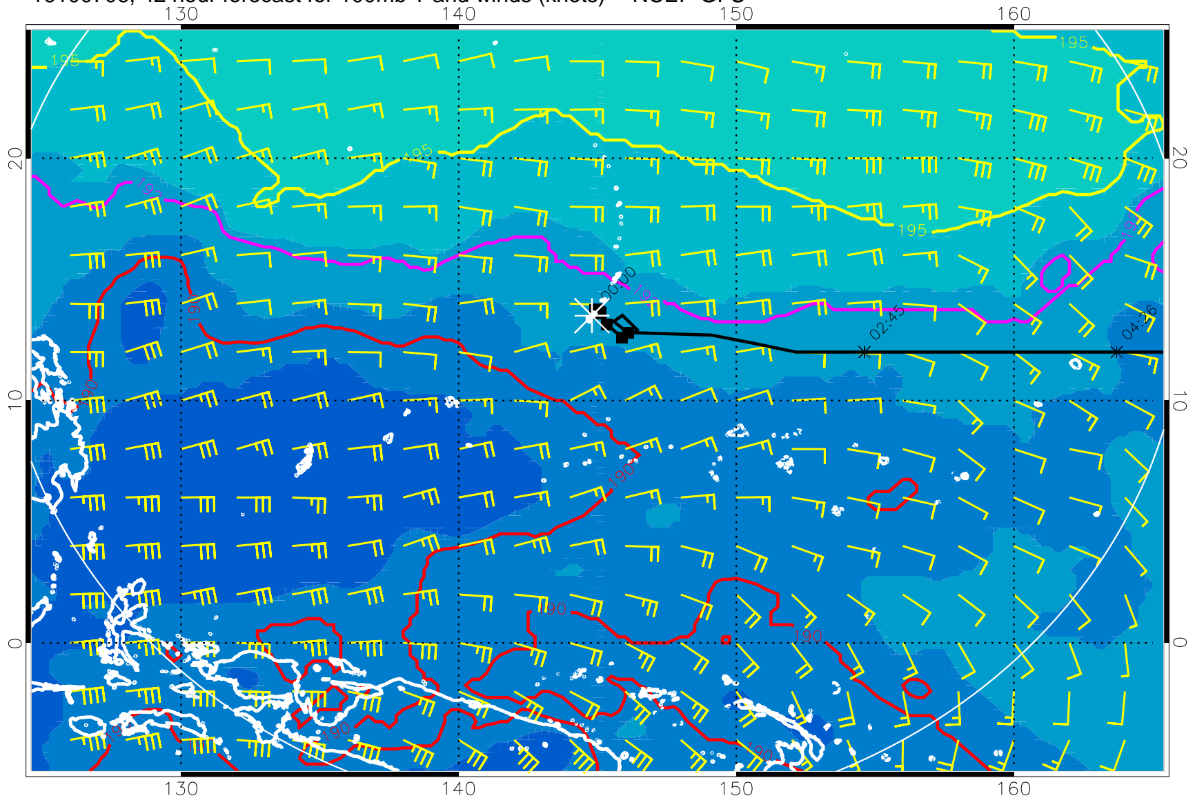
16100706, 42 hour forecast for 100mb T and winds (knots) -- NCEP GFS
