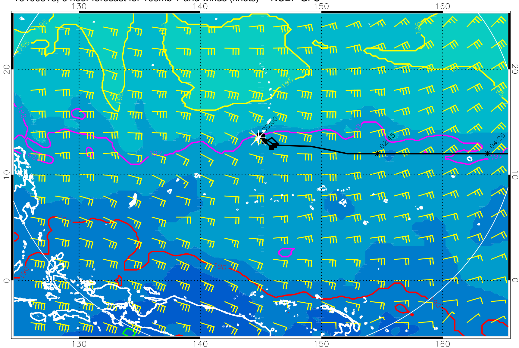
16100518, 6 hour forecast for 100mb T and winds (knots) -- NCEP GFS
