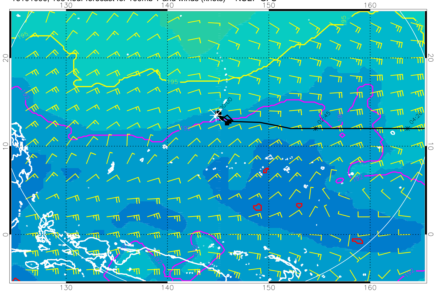
16101000, 108 hour forecast for 100mb T and winds (knots) -- NCEP GFS
