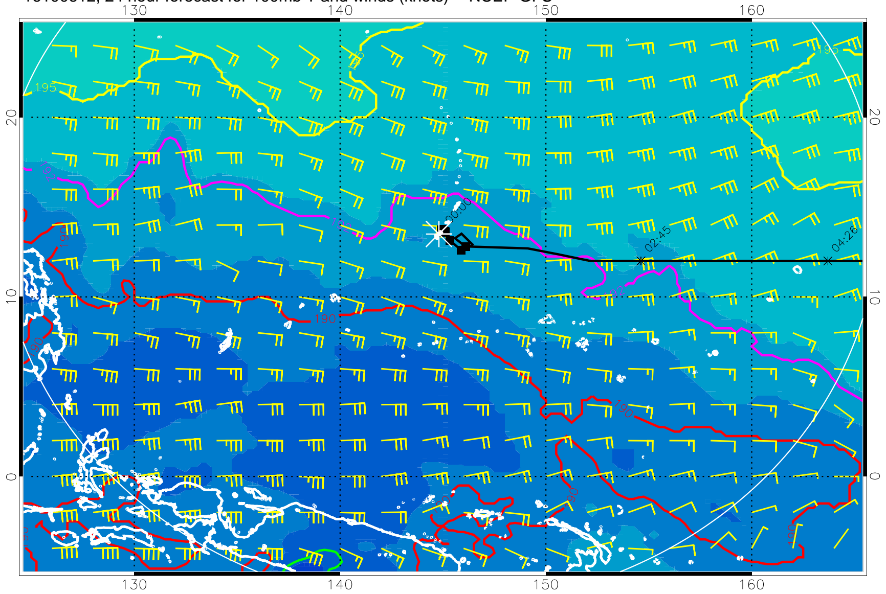
16100612, 24 hour forecast for 100mb T and winds (knots) -- NCEP GFS
