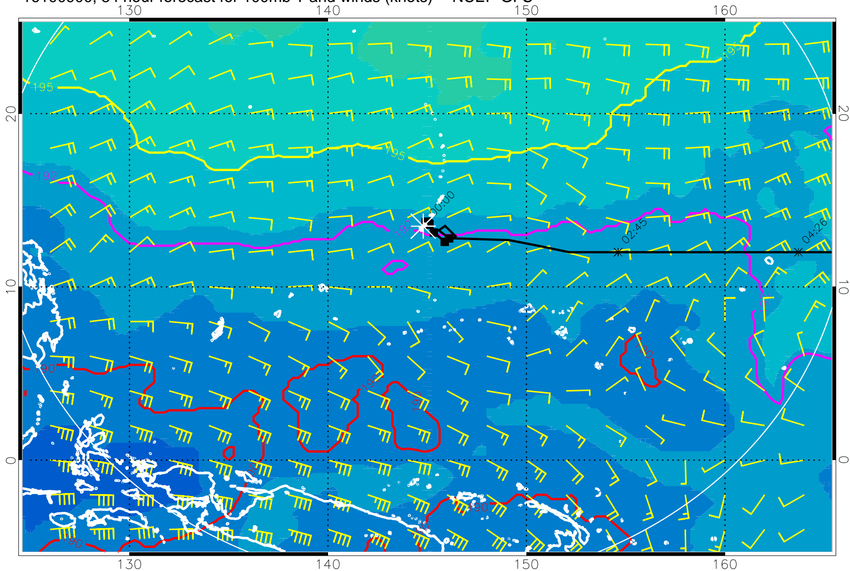
16100900, 84 hour forecast for 100mb T and winds (knots) -- NCEP GFS
