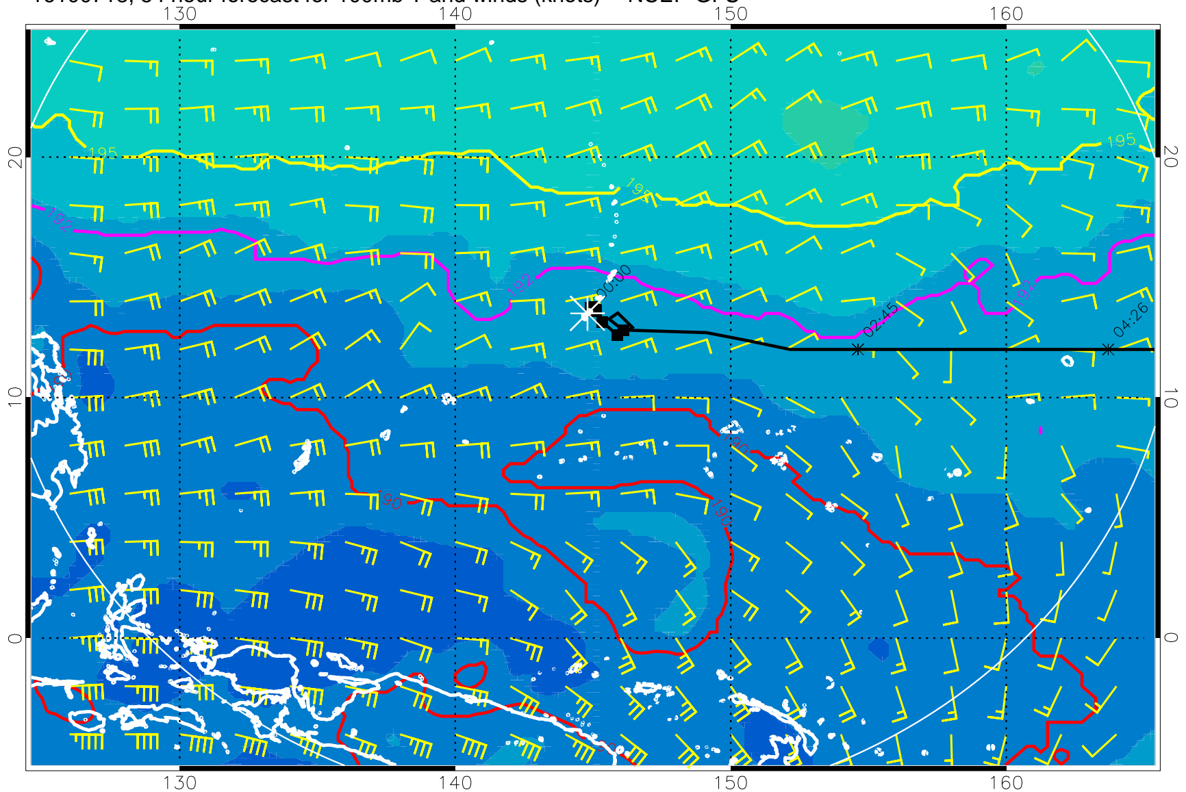
16100718, 54 hour forecast for 100mb T and winds (knots) -- NCEP GFS
