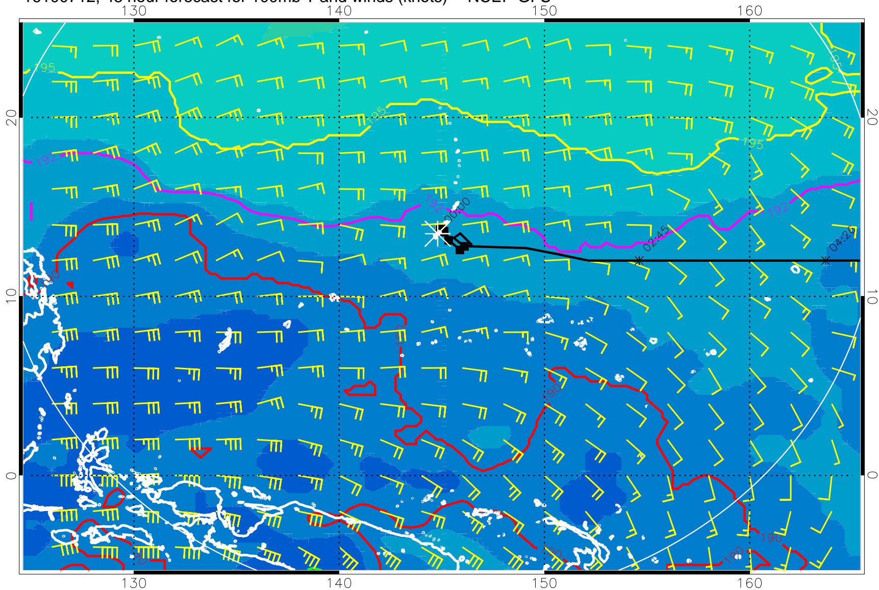
16100712, 48 hour forecast for 100mb T and winds (knots) -- NCEP GFS
