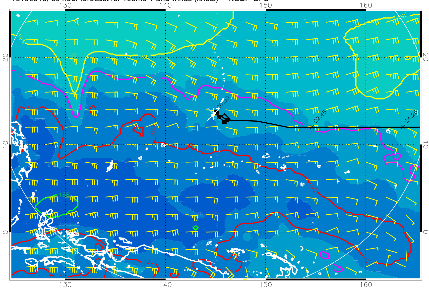
16100618, 30 hour forecast for 100mb T and winds (knots) -- NCEP GFS
