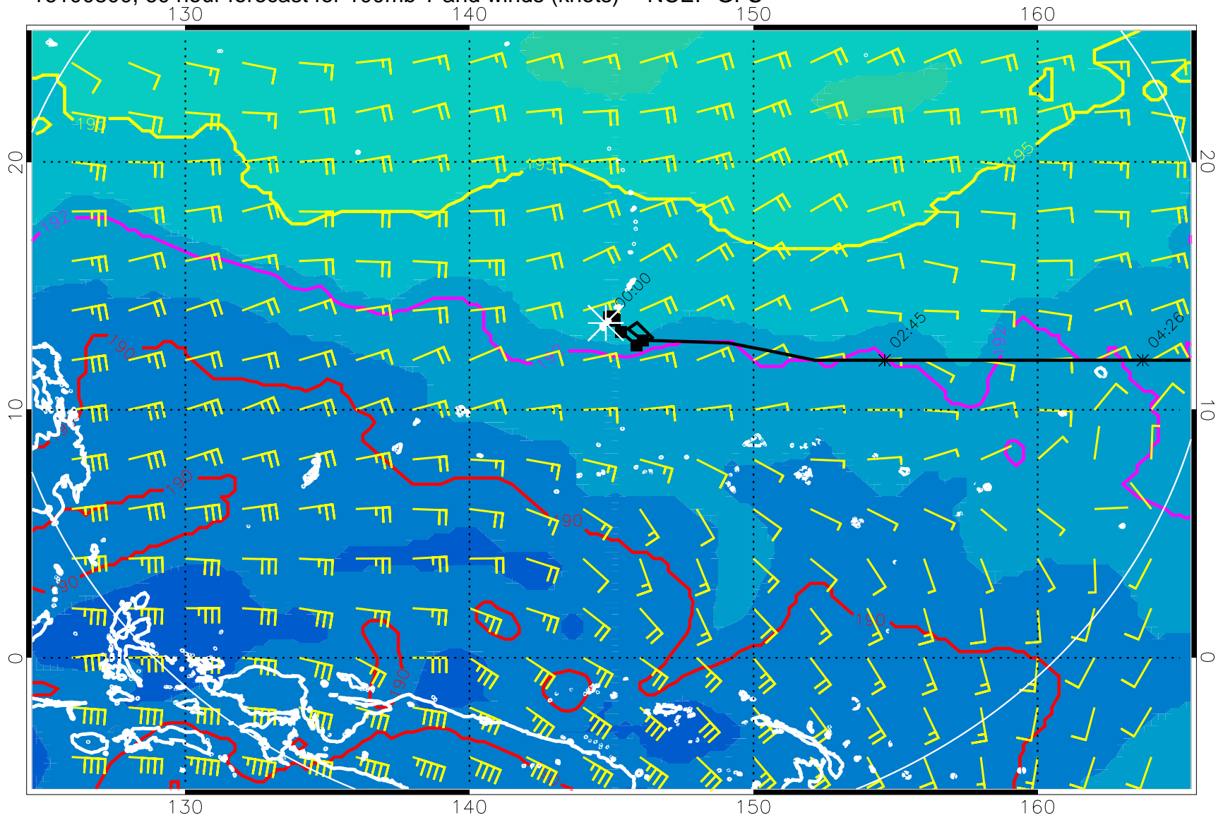
16100800, 60 hour forecast for 100mb T and winds (knots) -- NCEP GFS
