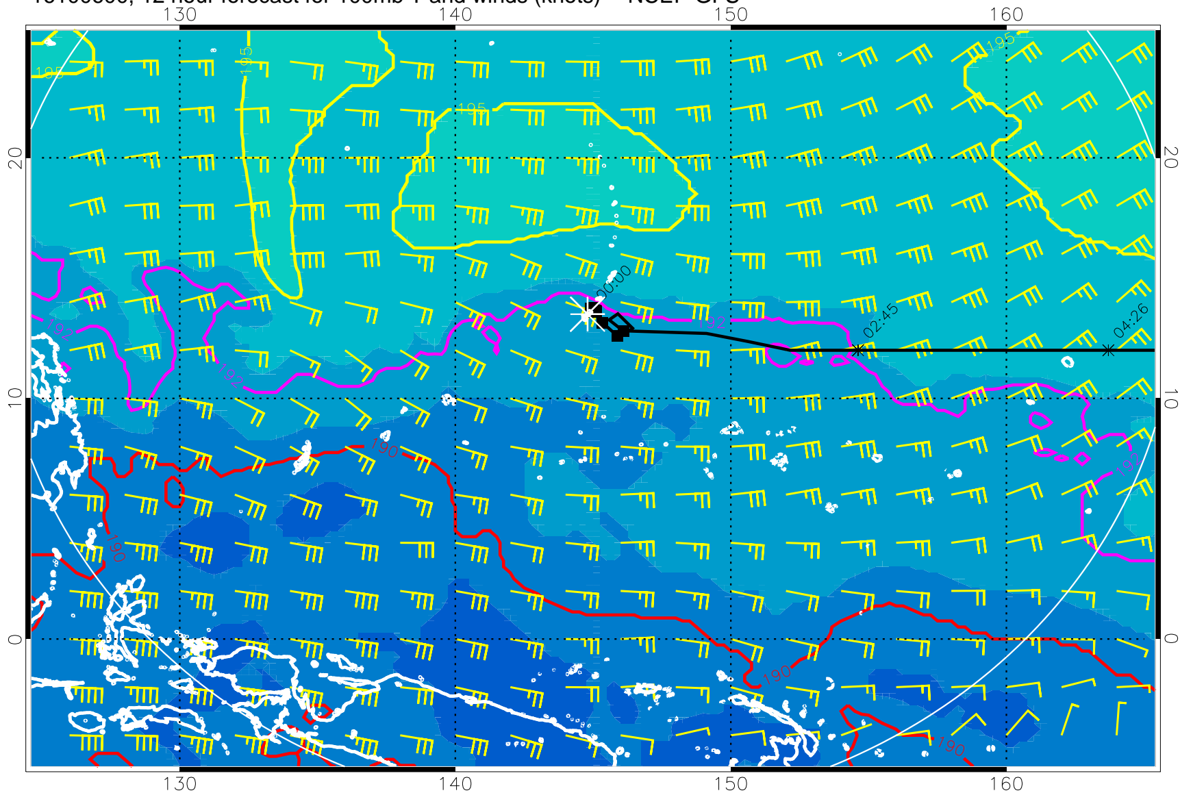
16100600, 12 hour forecast for 100mb T and winds (knots) -- NCEP GFS
