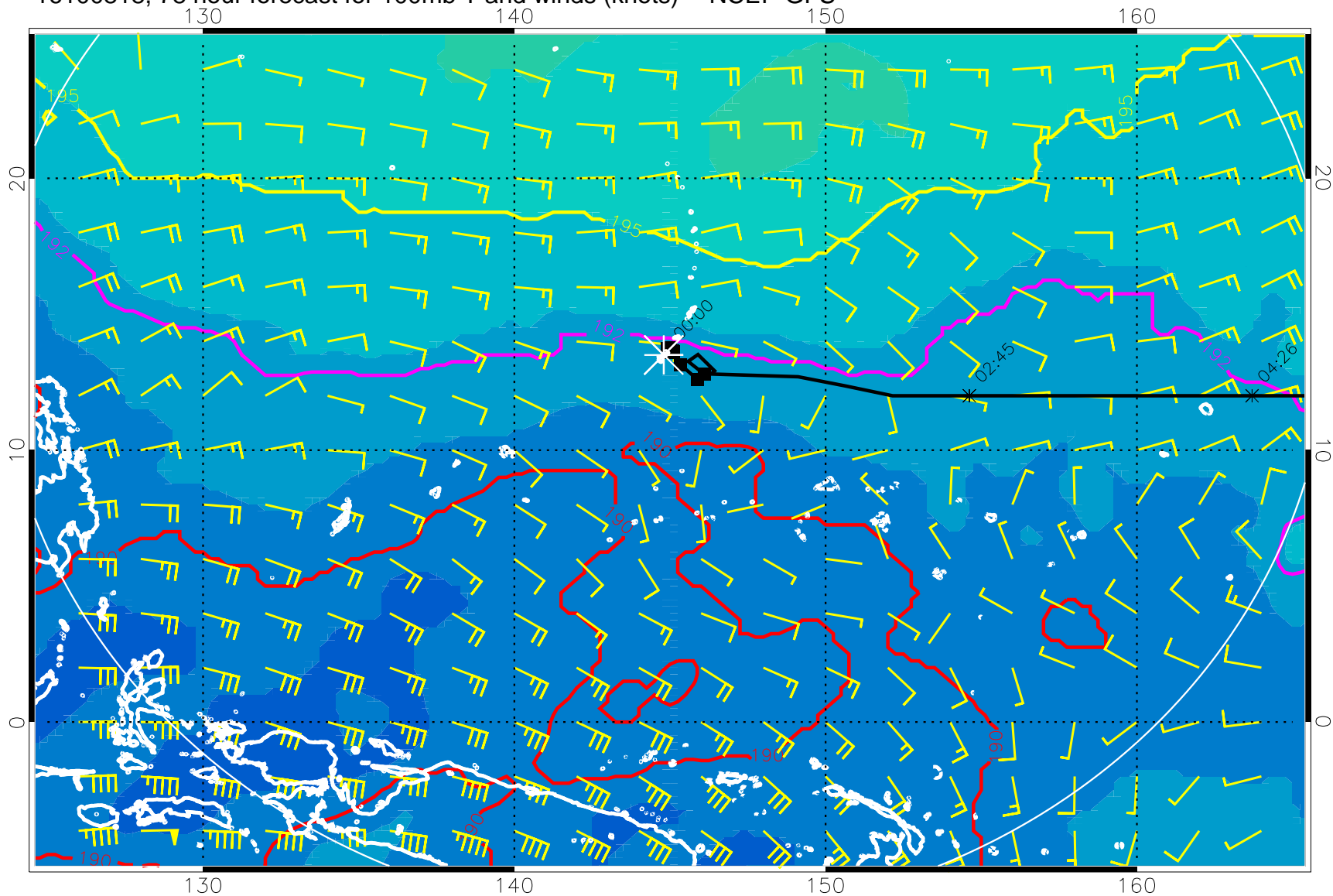
16100818, 78 hour forecast for 100mb T and winds (knots) -- NCEP GFS
