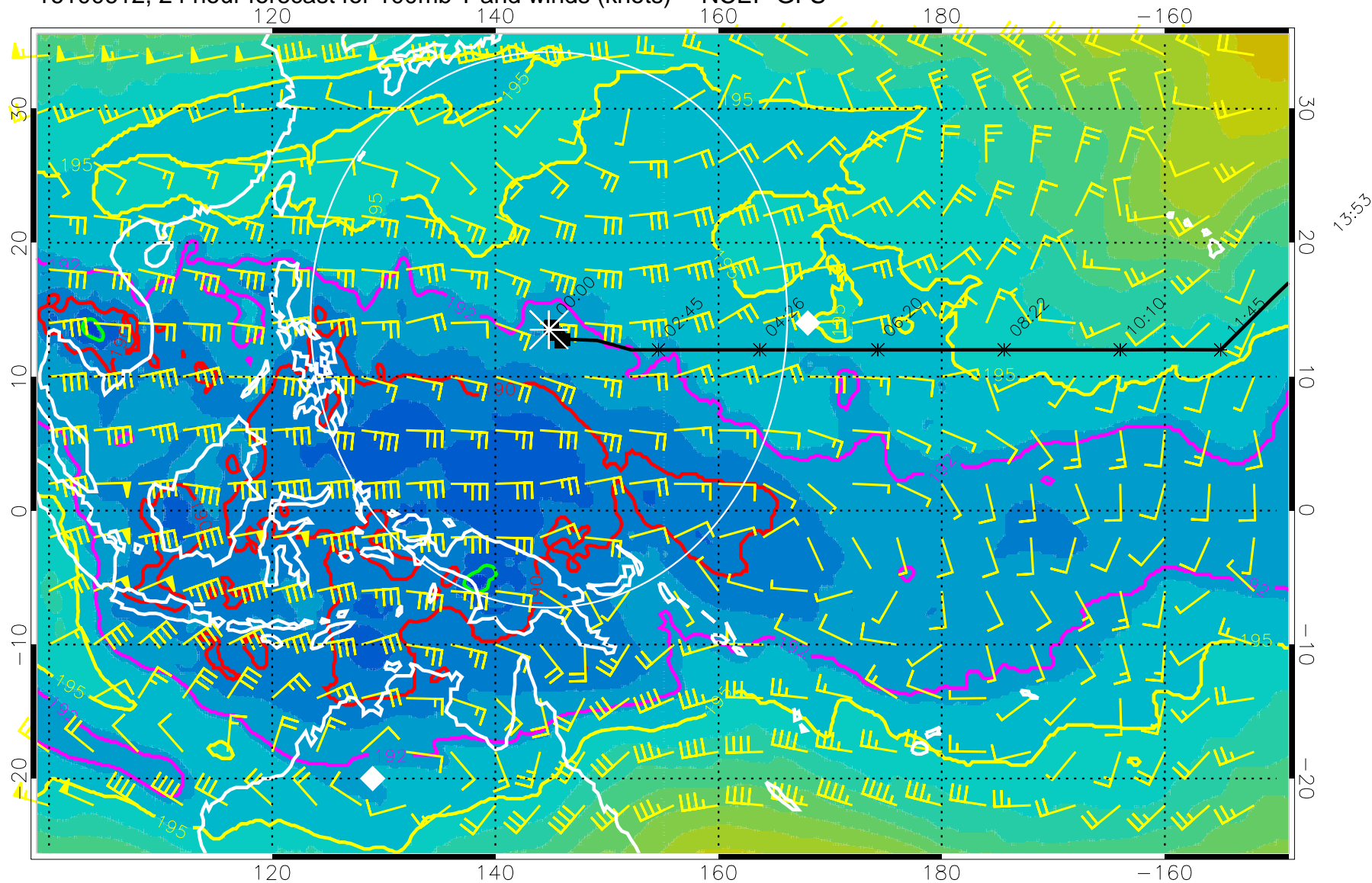
16100612, 24 hour forecast for 100mb T and winds (knots) -- NCEP GFS
