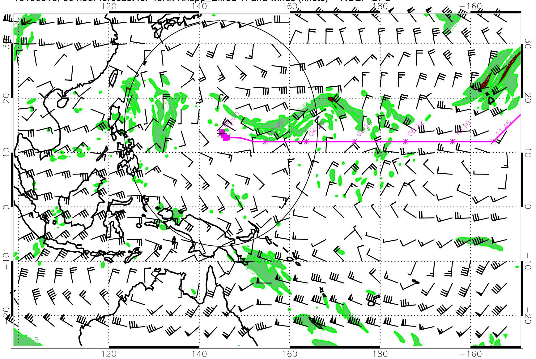
16100618, 30 hour forecast for 45Kft Knapp_Ellrod TI and winds (knots) -- NCEP GFS
