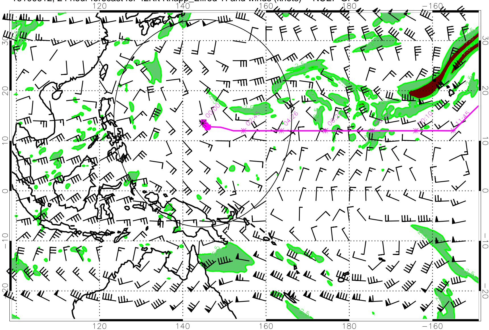
16100612, 24 hour forecast for 42Kft Knapp_Ellrod TI and winds (knots) -- NCEP GFS
