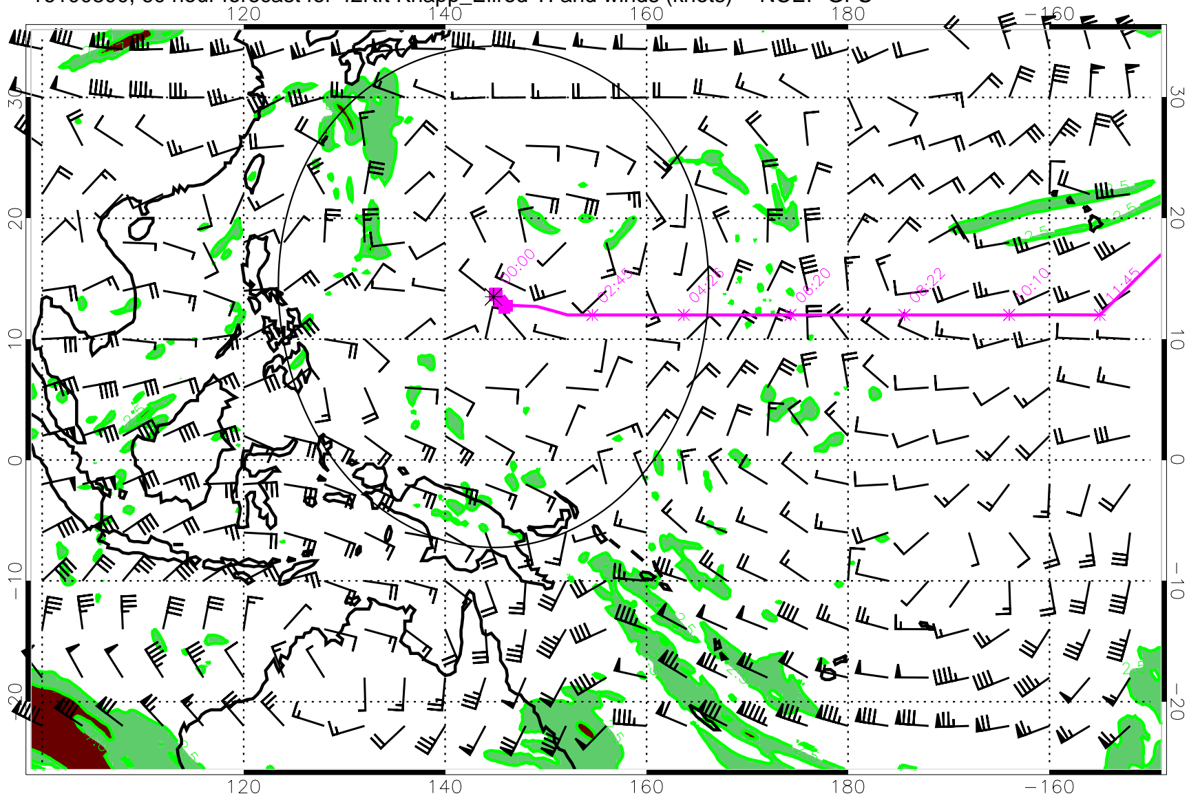
16100800, 60 hour forecast for 42Kft Knapp_Ellrod TI and winds (knots) -- NCEP GFS
