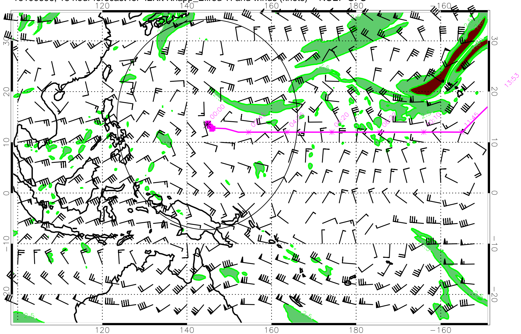
16100606, 18 hour forecast for 42Kft Knapp_Ellrod TI and winds (knots) -- NCEP GFS
