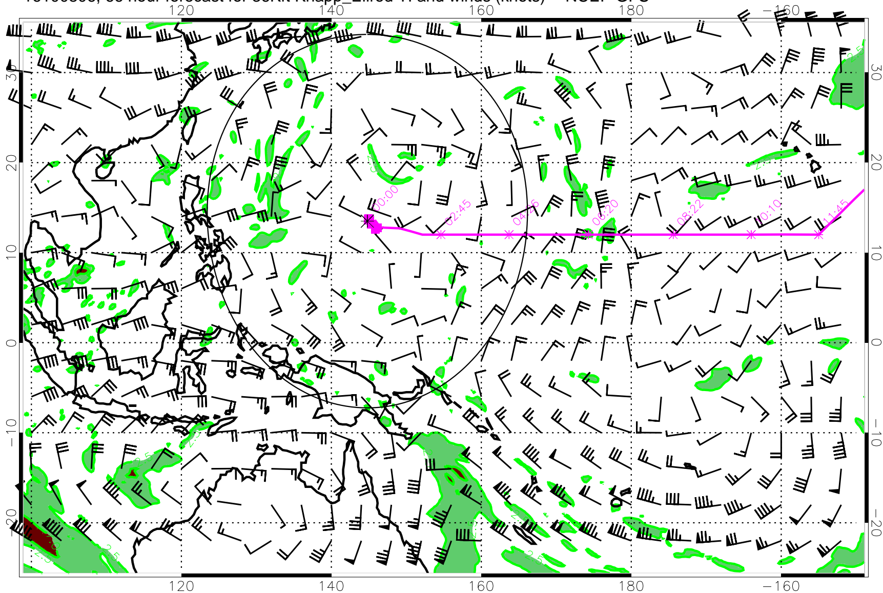
16100806, 66 hour forecast for 36Kft Knapp_Ellrod TI and winds (knots) -- NCEP GFS
