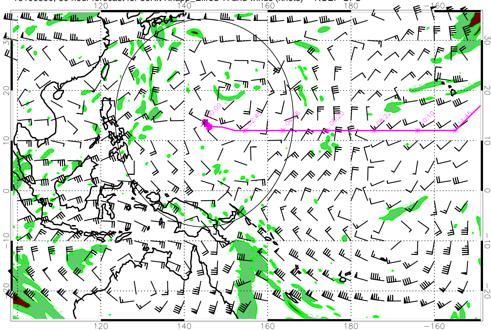
16100800, 60 hour forecast for 36Kft Knapp_Ellrod TI and winds (knots) -- NCEP GFS
