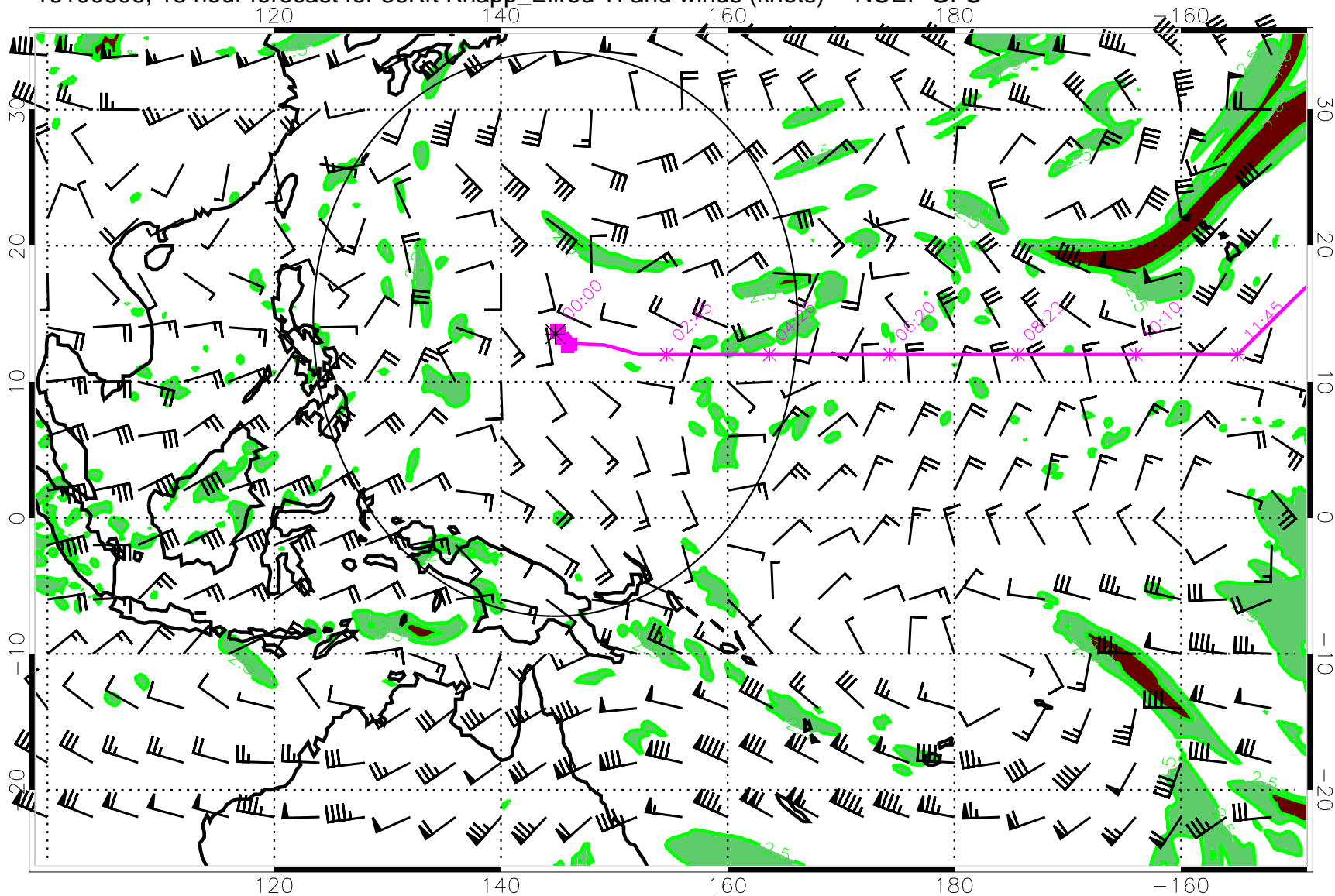
16100606, 18 hour forecast for 36Kft Knapp_Ellrod TI and winds (knots) -- NCEP GFS
