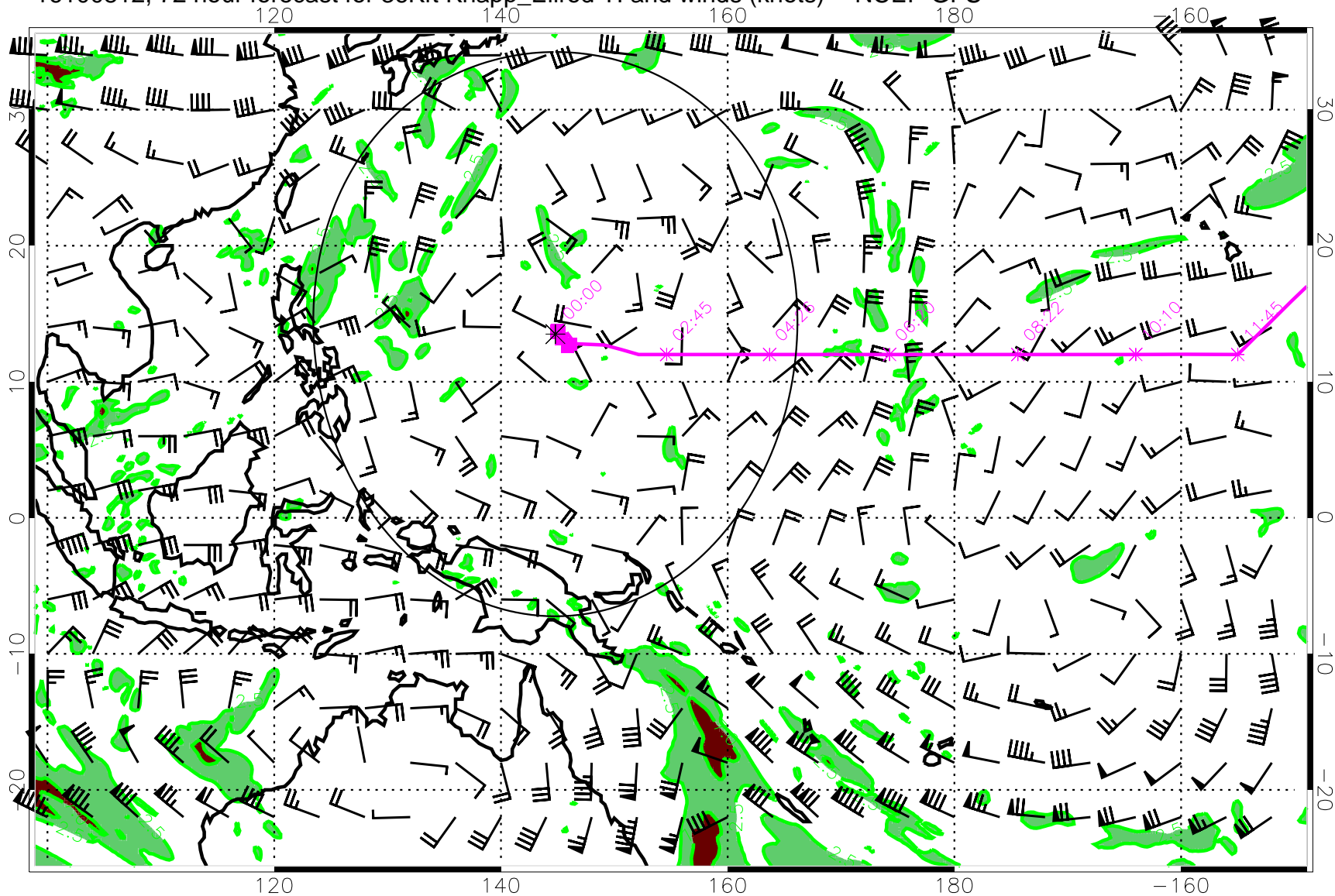
16100812, 72 hour forecast for 36Kft Knapp_Ellrod TI and winds (knots) -- NCEP GFS
