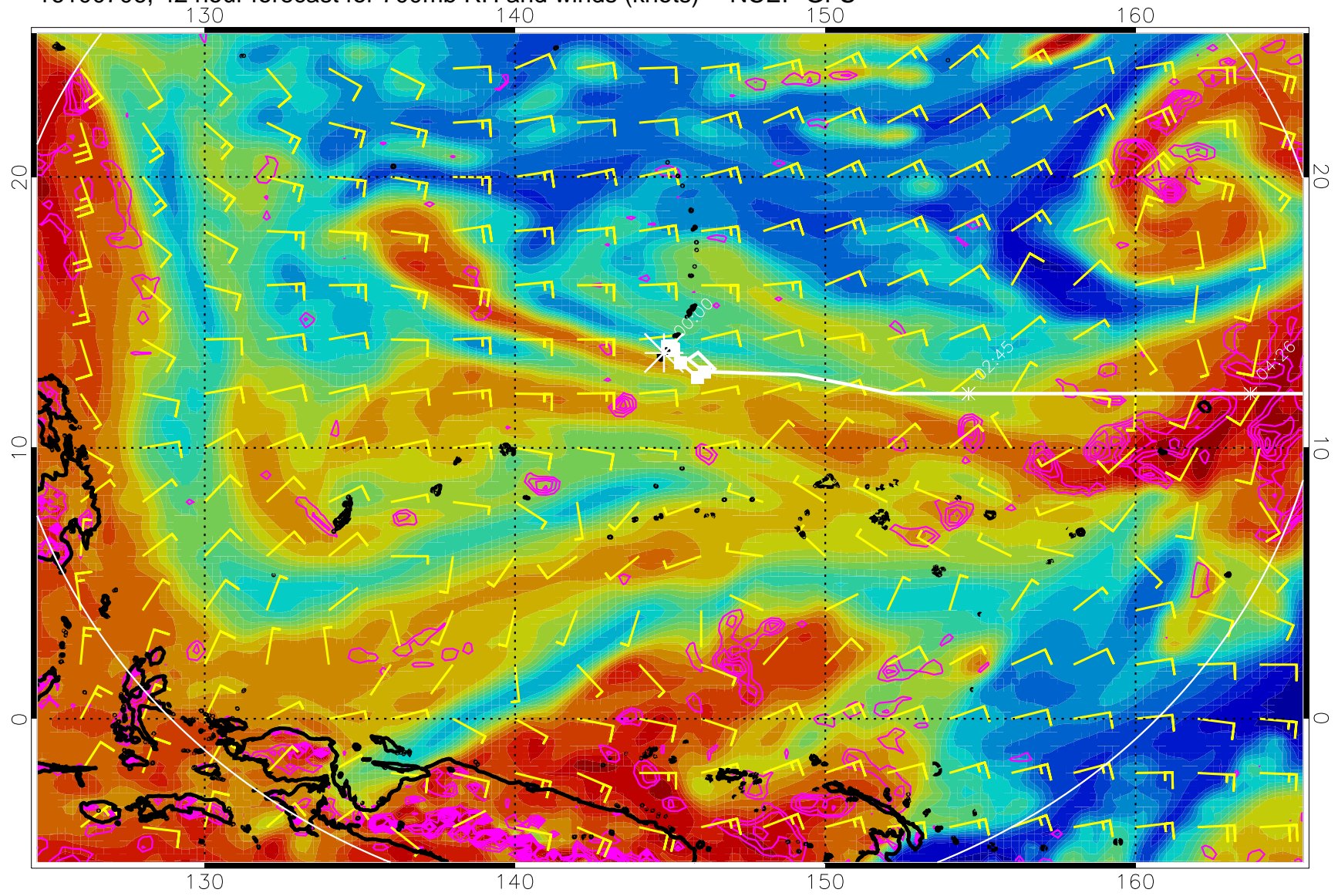
16100706, 42 hour forecast for 700mb RH and winds (knots) -- NCEP GFS
