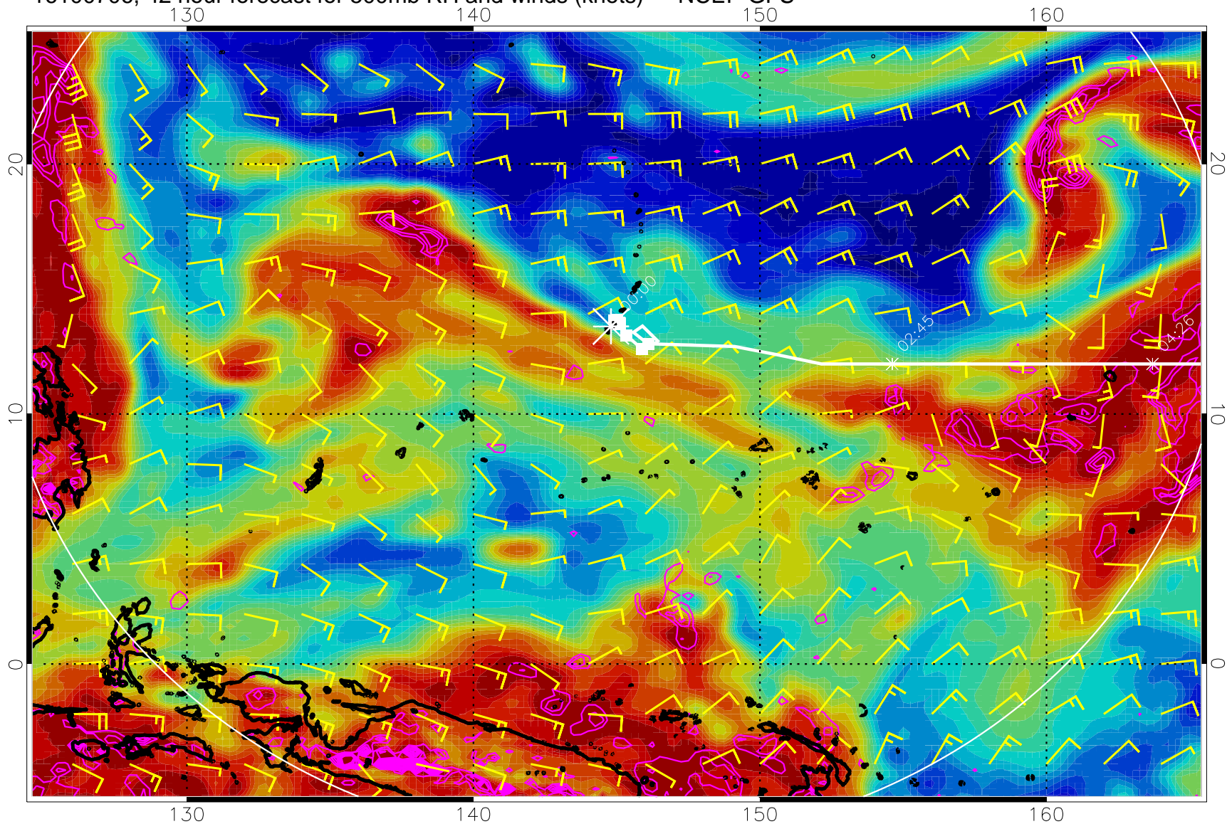
16100706, 42 hour forecast for 500mb RH and winds (knots) -- NCEP GFS
