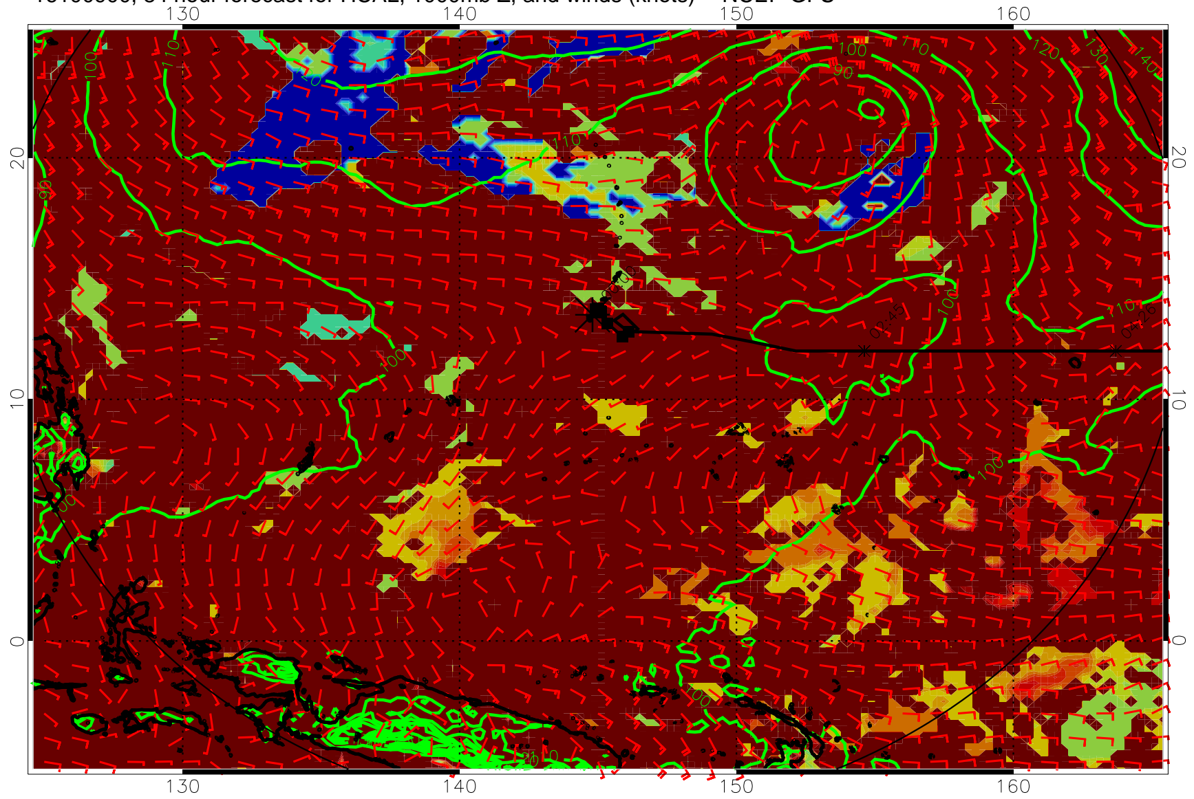
16100900, 84 hour forecast for HCAL, 1000mb Z, and winds (knots) -- NCEP GFS
