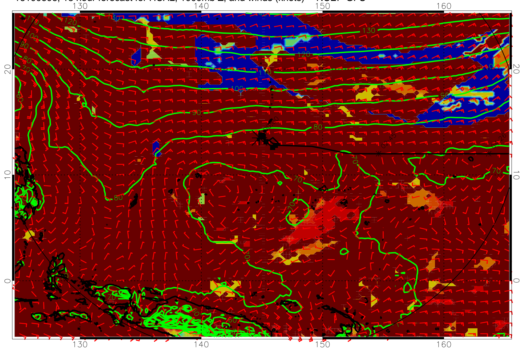
16100606, 18 hour forecast for HCAL, 1000mb Z, and winds (knots) -- NCEP GFS
