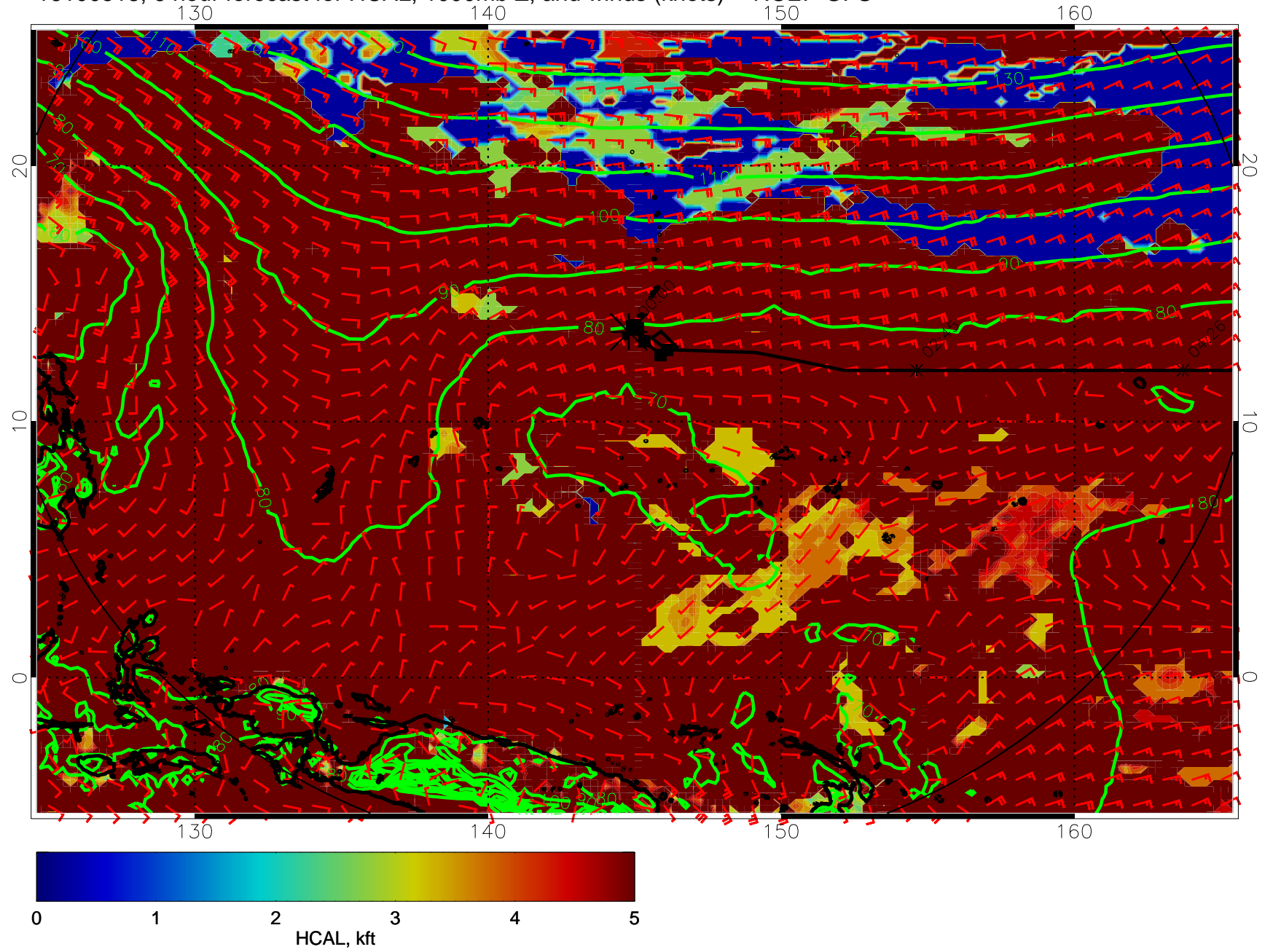
16100518, 6 hour forecast for HCAL, 1000mb Z, and winds (knots) -- NCEP GFS
