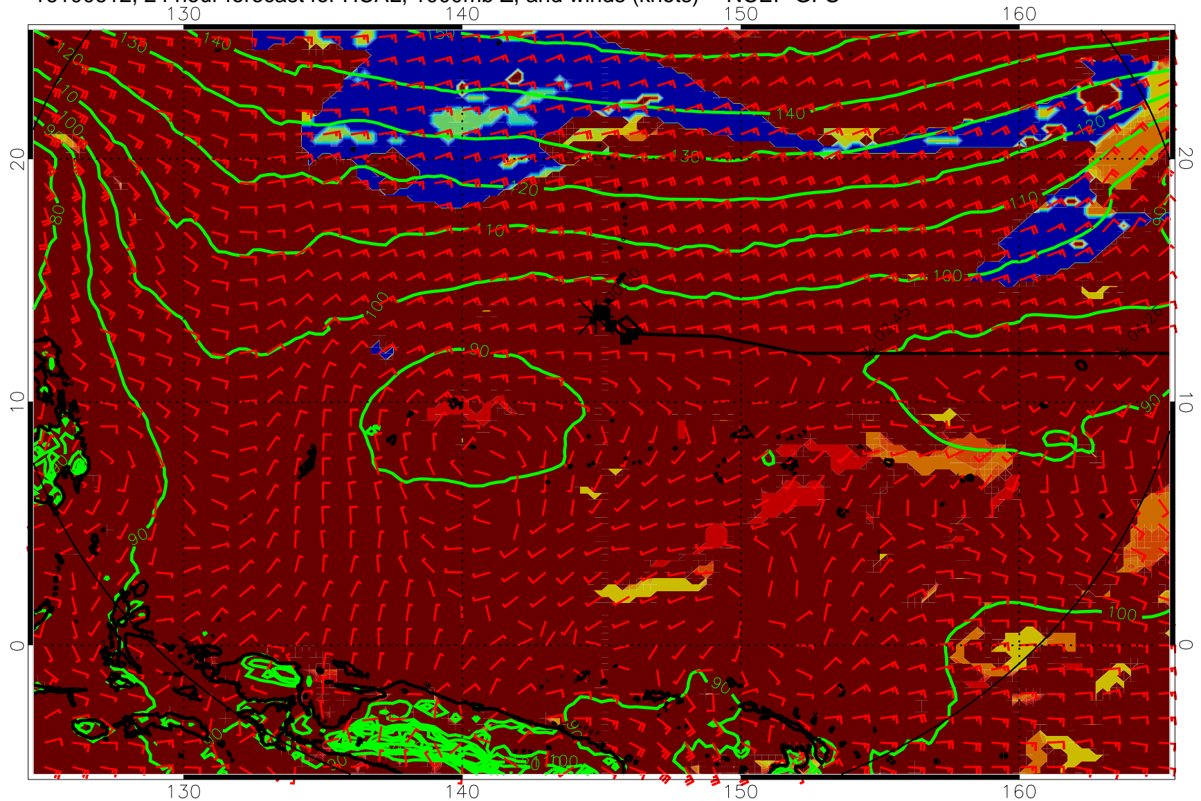
16100612, 24 hour forecast for HCAL, 1000mb Z, and winds (knots) -- NCEP GFS
