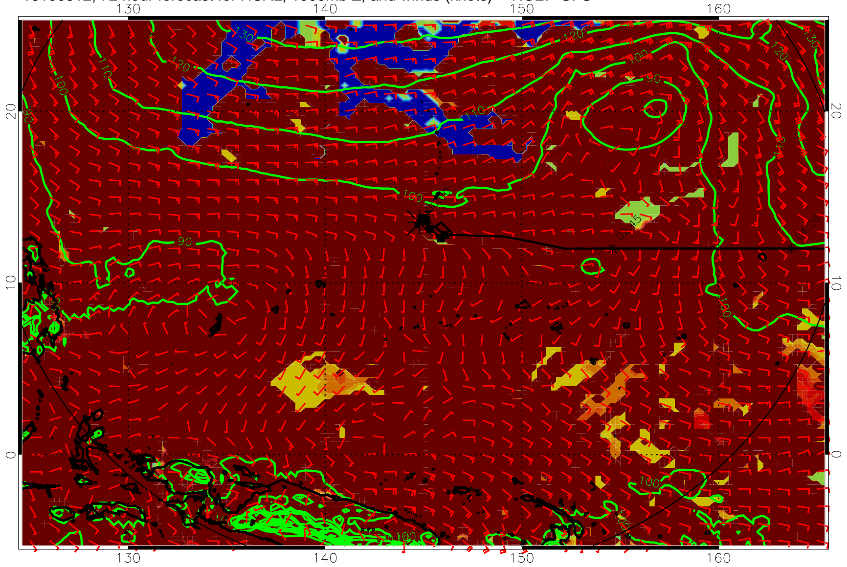
16100812, 72 hour forecast for HCAL, 1000mb Z, and winds (knots) -- NCEP GFS
