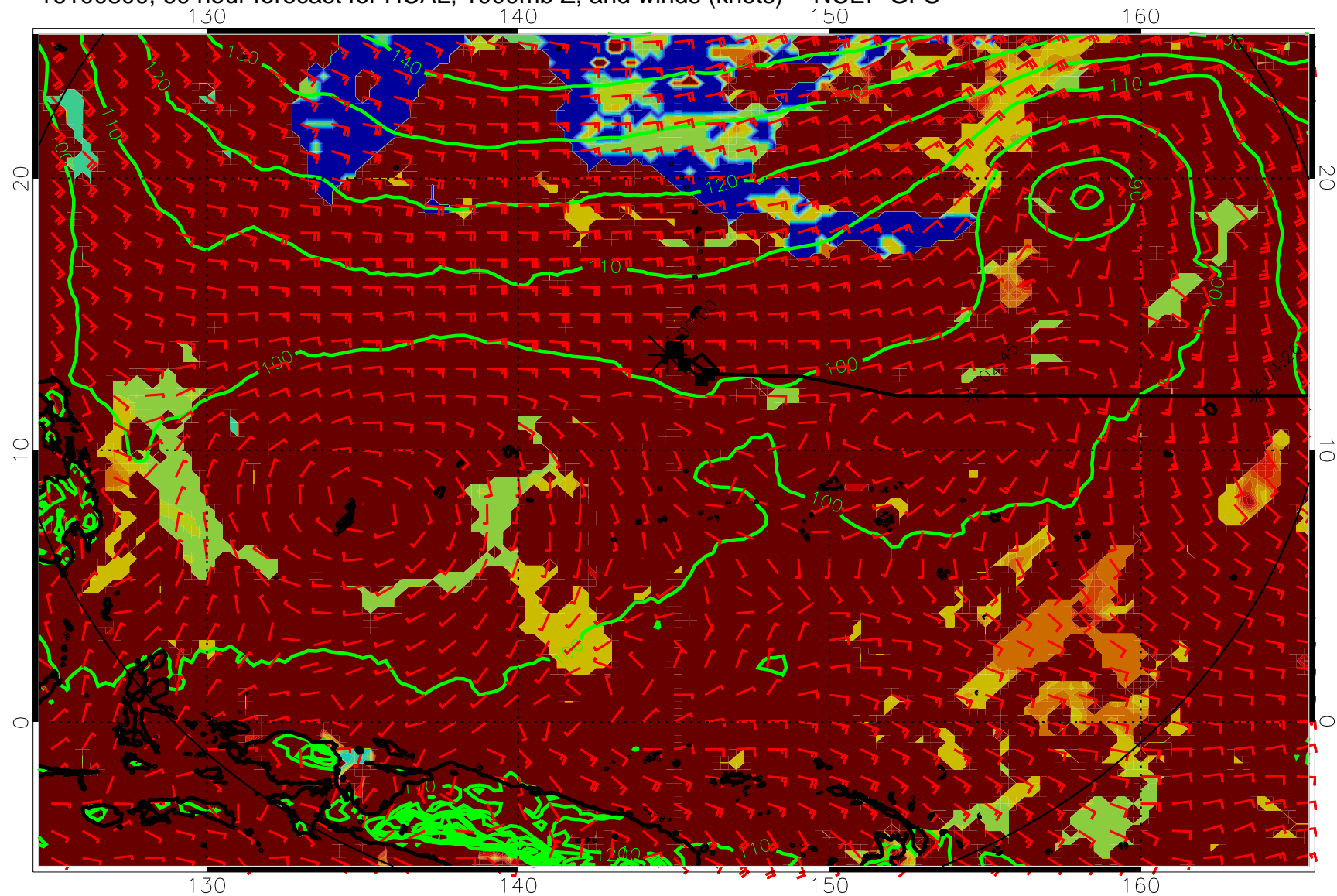
16100800, 60 hour forecast for HCAL, 1000mb Z, and winds (knots) -- NCEP GFS
