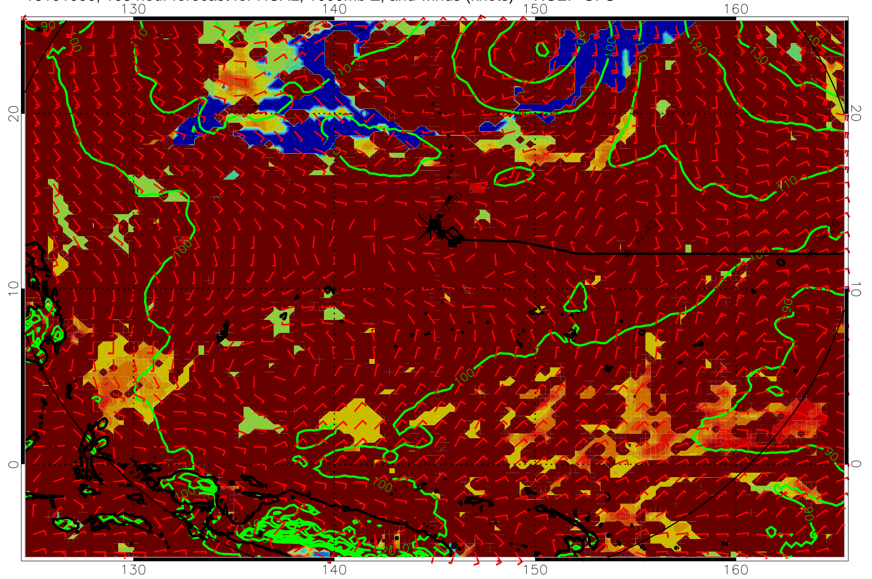
16101000, 108 hour forecast for HCAL, 1000mb Z, and winds (knots) -- NCEP GFS
