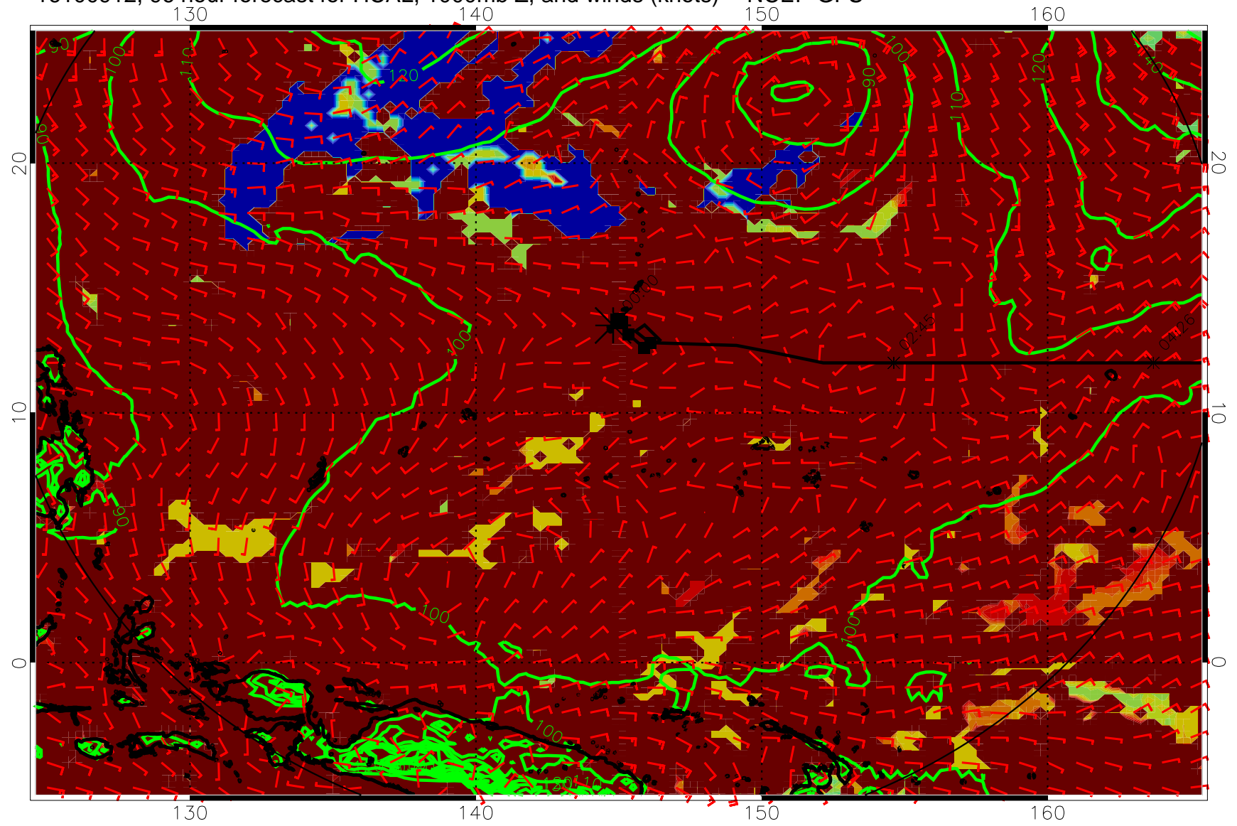
16100912, 96 hour forecast for HCAL, 1000mb Z, and winds (knots) -- NCEP GFS
