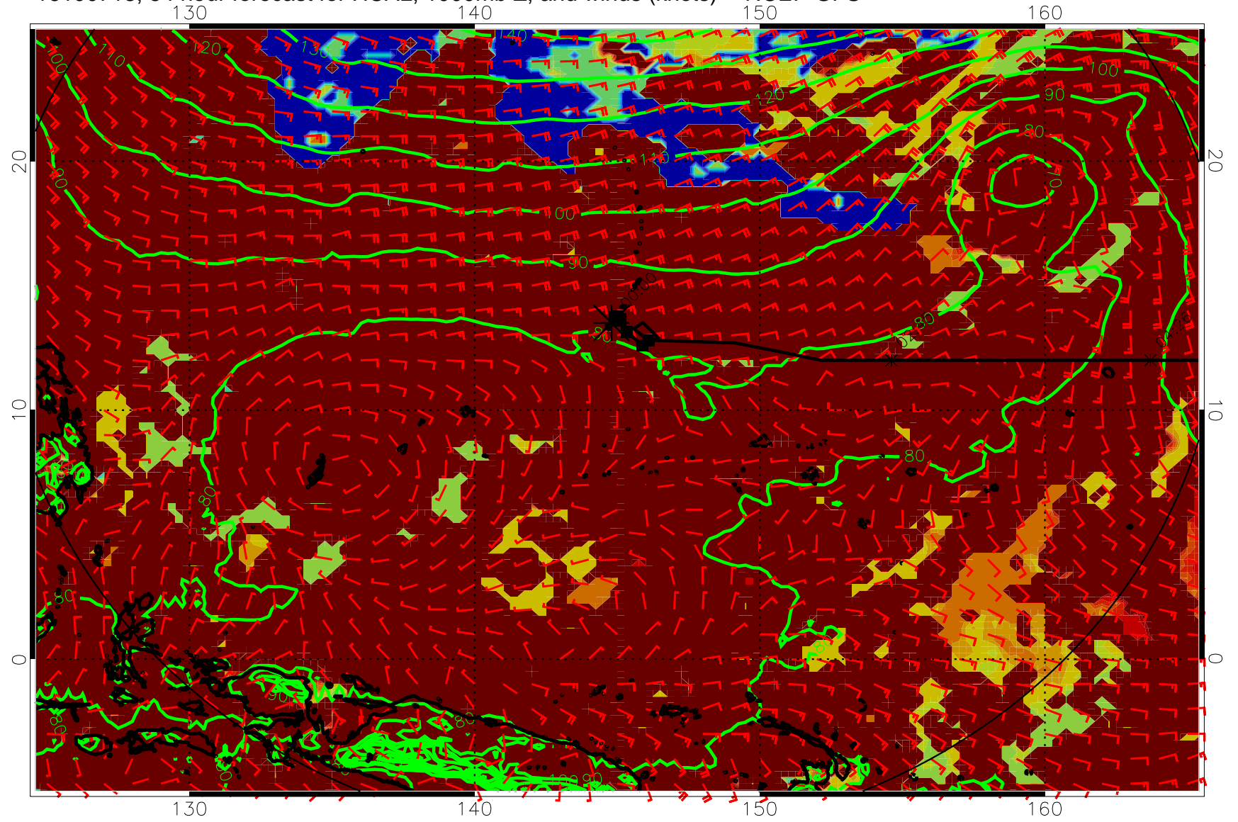
16100718, 54 hour forecast for HCAL, 1000mb Z, and winds (knots) -- NCEP GFS
