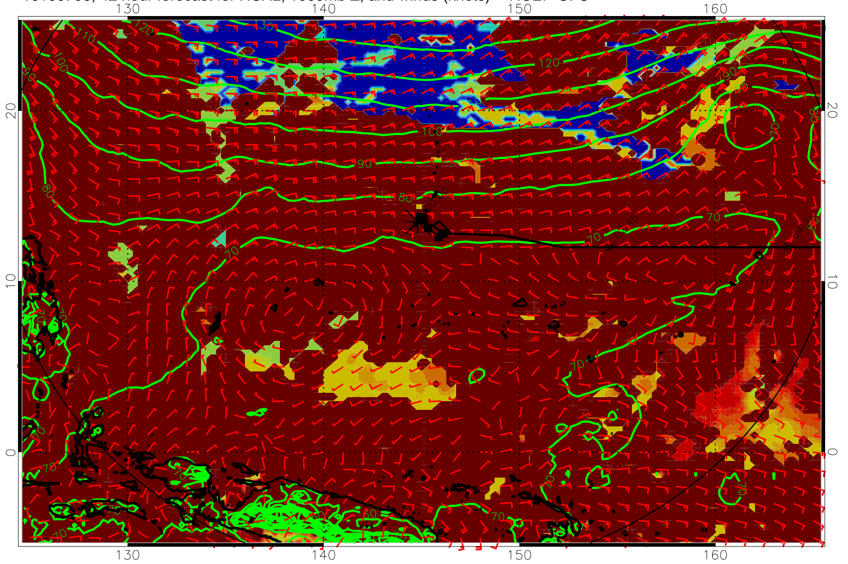
16100706, 42 hour forecast for HCAL, 1000mb Z, and winds (knots) -- NCEP GFS
