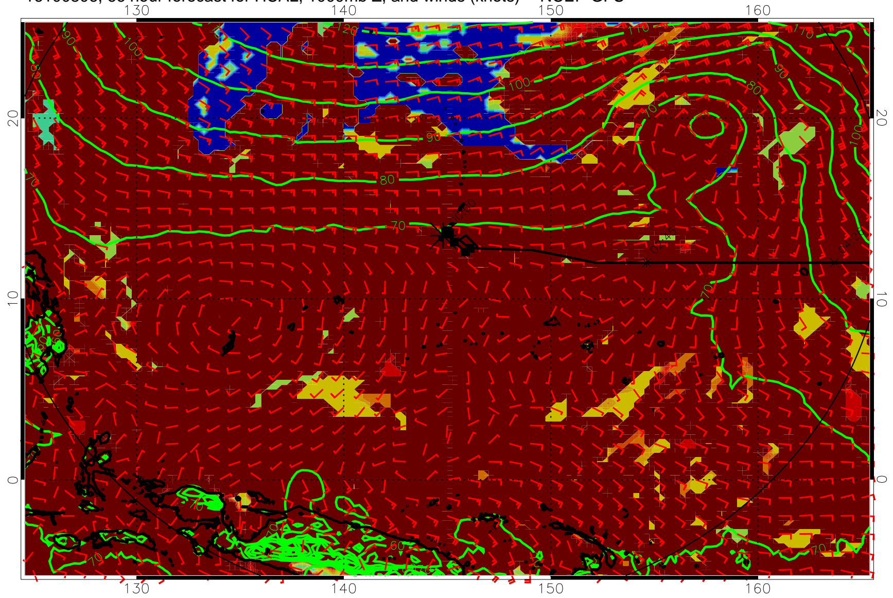
16100806, 66 hour forecast for HCAL, 1000mb Z, and winds (knots) -- NCEP GFS
