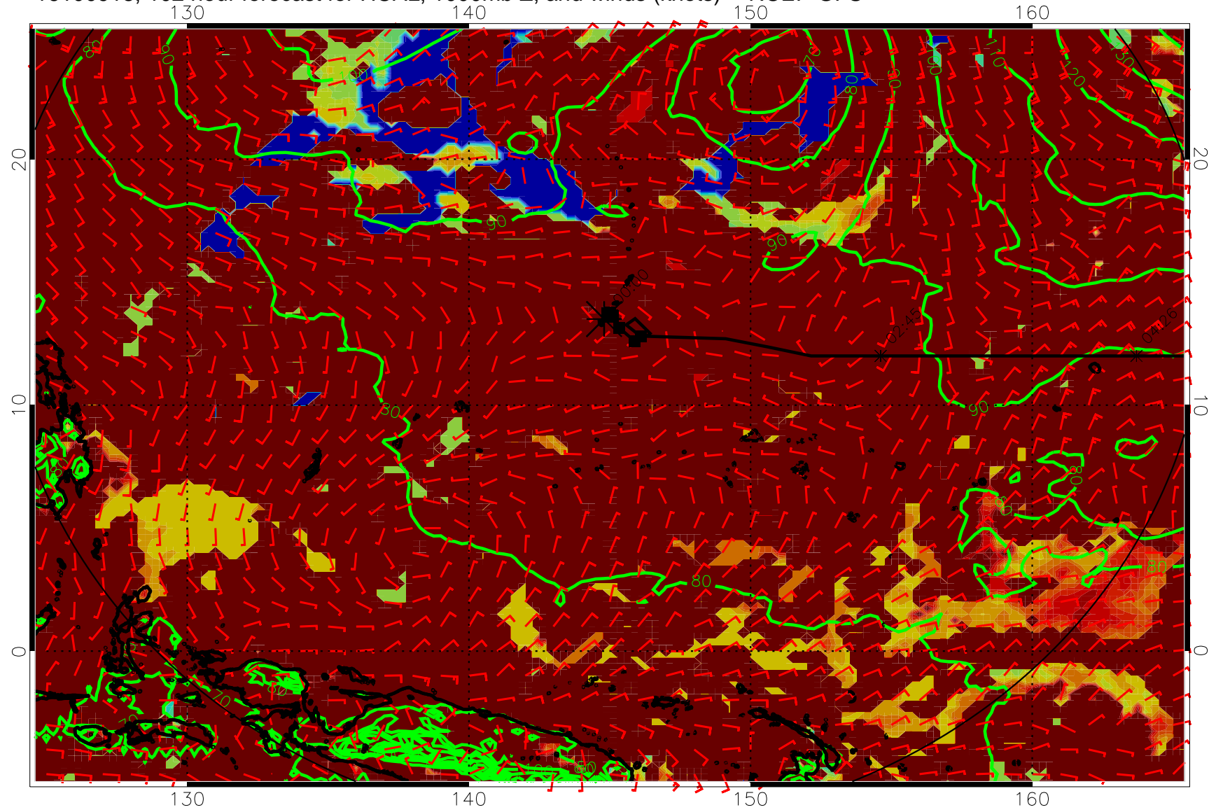
16100918, 102 hour forecast for HCAL, 1000mb Z, and winds (knots) -- NCEP GFS
