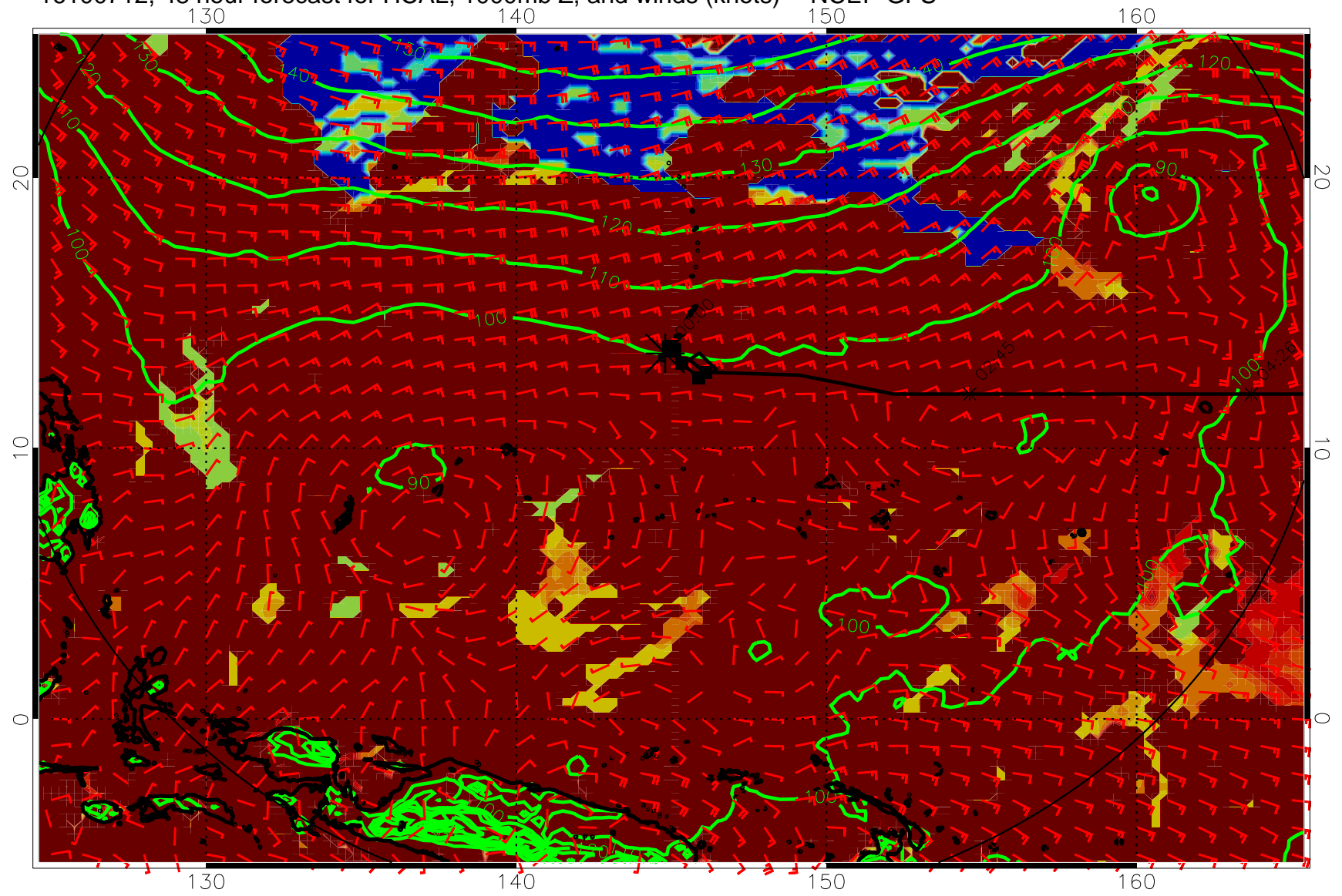
16100712, 48 hour forecast for HCAL, 1000mb Z, and winds (knots) -- NCEP GFS
