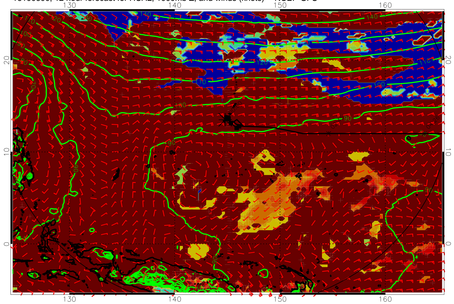
16100600, 12 hour forecast for HCAL, 1000mb Z, and winds (knots) -- NCEP GFS
