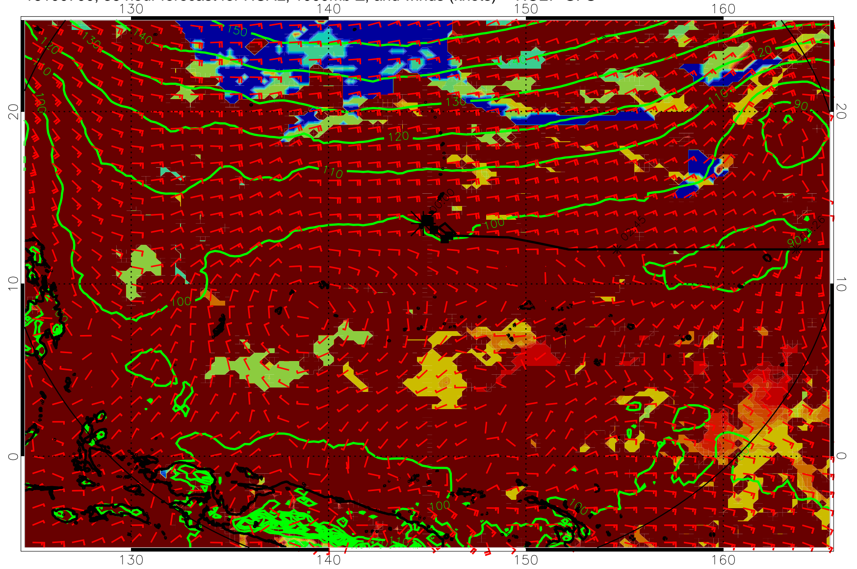
16100700, 36 hour forecast for HCAL, 1000mb Z, and winds (knots) -- NCEP GFS
