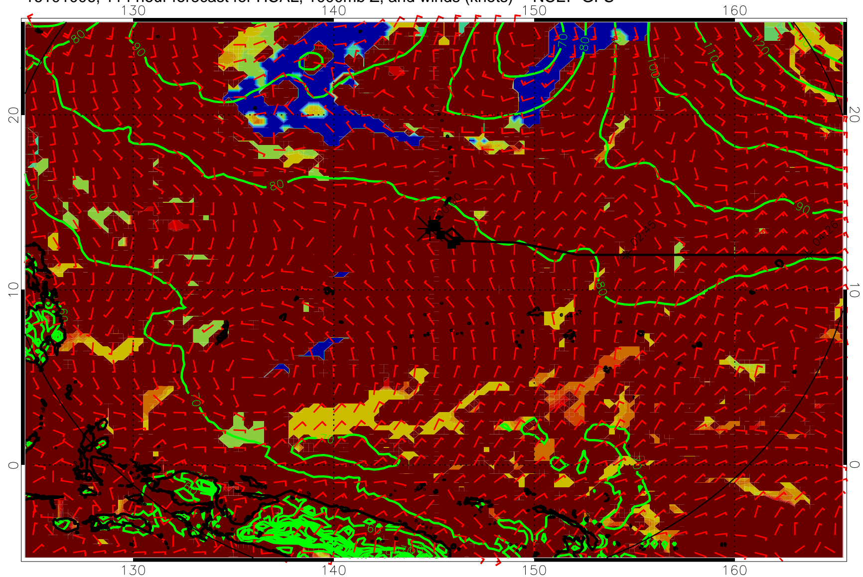
16101006, 114 hour forecast for HCAL, 1000mb Z, and winds (knots) -- NCEP GFS
