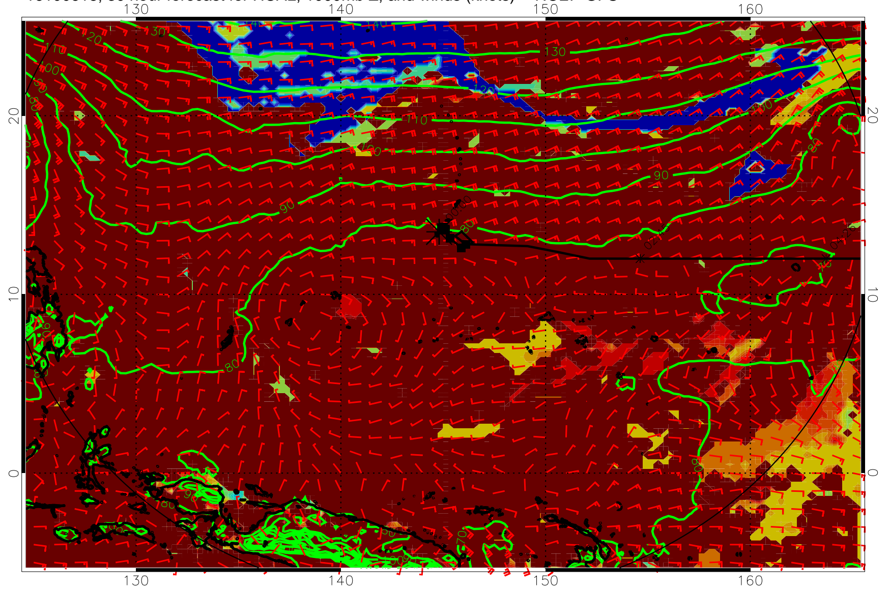
16100618, 30 hour forecast for HCAL, 1000mb Z, and winds (knots) -- NCEP GFS
