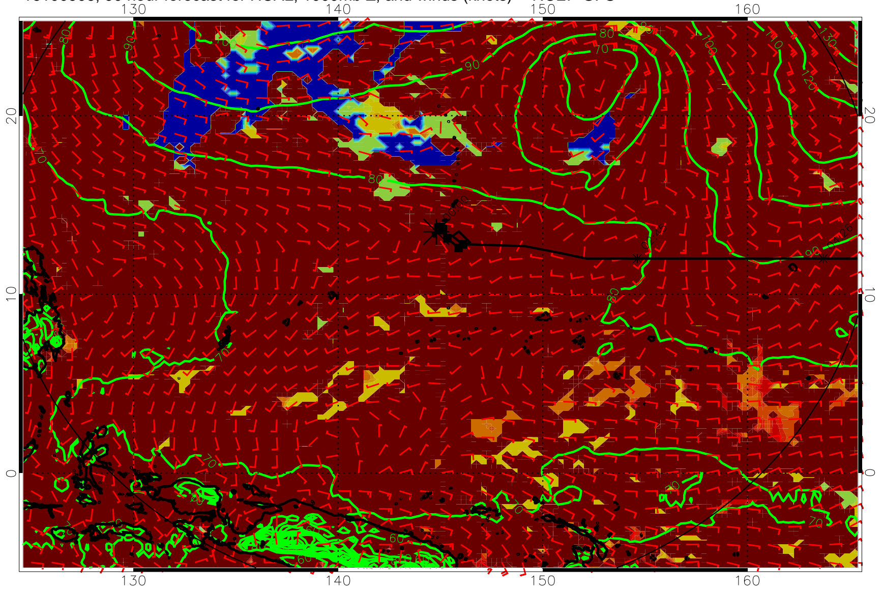
16100906, 90 hour forecast for HCAL, 1000mb Z, and winds (knots) -- NCEP GFS
