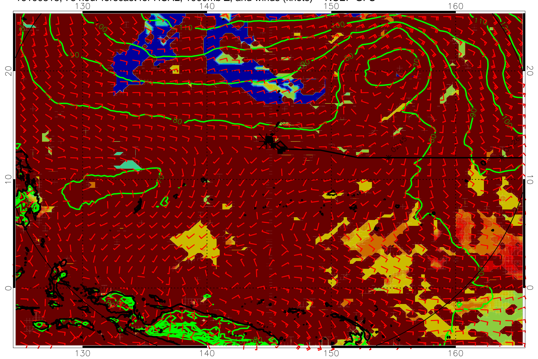
16100818, 78 hour forecast for HCAL, 1000mb Z, and winds (knots) -- NCEP GFS
