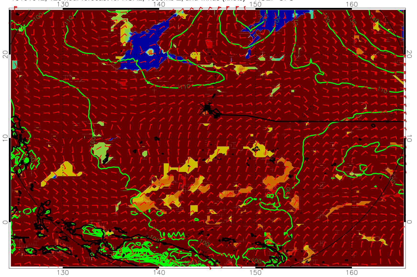
16101012, 120 hour forecast for HCAL, 1000mb Z, and winds (knots) -- NCEP GFS
