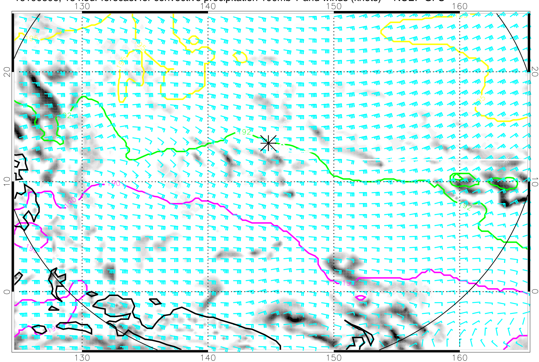
16100606, 18 hour forecast for convective precipitation 100mb T and winds (knots) -- NCEP GFS
