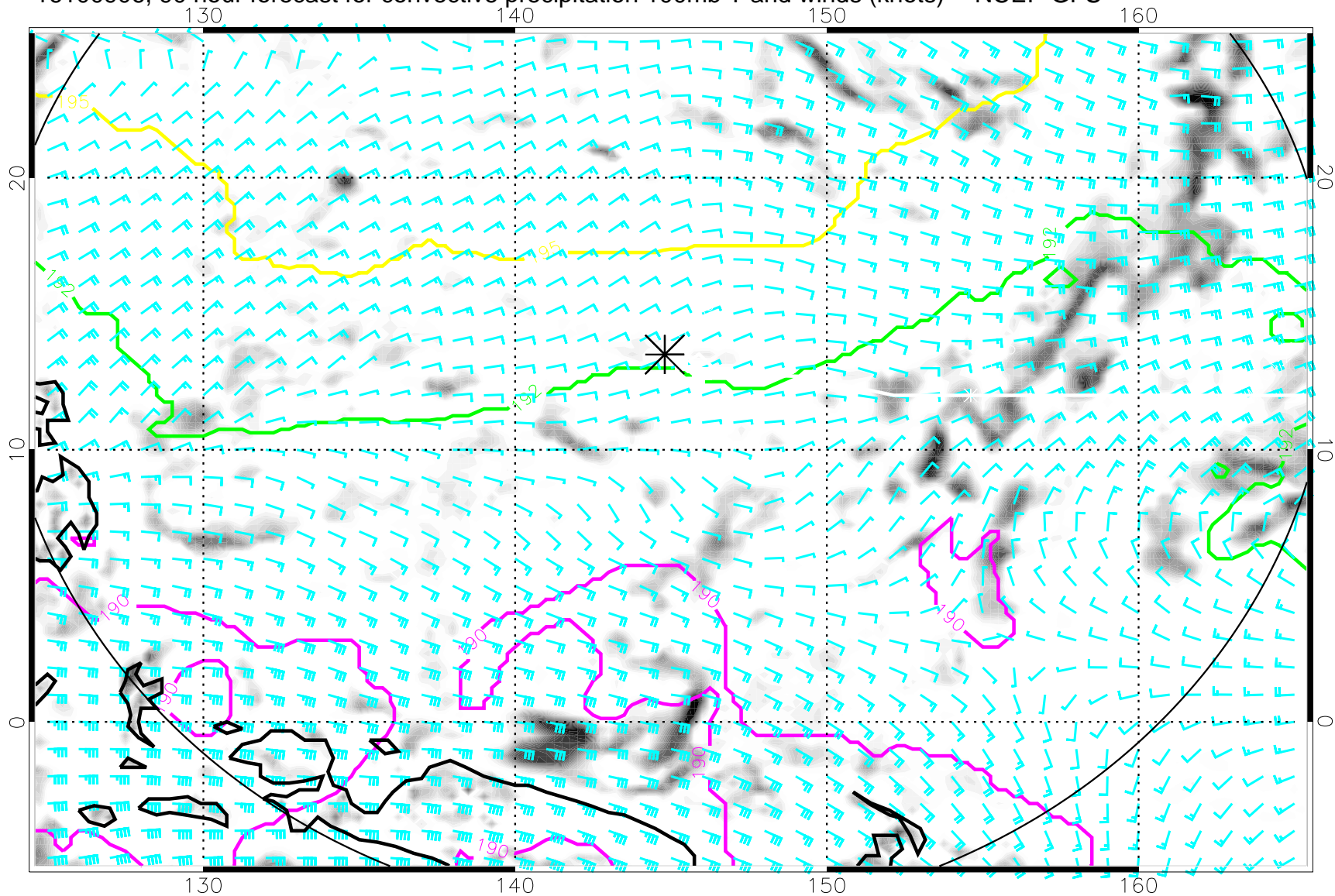
16100906, 90 hour forecast for convective precipitation 100mb T and winds (knots) -- NCEP GFS
