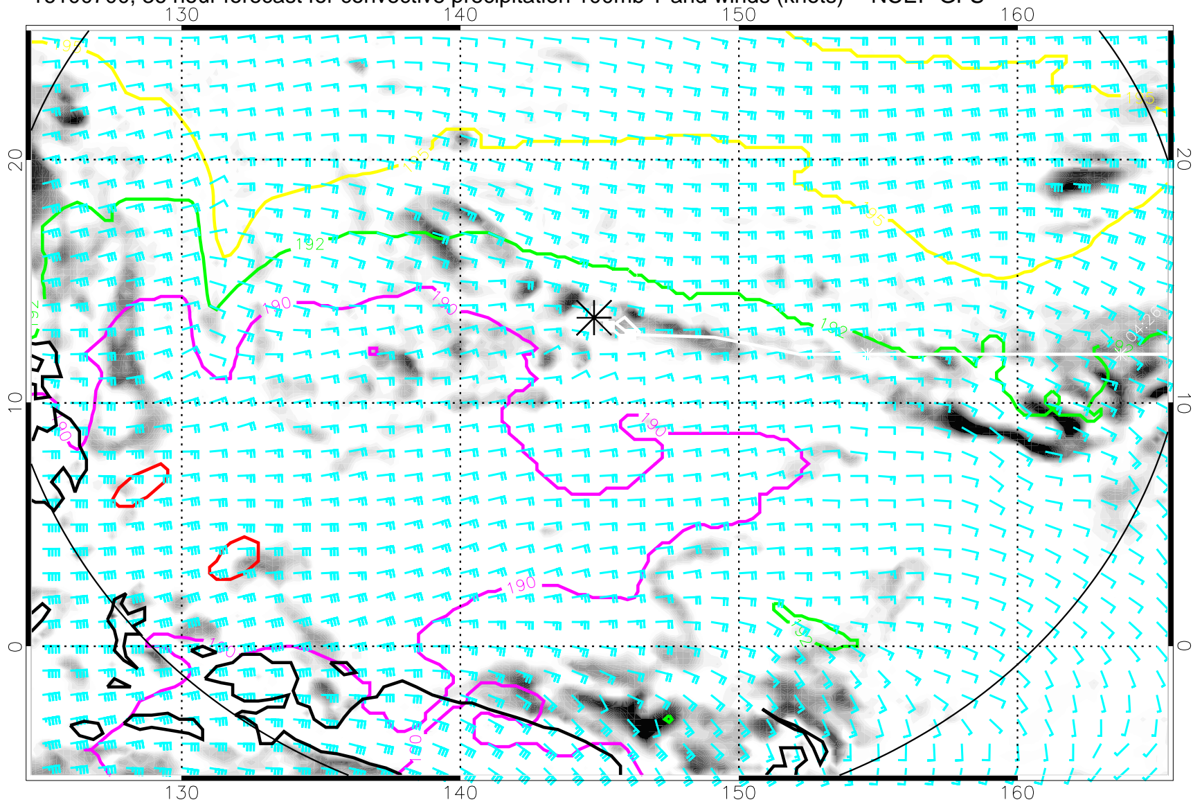
16100700, 36 hour forecast for convective precipitation 100mb T and winds (knots) -- NCEP GFS
