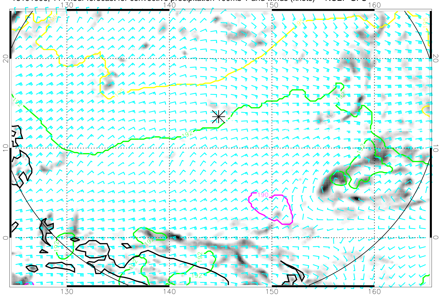
16101006, 114 hour forecast for convective precipitation 100mb T and winds (knots) -- NCEP GFS
