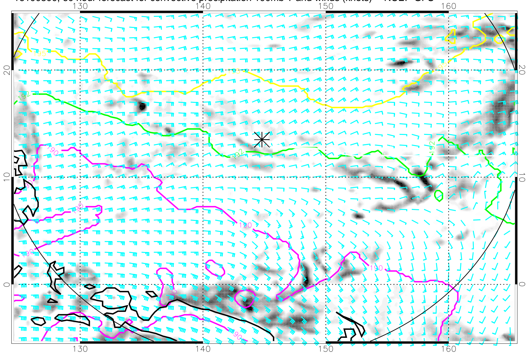
16100800, 60 hour forecast for convective precipitation 100mb T and winds (knots) -- NCEP GFS
