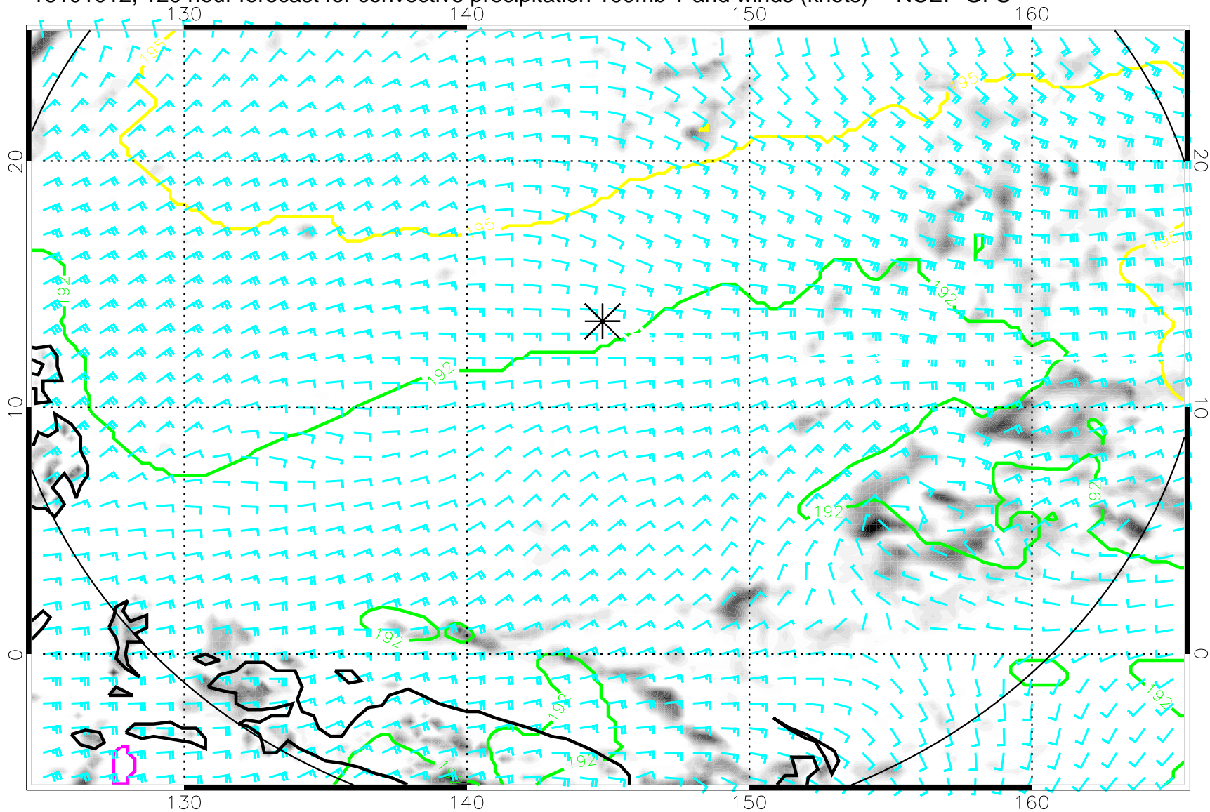
16101012, 120 hour forecast for convective precipitation 100mb T and winds (knots) -- NCEP GFS
