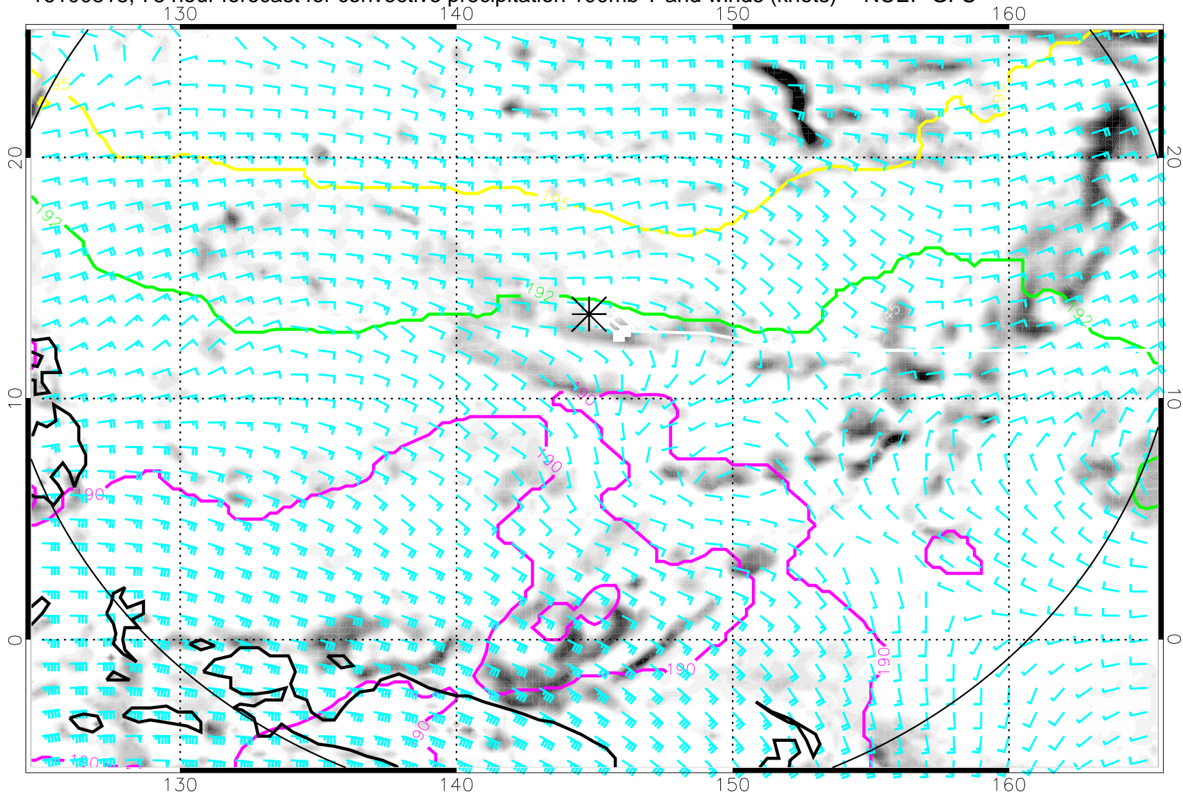
16100818, 78 hour forecast for convective precipitation 100mb T and winds (knots) -- NCEP GFS
