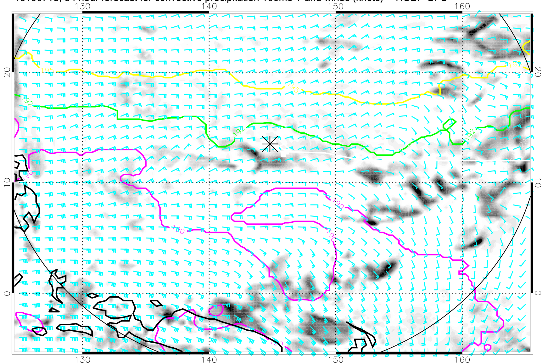
16100718, 54 hour forecast for convective precipitation 100mb T and winds (knots) -- NCEP GFS
