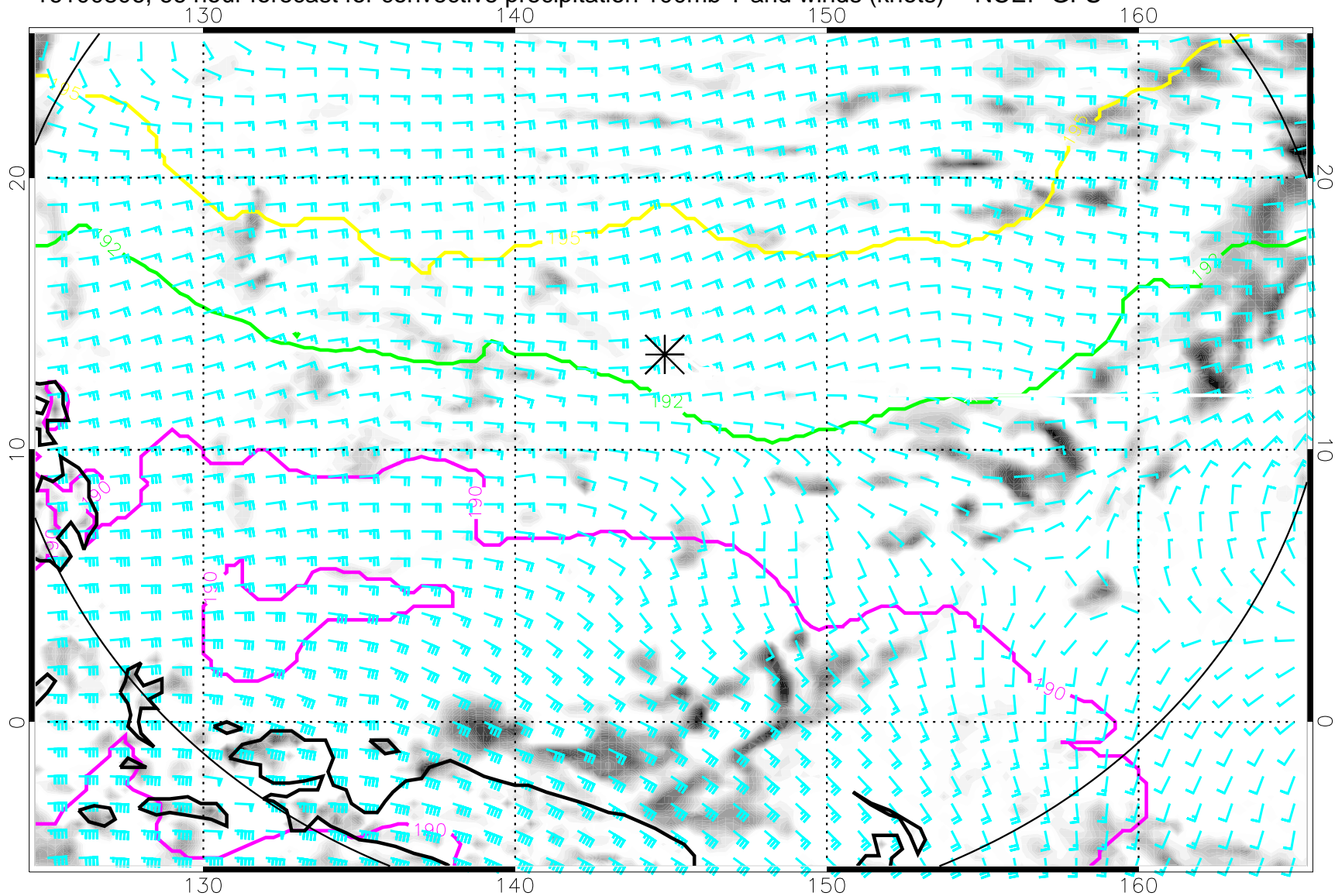
16100806, 66 hour forecast for convective precipitation 100mb T and winds (knots) -- NCEP GFS
