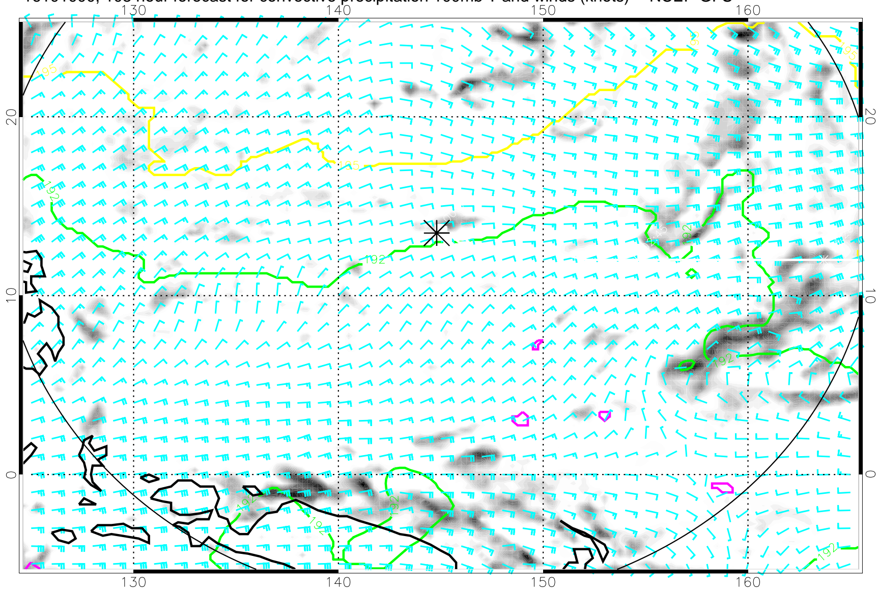
16101000, 108 hour forecast for convective precipitation 100mb T and winds (knots) -- NCEP GFS
