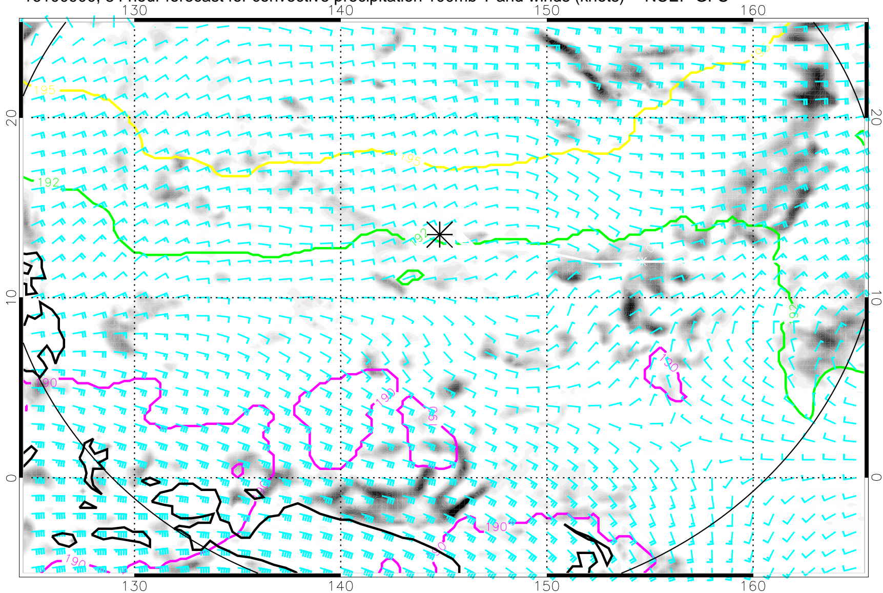
16100900, 84 hour forecast for convective precipitation 100mb T and winds (knots) -- NCEP GFS
