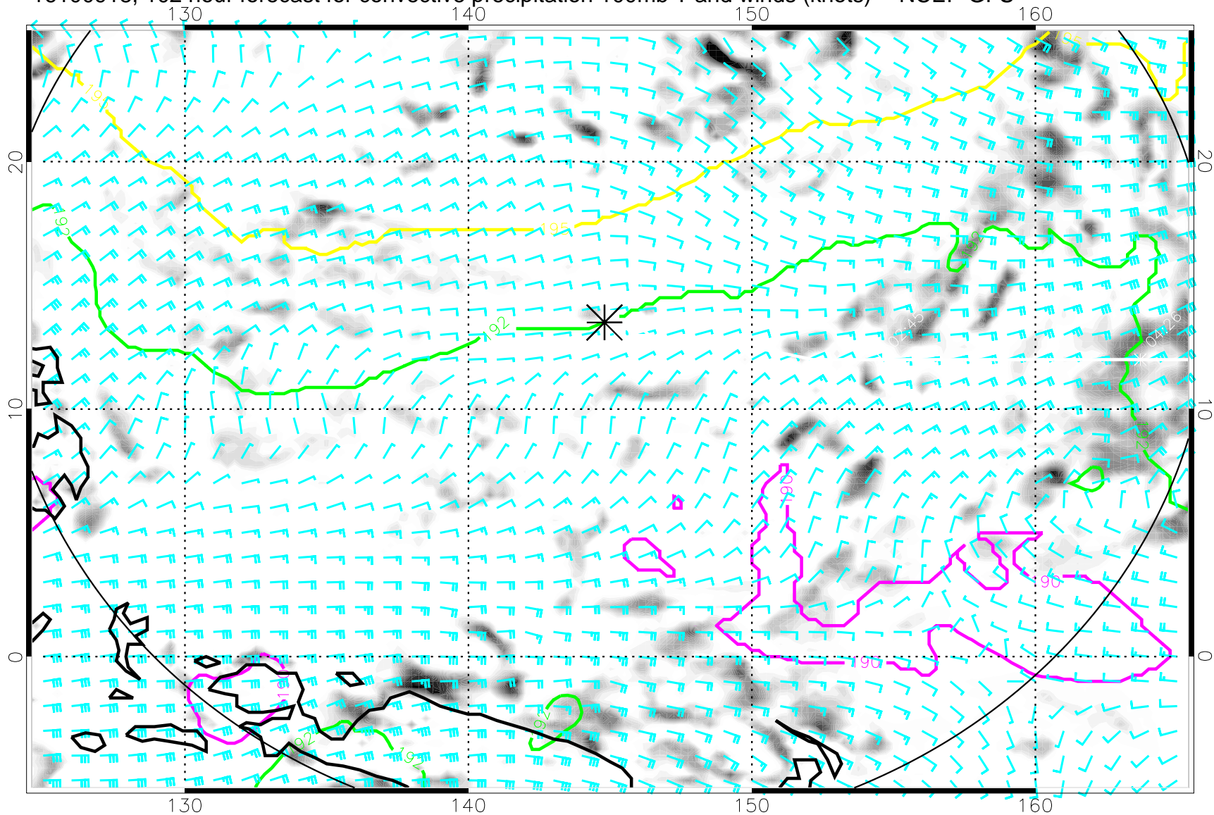
16100918, 102 hour forecast for convective precipitation 100mb T and winds (knots) -- NCEP GFS
