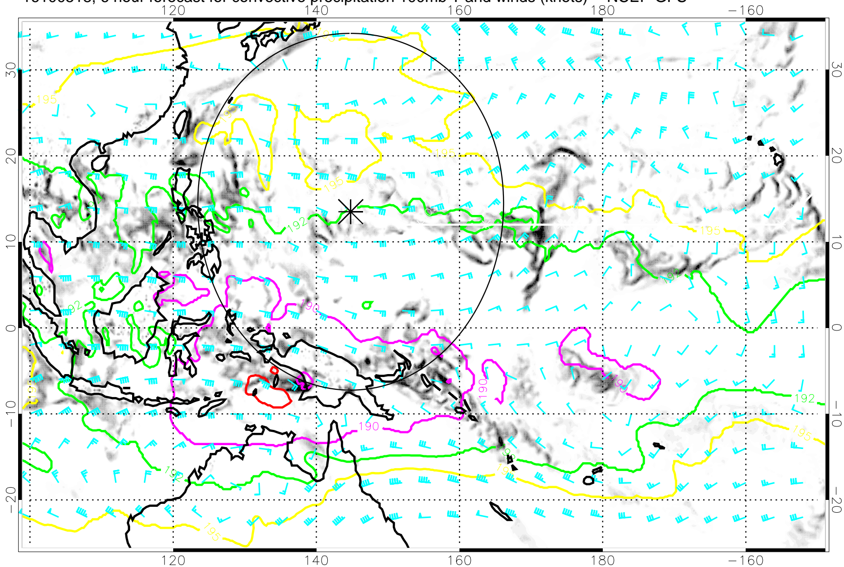
16100518, 6 hour forecast for convective precipitation 100mb T and winds (knots) -- NCEP GFS
