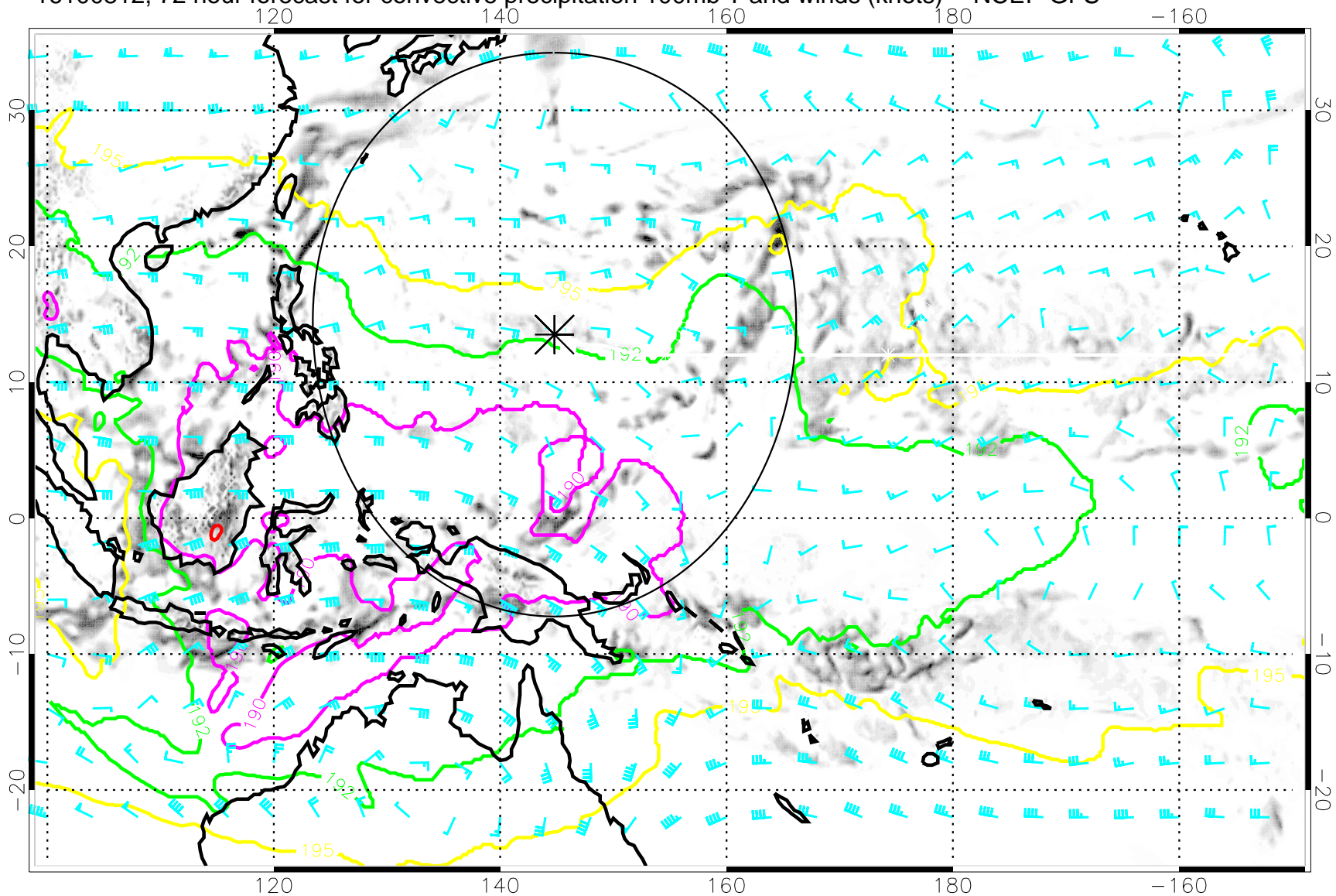
16100812, 72 hour forecast for convective precipitation 100mb T and winds (knots) -- NCEP GFS
