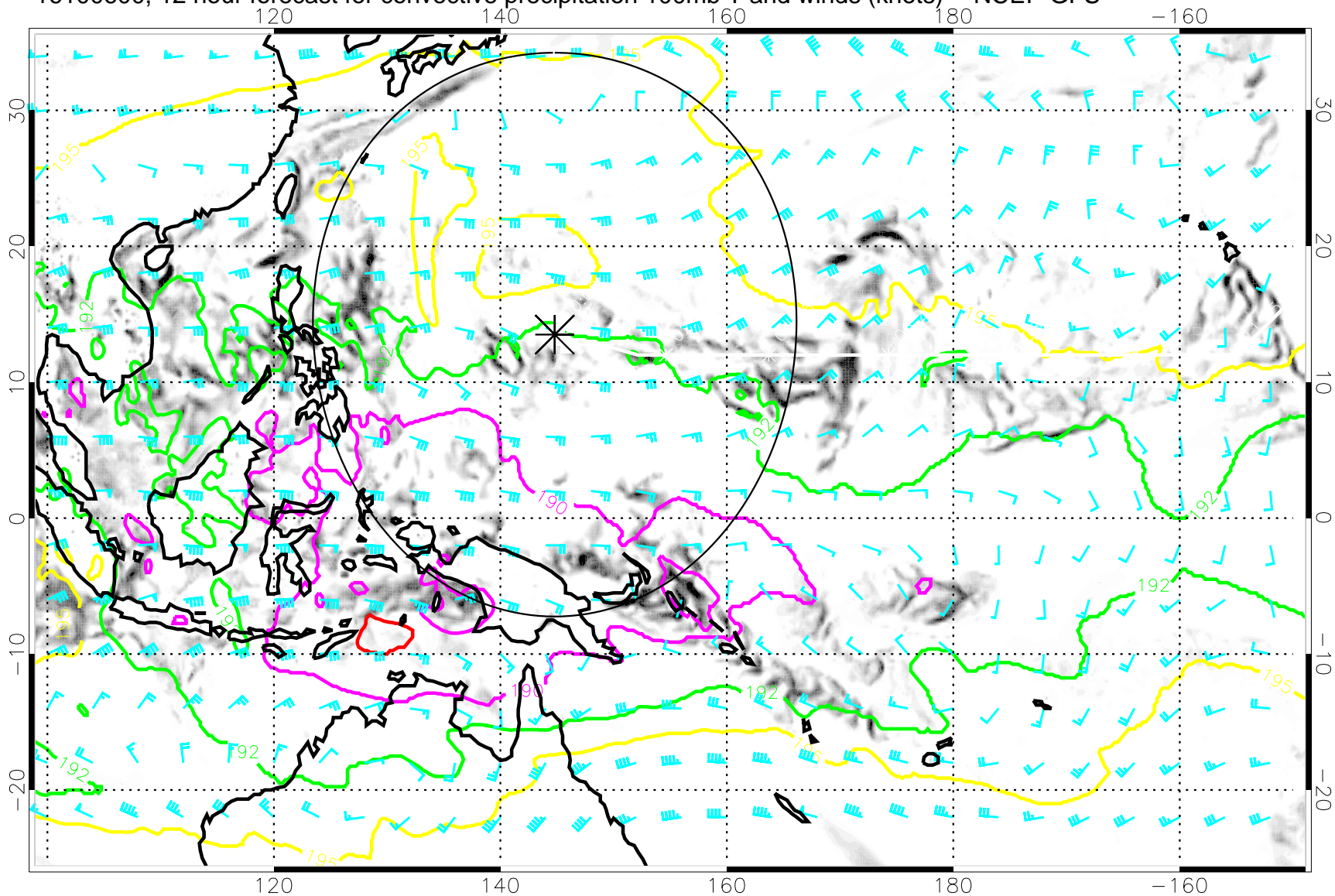
16100600, 12 hour forecast for convective precipitation 100mb T and winds (knots) -- NCEP GFS
