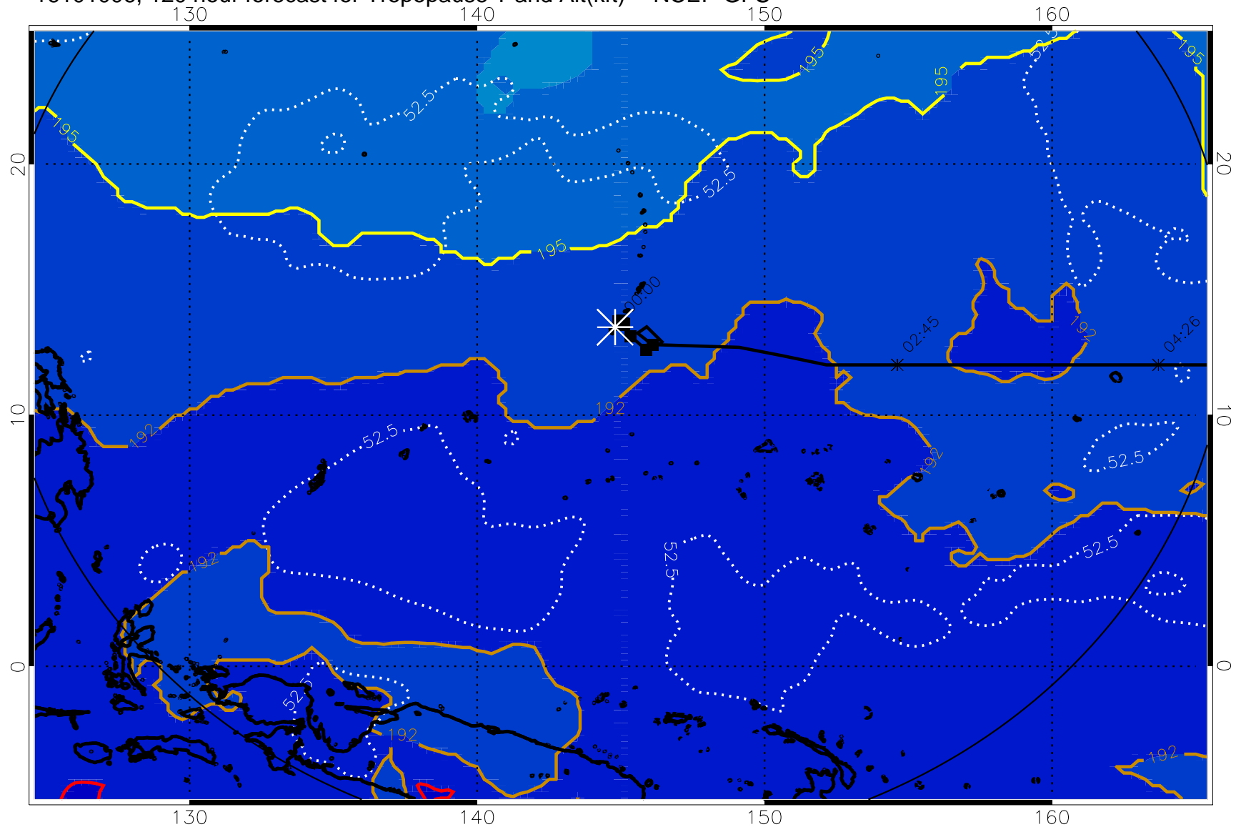
16101006, 120 hour forecast for Tropopause T and Alt(kft) -- NCEP GFS
