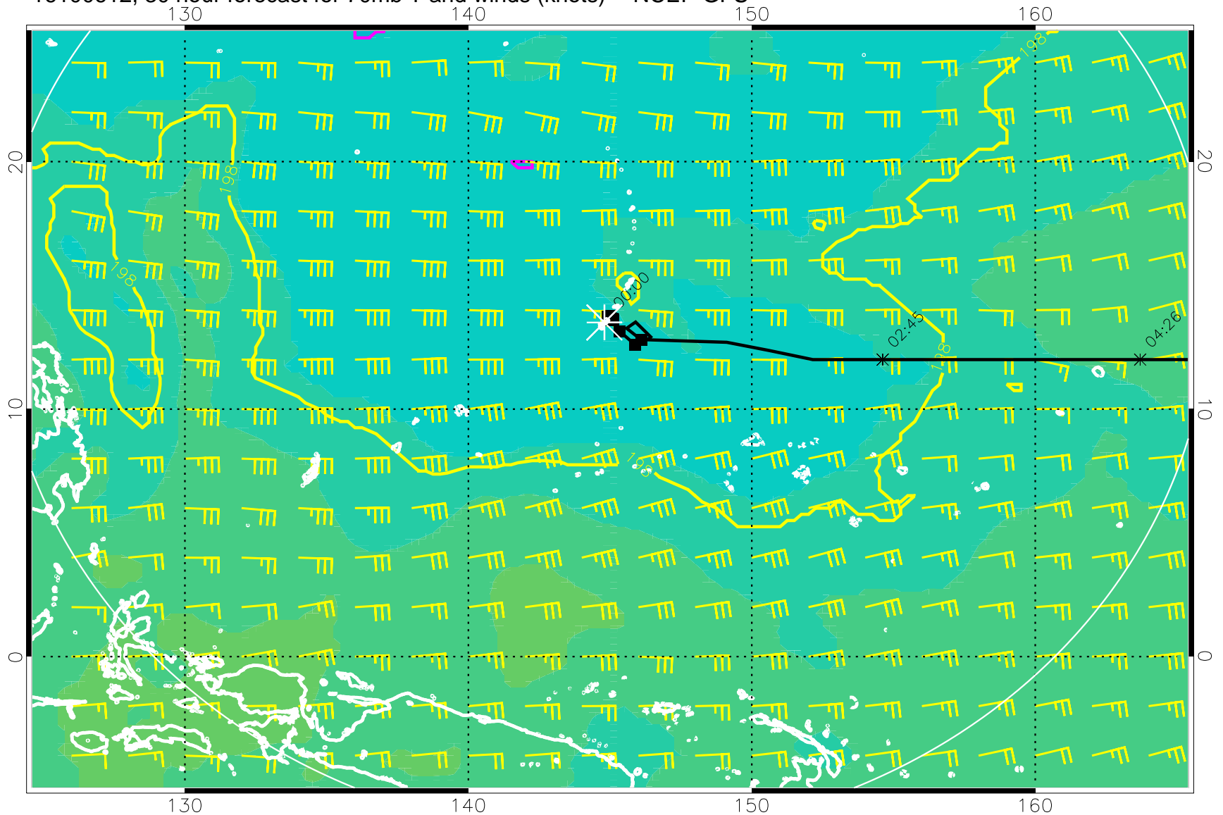
16100612, 30 hour forecast for 70mb T and winds (knots) -- NCEP GFS
