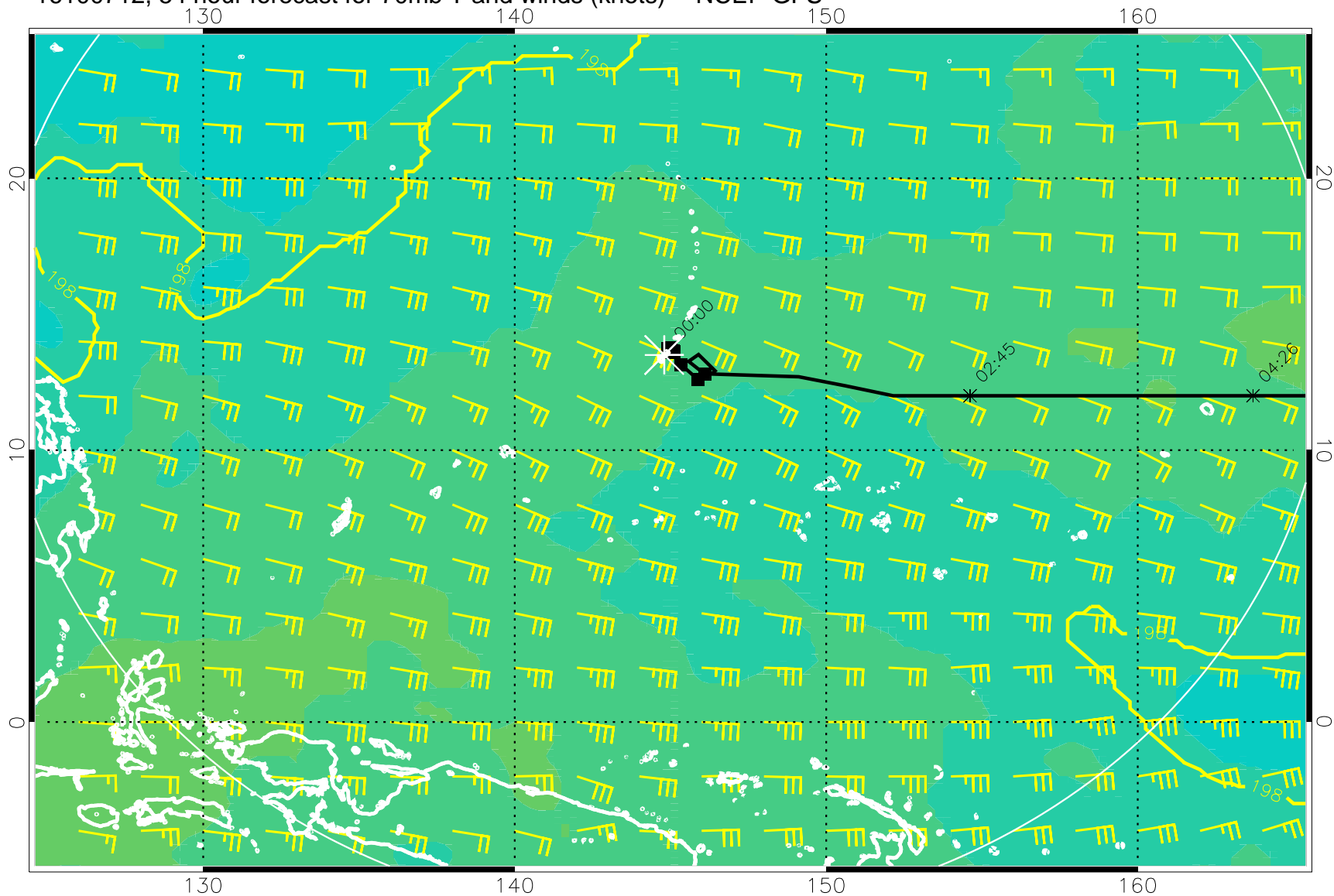
16100712, 54 hour forecast for 70mb T and winds (knots) -- NCEP GFS
