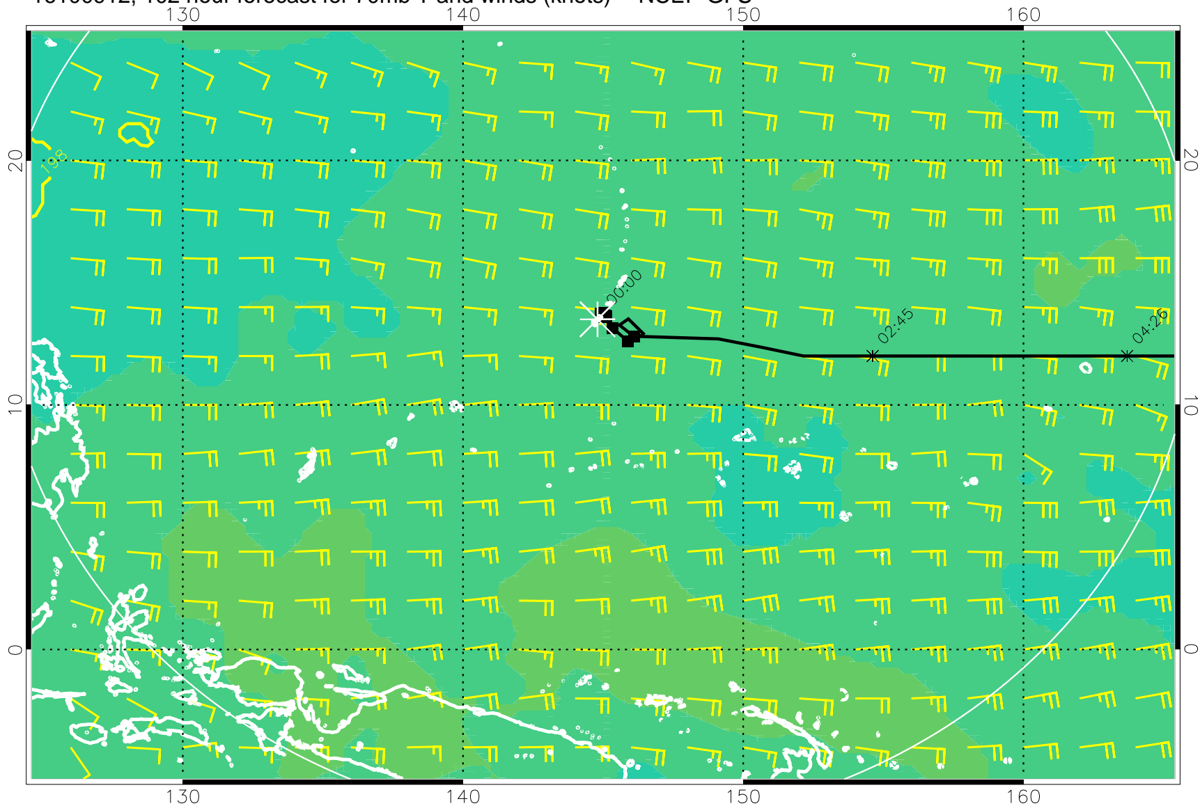
16100912, 102 hour forecast for 70mb T and winds (knots) -- NCEP GFS
