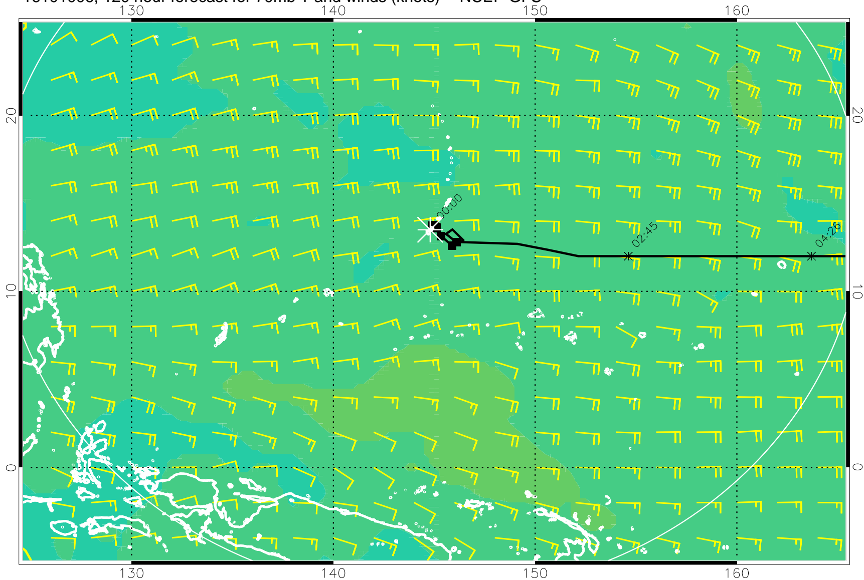
16101006, 120 hour forecast for 70mb T and winds (knots) -- NCEP GFS
