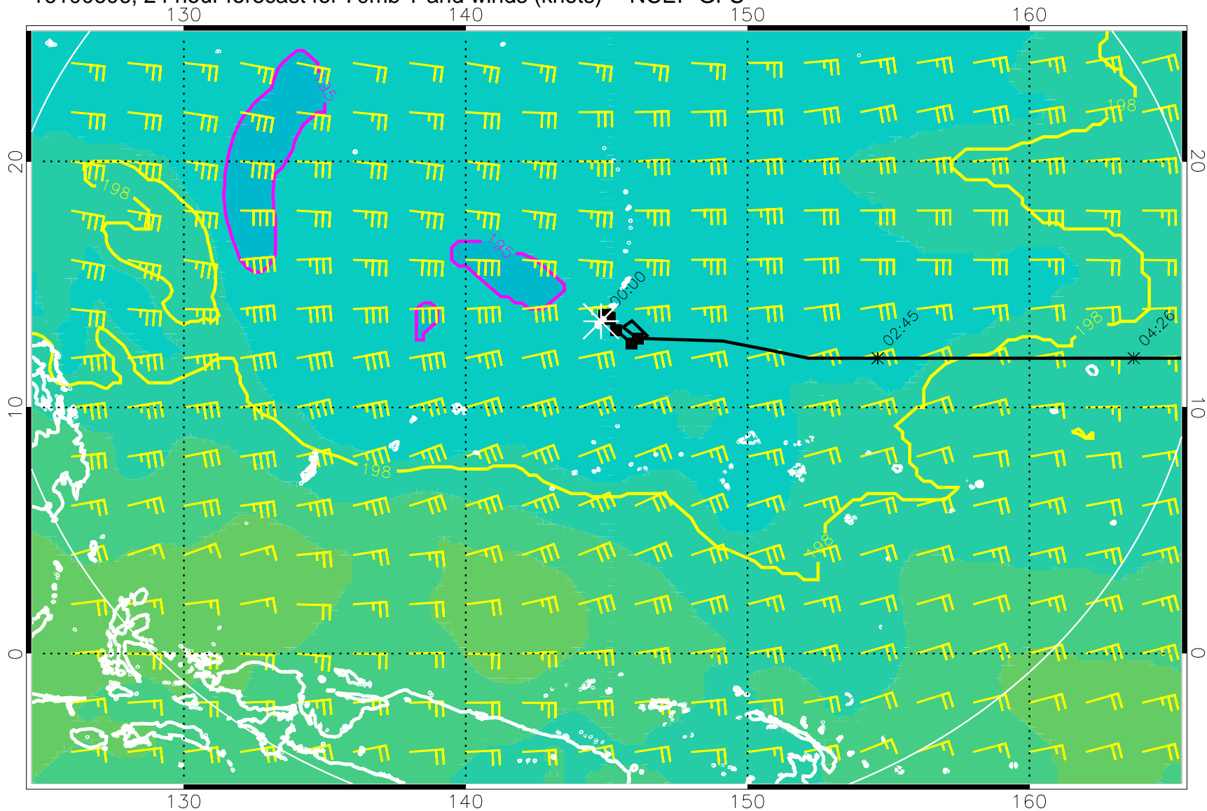
16100606, 24 hour forecast for 70mb T and winds (knots) -- NCEP GFS
