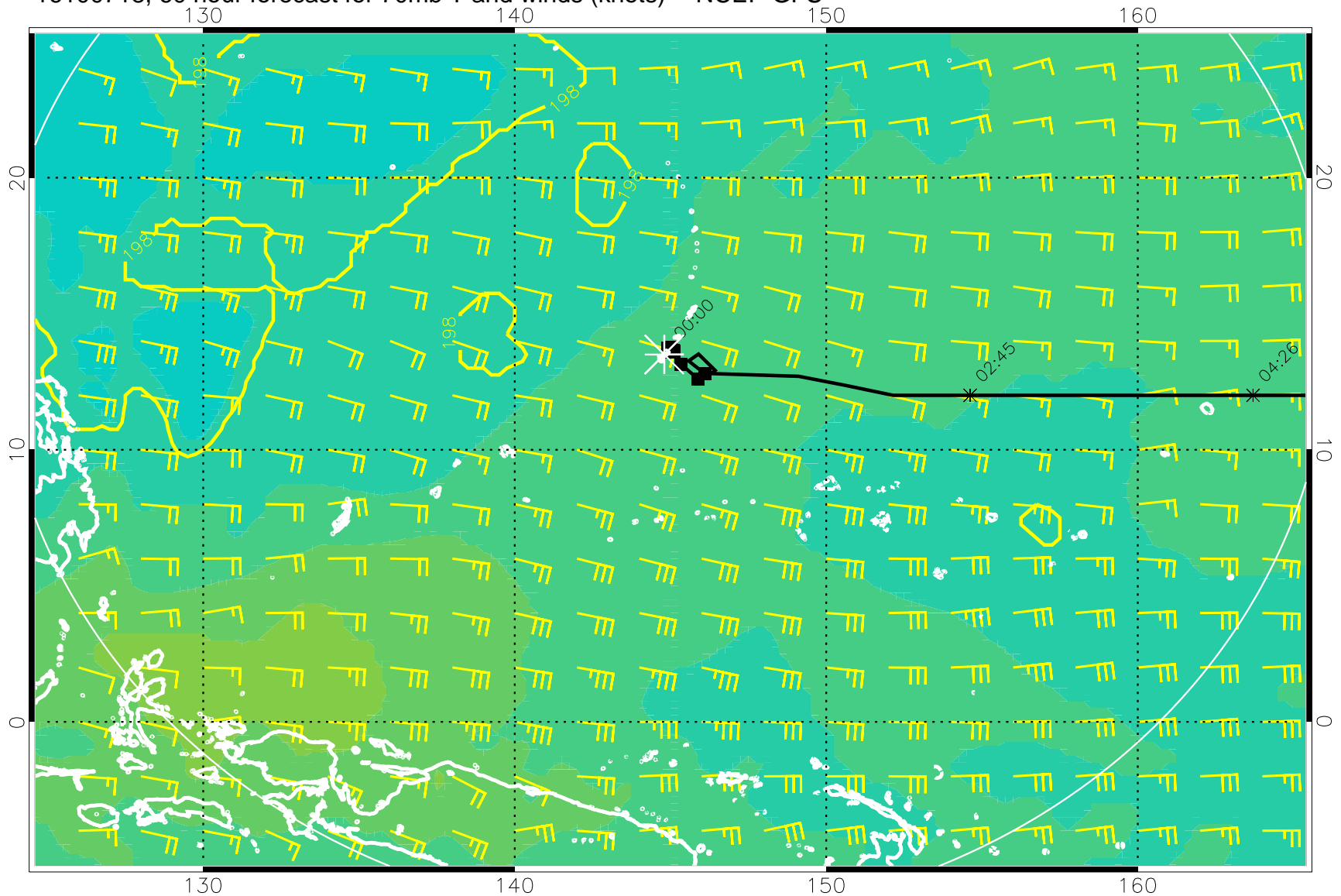
16100718, 60 hour forecast for 70mb T and winds (knots) -- NCEP GFS
