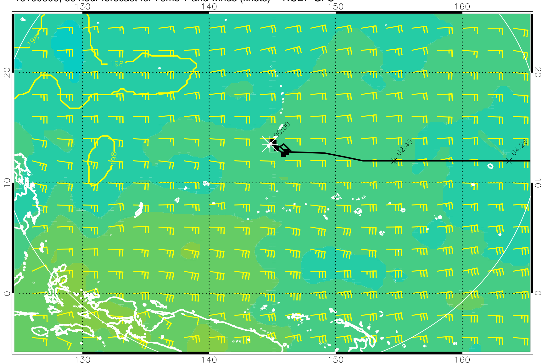
16100800, 66 hour forecast for 70mb T and winds (knots) -- NCEP GFS
