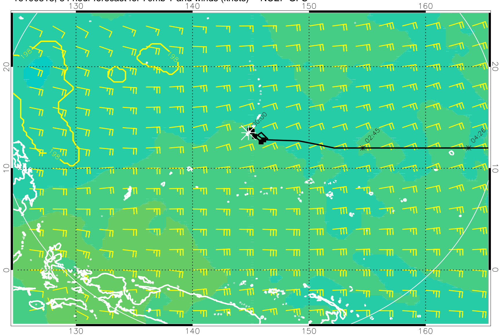
16100818, 84 hour forecast for 70mb T and winds (knots) -- NCEP GFS
