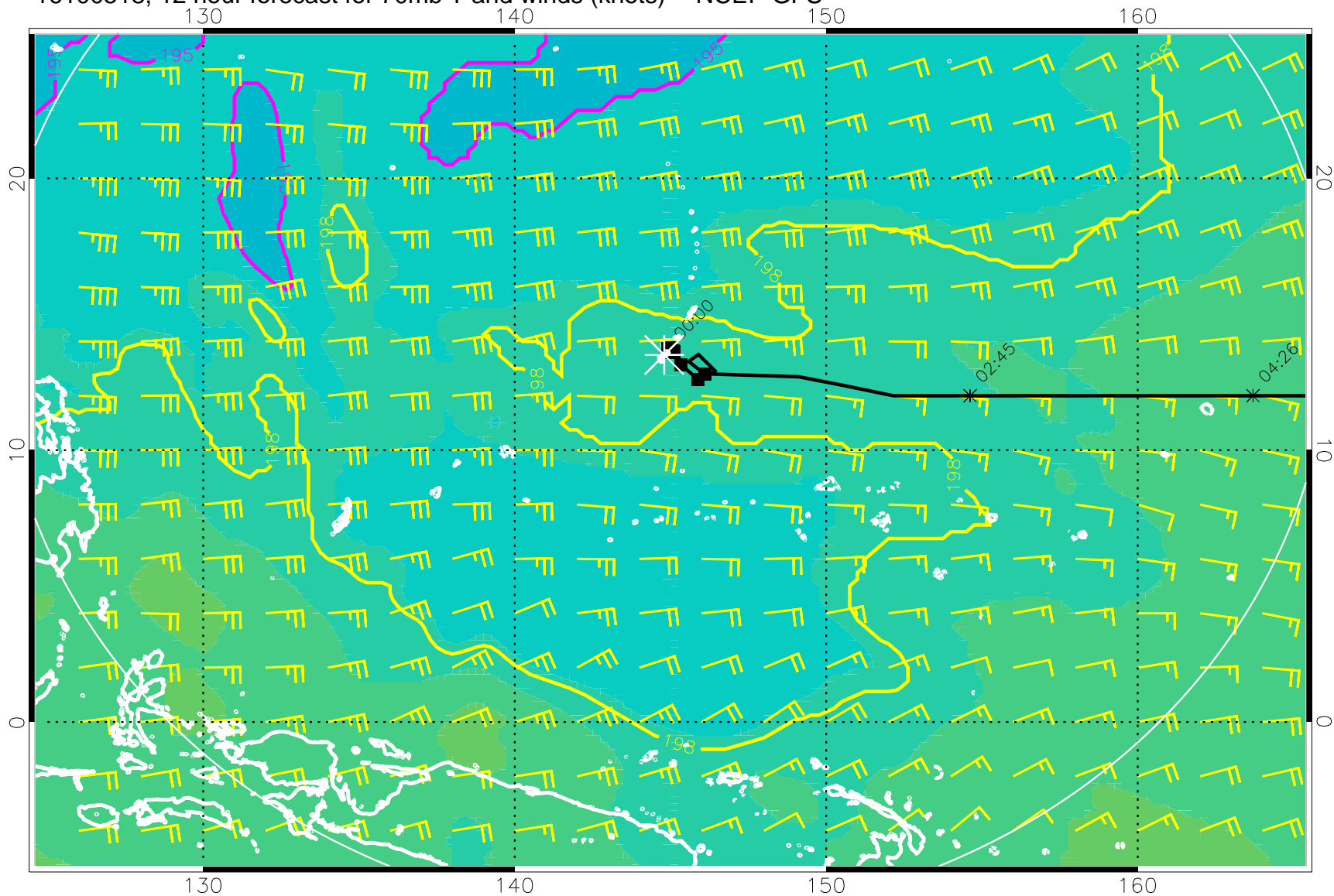
16100518, 12 hour forecast for 70mb T and winds (knots) -- NCEP GFS
