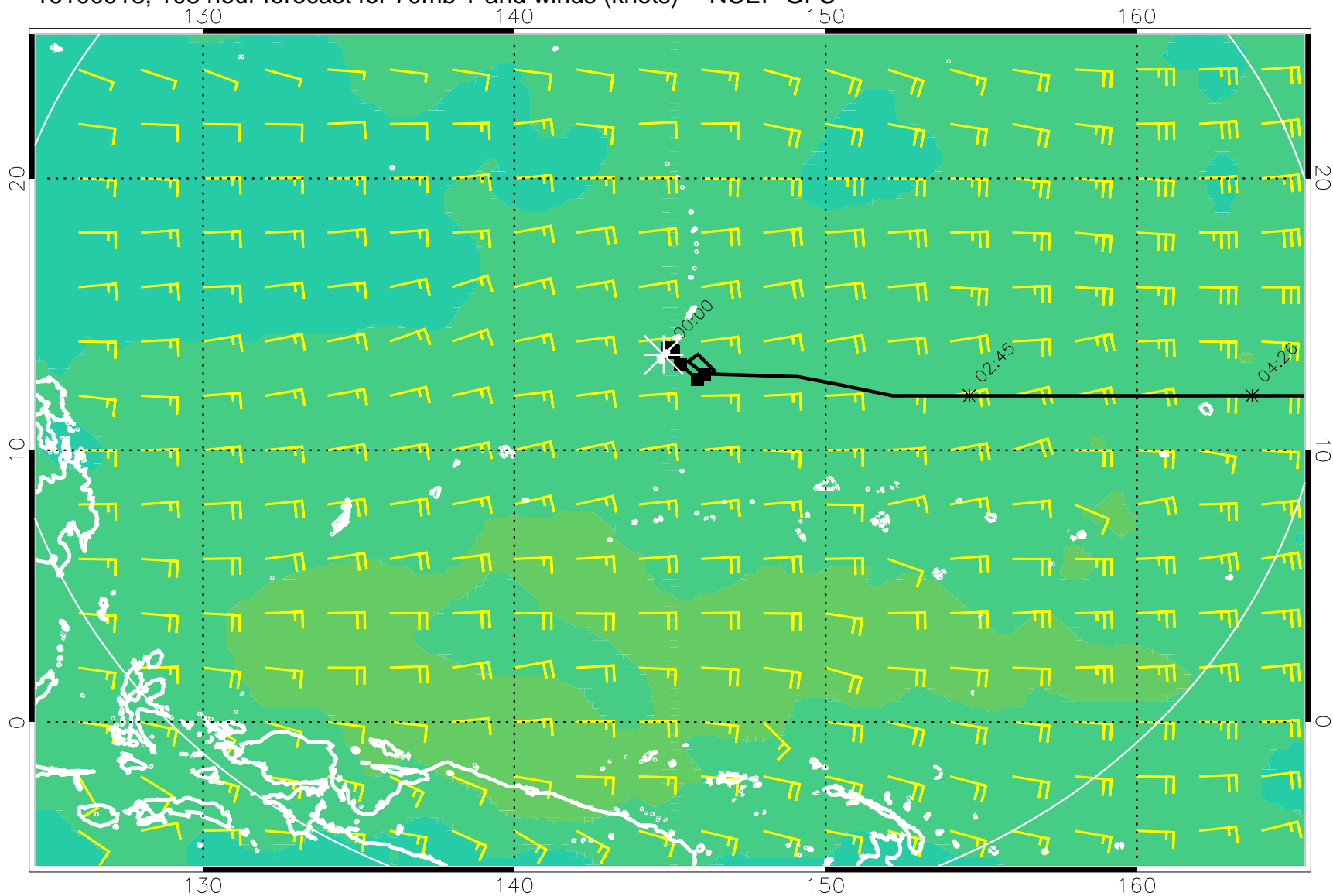
16100918, 108 hour forecast for 70mb T and winds (knots) -- NCEP GFS
