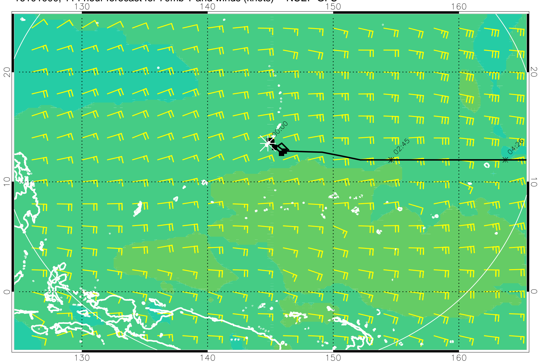
16101000, 114 hour forecast for 70mb T and winds (knots) -- NCEP GFS
