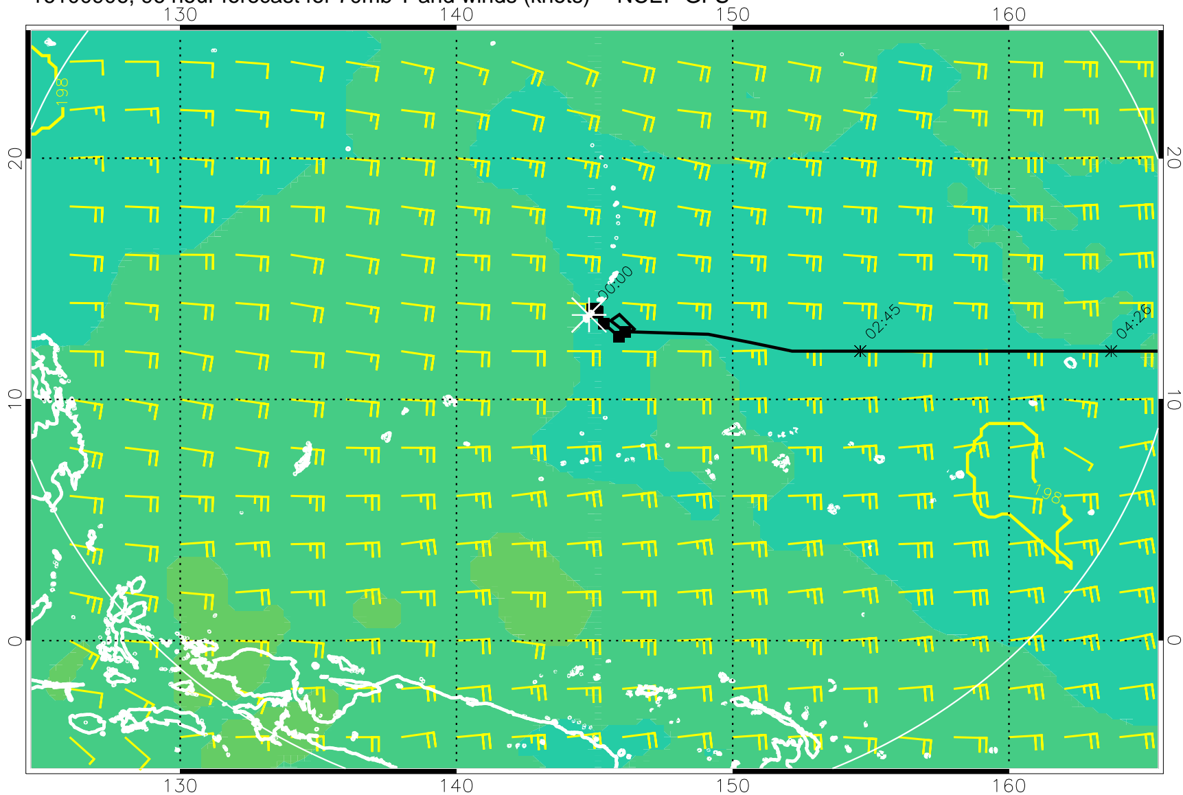
16100906, 96 hour forecast for 70mb T and winds (knots) -- NCEP GFS
