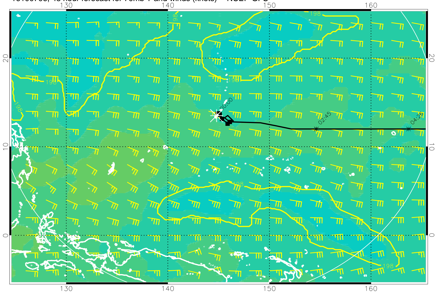
16100706, 48 hour forecast for 70mb T and winds (knots) -- NCEP GFS
