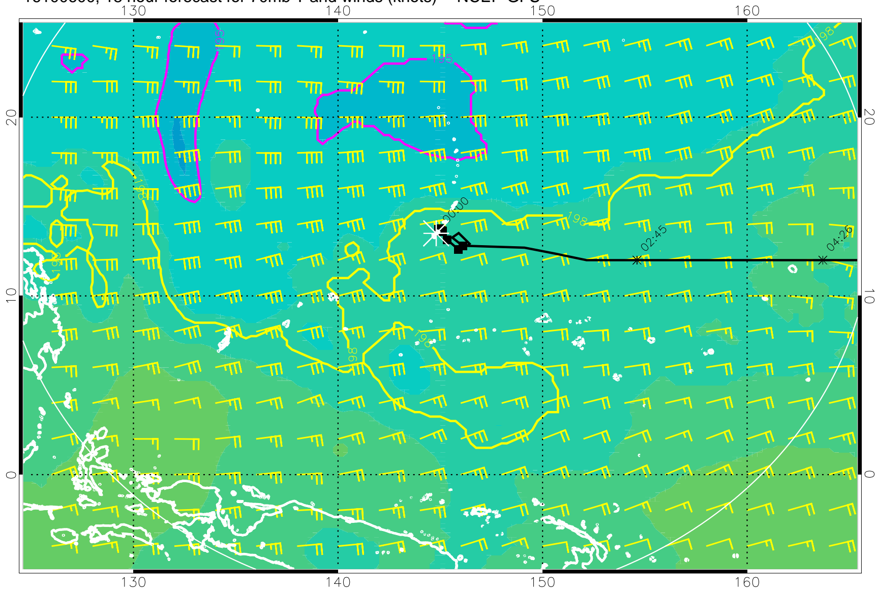
16100600, 18 hour forecast for 70mb T and winds (knots) -- NCEP GFS
