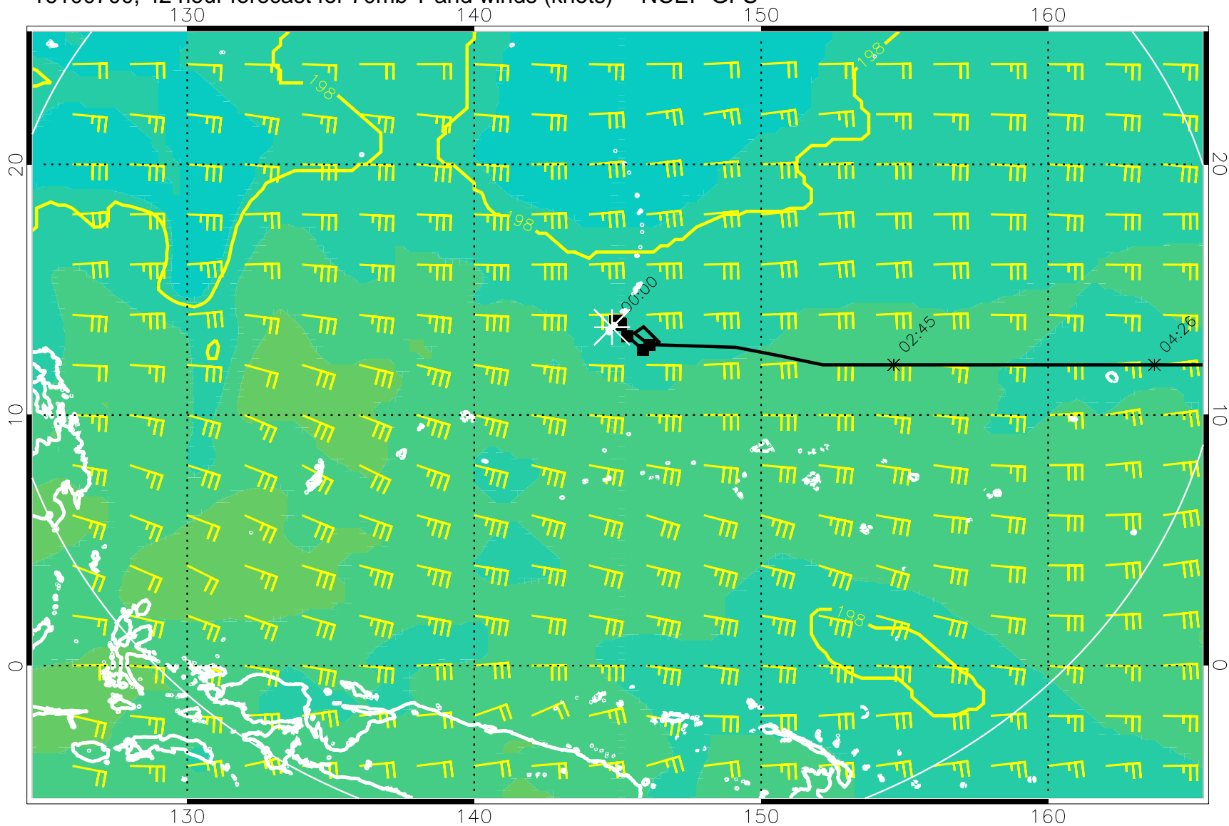
16100700, 42 hour forecast for 70mb T and winds (knots) -- NCEP GFS
