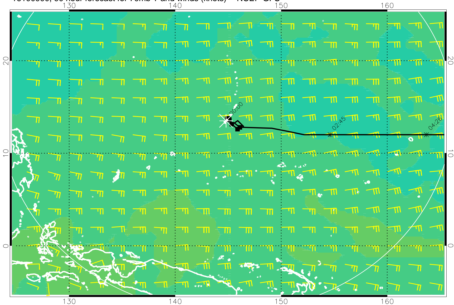
16100900, 90 hour forecast for 70mb T and winds (knots) -- NCEP GFS
