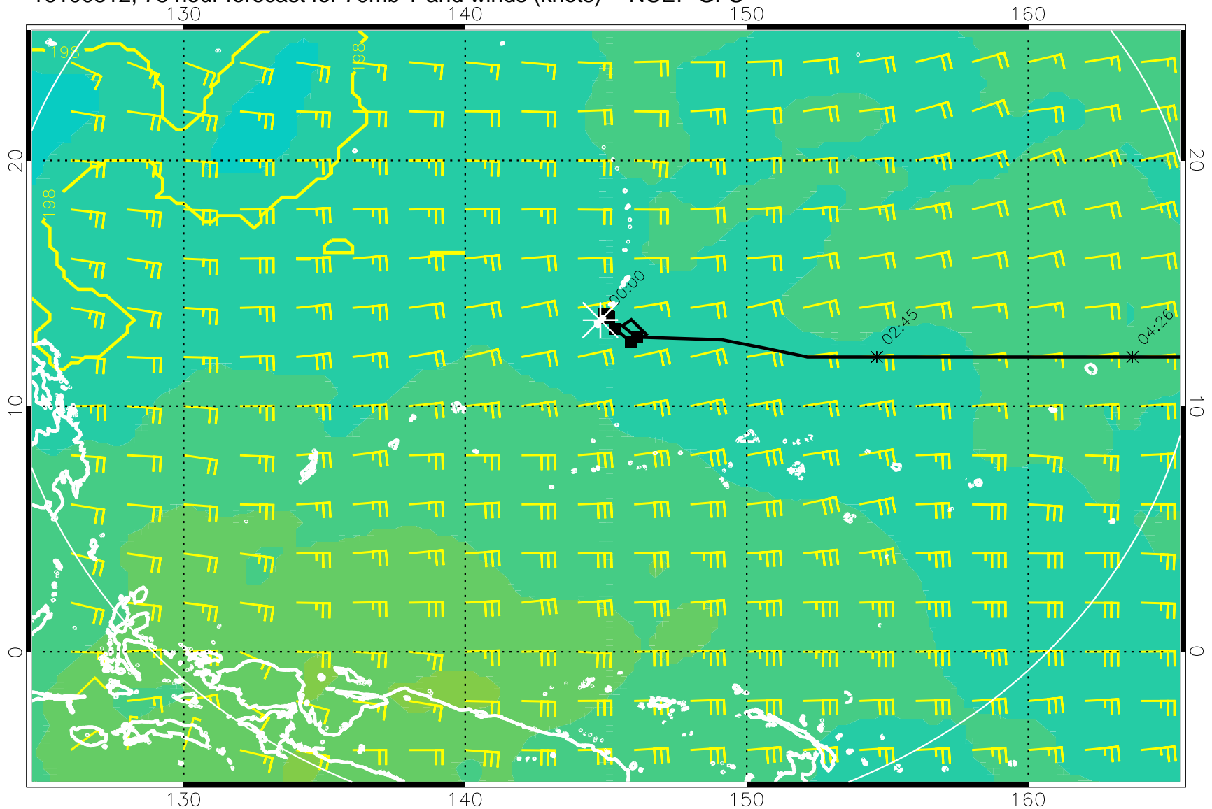
16100812, 78 hour forecast for 70mb T and winds (knots) -- NCEP GFS
