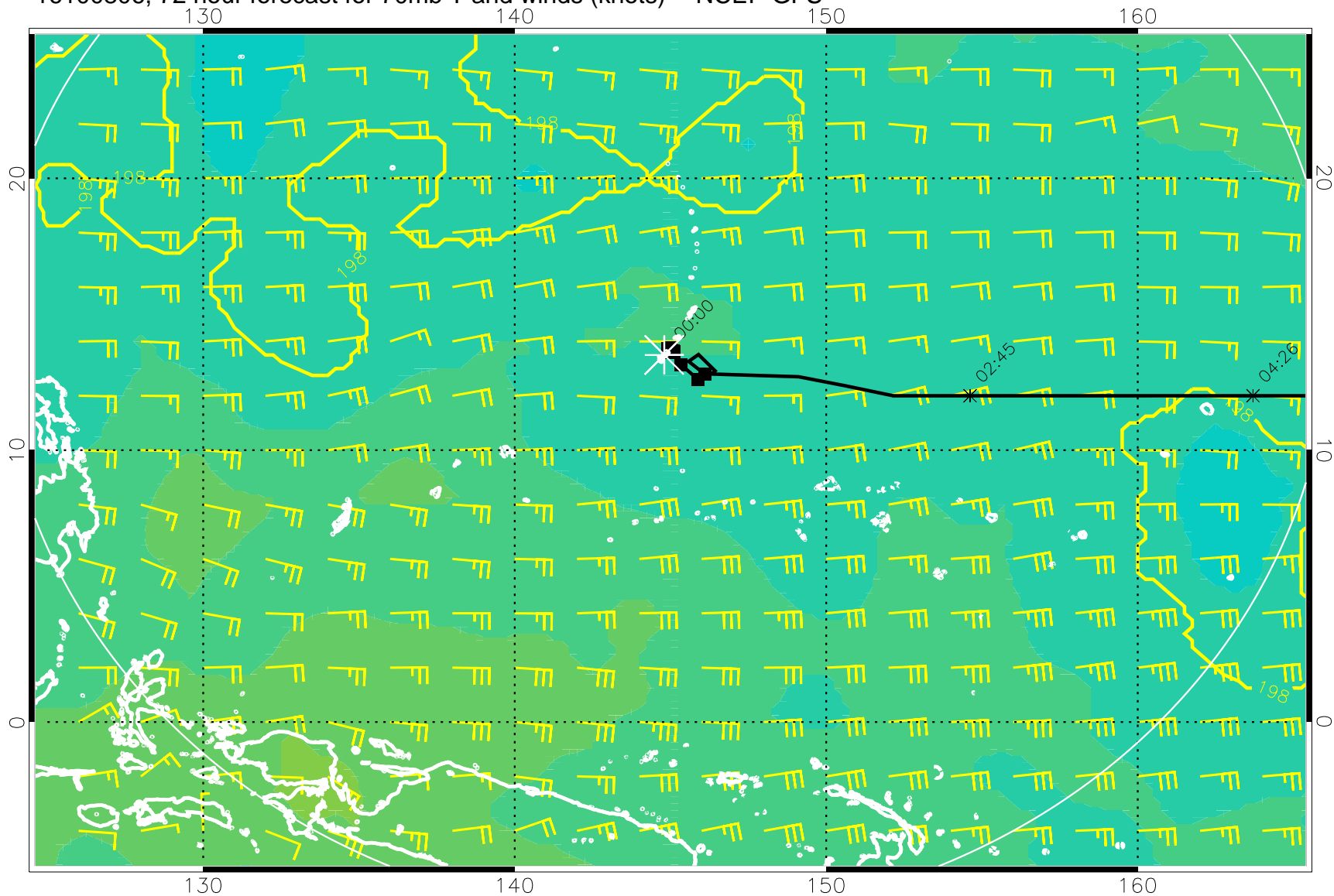
16100806, 72 hour forecast for 70mb T and winds (knots) -- NCEP GFS
