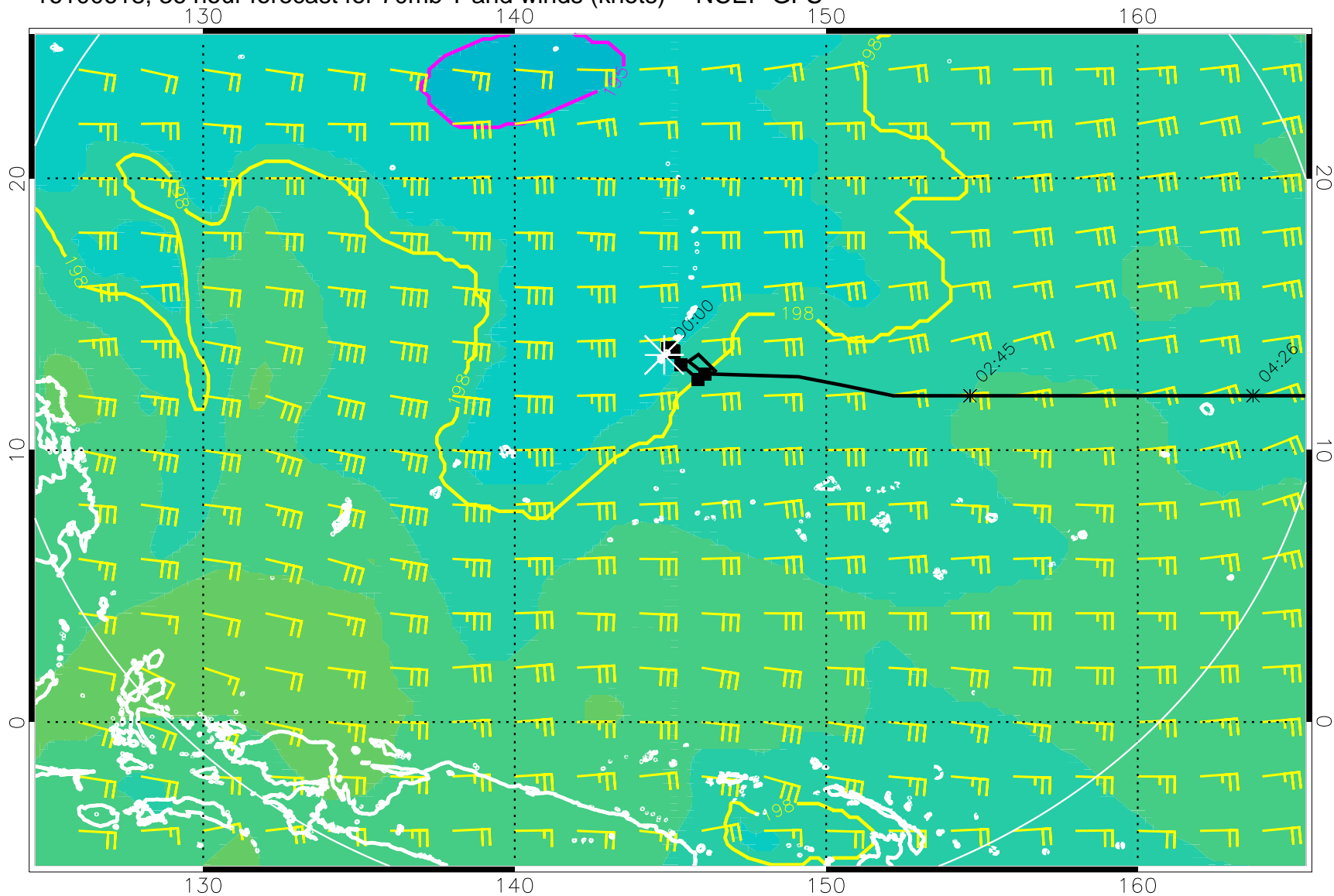
16100618, 36 hour forecast for 70mb T and winds (knots) -- NCEP GFS
