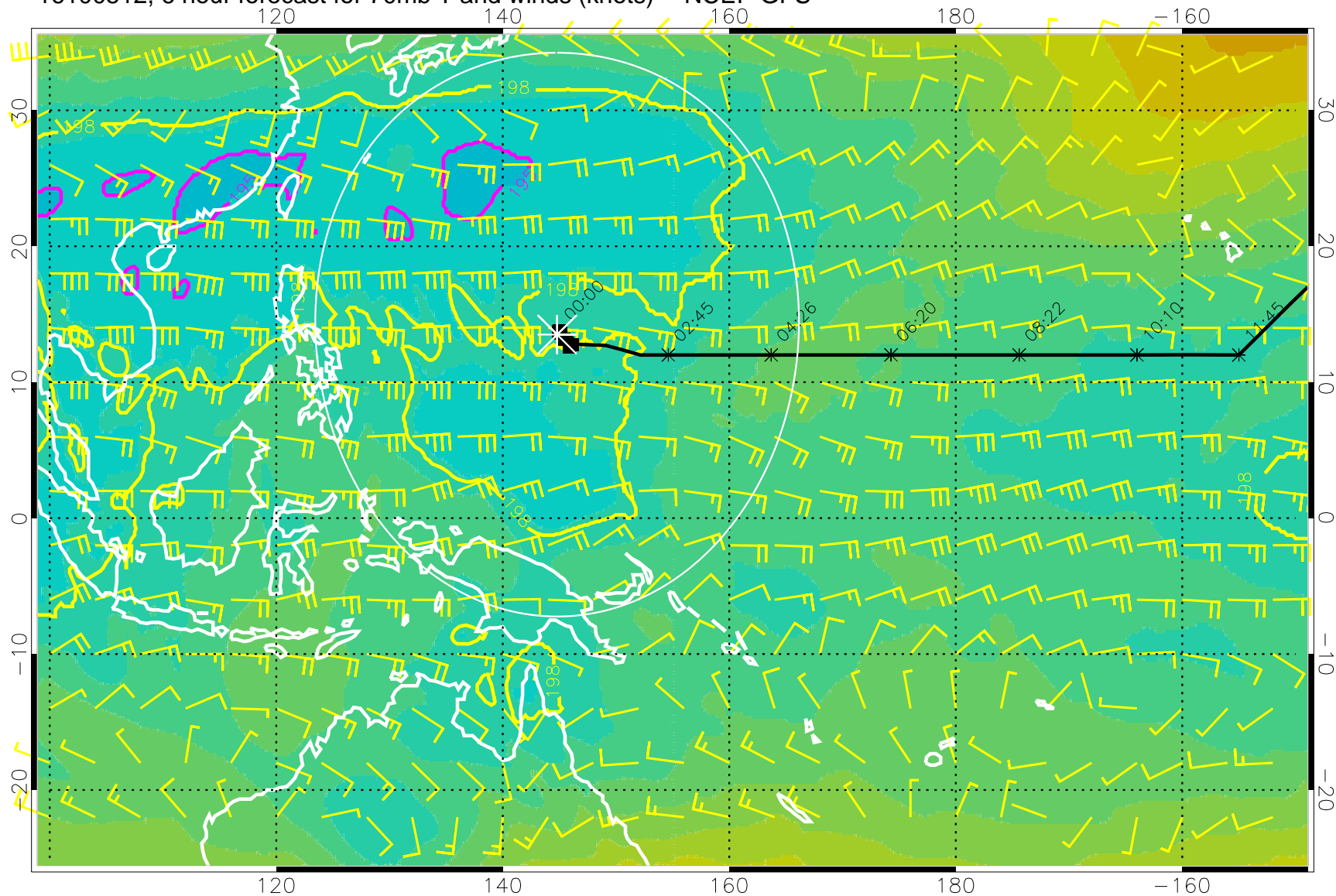
16100512, 6 hour forecast for 70mb T and winds (knots) -- NCEP GFS
