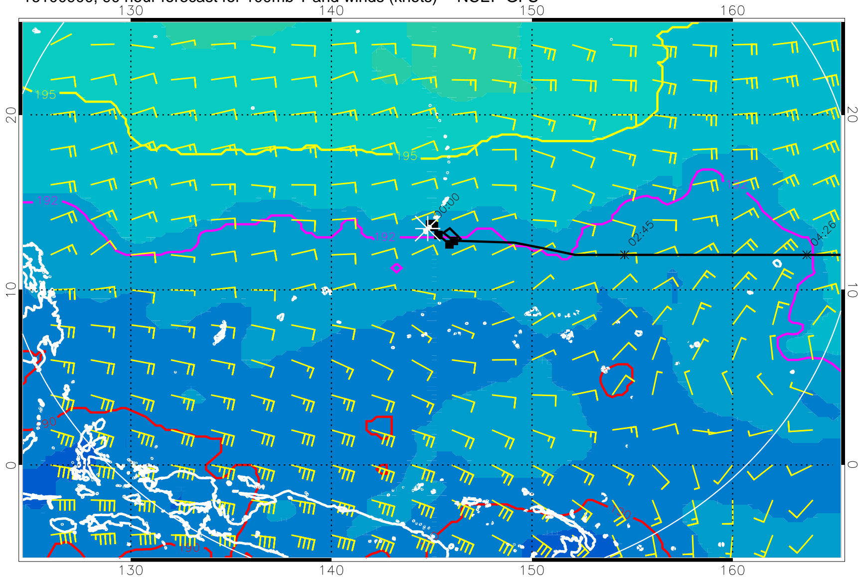
16100900, 90 hour forecast for 100mb T and winds (knots) -- NCEP GFS
