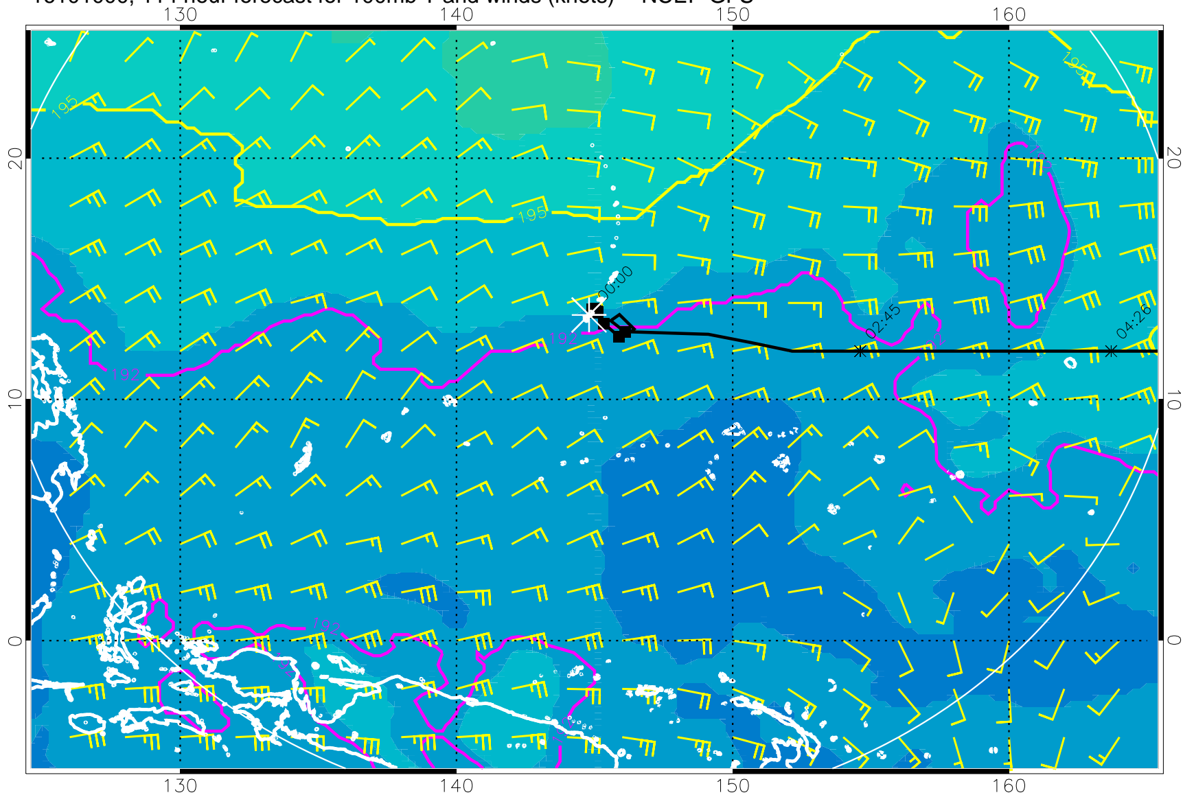
16101000, 114 hour forecast for 100mb T and winds (knots) -- NCEP GFS
