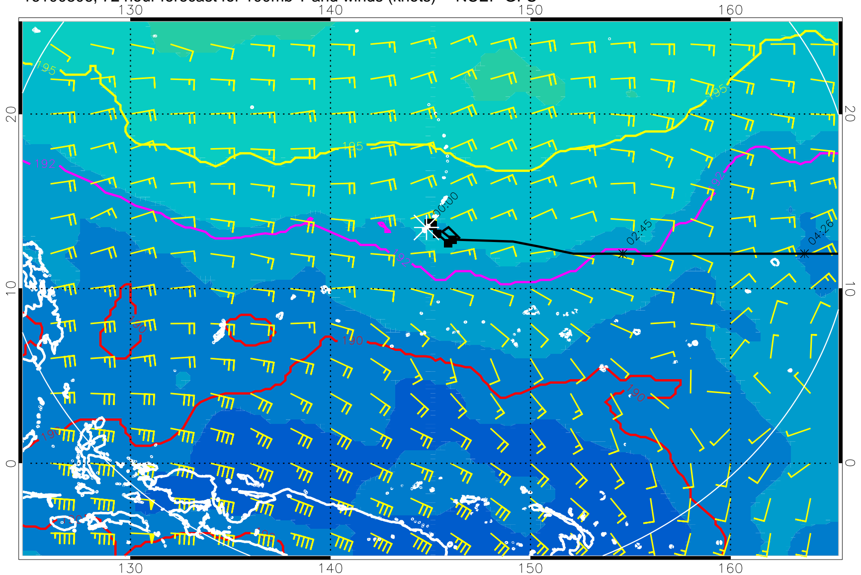
16100806, 72 hour forecast for 100mb T and winds (knots) -- NCEP GFS
