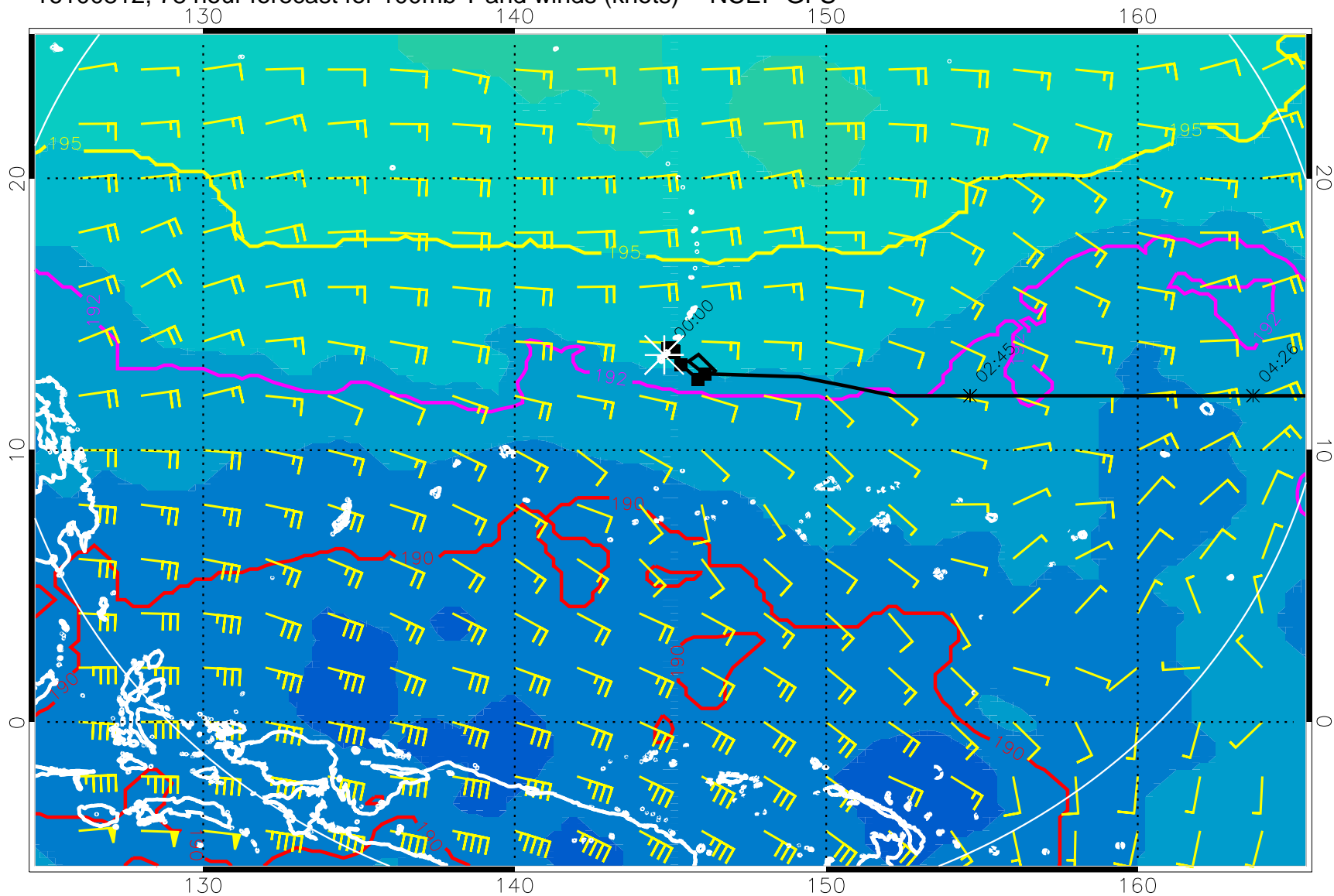
16100812, 78 hour forecast for 100mb T and winds (knots) -- NCEP GFS
