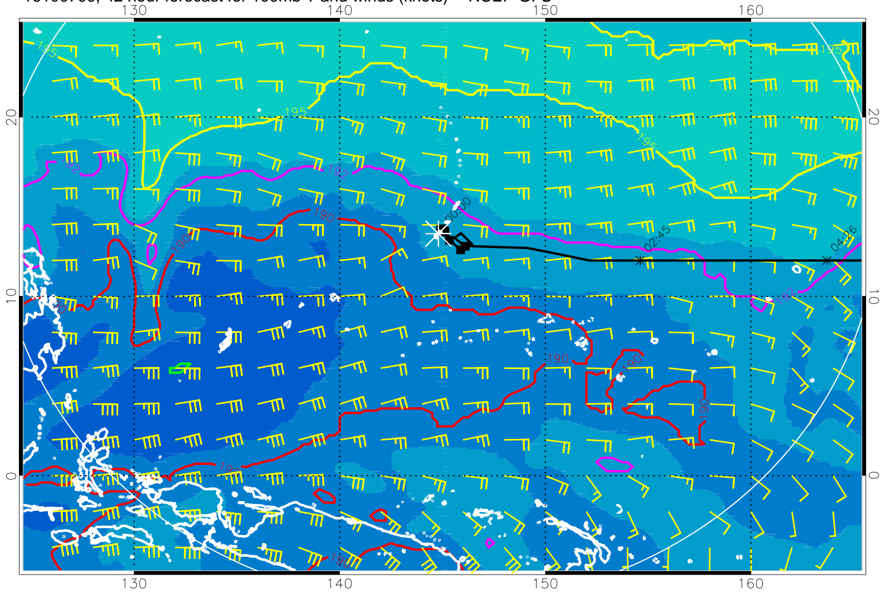
16100700, 42 hour forecast for 100mb T and winds (knots) -- NCEP GFS
