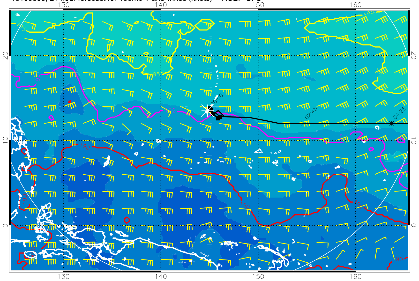
16100606, 24 hour forecast for 100mb T and winds (knots) -- NCEP GFS
