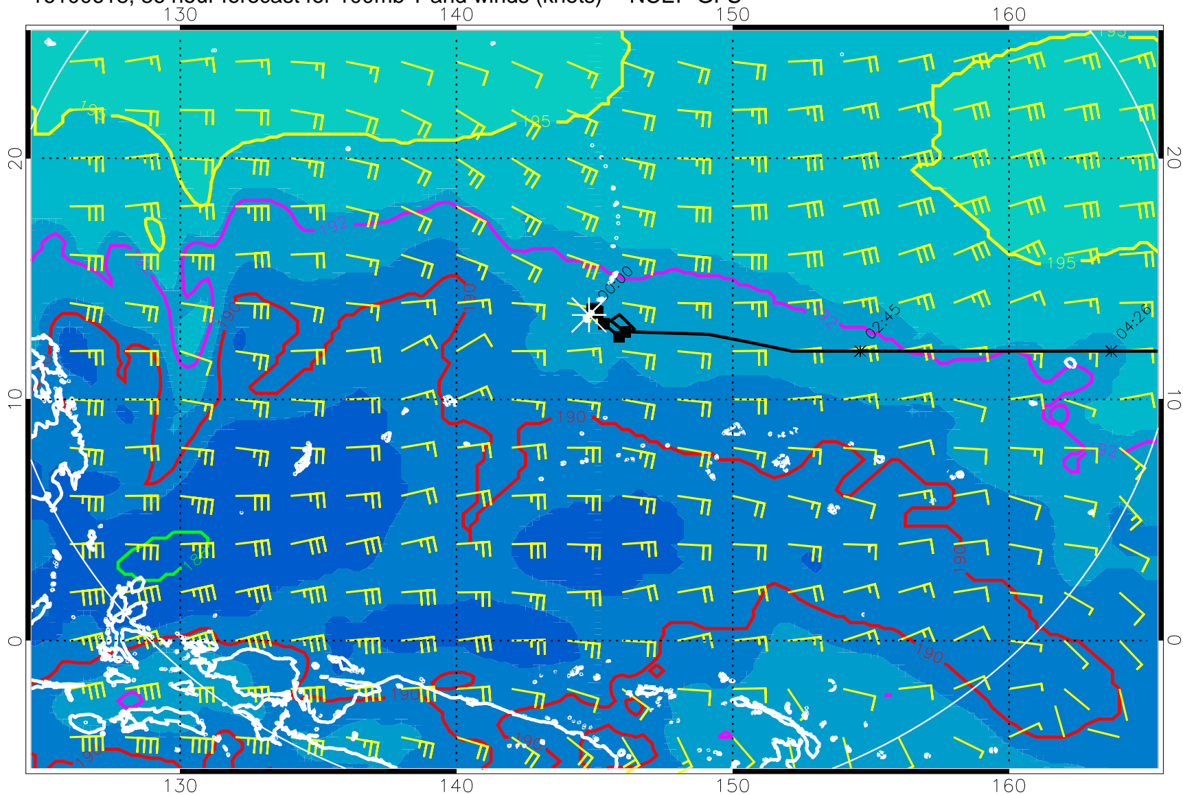
16100618, 36 hour forecast for 100mb T and winds (knots) -- NCEP GFS
