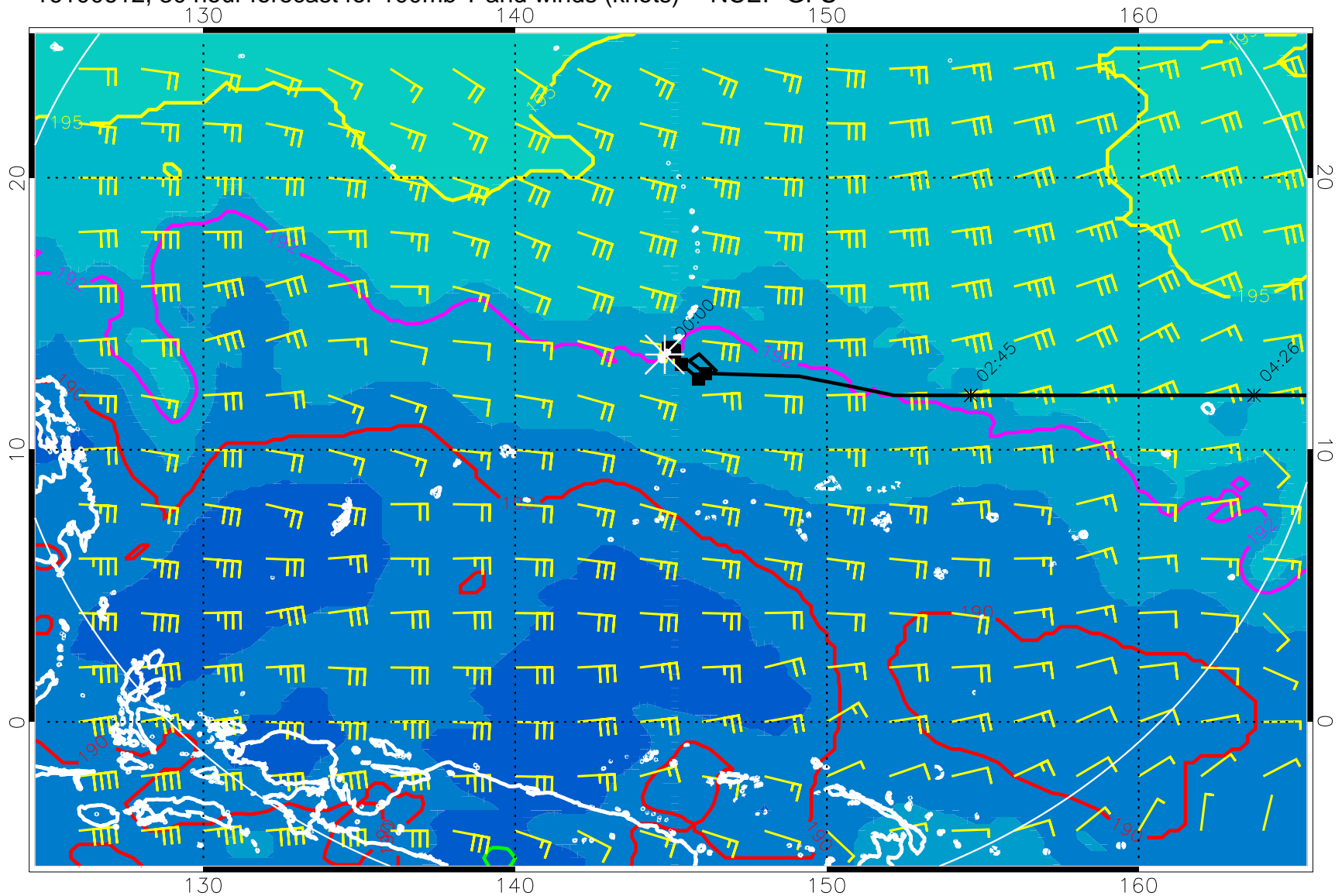
16100612, 30 hour forecast for 100mb T and winds (knots) -- NCEP GFS
