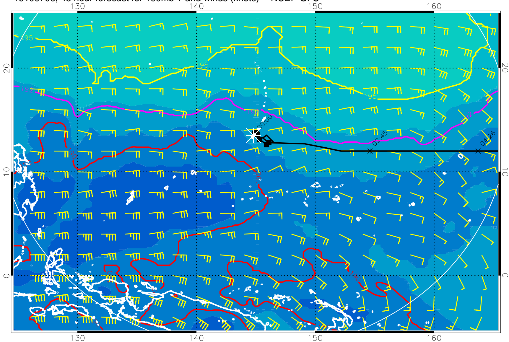
16100706, 48 hour forecast for 100mb T and winds (knots) -- NCEP GFS
