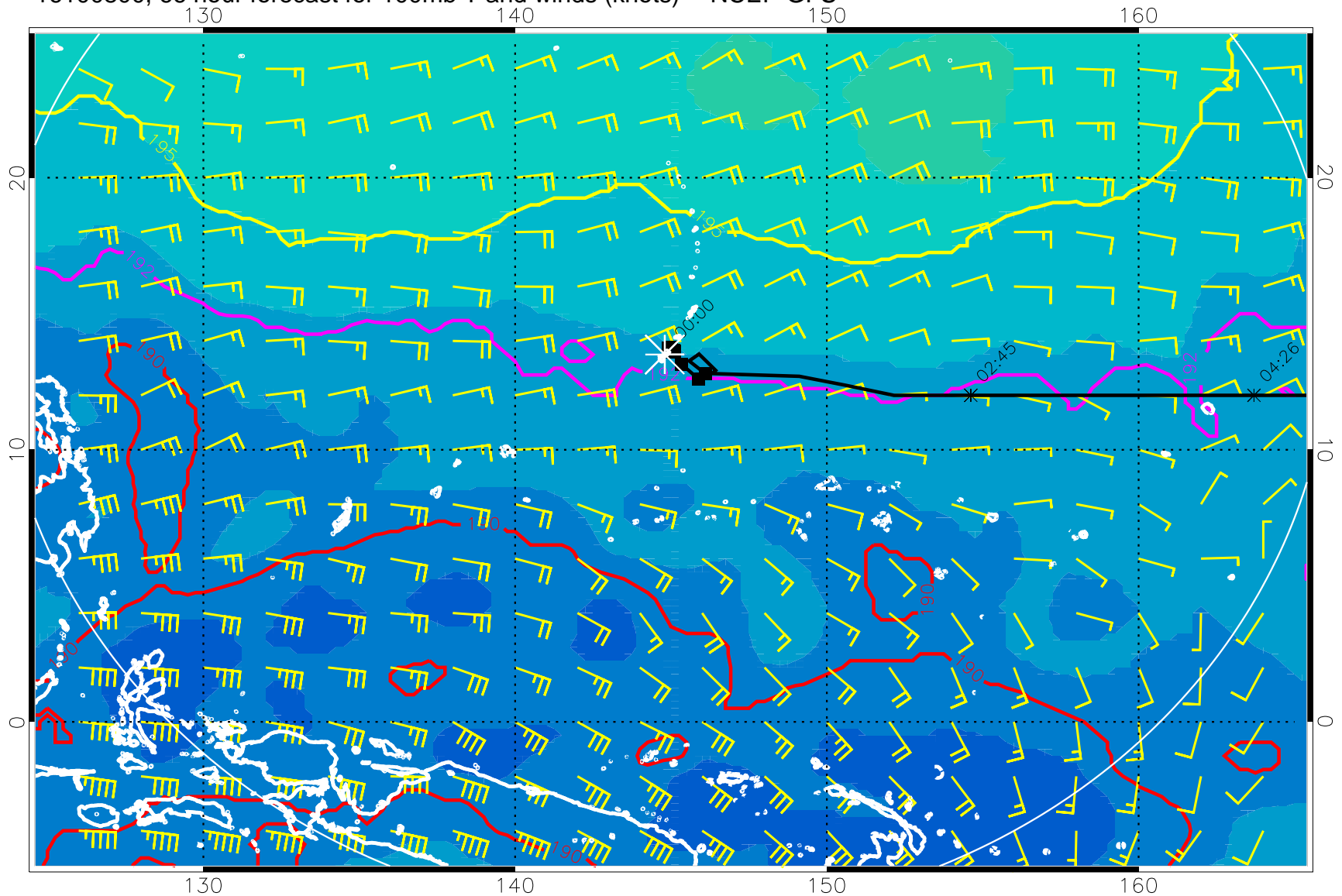
16100800, 66 hour forecast for 100mb T and winds (knots) -- NCEP GFS
