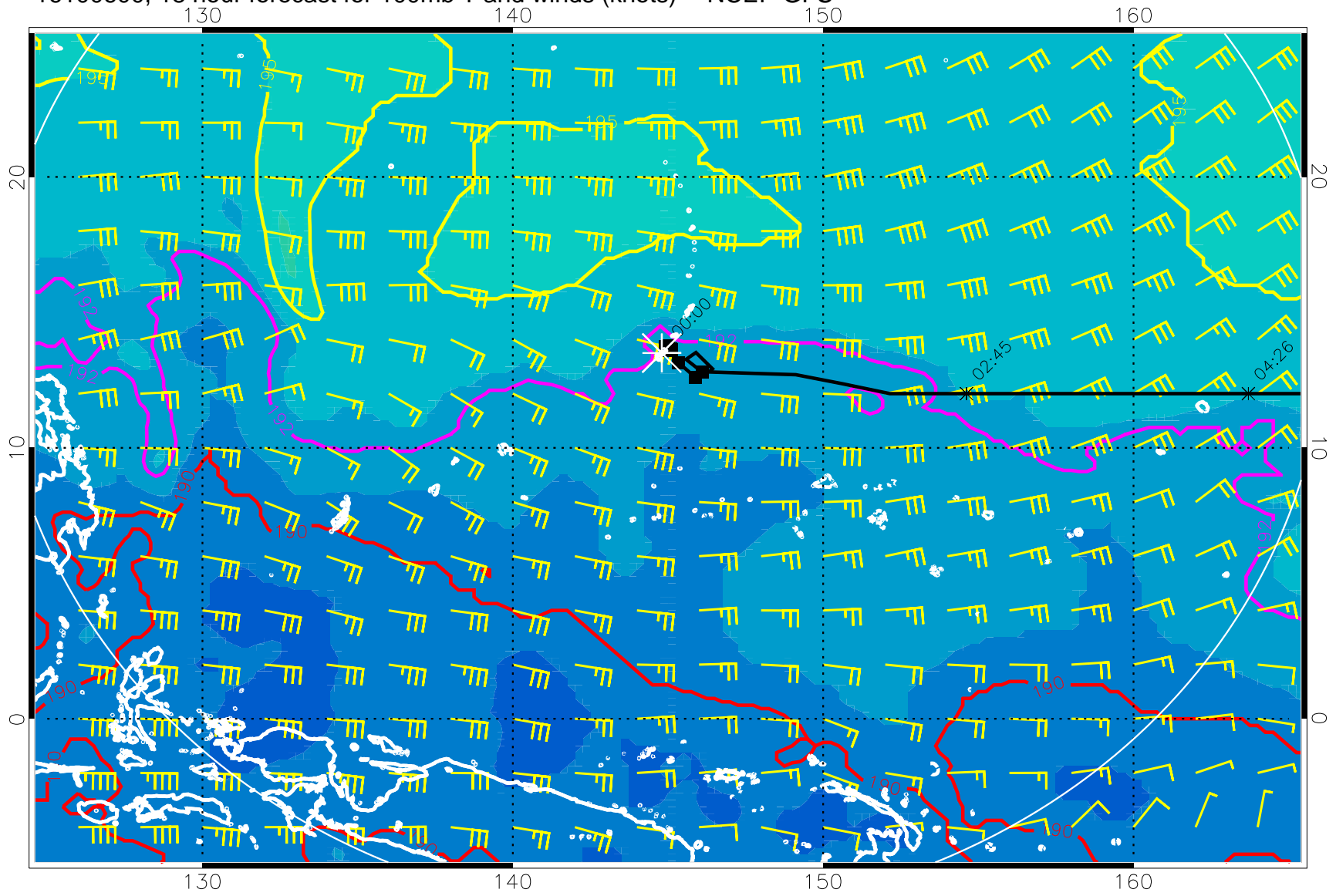
16100600, 18 hour forecast for 100mb T and winds (knots) -- NCEP GFS
