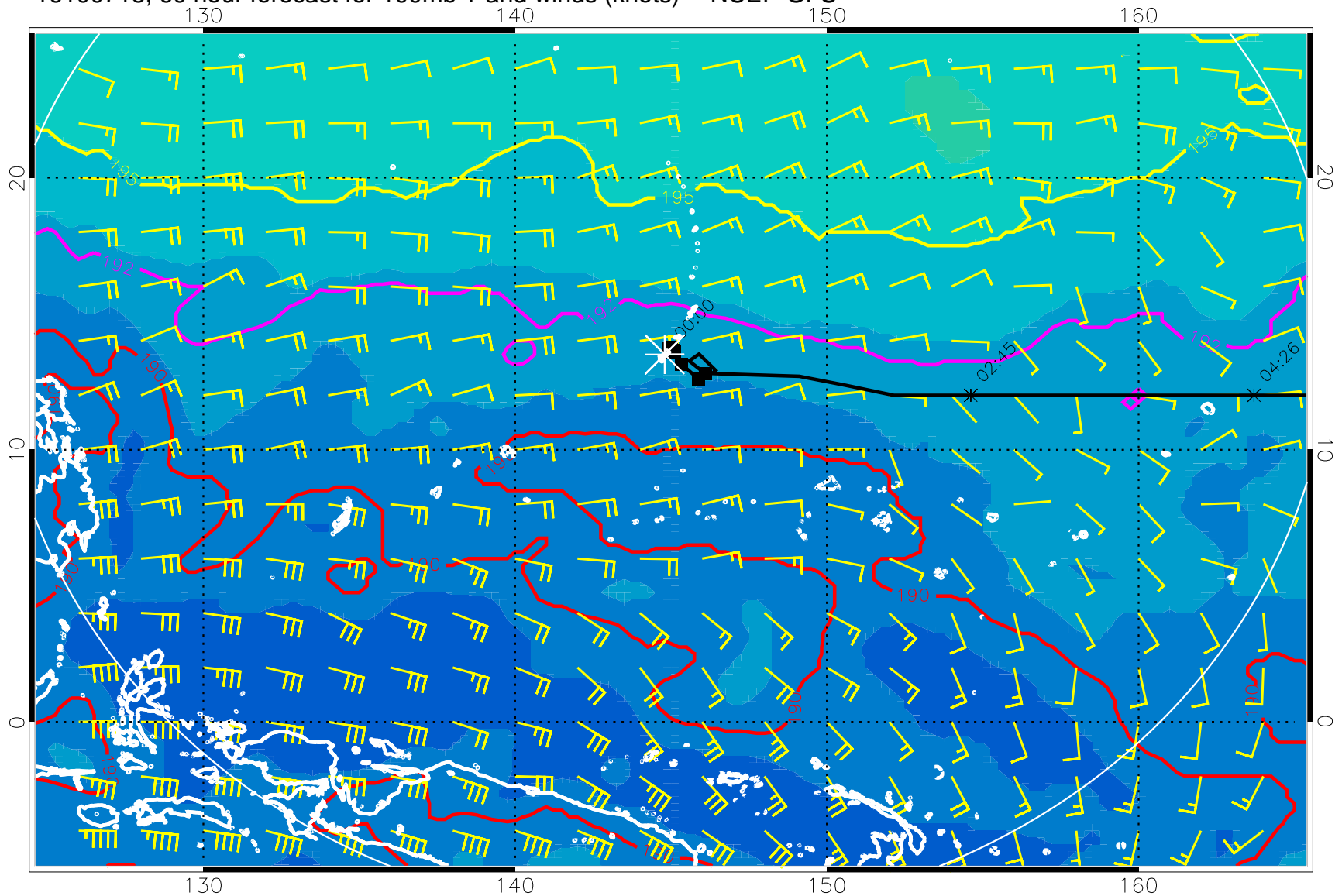
16100718, 60 hour forecast for 100mb T and winds (knots) -- NCEP GFS
