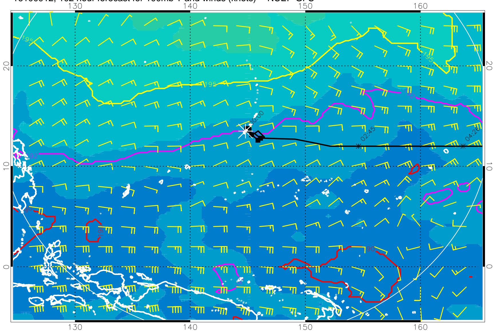
16100912, 102 hour forecast for 100mb T and winds (knots) -- NCEP GFS
