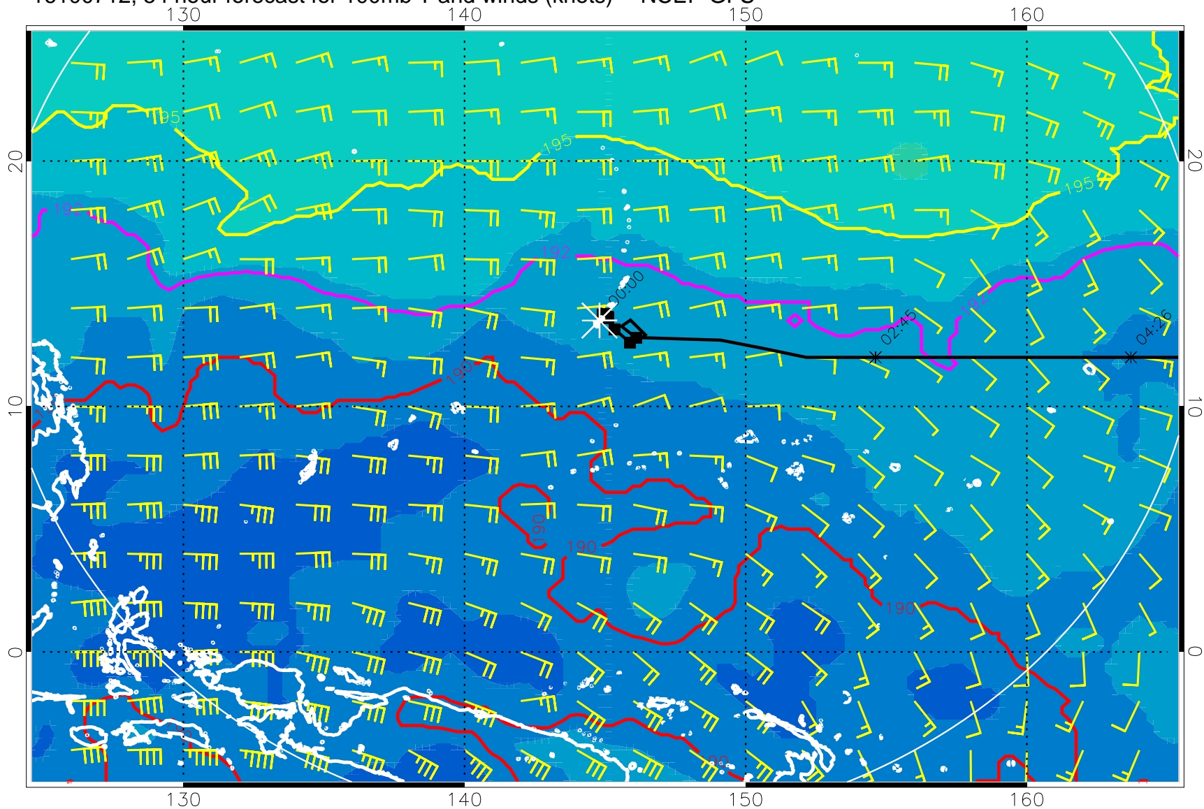
16100712, 54 hour forecast for 100mb T and winds (knots) -- NCEP GFS
