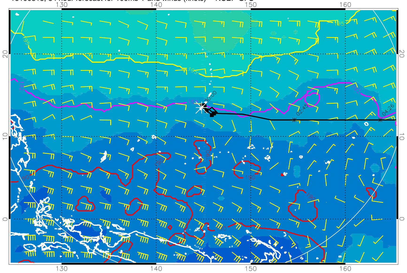
16100818, 84 hour forecast for 100mb T and winds (knots) -- NCEP GFS
