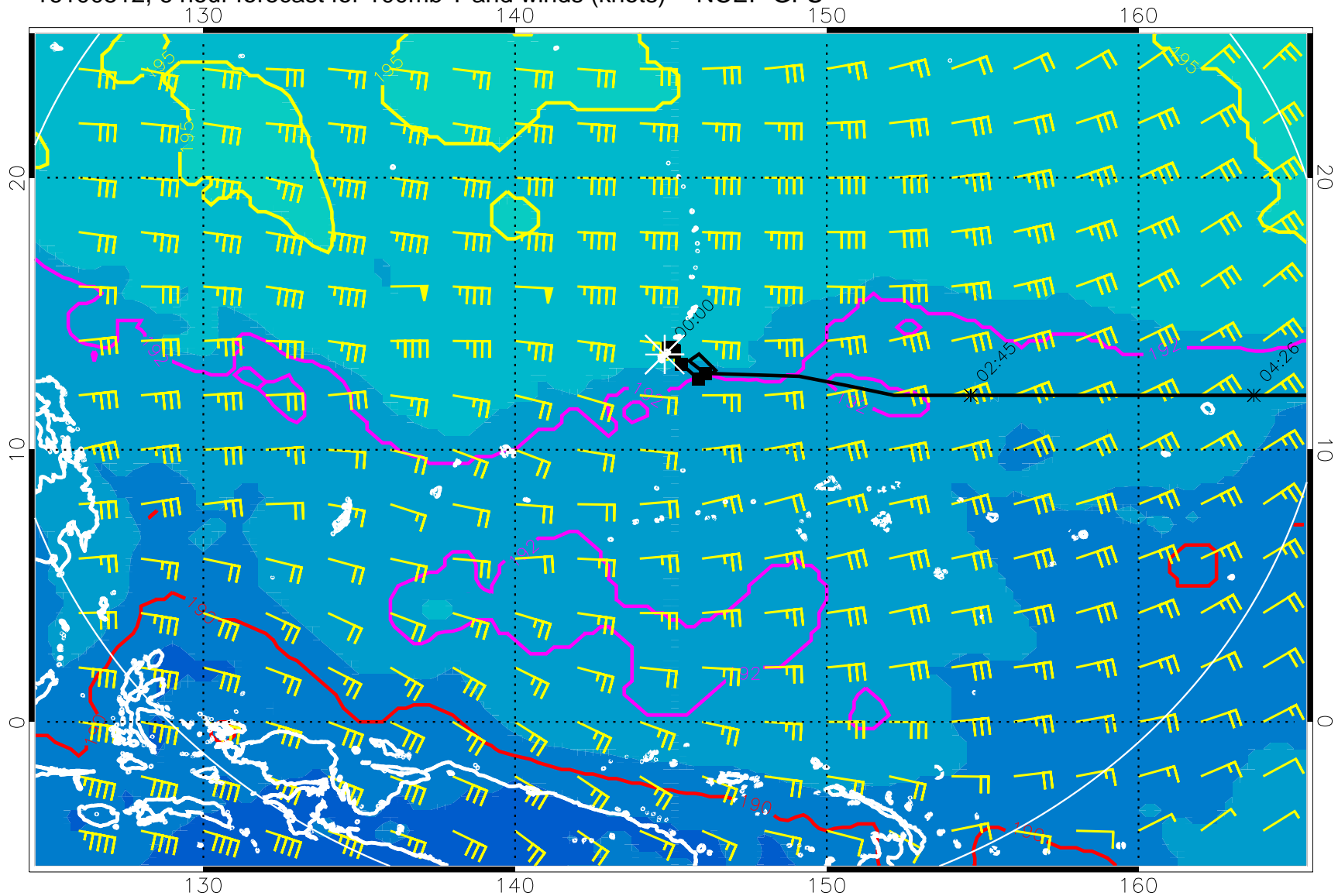
16100512, 6 hour forecast for 100mb T and winds (knots) -- NCEP GFS
