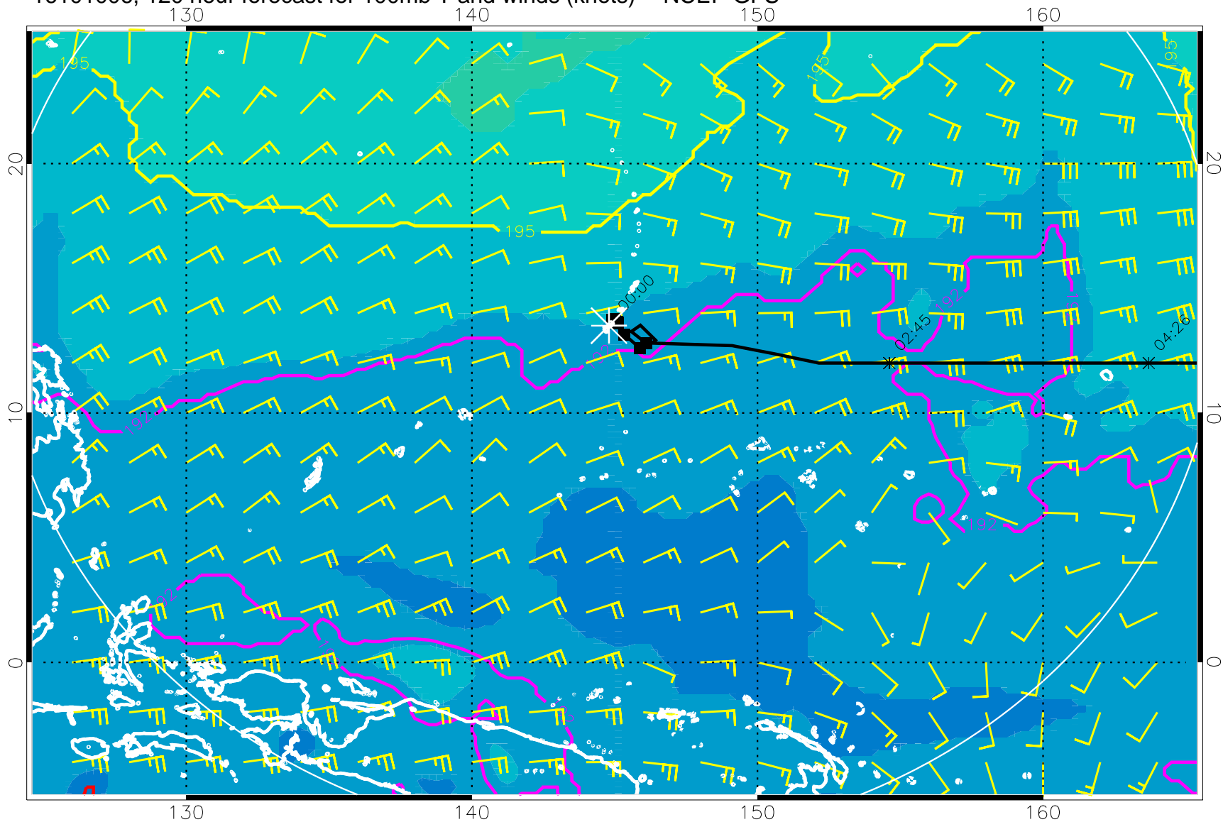
16101006, 120 hour forecast for 100mb T and winds (knots) -- NCEP GFS
