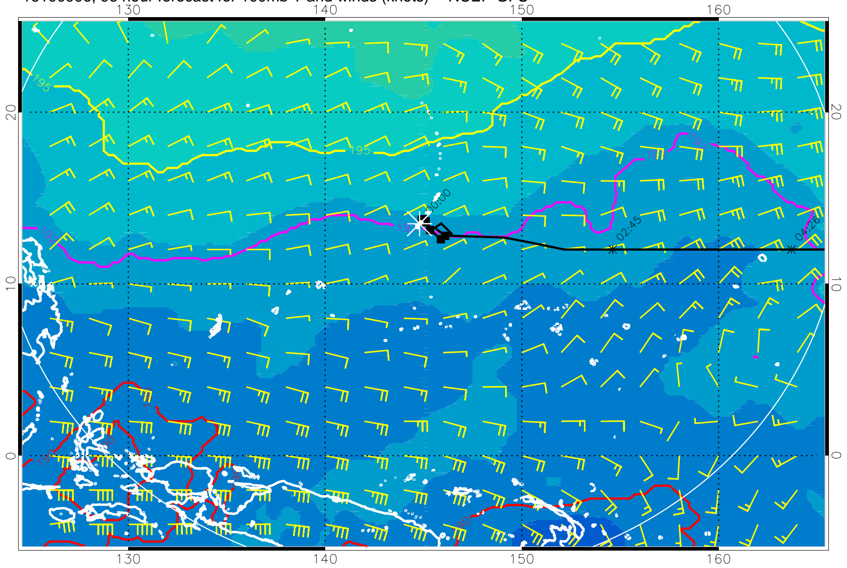
16100906, 96 hour forecast for 100mb T and winds (knots) -- NCEP GFS
