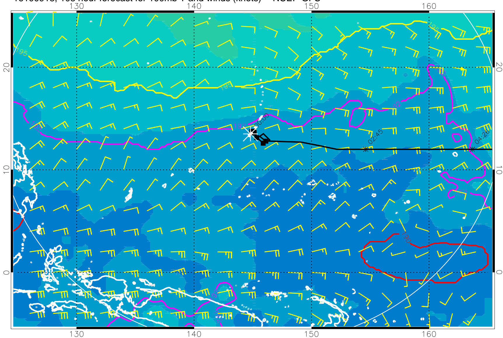
16100918, 108 hour forecast for 100mb T and winds (knots) -- NCEP GFS
