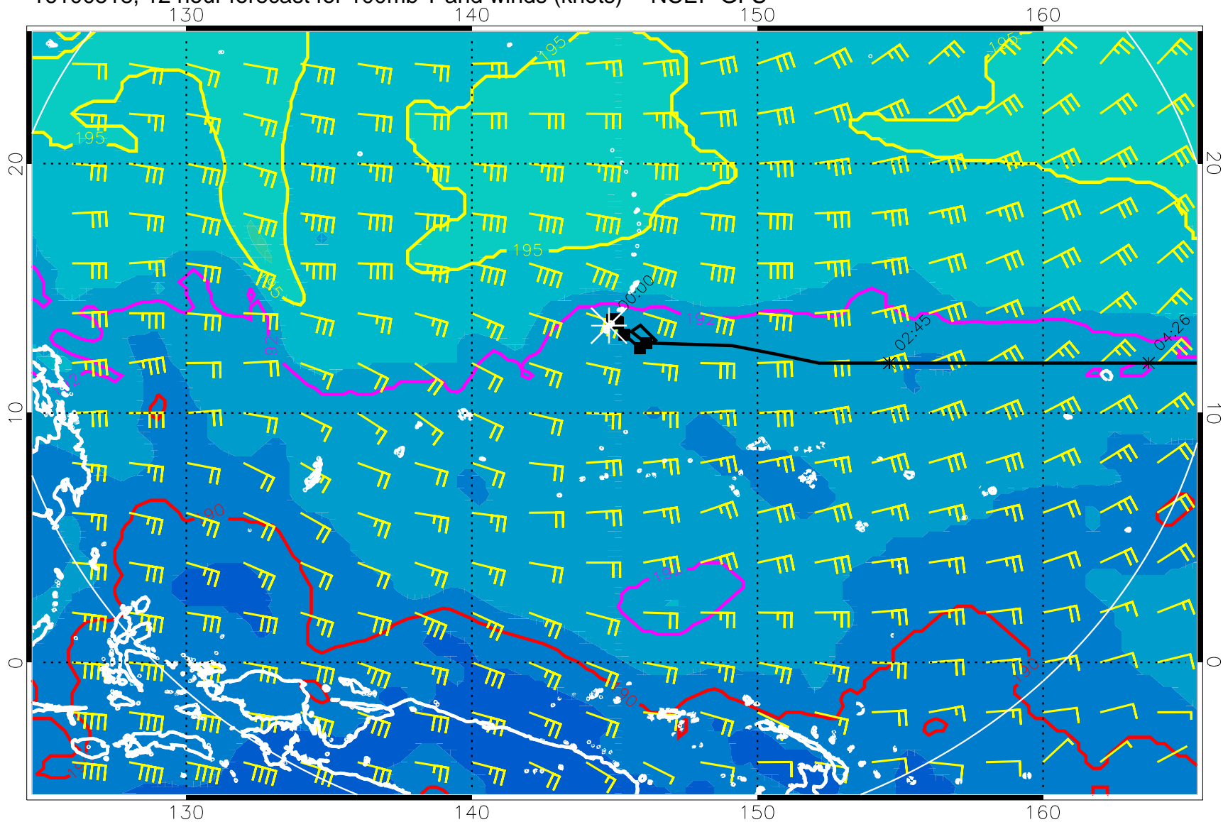
16100518, 12 hour forecast for 100mb T and winds (knots) -- NCEP GFS
