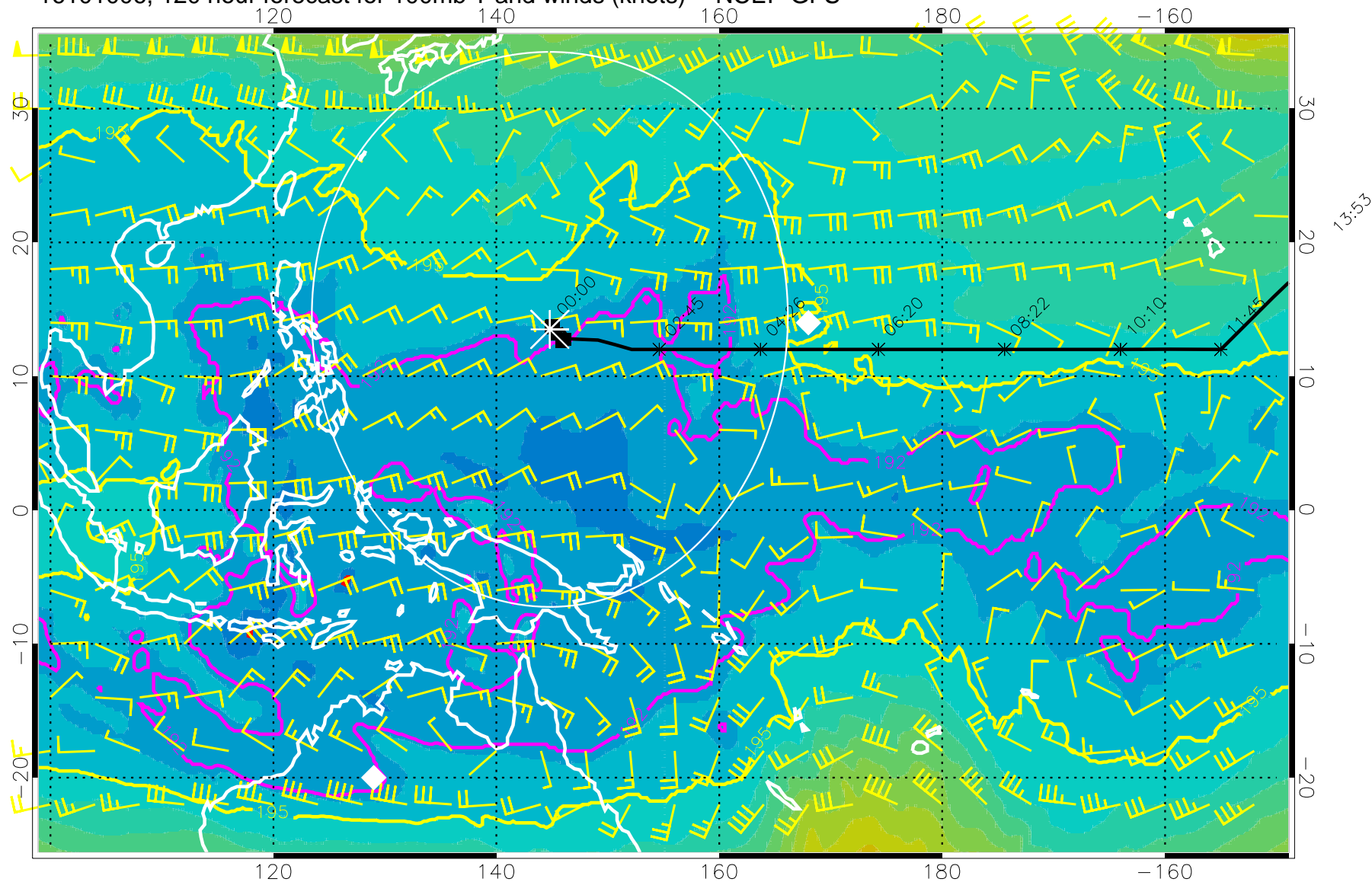
16101006, 120 hour forecast for 100mb T and winds (knots) -- NCEP GFS
