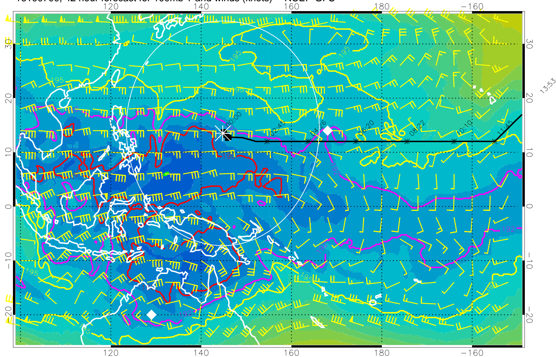
16100700, 42 hour forecast for 100mb T and winds (knots) -- NCEP GFS
