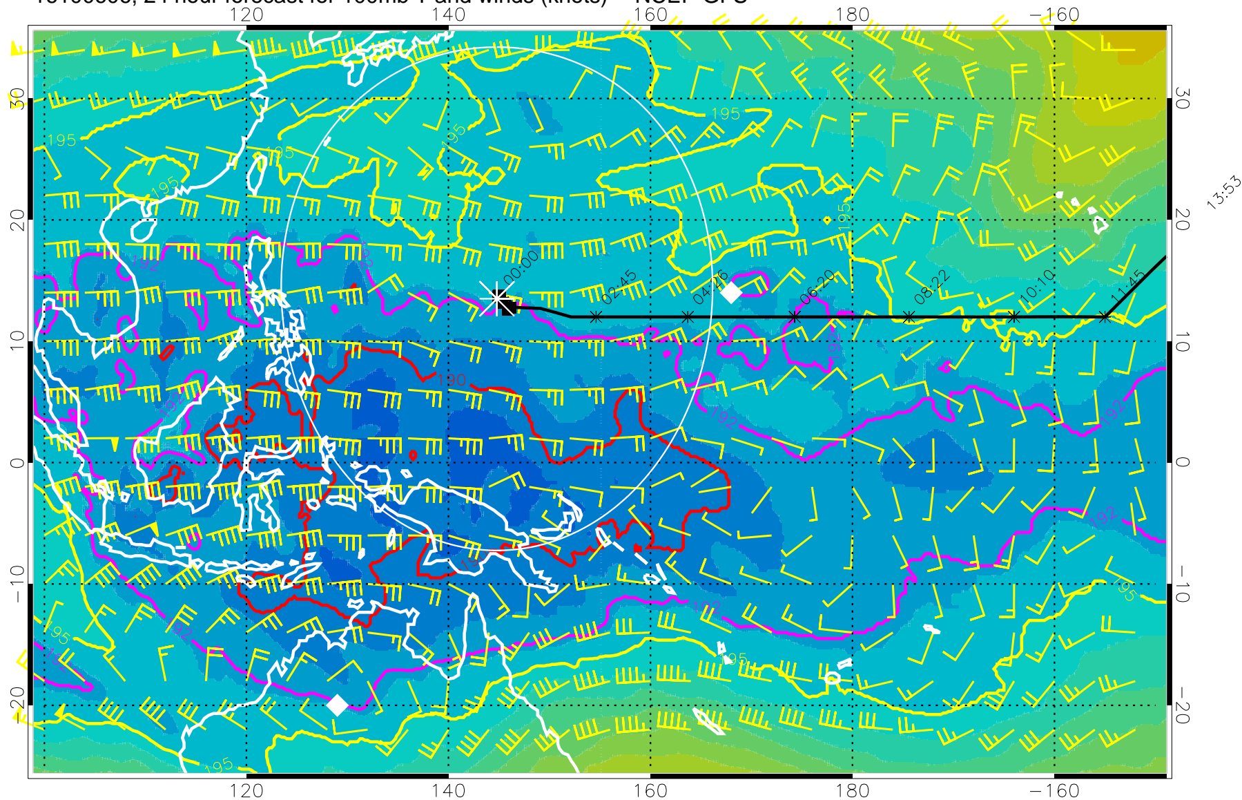
16100606, 24 hour forecast for 100mb T and winds (knots) -- NCEP GFS
