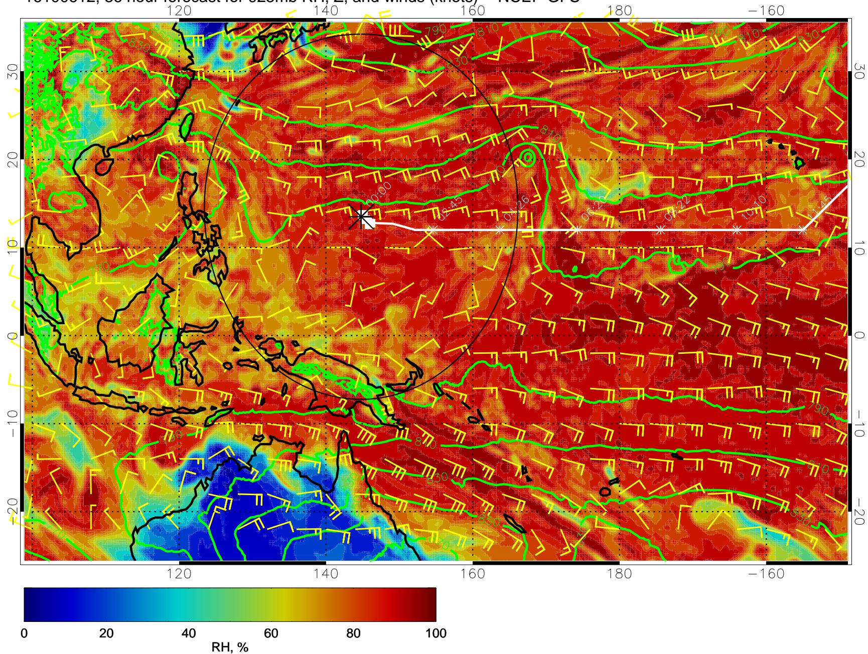
16100612, 36 hour forecast for 925mb RH, Z, and winds (knots) -- NCEP GFS
