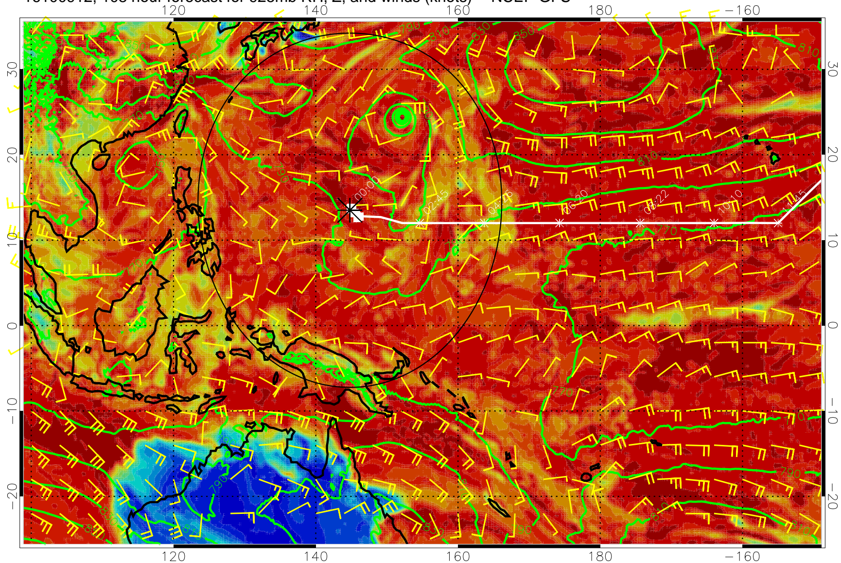
16100912, 108 hour forecast for 925mb RH, Z, and winds (knots) -- NCEP GFS
