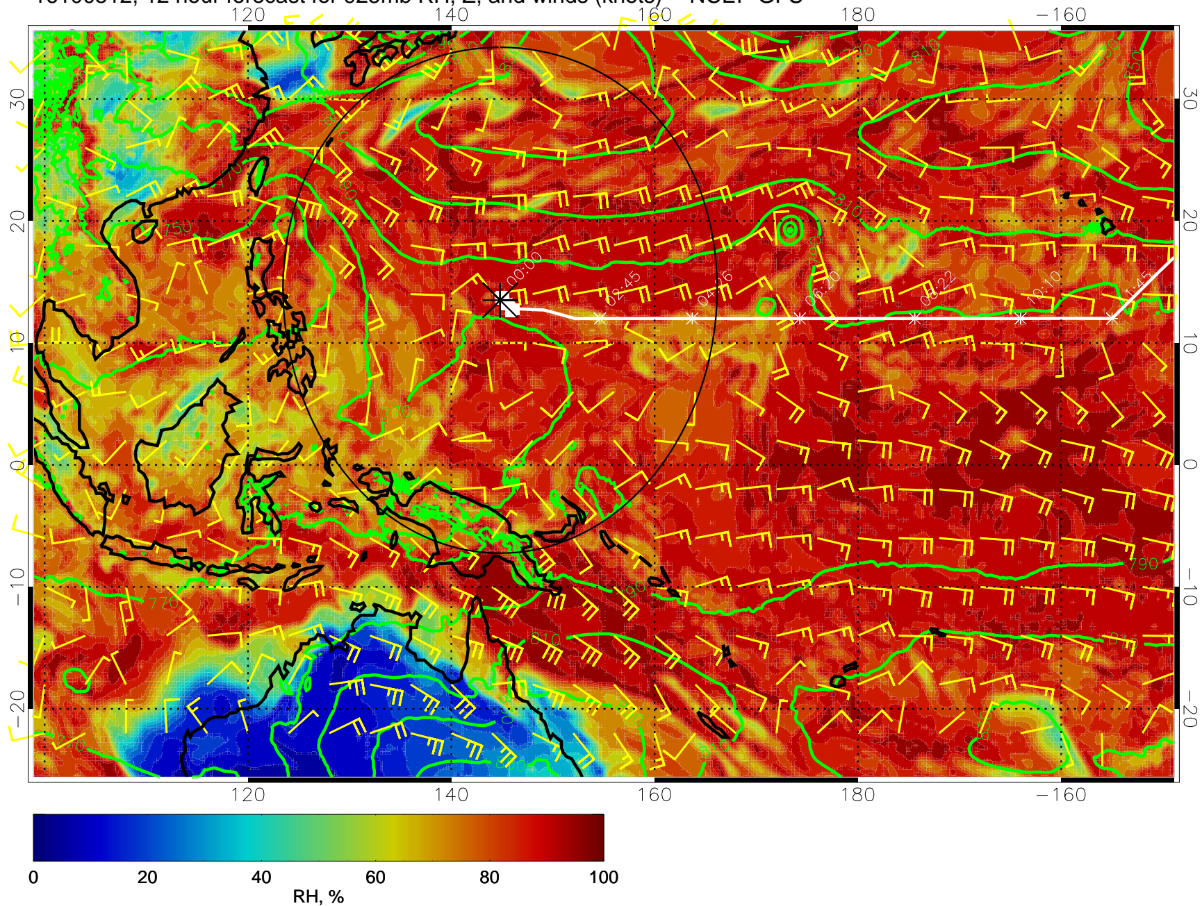
16100512, 12 hour forecast for 925mb RH, Z, and winds (knots) -- NCEP GFS
