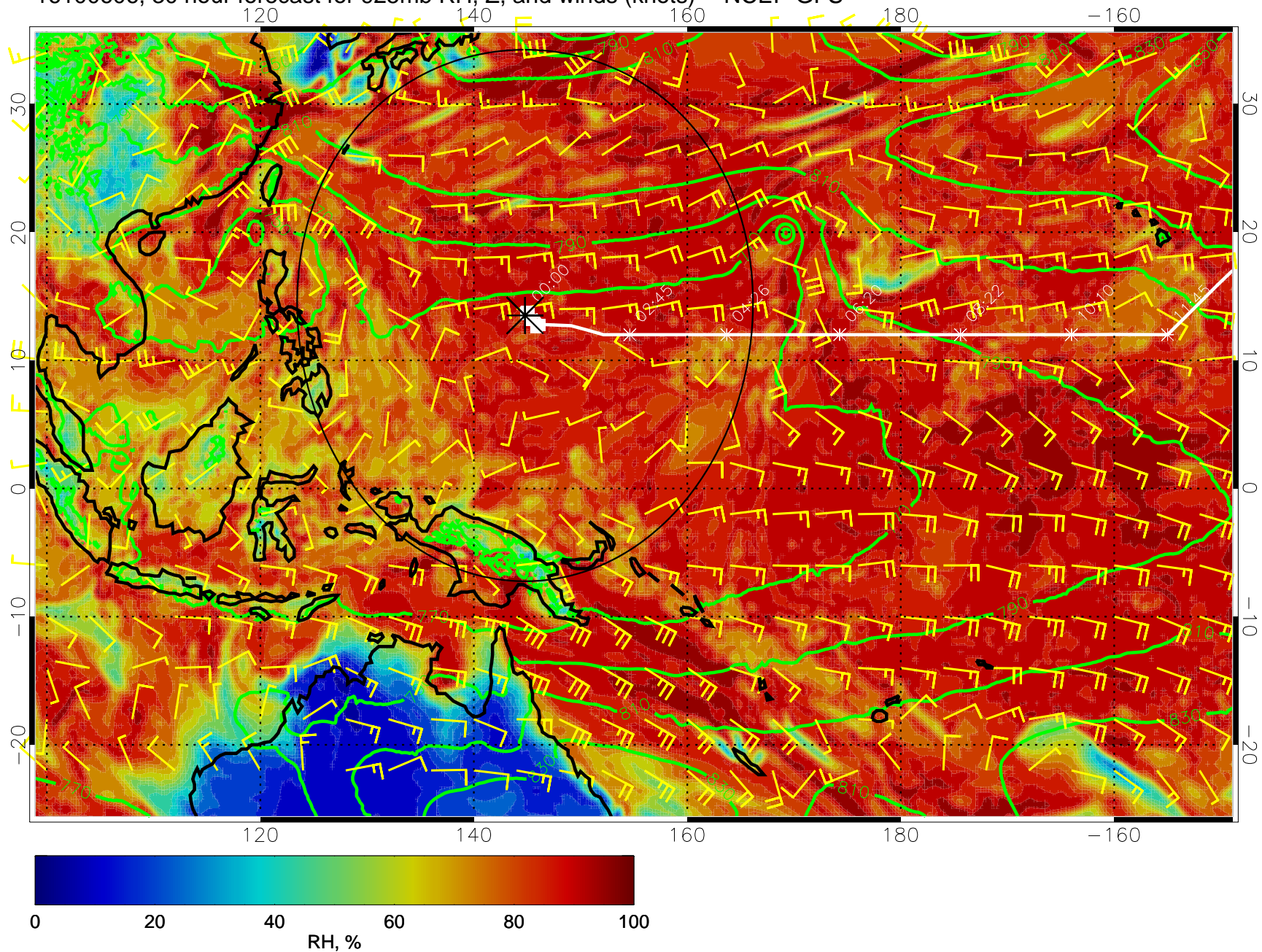
16100606, 30 hour forecast for 925mb RH, Z, and winds (knots) -- NCEP GFS
