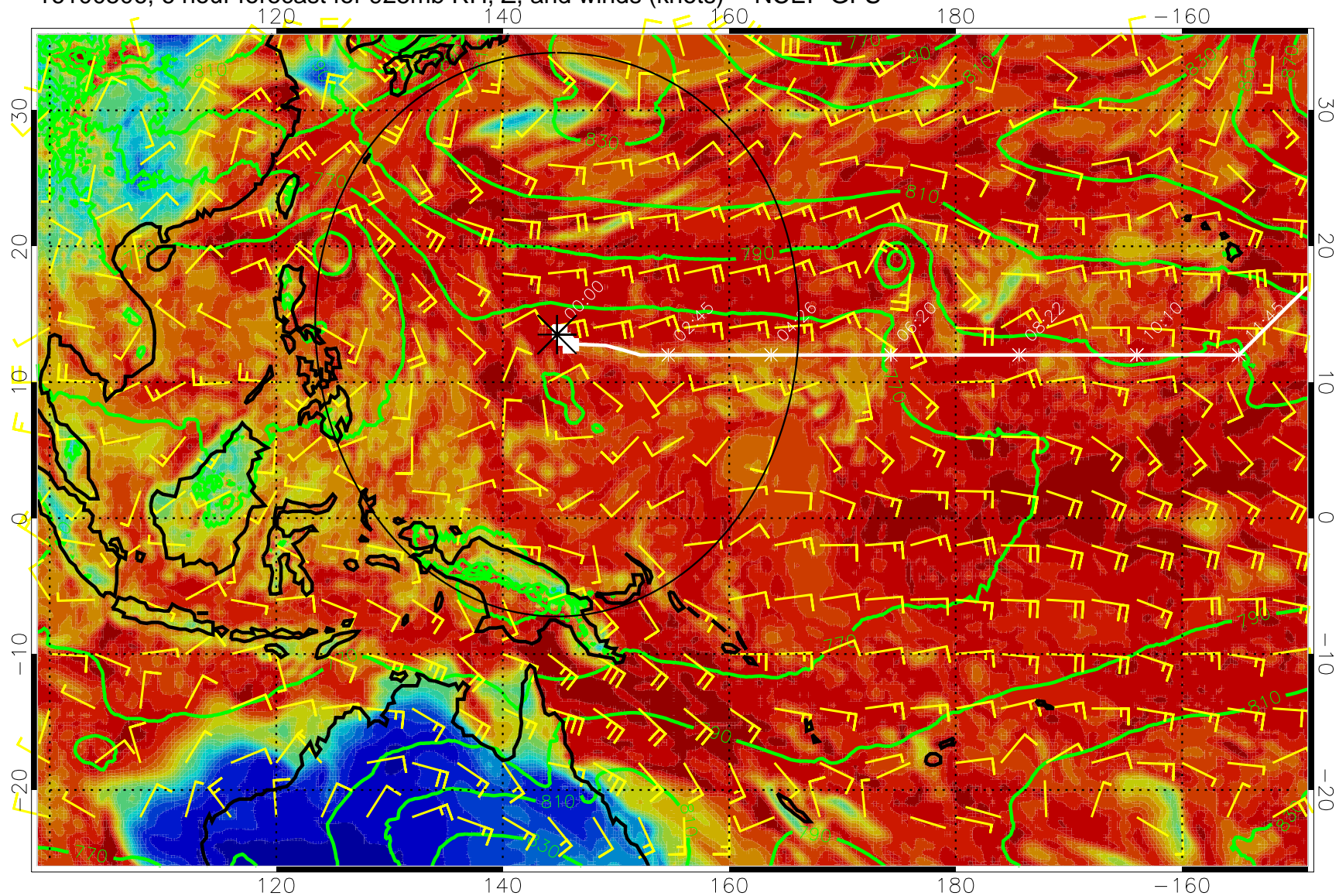
16100506, 6 hour forecast for 925mb RH, Z, and winds (knots) -- NCEP GFS
