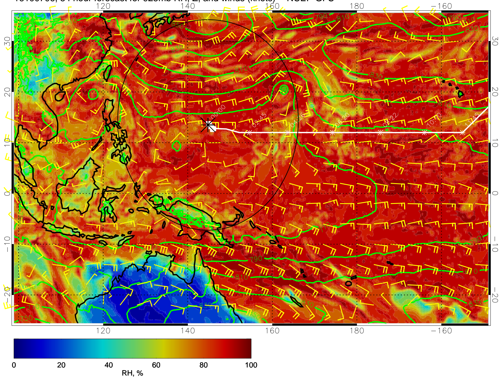
16100706, 54 hour forecast for 925mb RH, Z, and winds (knots) -- NCEP GFS
