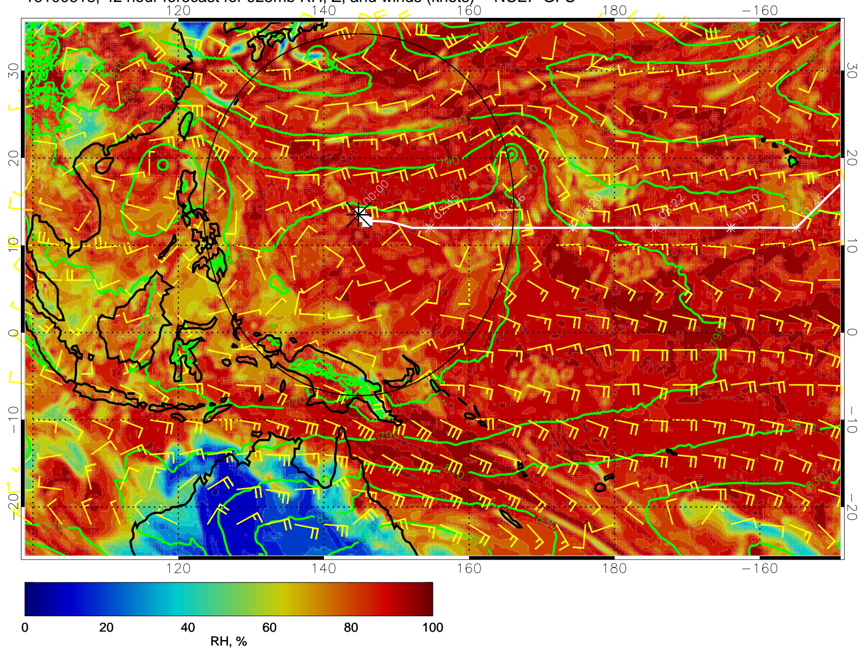
16100618, 42 hour forecast for 925mb RH, Z, and winds (knots) -- NCEP GFS
