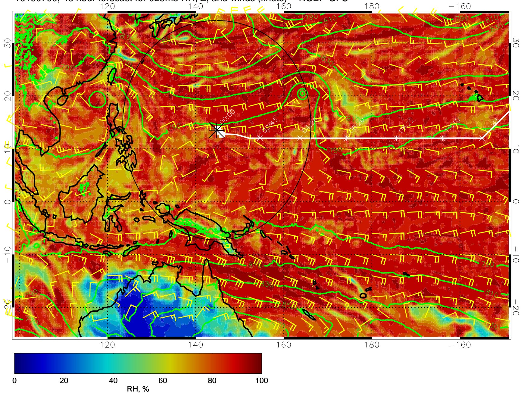
16100700, 48 hour forecast for 925mb RH, Z, and winds (knots) -- NCEP GFS
