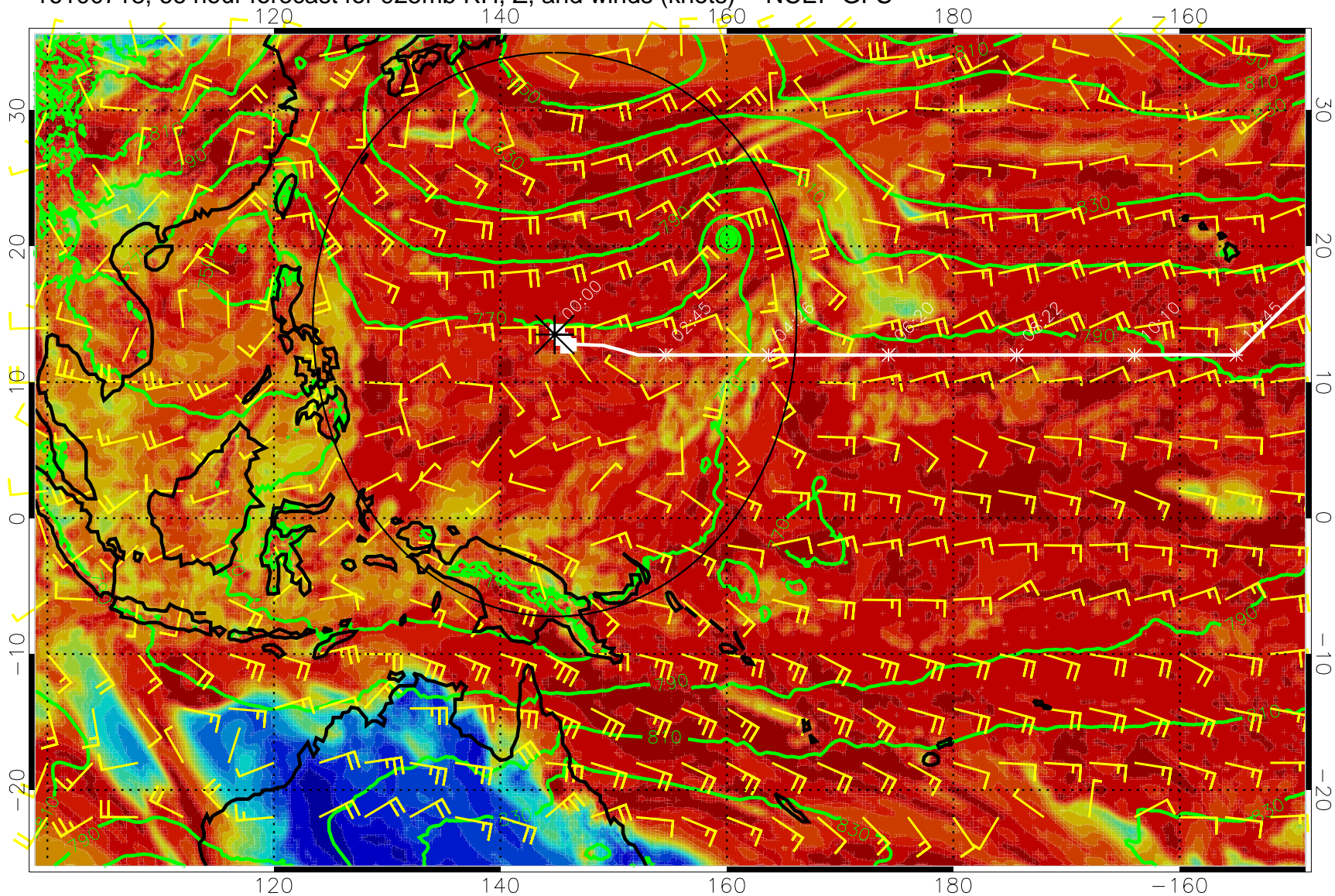
16100718, 66 hour forecast for 925mb RH, Z, and winds (knots) -- NCEP GFS
