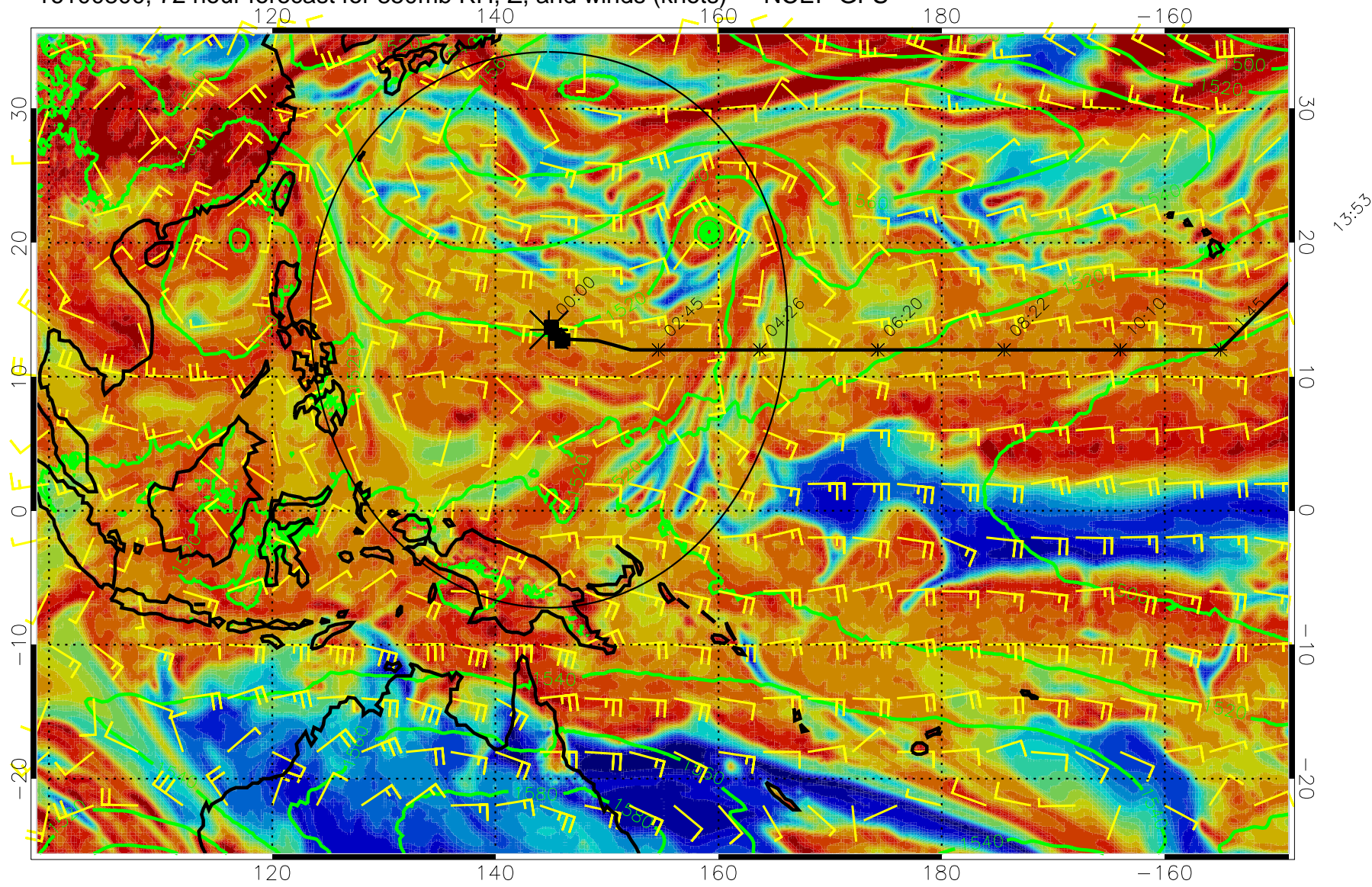
Precip (tot dot, conv sol) mm/day 40 mm/day contours, min 20
