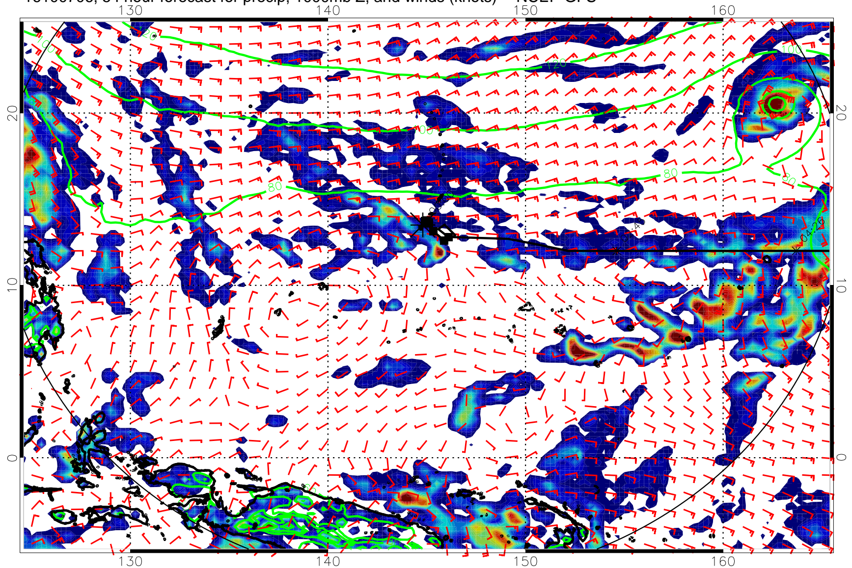
16100706, 54 hour forecast for precip, 1000mb Z, and winds (knots) -- NCEP GFS
