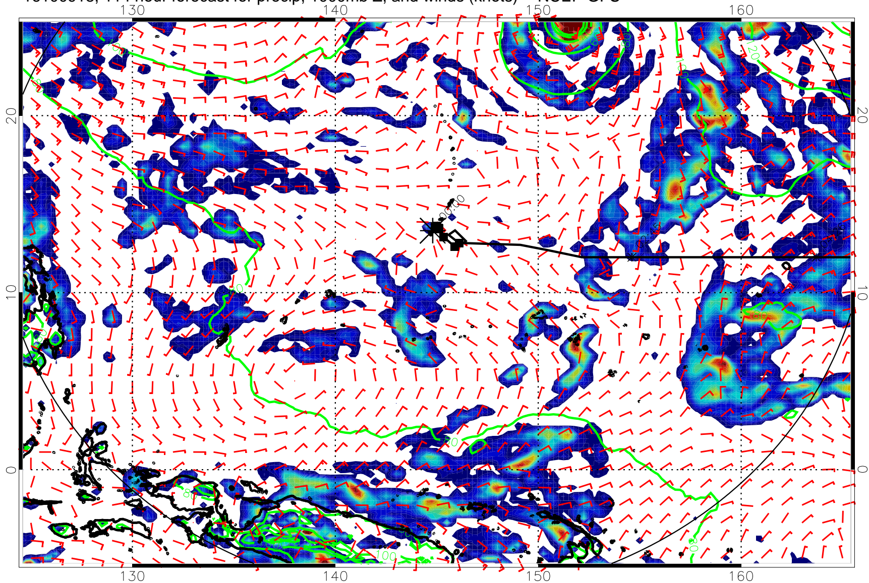
16100918, 114 hour forecast for precip, 1000mb Z, and winds (knots) -- NCEP GFS
