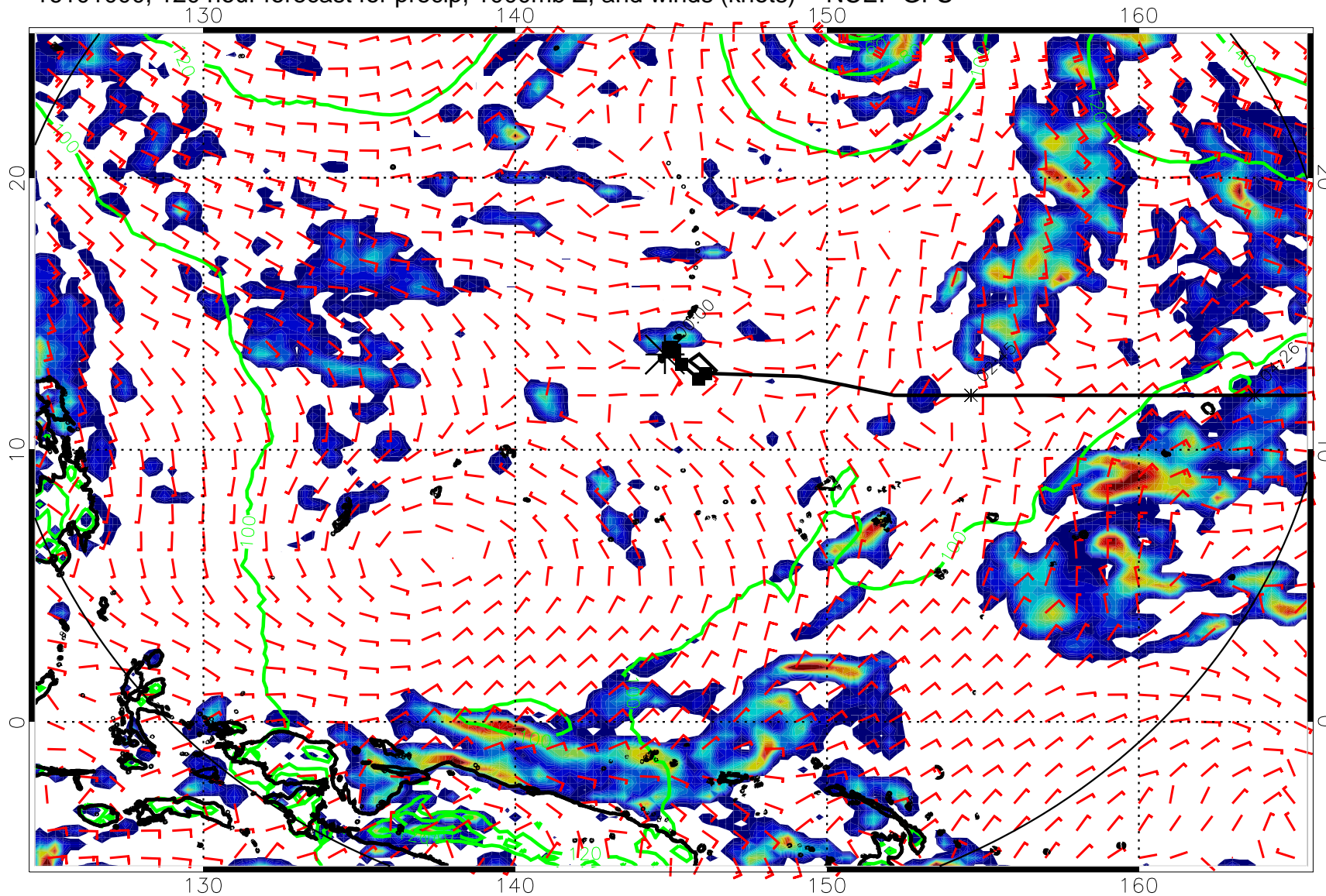
16101000, 120 hour forecast for precip, 1000mb Z, and winds (knots) -- NCEP GFS
