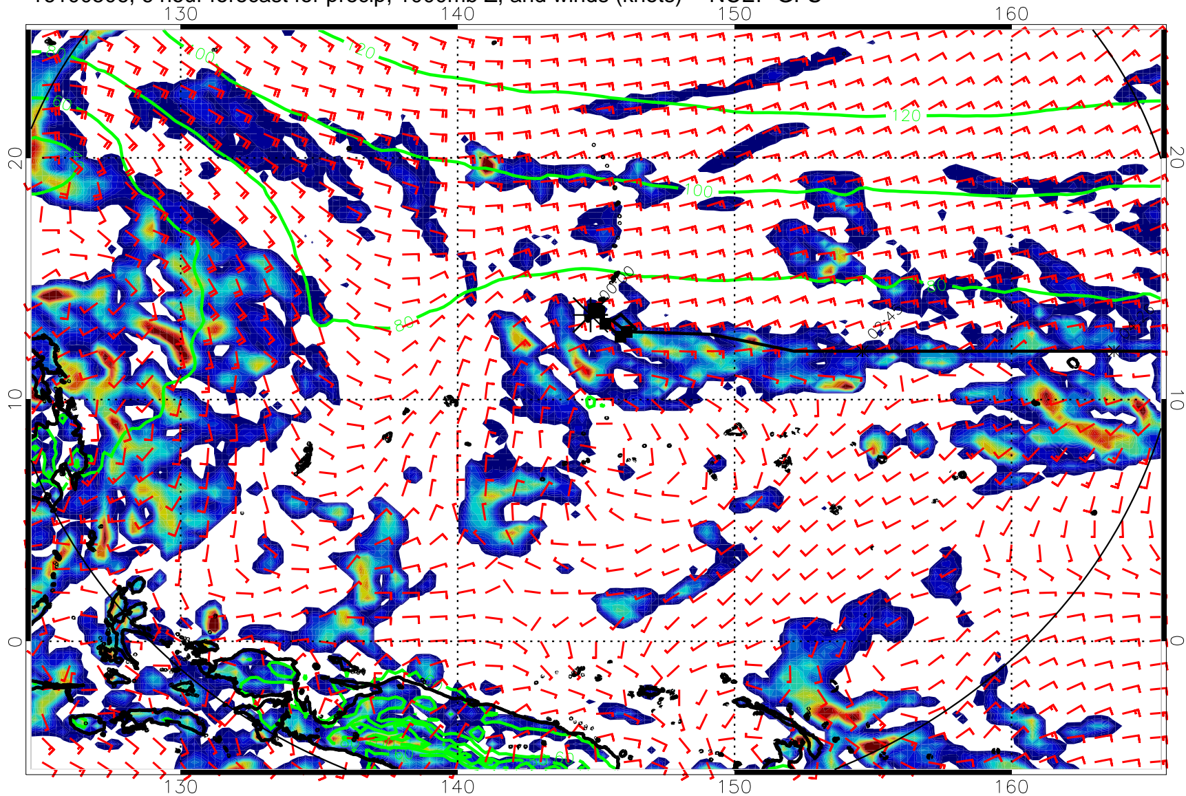
16100506, 6 hour forecast for precip, 1000mb Z, and winds (knots) -- NCEP GFS
