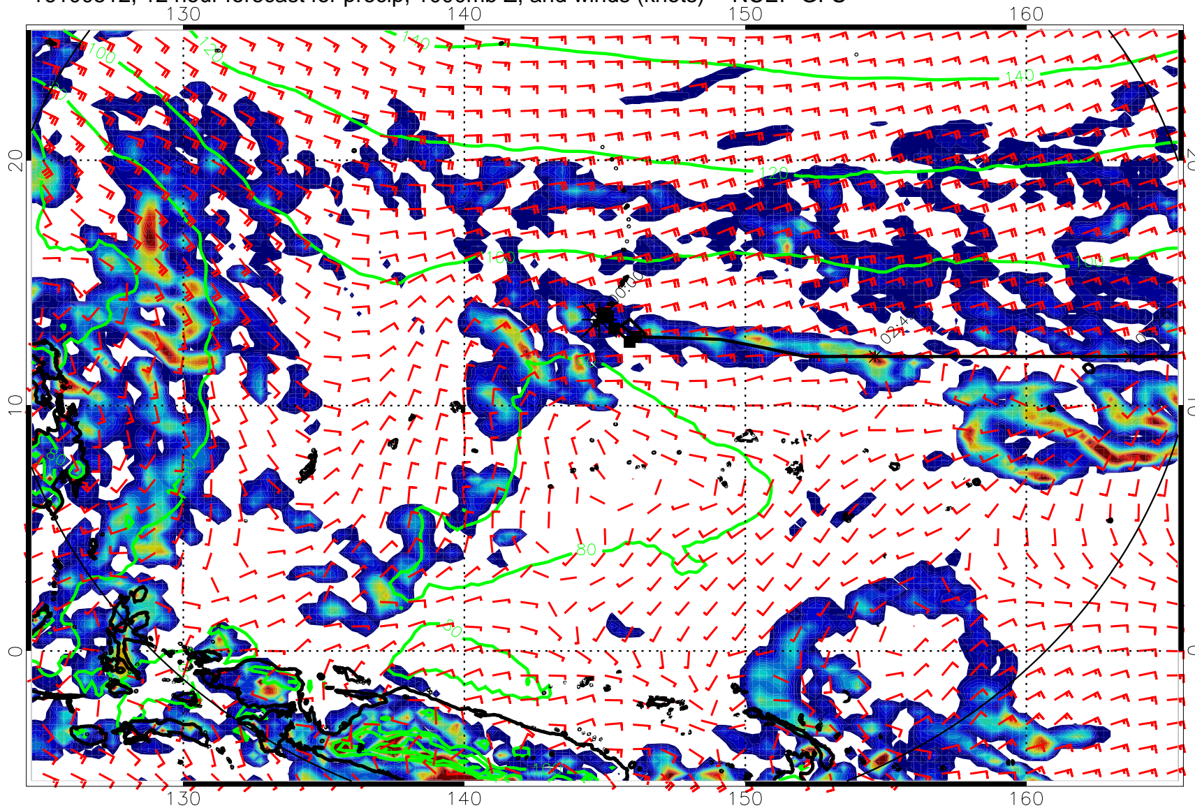
16100512, 12 hour forecast for precip, 1000mb Z, and winds (knots) -- NCEP GFS
