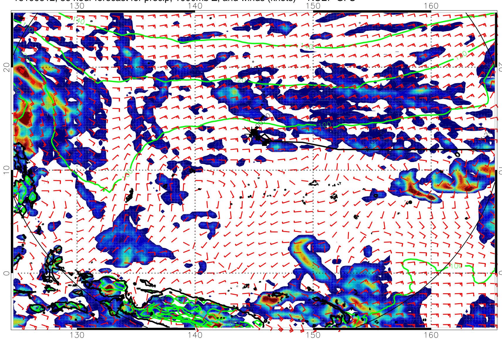
16100612, 36 hour forecast for precip, 1000mb Z, and winds (knots) -- NCEP GFS
