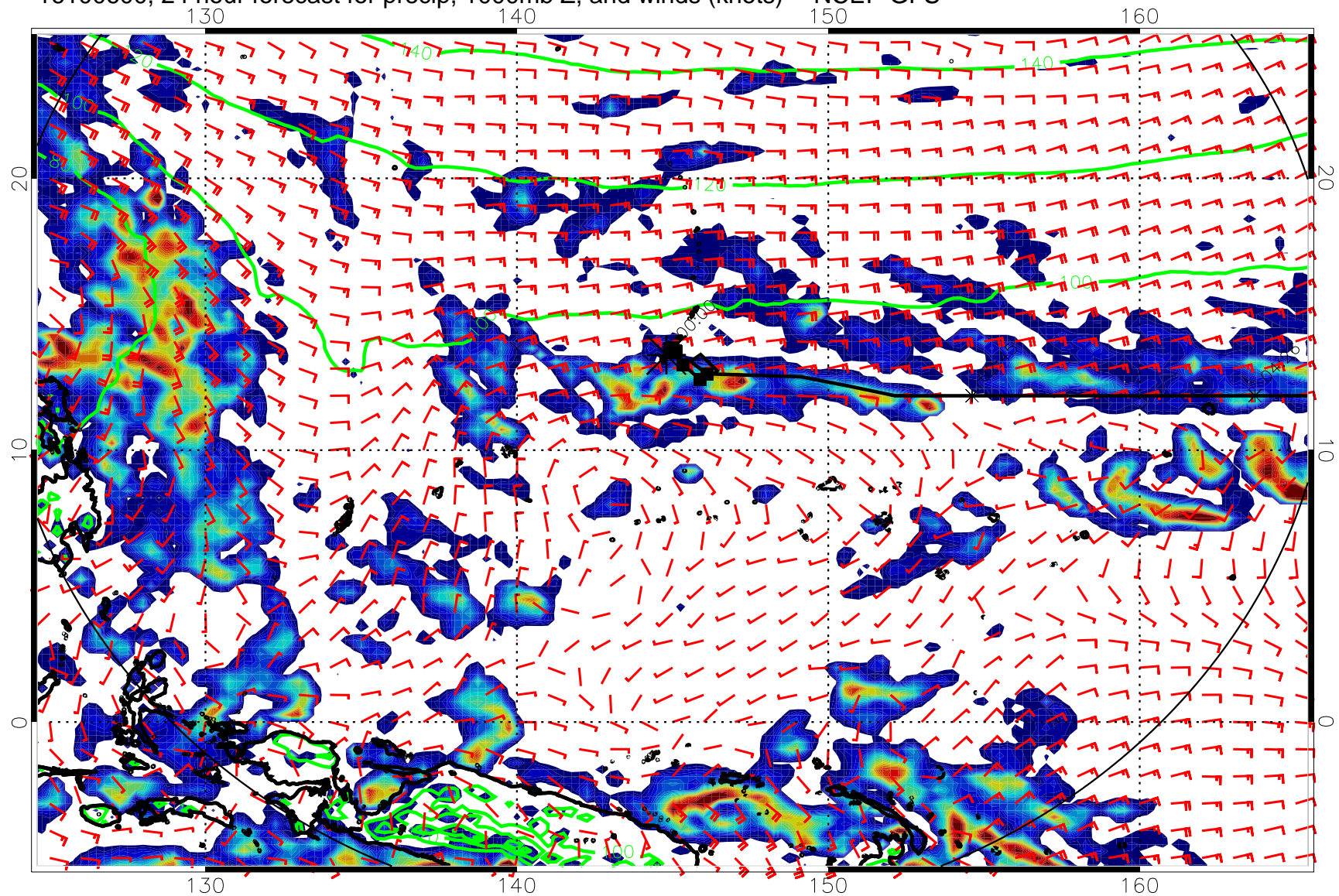
16100600, 24 hour forecast for precip, 1000mb Z, and winds (knots) -- NCEP GFS
