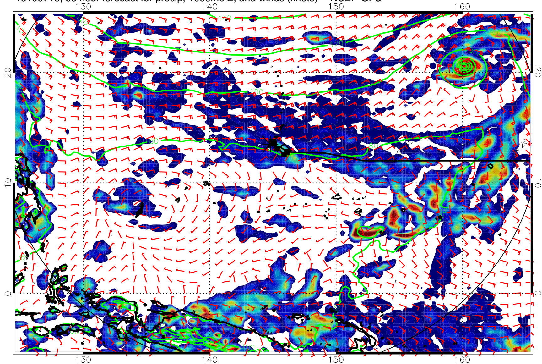
16100718, 66 hour forecast for precip, 1000mb Z, and winds (knots) -- NCEP GFS
