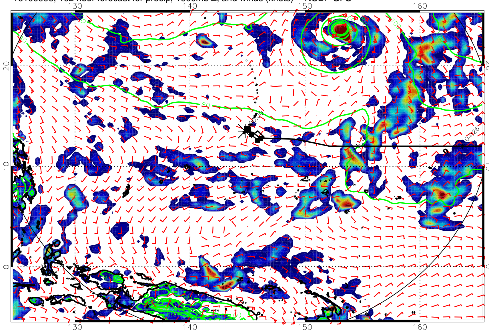
16100906, 102 hour forecast for precip, 1000mb Z, and winds (knots) -- NCEP GFS
