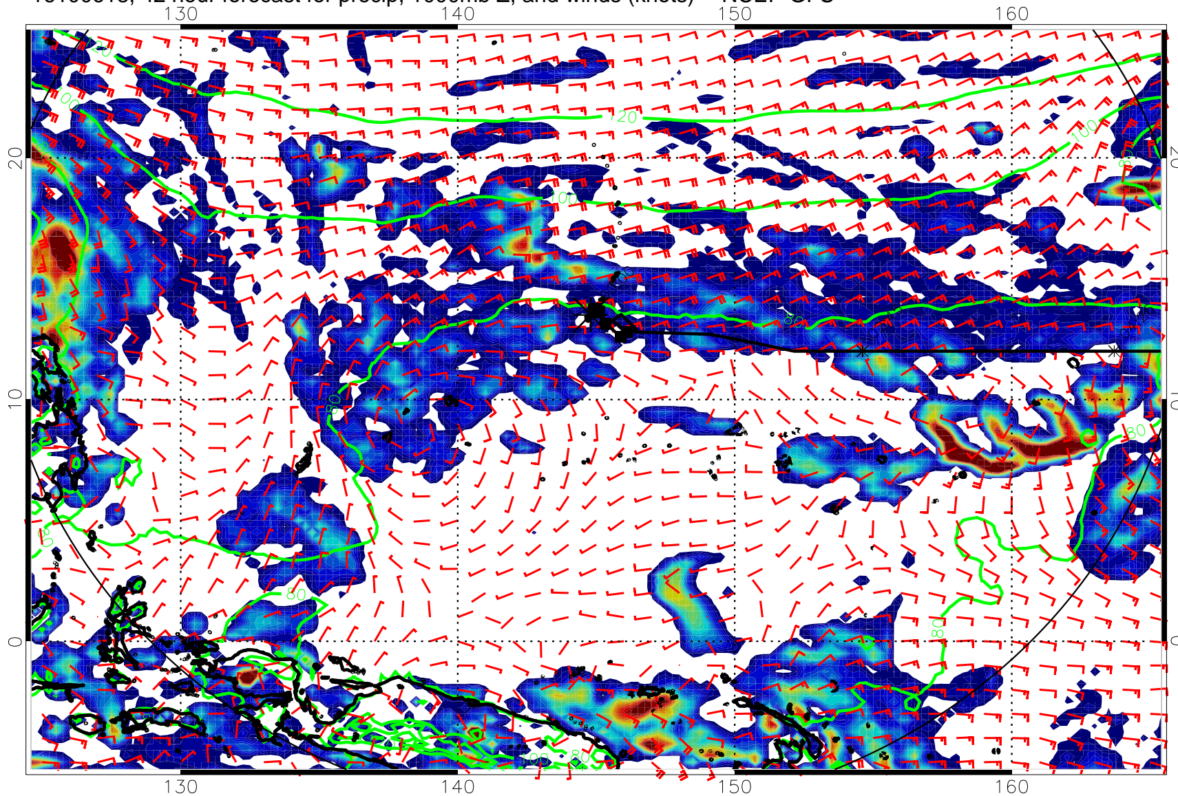
16100618, 42 hour forecast for precip, 1000mb Z, and winds (knots) -- NCEP GFS
