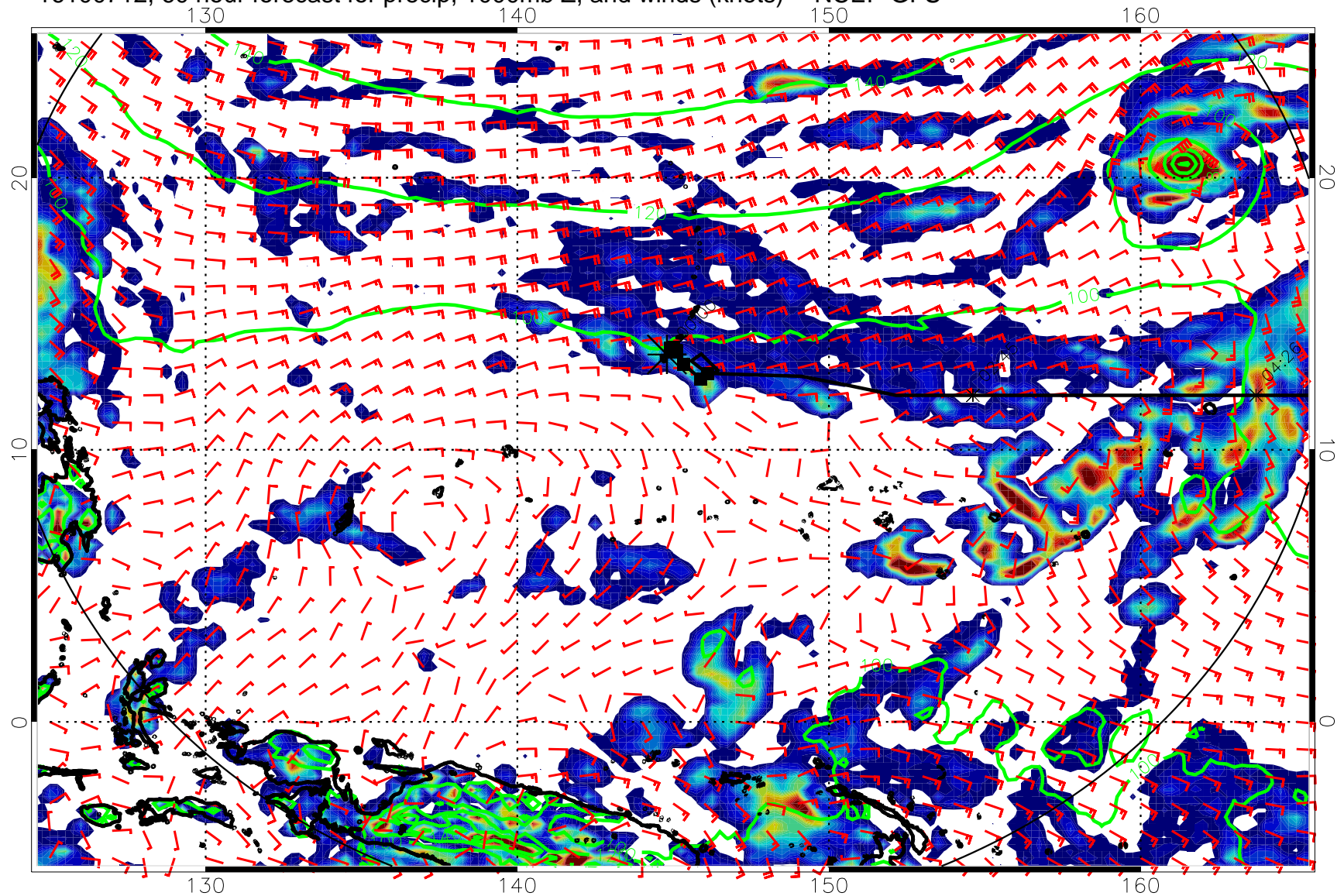
16100712, 60 hour forecast for precip, 1000mb Z, and winds (knots) -- NCEP GFS
