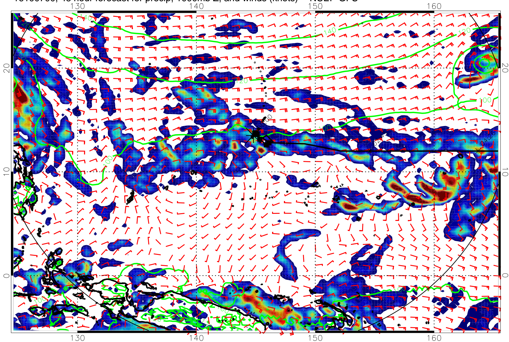
16100700, 48 hour forecast for precip, 1000mb Z, and winds (knots) -- NCEP GFS
