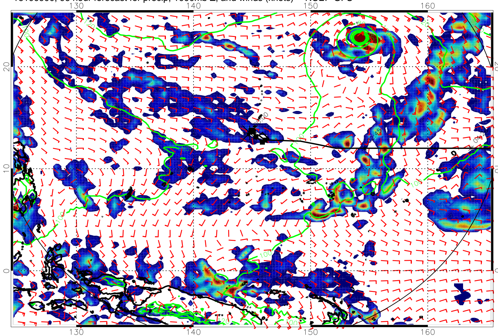
16100900, 96 hour forecast for precip, 1000mb Z, and winds (knots) -- NCEP GFS
