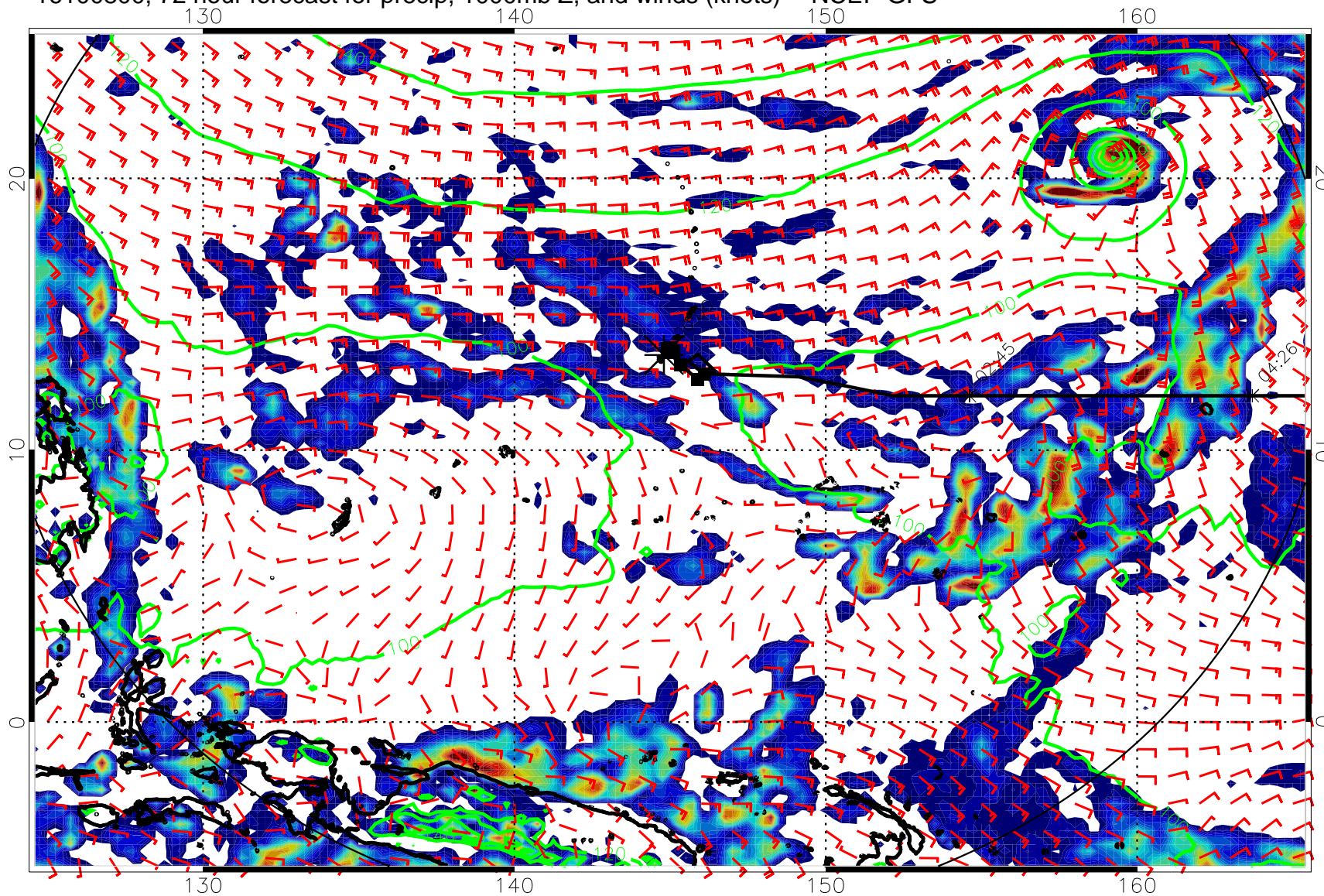
16100800, 72 hour forecast for precip, 1000mb Z, and winds (knots) -- NCEP GFS
