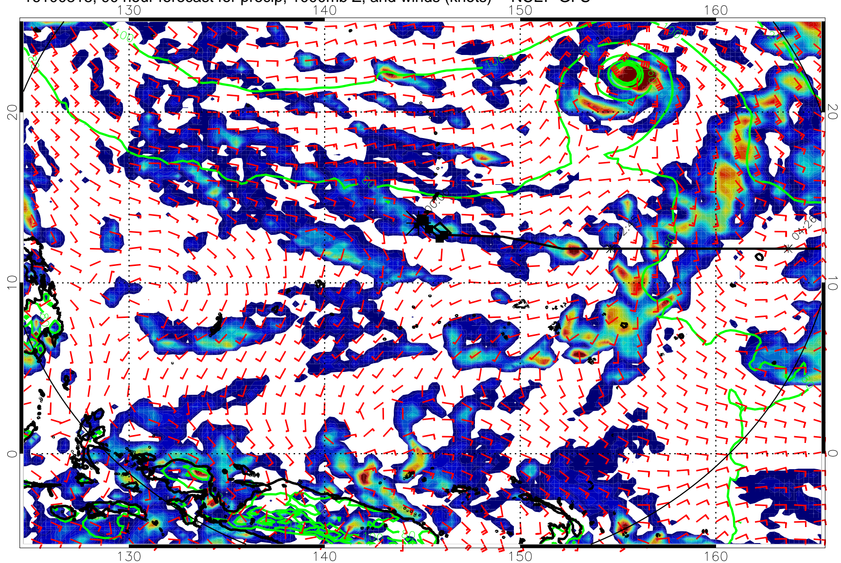
16100818, 90 hour forecast for precip, 1000mb Z, and winds (knots) -- NCEP GFS
