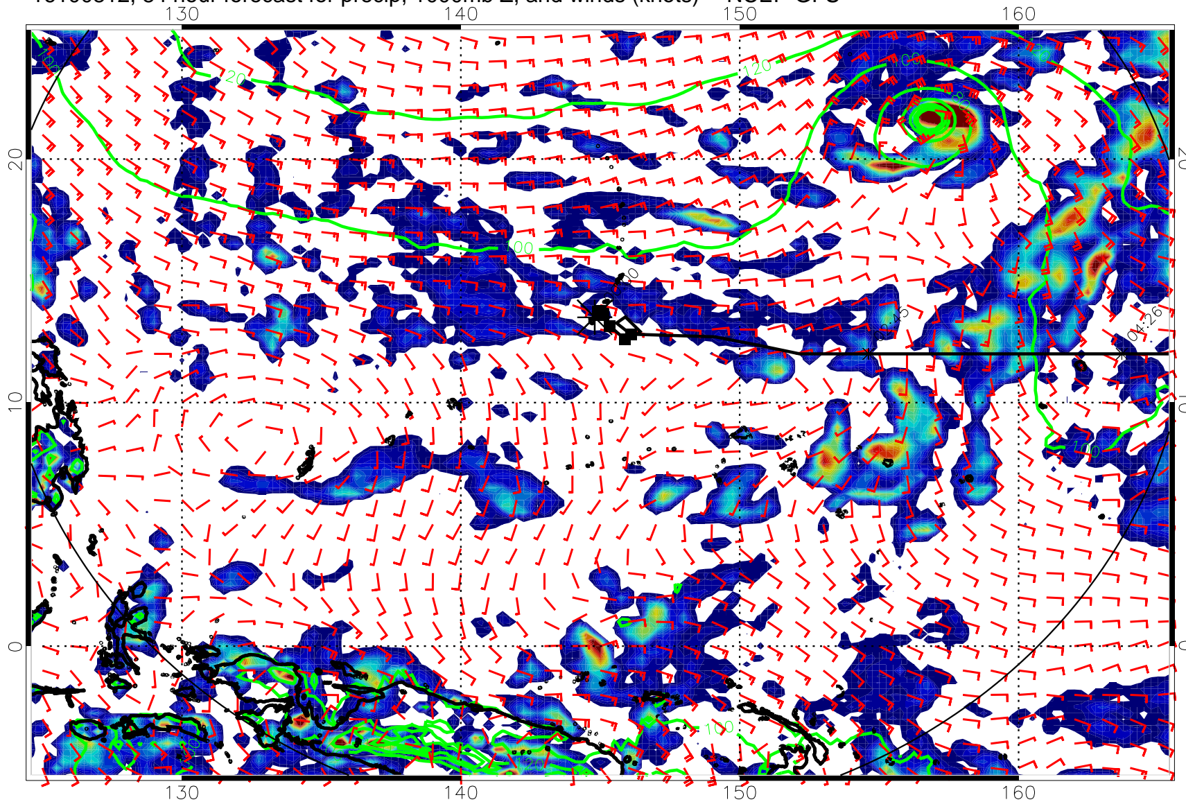
16100812, 84 hour forecast for precip, 1000mb Z, and winds (knots) -- NCEP GFS
