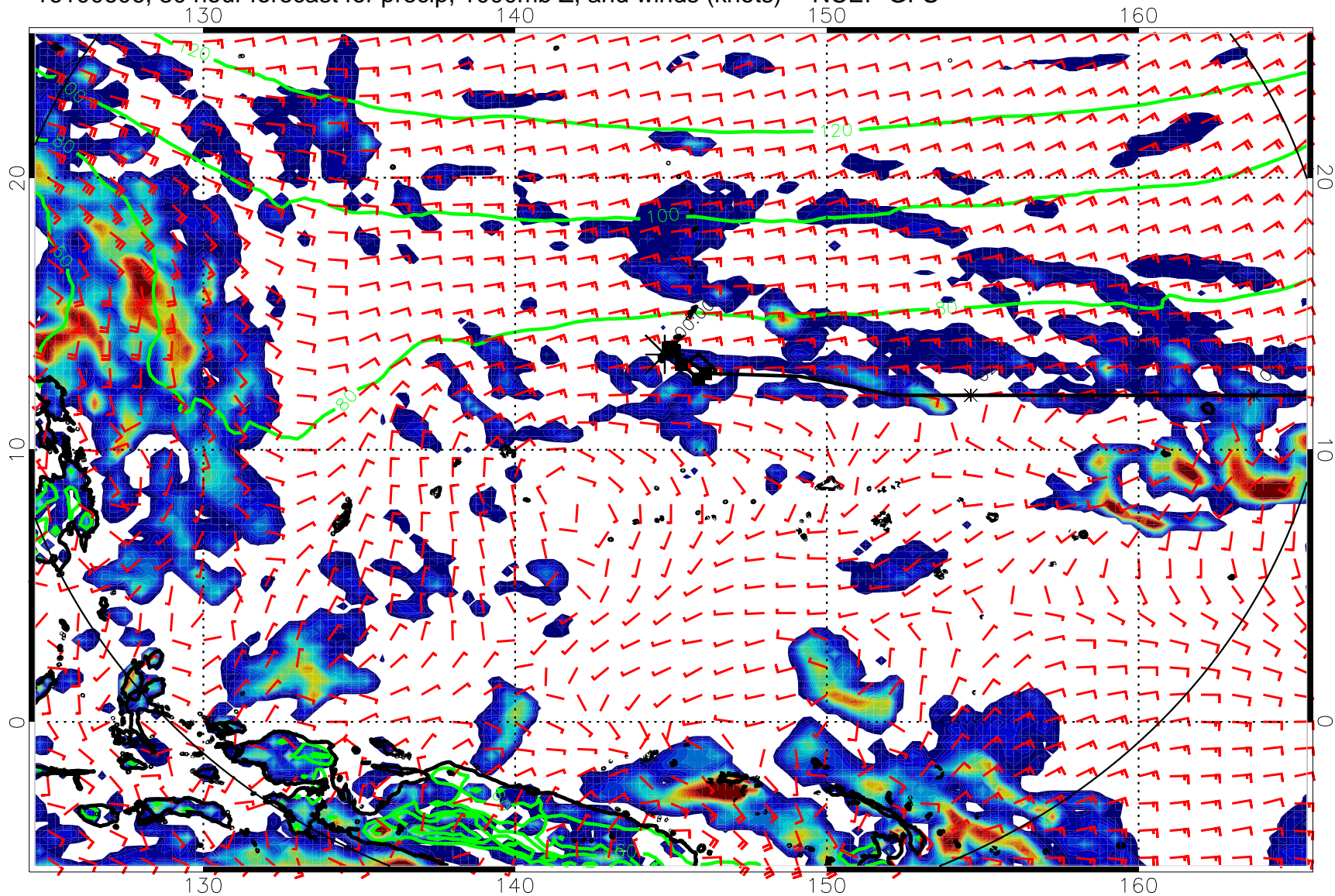
16100606, 30 hour forecast for precip, 1000mb Z, and winds (knots) -- NCEP GFS
