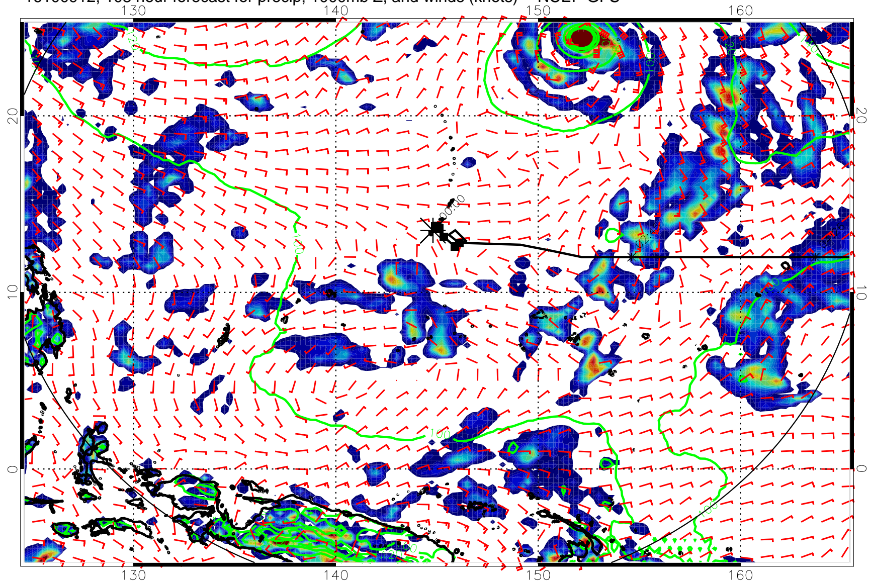
16100912, 108 hour forecast for precip, 1000mb Z, and winds (knots) -- NCEP GFS
