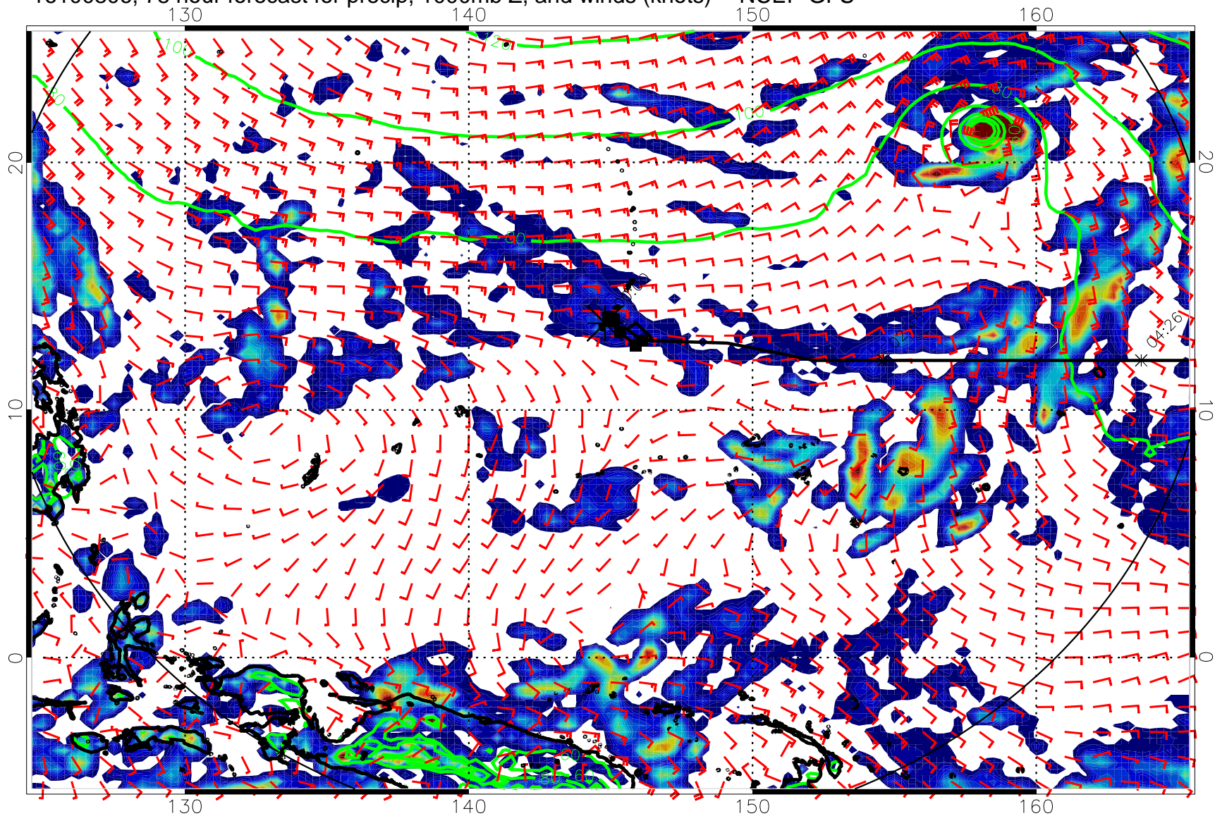
16100806, 78 hour forecast for precip, 1000mb Z, and winds (knots) -- NCEP GFS
