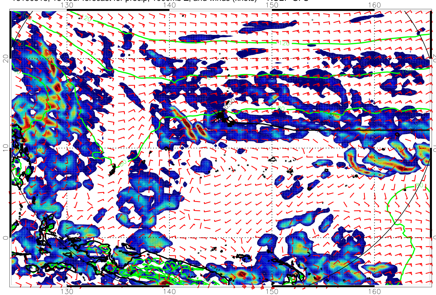
16100518, 18 hour forecast for precip, 1000mb Z, and winds (knots) -- NCEP GFS
