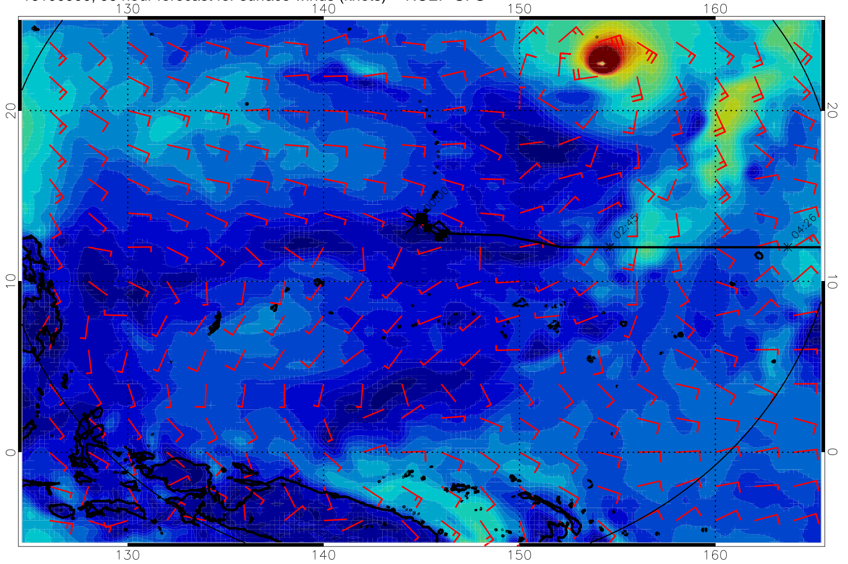
16100900, 96 hour forecast for surface winds (knots) -- NCEP GFS
