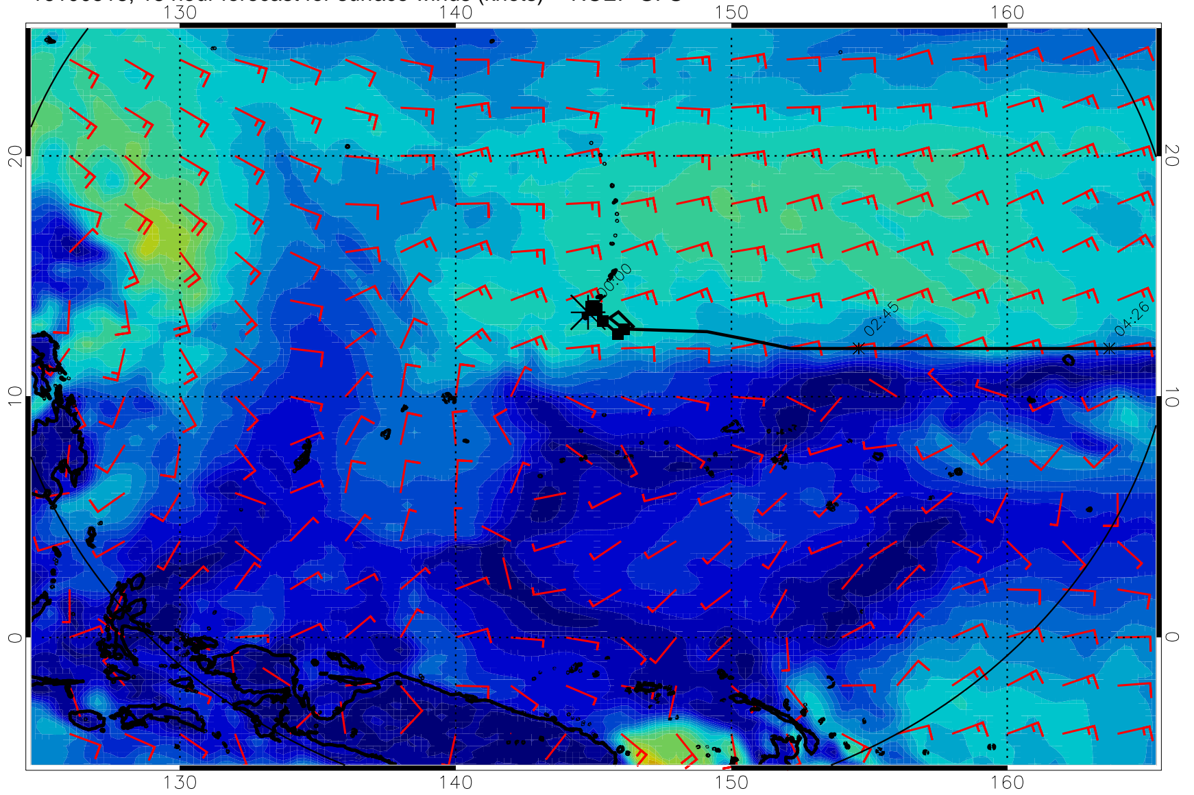
16100518, 18 hour forecast for surface winds (knots) -- NCEP GFS
