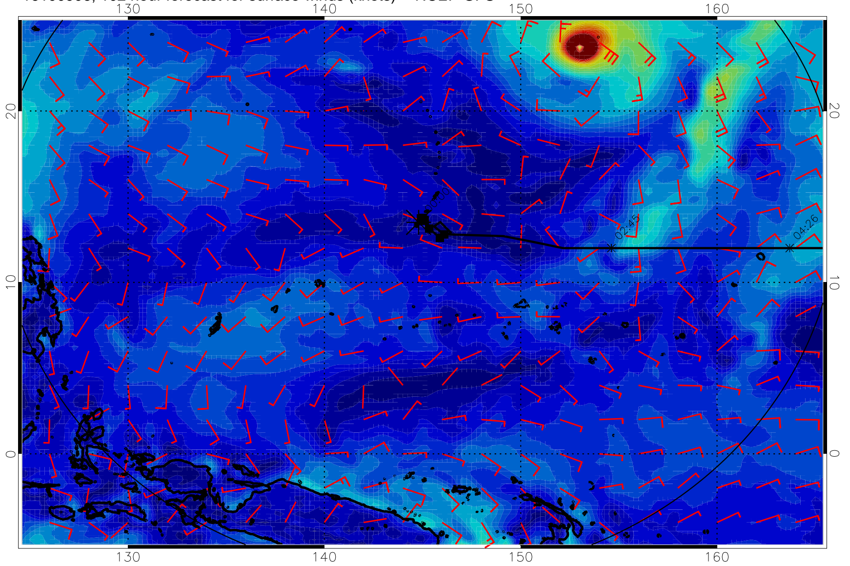
16100906, 102 hour forecast for surface winds (knots) -- NCEP GFS
