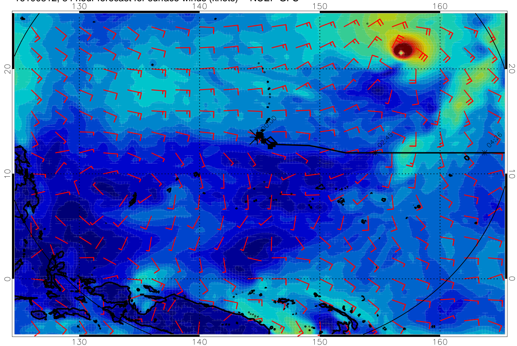
16100812, 84 hour forecast for surface winds (knots) -- NCEP GFS
