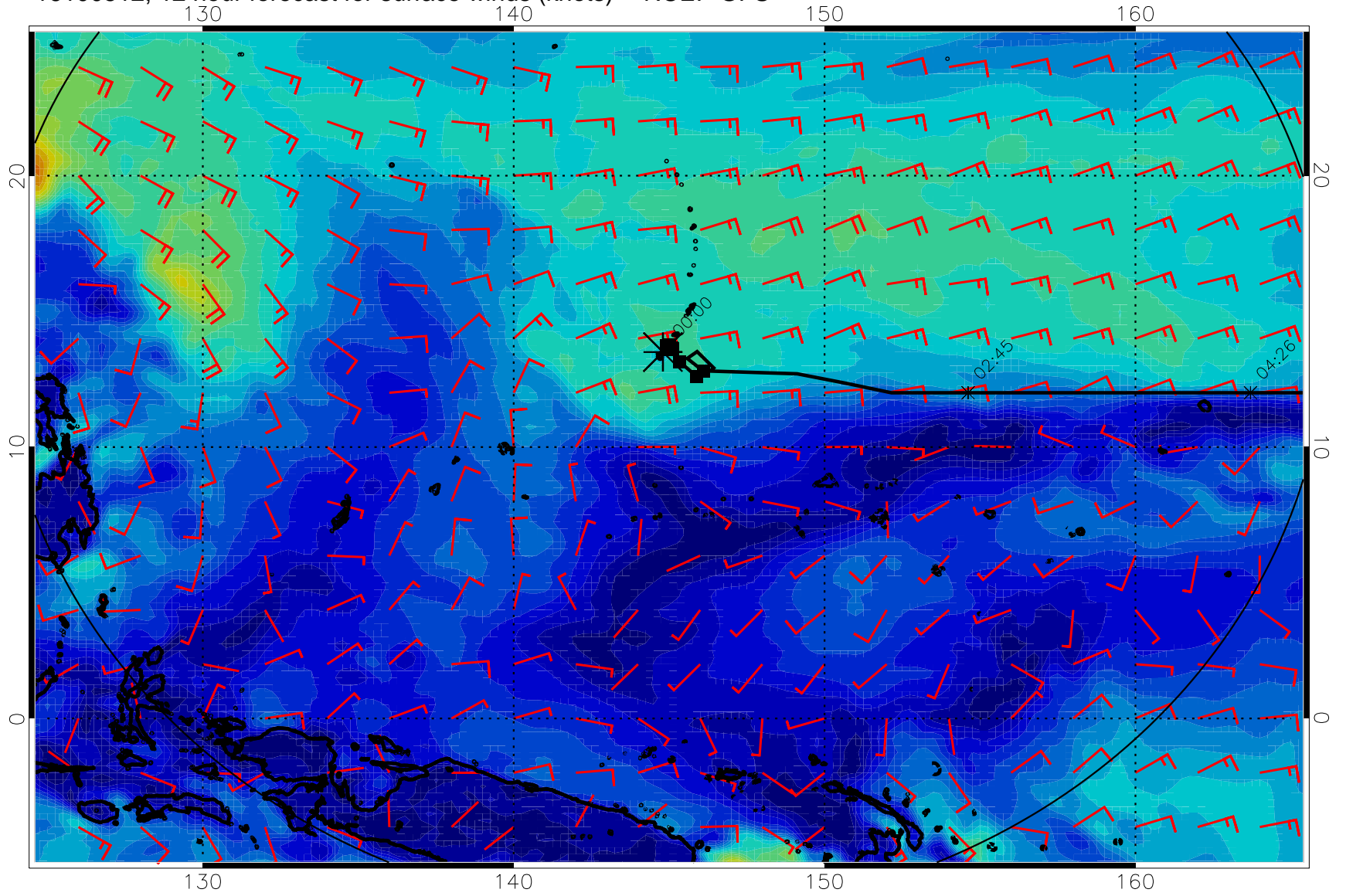
16100512, 12 hour forecast for surface winds (knots) -- NCEP GFS
