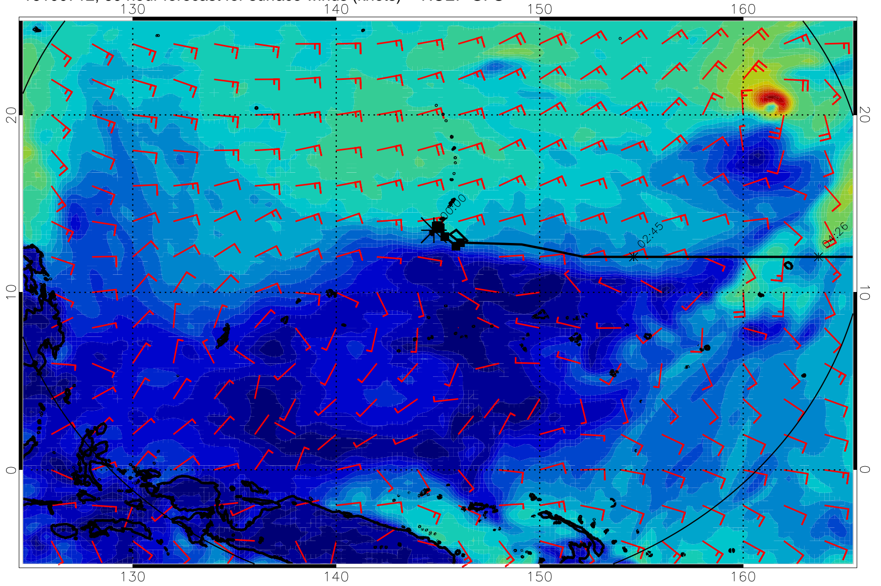
16100712, 60 hour forecast for surface winds (knots) -- NCEP GFS
