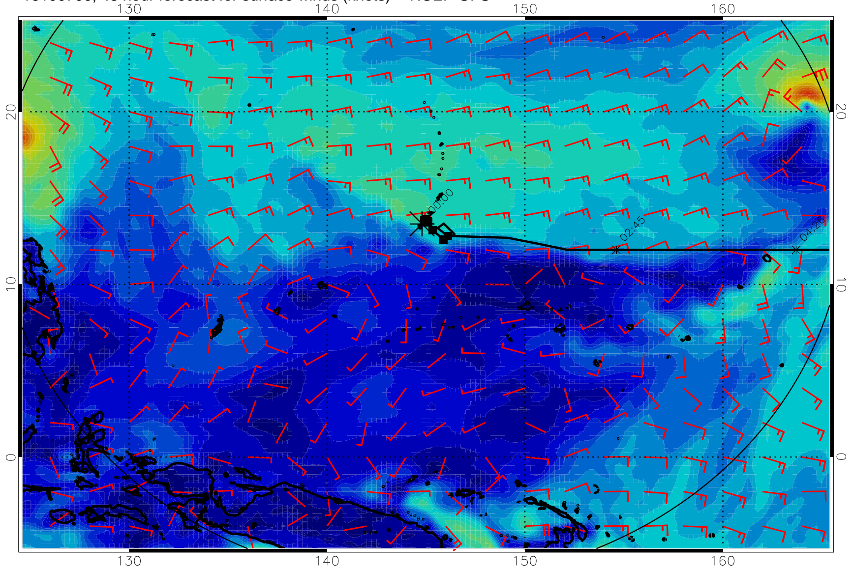
16100700, 48 hour forecast for surface winds (knots) -- NCEP GFS
