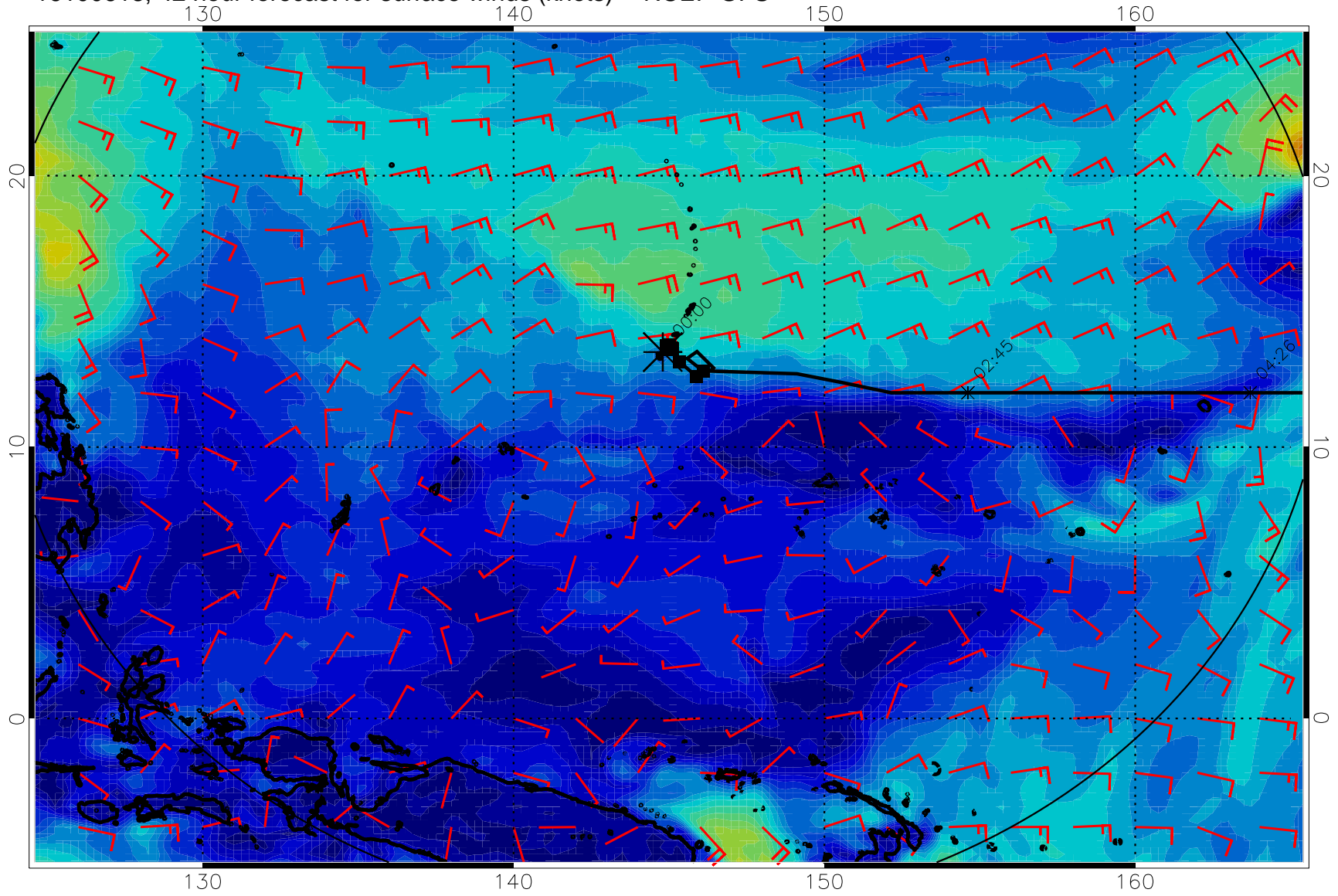
16100618, 42 hour forecast for surface winds (knots) -- NCEP GFS
