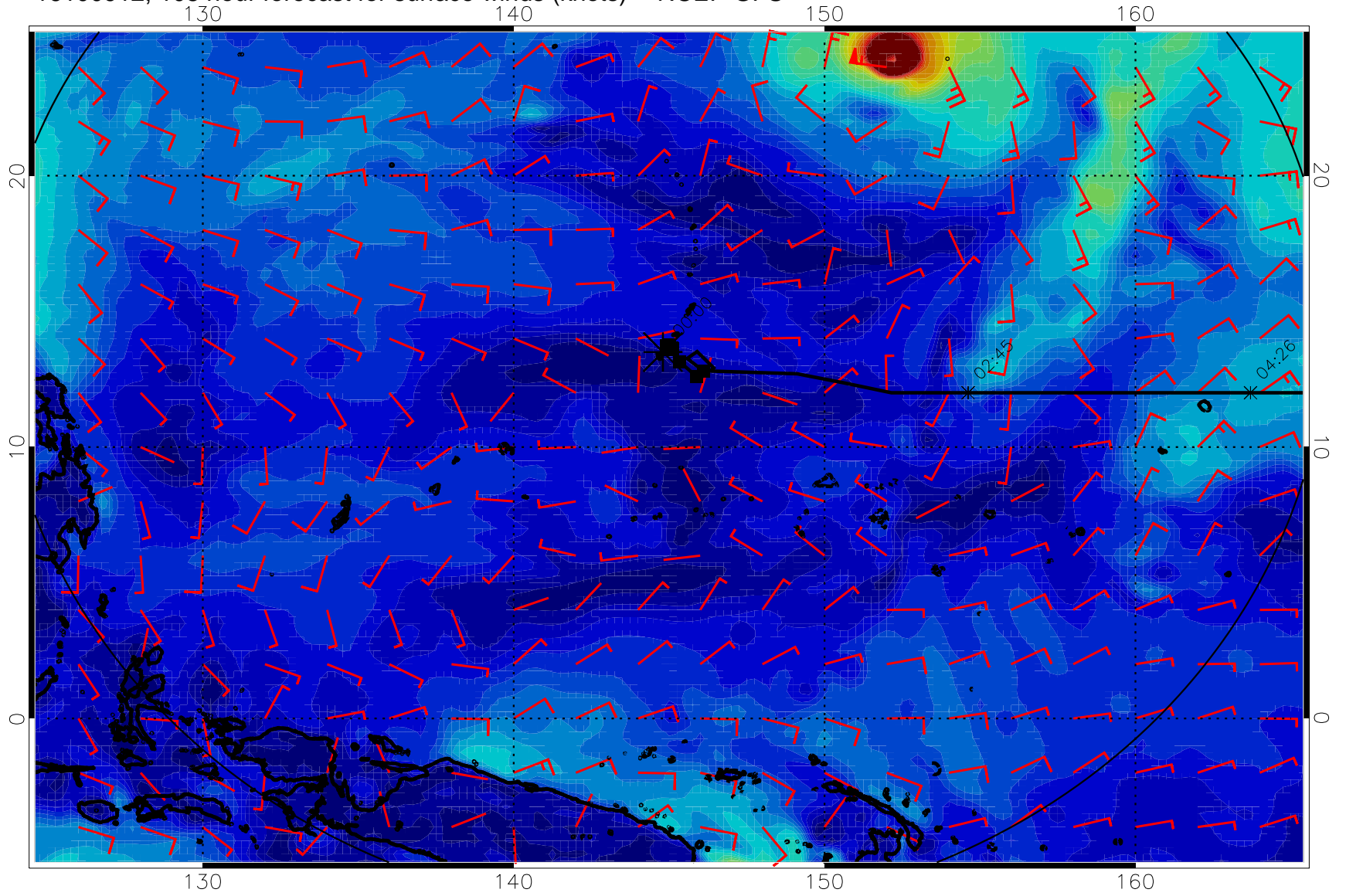
16100912, 108 hour forecast for surface winds (knots) -- NCEP GFS
