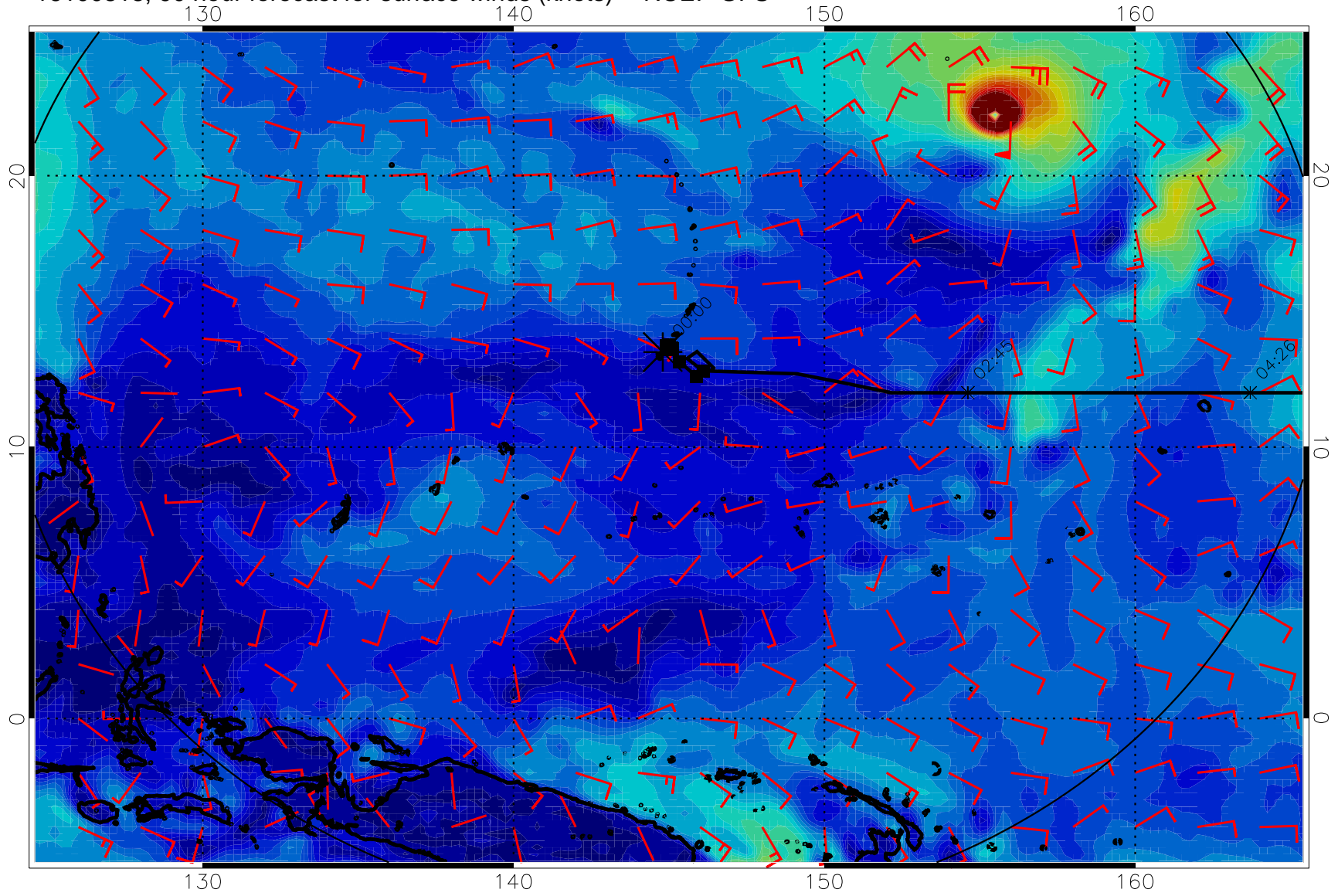
16100818, 90 hour forecast for surface winds (knots) -- NCEP GFS
