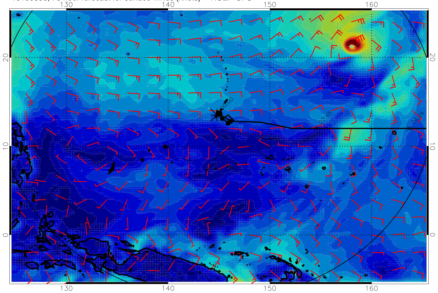
16100806, 78 hour forecast for surface winds (knots) -- NCEP GFS
