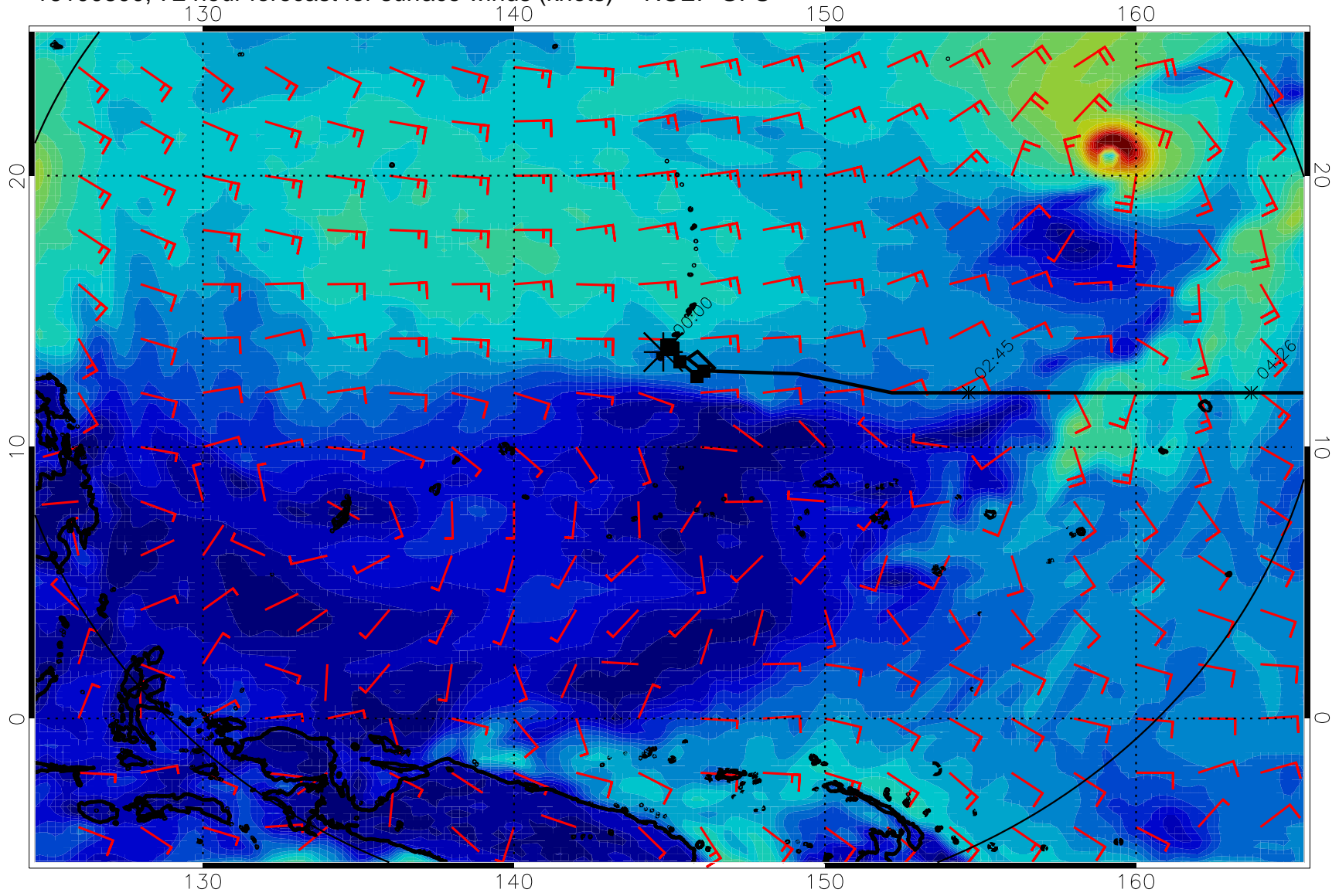
16100800, 72 hour forecast for surface winds (knots) -- NCEP GFS
