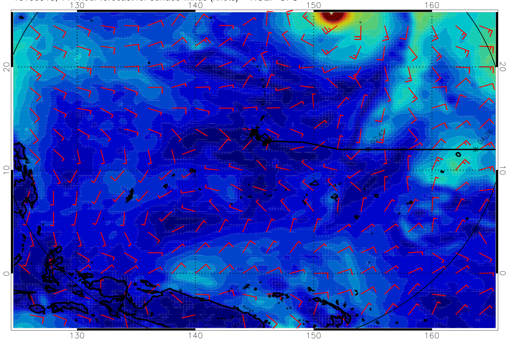
16100918, 114 hour forecast for surface winds (knots) -- NCEP GFS
