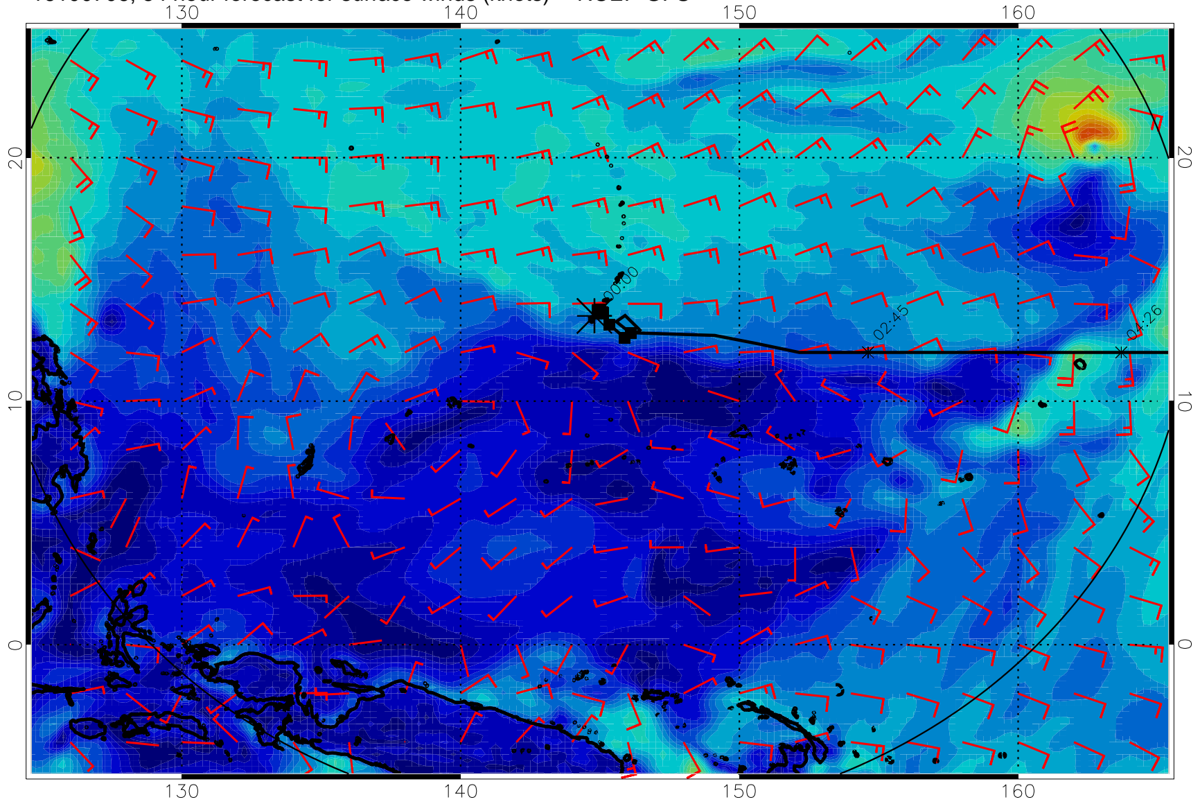
16100706, 54 hour forecast for surface winds (knots) -- NCEP GFS
