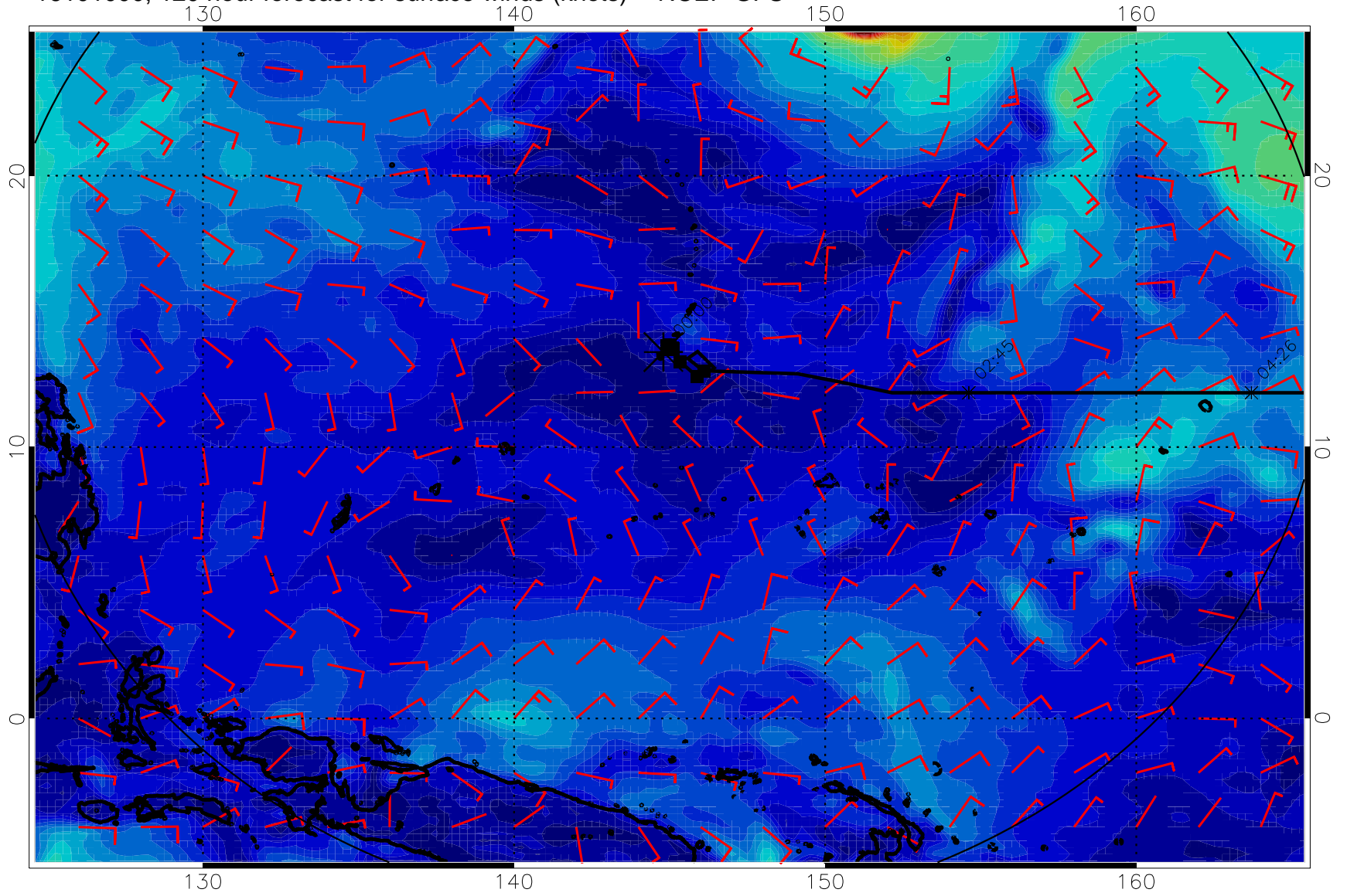
16101000, 120 hour forecast for surface winds (knots) -- NCEP GFS
