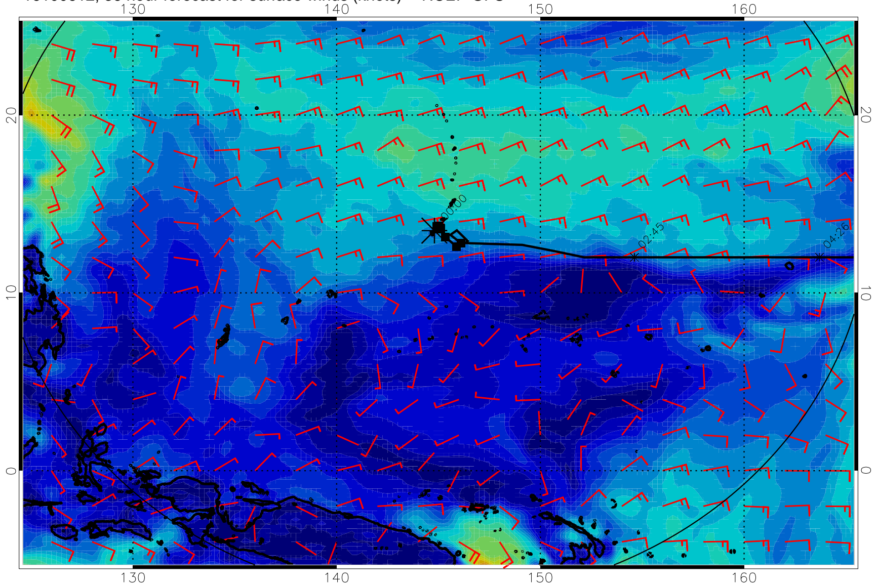
16100612, 36 hour forecast for surface winds (knots) -- NCEP GFS
