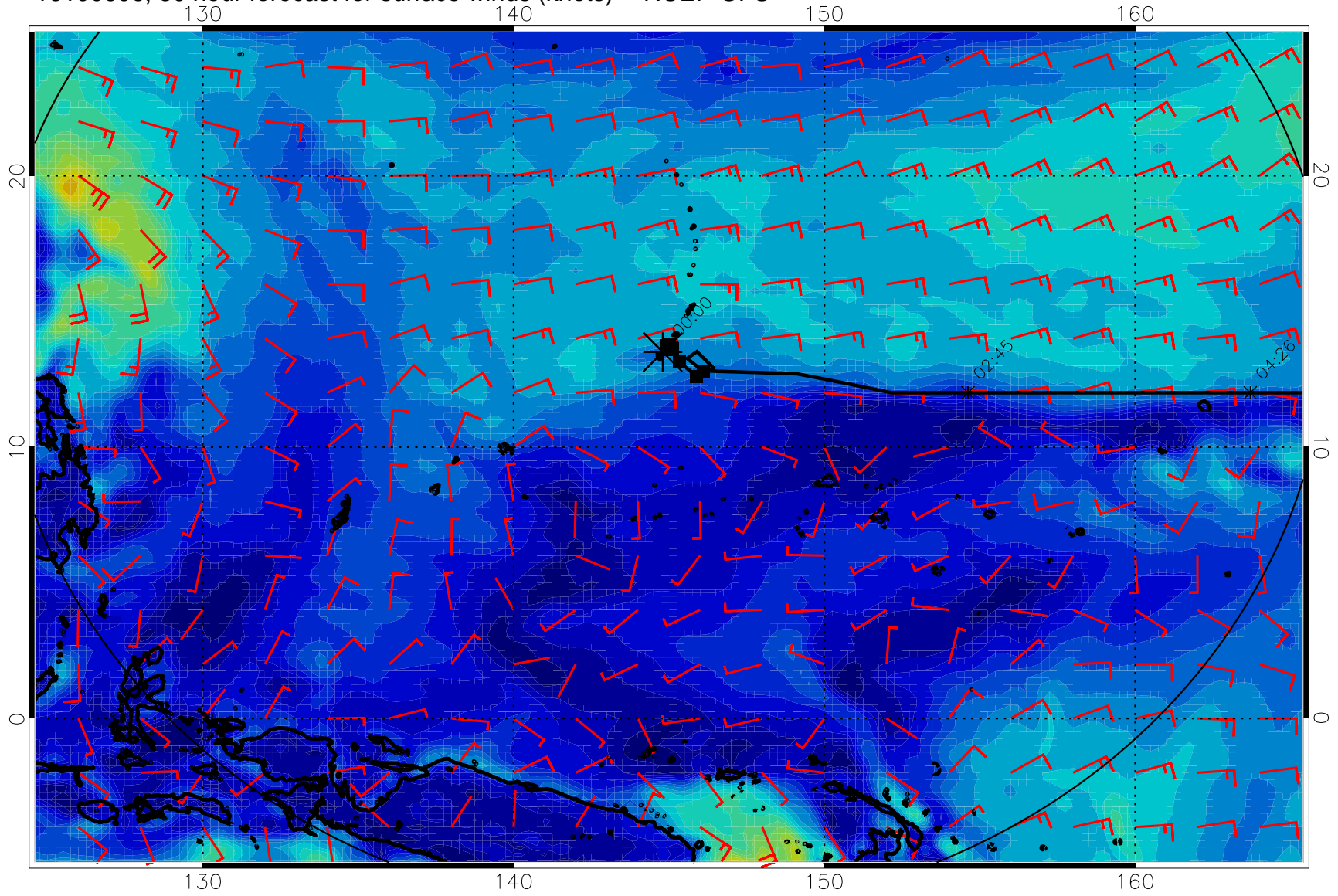
16100606, 30 hour forecast for surface winds (knots) -- NCEP GFS
