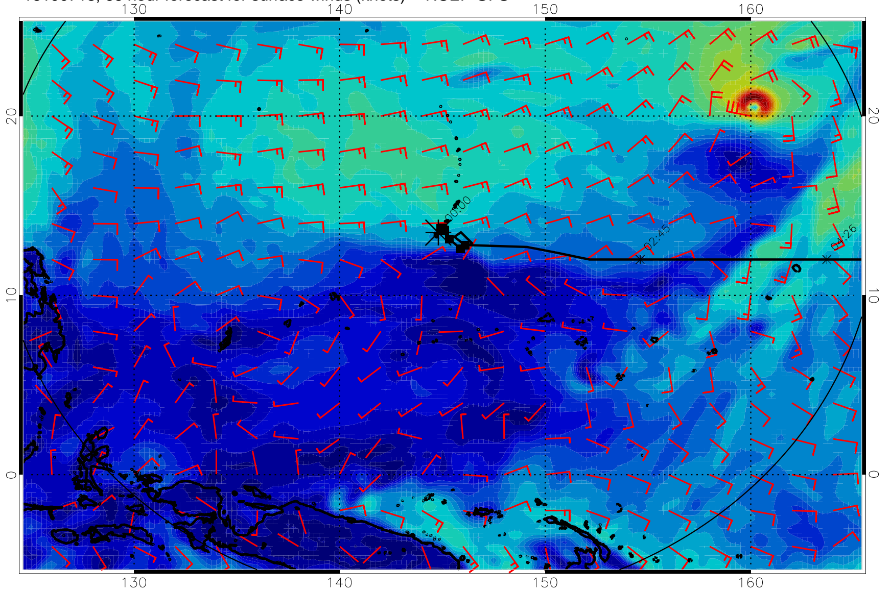
16100718, 66 hour forecast for surface winds (knots) -- NCEP GFS
