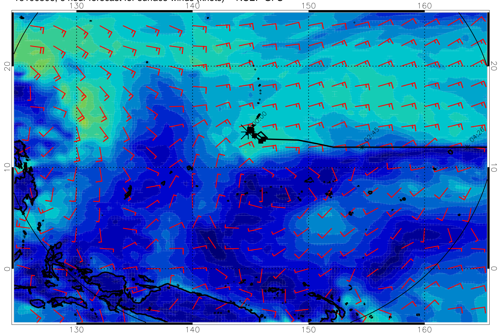
16100506, 6 hour forecast for surface winds (knots) -- NCEP GFS
