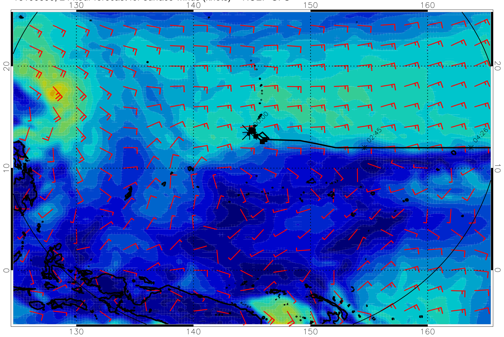
16100600, 24 hour forecast for surface winds (knots) -- NCEP GFS
