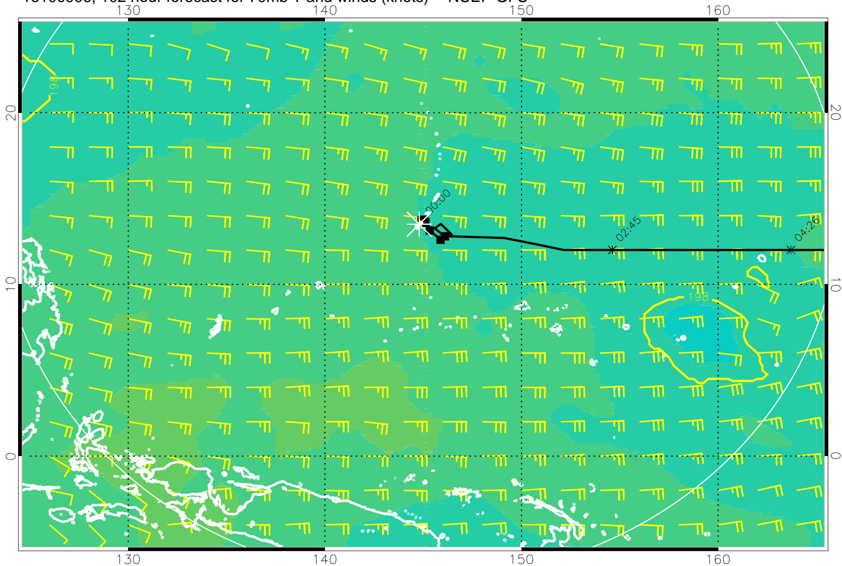
16100906, 102 hour forecast for 70mb T and winds (knots) -- NCEP GFS
