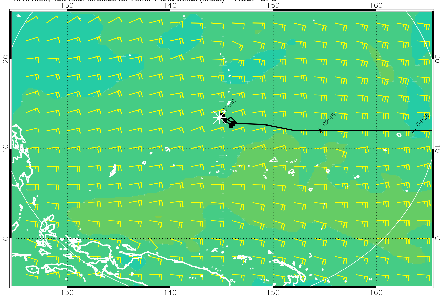
16101000, 120 hour forecast for 70mb T and winds (knots) -- NCEP GFS
