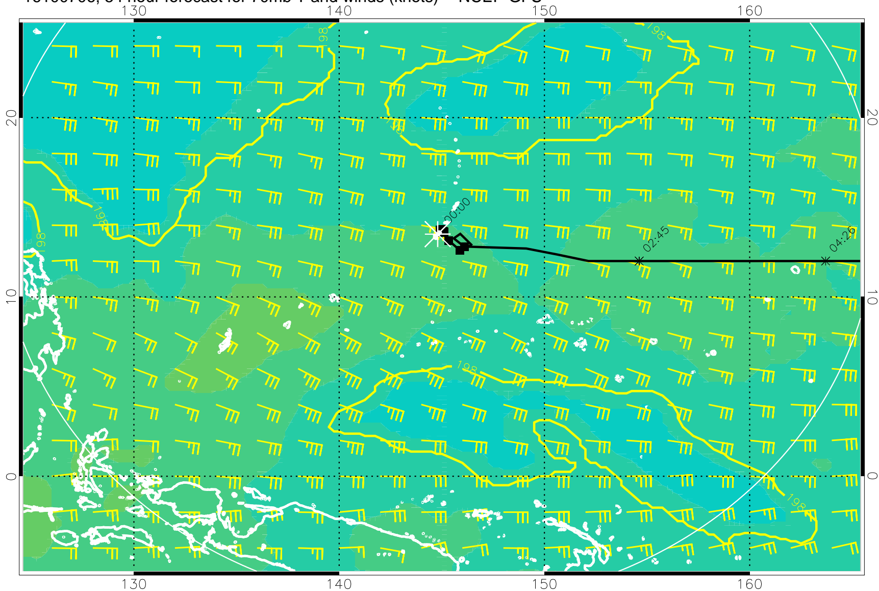
16100706, 54 hour forecast for 70mb T and winds (knots) -- NCEP GFS
