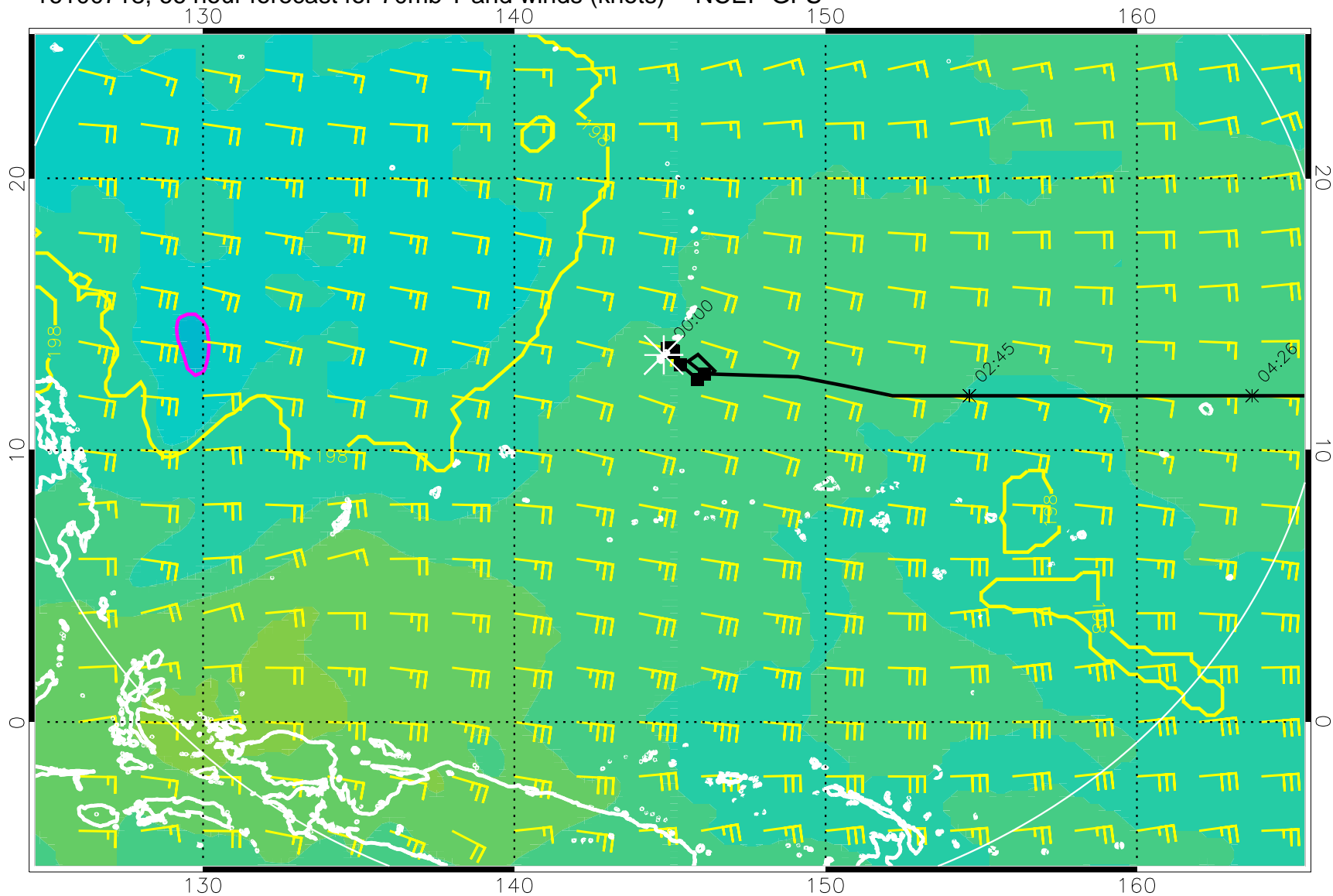
16100718, 66 hour forecast for 70mb T and winds (knots) -- NCEP GFS
