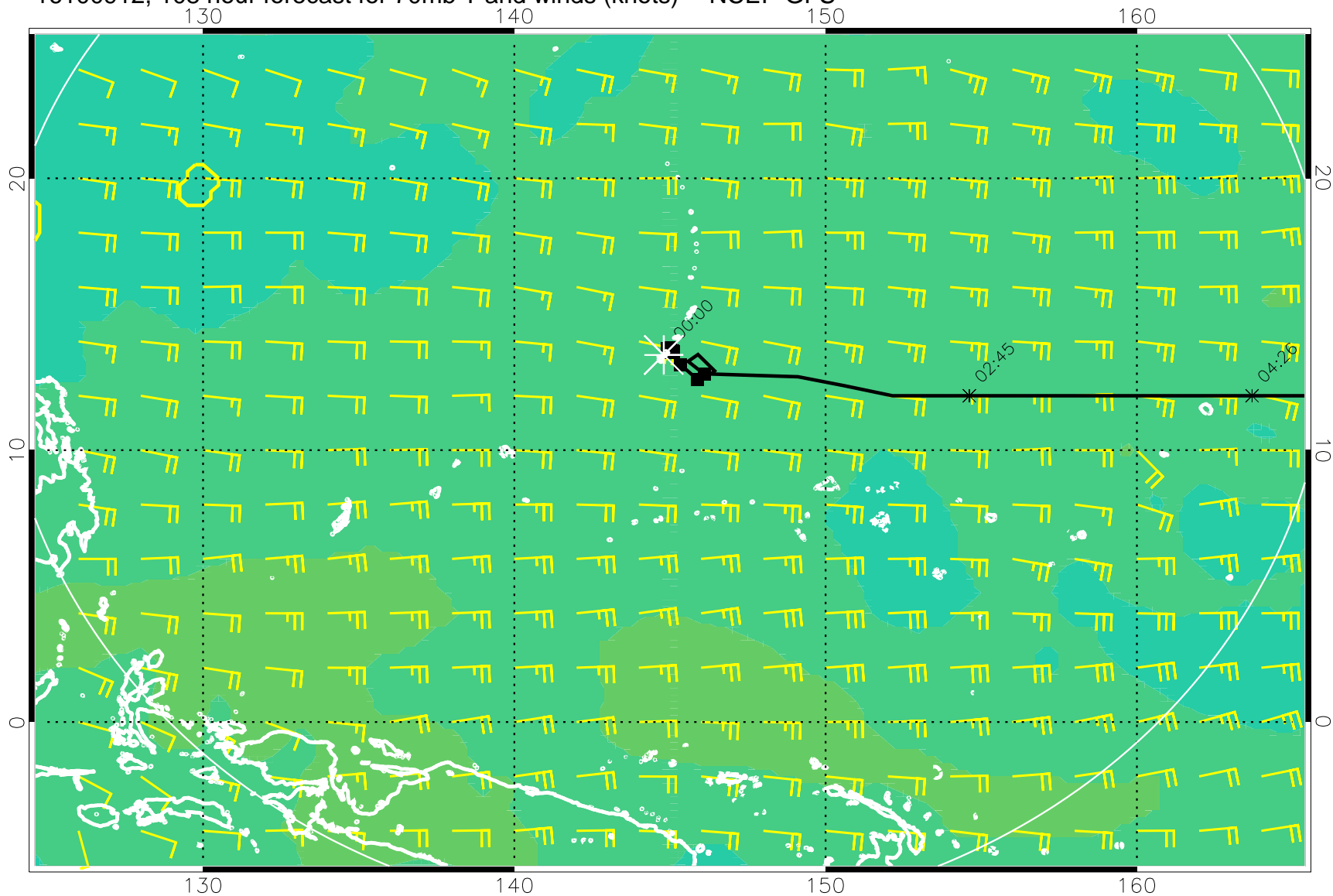
16100912, 108 hour forecast for 70mb T and winds (knots) -- NCEP GFS
