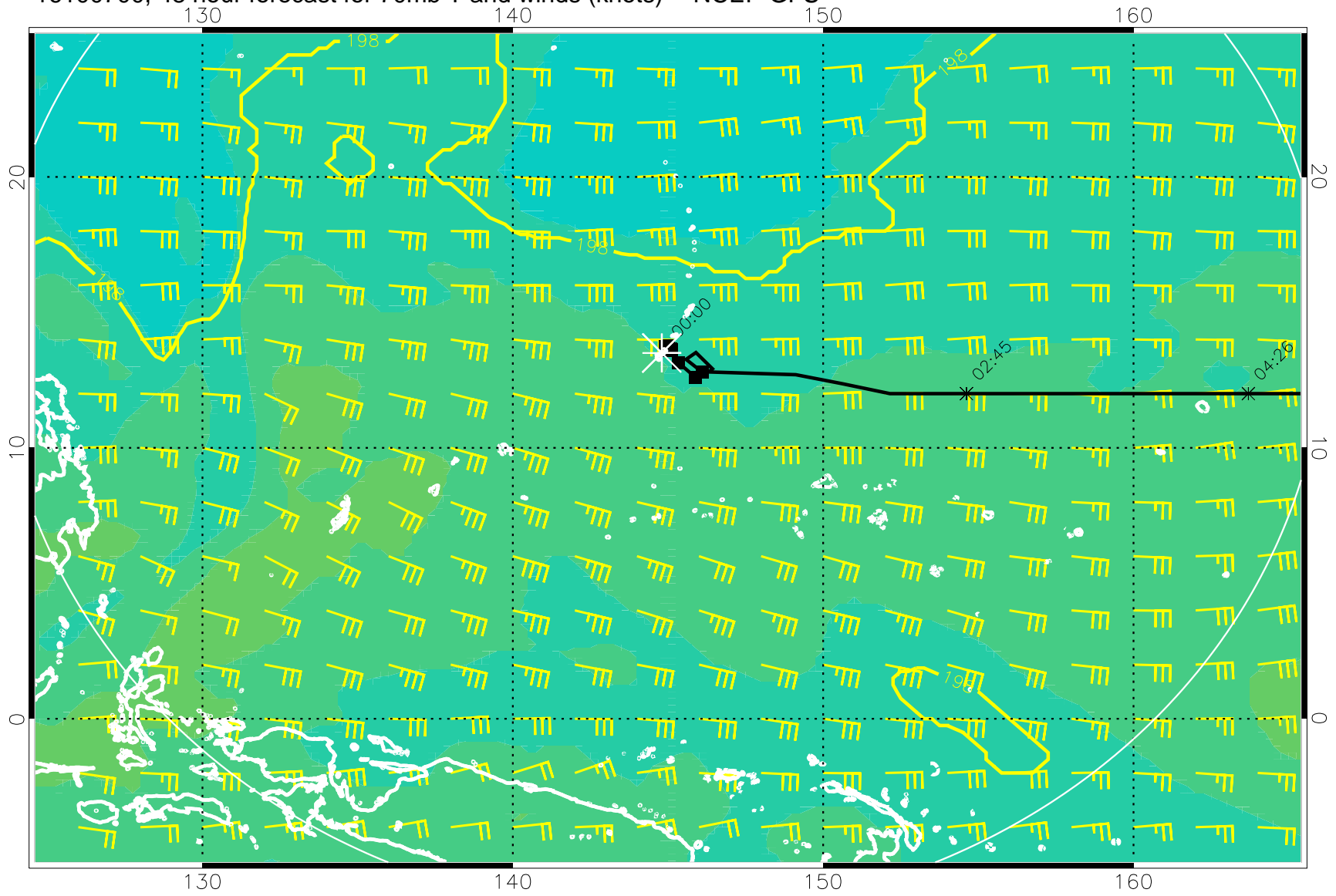
16100700, 48 hour forecast for 70mb T and winds (knots) -- NCEP GFS
