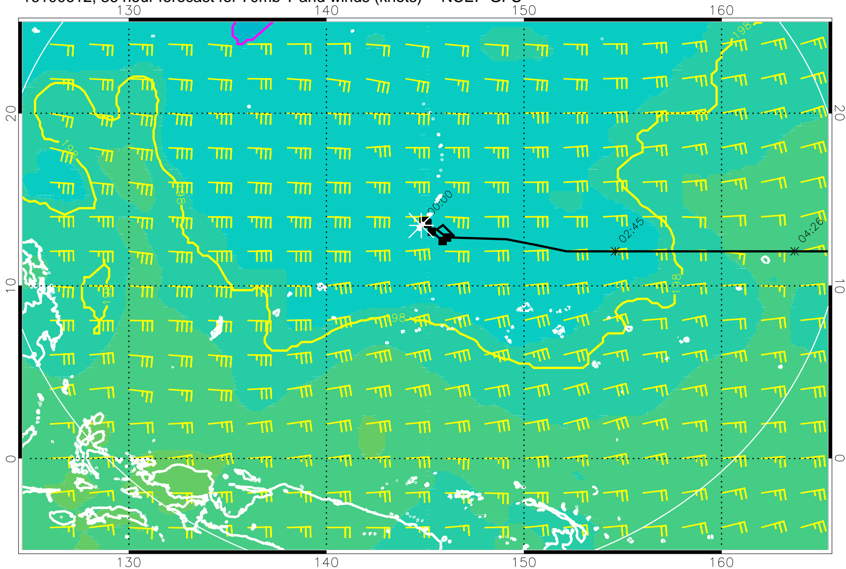
16100612, 36 hour forecast for 70mb T and winds (knots) -- NCEP GFS
