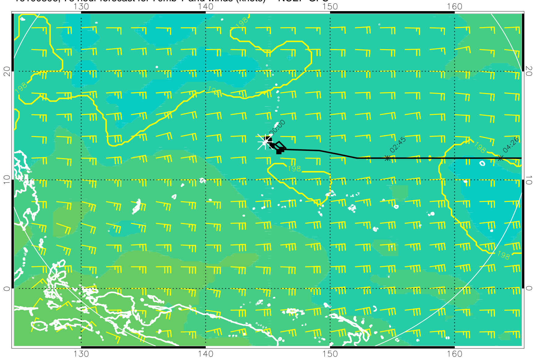
16100806, 78 hour forecast for 70mb T and winds (knots) -- NCEP GFS
