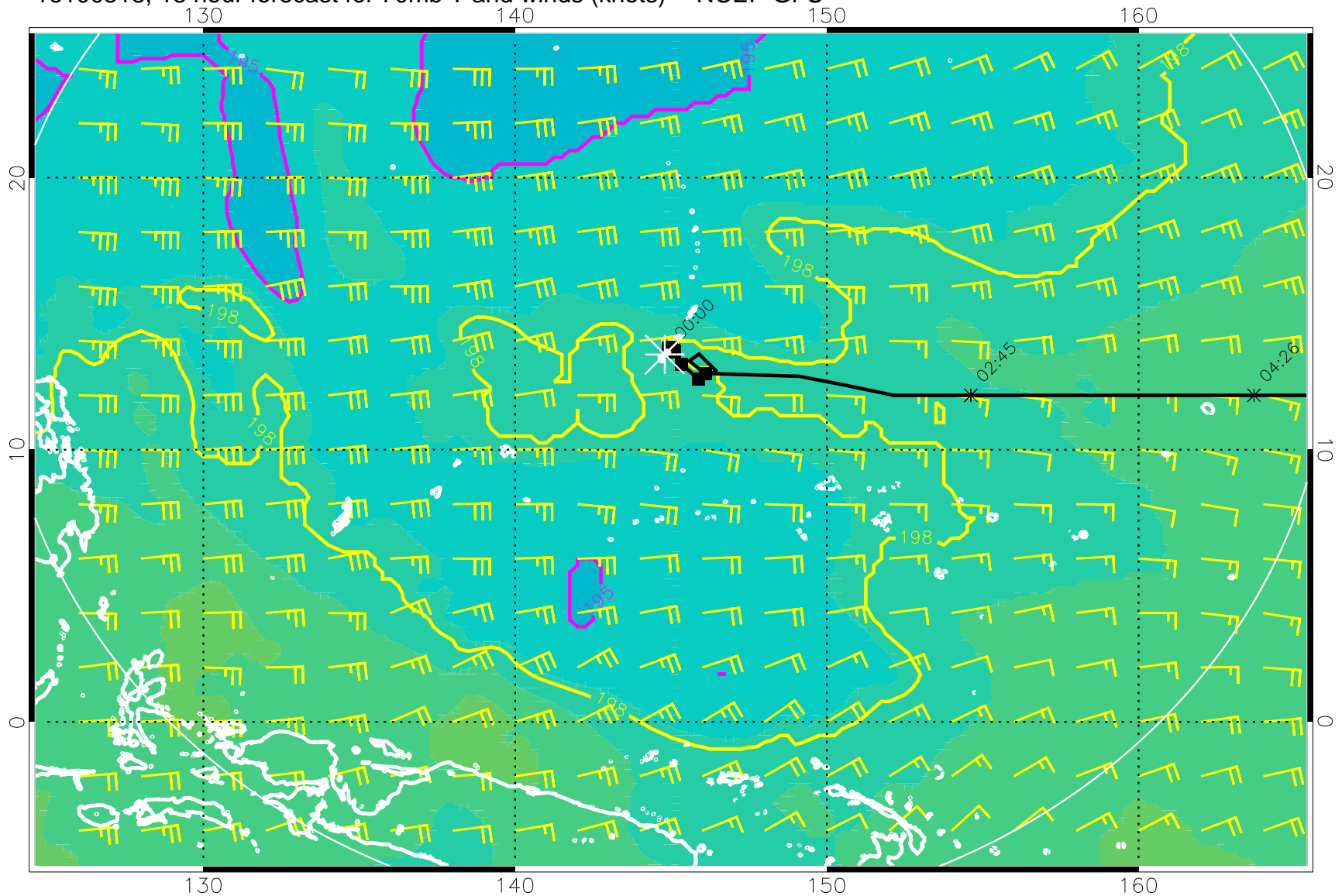
16100518, 18 hour forecast for 70mb T and winds (knots) -- NCEP GFS
