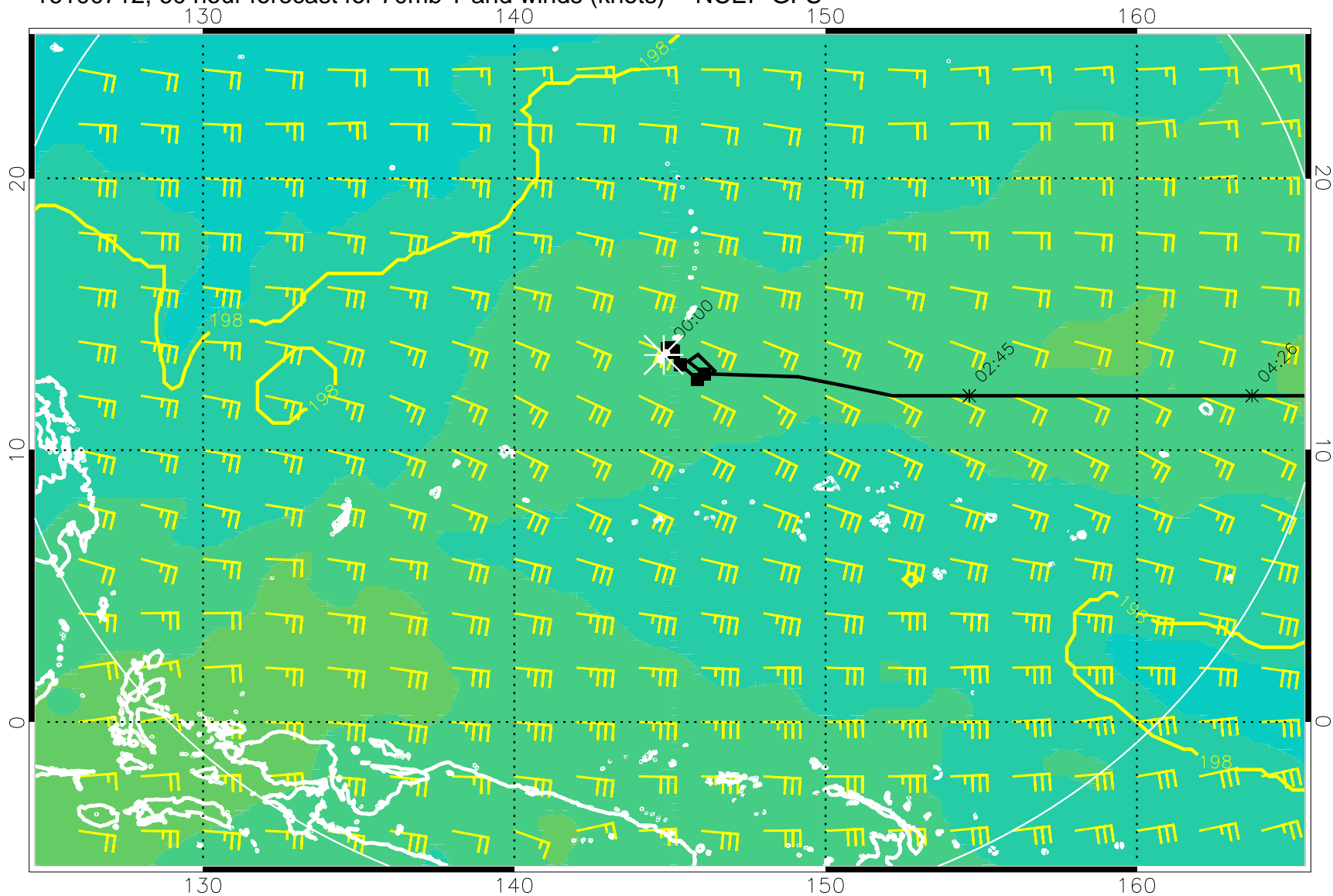
16100712, 60 hour forecast for 70mb T and winds (knots) -- NCEP GFS
