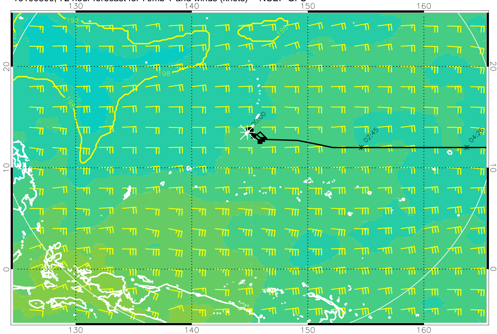
16100800, 72 hour forecast for 70mb T and winds (knots) -- NCEP GFS
