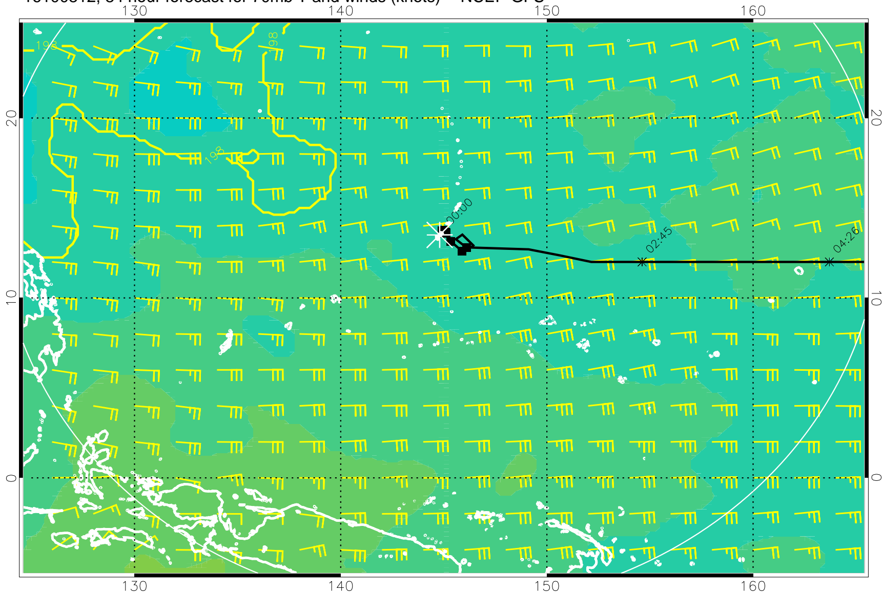
16100812, 84 hour forecast for 70mb T and winds (knots) -- NCEP GFS
