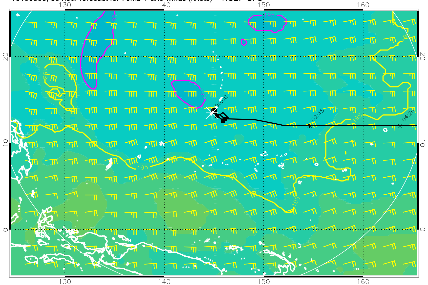
16100606, 30 hour forecast for 70mb T and winds (knots) -- NCEP GFS
