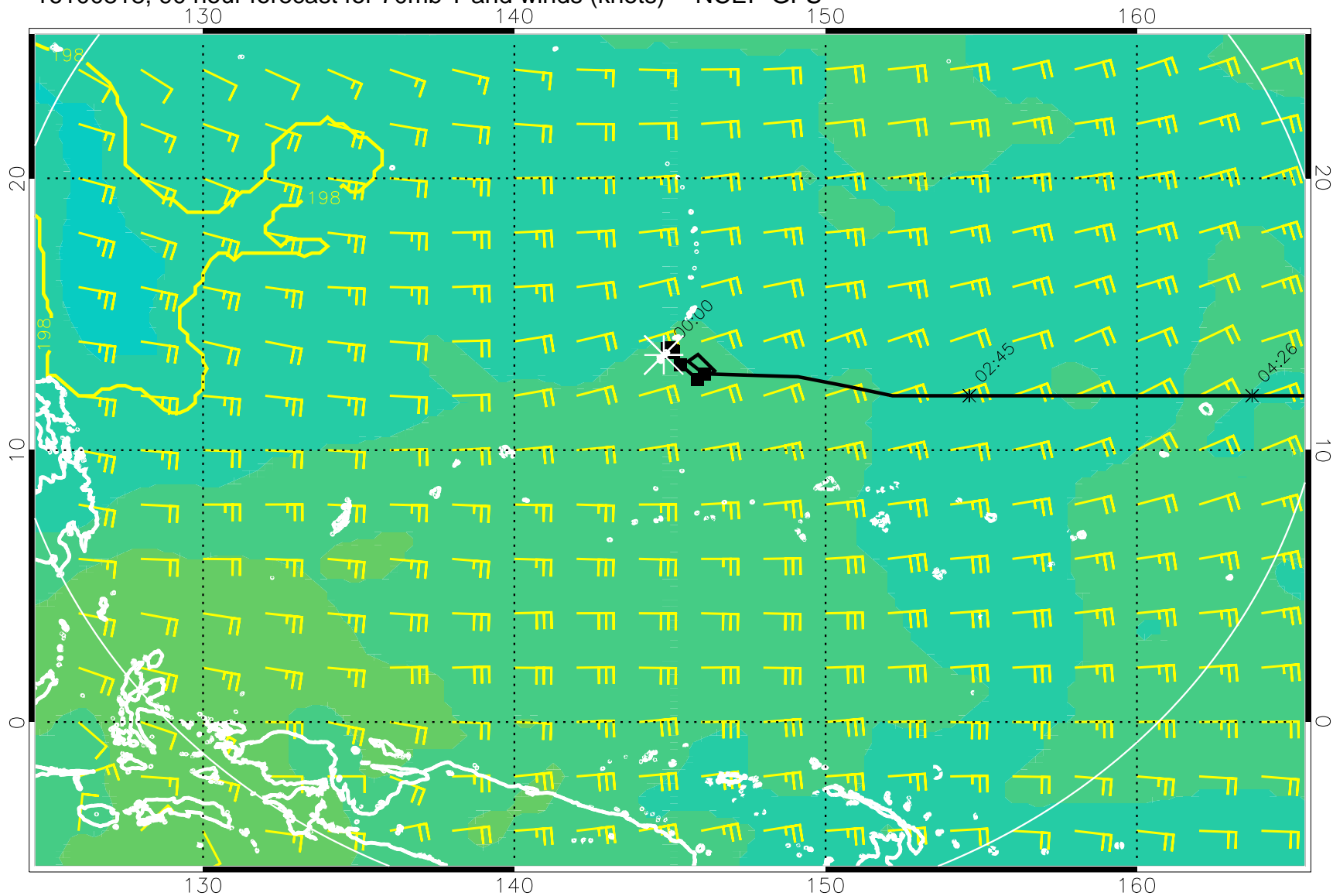
16100818, 90 hour forecast for 70mb T and winds (knots) -- NCEP GFS
