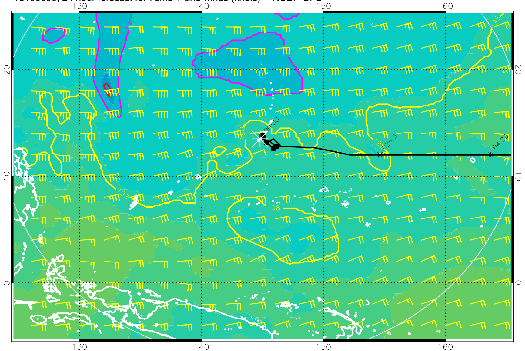
16100600, 24 hour forecast for 70mb T and winds (knots) -- NCEP GFS
