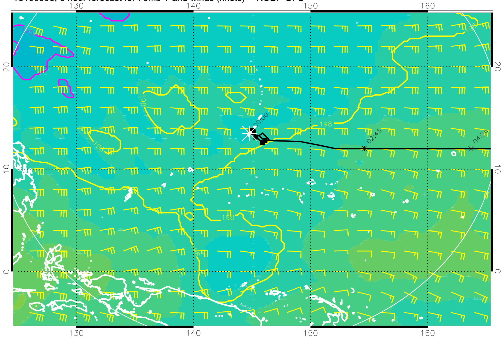
16100506, 6 hour forecast for 70mb T and winds (knots) -- NCEP GFS
