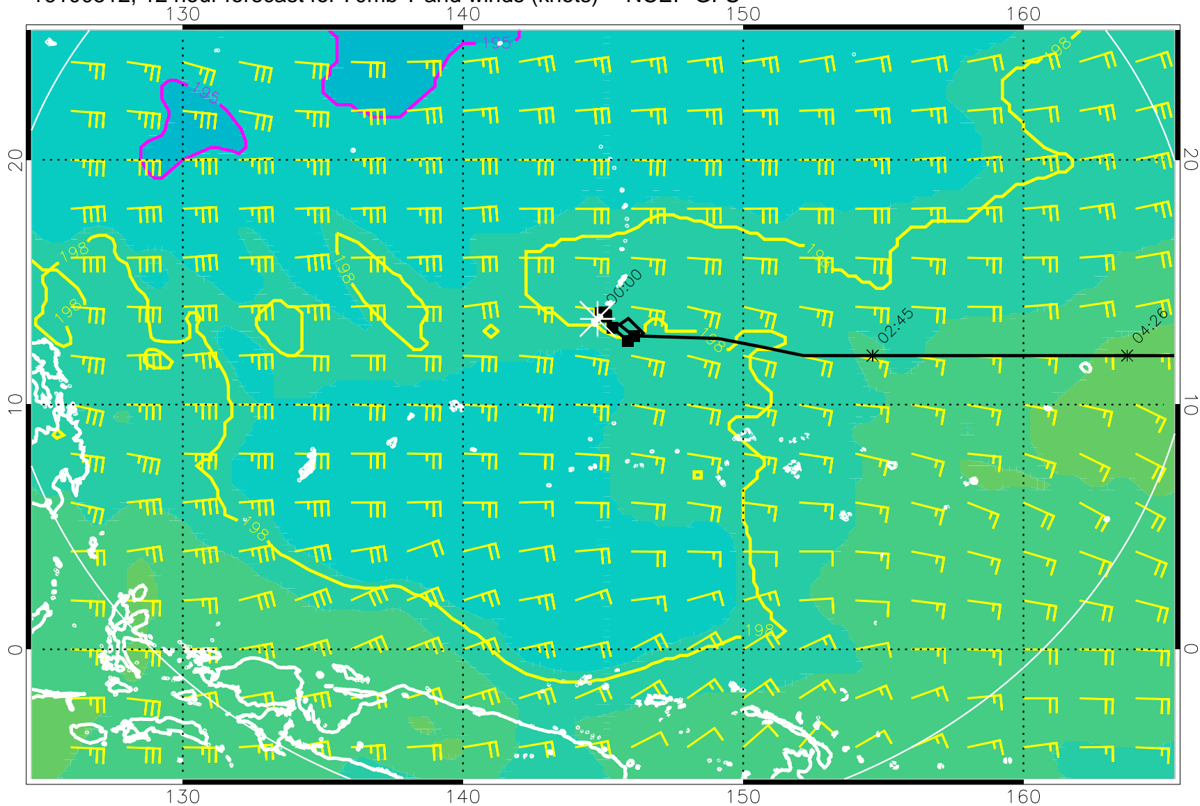
16100512, 12 hour forecast for 70mb T and winds (knots) -- NCEP GFS
