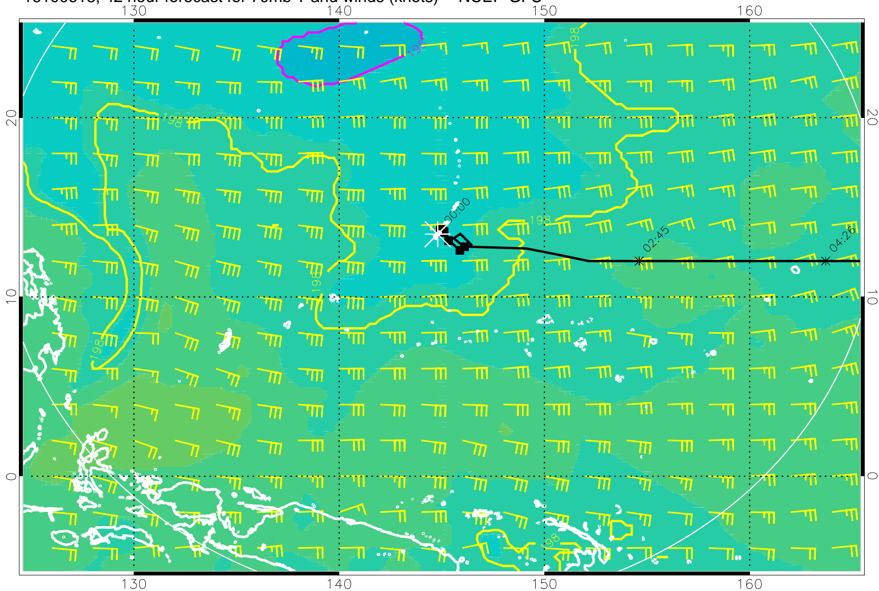
16100618, 42 hour forecast for 70mb T and winds (knots) -- NCEP GFS
