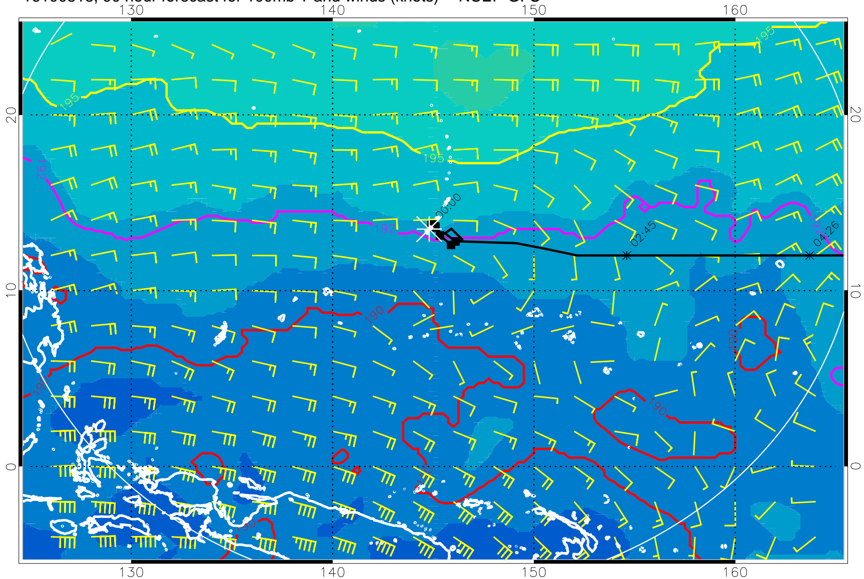
16100818, 90 hour forecast for 100mb T and winds (knots) -- NCEP GFS
