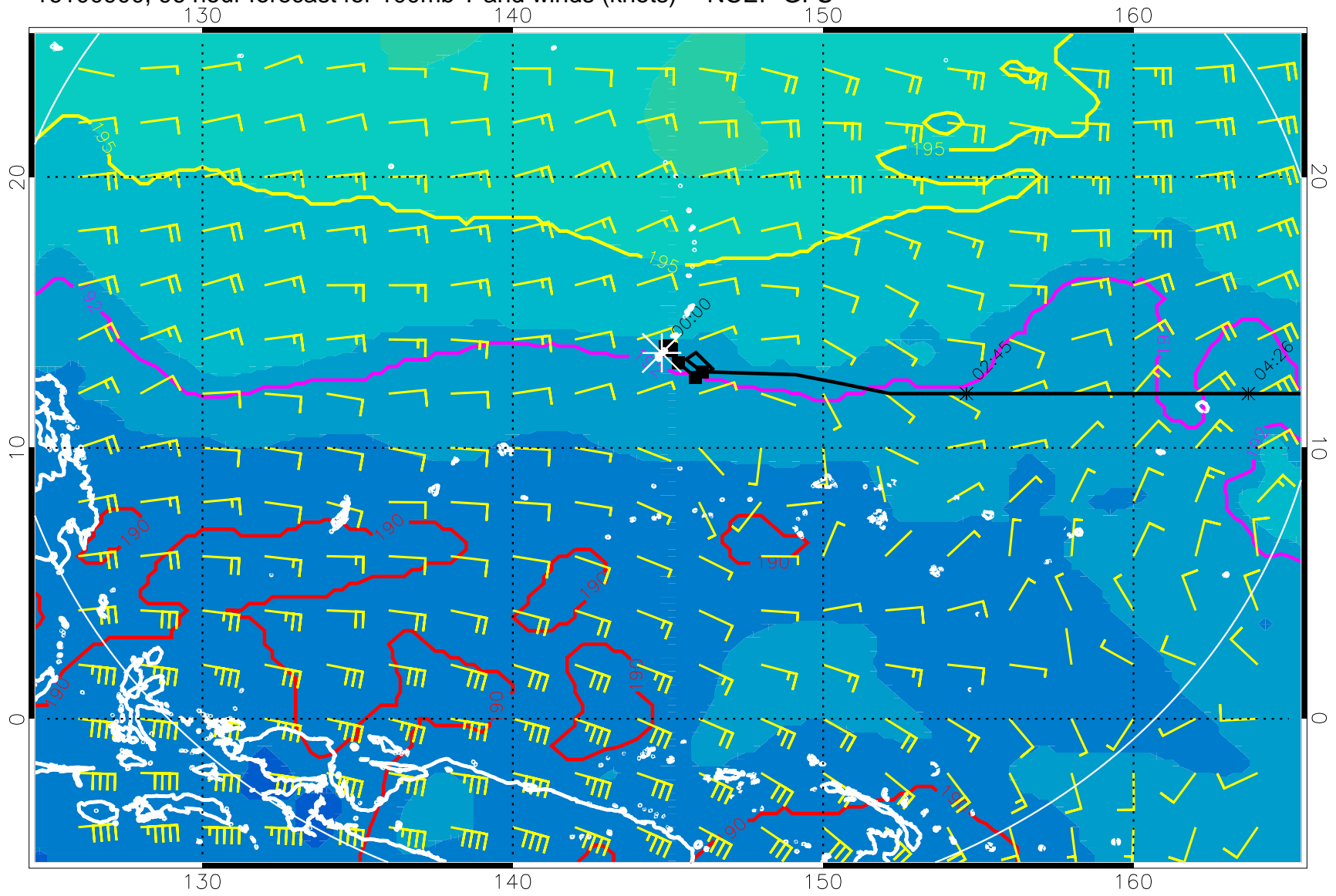
16100900, 96 hour forecast for 100mb T and winds (knots) -- NCEP GFS
