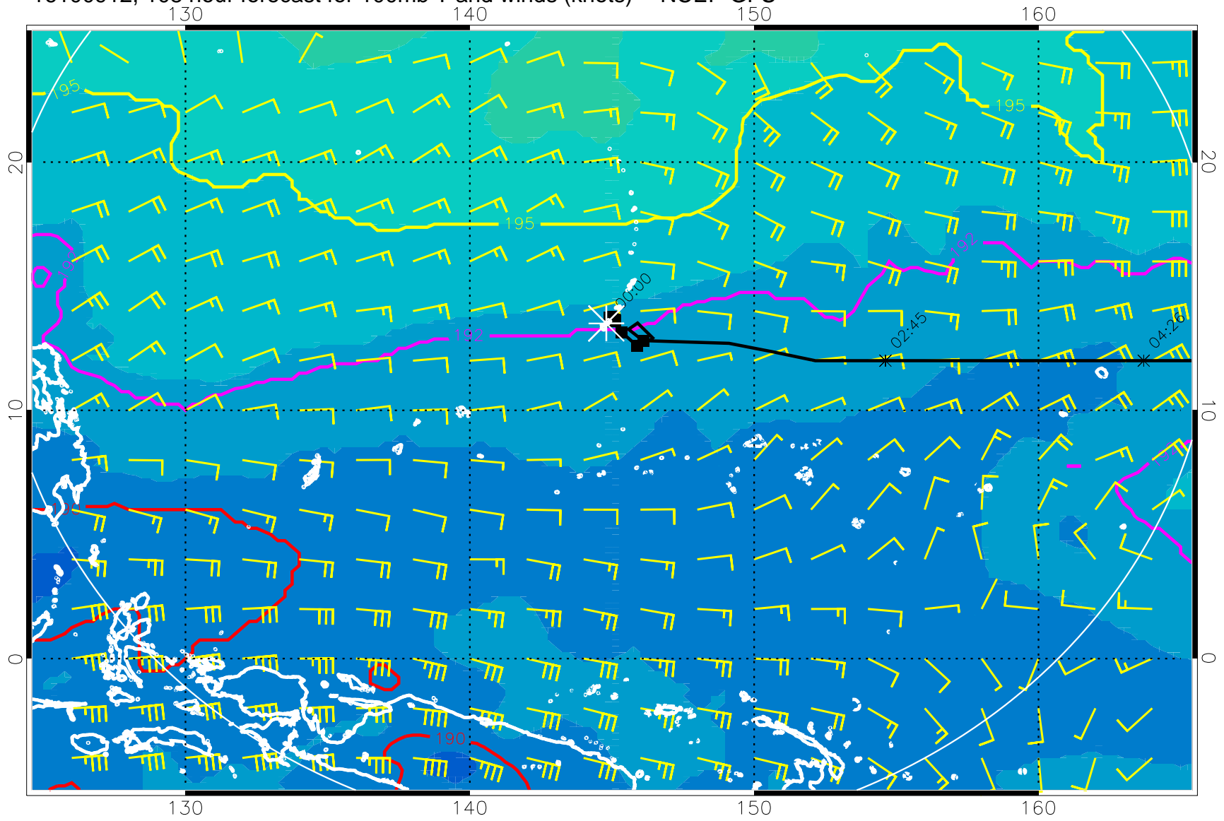
16100912, 108 hour forecast for 100mb T and winds (knots) -- NCEP GFS
