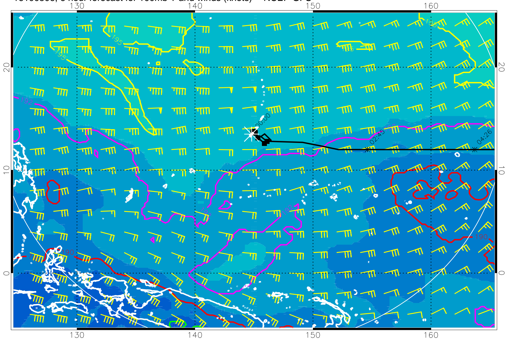
16100506, 6 hour forecast for 100mb T and winds (knots) -- NCEP GFS
