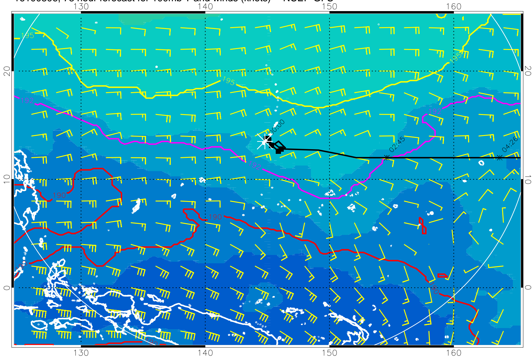
16100806, 78 hour forecast for 100mb T and winds (knots) -- NCEP GFS
