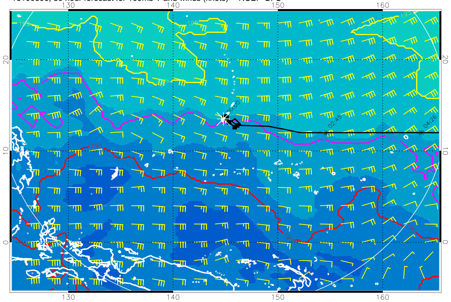
16100606, 30 hour forecast for 100mb T and winds (knots) -- NCEP GFS
