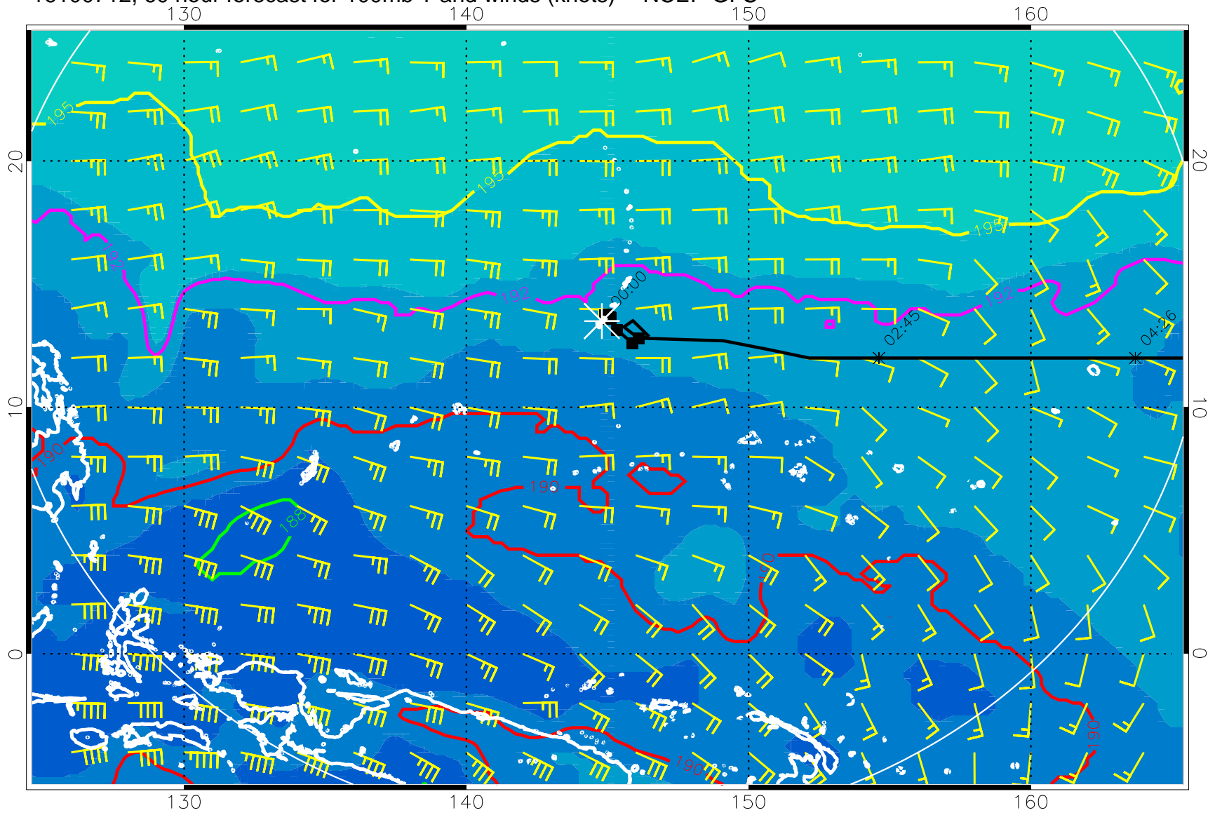
16100712, 60 hour forecast for 100mb T and winds (knots) -- NCEP GFS
