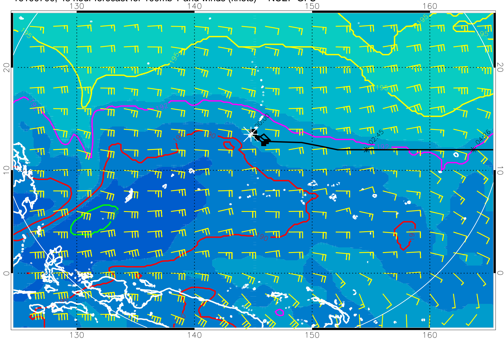
16100700, 48 hour forecast for 100mb T and winds (knots) -- NCEP GFS
