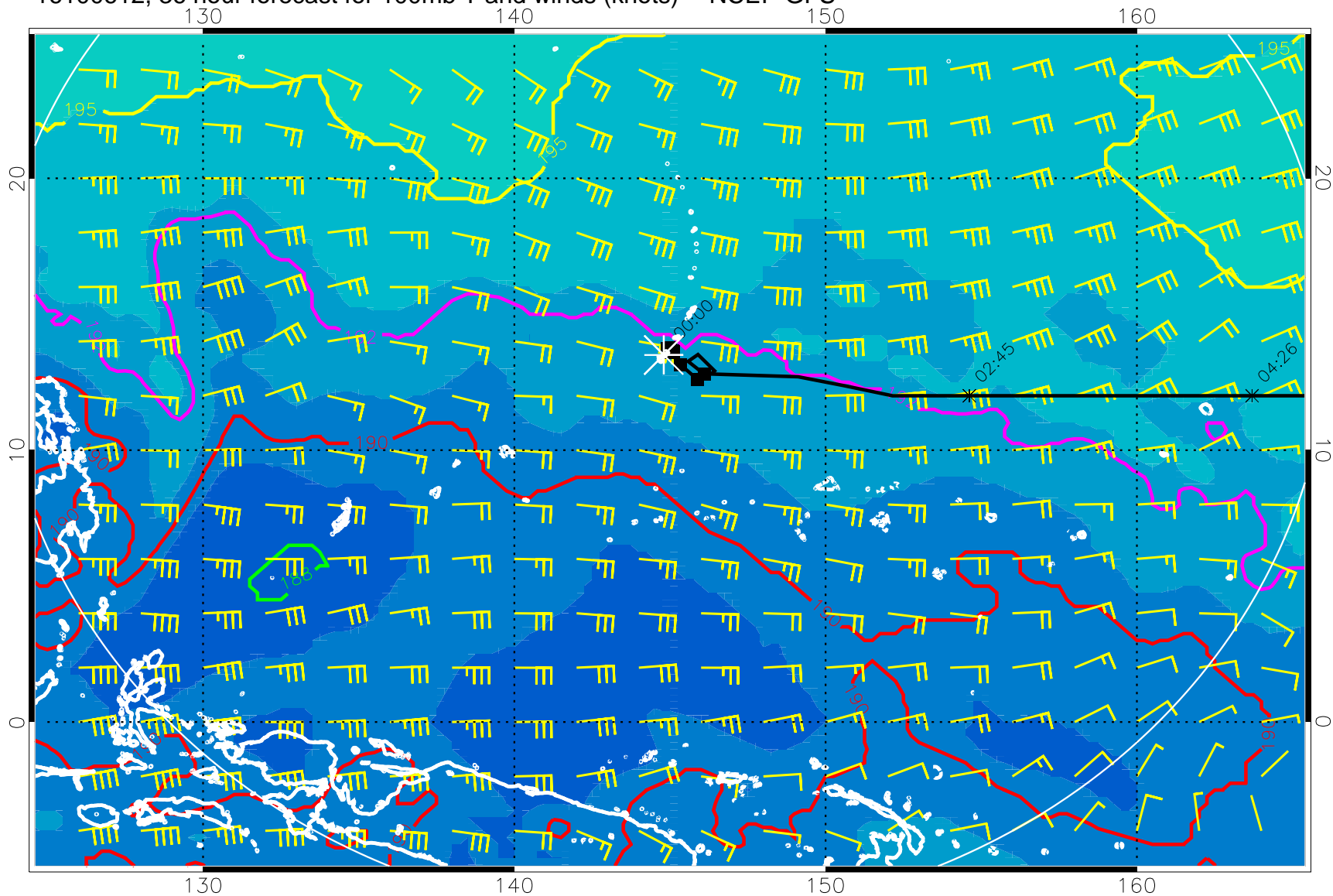
16100612, 36 hour forecast for 100mb T and winds (knots) -- NCEP GFS
