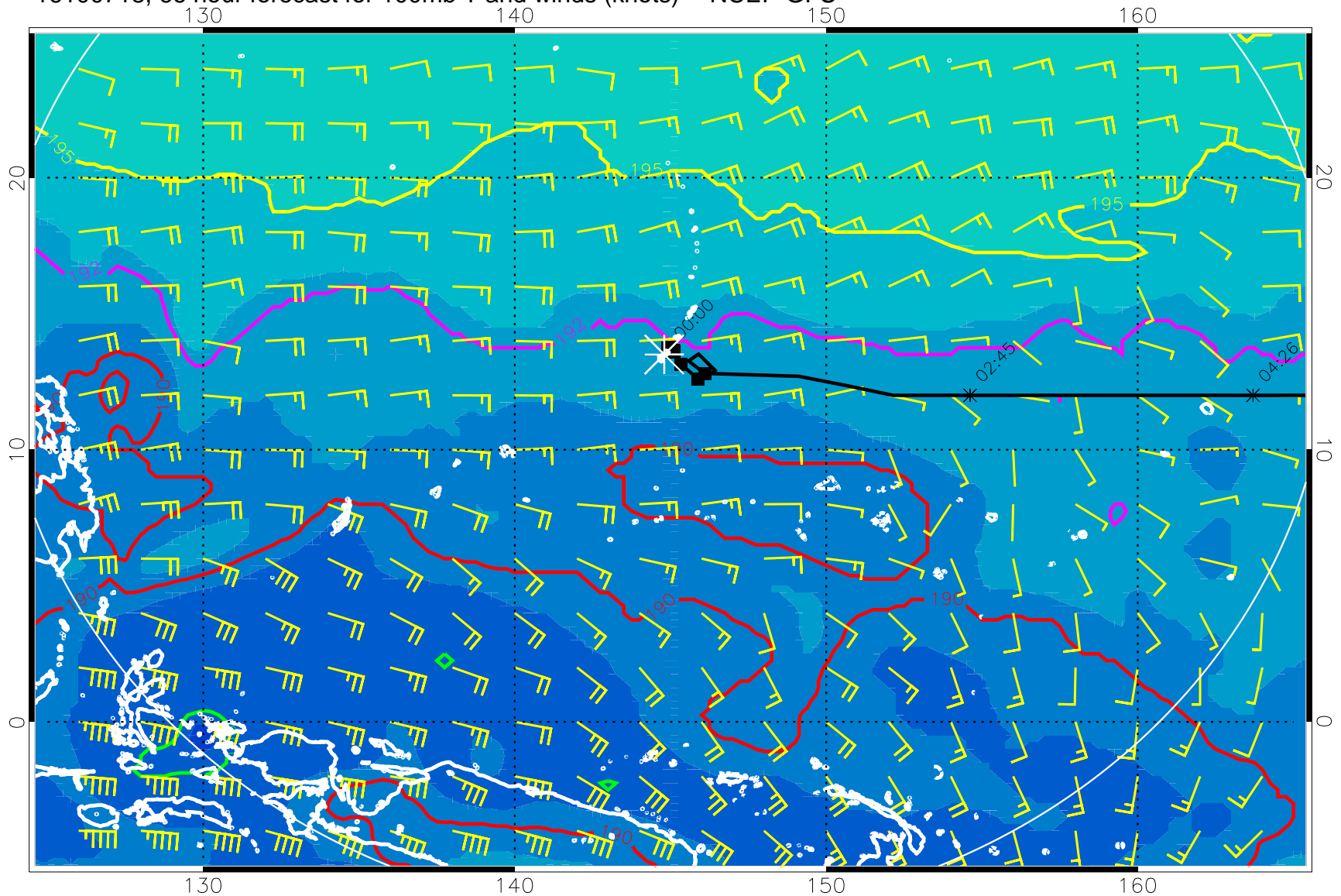
16100718, 66 hour forecast for 100mb T and winds (knots) -- NCEP GFS
