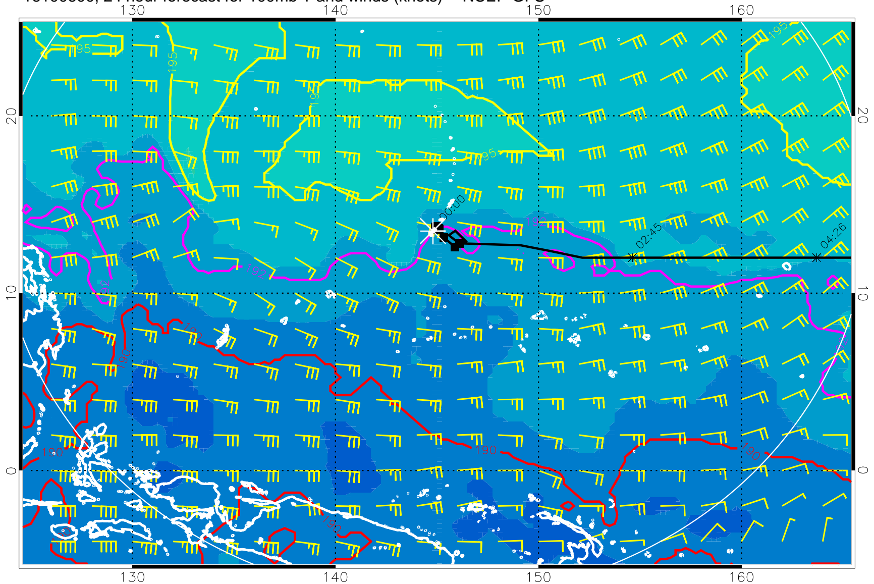
16100600, 24 hour forecast for 100mb T and winds (knots) -- NCEP GFS
