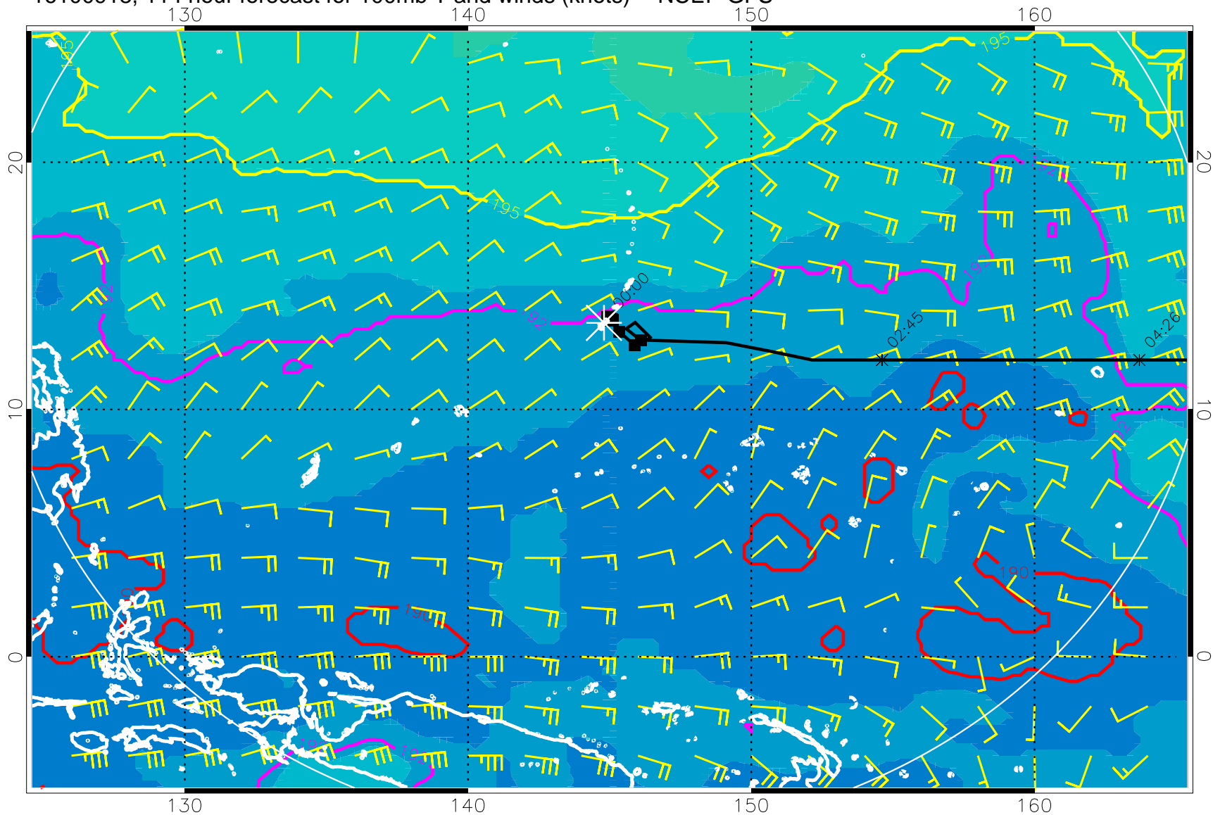
16100918, 114 hour forecast for 100mb T and winds (knots) -- NCEP GFS
