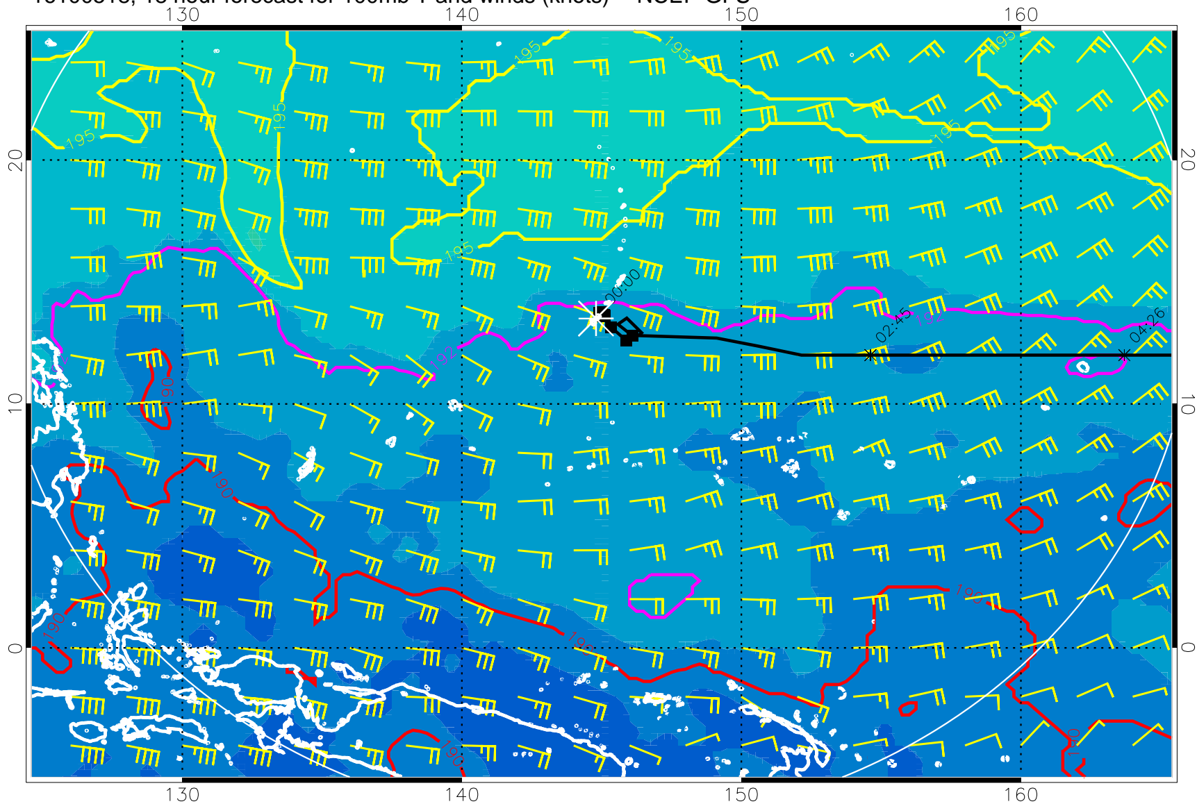
16100518, 18 hour forecast for 100mb T and winds (knots) -- NCEP GFS
