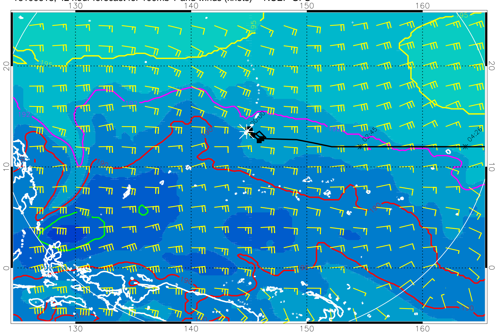
16100618, 42 hour forecast for 100mb T and winds (knots) -- NCEP GFS
