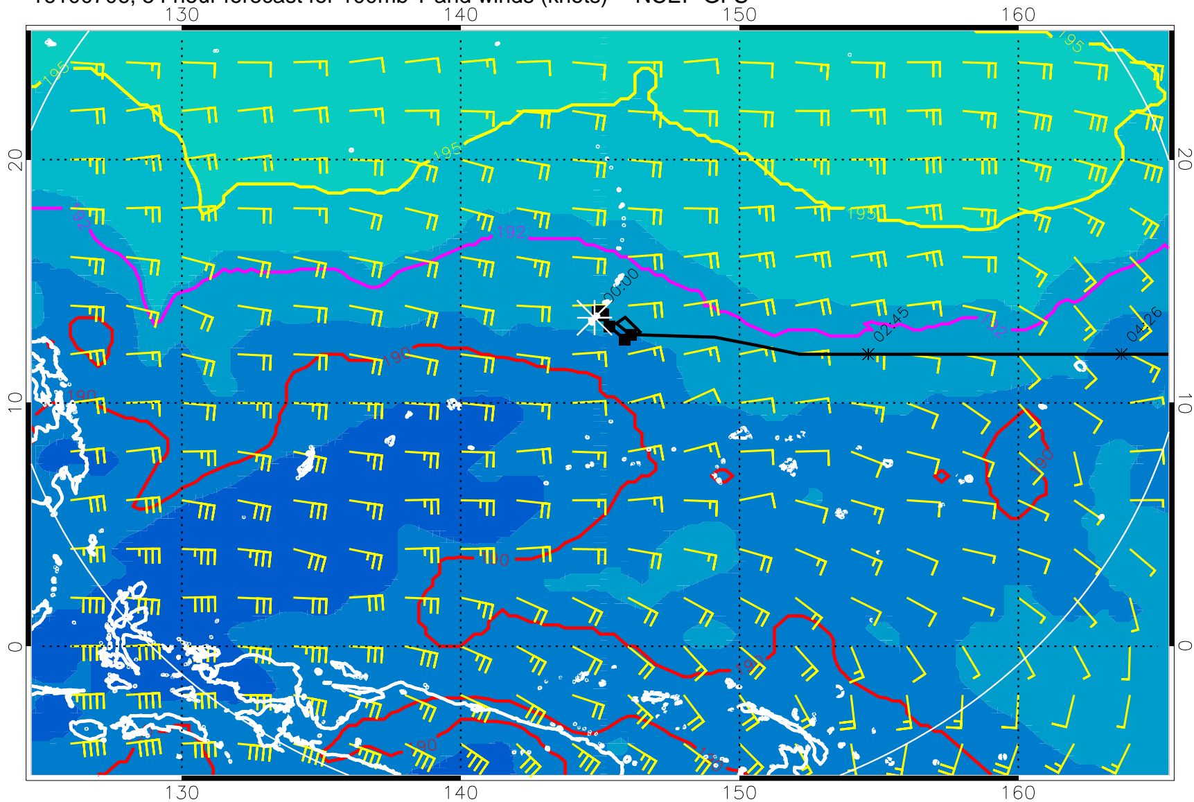
16100706, 54 hour forecast for 100mb T and winds (knots) -- NCEP GFS
