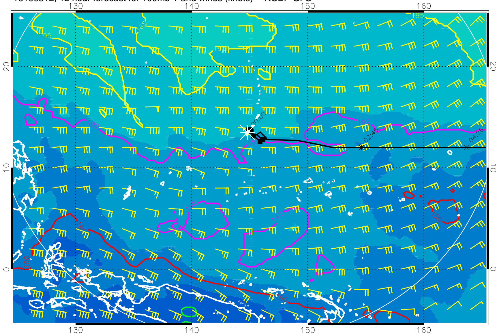
16100512, 12 hour forecast for 100mb T and winds (knots) -- NCEP GFS
