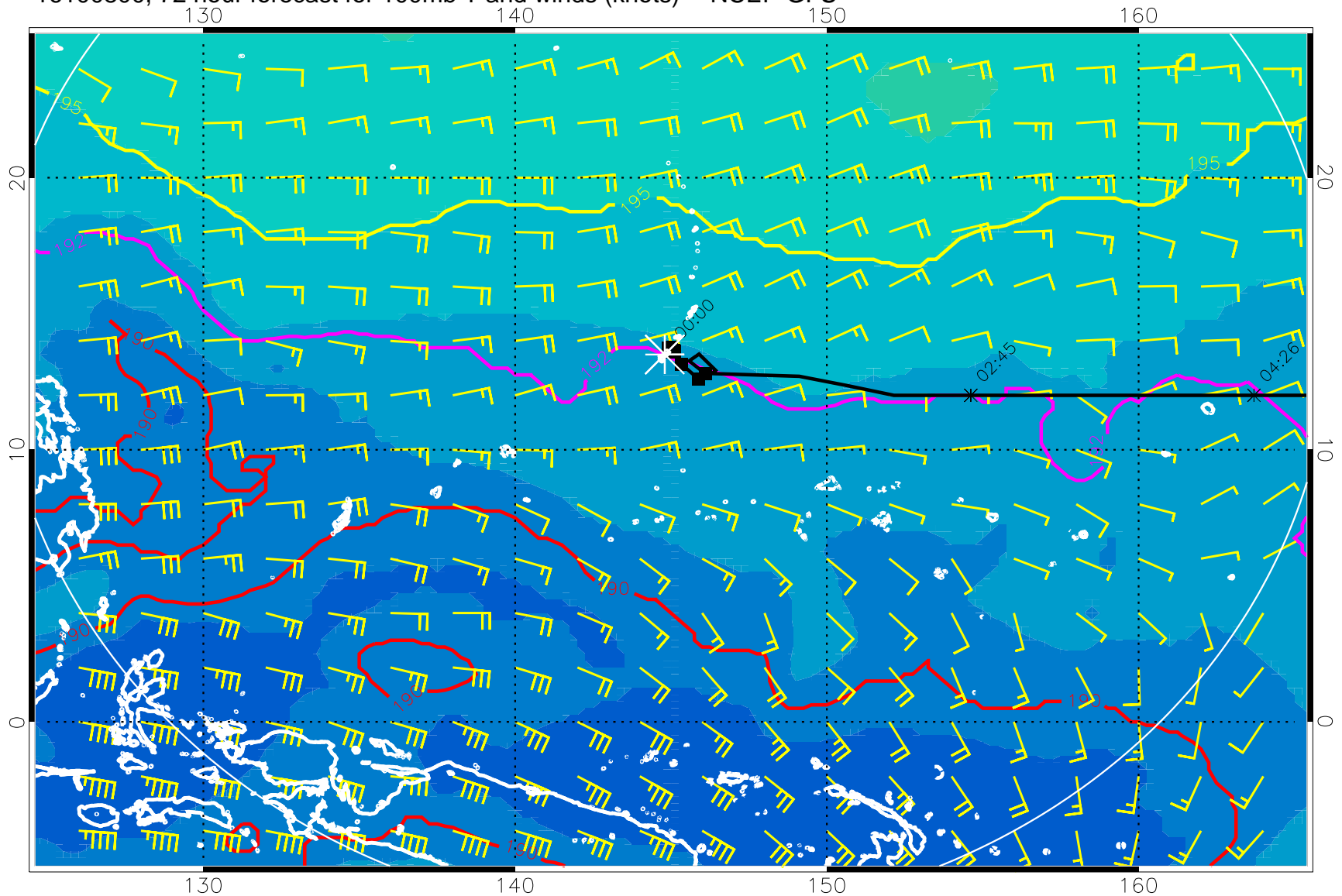
16100800, 72 hour forecast for 100mb T and winds (knots) -- NCEP GFS
