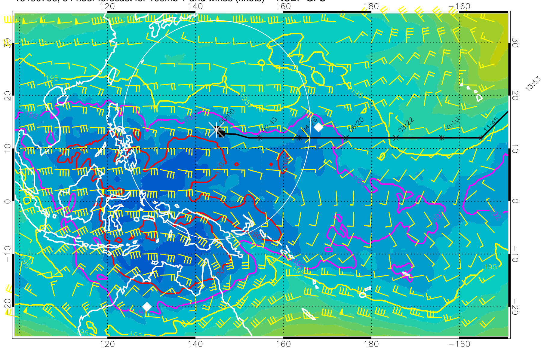
16100706, 54 hour forecast for 100mb T and winds (knots) -- NCEP GFS
