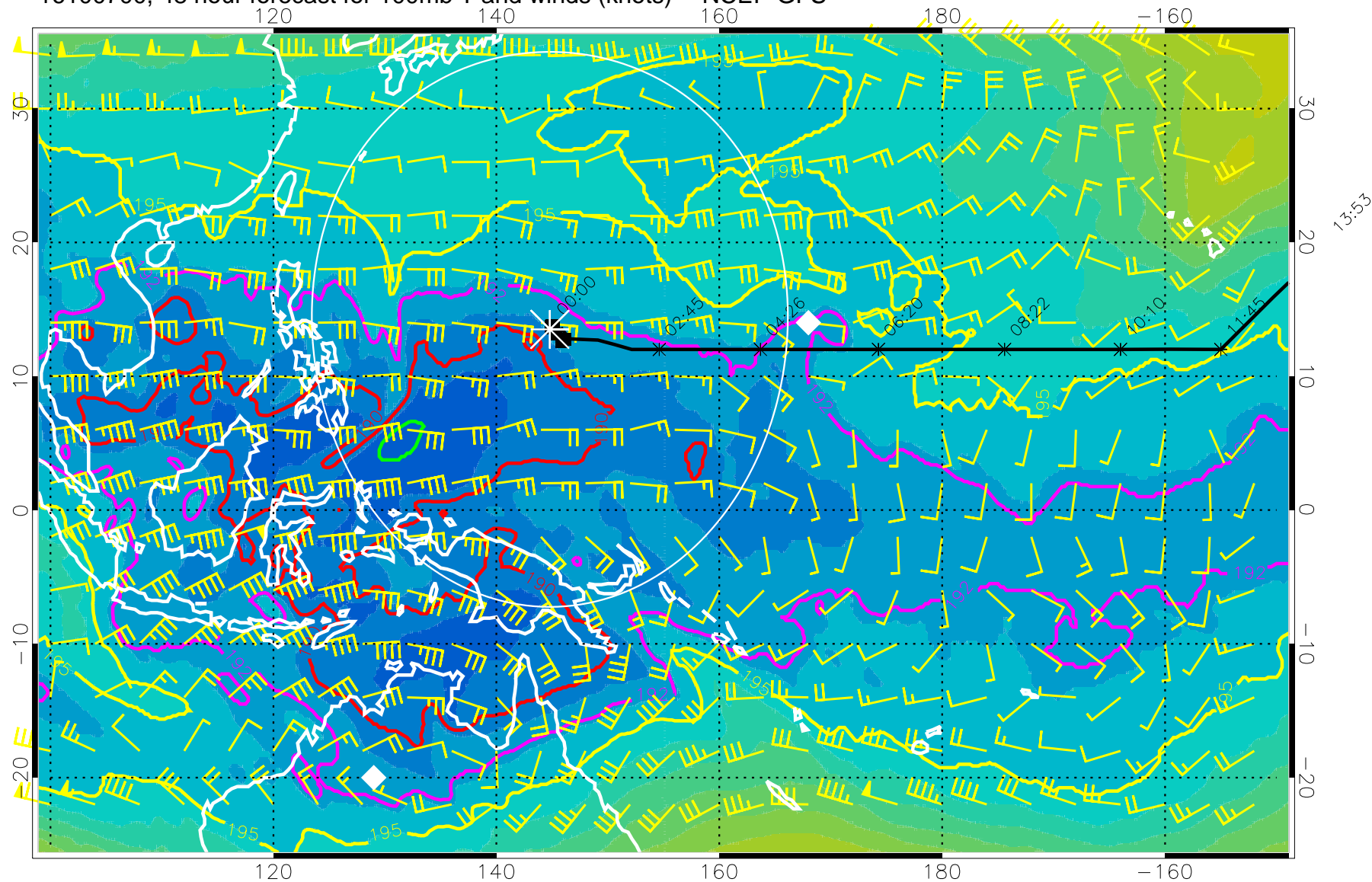
16100700, 48 hour forecast for 100mb T and winds (knots) -- NCEP GFS
