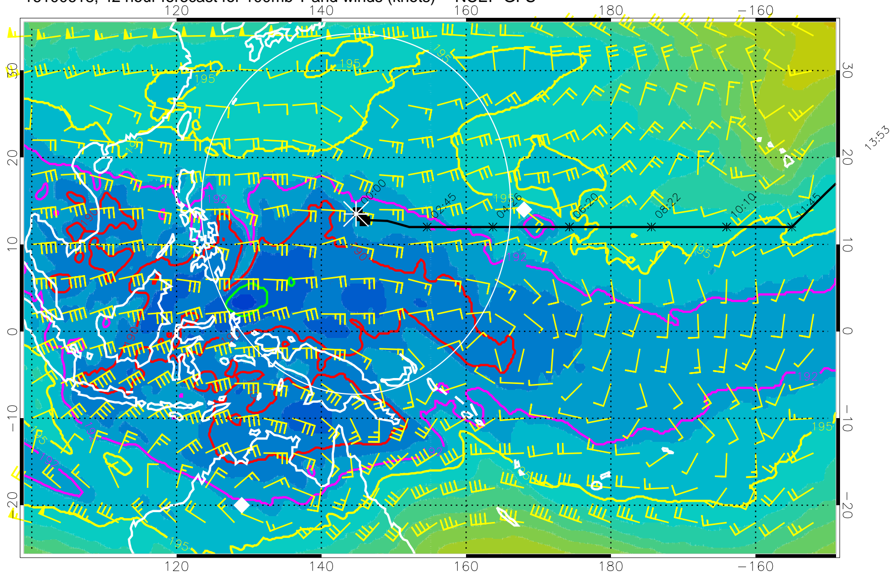
16100618, 42 hour forecast for 100mb T and winds (knots) -- NCEP GFS
