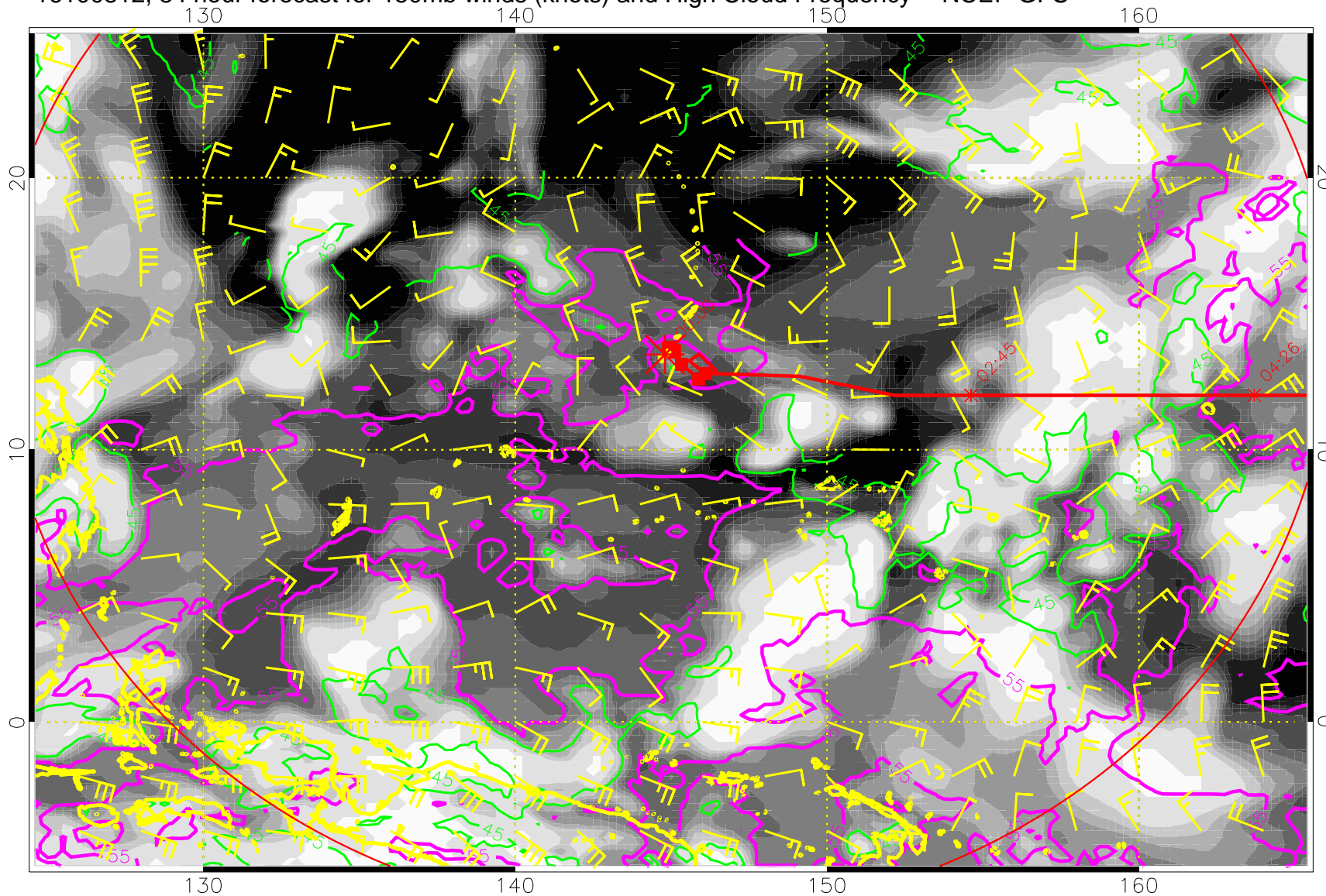
16100812, 84 hour forecast for 150mb winds (knots) and High Cloud Frequency -- NCEP GFS
