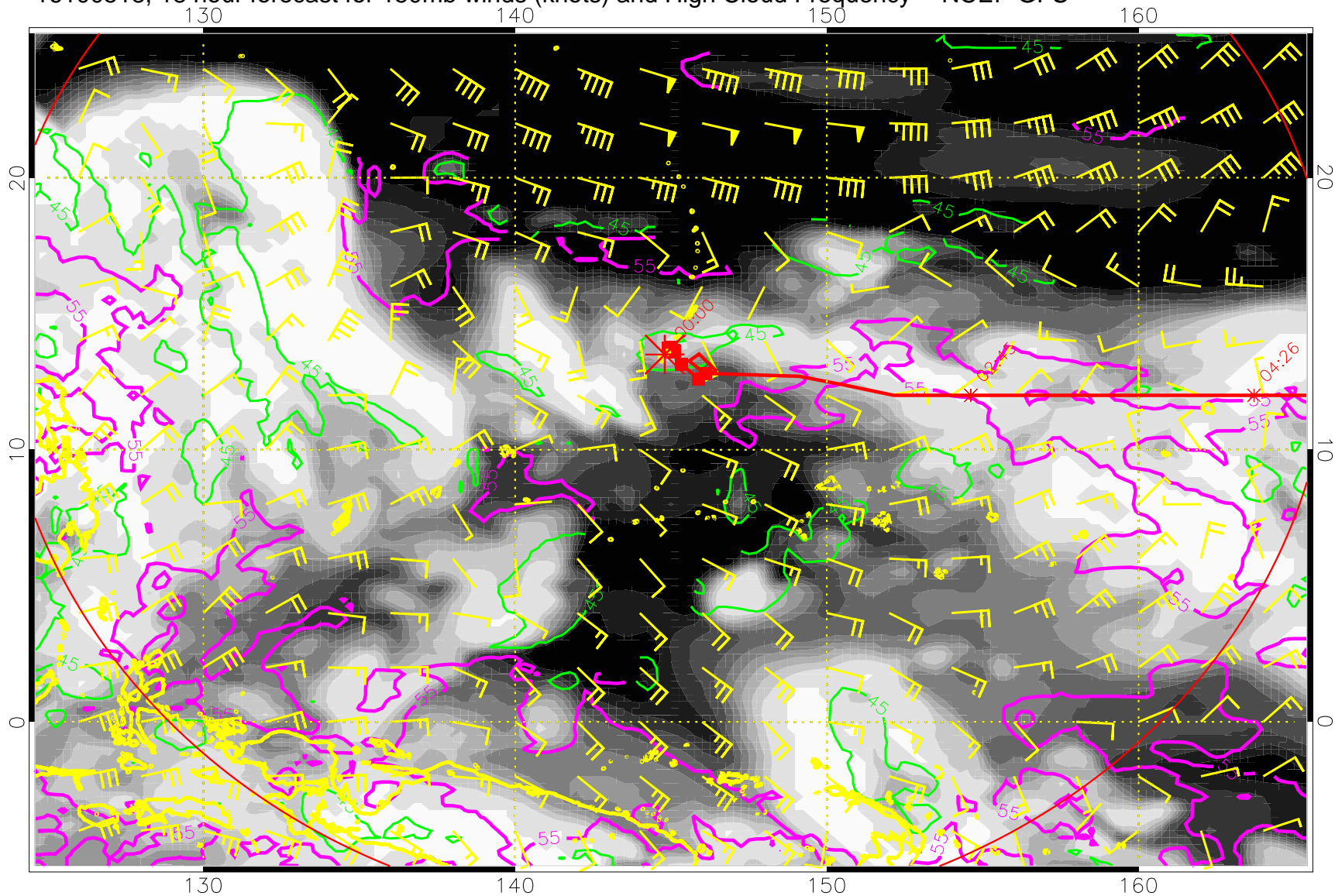
16100518, 18 hour forecast for 150mb winds (knots) and High Cloud Frequency -- NCEP GFS
