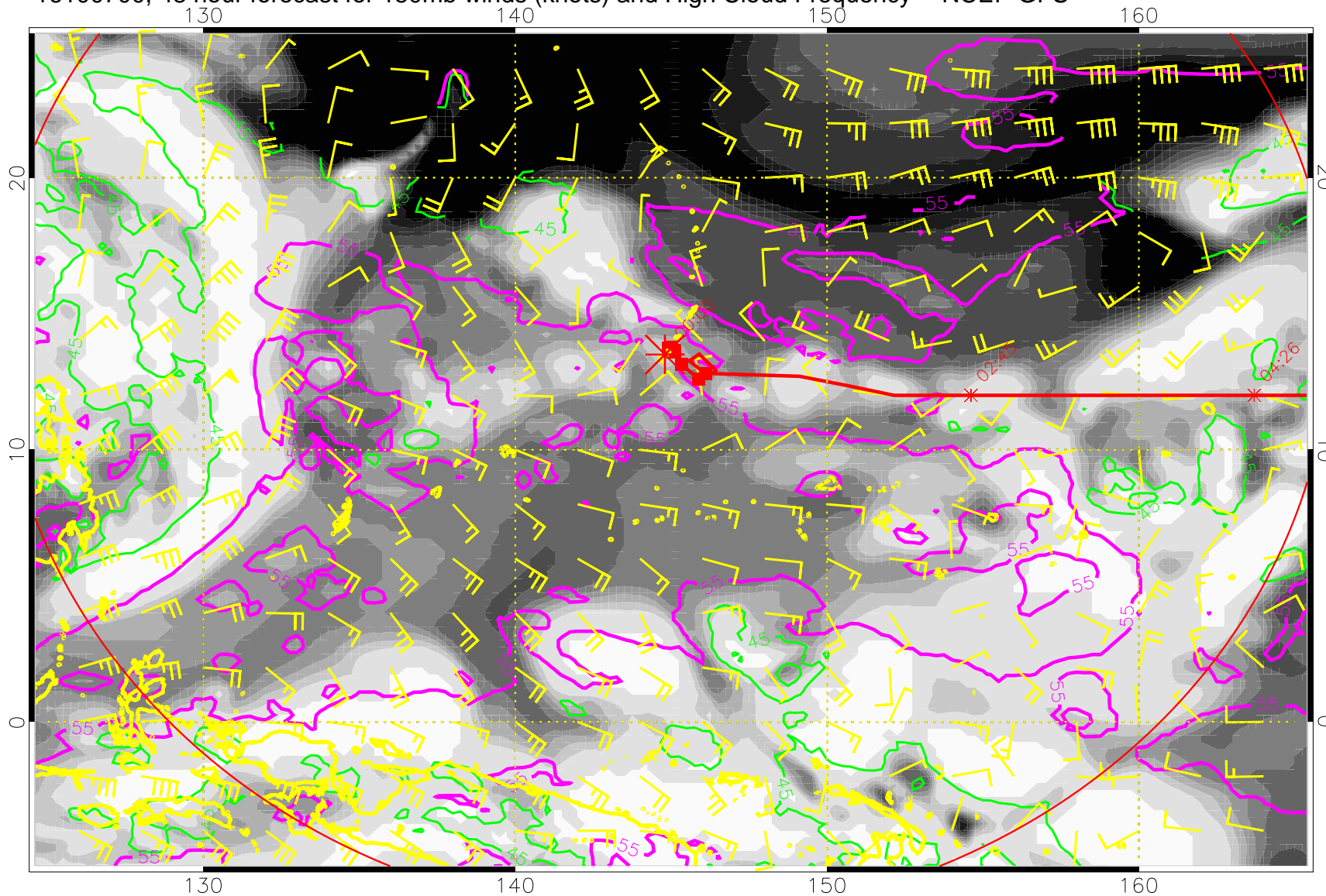
16100700, 48 hour forecast for 150mb winds (knots) and High Cloud Frequency -- NCEP GFS
