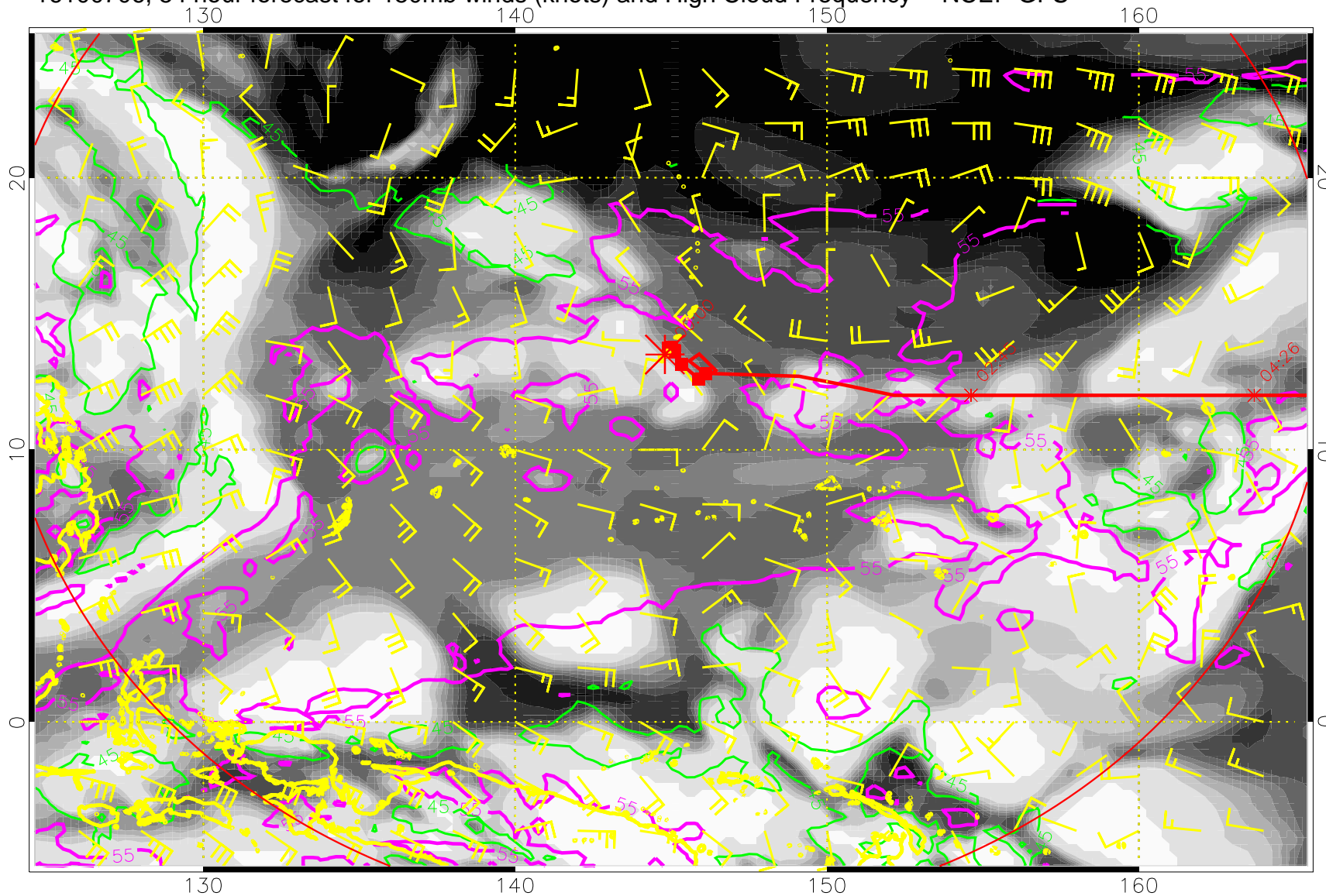
16100706, 54 hour forecast for 150mb winds (knots) and High Cloud Frequency -- NCEP GFS
