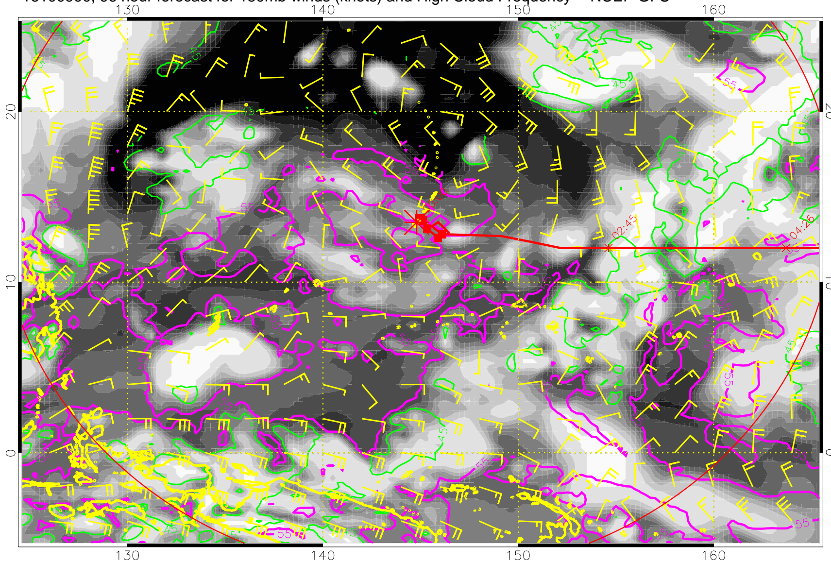
16100900, 96 hour forecast for 150mb winds (knots) and High Cloud Frequency -- NCEP GFS
