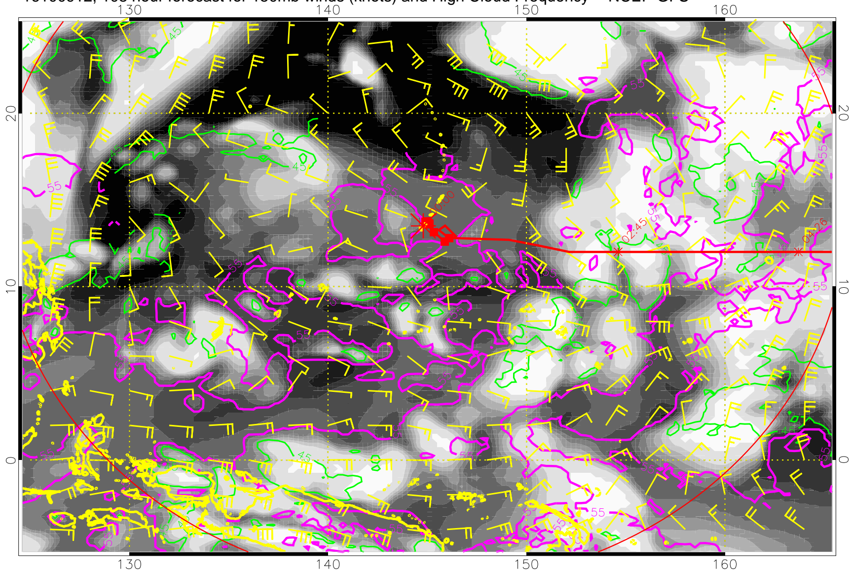
16100912, 108 hour forecast for 150mb winds (knots) and High Cloud Frequency -- NCEP GFS
