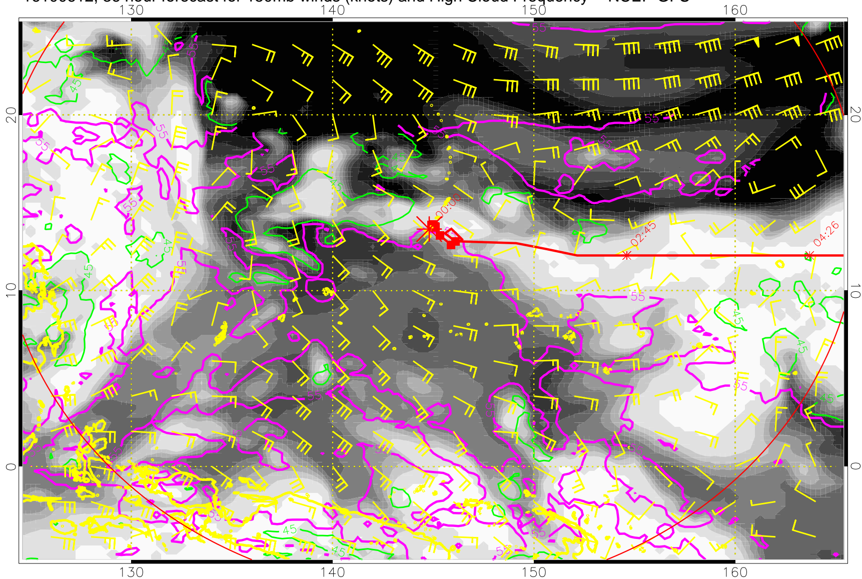
16100612, 36 hour forecast for 150mb winds (knots) and High Cloud Frequency -- NCEP GFS
