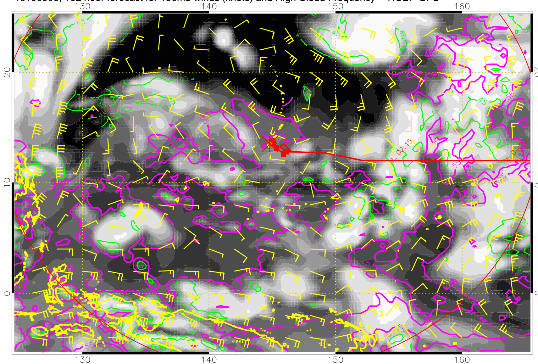
16100906, 102 hour forecast for 150mb winds (knots) and High Cloud Frequency -- NCEP GFS
