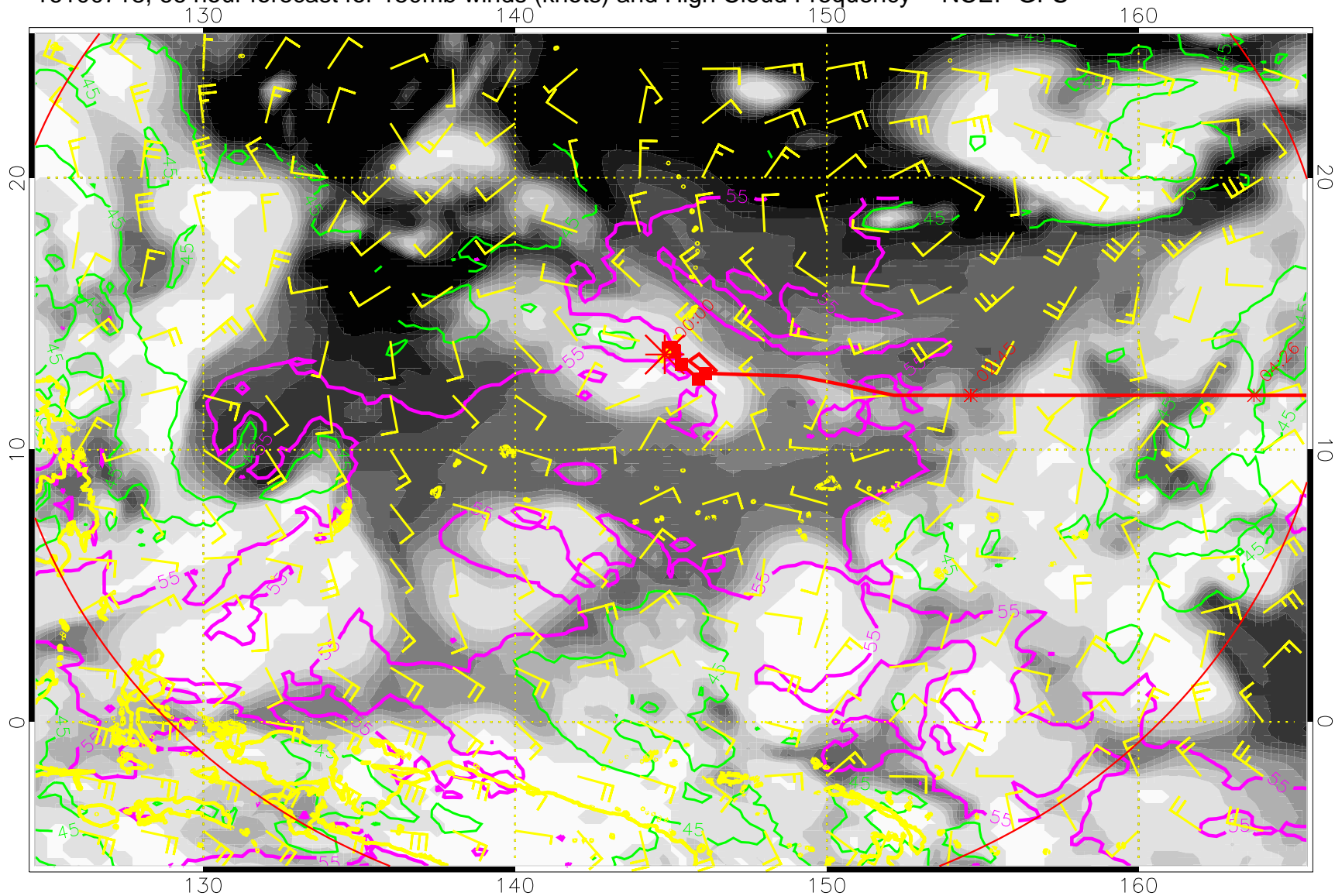
16100718, 66 hour forecast for 150mb winds (knots) and High Cloud Frequency -- NCEP GFS
