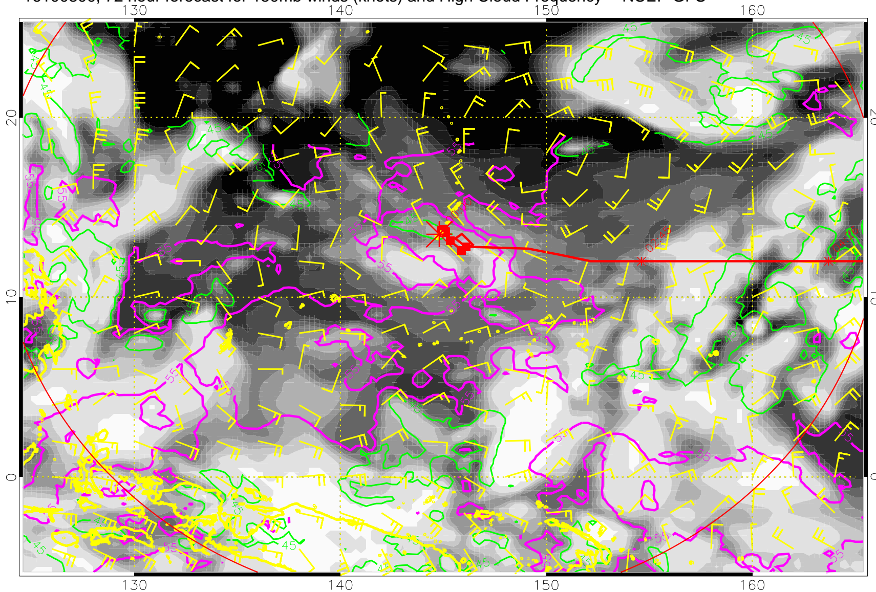
16100800, 72 hour forecast for 150mb winds (knots) and High Cloud Frequency -- NCEP GFS
