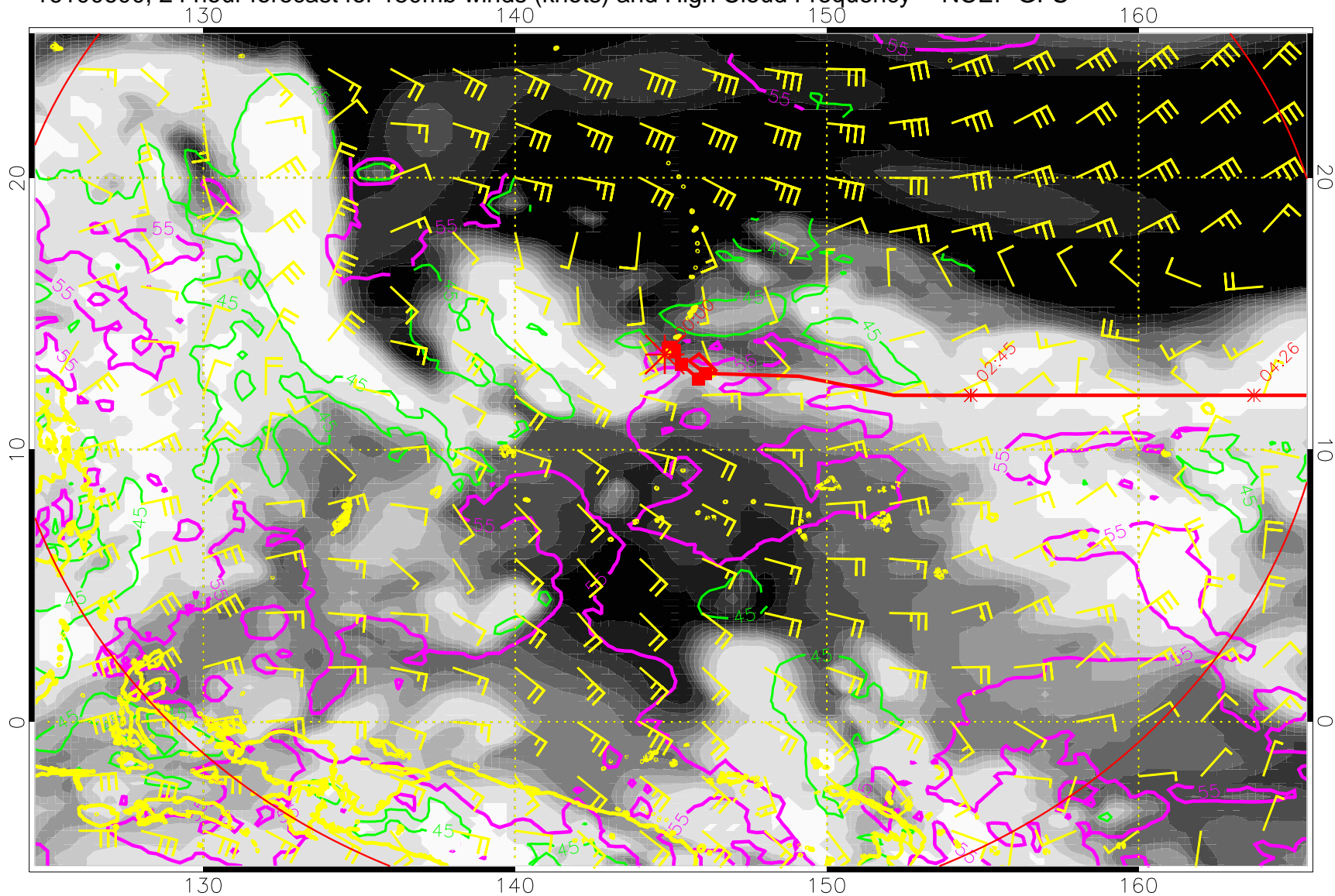
16100600, 24 hour forecast for 150mb winds (knots) and High Cloud Frequency -- NCEP GFS
