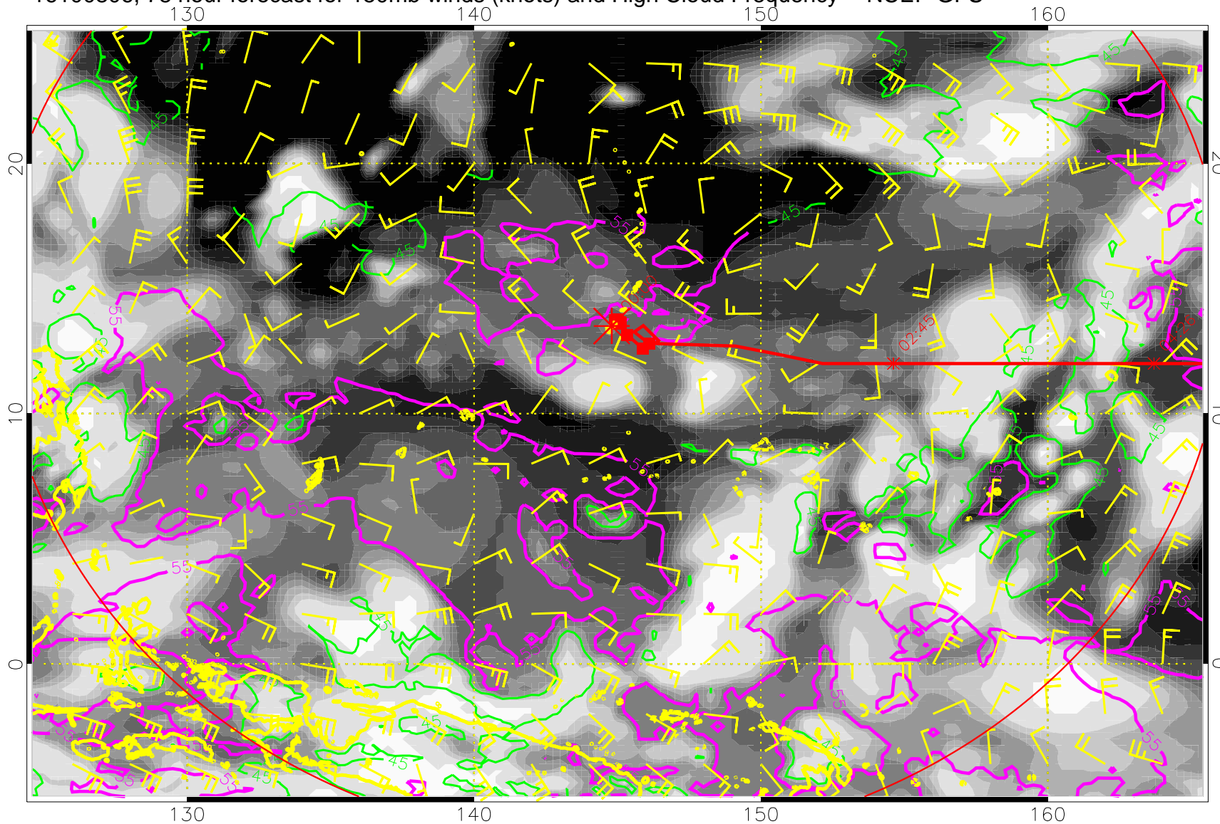
16100806, 78 hour forecast for 150mb winds (knots) and High Cloud Frequency -- NCEP GFS
