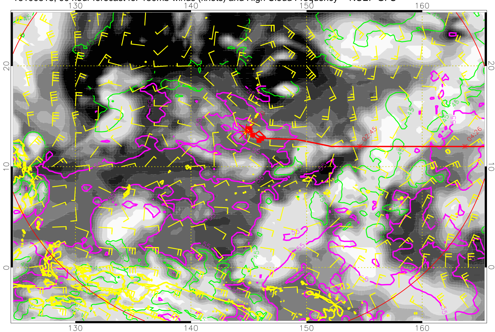
16100818, 90 hour forecast for 150mb winds (knots) and High Cloud Frequency -- NCEP GFS
