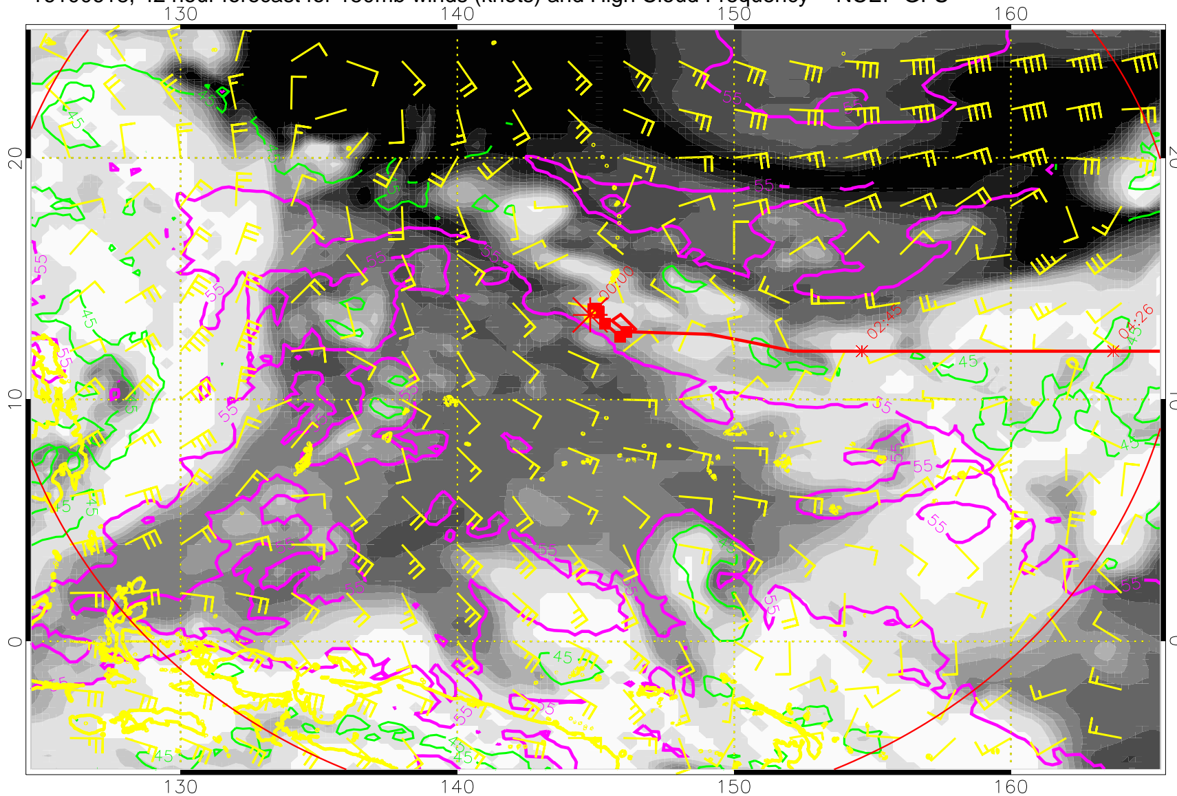
16100618, 42 hour forecast for 150mb winds (knots) and High Cloud Frequency -- NCEP GFS
