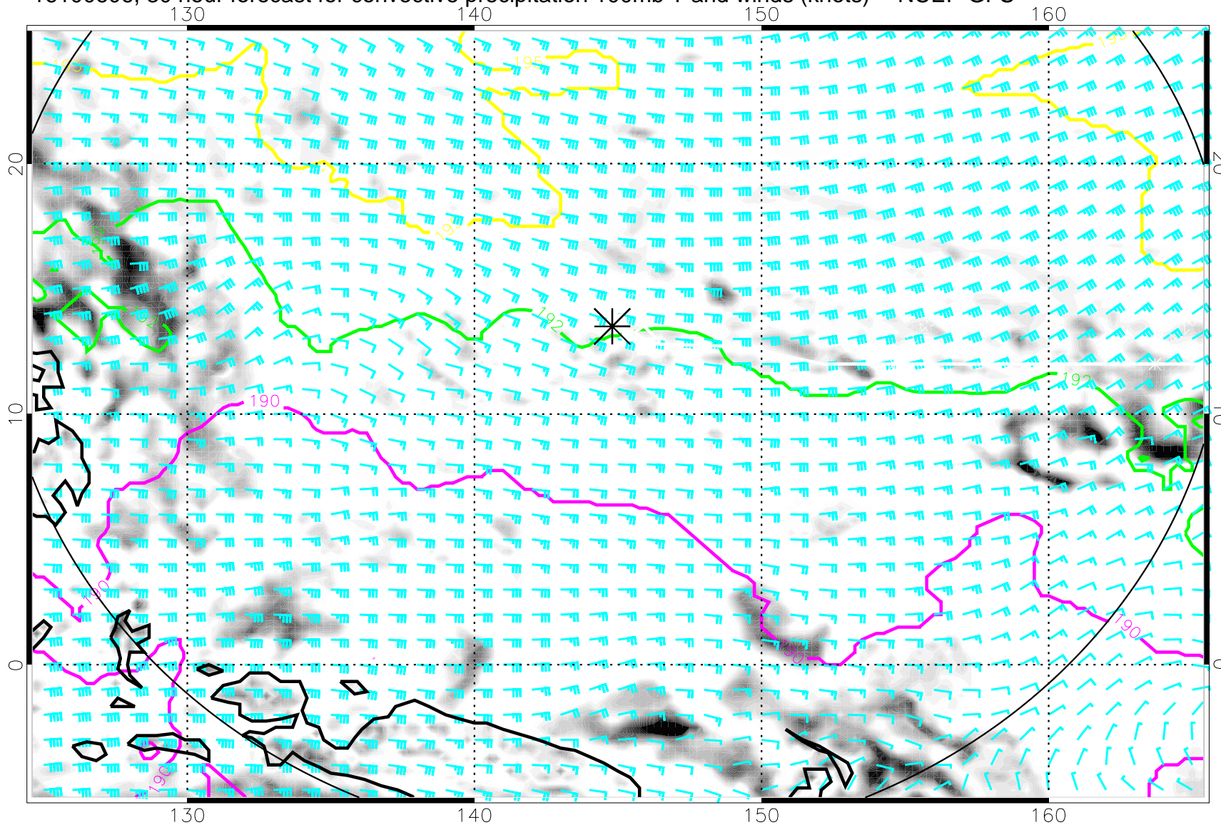
16100606, 30 hour forecast for convective precipitation 100mb T and winds (knots) -- NCEP GFS
