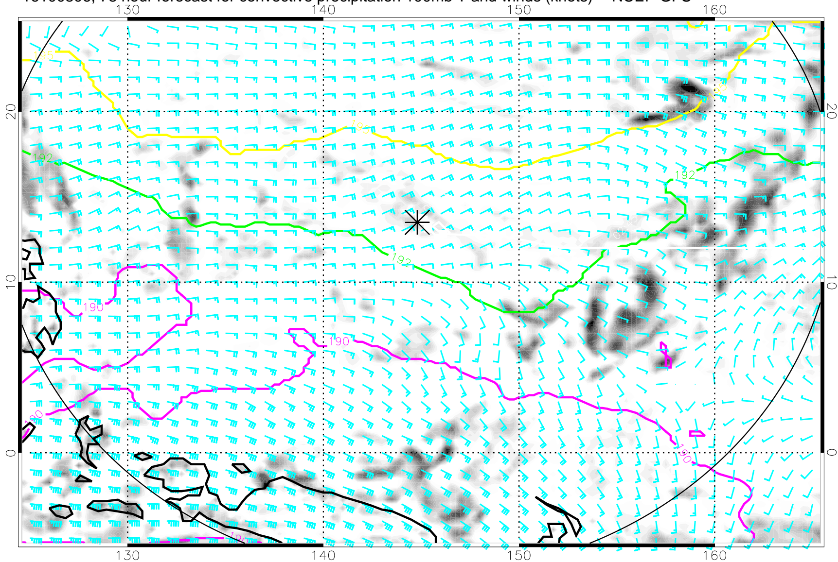
16100806, 78 hour forecast for convective precipitation 100mb T and winds (knots) -- NCEP GFS
