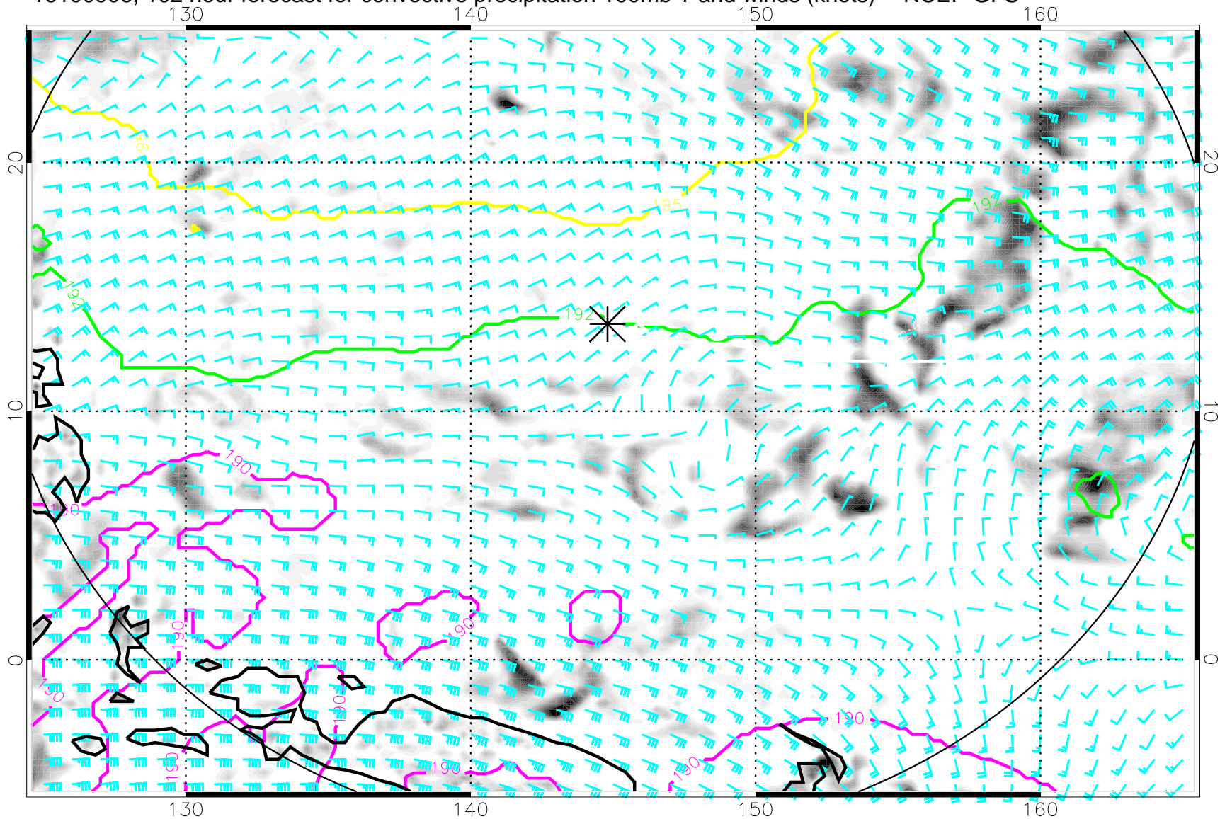
16100906, 102 hour forecast for convective precipitation 100mb T and winds (knots) -- NCEP GFS
