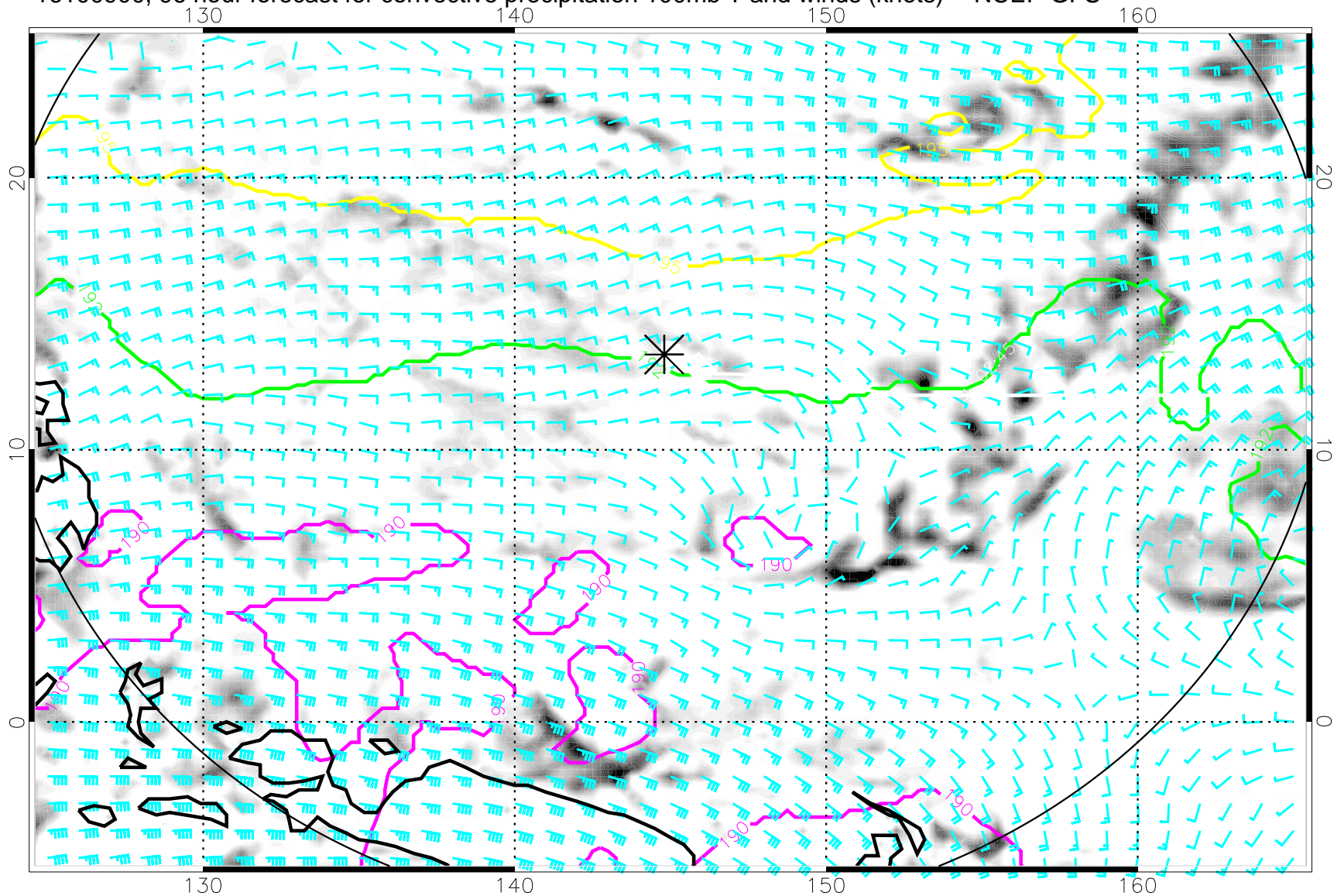
16100900, 96 hour forecast for convective precipitation 100mb T and winds (knots) -- NCEP GFS
