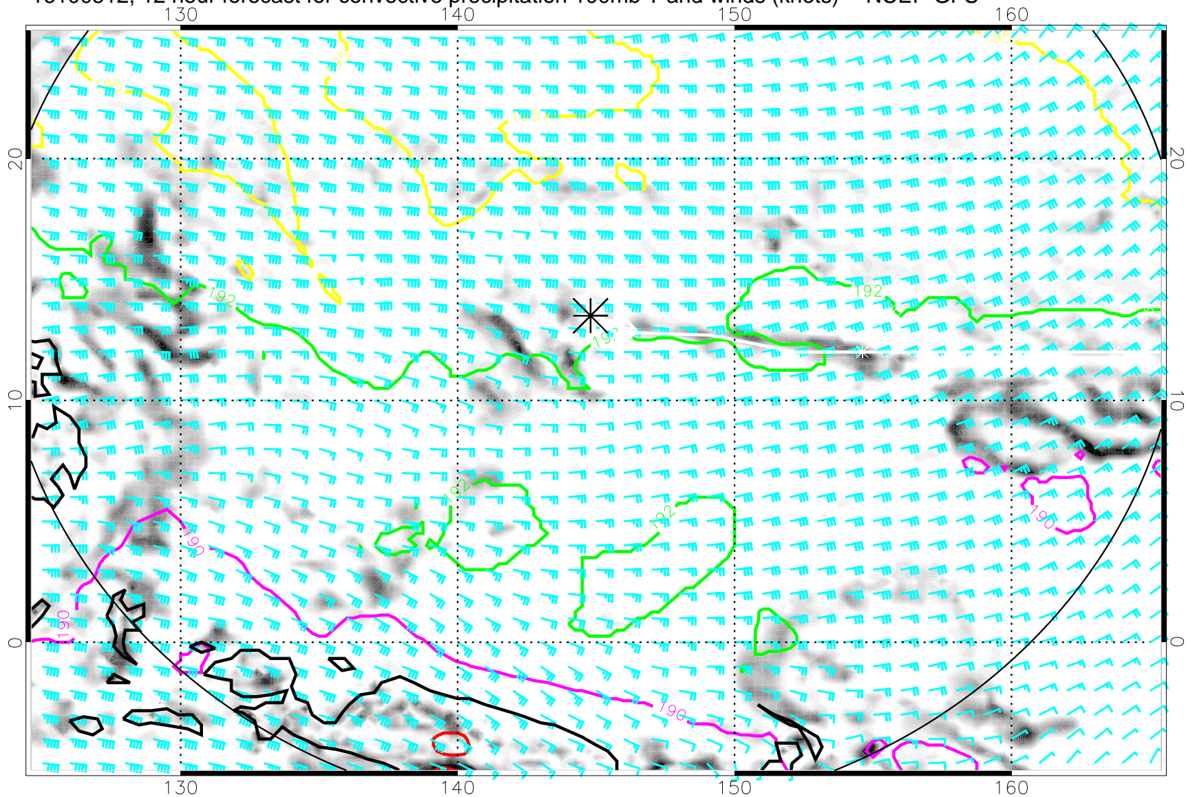
16100512, 12 hour forecast for convective precipitation 100mb T and winds (knots) -- NCEP GFS
