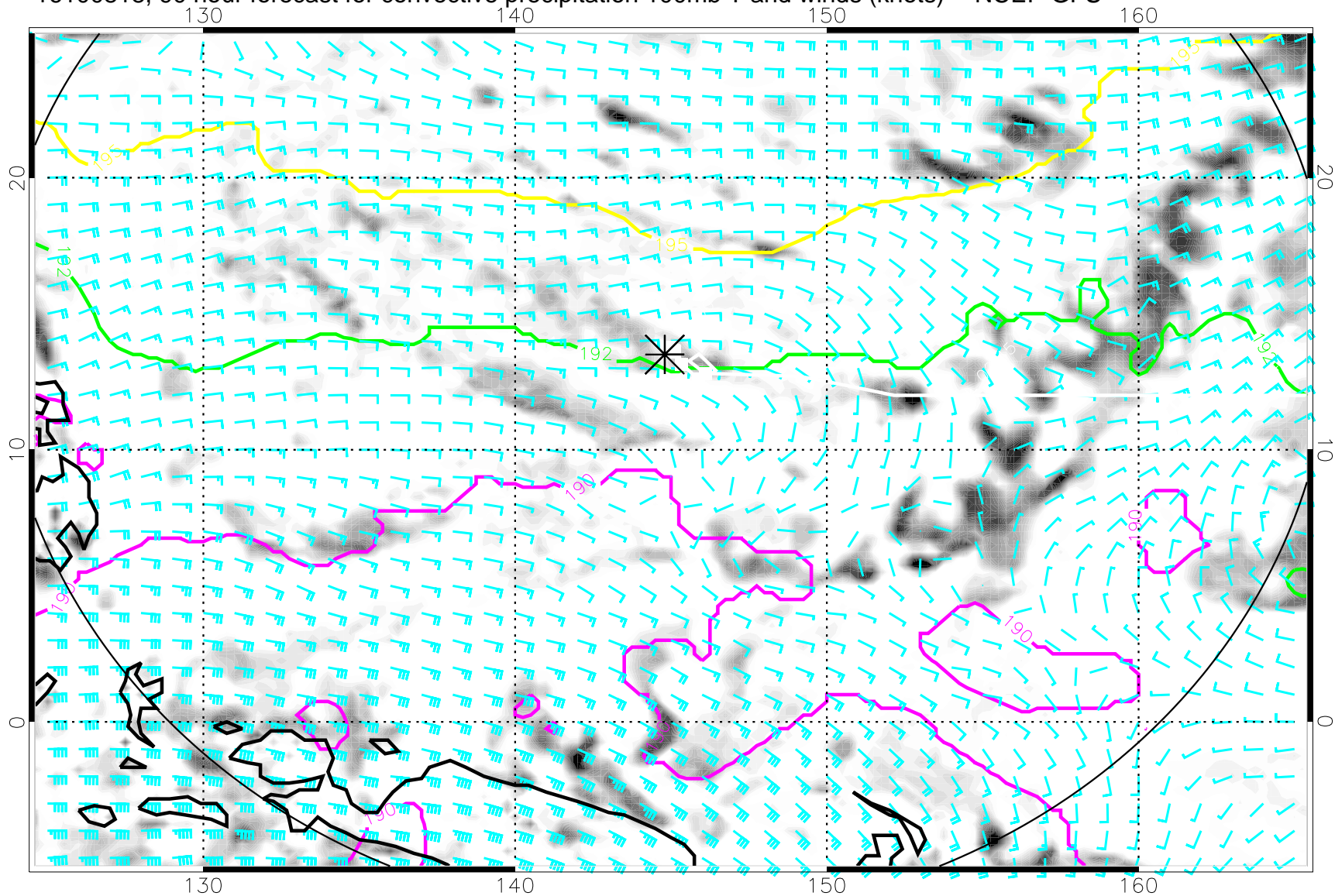
16100818, 90 hour forecast for convective precipitation 100mb T and winds (knots) -- NCEP GFS
