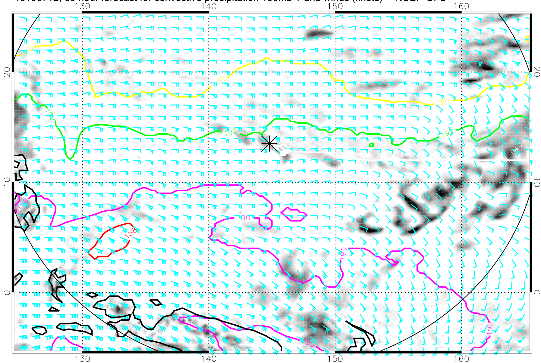
16100712, 60 hour forecast for convective precipitation 100mb T and winds (knots) -- NCEP GFS
