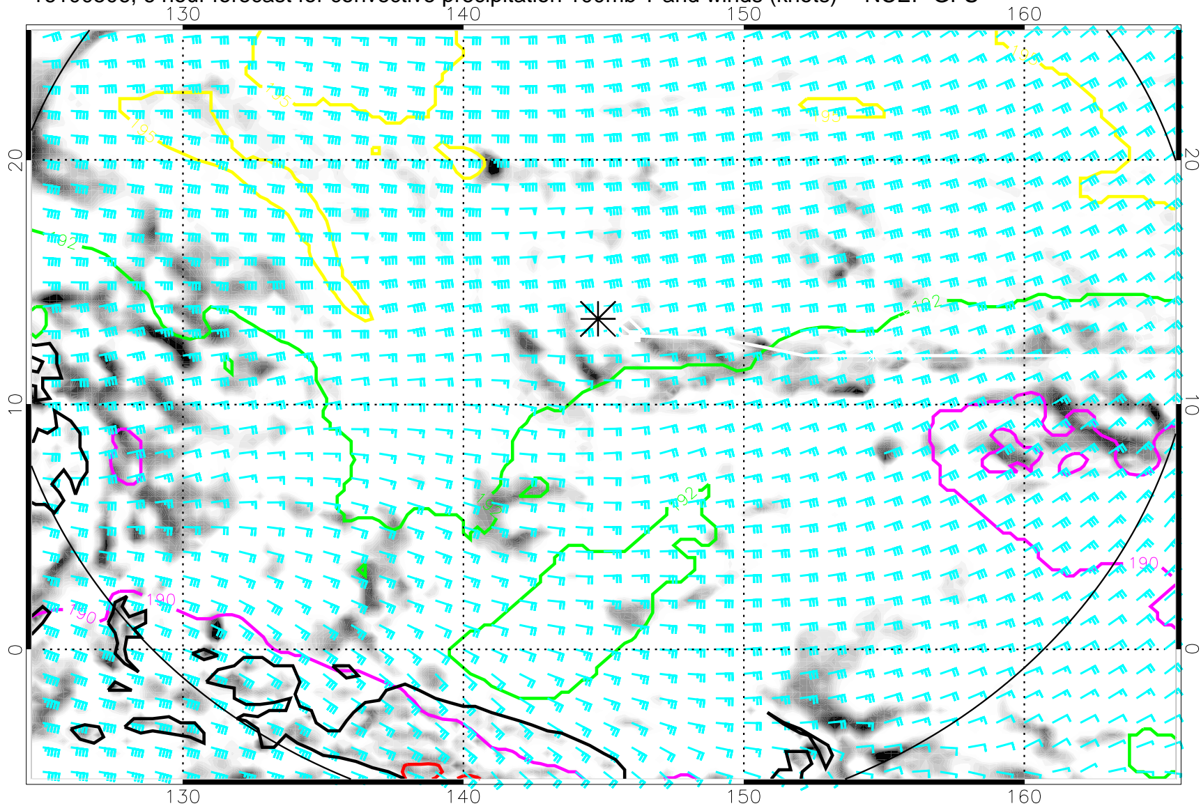
16100506, 6 hour forecast for convective precipitation 100mb T and winds (knots) -- NCEP GFS
