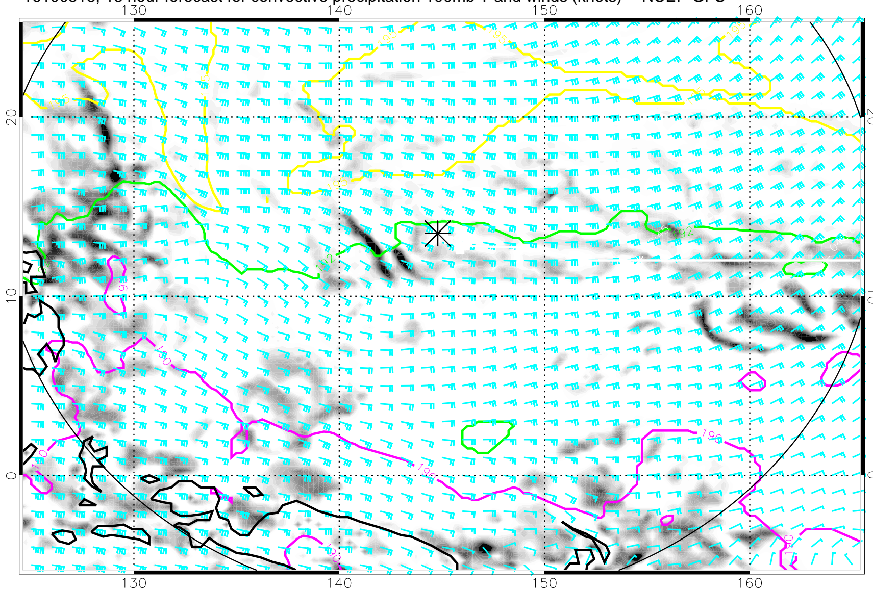
16100518, 18 hour forecast for convective precipitation 100mb T and winds (knots) -- NCEP GFS
