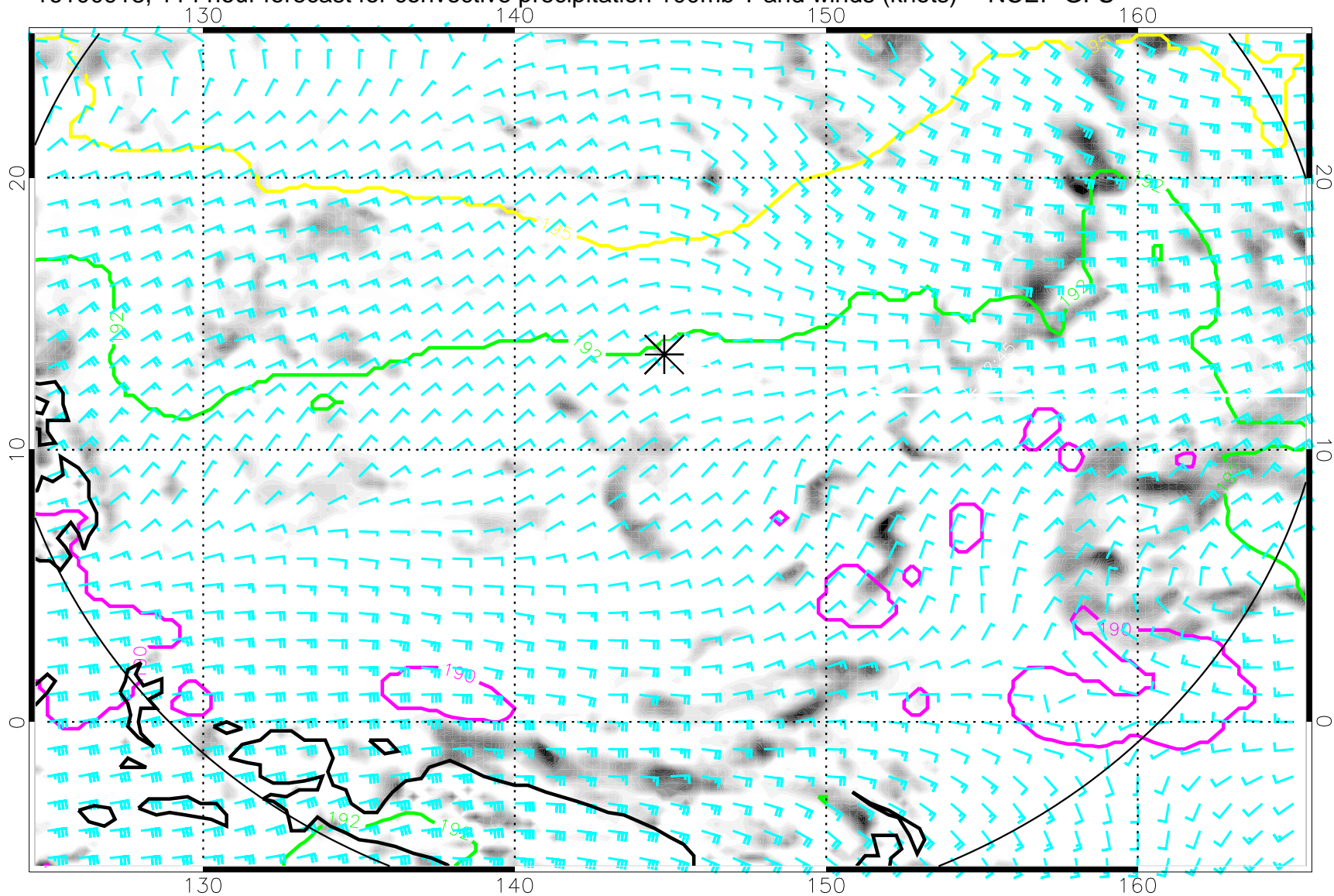
16100918, 114 hour forecast for convective precipitation 100mb T and winds (knots) -- NCEP GFS
