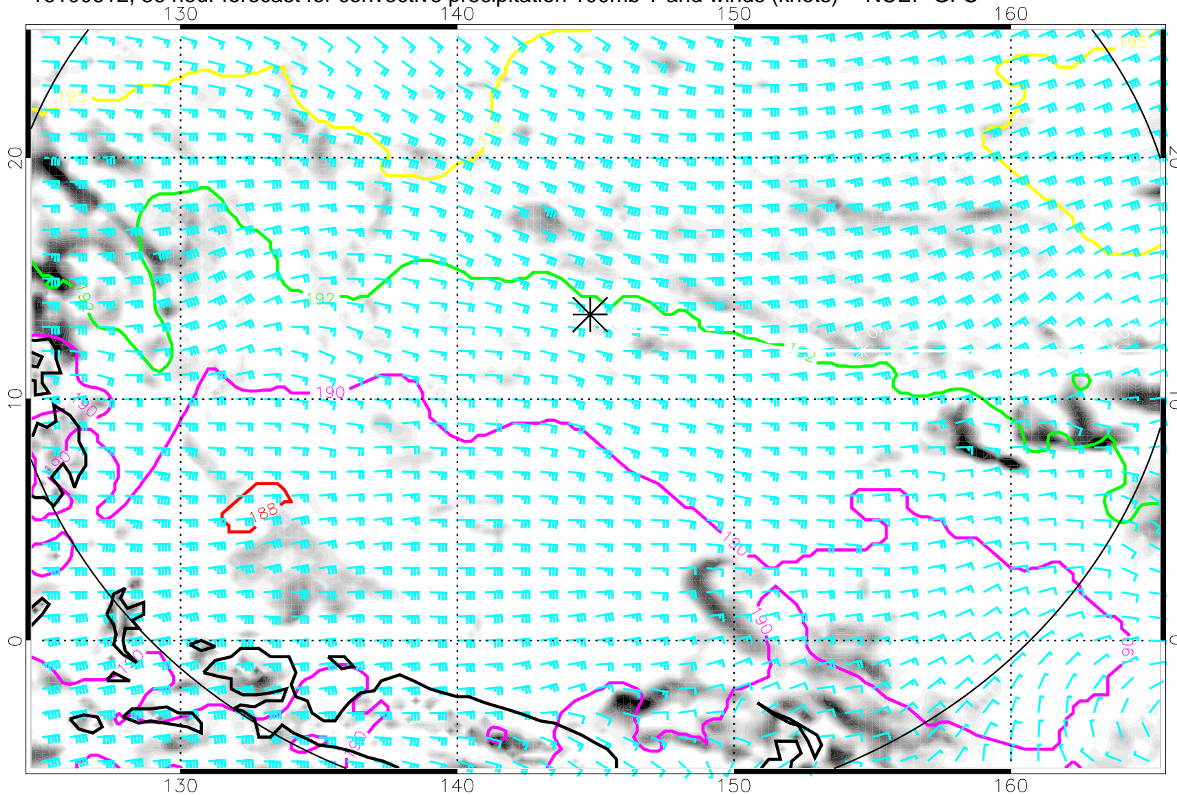
16100612, 36 hour forecast for convective precipitation 100mb T and winds (knots) -- NCEP GFS
