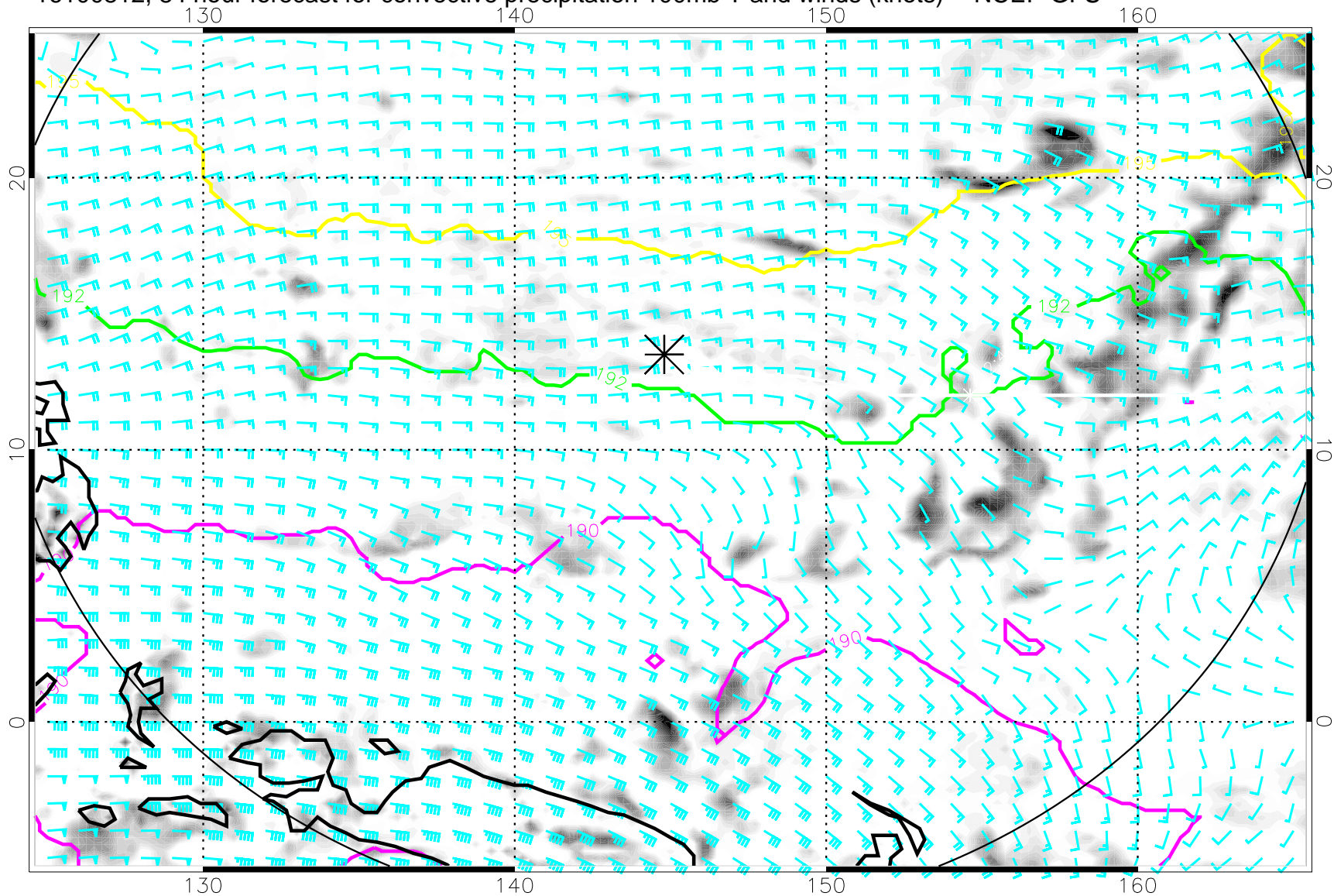
16100812, 84 hour forecast for convective precipitation 100mb T and winds (knots) -- NCEP GFS
