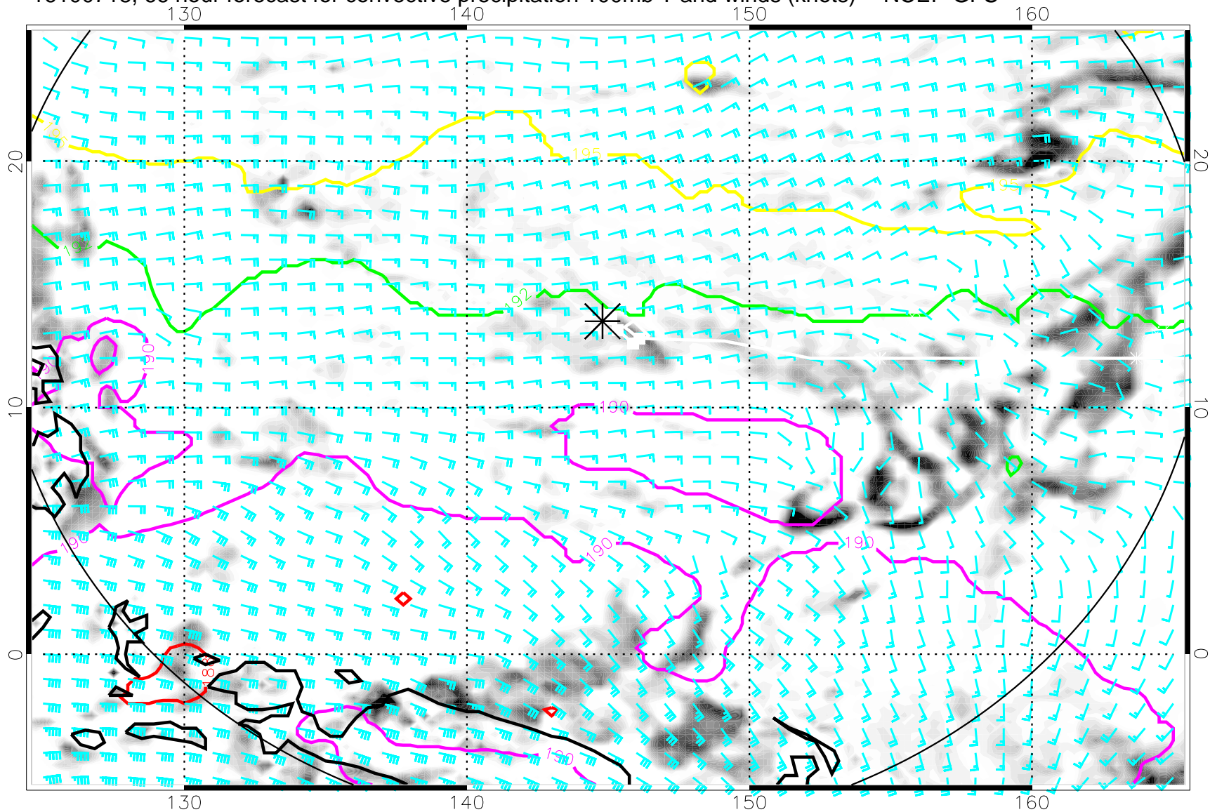
16100718, 66 hour forecast for convective precipitation 100mb T and winds (knots) -- NCEP GFS
