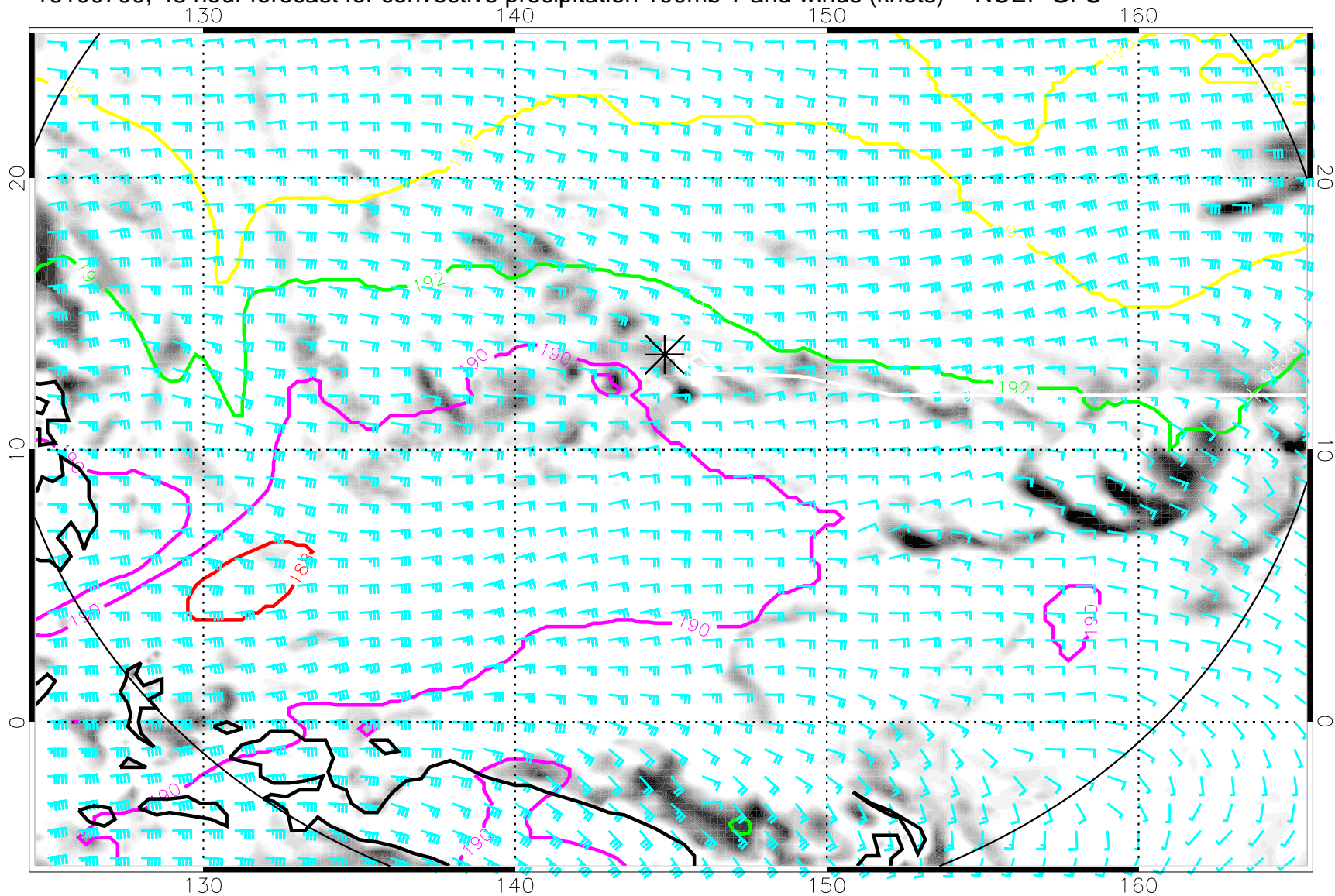
16100700, 48 hour forecast for convective precipitation 100mb T and winds (knots) -- NCEP GFS
