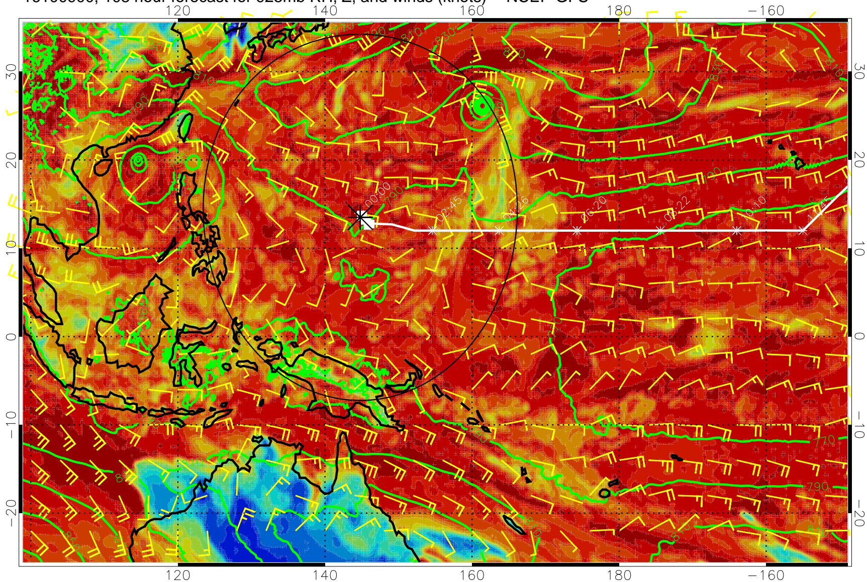
16100900, 108 hour forecast for 925mb RH, Z, and winds (knots) -- NCEP GFS
