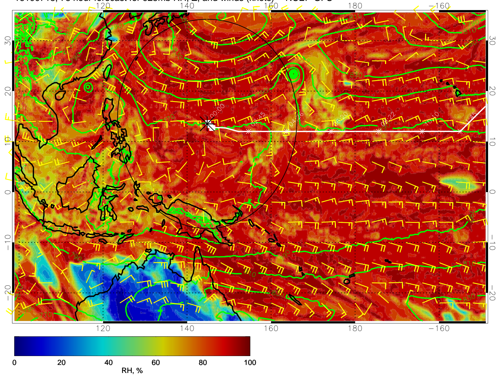
16100718, 78 hour forecast for 925mb RH, Z, and winds (knots) -- NCEP GFS
