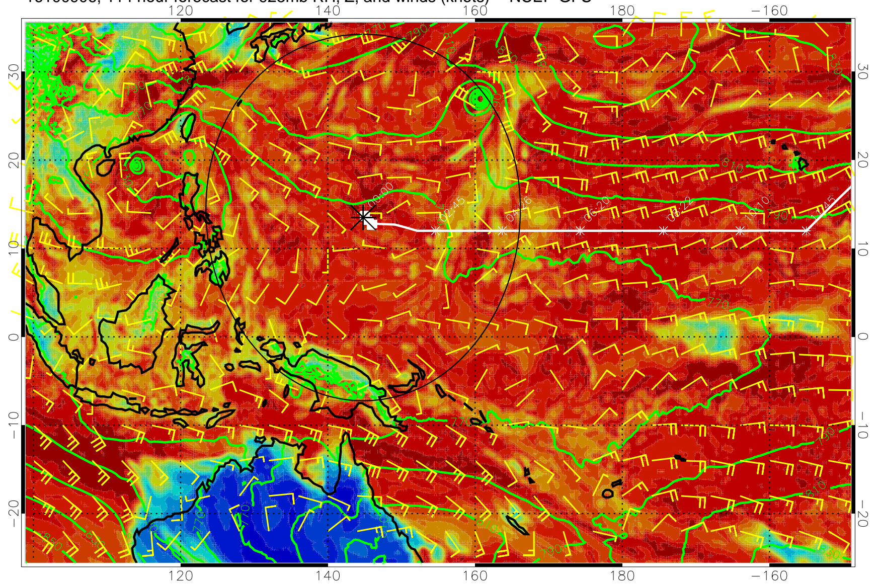
16100906, 114 hour forecast for 925mb RH, Z, and winds (knots) -- NCEP GFS
