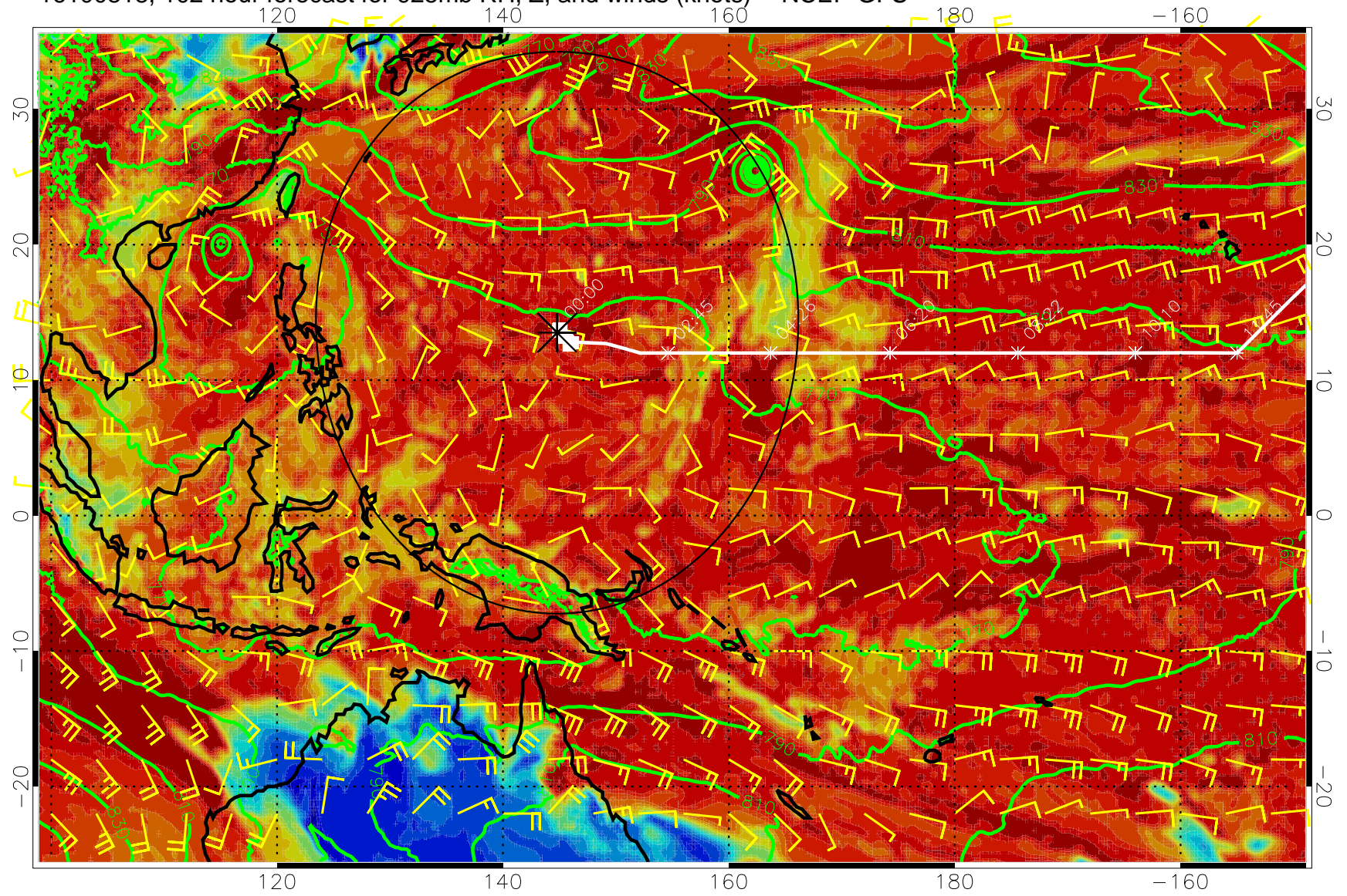
16100818, 102 hour forecast for 925mb RH, Z, and winds (knots) -- NCEP GFS
