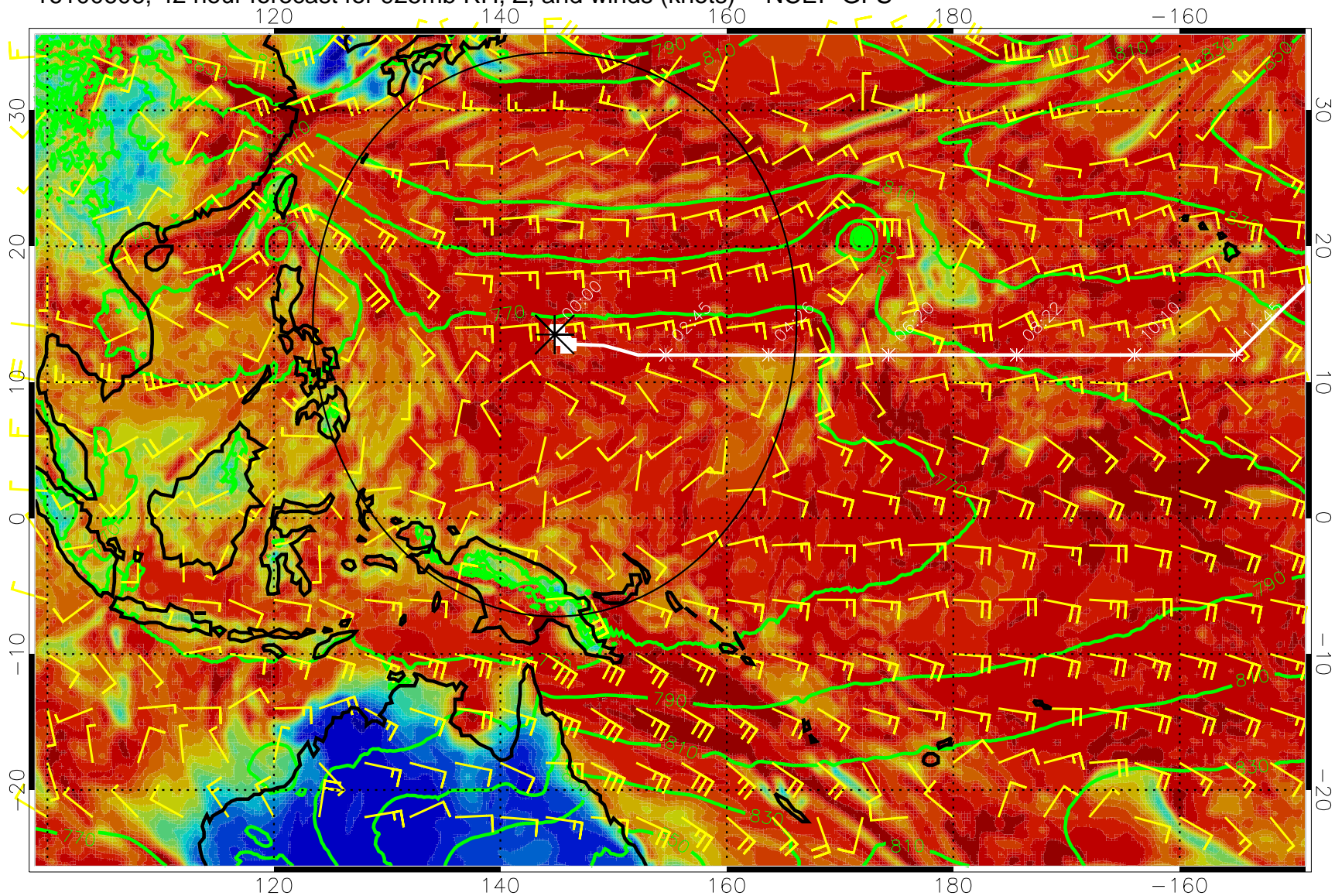
16100606, 42 hour forecast for 925mb RH, Z, and winds (knots) -- NCEP GFS
