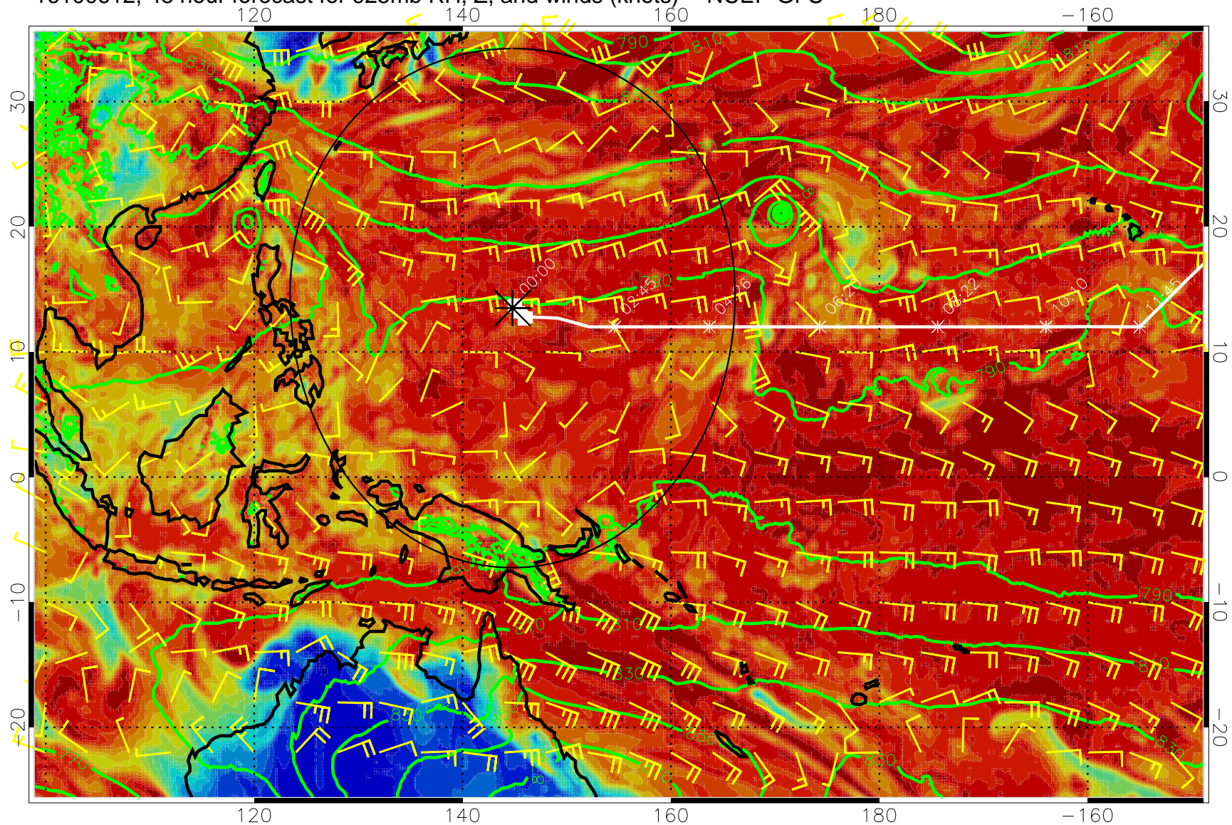
16100612, 48 hour forecast for 925mb RH, Z, and winds (knots) -- NCEP GFS
