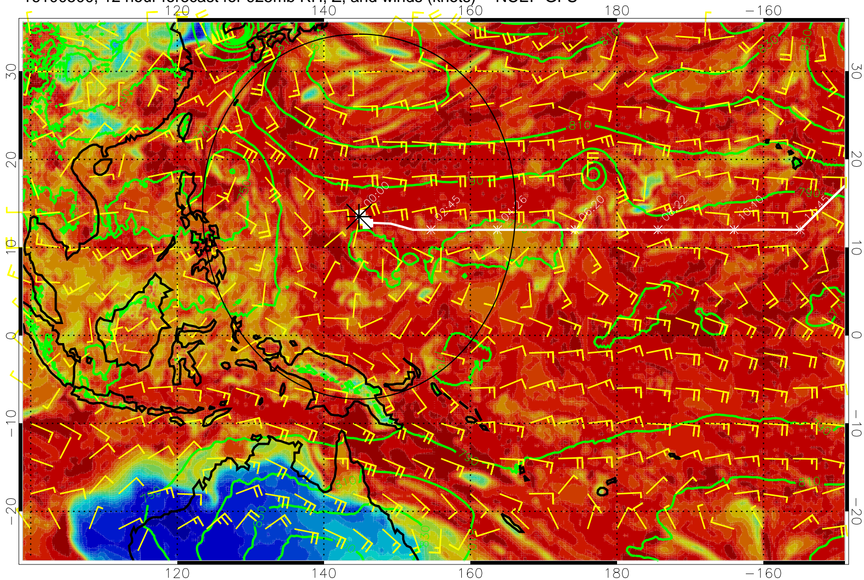
16100500, 12 hour forecast for 925mb RH, Z, and winds (knots) -- NCEP GFS
