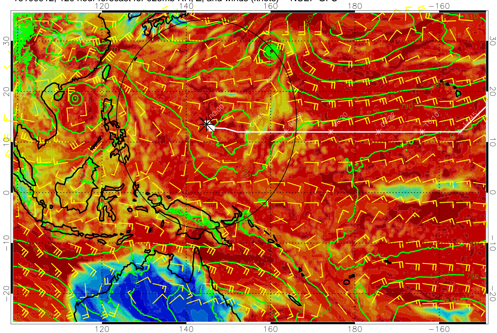
16100912, 120 hour forecast for 925mb RH, Z, and winds (knots) -- NCEP GFS
