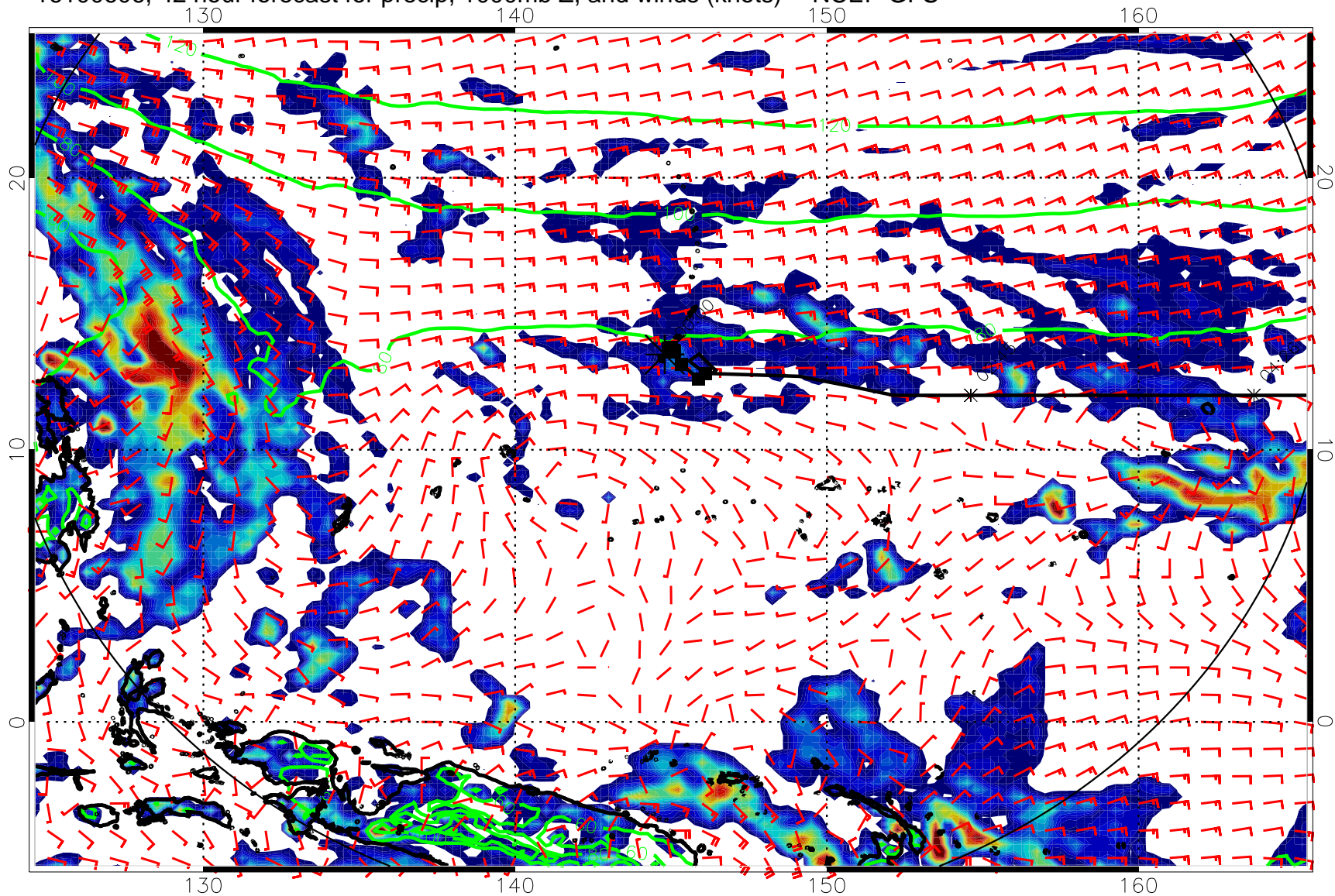
16100606, 42 hour forecast for precip, 1000mb Z, and winds (knots) -- NCEP GFS
