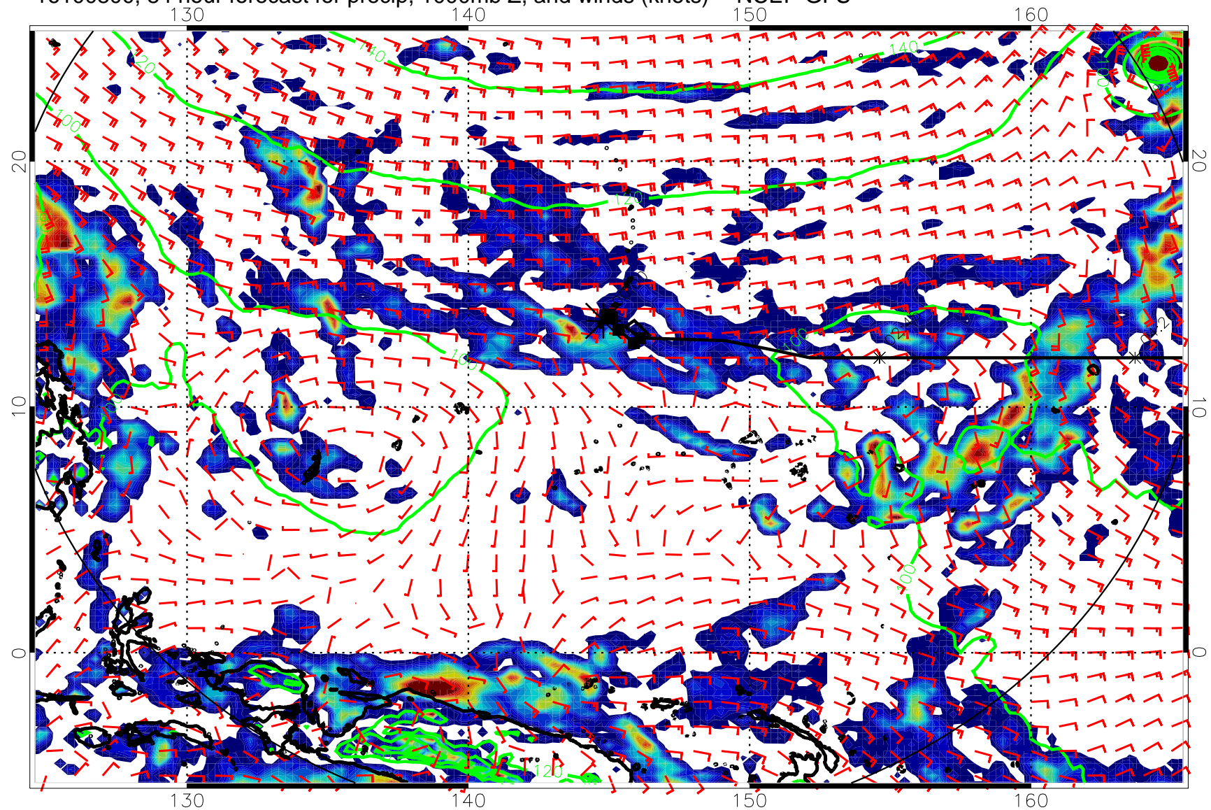
16100800, 84 hour forecast for precip, 1000mb Z, and winds (knots) -- NCEP GFS
