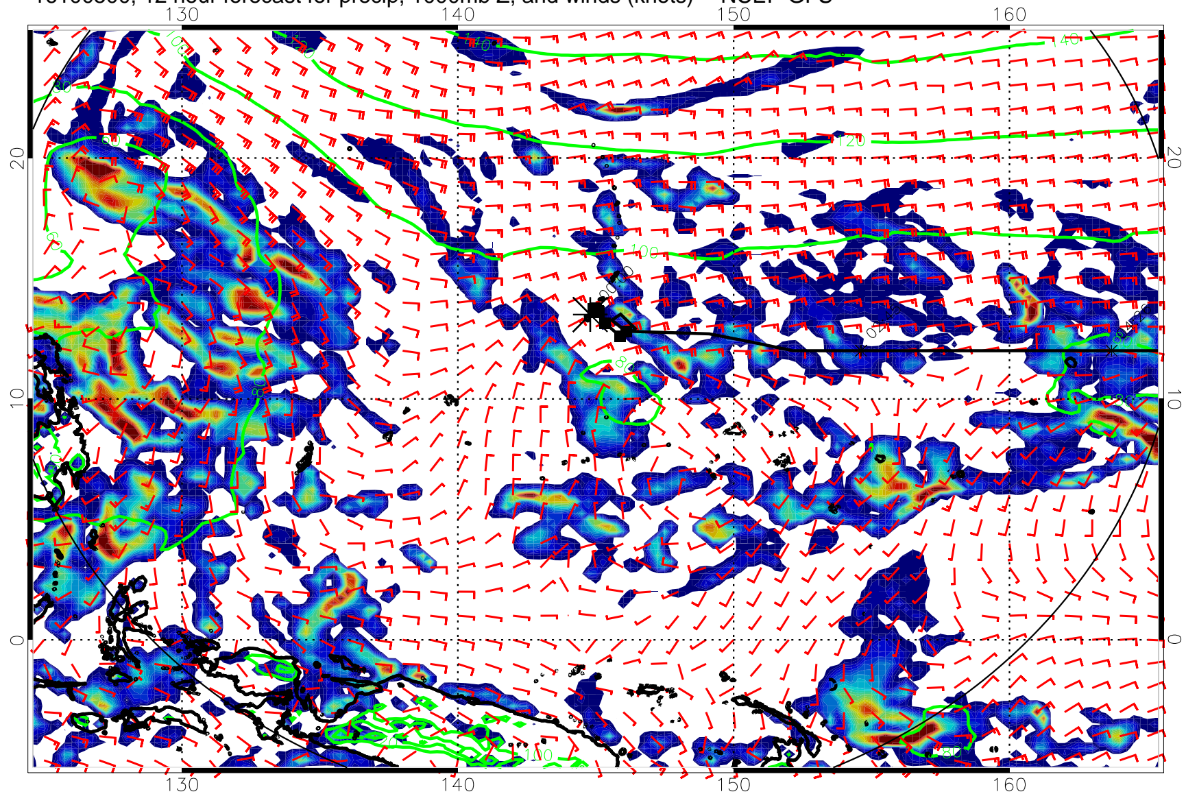
16100500, 12 hour forecast for precip, 1000mb Z, and winds (knots) -- NCEP GFS
