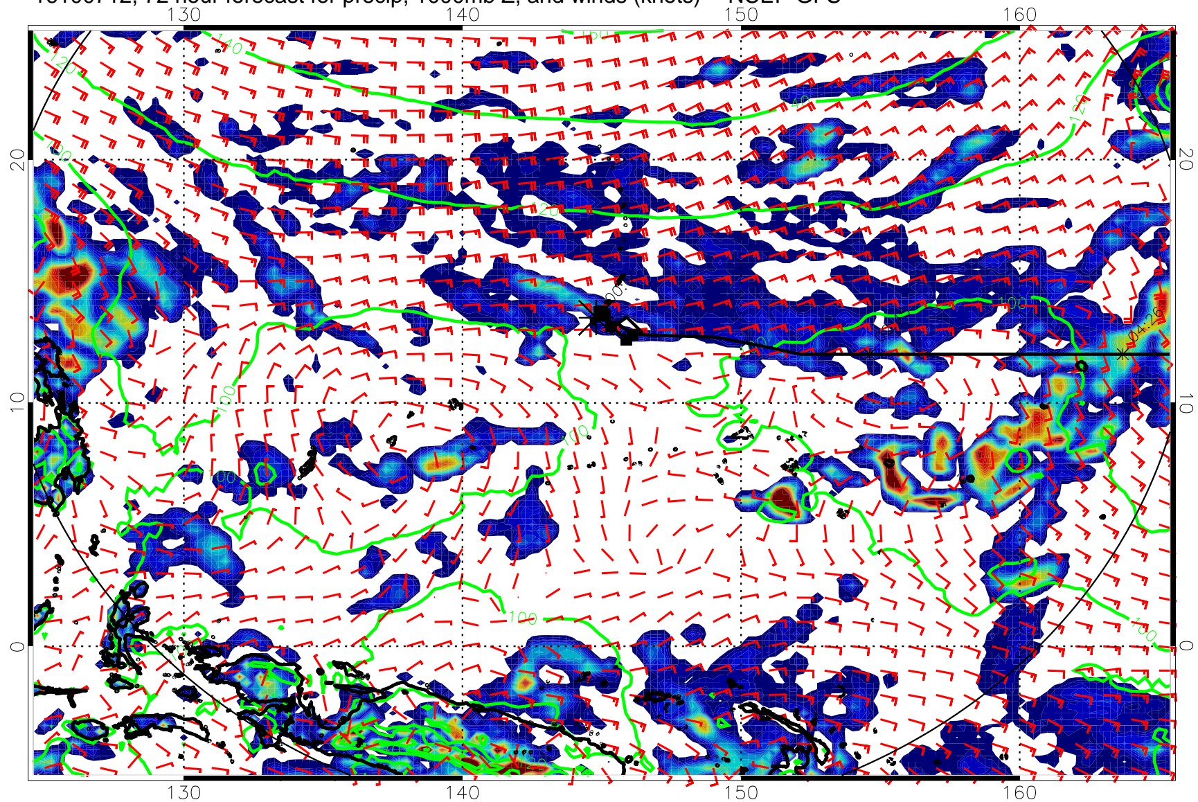
16100712, 72 hour forecast for precip, 1000mb Z, and winds (knots) -- NCEP GFS
