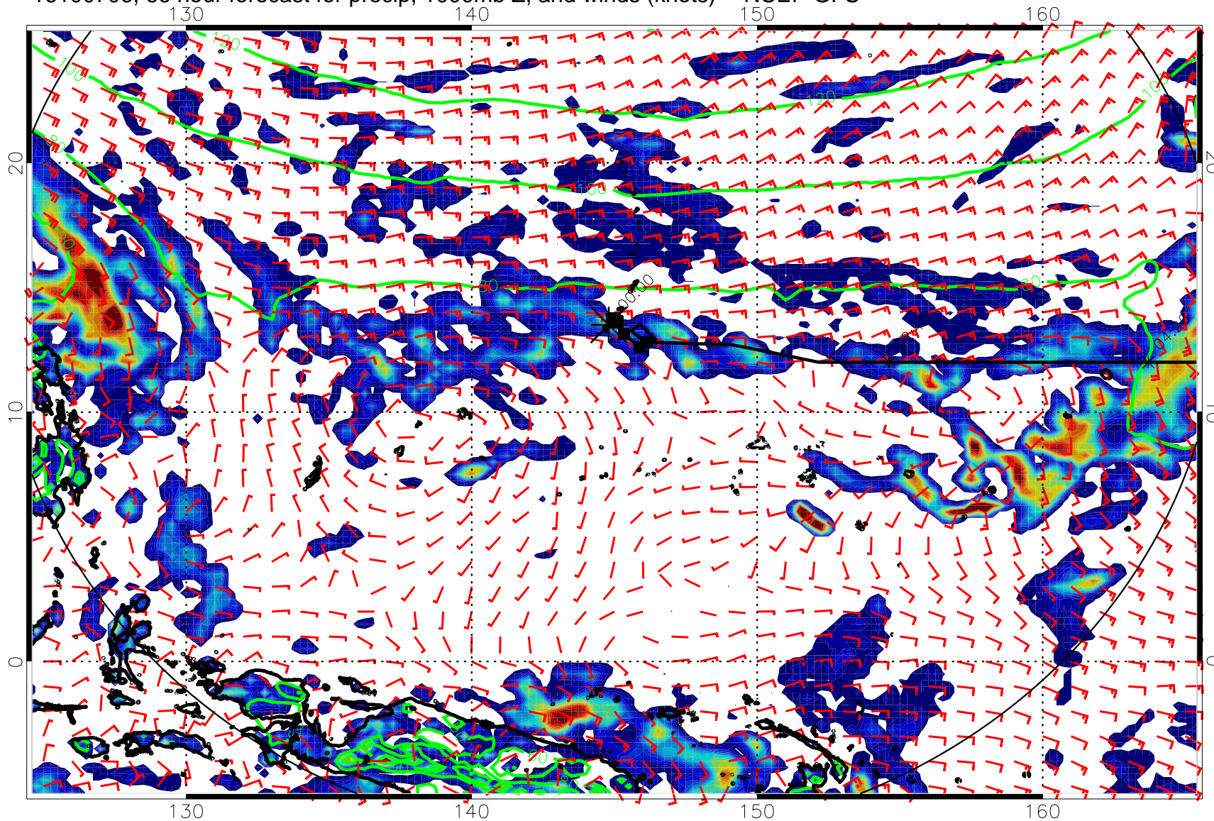
16100706, 66 hour forecast for precip, 1000mb Z, and winds (knots) -- NCEP GFS
