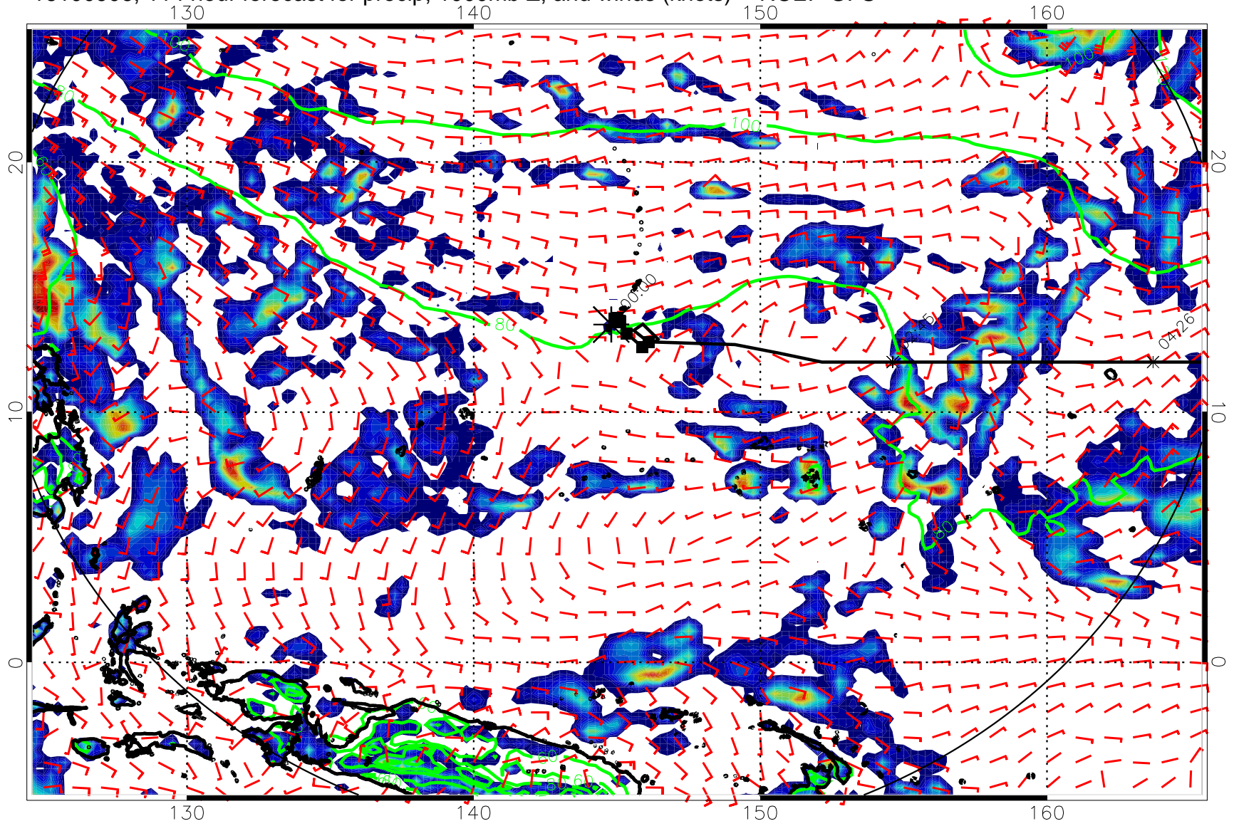
16100906, 114 hour forecast for precip, 1000mb Z, and winds (knots) -- NCEP GFS
