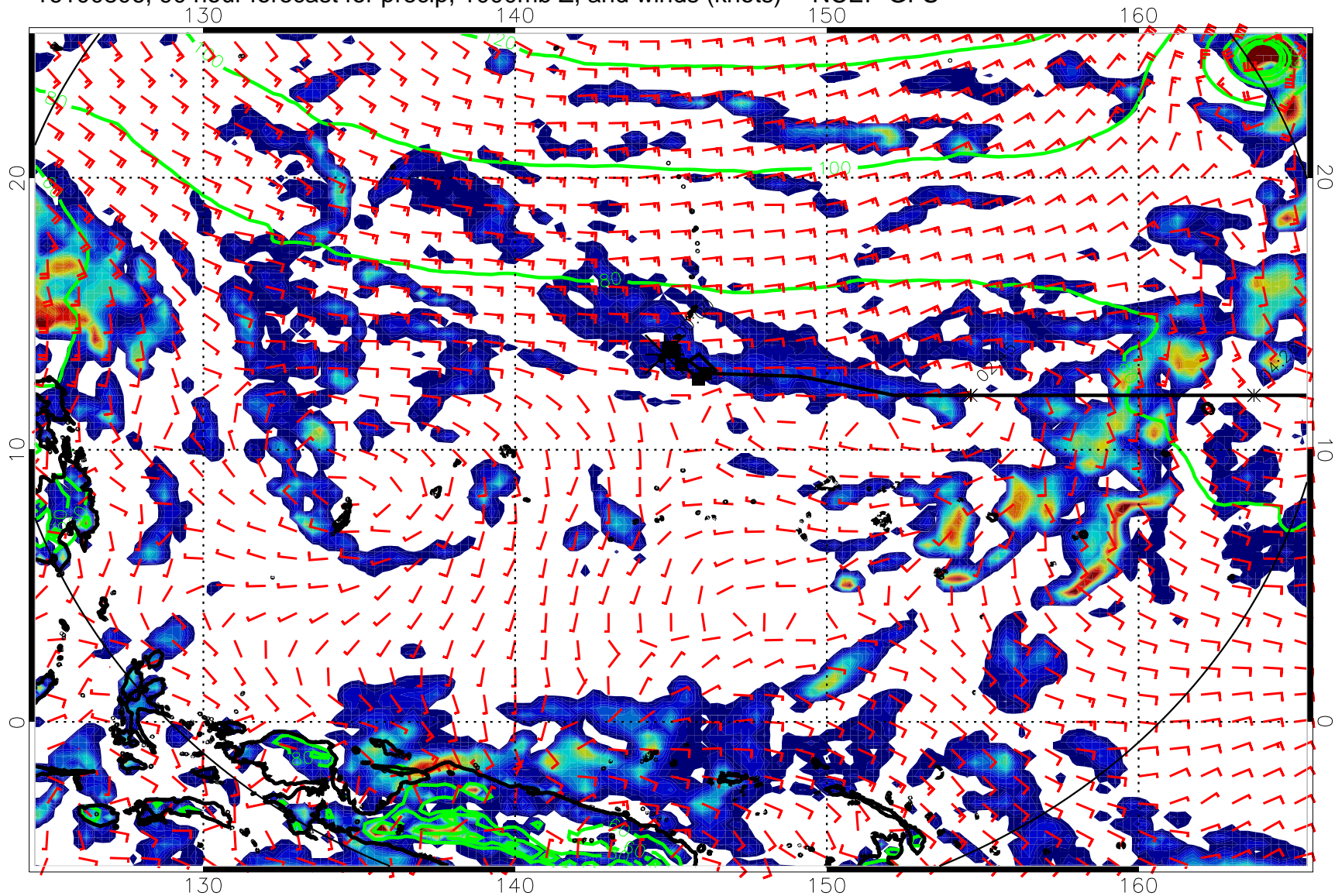
16100806, 90 hour forecast for precip, 1000mb Z, and winds (knots) -- NCEP GFS
