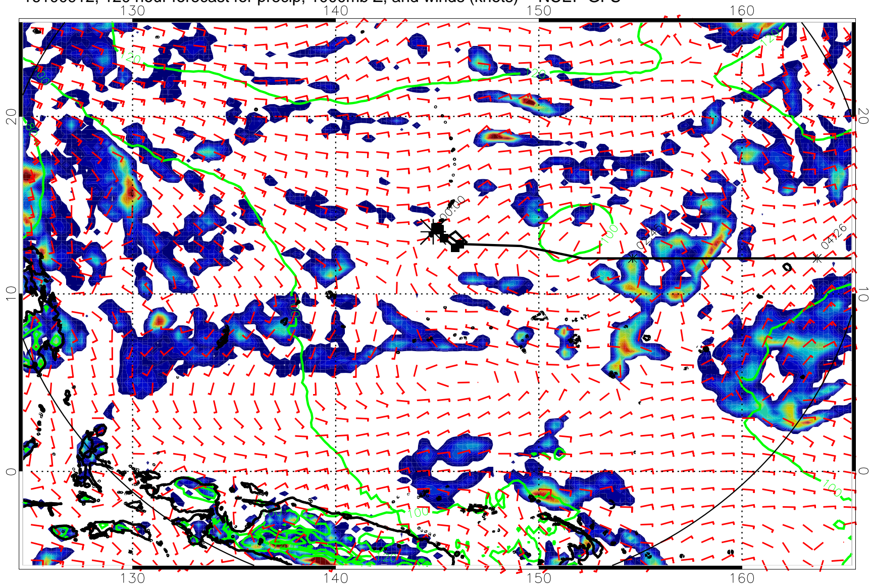
16100912, 120 hour forecast for precip, 1000mb Z, and winds (knots) -- NCEP GFS
