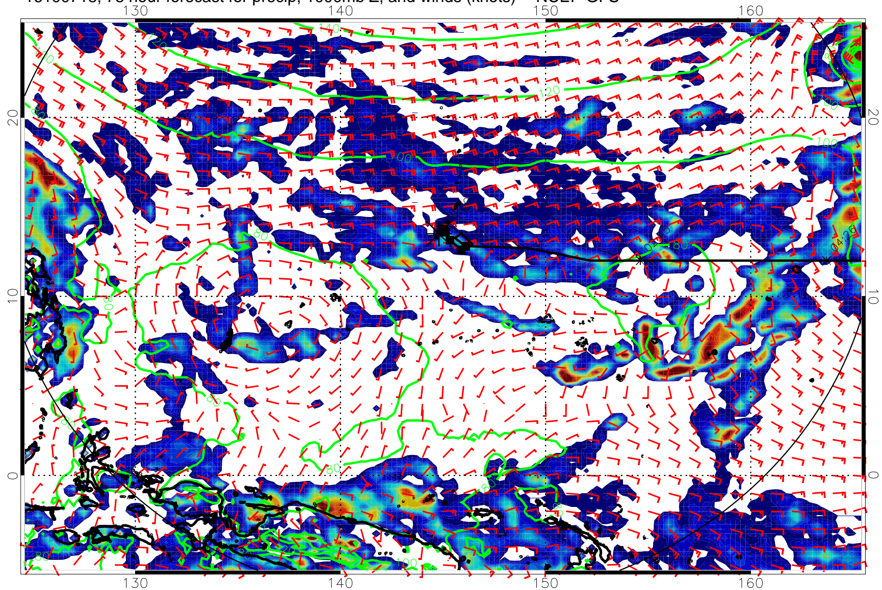
16100718, 78 hour forecast for precip, 1000mb Z, and winds (knots) -- NCEP GFS
