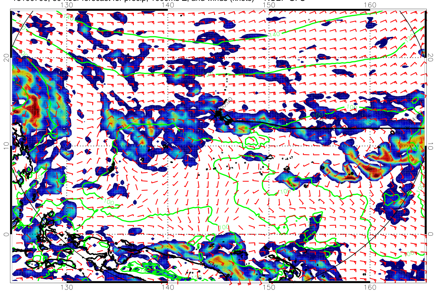
16100700, 60 hour forecast for precip, 1000mb Z, and winds (knots) -- NCEP GFS
