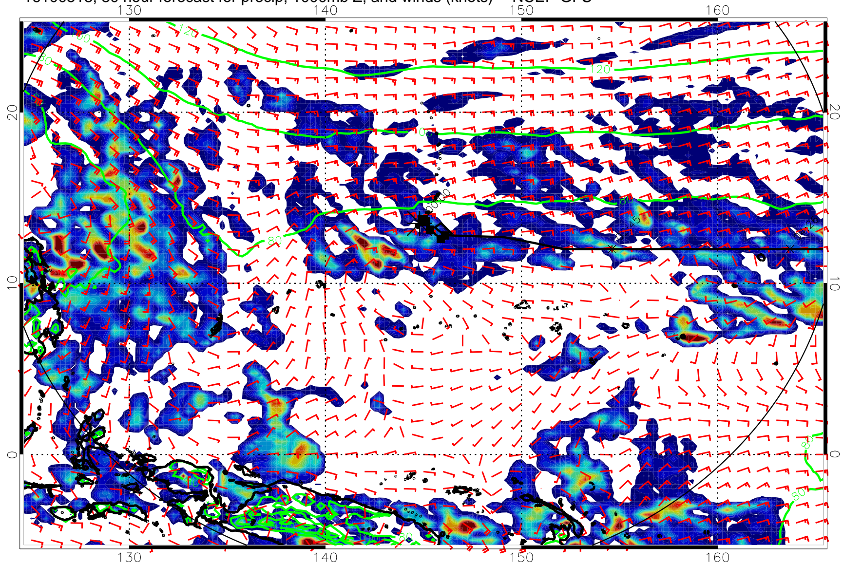
16100518, 30 hour forecast for precip, 1000mb Z, and winds (knots) -- NCEP GFS
