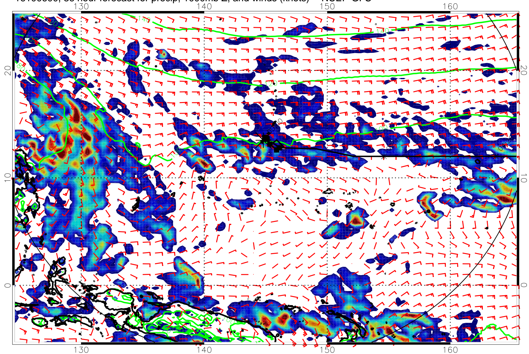
16100600, 36 hour forecast for precip, 1000mb Z, and winds (knots) -- NCEP GFS
