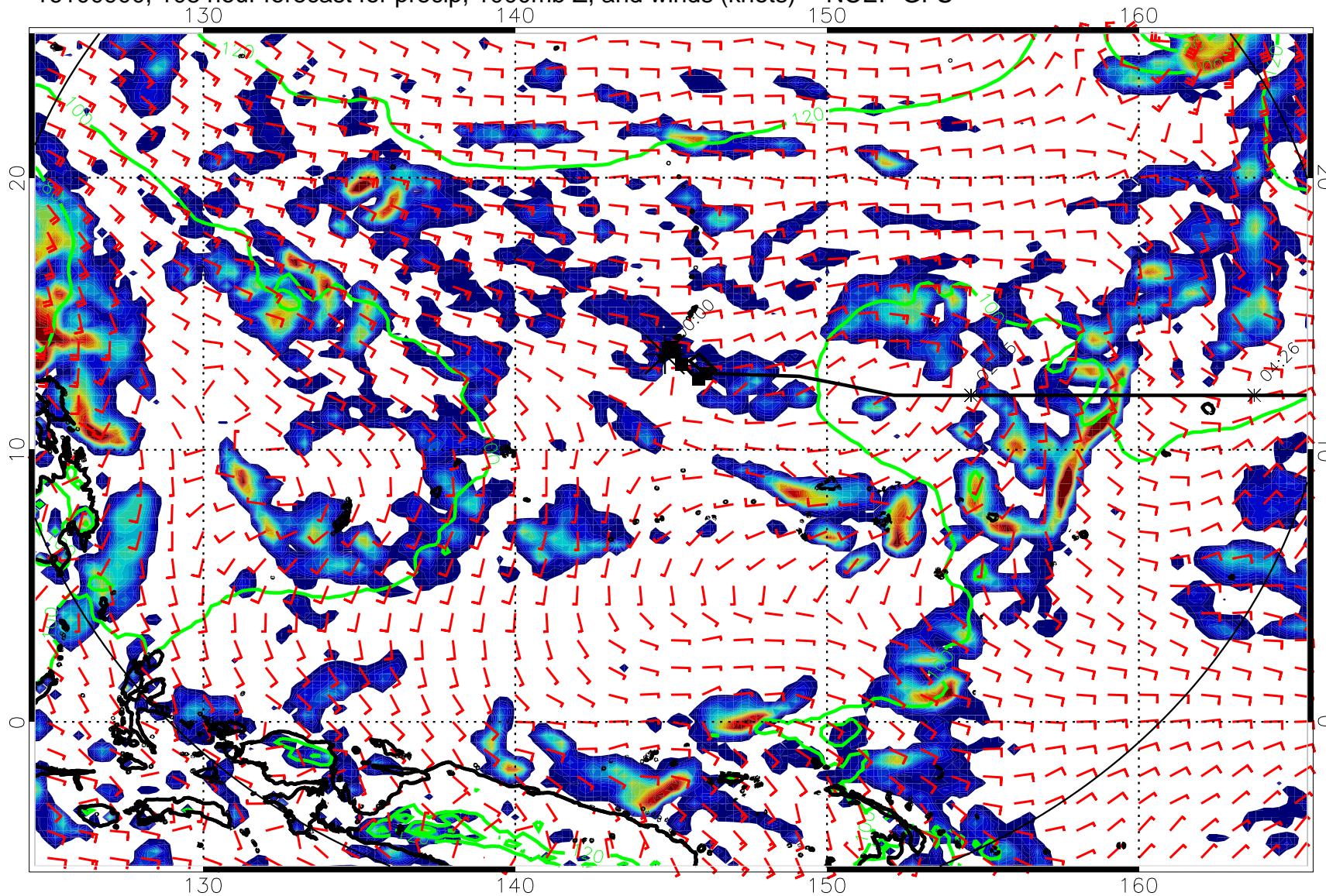
16100900, 108 hour forecast for precip, 1000mb Z, and winds (knots) -- NCEP GFS
