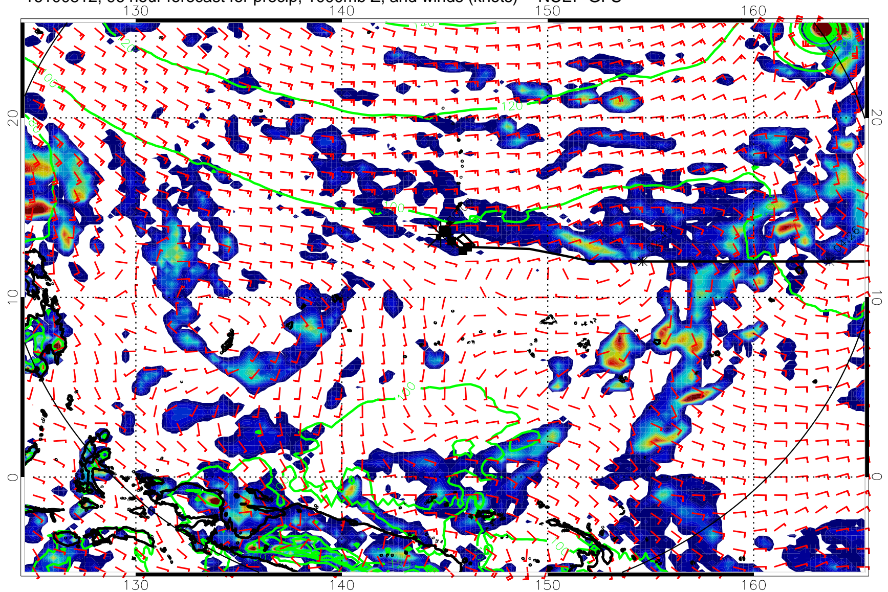
16100812, 96 hour forecast for precip, 1000mb Z, and winds (knots) -- NCEP GFS
