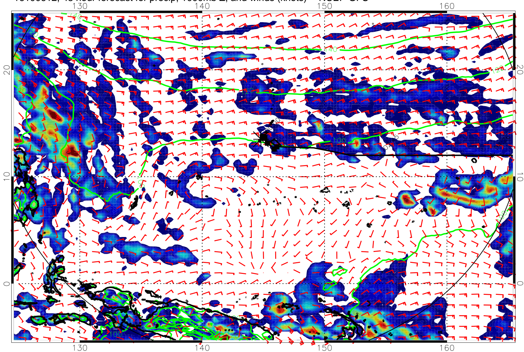
16100612, 48 hour forecast for precip, 1000mb Z, and winds (knots) -- NCEP GFS
