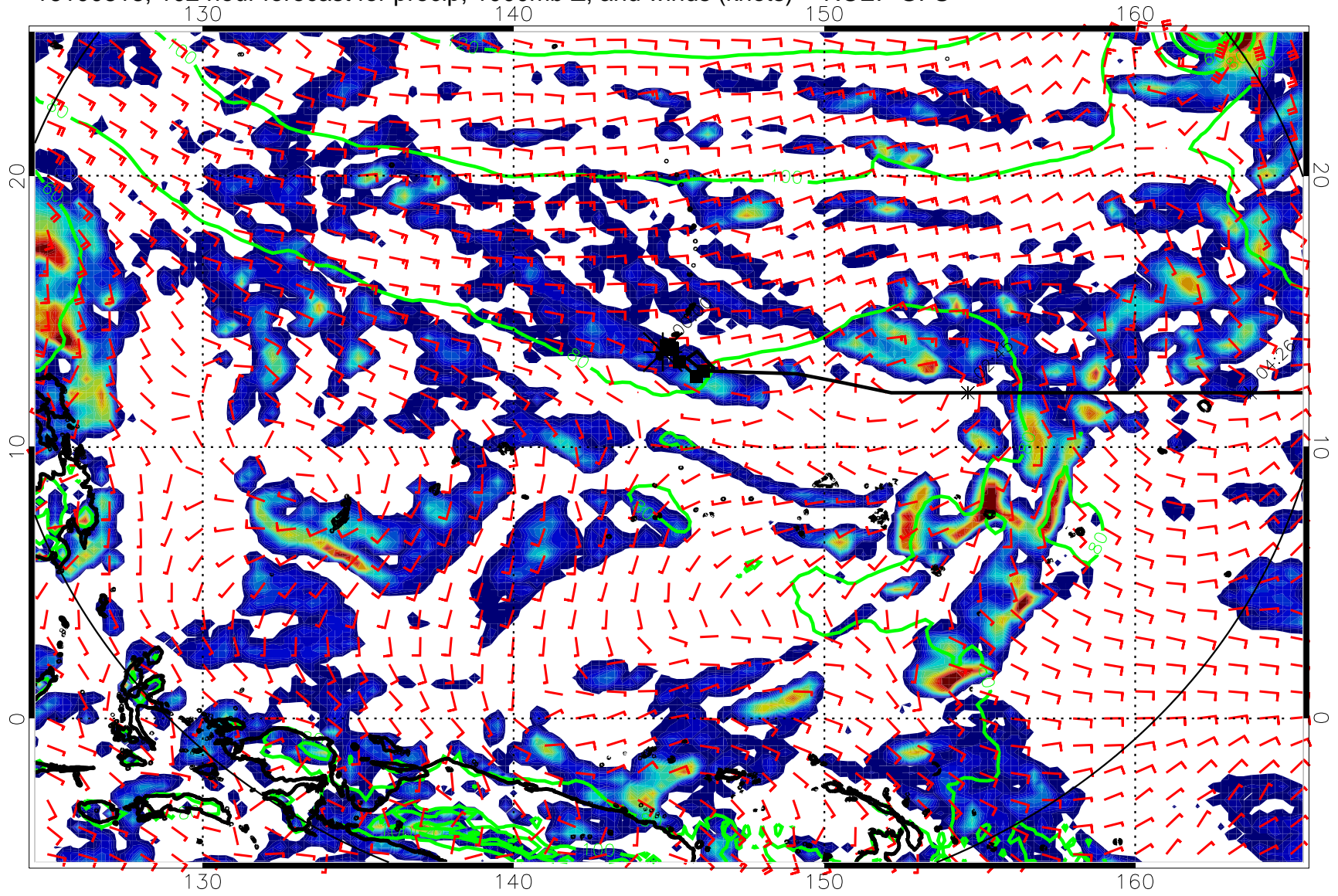
16100818, 102 hour forecast for precip, 1000mb Z, and winds (knots) -- NCEP GFS
