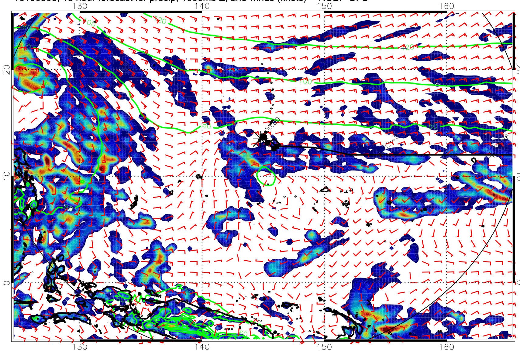
16100506, 18 hour forecast for precip, 1000mb Z, and winds (knots) -- NCEP GFS
