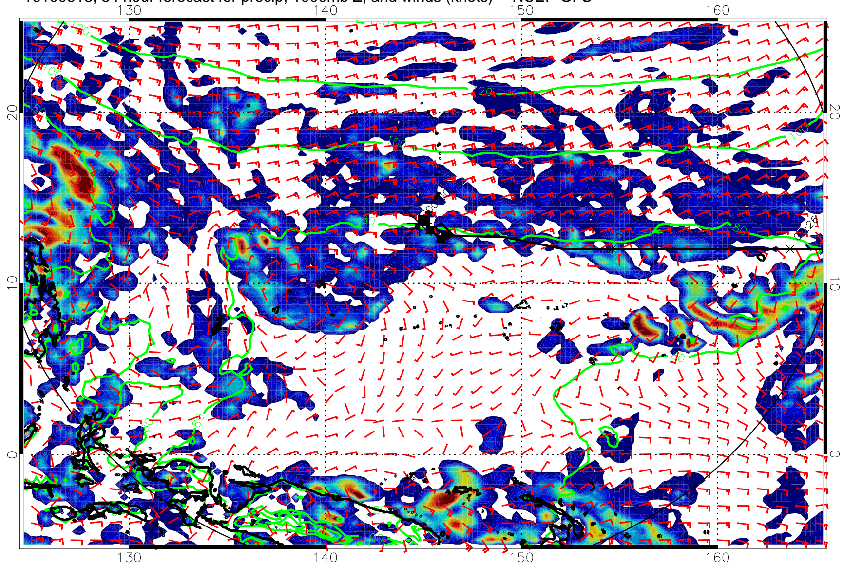
16100618, 54 hour forecast for precip, 1000mb Z, and winds (knots) -- NCEP GFS
