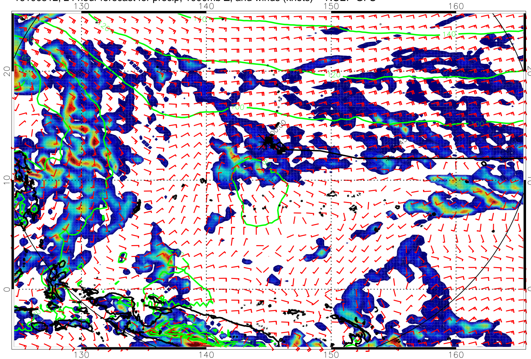
16100512, 24 hour forecast for precip, 1000mb Z, and winds (knots) -- NCEP GFS
