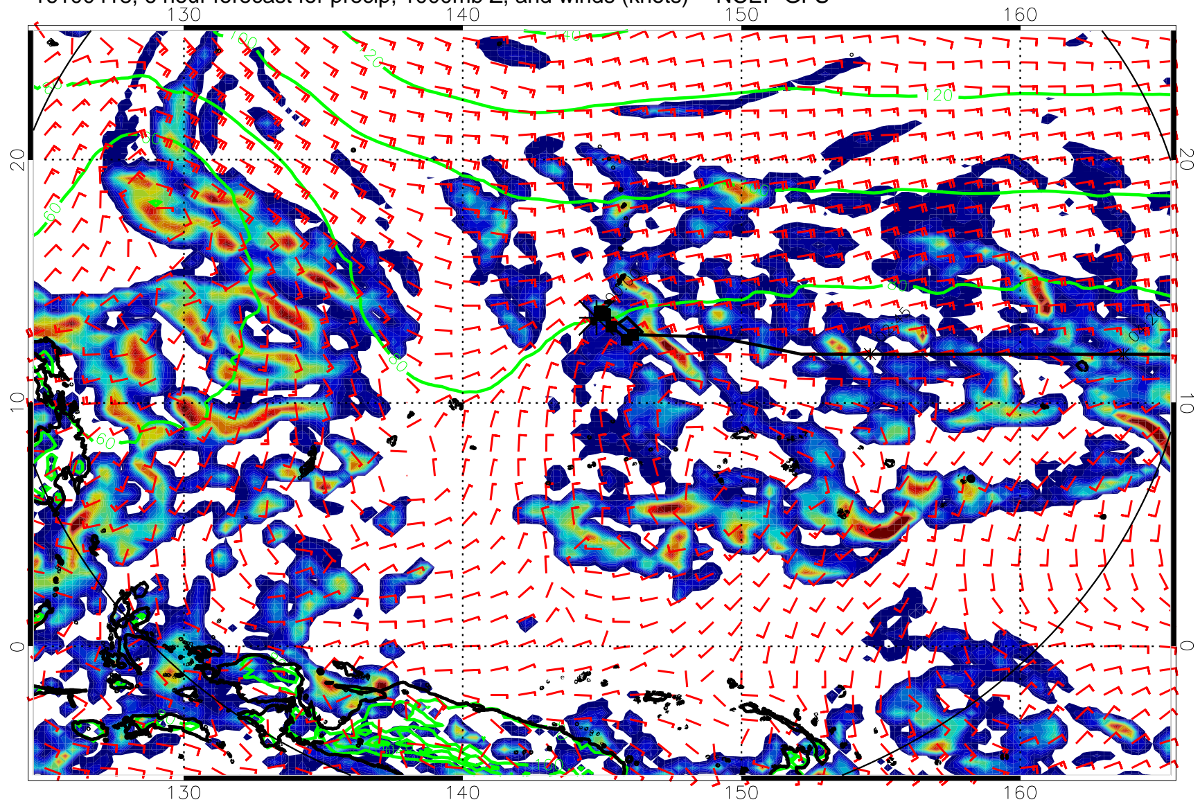
16100418, 6 hour forecast for precip, 1000mb Z, and winds (knots) -- NCEP GFS
