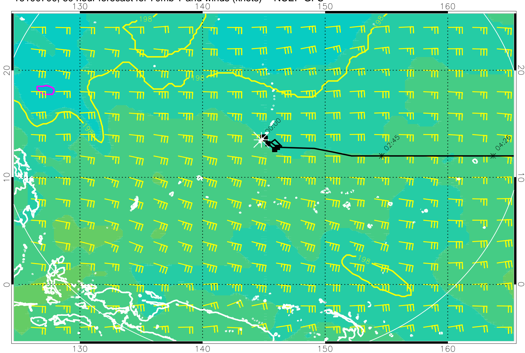
16100700, 60 hour forecast for 70mb T and winds (knots) -- NCEP GFS
