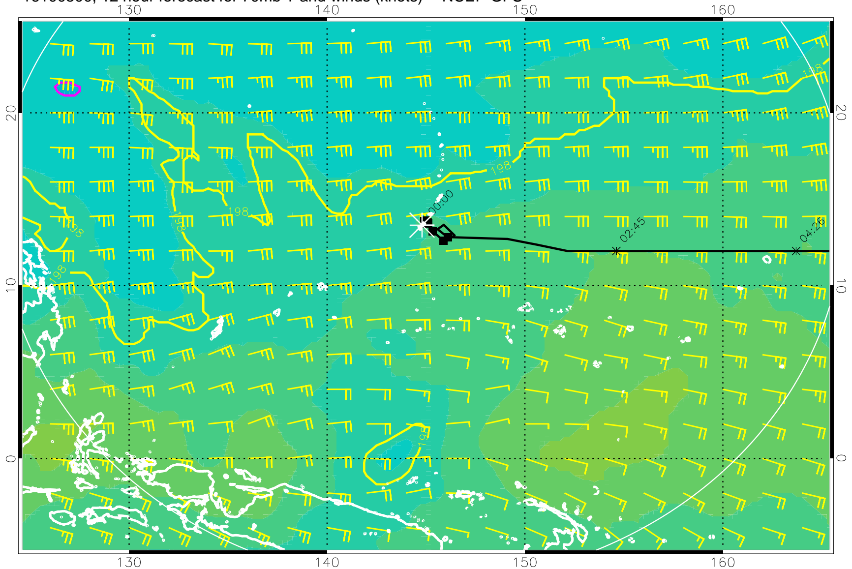
16100500, 12 hour forecast for 70mb T and winds (knots) -- NCEP GFS
