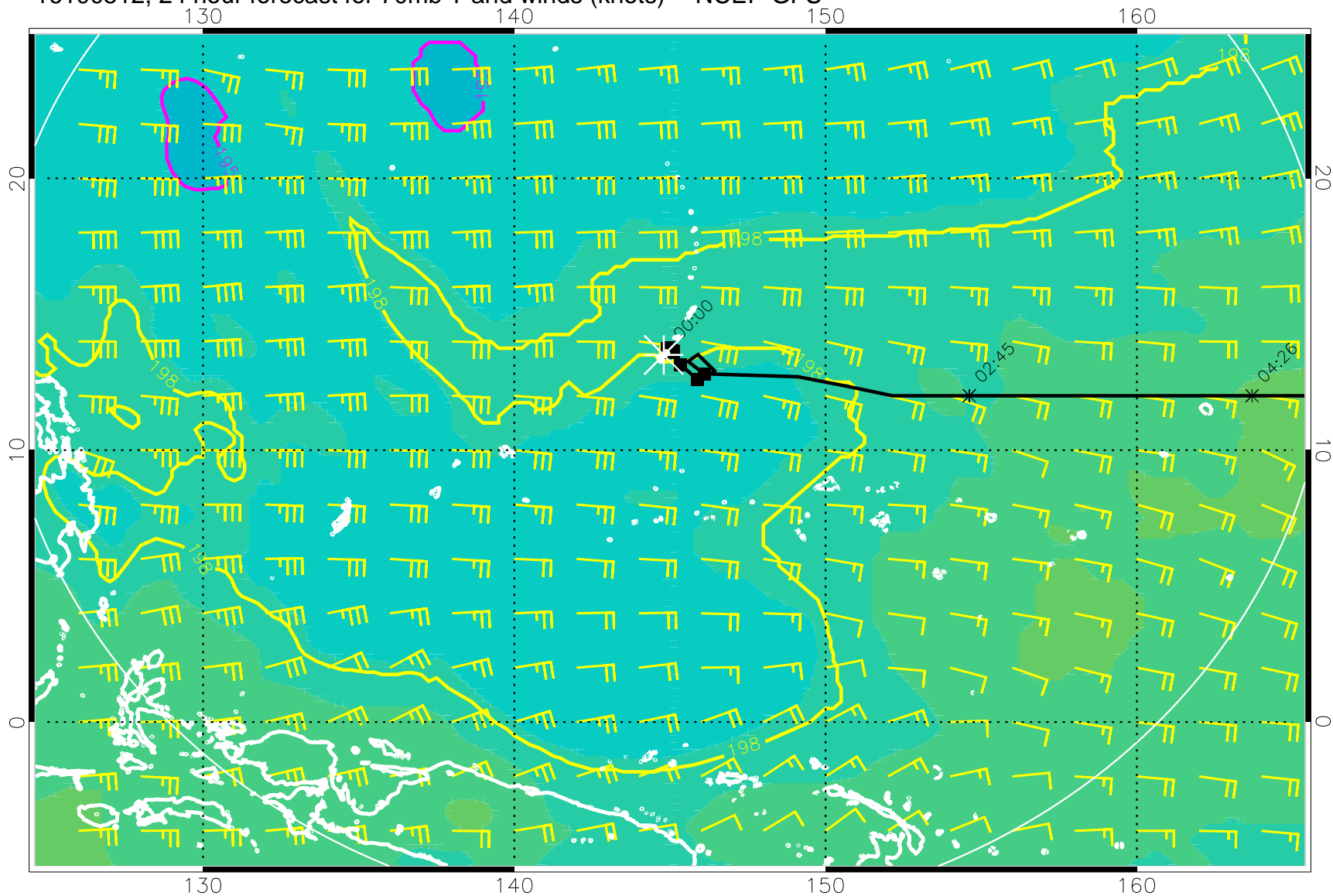
16100512, 24 hour forecast for 70mb T and winds (knots) -- NCEP GFS
