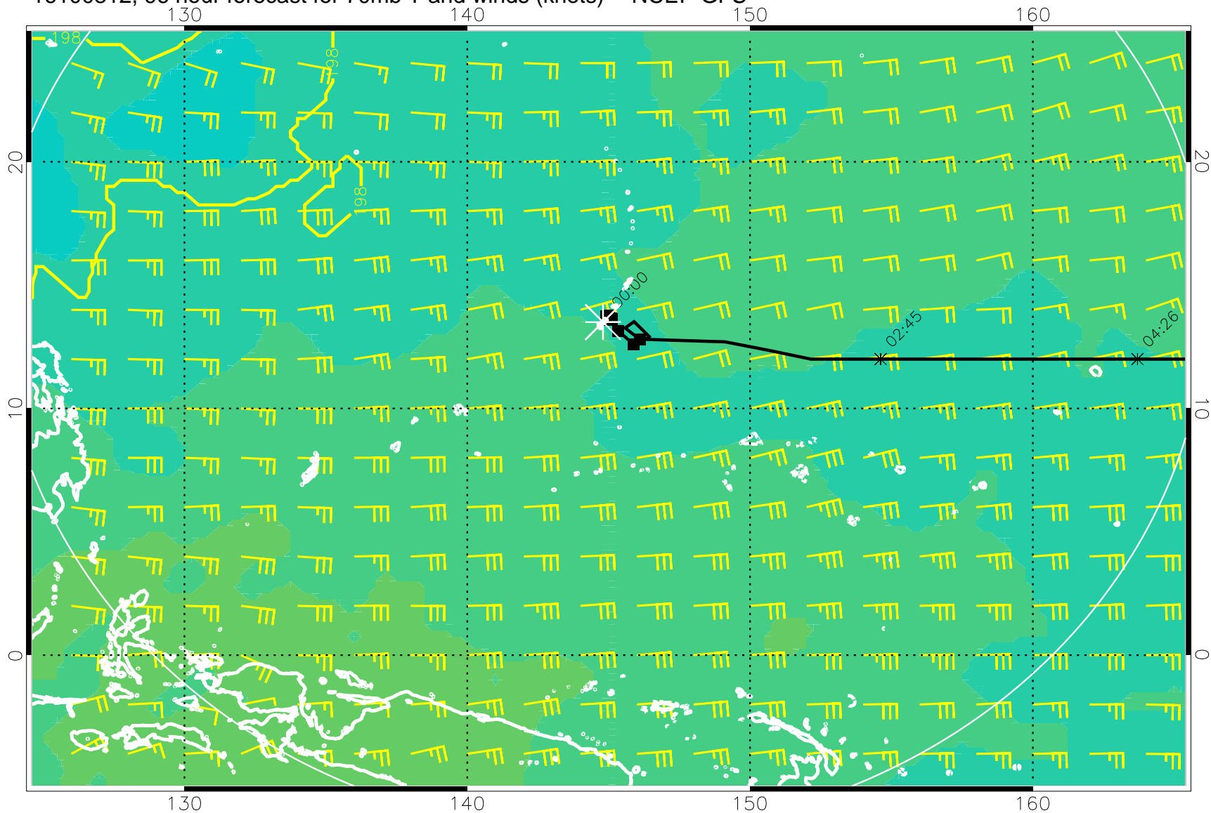
16100812, 96 hour forecast for 70mb T and winds (knots) -- NCEP GFS
