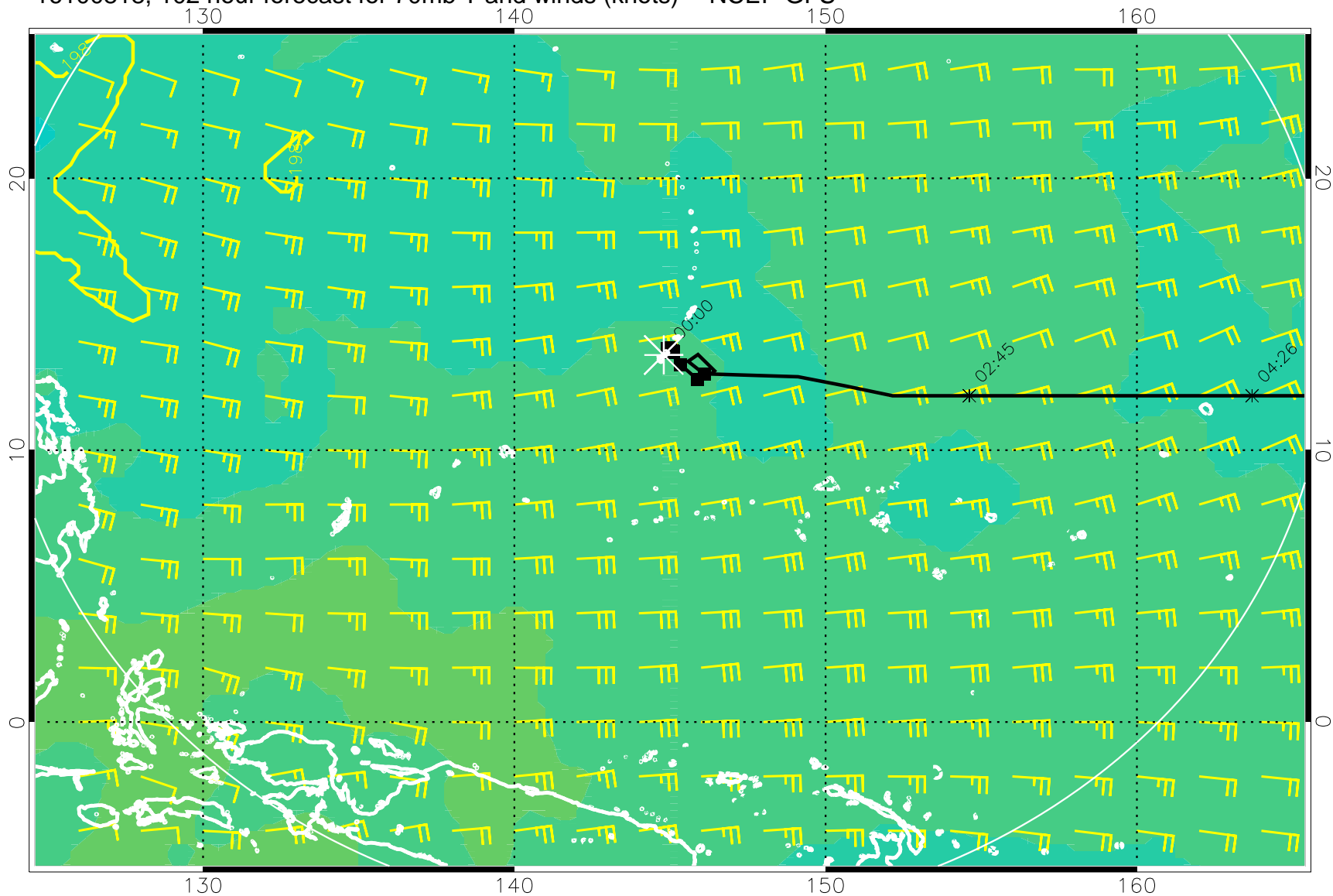
16100818, 102 hour forecast for 70mb T and winds (knots) -- NCEP GFS
