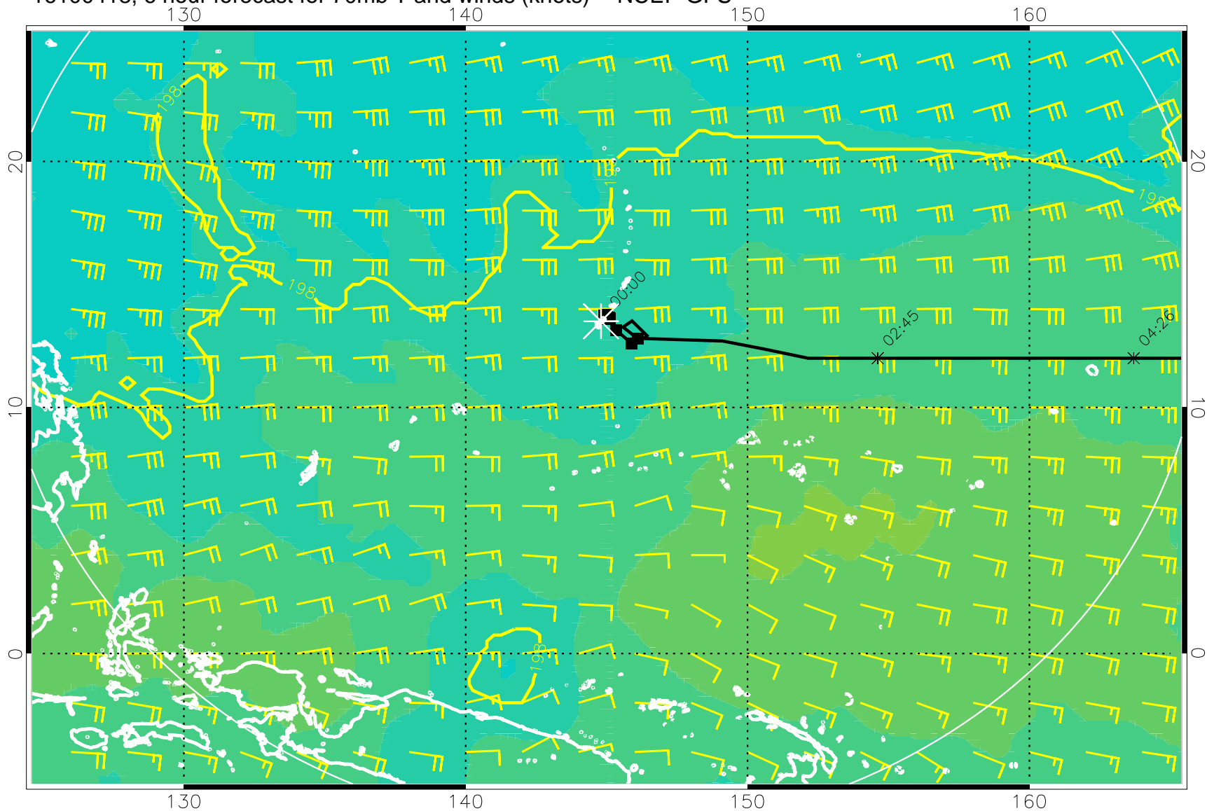
16100418, 6 hour forecast for 70mb T and winds (knots) -- NCEP GFS
