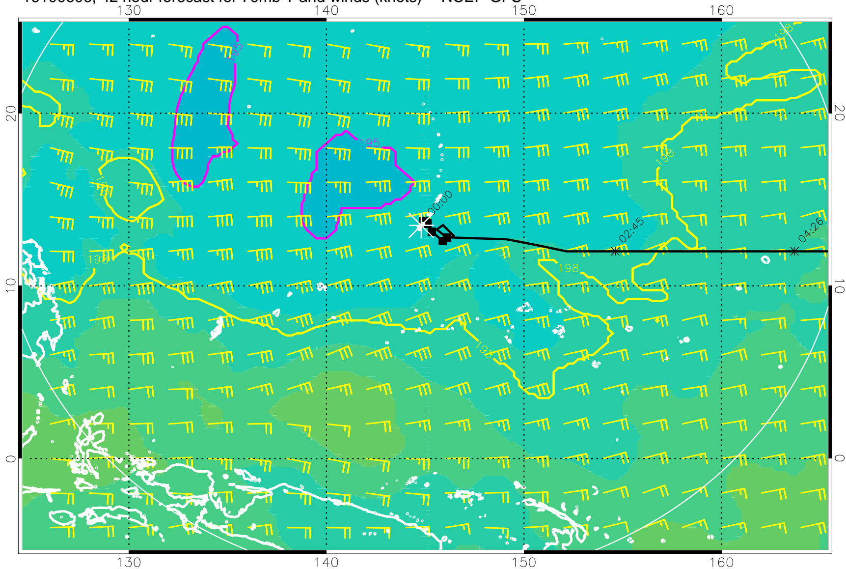
16100606, 42 hour forecast for 70mb T and winds (knots) -- NCEP GFS
