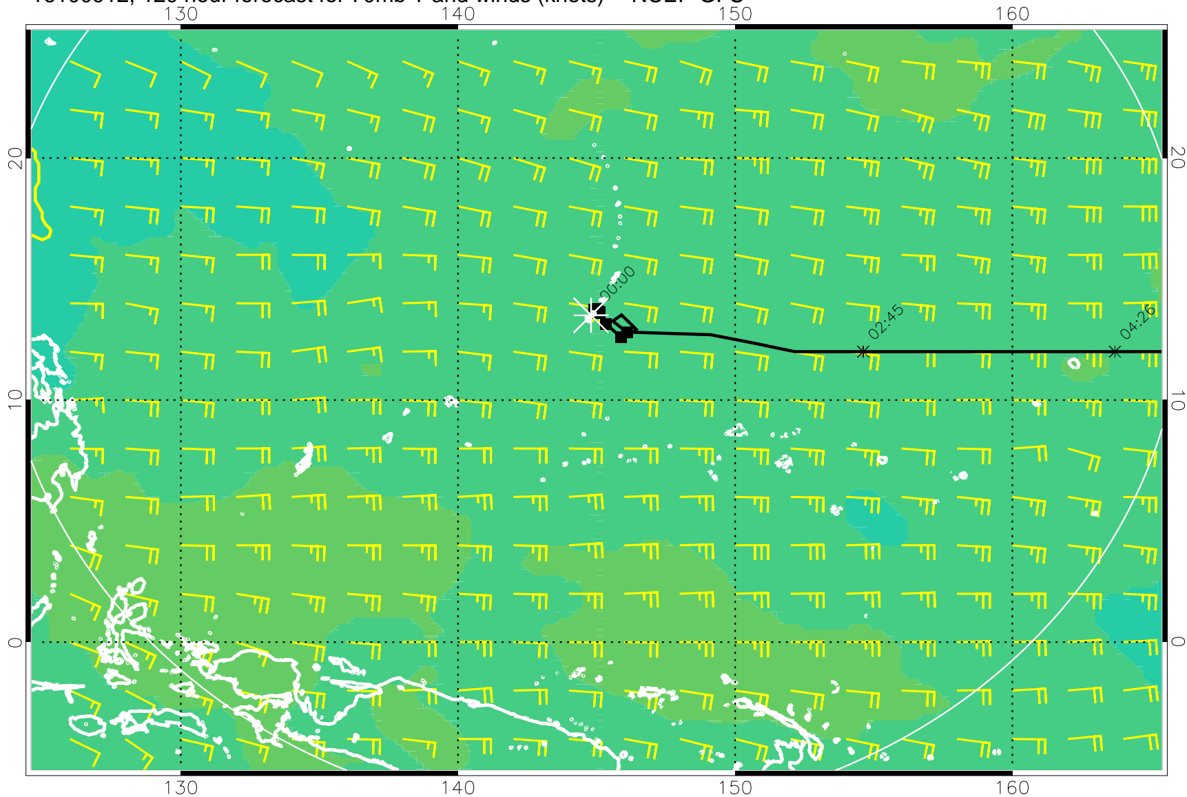
16100912, 120 hour forecast for 70mb T and winds (knots) -- NCEP GFS
