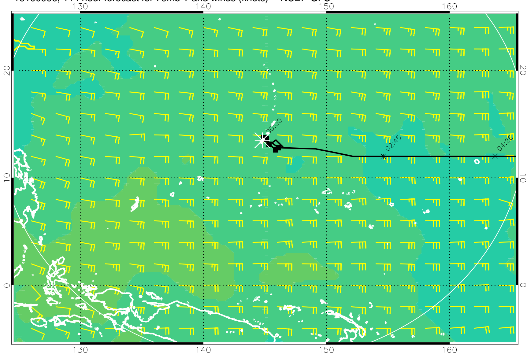
16100906, 114 hour forecast for 70mb T and winds (knots) -- NCEP GFS
