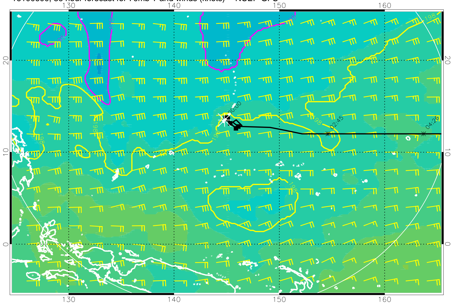
16100600, 36 hour forecast for 70mb T and winds (knots) -- NCEP GFS
