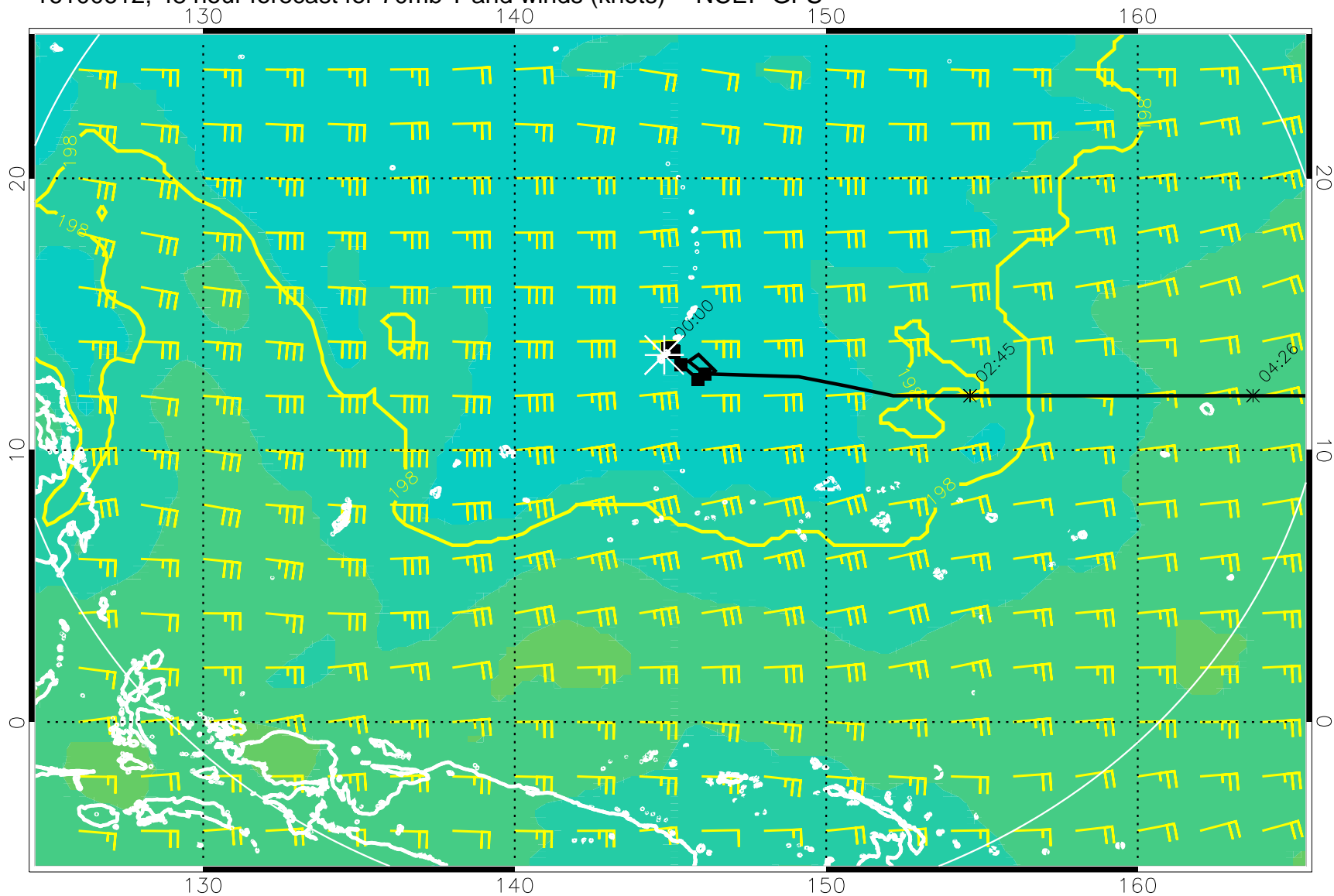
16100612, 48 hour forecast for 70mb T and winds (knots) -- NCEP GFS
