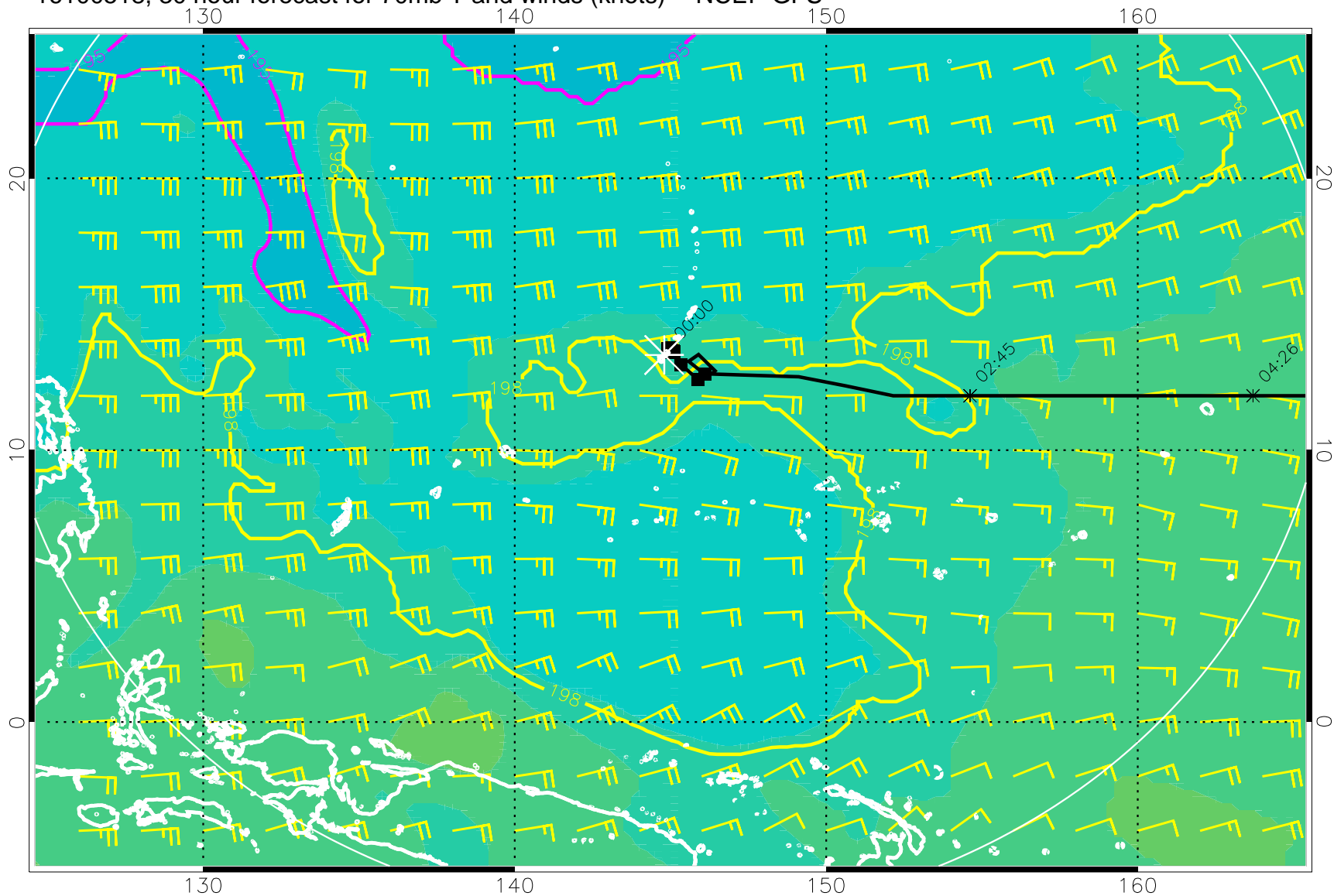
16100518, 30 hour forecast for 70mb T and winds (knots) -- NCEP GFS
