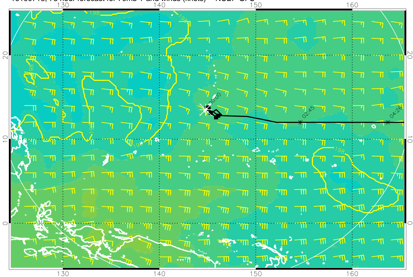
16100718, 78 hour forecast for 70mb T and winds (knots) -- NCEP GFS
