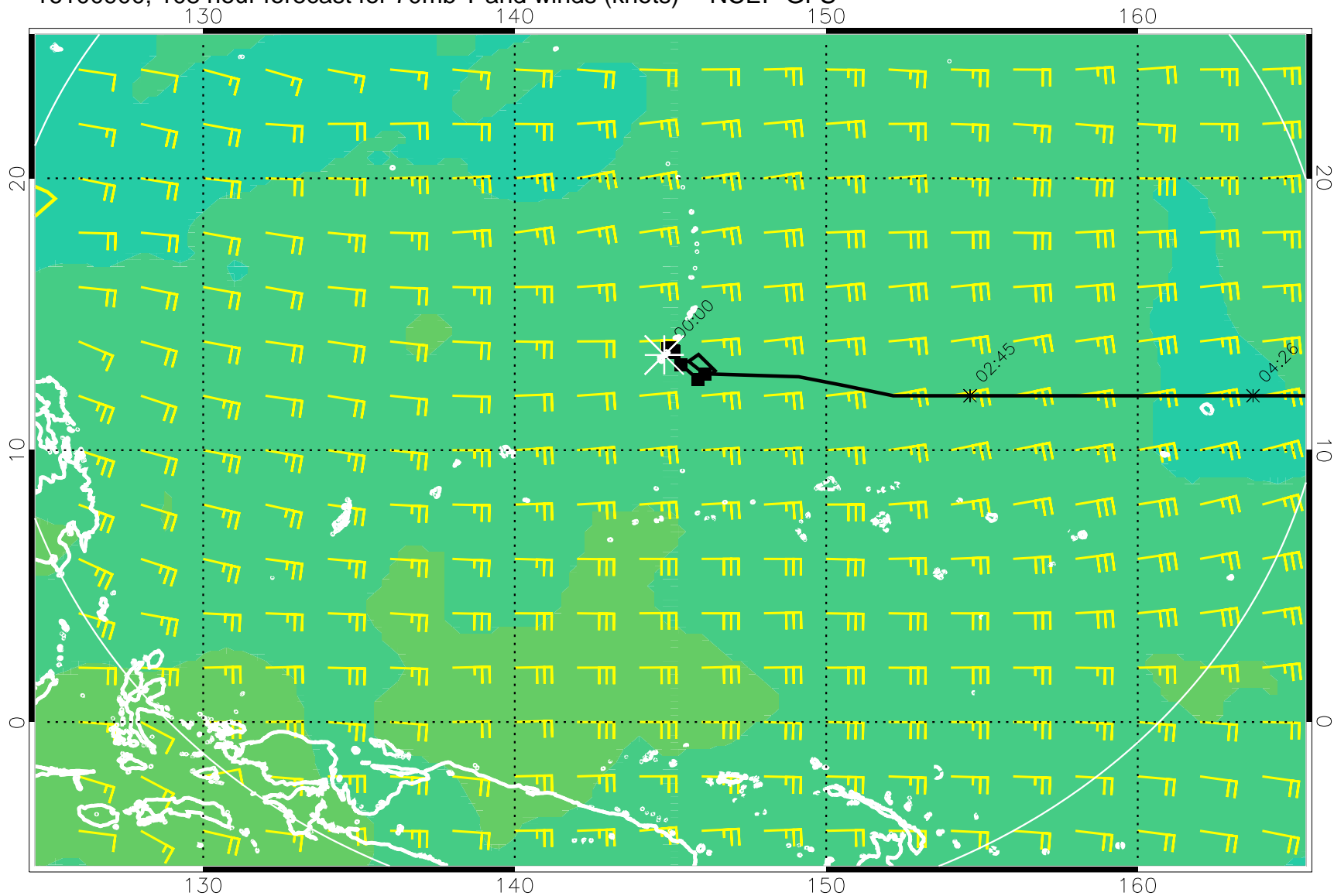
16100900, 108 hour forecast for 70mb T and winds (knots) -- NCEP GFS
