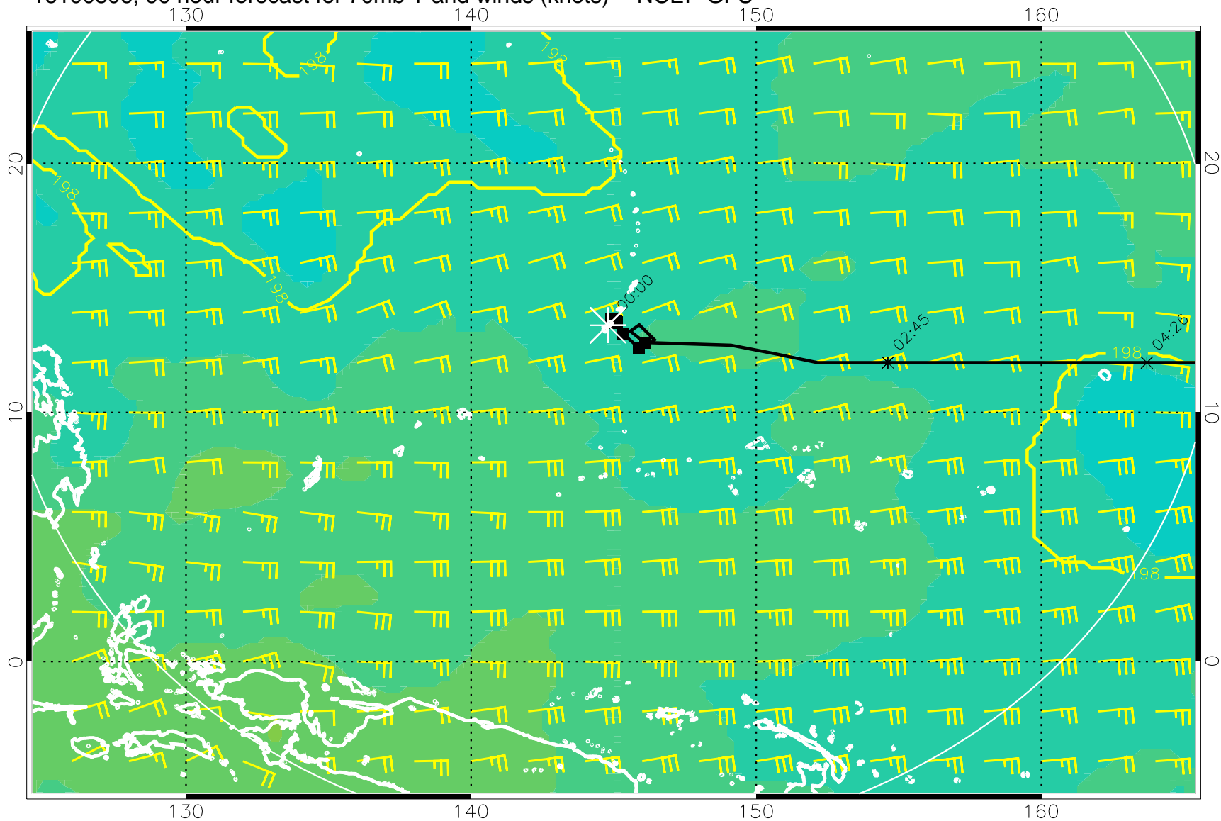
16100806, 90 hour forecast for 70mb T and winds (knots) -- NCEP GFS
