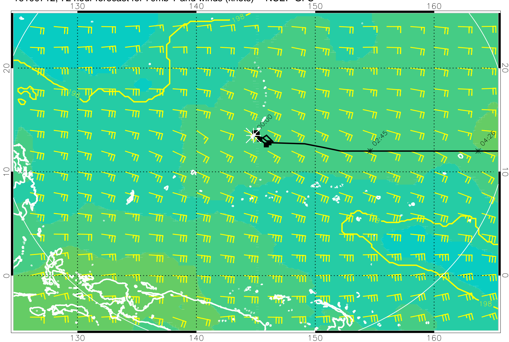
16100712, 72 hour forecast for 70mb T and winds (knots) -- NCEP GFS
