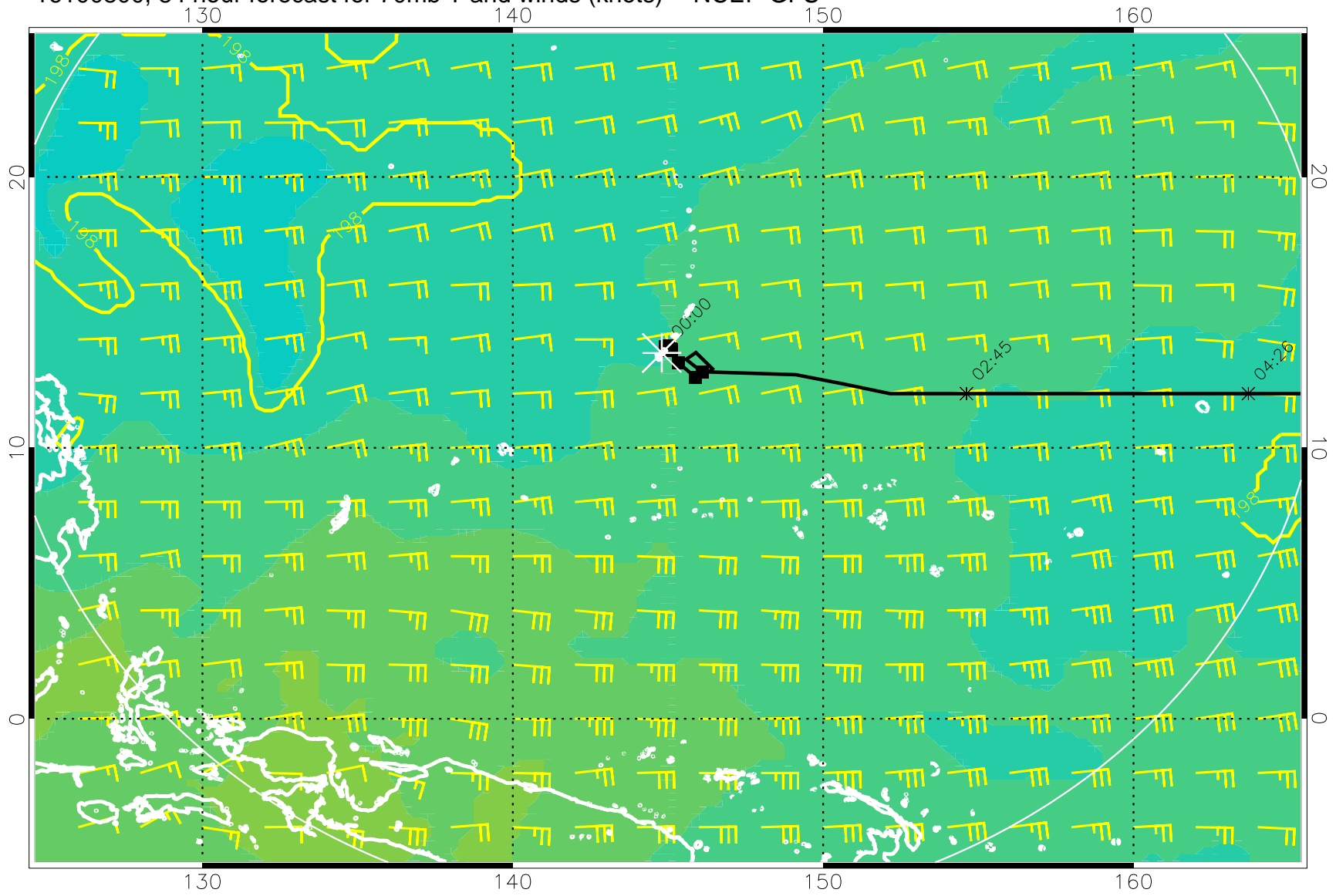
16100800, 84 hour forecast for 70mb T and winds (knots) -- NCEP GFS
