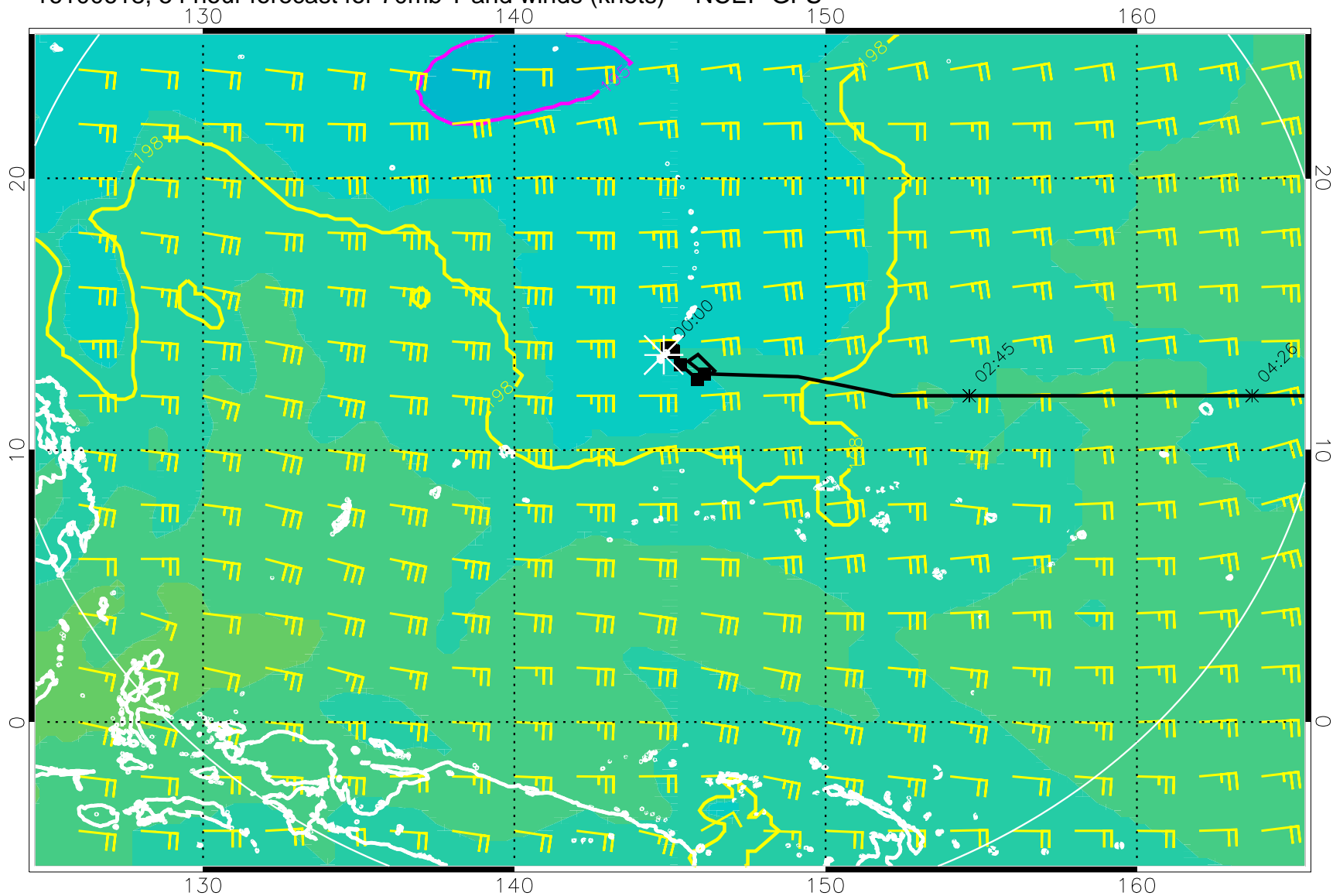
16100618, 54 hour forecast for 70mb T and winds (knots) -- NCEP GFS
