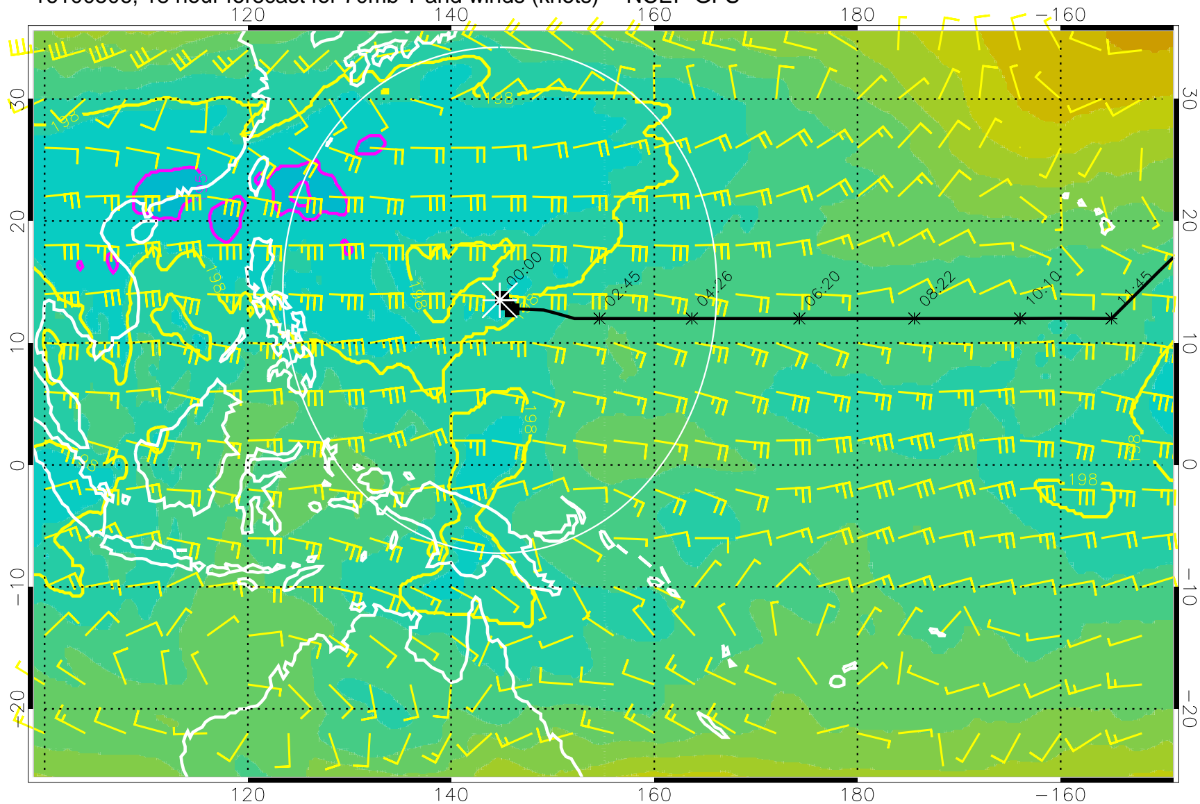
16100506, 18 hour forecast for 70mb T and winds (knots) -- NCEP GFS
