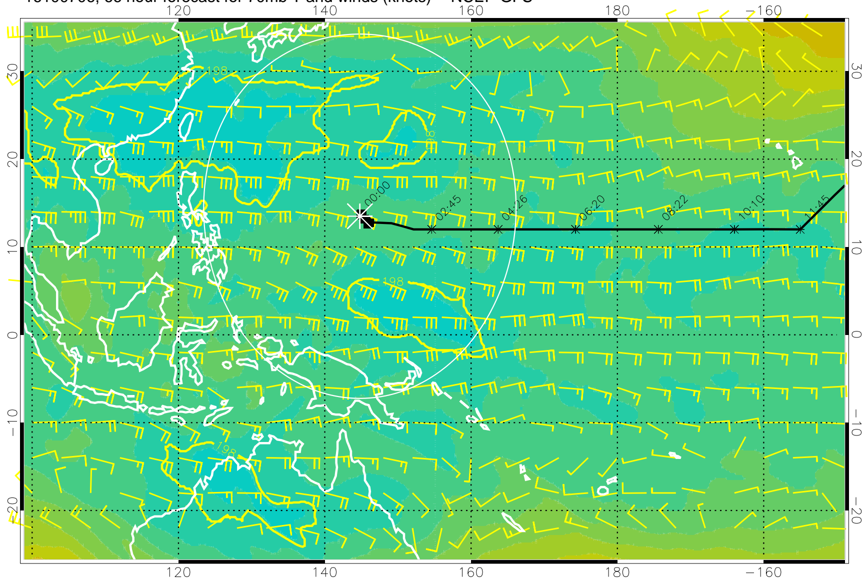
16100706, 66 hour forecast for 70mb T and winds (knots) -- NCEP GFS
