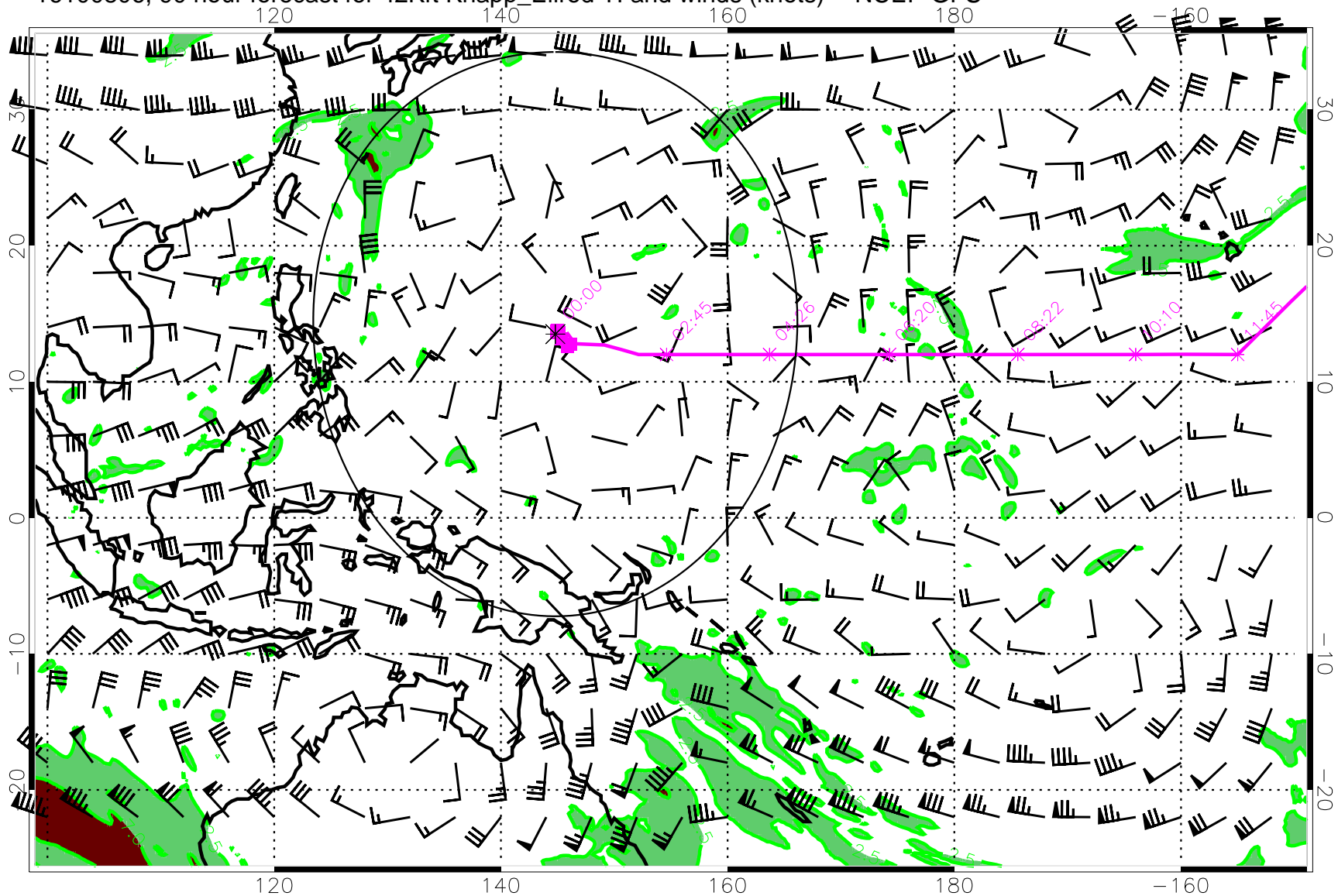
16100806, 90 hour forecast for 42Kft Knapp_Ellrod TI and winds (knots) -- NCEP GFS
