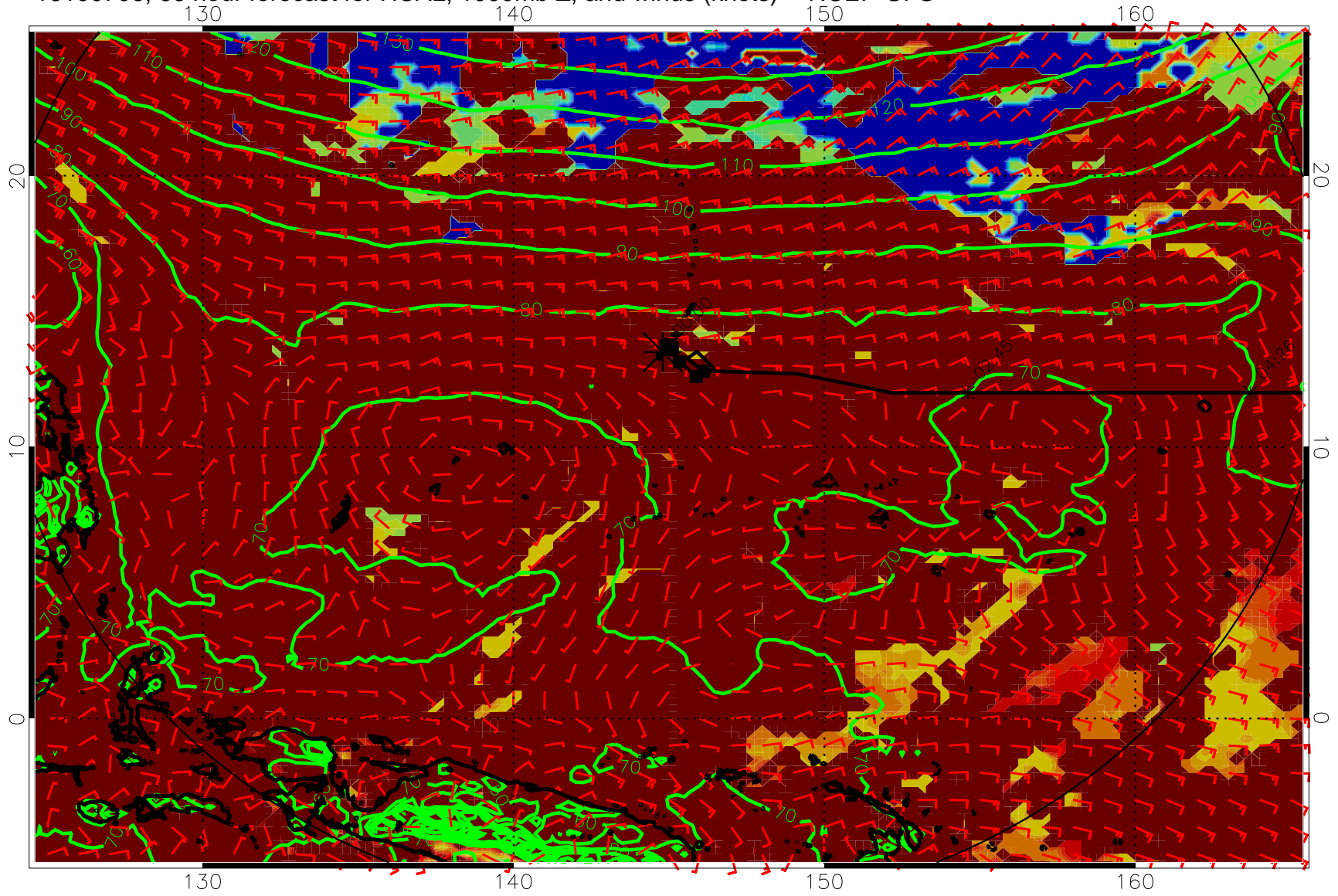
16100706, 66 hour forecast for HCAL, 1000mb Z, and winds (knots) -- NCEP GFS
