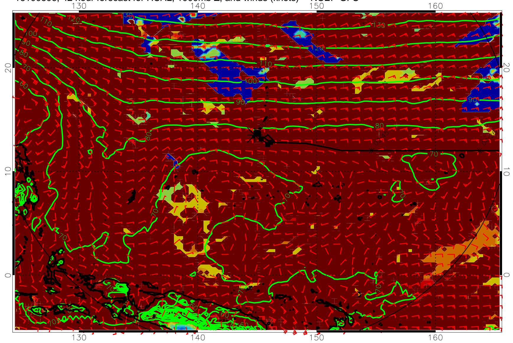
16100606, 42 hour forecast for HCAL, 1000mb Z, and winds (knots) -- NCEP GFS
