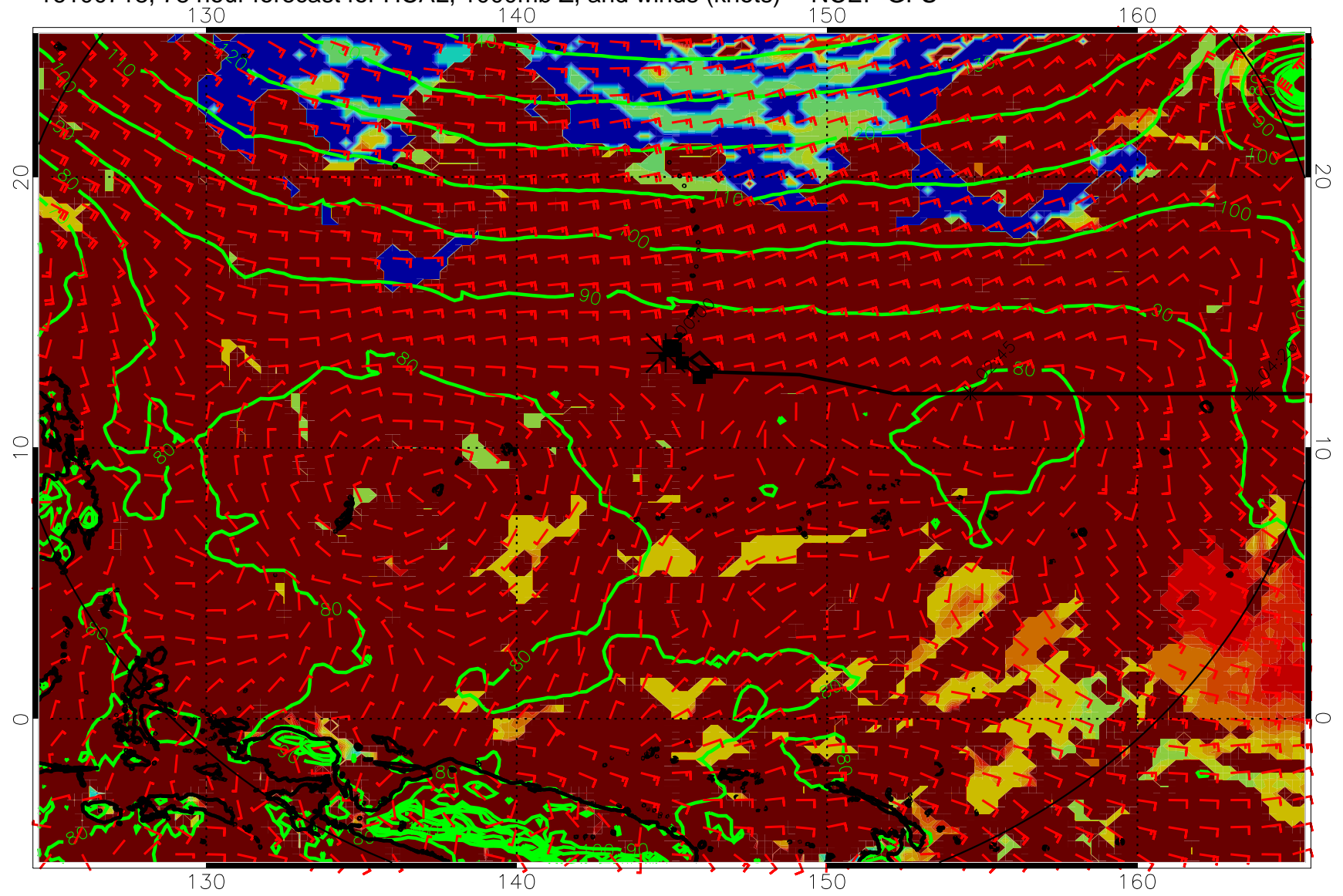
16100718, 78 hour forecast for HCAL, 1000mb Z, and winds (knots) -- NCEP GFS
