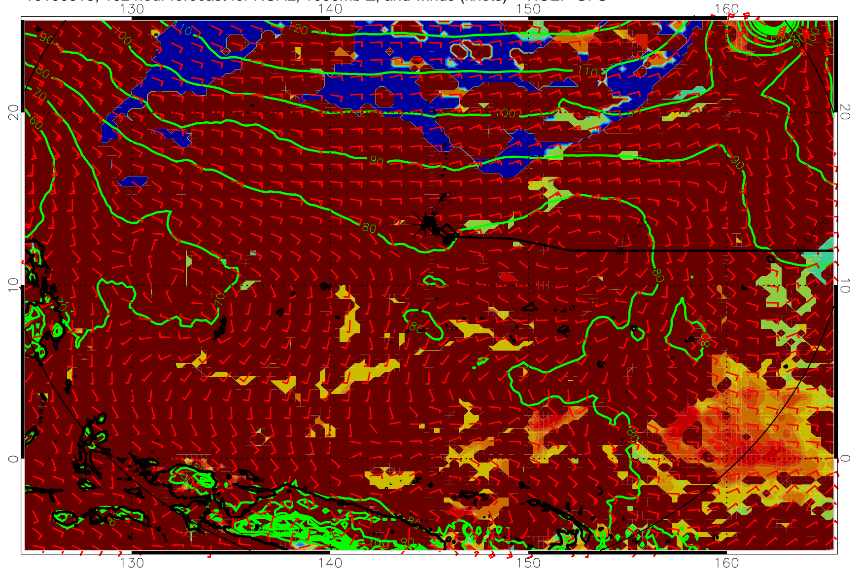
16100818, 102 hour forecast for HCAL, 1000mb Z, and winds (knots) -- NCEP GFS
