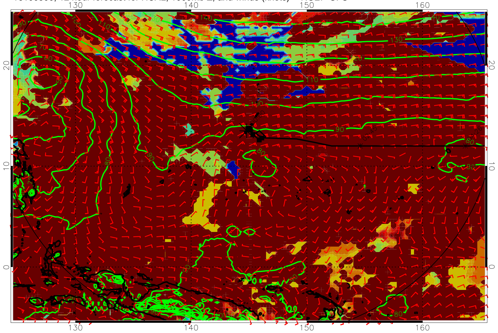
16100500, 12 hour forecast for HCAL, 1000mb Z, and winds (knots) -- NCEP GFS
