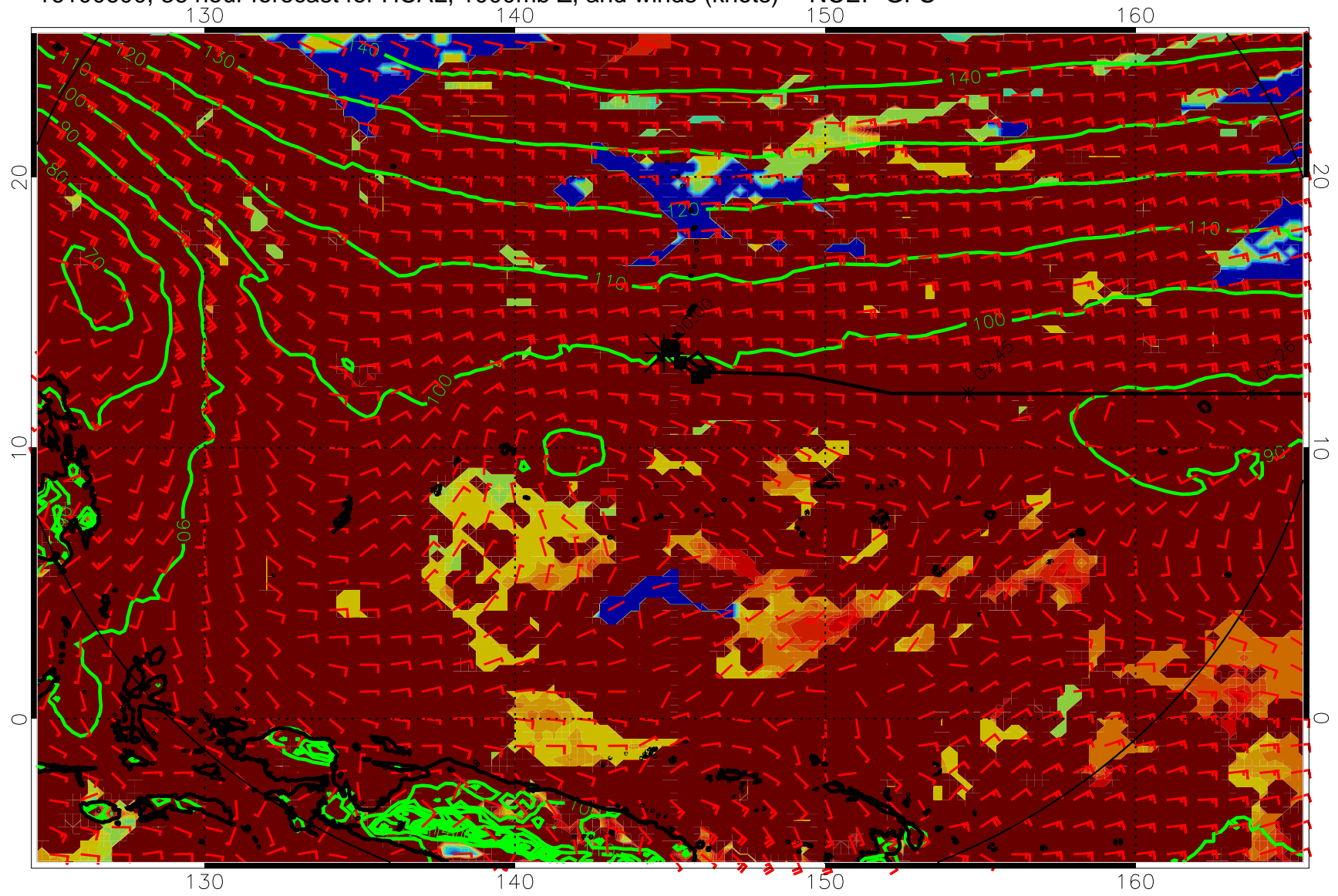
16100600, 36 hour forecast for HCAL, 1000mb Z, and winds (knots) -- NCEP GFS
