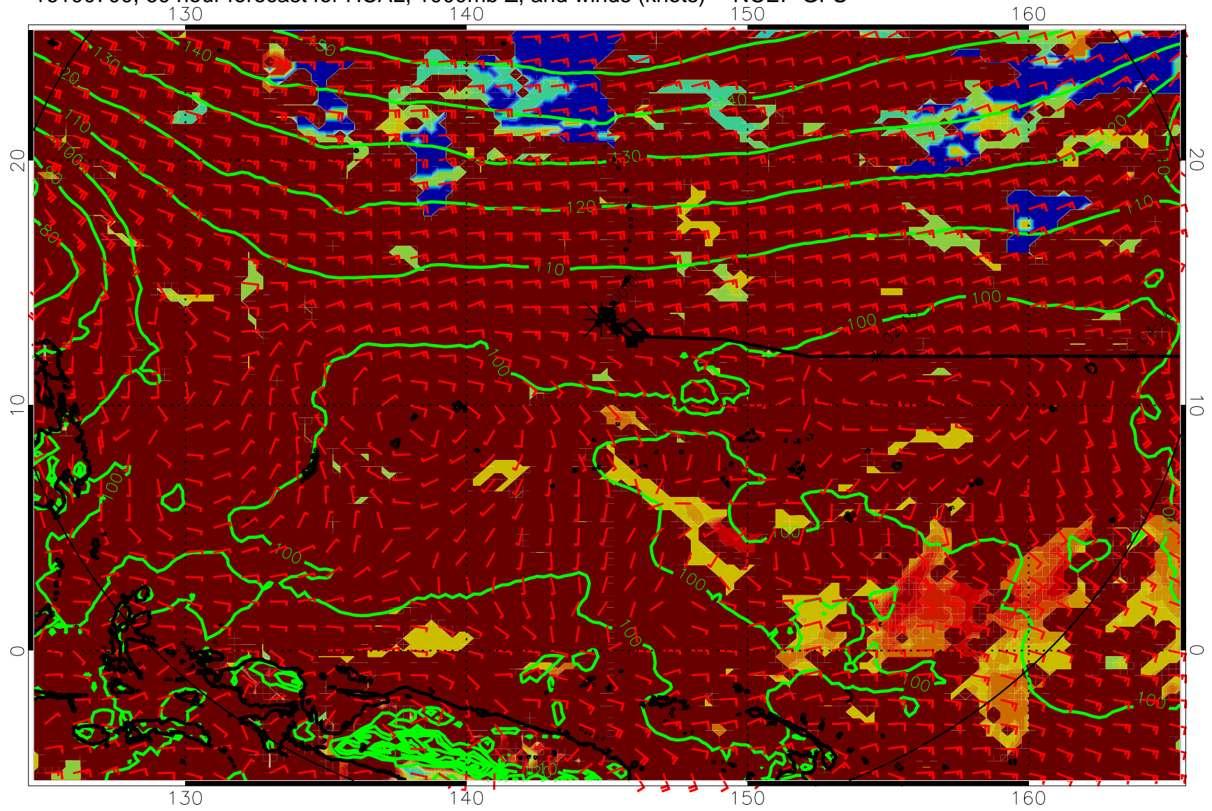
16100700, 60 hour forecast for HCAL, 1000mb Z, and winds (knots) -- NCEP GFS
