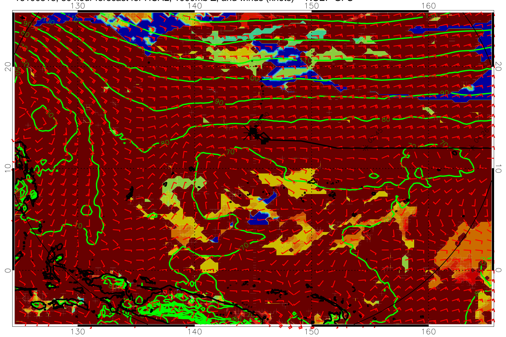
16100518, 30 hour forecast for HCAL, 1000mb Z, and winds (knots) -- NCEP GFS
