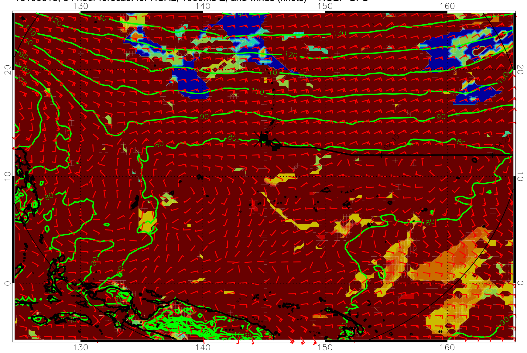
16100618, 54 hour forecast for HCAL, 1000mb Z, and winds (knots) -- NCEP GFS
