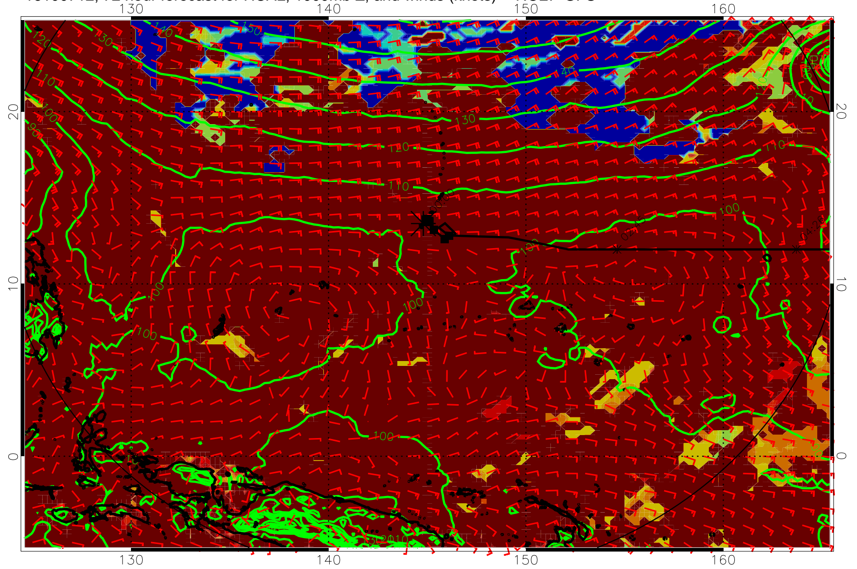
16100712, 72 hour forecast for HCAL, 1000mb Z, and winds (knots) -- NCEP GFS
