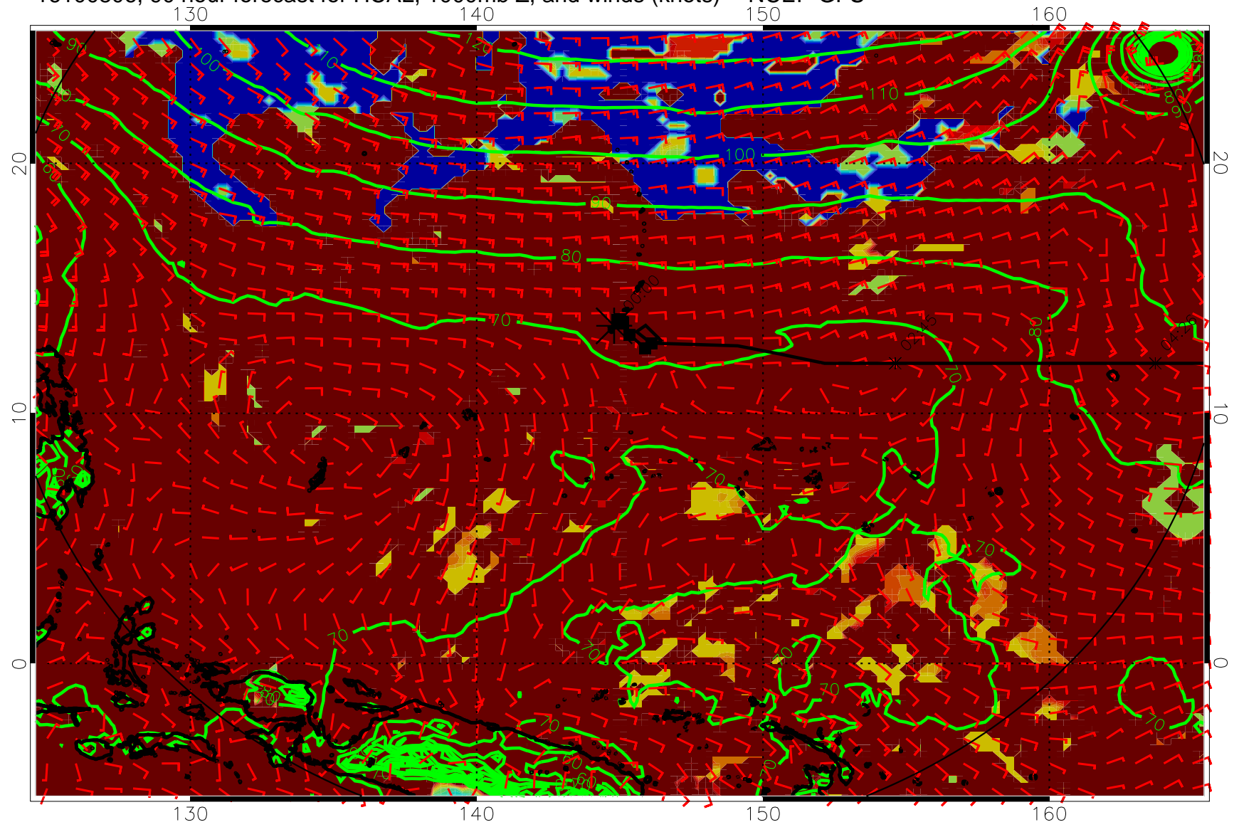
16100806, 90 hour forecast for HCAL, 1000mb Z, and winds (knots) -- NCEP GFS
