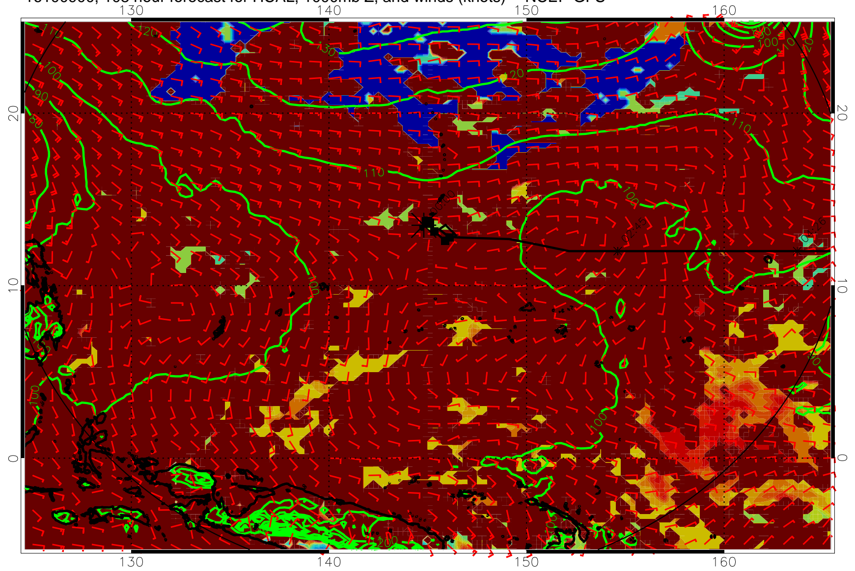
16100900, 108 hour forecast for HCAL, 1000mb Z, and winds (knots) -- NCEP GFS
