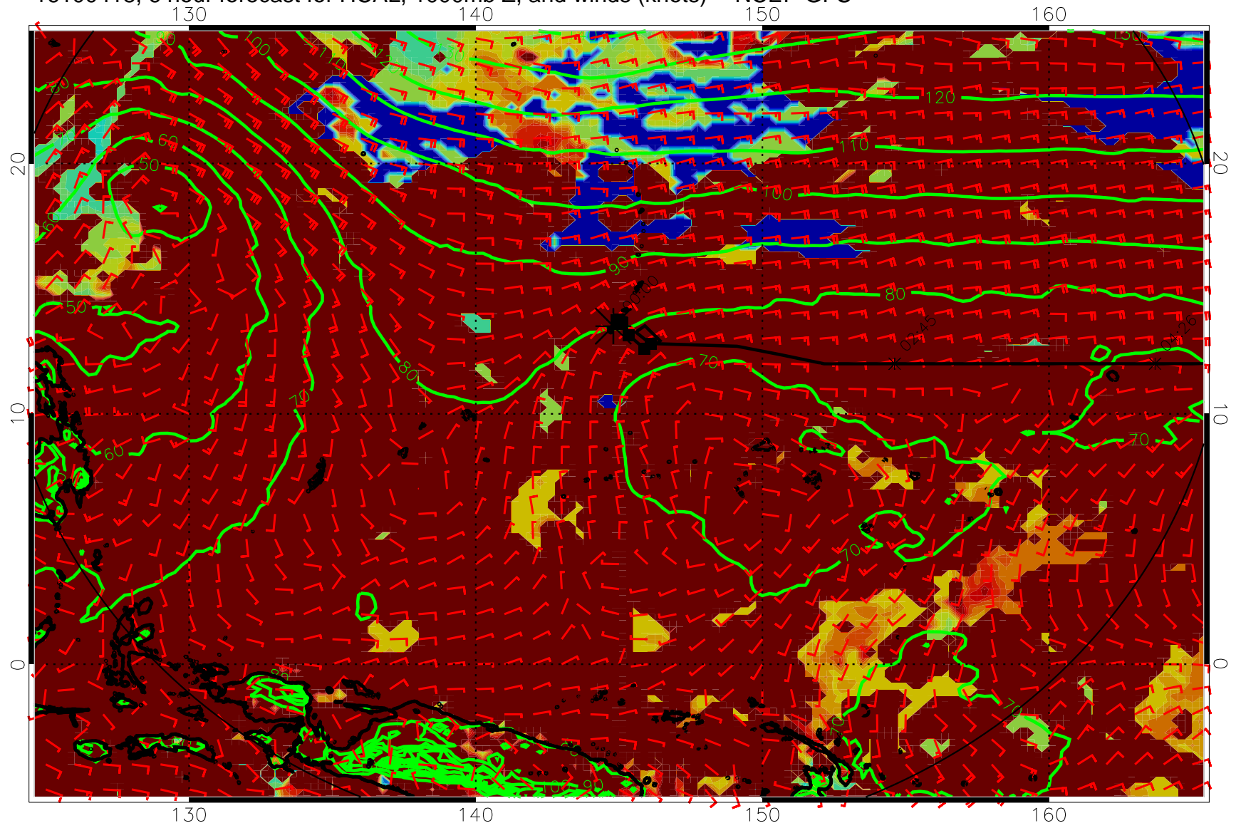
16100418, 6 hour forecast for HCAL, 1000mb Z, and winds (knots) -- NCEP GFS
