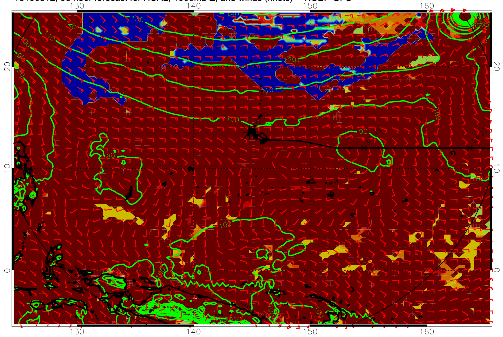
16100812, 96 hour forecast for HCAL, 1000mb Z, and winds (knots) -- NCEP GFS
