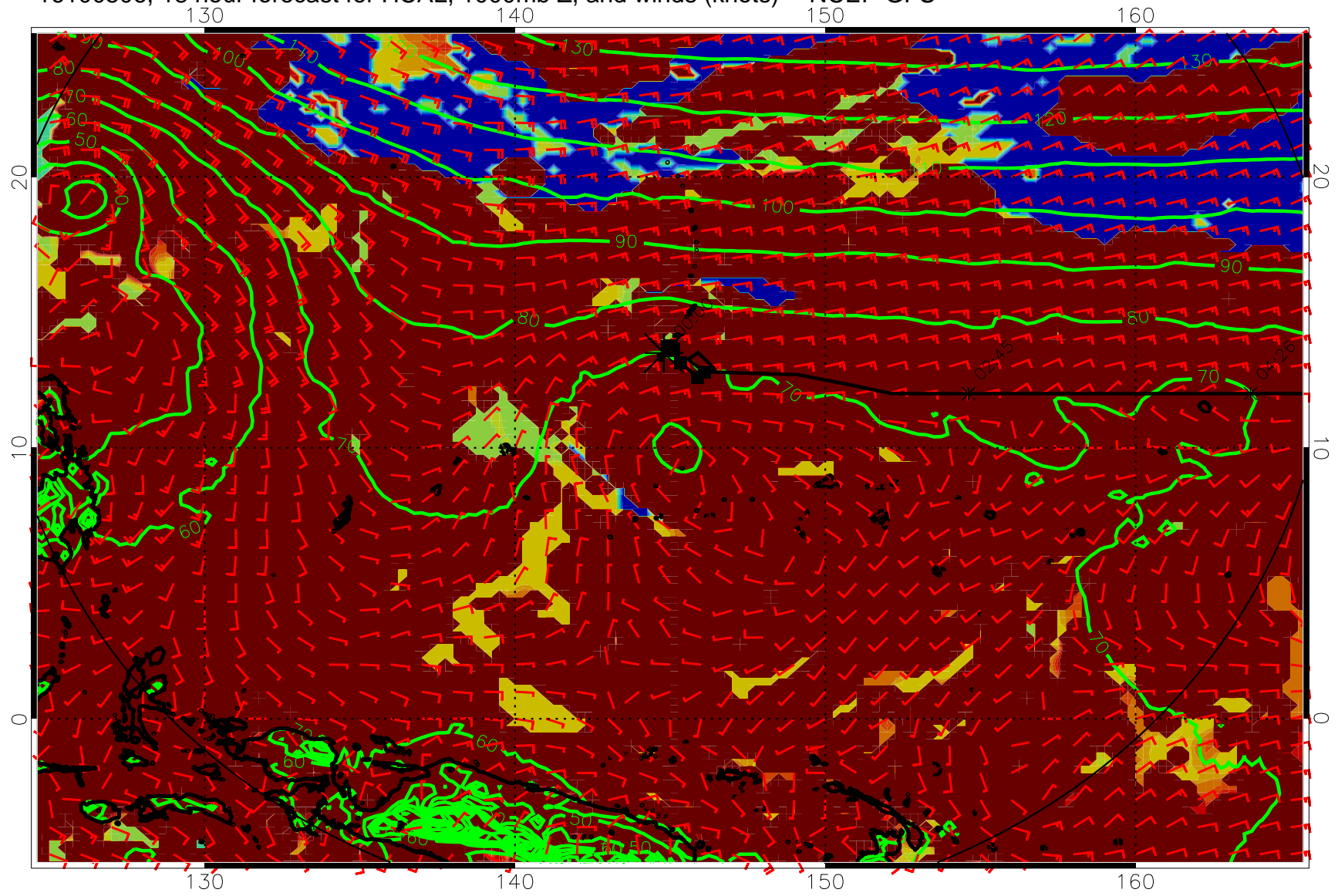
16100506, 18 hour forecast for HCAL, 1000mb Z, and winds (knots) -- NCEP GFS
