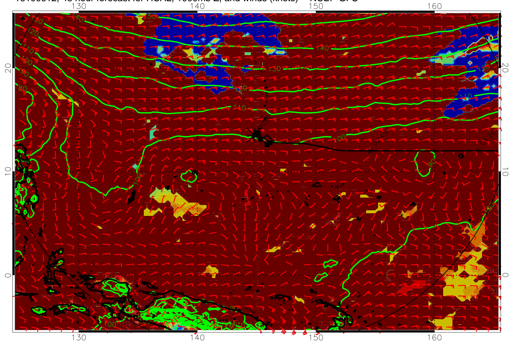
16100612, 48 hour forecast for HCAL, 1000mb Z, and winds (knots) -- NCEP GFS
