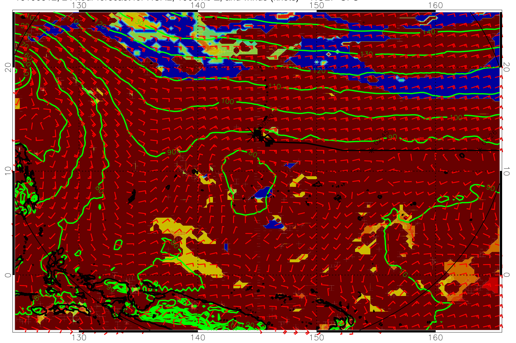
16100512, 24 hour forecast for HCAL, 1000mb Z, and winds (knots) -- NCEP GFS
