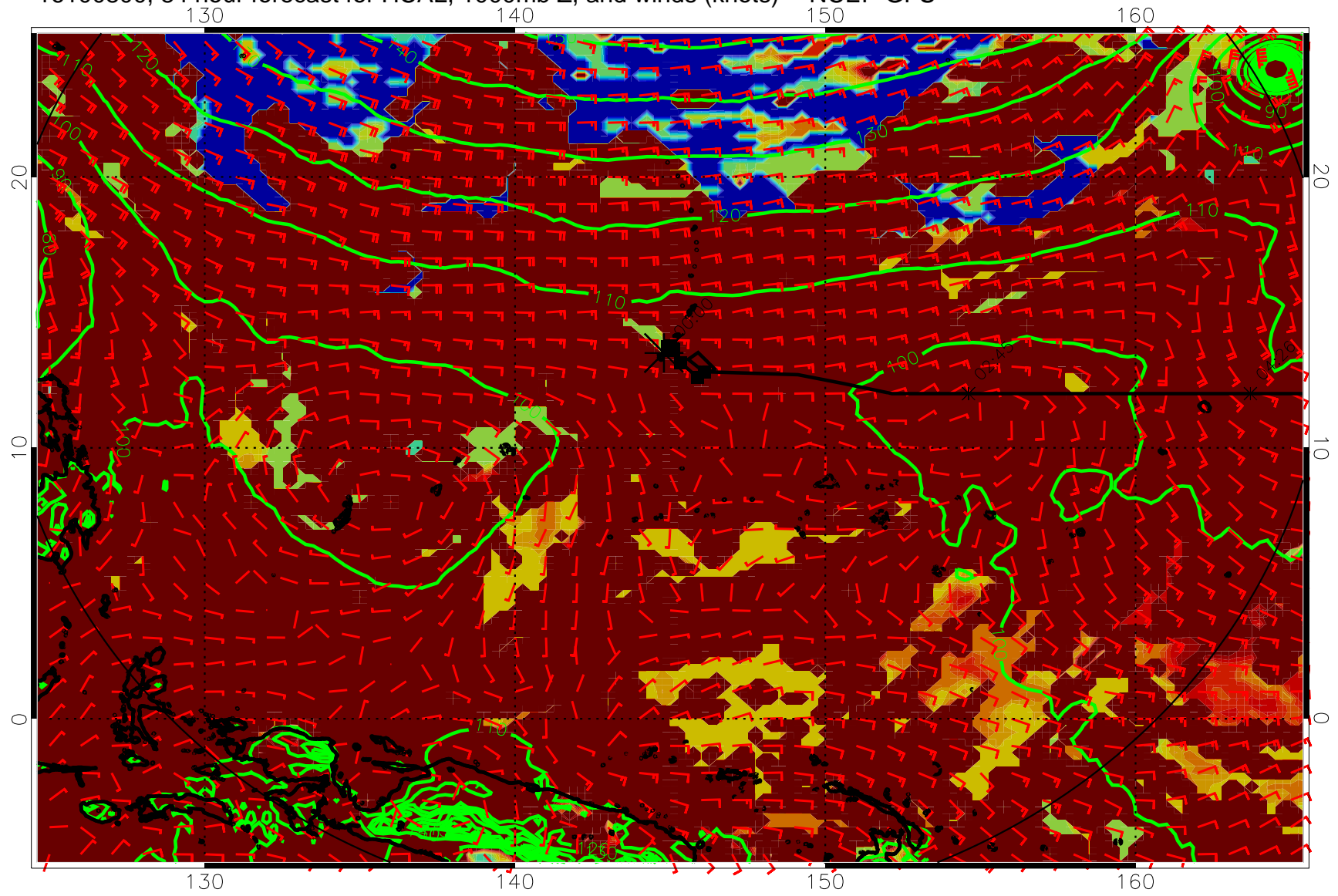
16100800, 84 hour forecast for HCAL, 1000mb Z, and winds (knots) -- NCEP GFS
