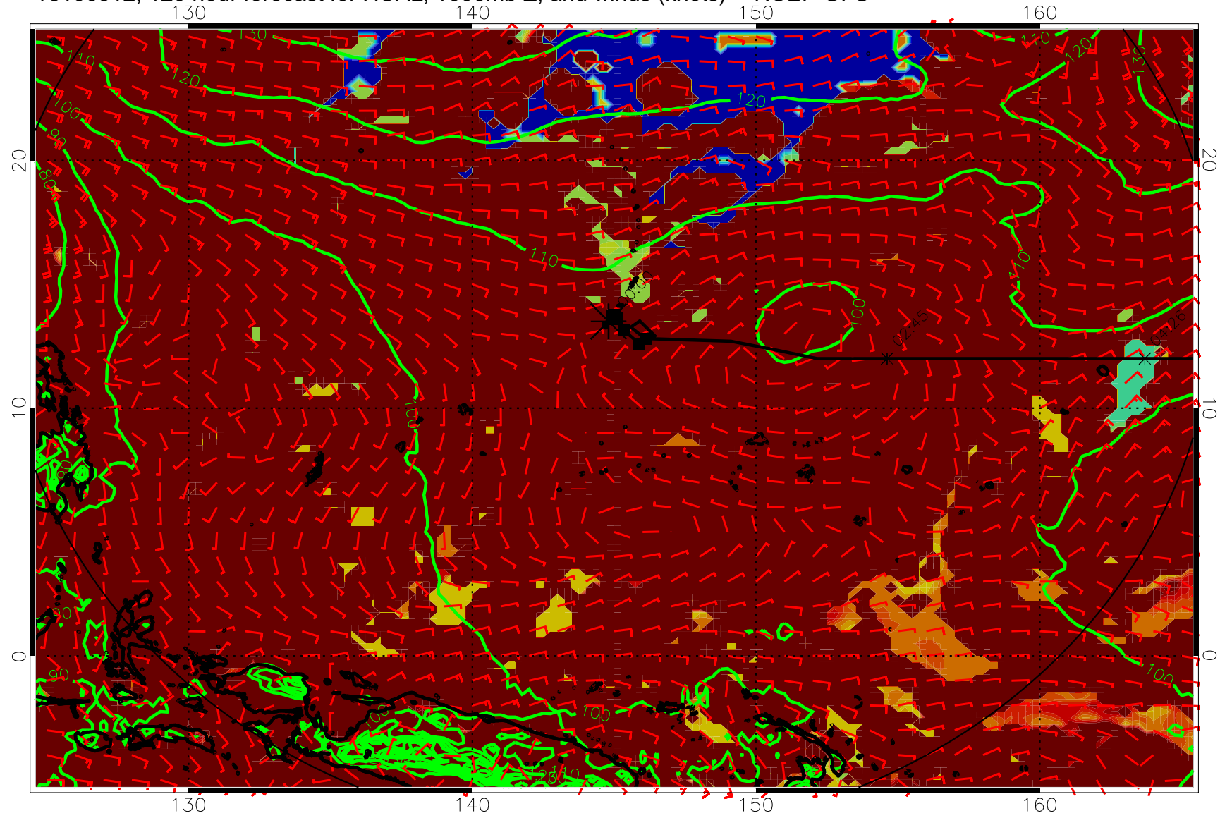
16100912, 120 hour forecast for HCAL, 1000mb Z, and winds (knots) -- NCEP GFS
