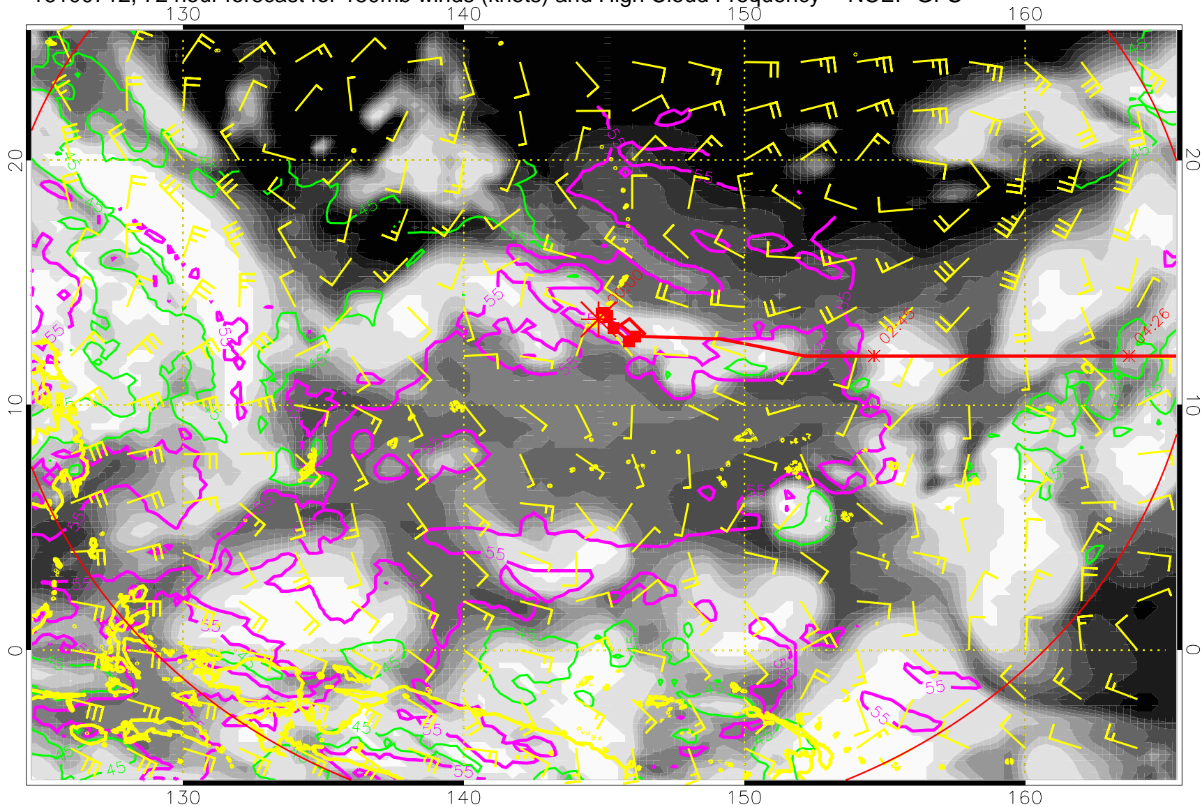
16100712, 72 hour forecast for 150mb winds (knots) and High Cloud Frequency -- NCEP GFS
