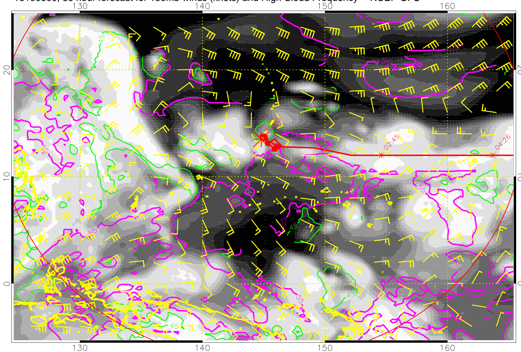
16100600, 36 hour forecast for 150mb winds (knots) and High Cloud Frequency -- NCEP GFS
