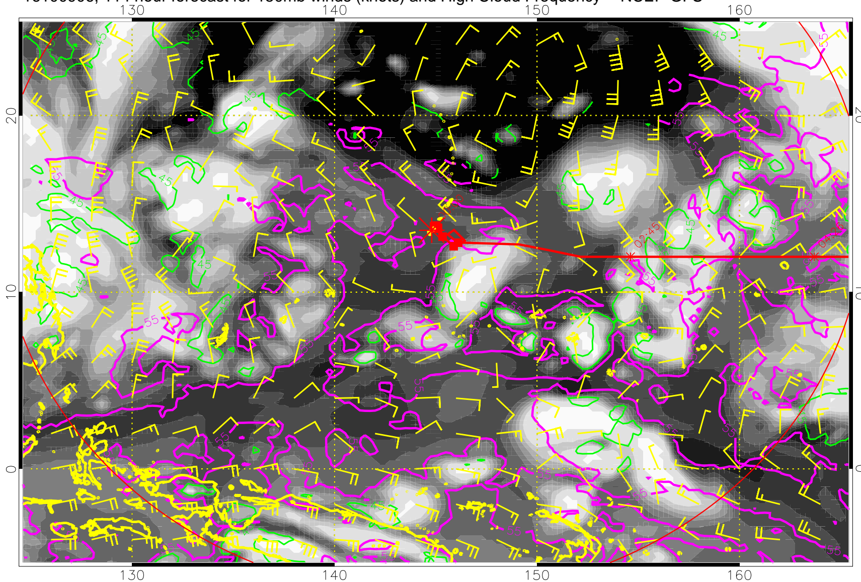
16100906, 114 hour forecast for 150mb winds (knots) and High Cloud Frequency -- NCEP GFS
