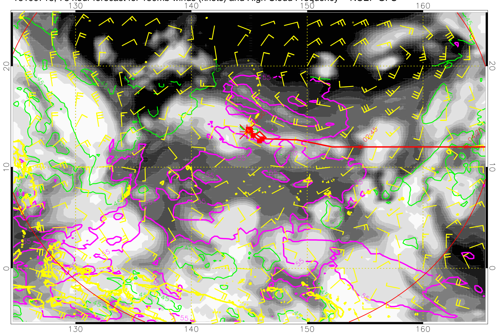
16100718, 78 hour forecast for 150mb winds (knots) and High Cloud Frequency -- NCEP GFS
