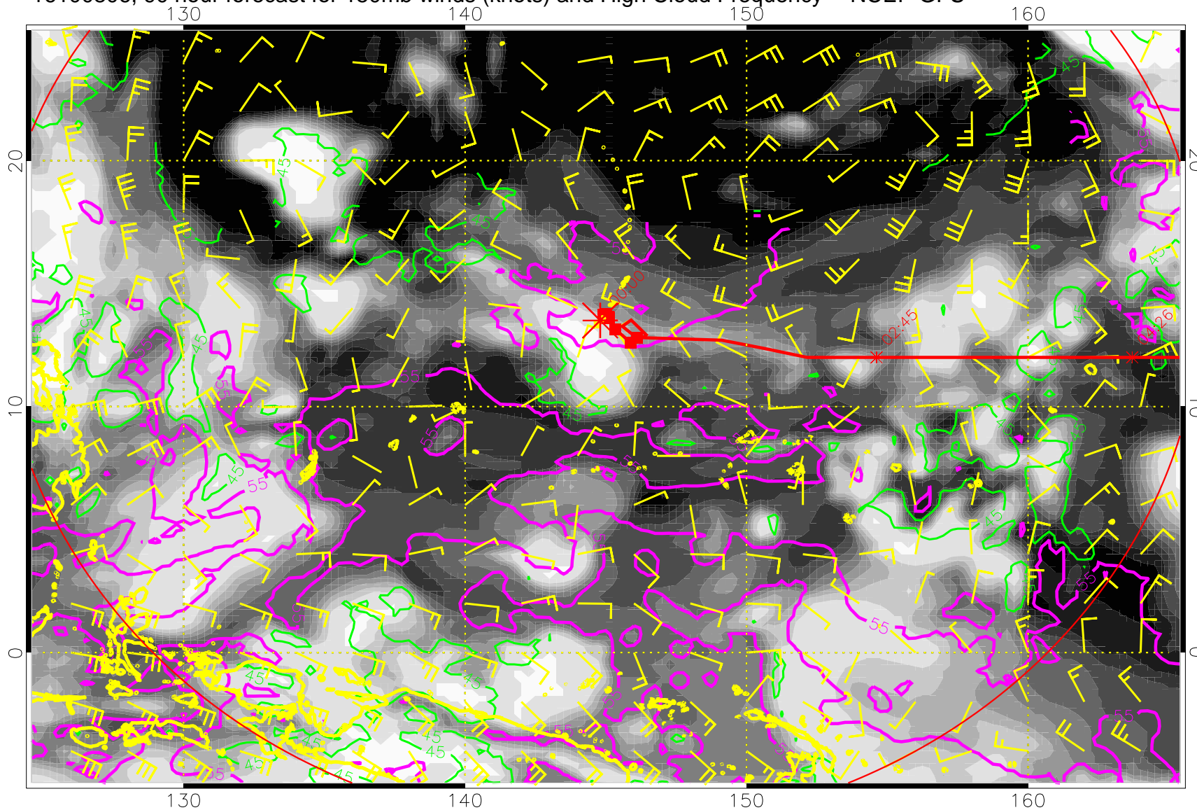
16100806, 90 hour forecast for 150mb winds (knots) and High Cloud Frequency -- NCEP GFS
