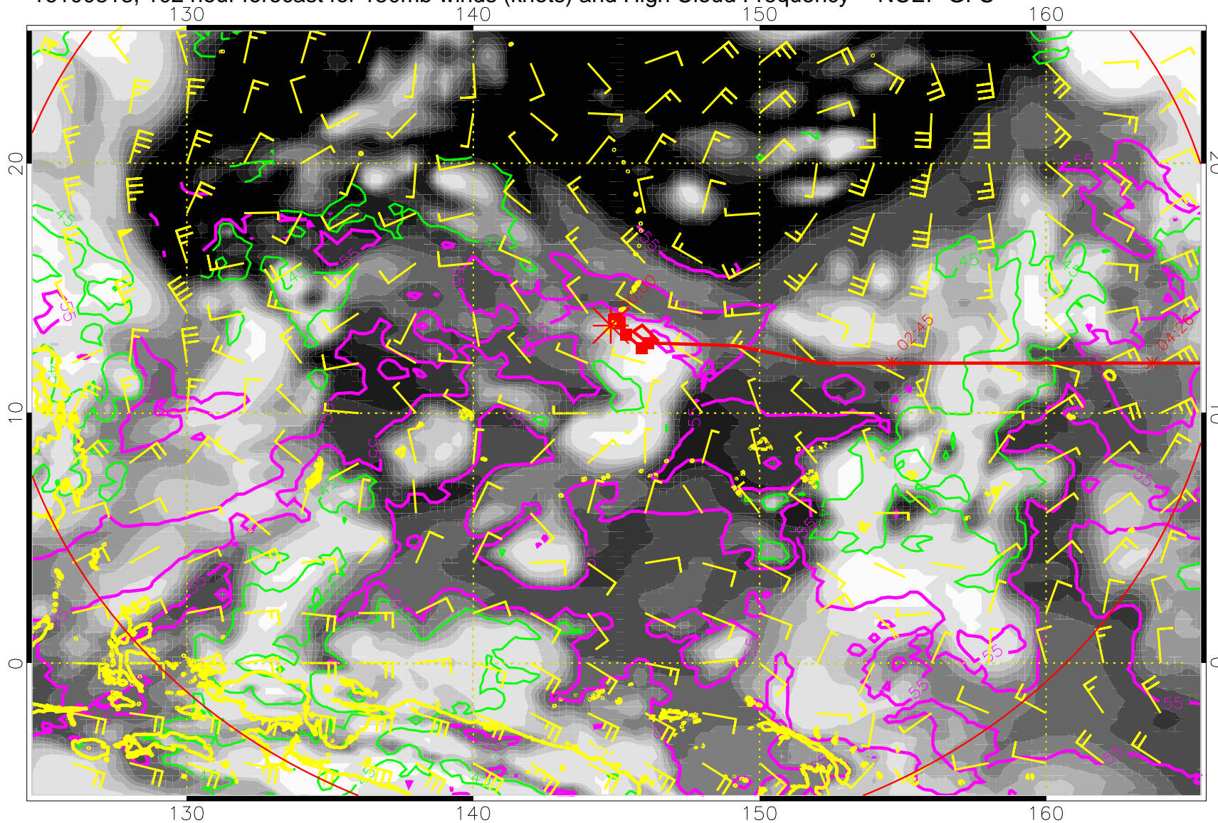
16100818, 102 hour forecast for 150mb winds (knots) and High Cloud Frequency -- NCEP GFS
