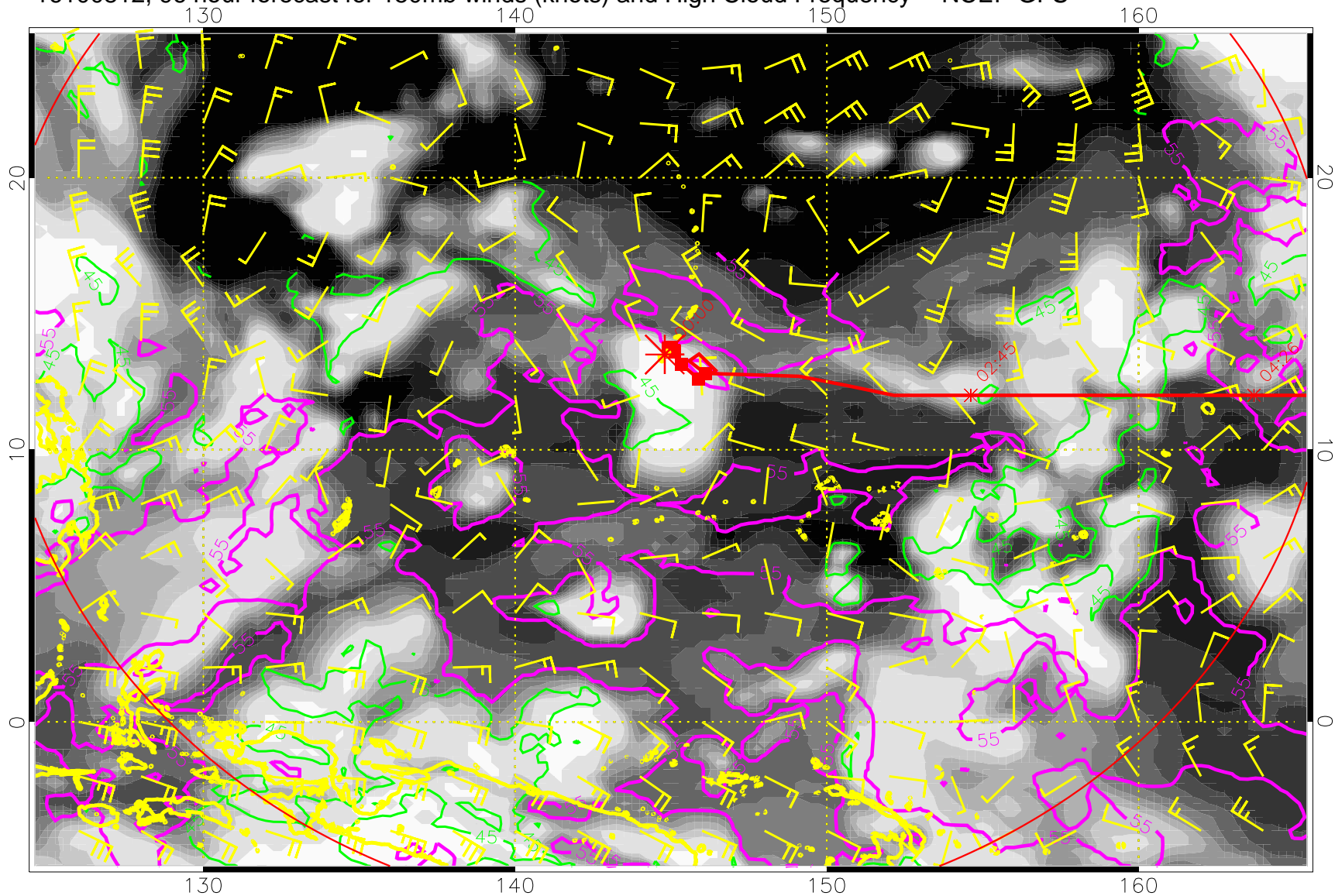
16100812, 96 hour forecast for 150mb winds (knots) and High Cloud Frequency -- NCEP GFS
