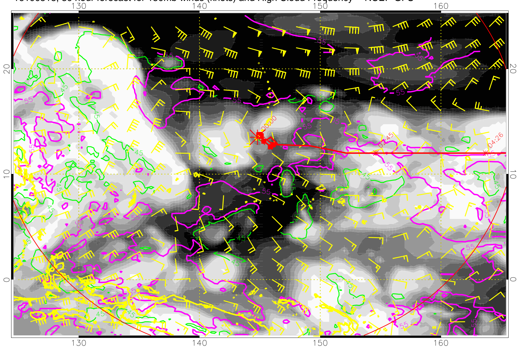
16100518, 30 hour forecast for 150mb winds (knots) and High Cloud Frequency -- NCEP GFS
