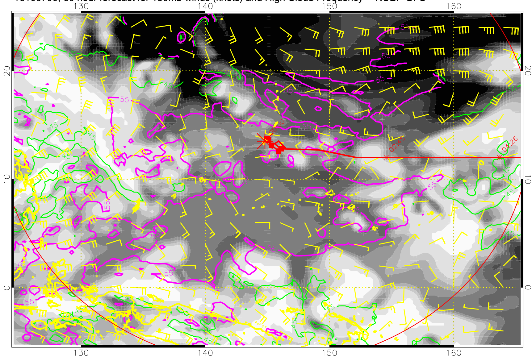
16100700, 60 hour forecast for 150mb winds (knots) and High Cloud Frequency -- NCEP GFS
