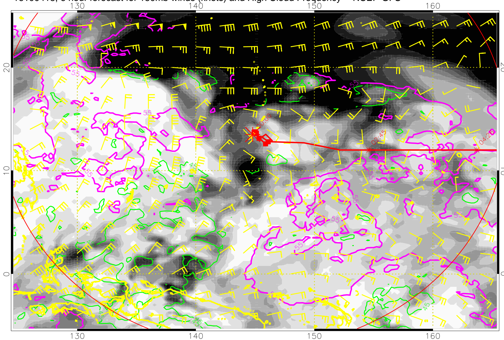
16100418, 6 hour forecast for 150mb winds (knots) and High Cloud Frequency -- NCEP GFS
