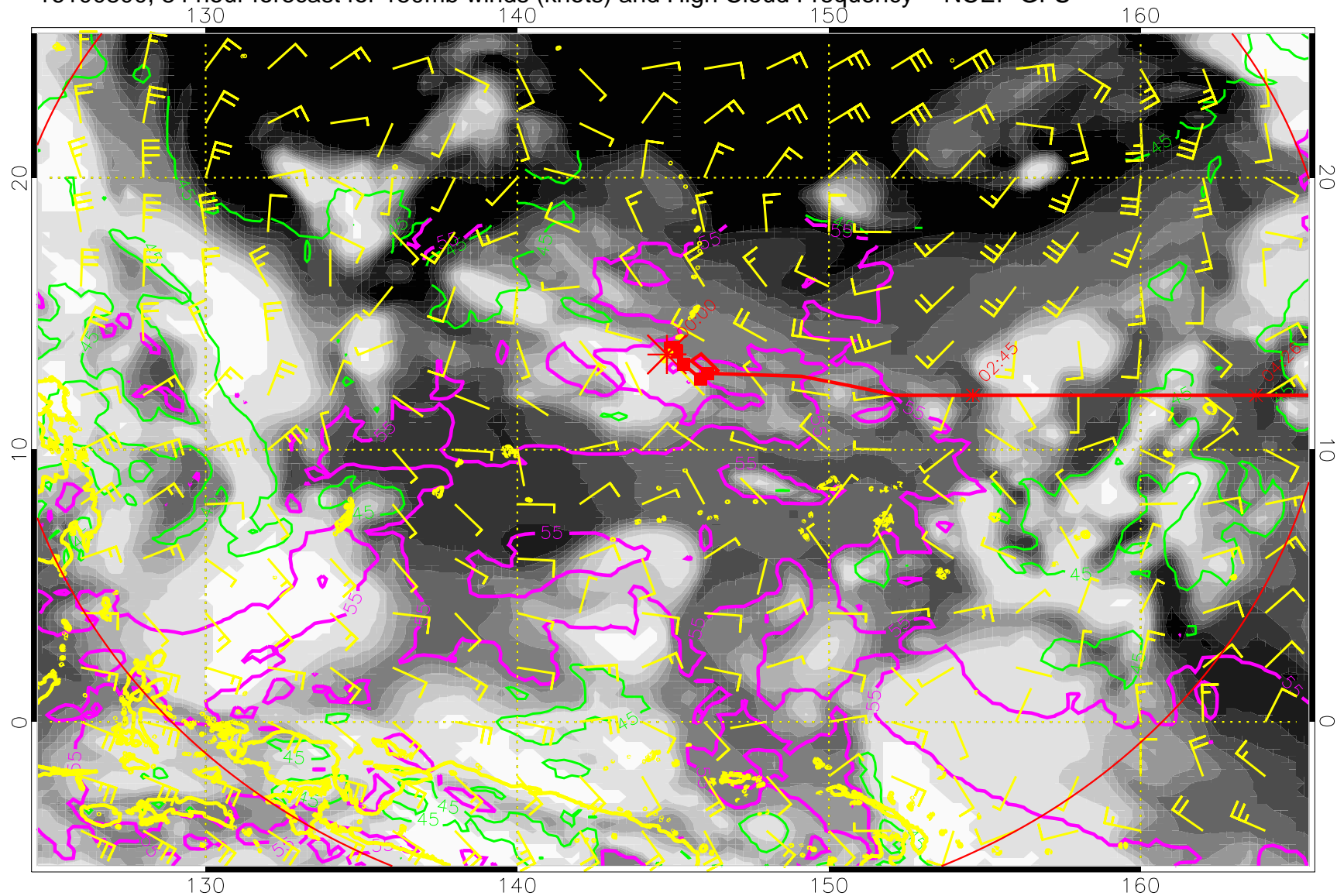
16100800, 84 hour forecast for 150mb winds (knots) and High Cloud Frequency -- NCEP GFS
