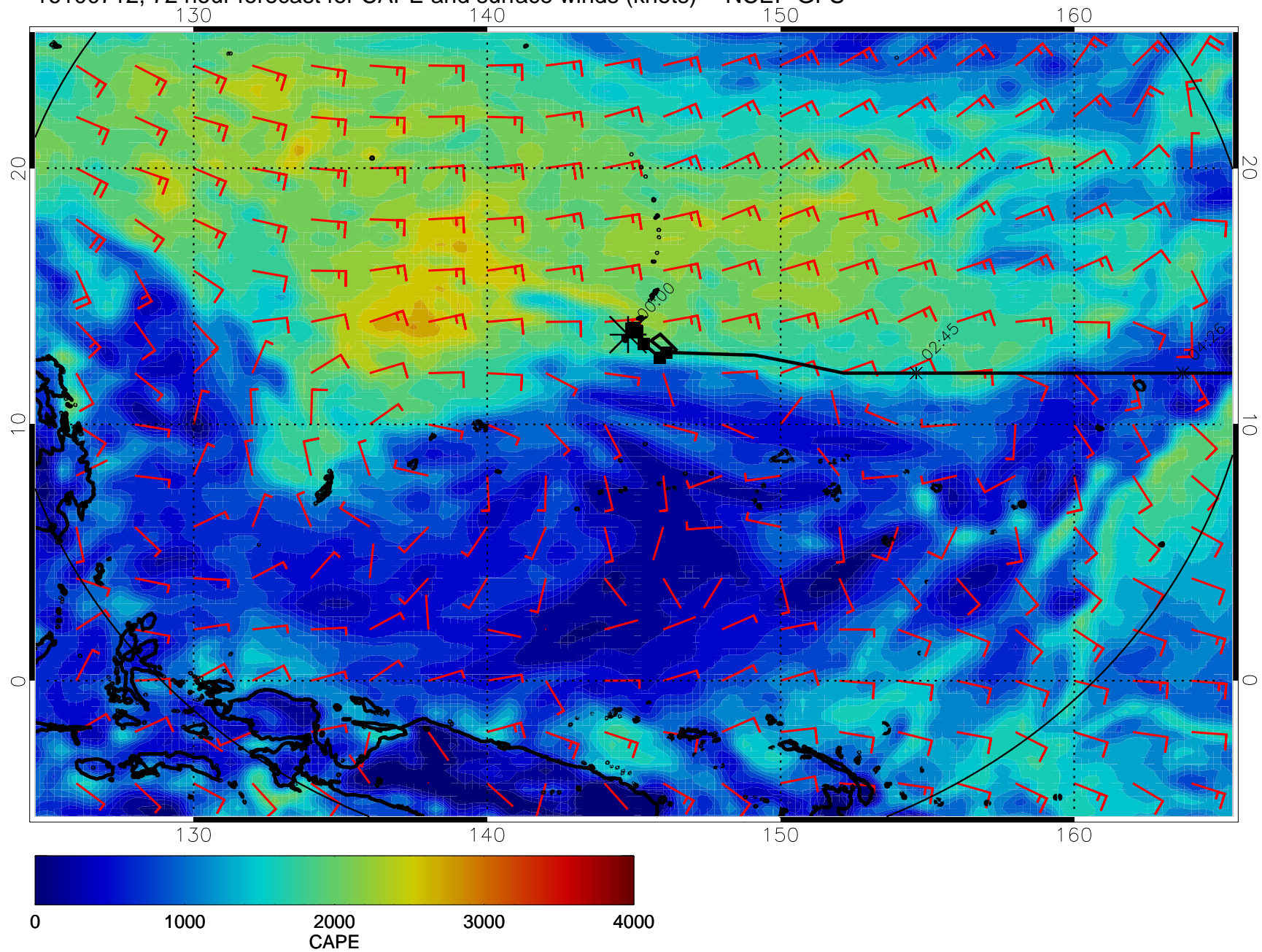
16100712, 72 hour forecast for CAPE and surface winds (knots) -- NCEP GFS
