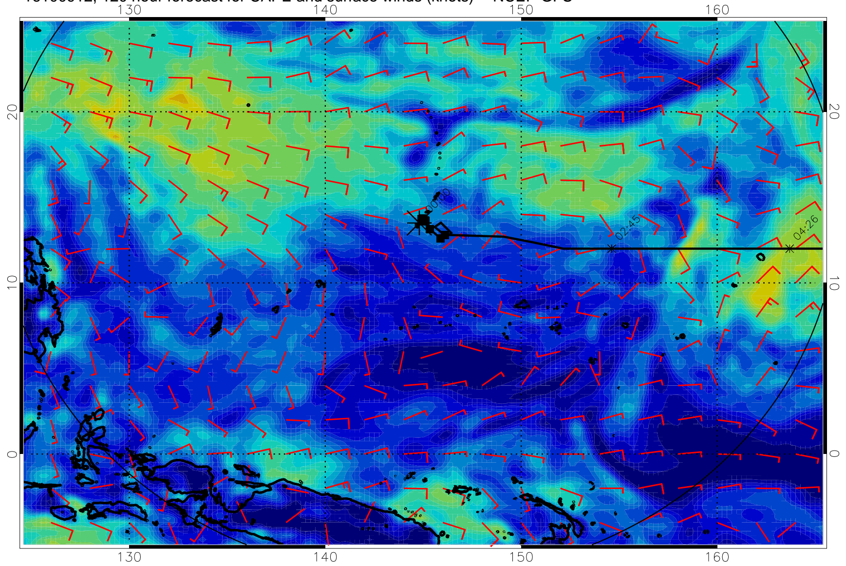
16100912, 120 hour forecast for CAPE and surface winds (knots) -- NCEP GFS
