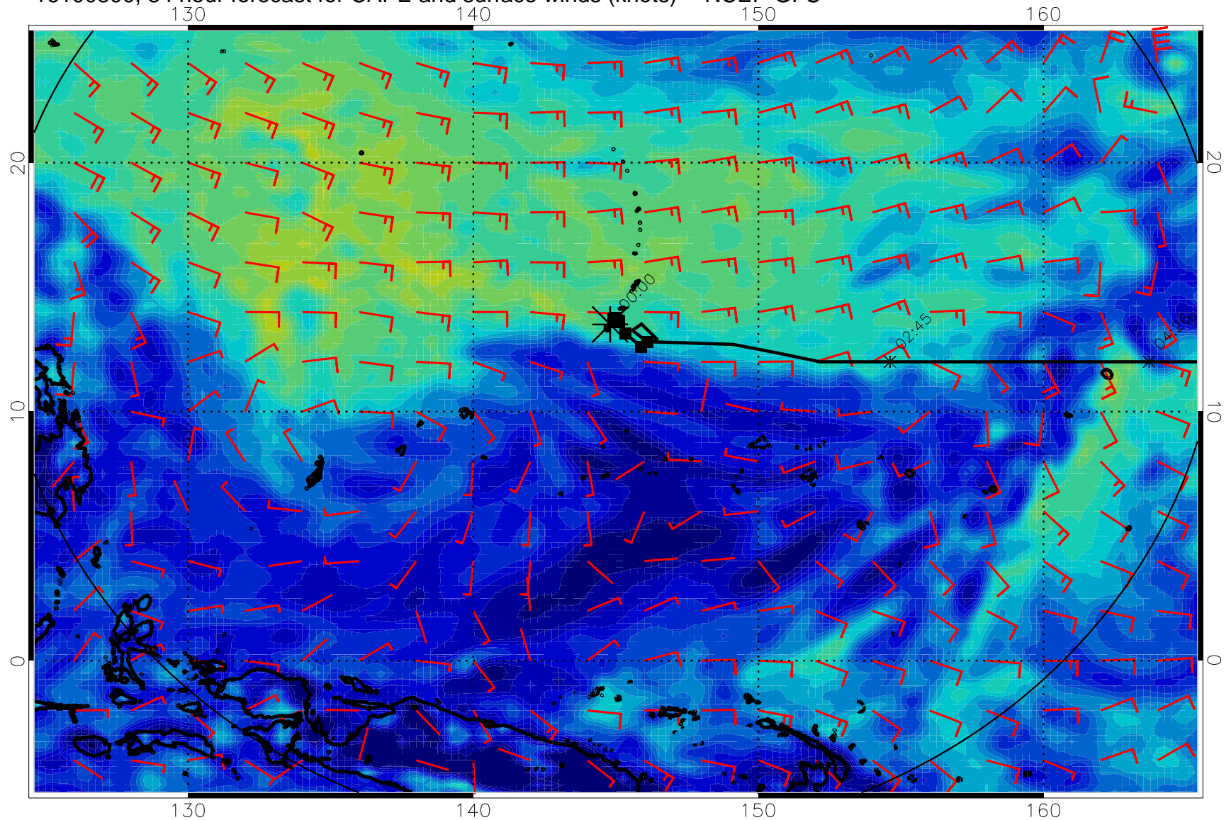
16100800, 84 hour forecast for CAPE and surface winds (knots) -- NCEP GFS
