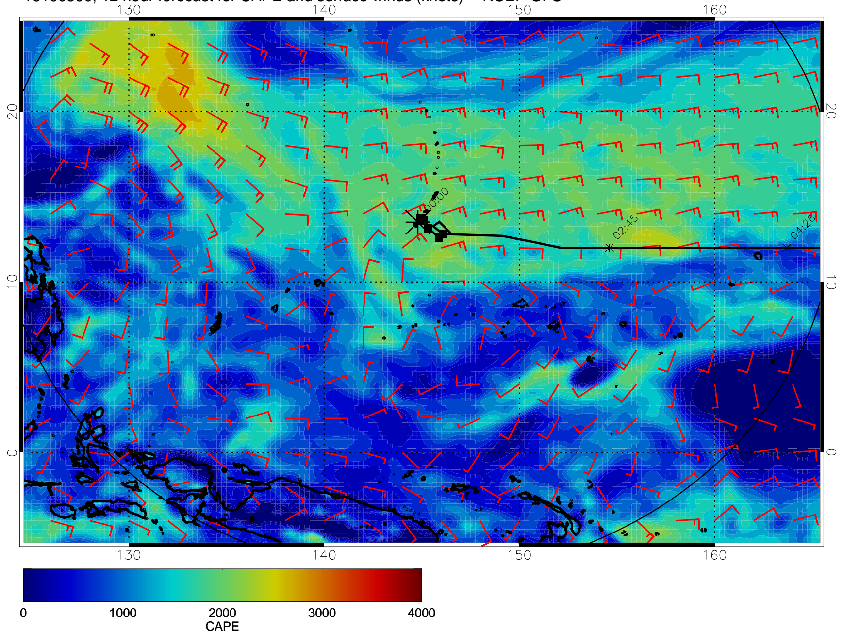
16100500, 12 hour forecast for CAPE and surface winds (knots) -- NCEP GFS
