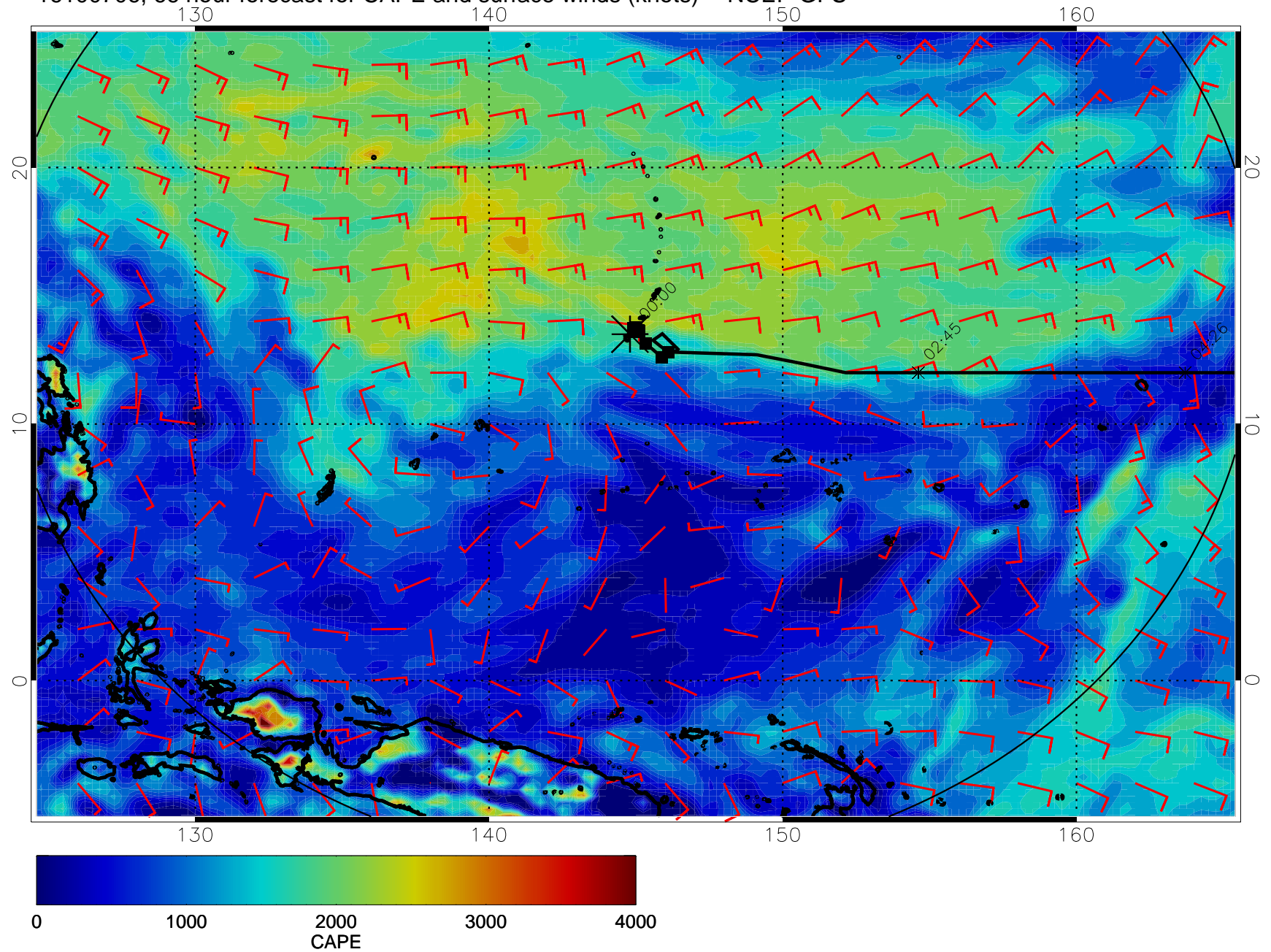
16100706, 66 hour forecast for CAPE and surface winds (knots) -- NCEP GFS
