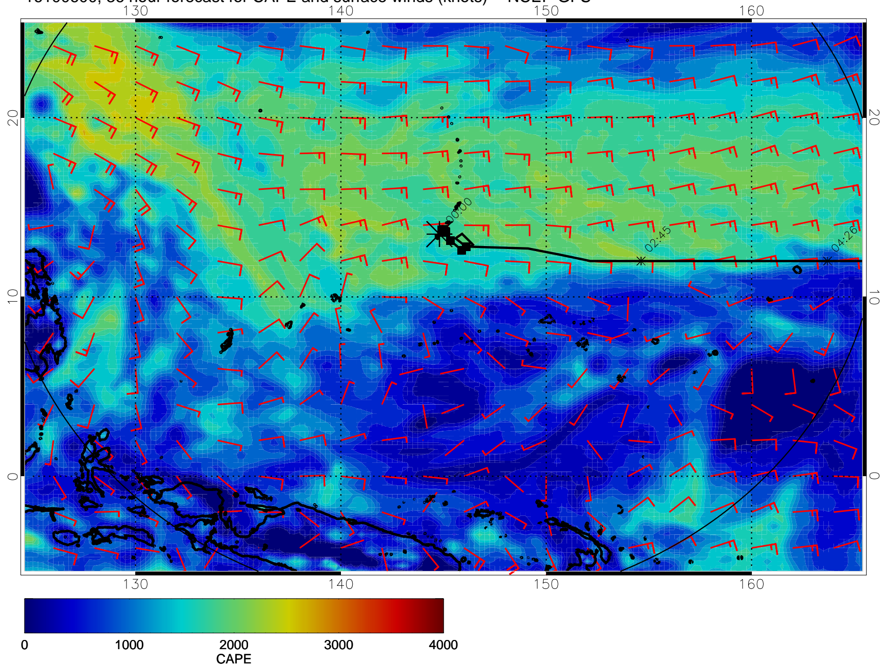
16100600, 36 hour forecast for CAPE and surface winds (knots) -- NCEP GFS
