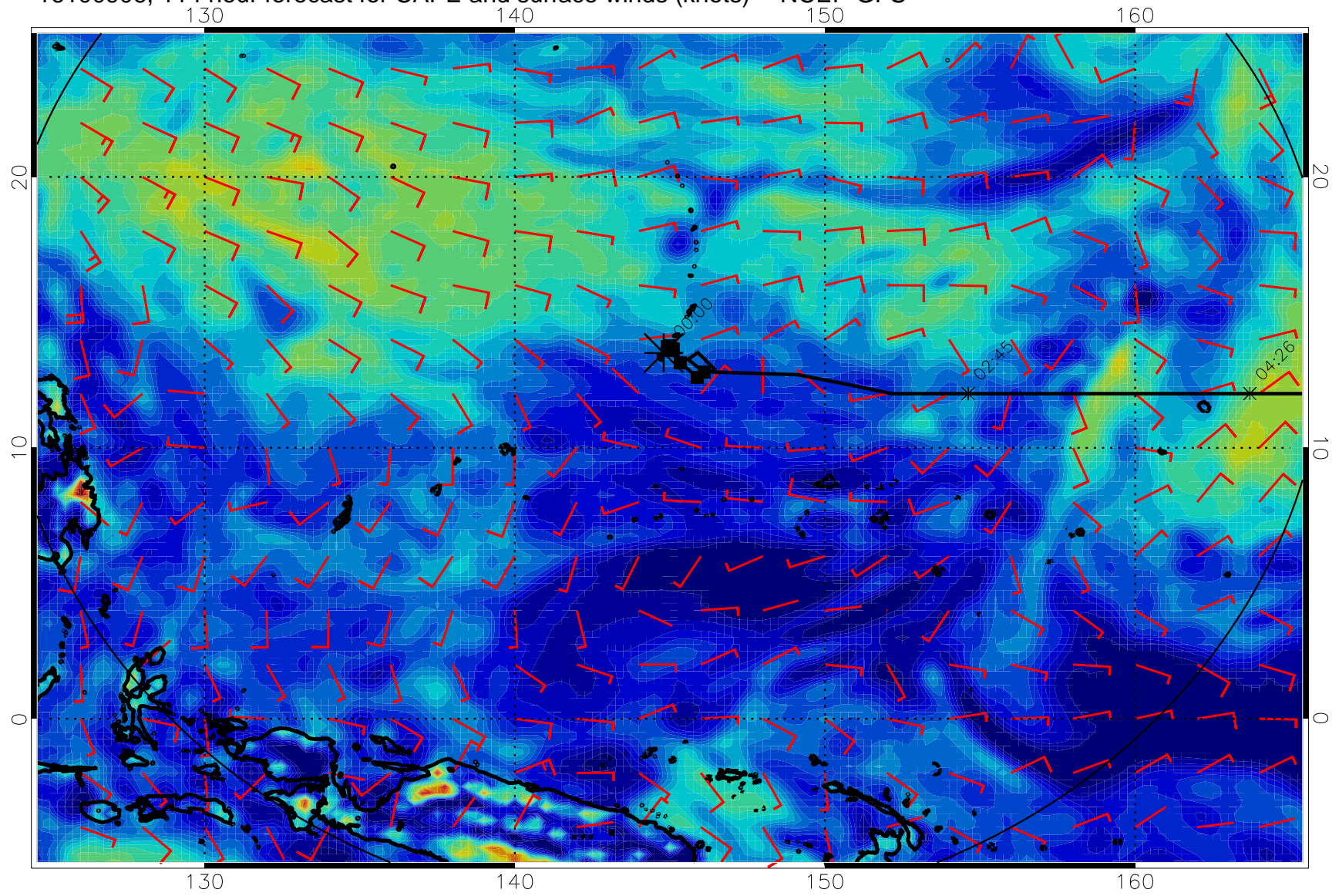
16100906, 114 hour forecast for CAPE and surface winds (knots) -- NCEP GFS
