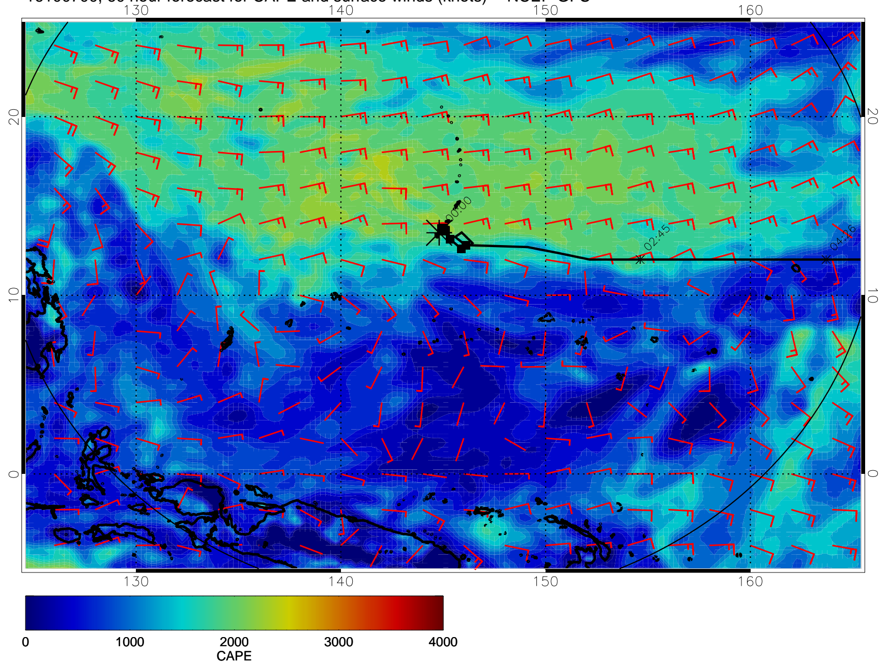
16100700, 60 hour forecast for CAPE and surface winds (knots) -- NCEP GFS
