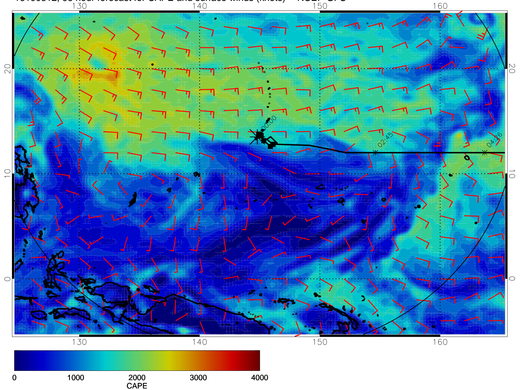
16100812, 96 hour forecast for CAPE and surface winds (knots) -- NCEP GFS
