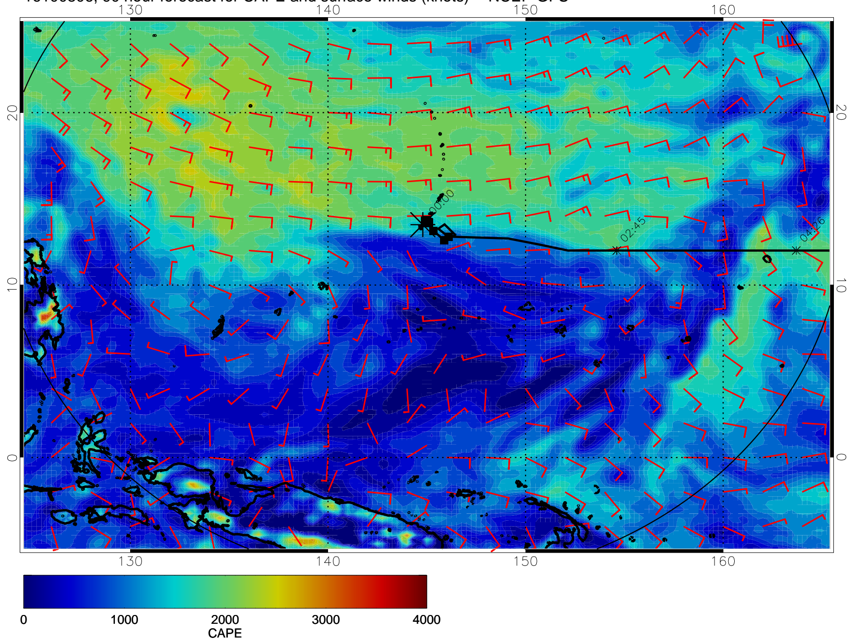
16100806, 90 hour forecast for CAPE and surface winds (knots) -- NCEP GFS
