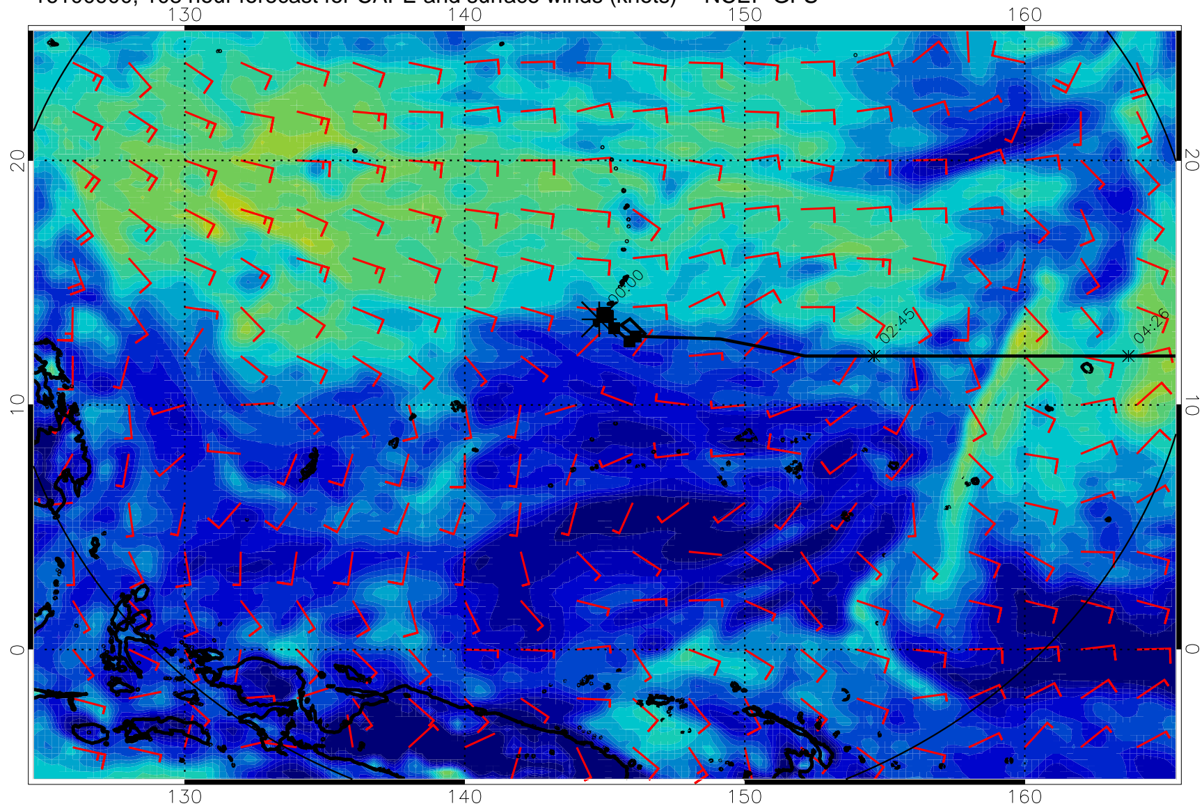
16100900, 108 hour forecast for CAPE and surface winds (knots) -- NCEP GFS
