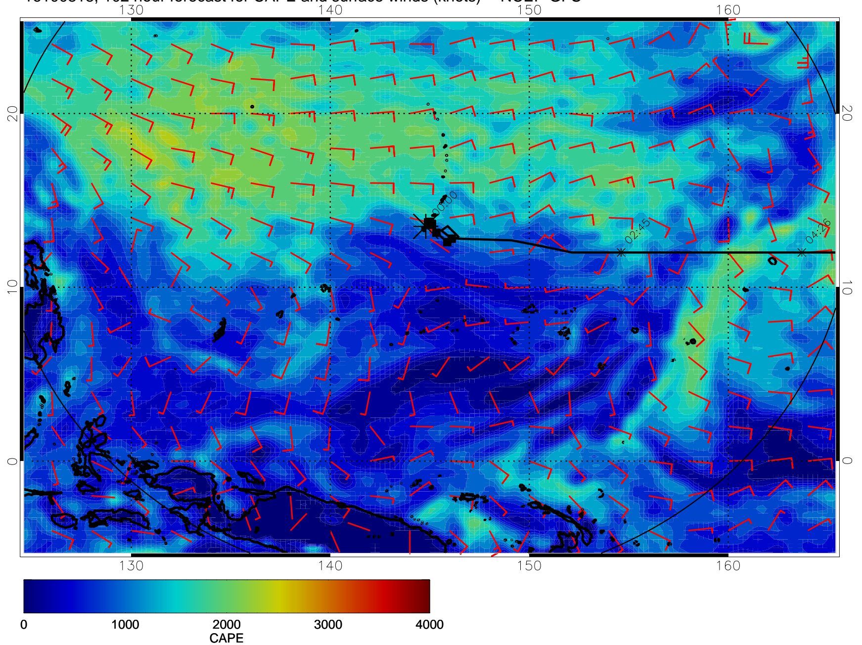
16100818, 102 hour forecast for CAPE and surface winds (knots) -- NCEP GFS
