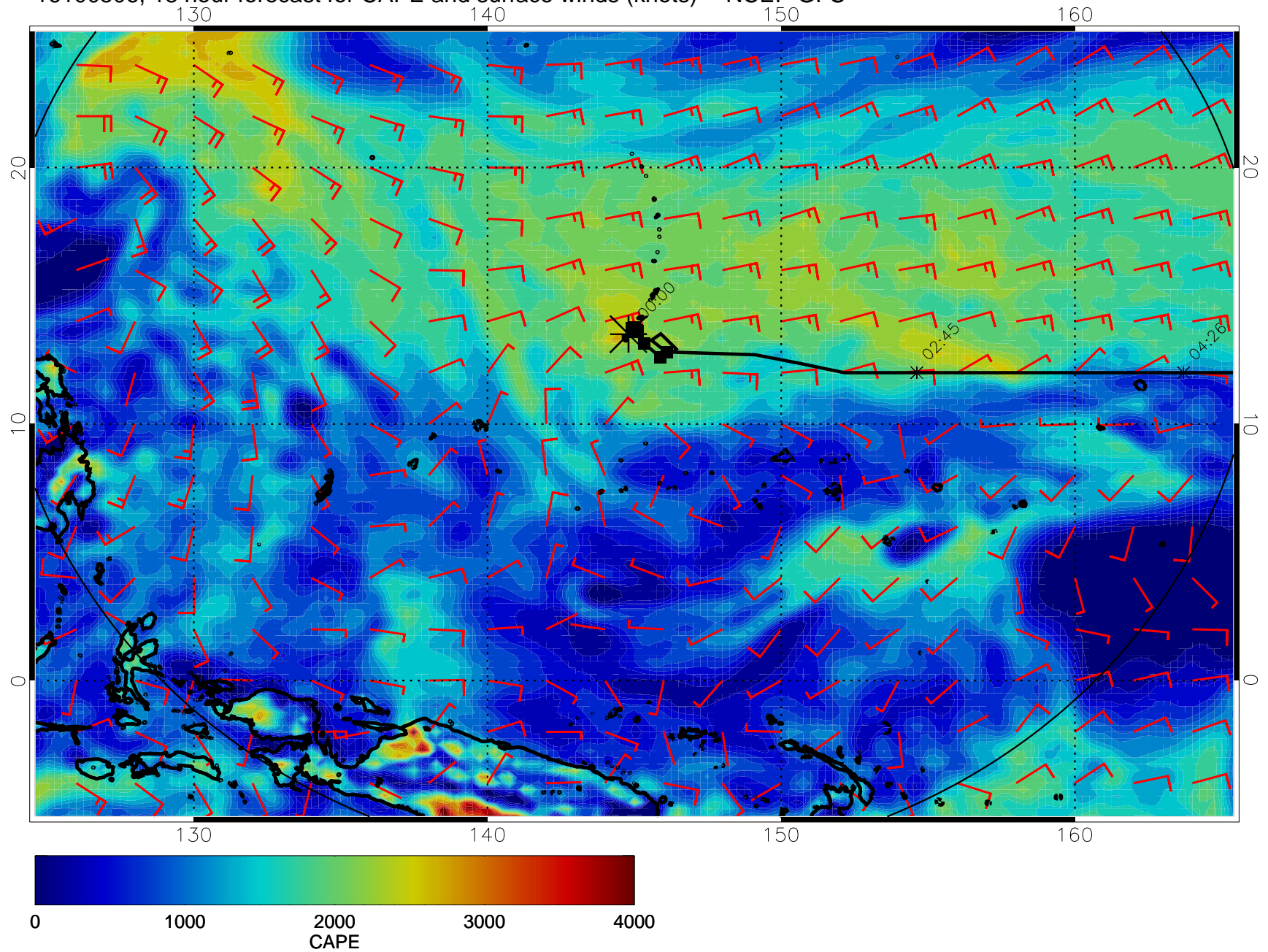
16100506, 18 hour forecast for CAPE and surface winds (knots) -- NCEP GFS
