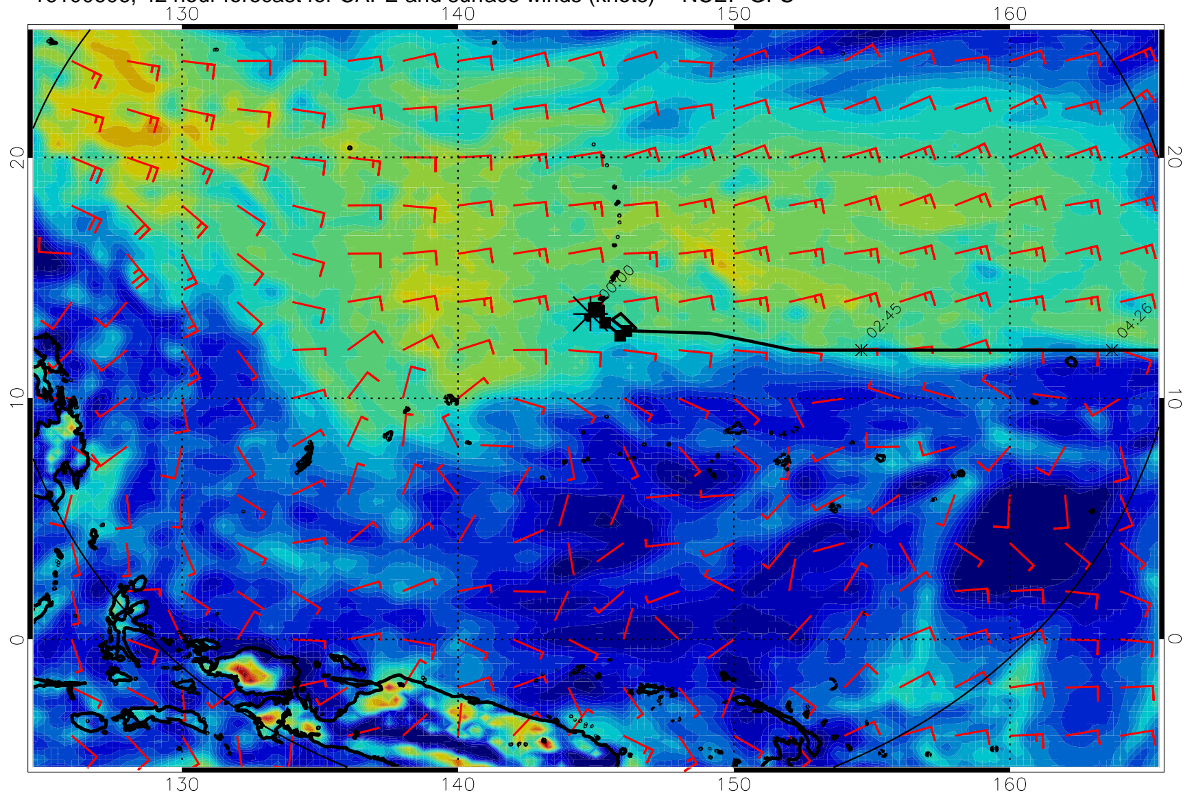
16100606, 42 hour forecast for CAPE and surface winds (knots) -- NCEP GFS
