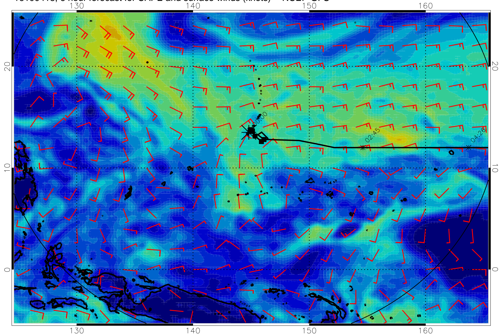
16100418, 6 hour forecast for CAPE and surface winds (knots) -- NCEP GFS
