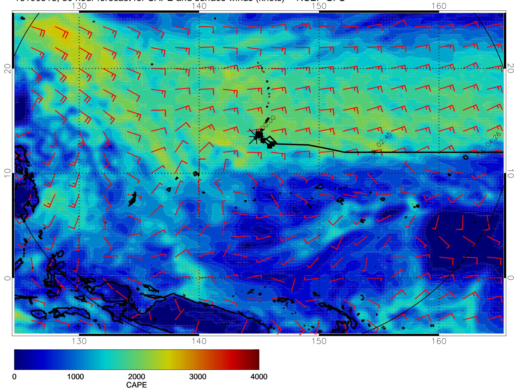
16100518, 30 hour forecast for CAPE and surface winds (knots) -- NCEP GFS
