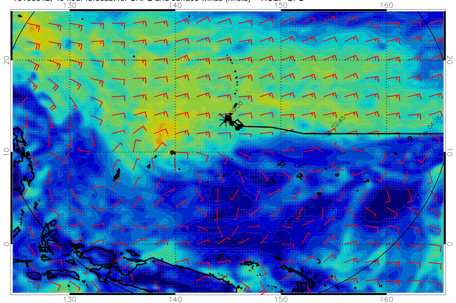
16100612, 48 hour forecast for CAPE and surface winds (knots) -- NCEP GFS
