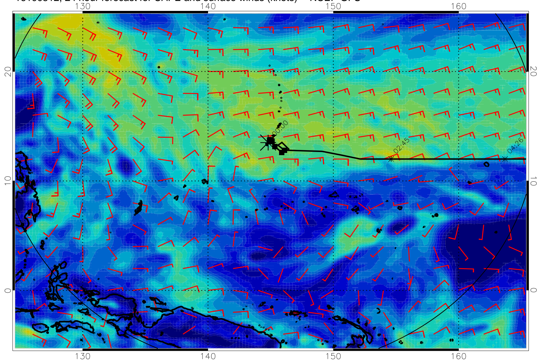
16100512, 24 hour forecast for CAPE and surface winds (knots) -- NCEP GFS
