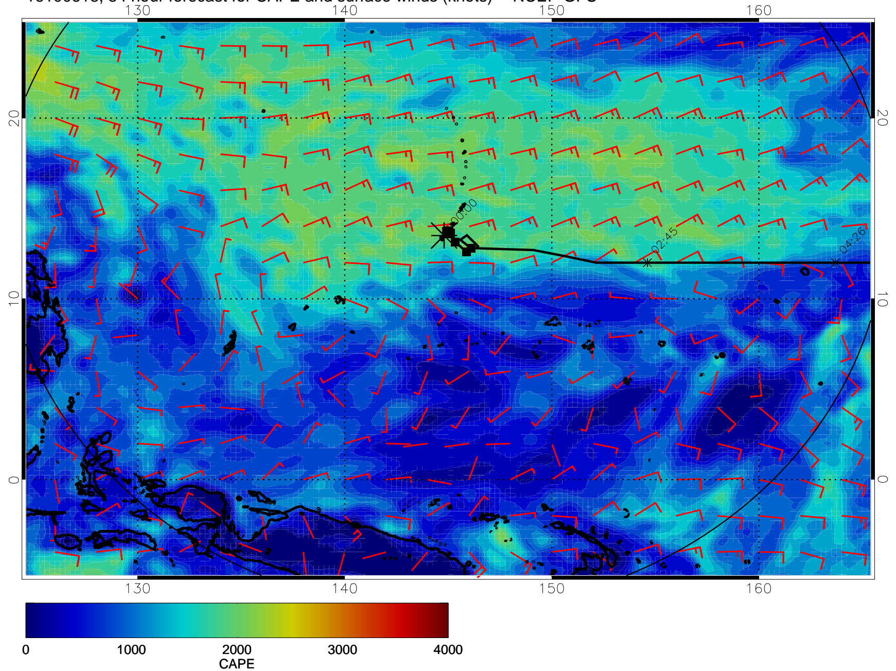
16100618, 54 hour forecast for CAPE and surface winds (knots) -- NCEP GFS
