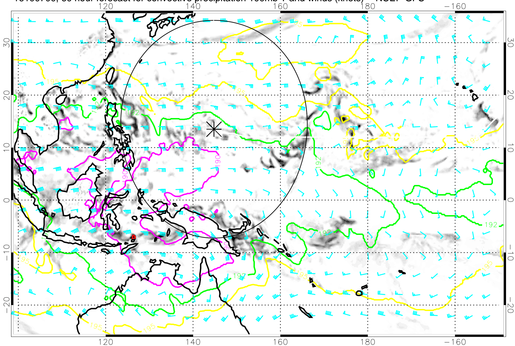
16100700, 60 hour forecast for convective precipitation 100mb T and winds (knots) -- NCEP GFS
