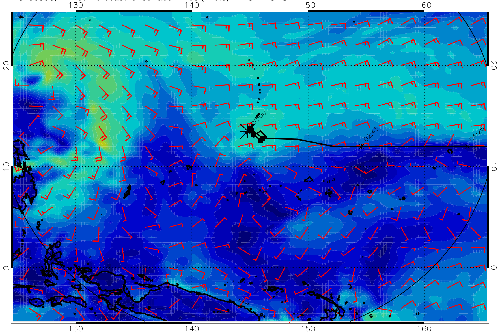
16100506, 24 hour forecast for surface winds (knots) -- NCEP GFS
