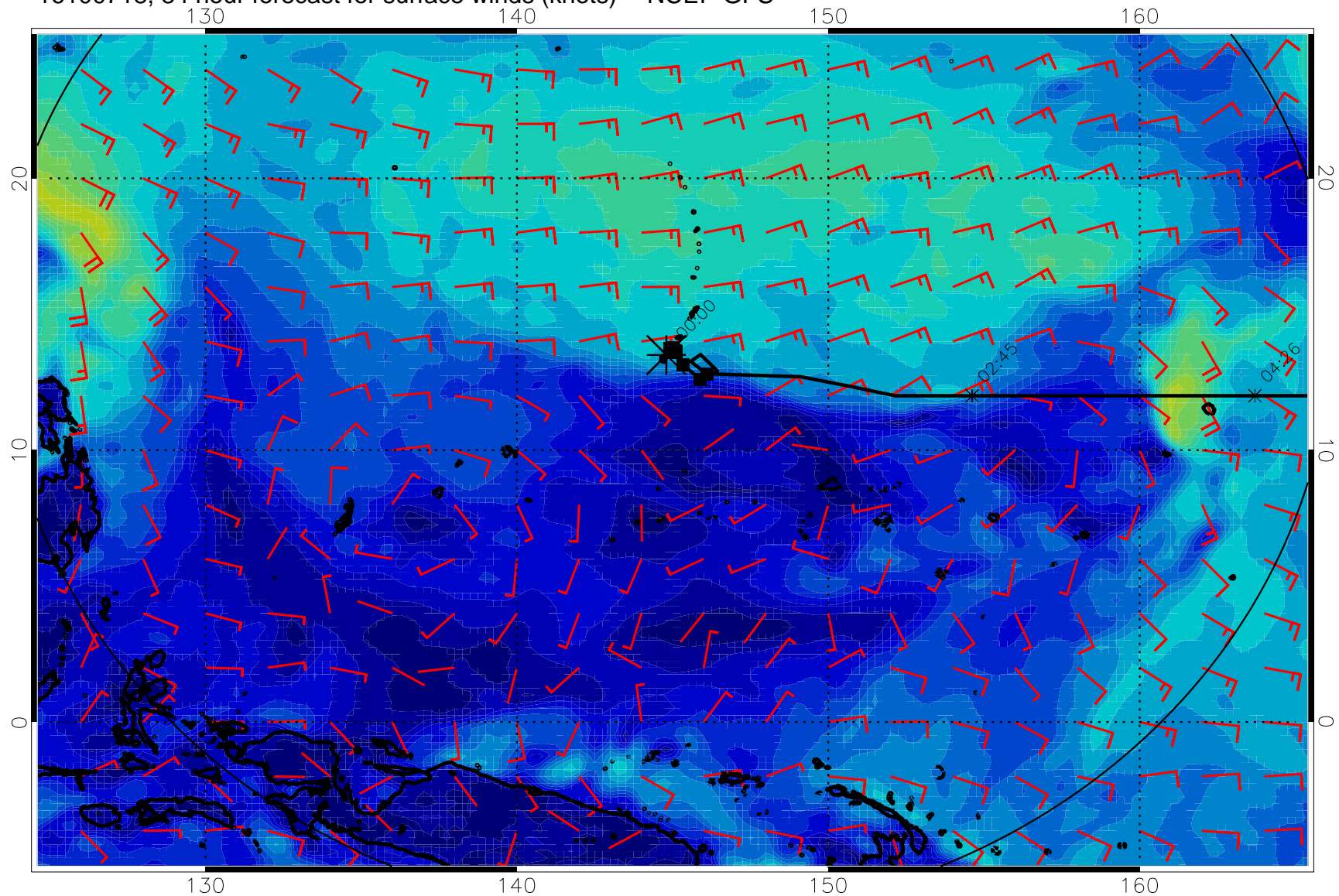
16100718, 84 hour forecast for surface winds (knots) -- NCEP GFS
