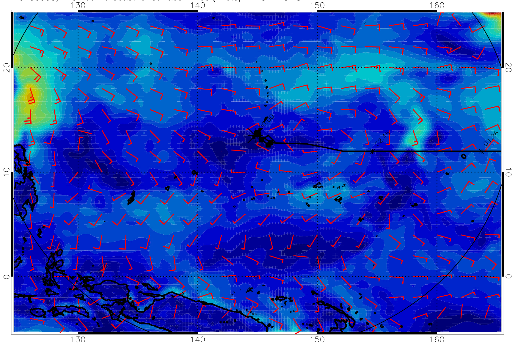
16100906, 120 hour forecast for surface winds (knots) -- NCEP GFS
