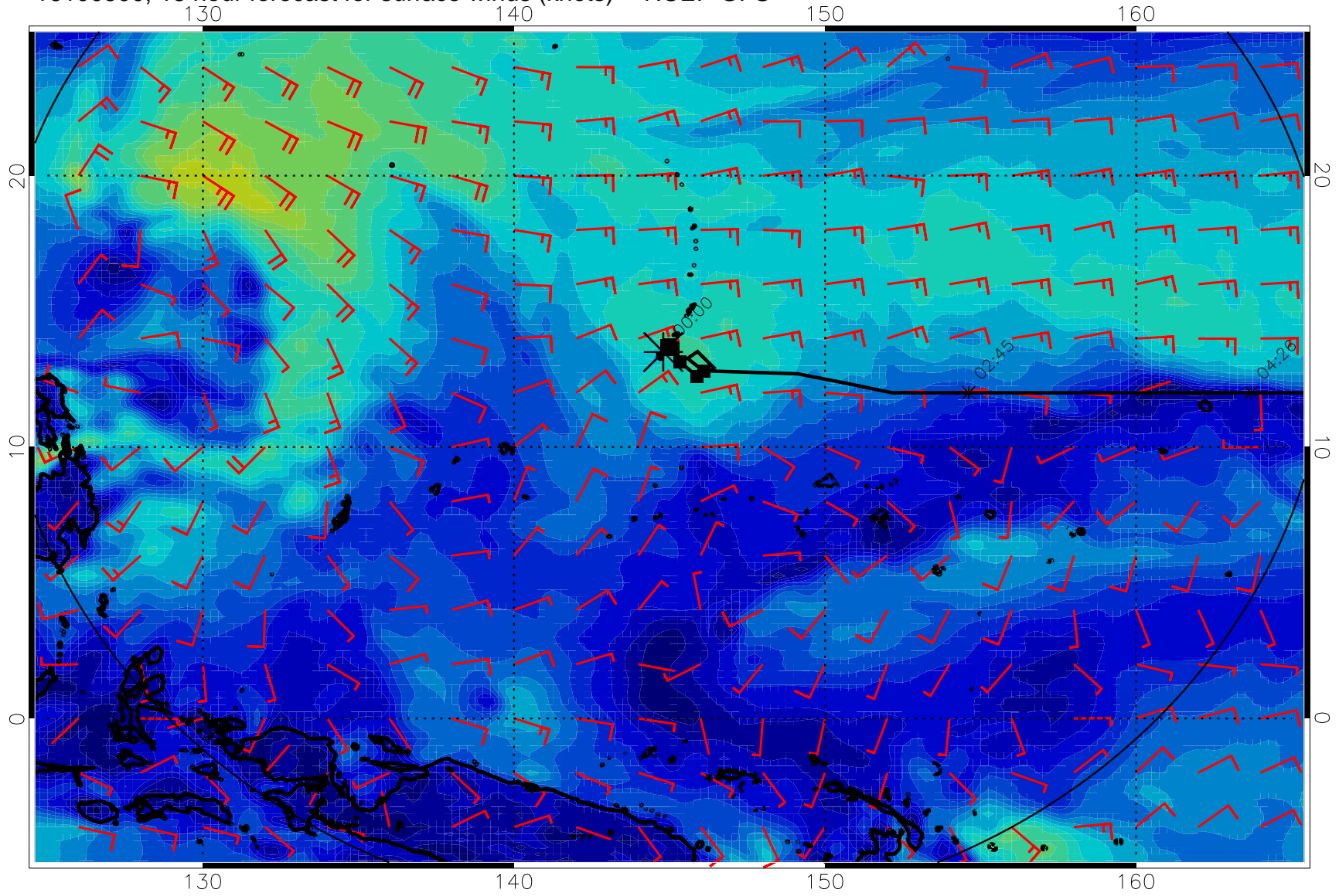
16100500, 18 hour forecast for surface winds (knots) -- NCEP GFS
