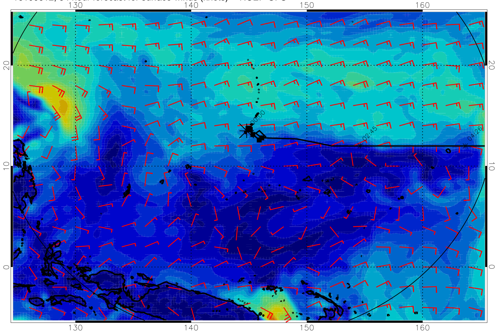
16100612, 54 hour forecast for surface winds (knots) -- NCEP GFS
