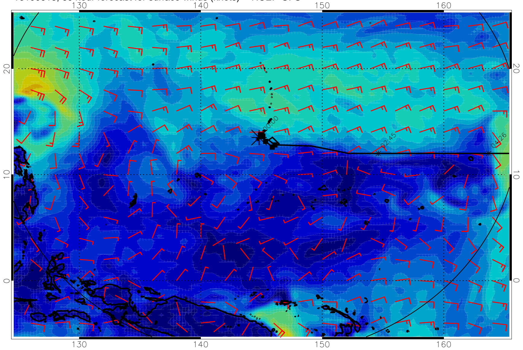
16100618, 60 hour forecast for surface winds (knots) -- NCEP GFS
