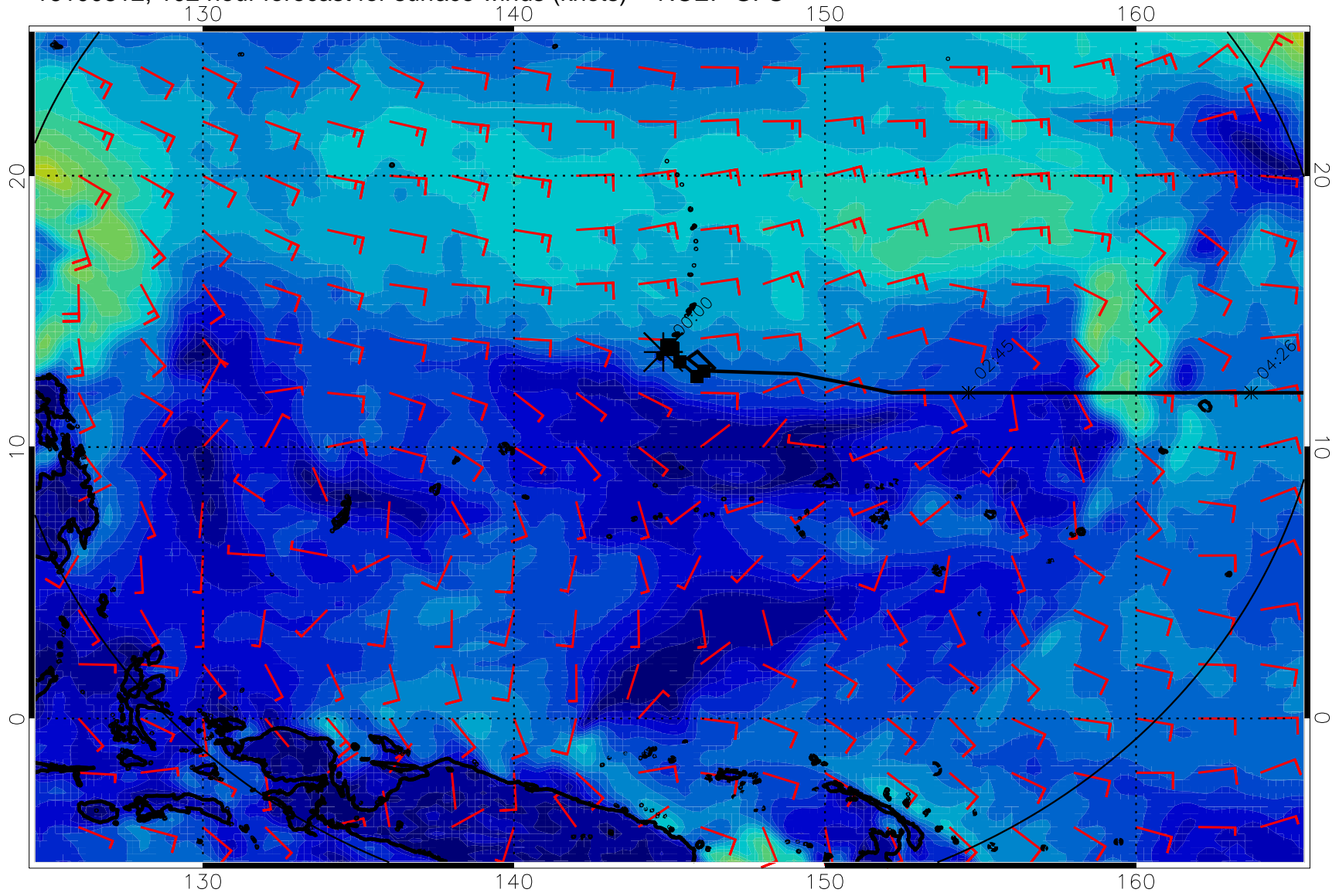
16100812, 102 hour forecast for surface winds (knots) -- NCEP GFS
