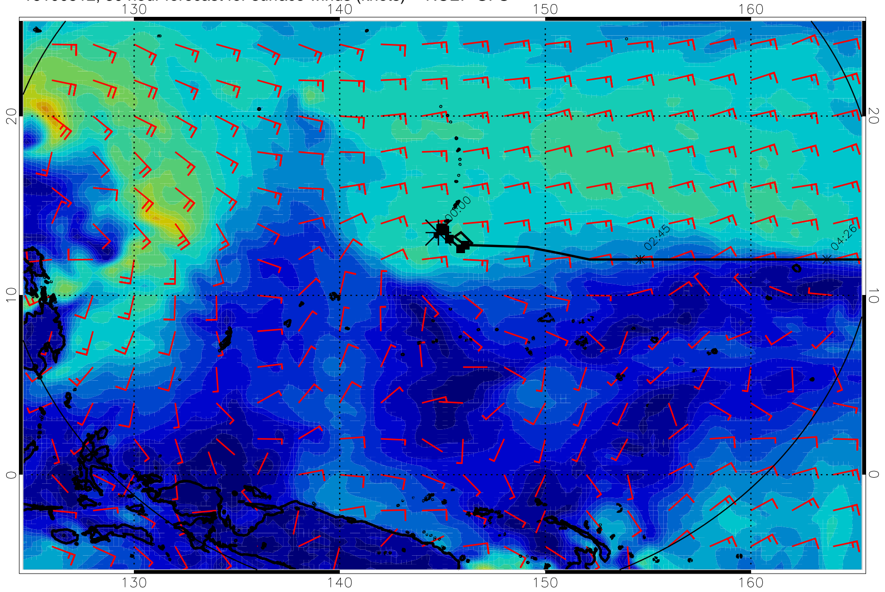
16100512, 30 hour forecast for surface winds (knots) -- NCEP GFS
