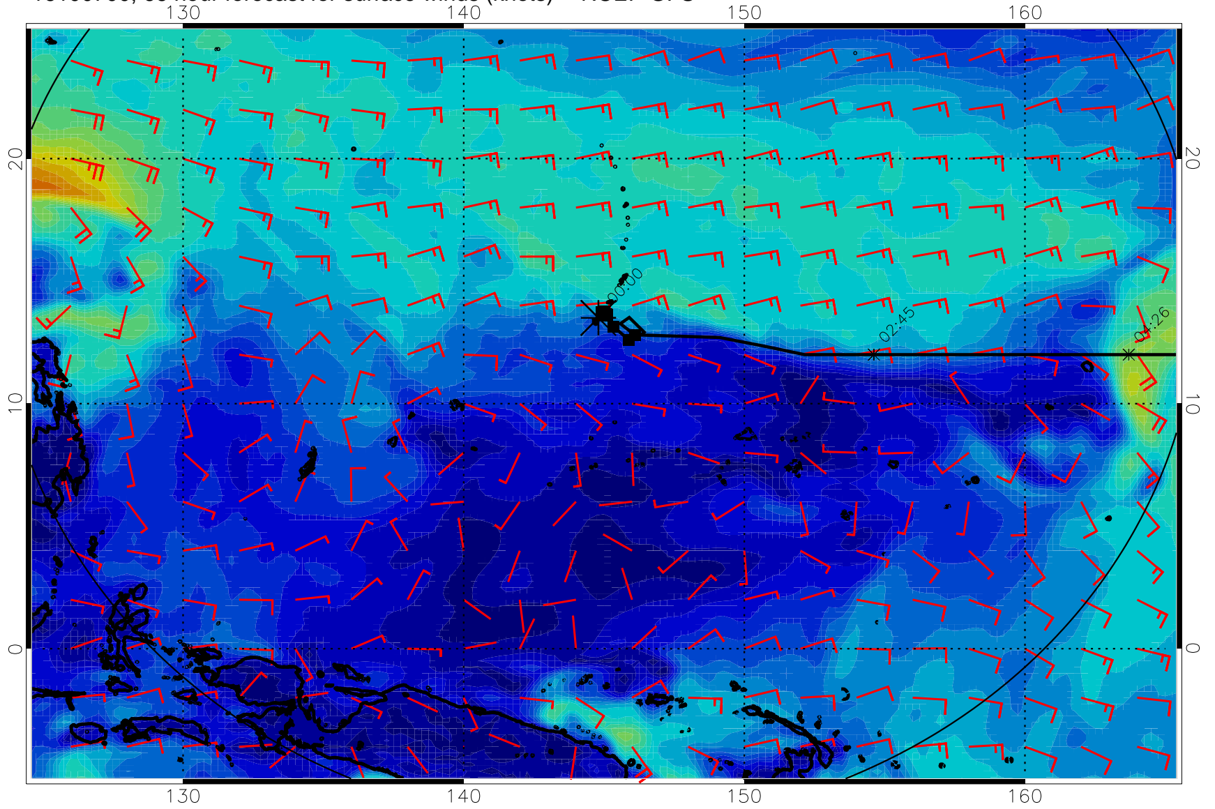
16100700, 66 hour forecast for surface winds (knots) -- NCEP GFS
