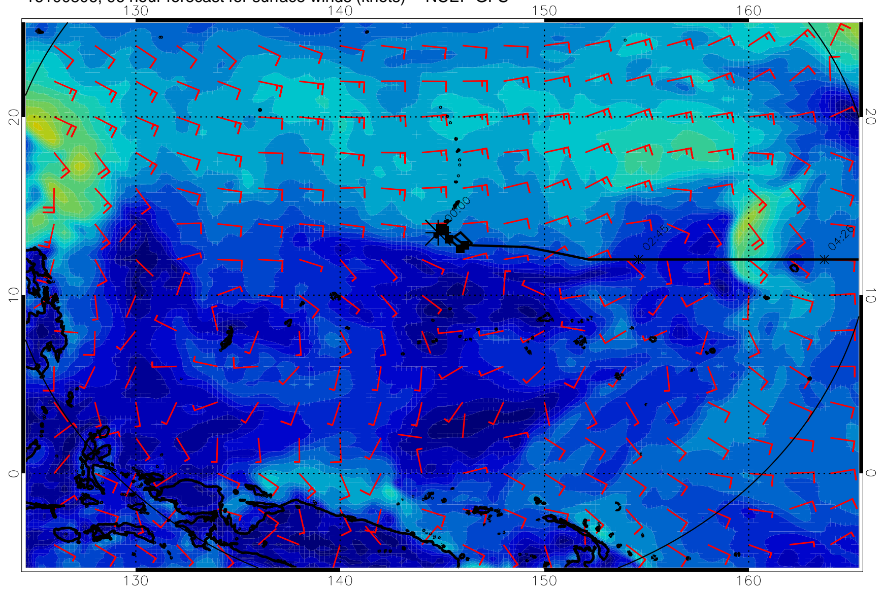
16100806, 96 hour forecast for surface winds (knots) -- NCEP GFS
