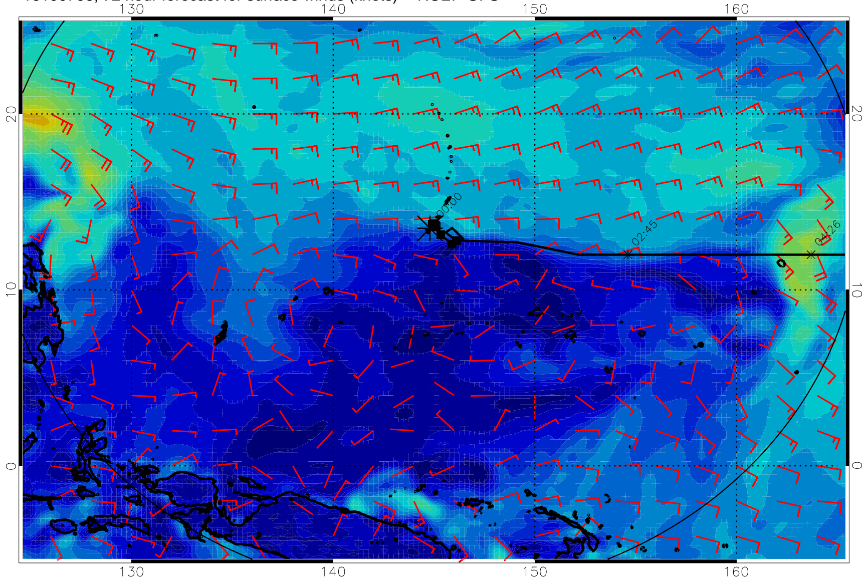
16100706, 72 hour forecast for surface winds (knots) -- NCEP GFS
