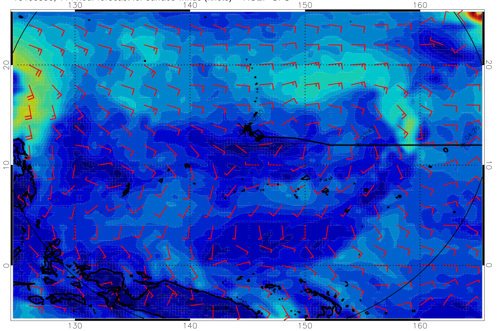
16100900, 114 hour forecast for surface winds (knots) -- NCEP GFS
