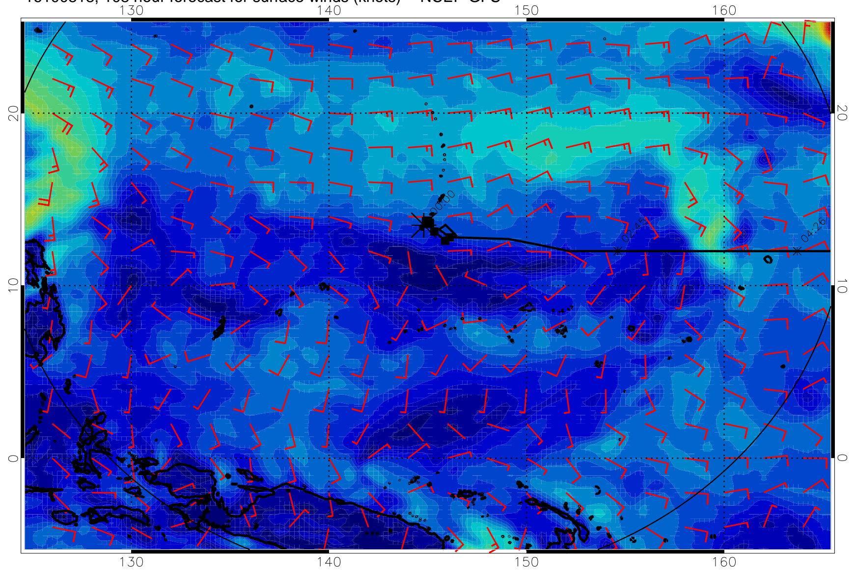
16100818, 108 hour forecast for surface winds (knots) -- NCEP GFS
