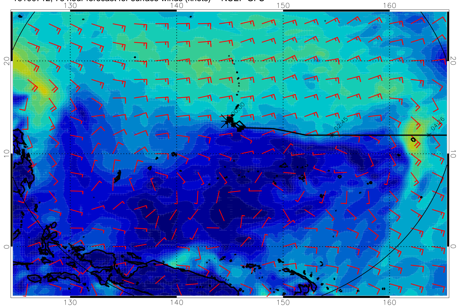
16100712, 78 hour forecast for surface winds (knots) -- NCEP GFS
