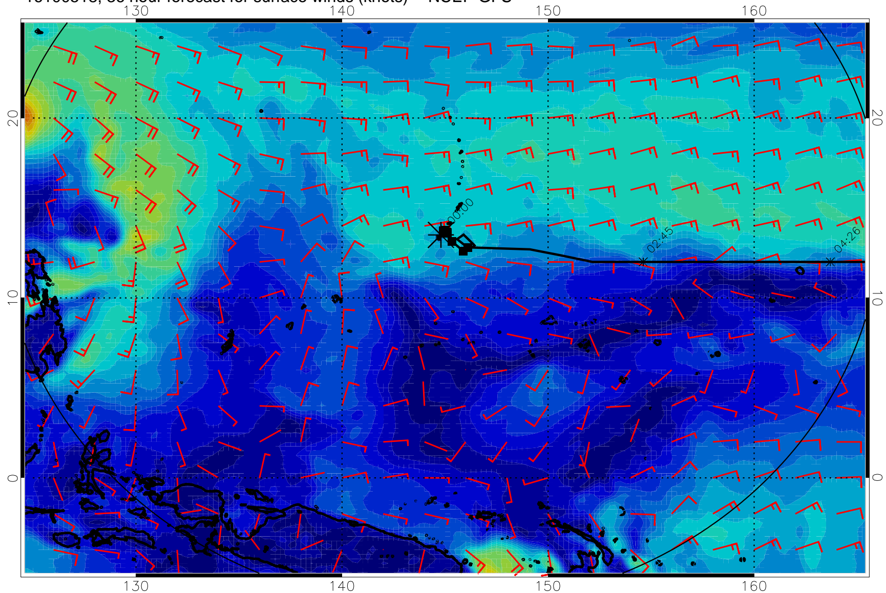
16100518, 36 hour forecast for surface winds (knots) -- NCEP GFS
