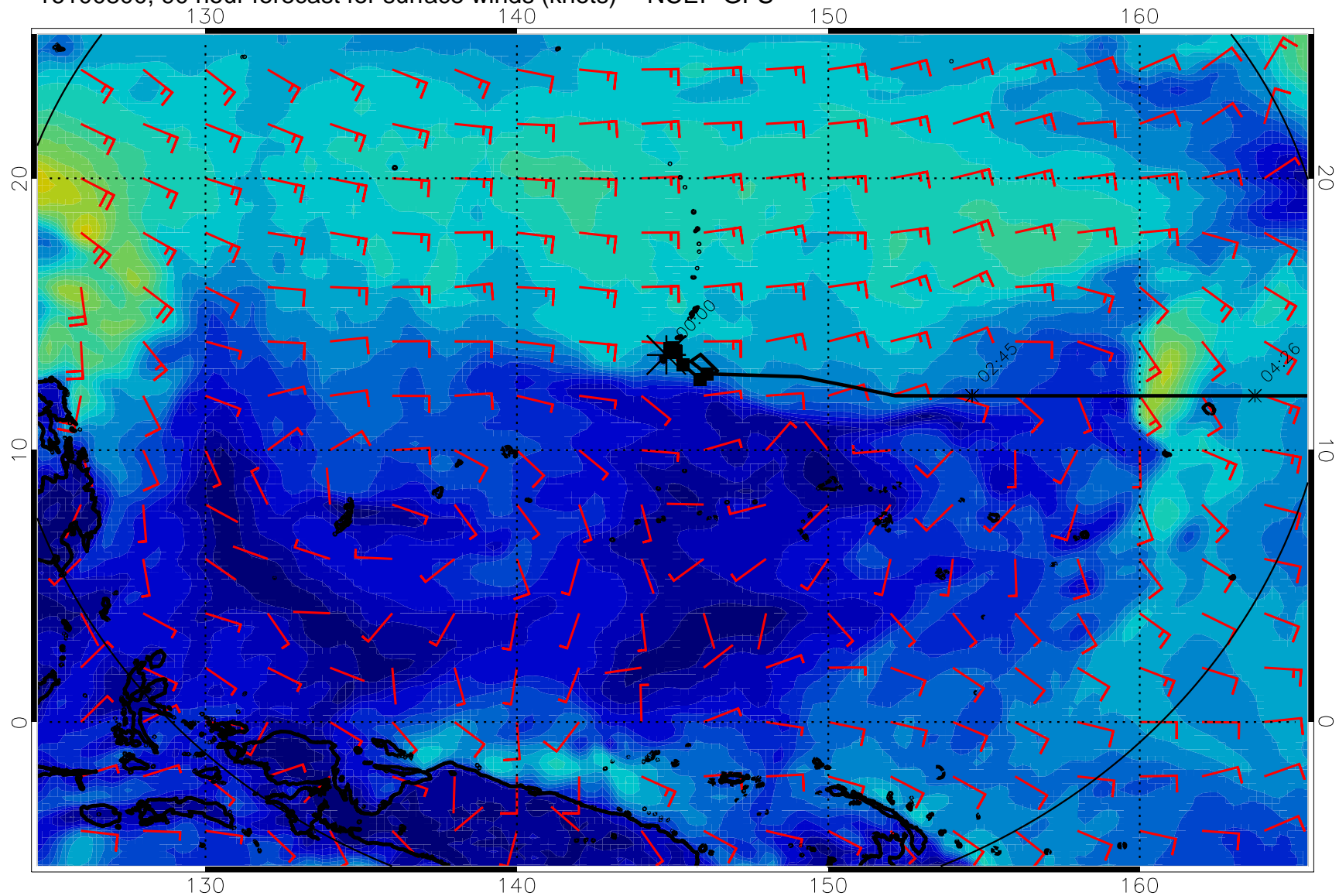
161100800, 90 hour forecast for surface winds (knots) -- NCEP GFS
