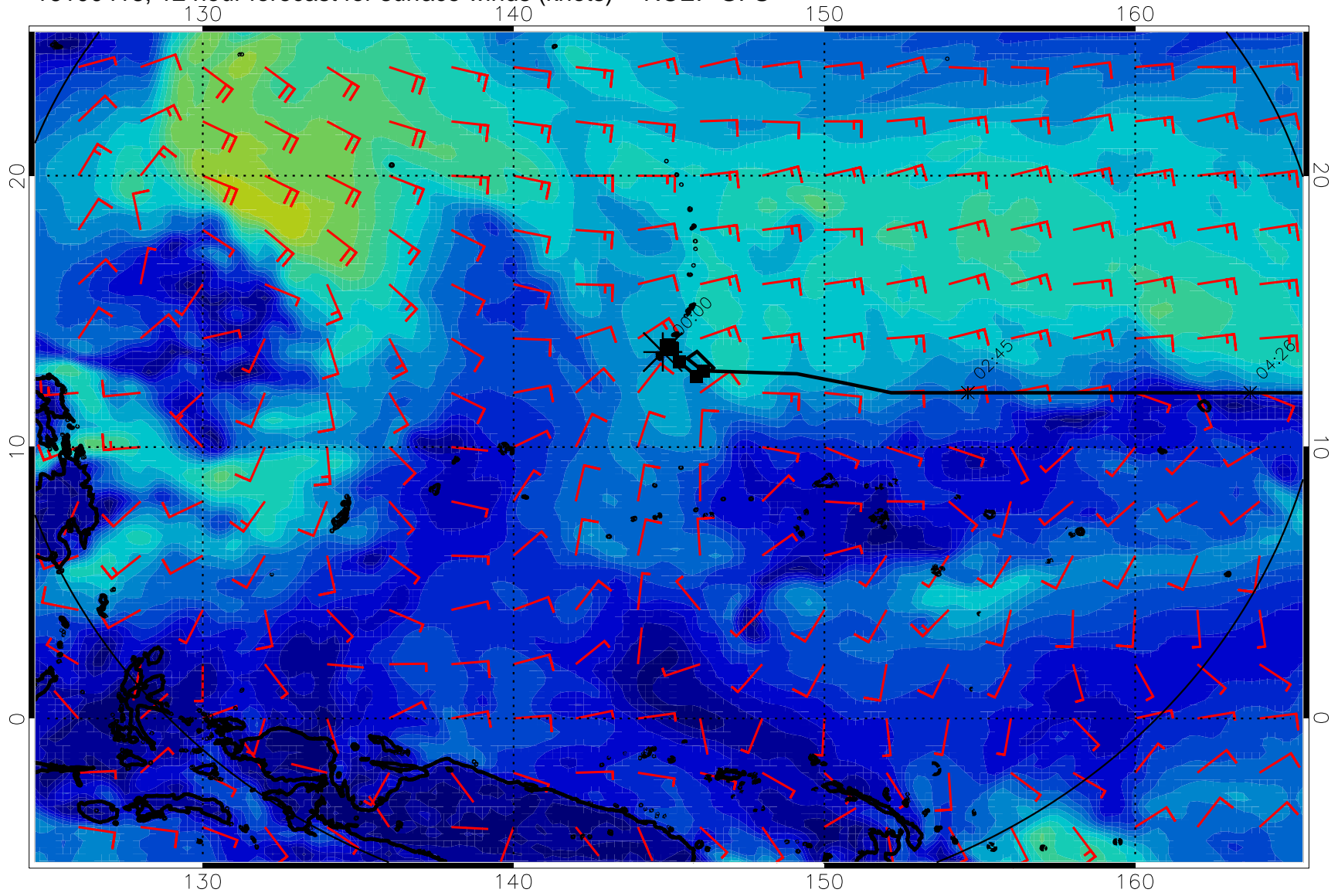
16100418, 12 hour forecast for surface winds (knots) -- NCEP GFS
