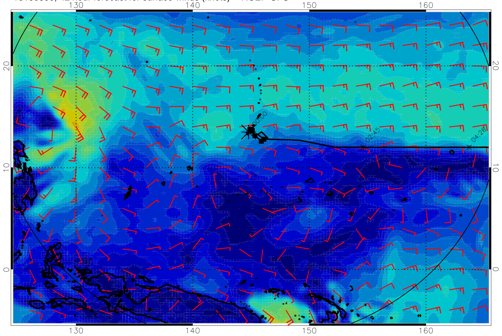
16100600, 42 hour forecast for surface winds (knots) -- NCEP GFS
