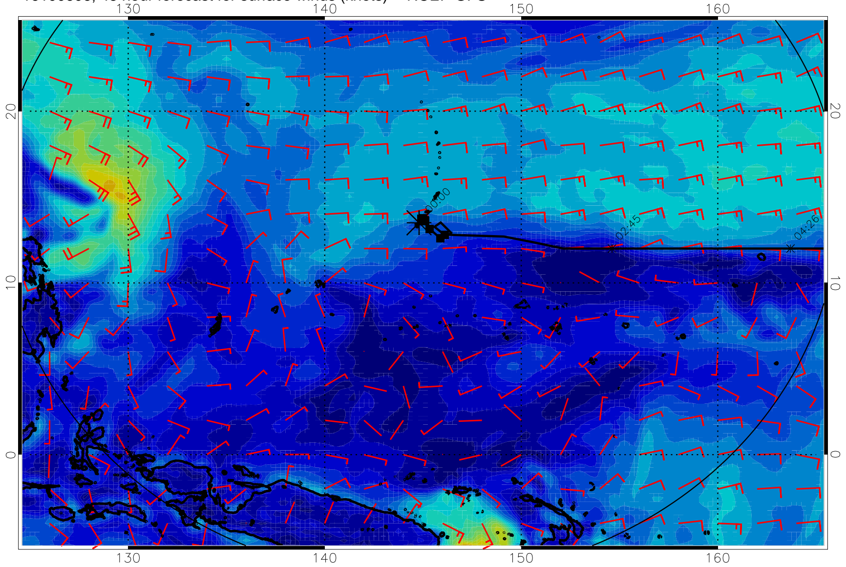
16100606, 48 hour forecast for surface winds (knots) -- NCEP GFS
