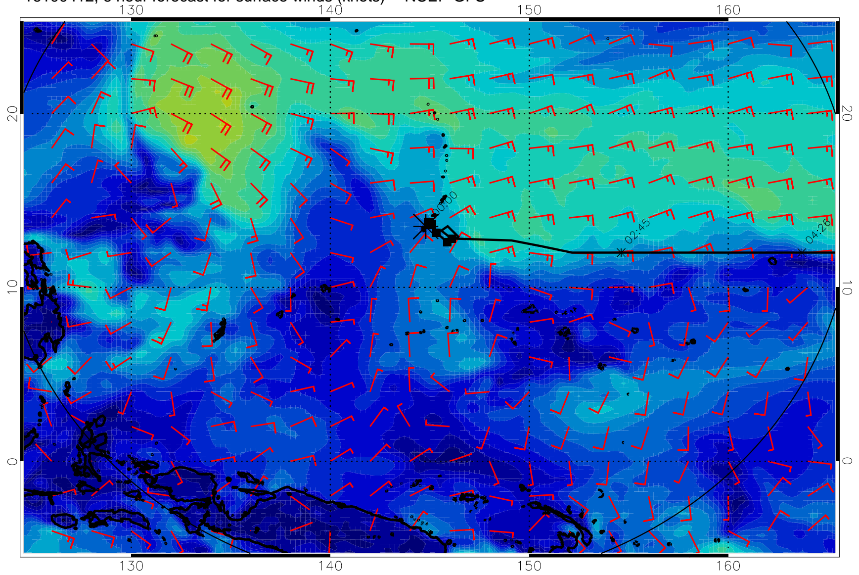
16100412, 6 hour forecast for surface winds (knots) -- NCEP GFS
