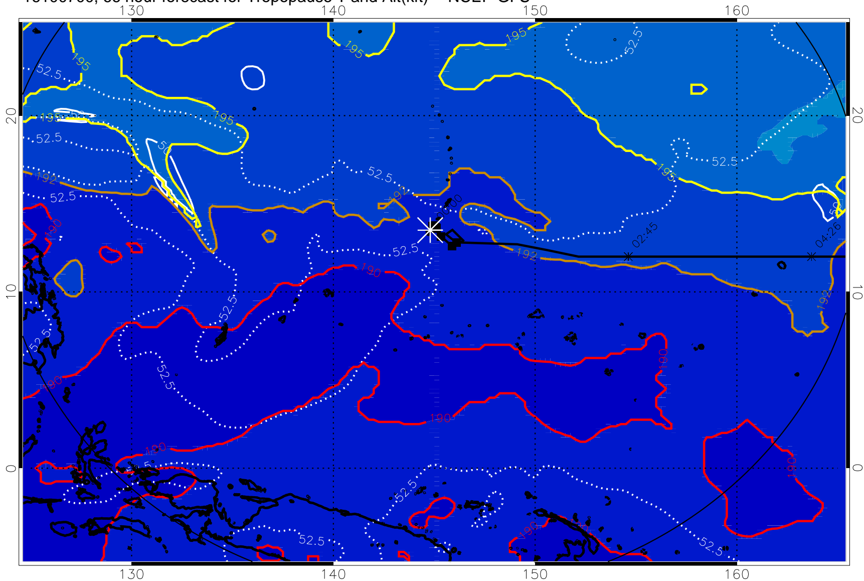
16100700, 66 hour forecast for Tropopause T and Alt(kft) -- NCEP GFS
