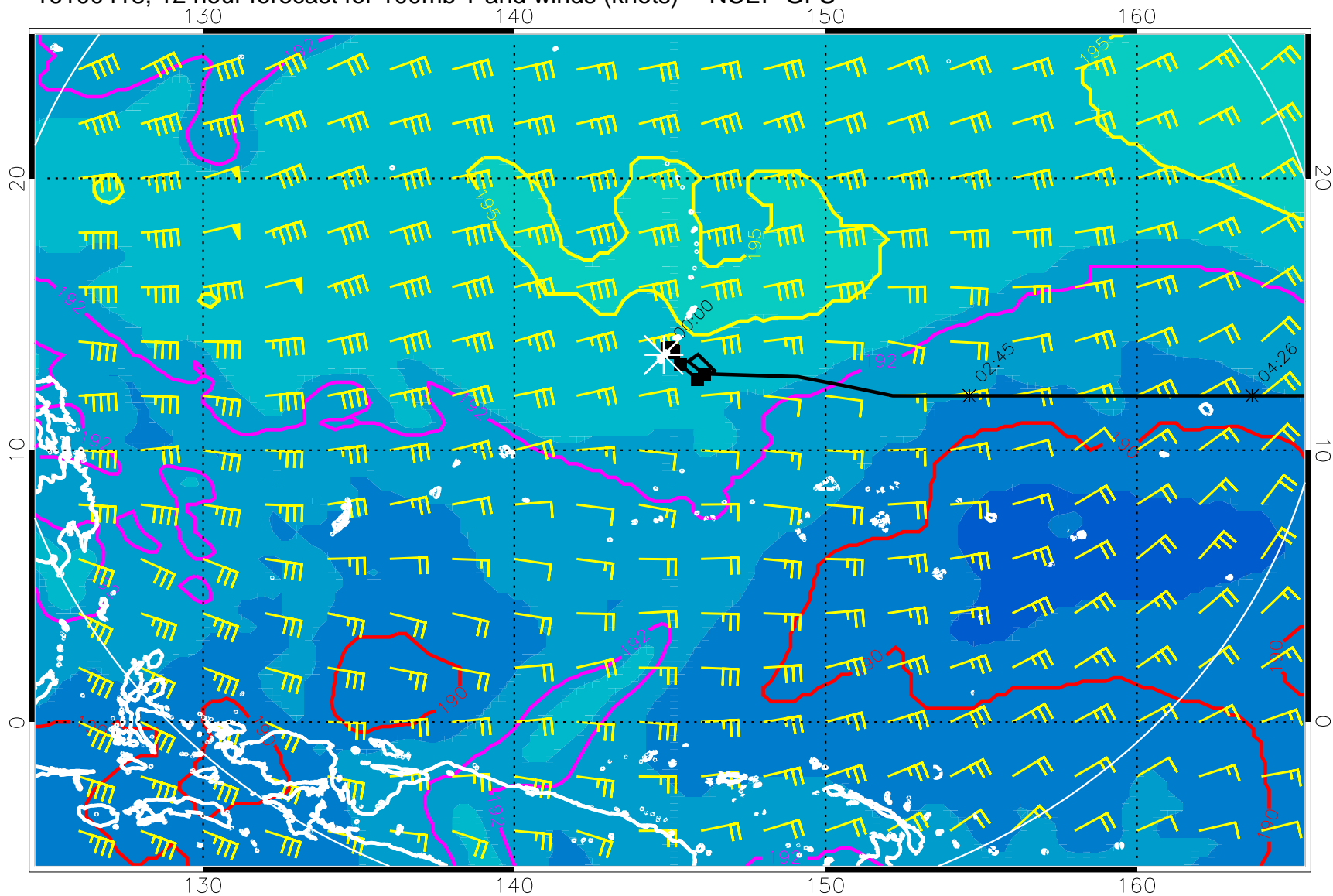
16100418, 12 hour forecast for 100mb T and winds (knots) -- NCEP GFS
