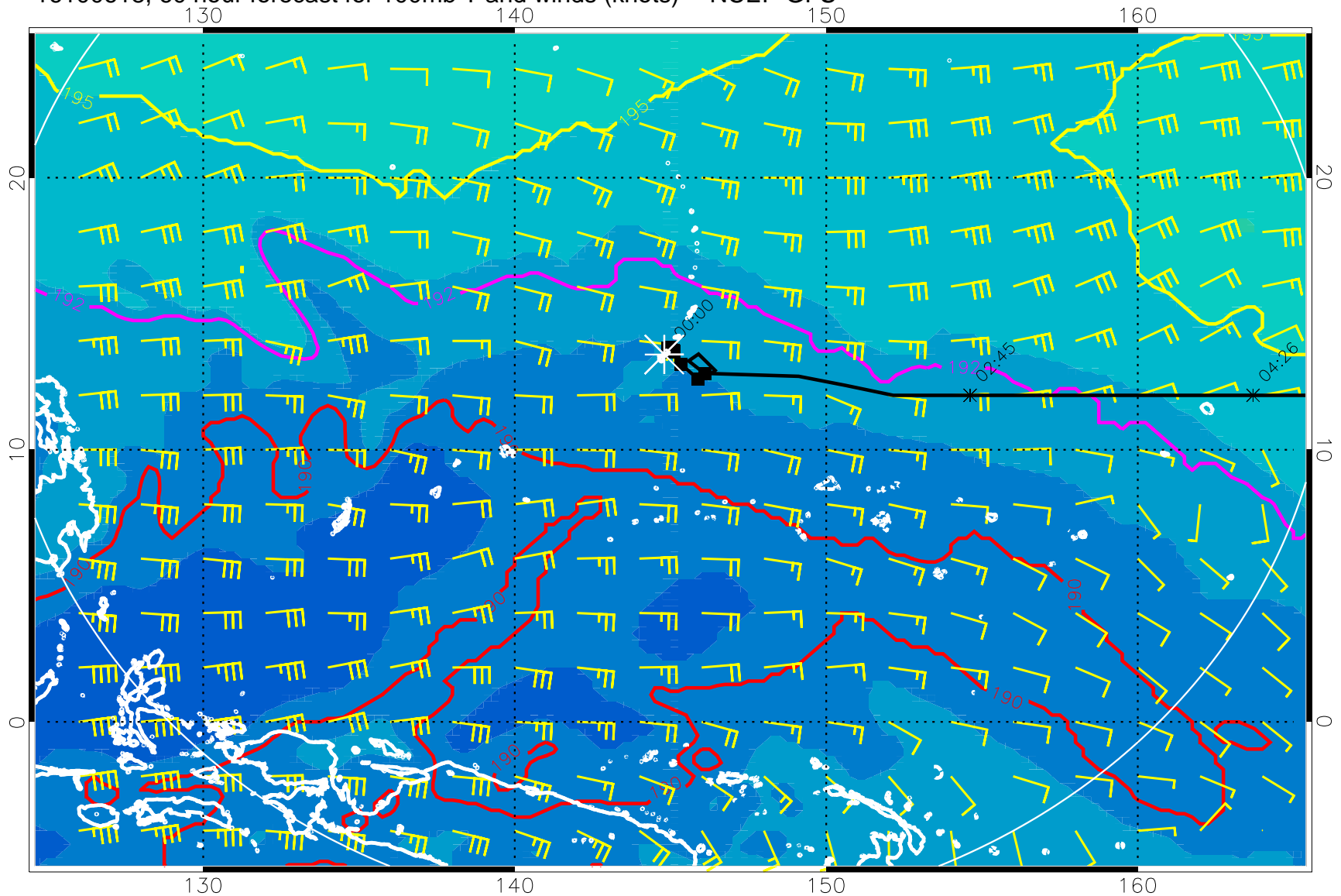
16100618, 60 hour forecast for 100mb T and winds (knots) -- NCEP GFS
