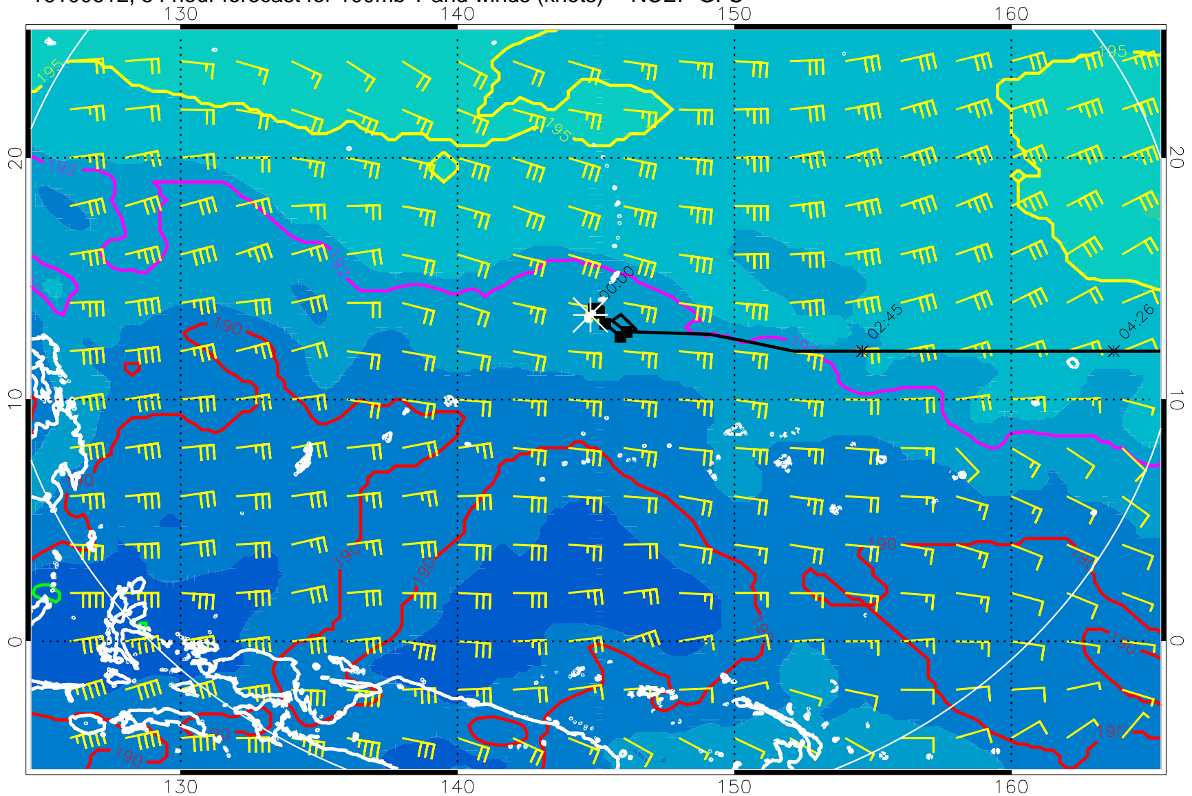
16100612, 54 hour forecast for 100mb T and winds (knots) -- NCEP GFS
