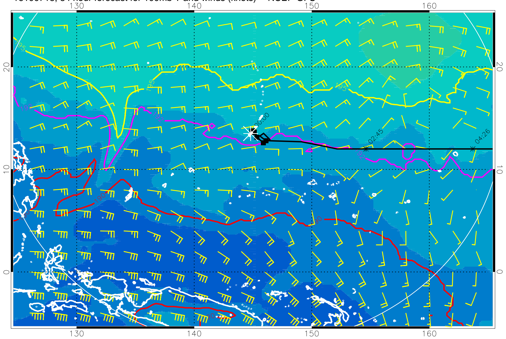
16100718, 84 hour forecast for 100mb T and winds (knots) -- NCEP GFS
