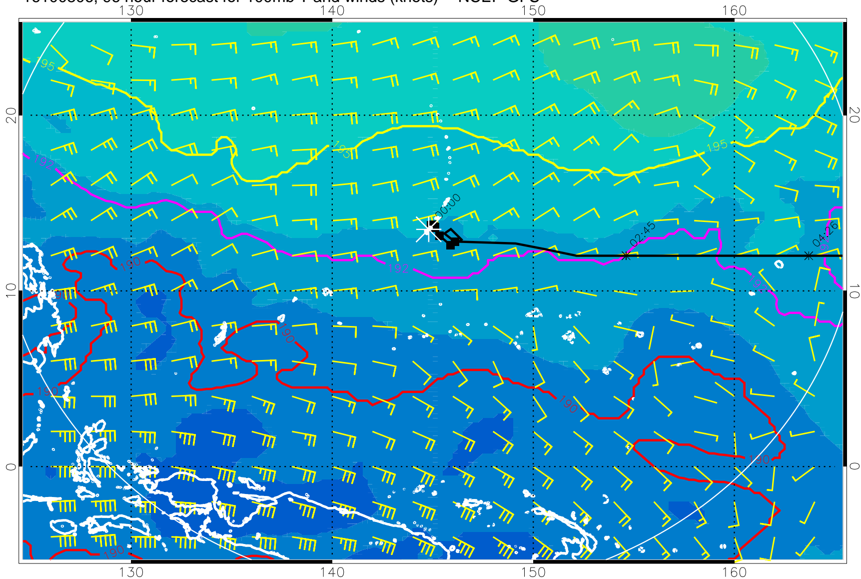
16100806, 96 hour forecast for 100mb T and winds (knots) -- NCEP GFS
