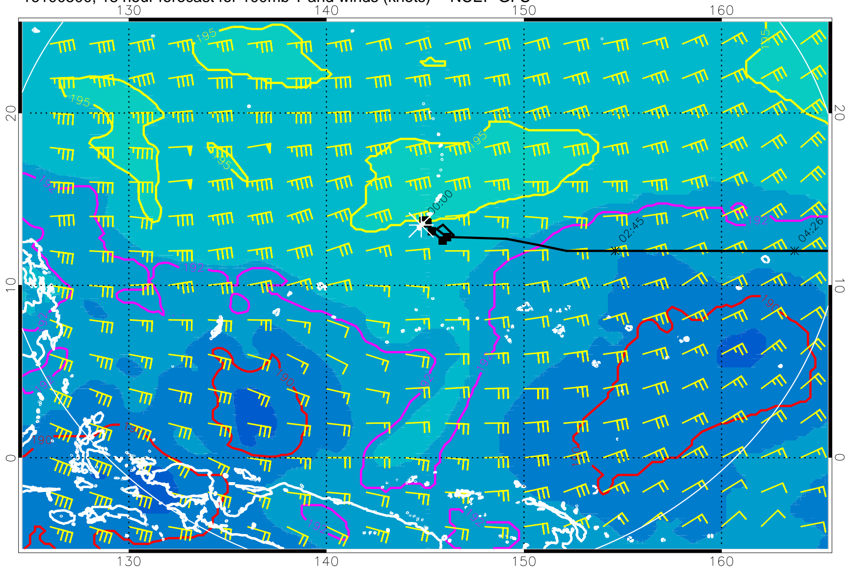
16100500, 18 hour forecast for 100mb T and winds (knots) -- NCEP GFS
