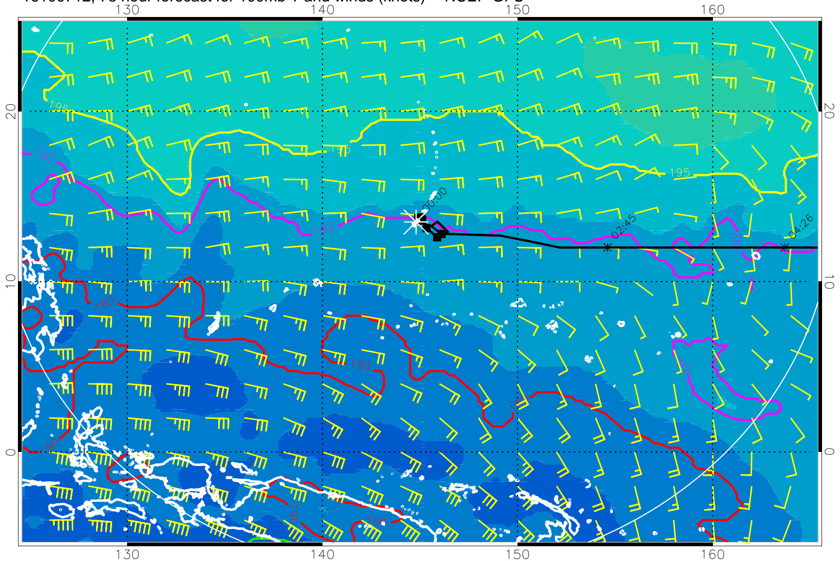
16100712, 78 hour forecast for 100mb T and winds (knots) -- NCEP GFS
