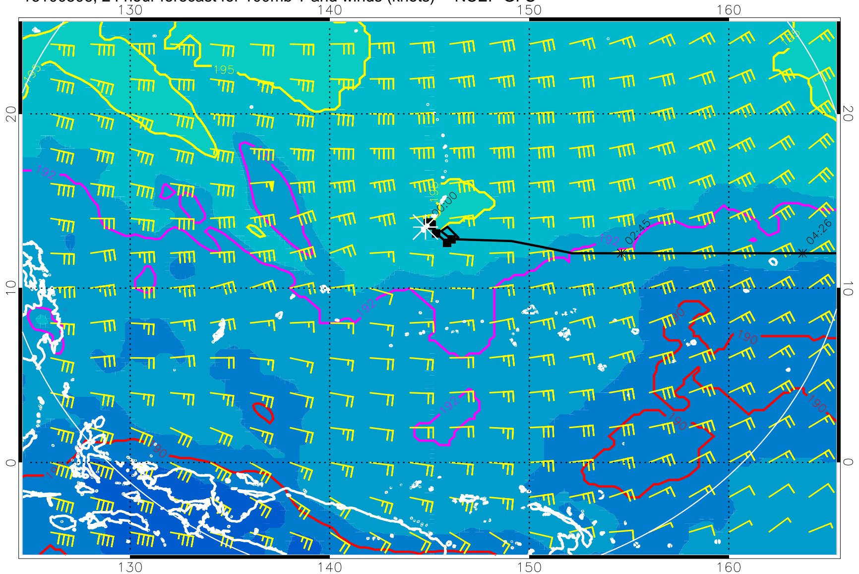
16100506, 24 hour forecast for 100mb T and winds (knots) -- NCEP GFS
