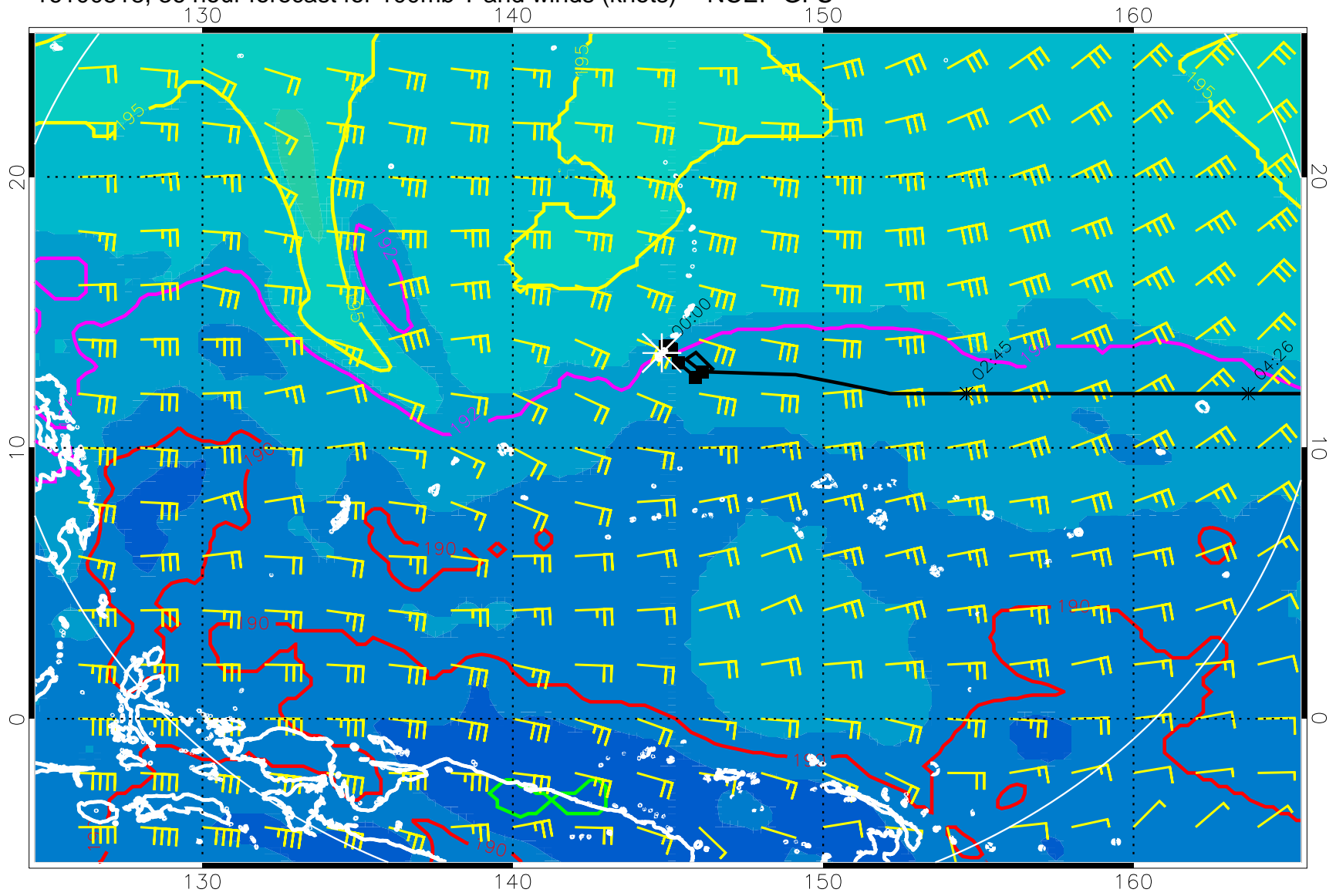
16100518, 36 hour forecast for 100mb T and winds (knots) -- NCEP GFS
