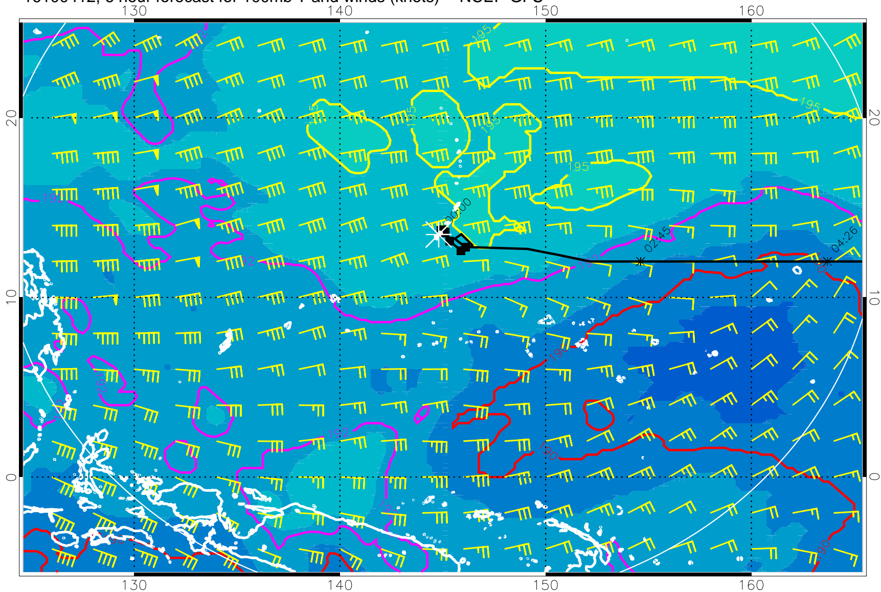
16100412, 6 hour forecast for 100mb T and winds (knots) -- NCEP GFS
