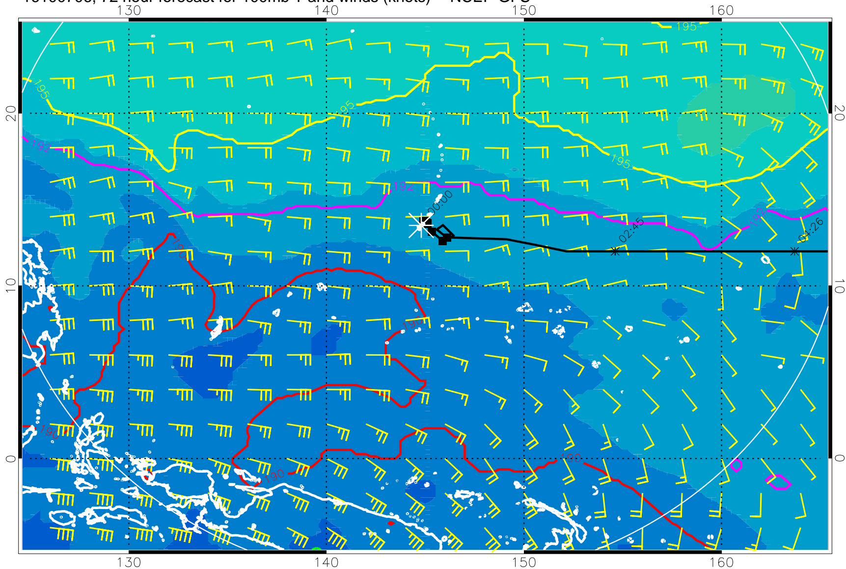
16100706, 72 hour forecast for 100mb T and winds (knots) -- NCEP GFS
