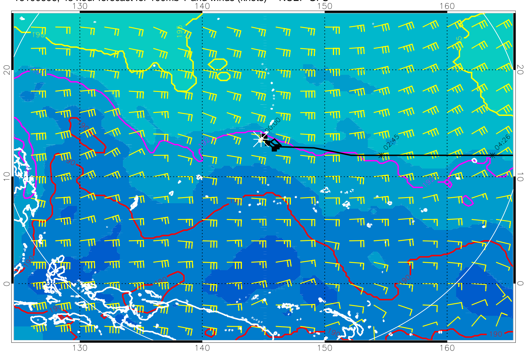
16100606, 48 hour forecast for 100mb T and winds (knots) -- NCEP GFS
