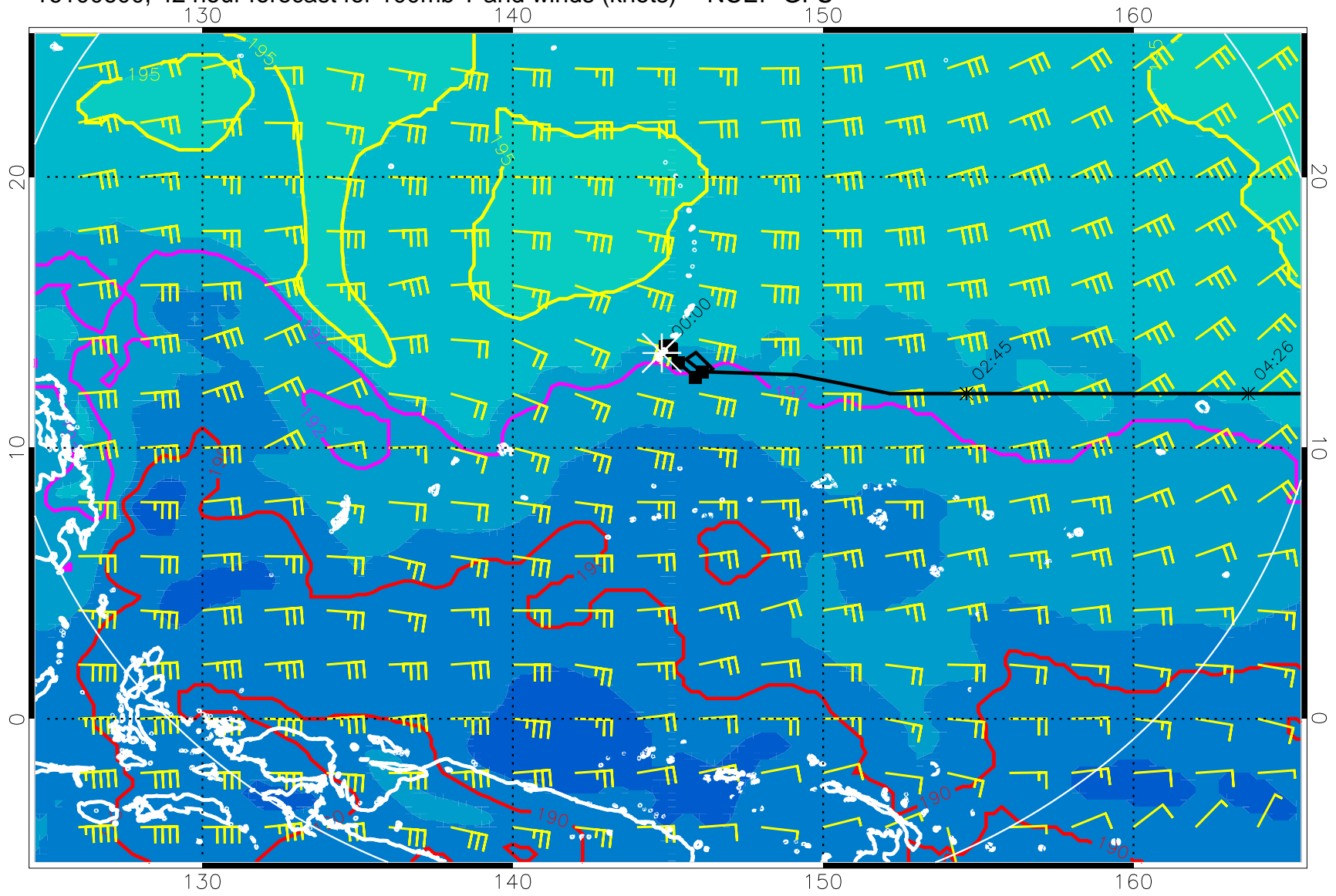
16100600, 42 hour forecast for 100mb T and winds (knots) -- NCEP GFS
