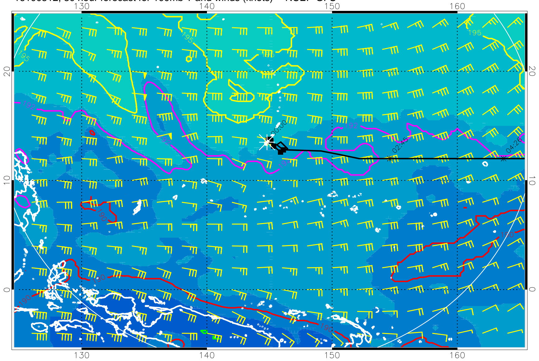
16100512, 30 hour forecast for 100mb T and winds (knots) -- NCEP GFS
