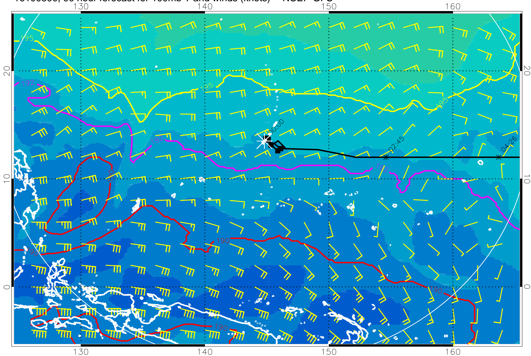
16100800, 90 hour forecast for 100mb T and winds (knots) -- NCEP GFS
