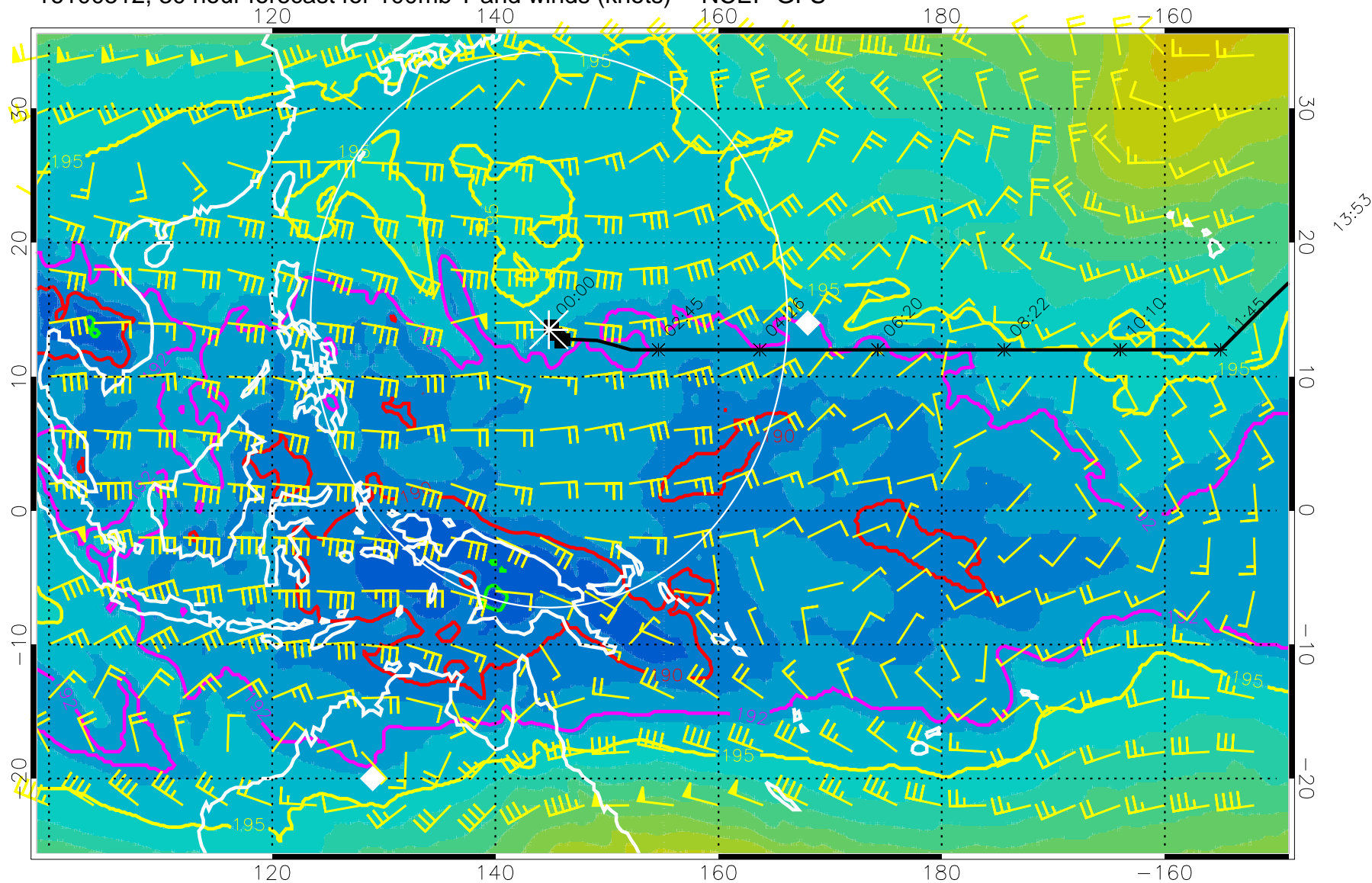
16100512, 30 hour forecast for 100mb T and winds (knots) -- NCEP GFS
