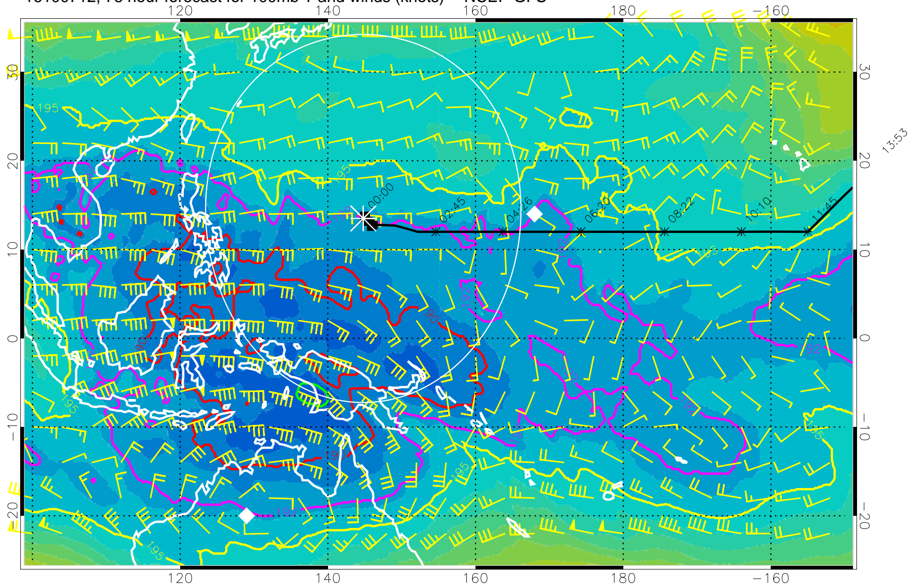
16100712, 78 hour forecast for 100mb T and winds (knots) -- NCEP GFS
