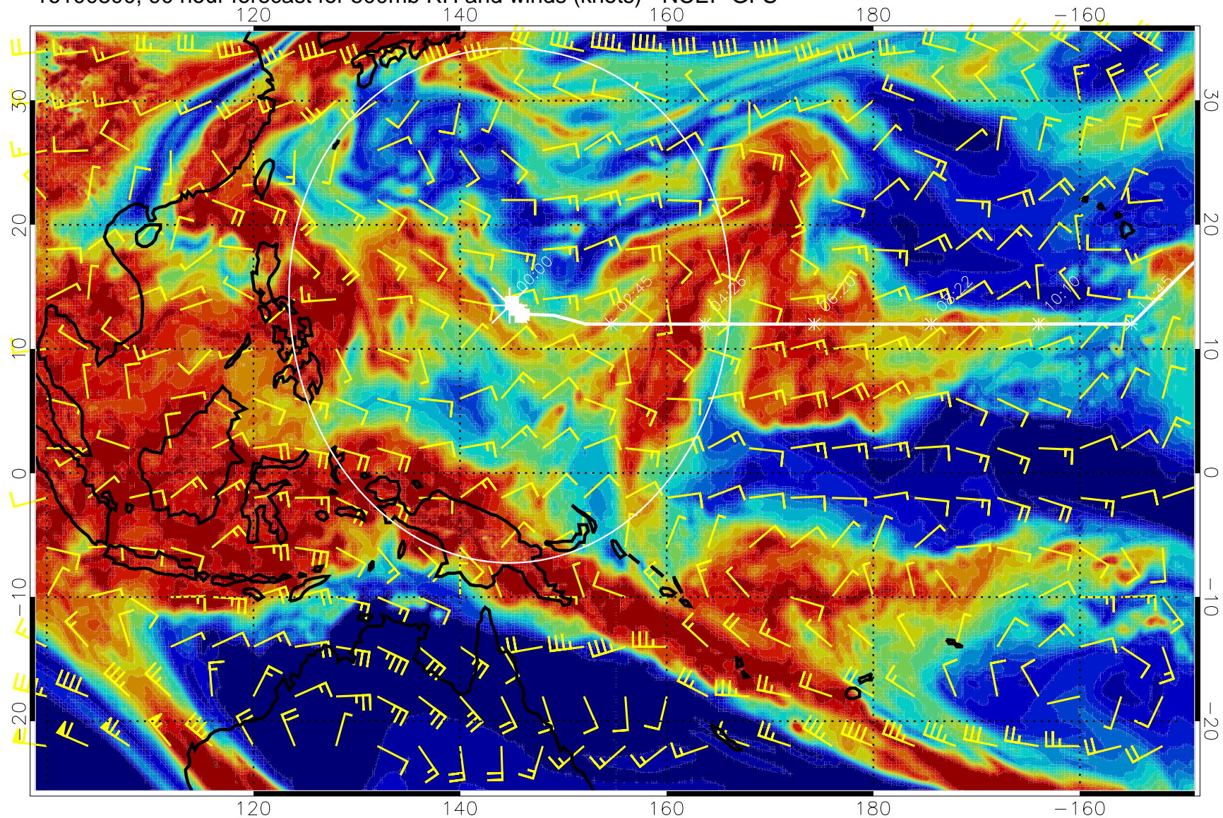
16100800, 90 hour forecast for 500mb RH and winds (knots) - NCEP GFS
