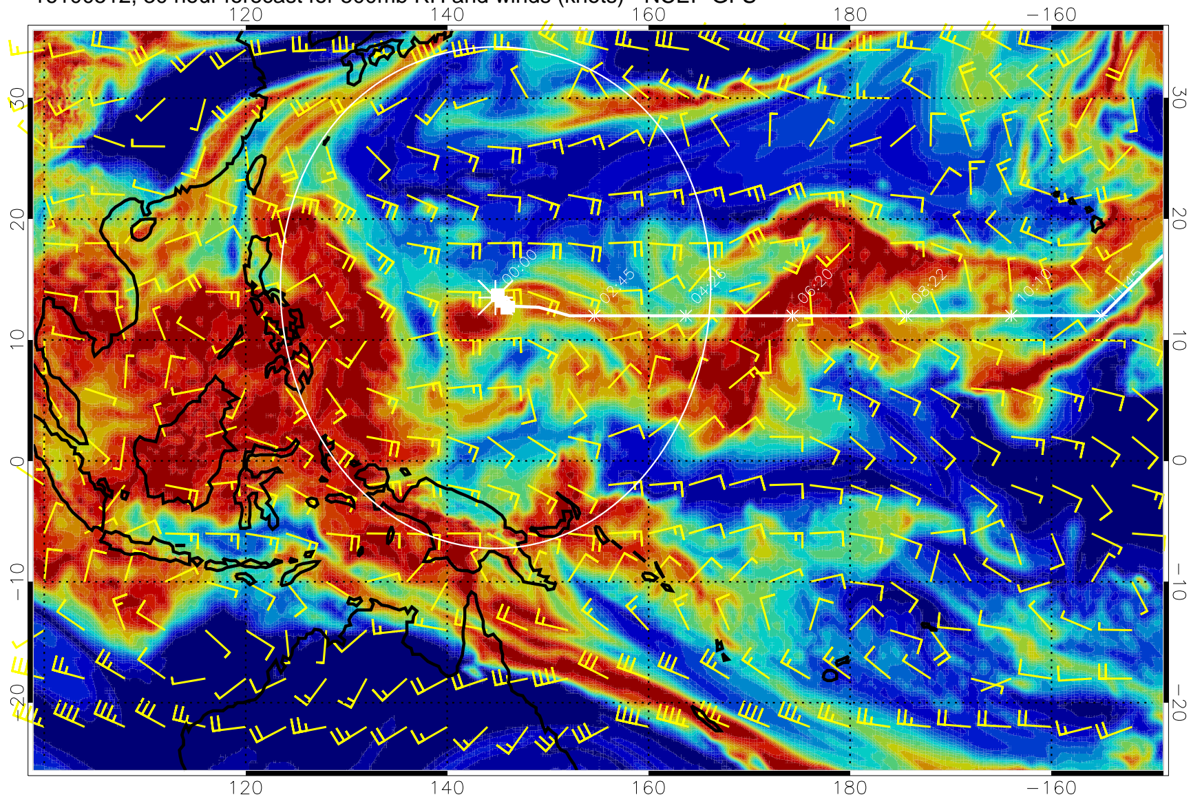
16100512, 30 hour forecast for 500mb RH and winds (knots) - NCEP GFS
