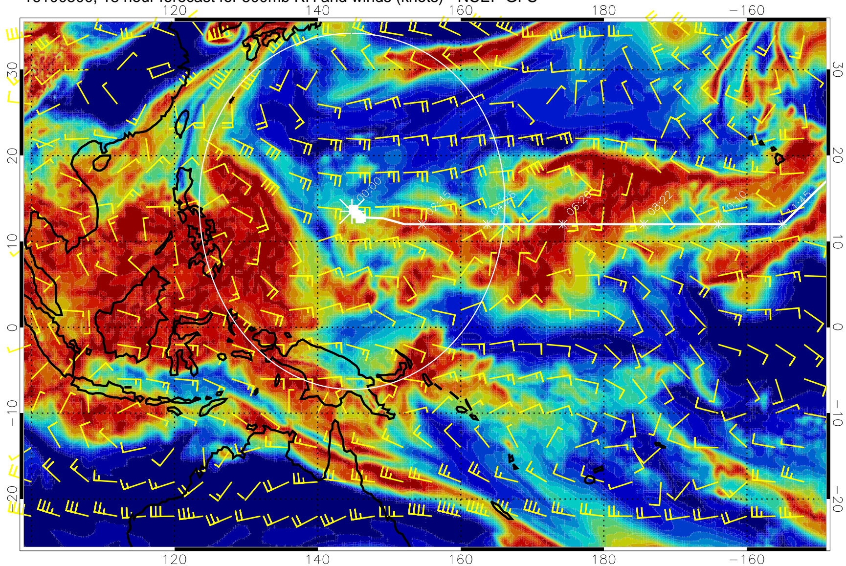
16100500, 18 hour forecast for 500mb RH and winds (knots) - NCEP GFS
