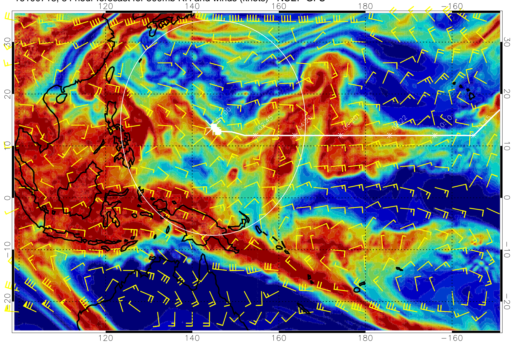
16100718, 84 hour forecast for 500mb RH and winds (knots) - NCEP GFS
