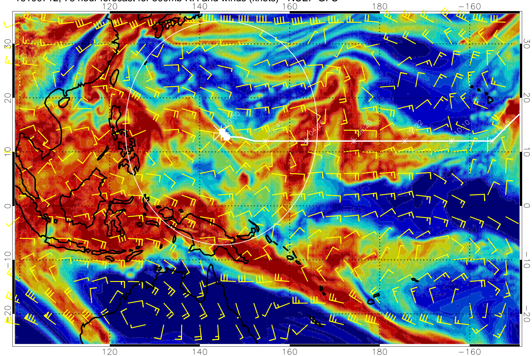
16100712, 78 hour forecast for 500mb RH and winds (knots) - NCEP GFS
