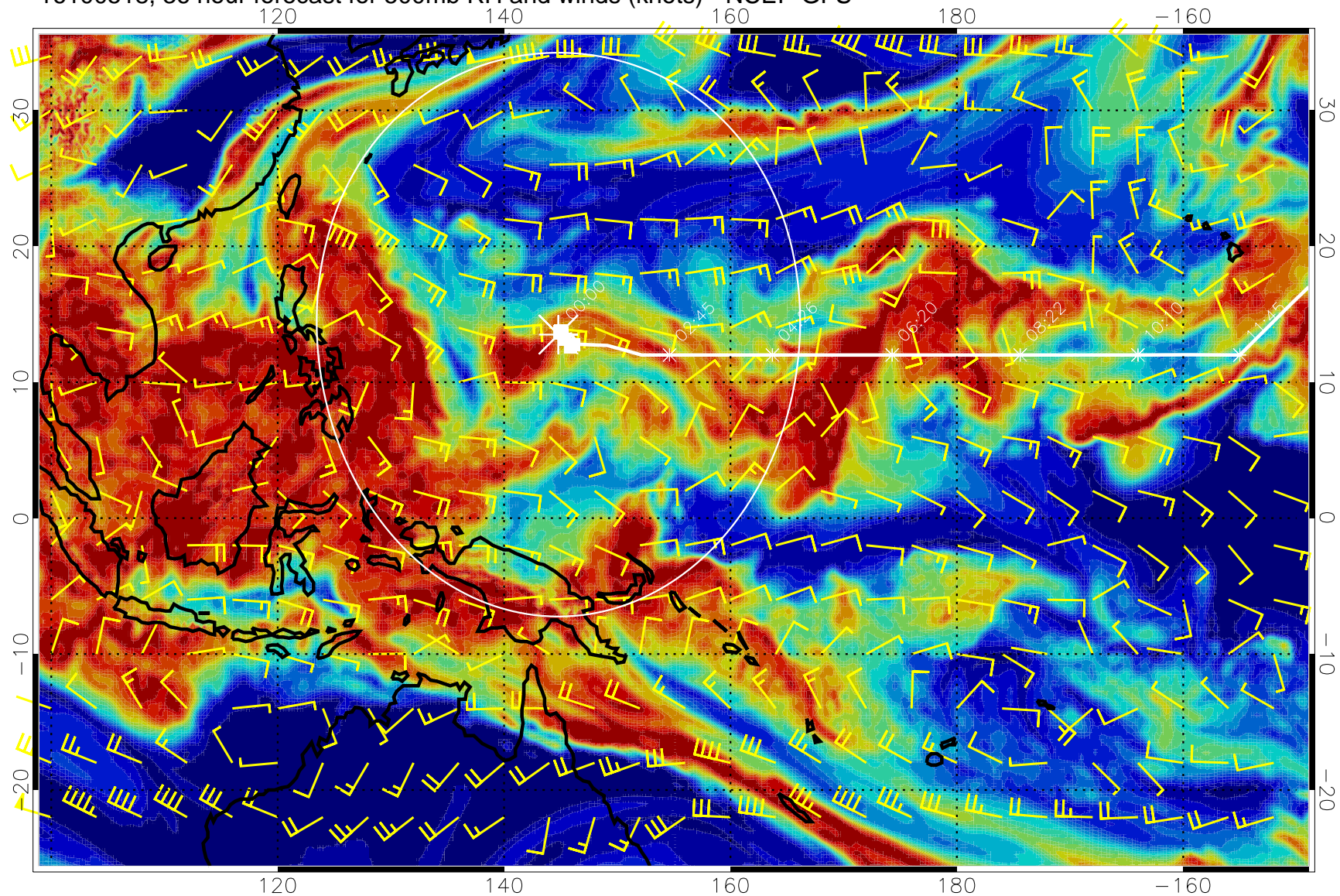
16100518, 36 hour forecast for 500mb RH and winds (knots) - NCEP GFS
