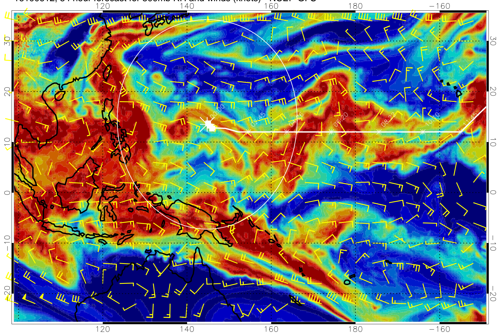
16100612, 54 hour forecast for 500mb RH and winds (knots) - NCEP GFS
