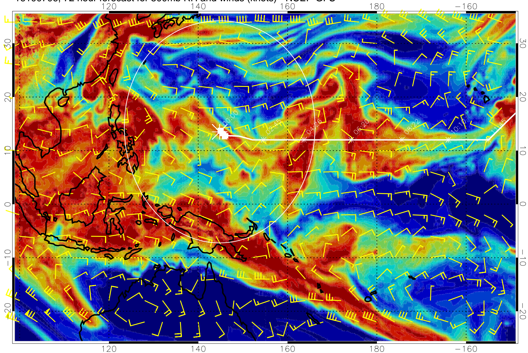
16100706, 72 hour forecast for 500mb RH and winds (knots) - NCEP GFS
