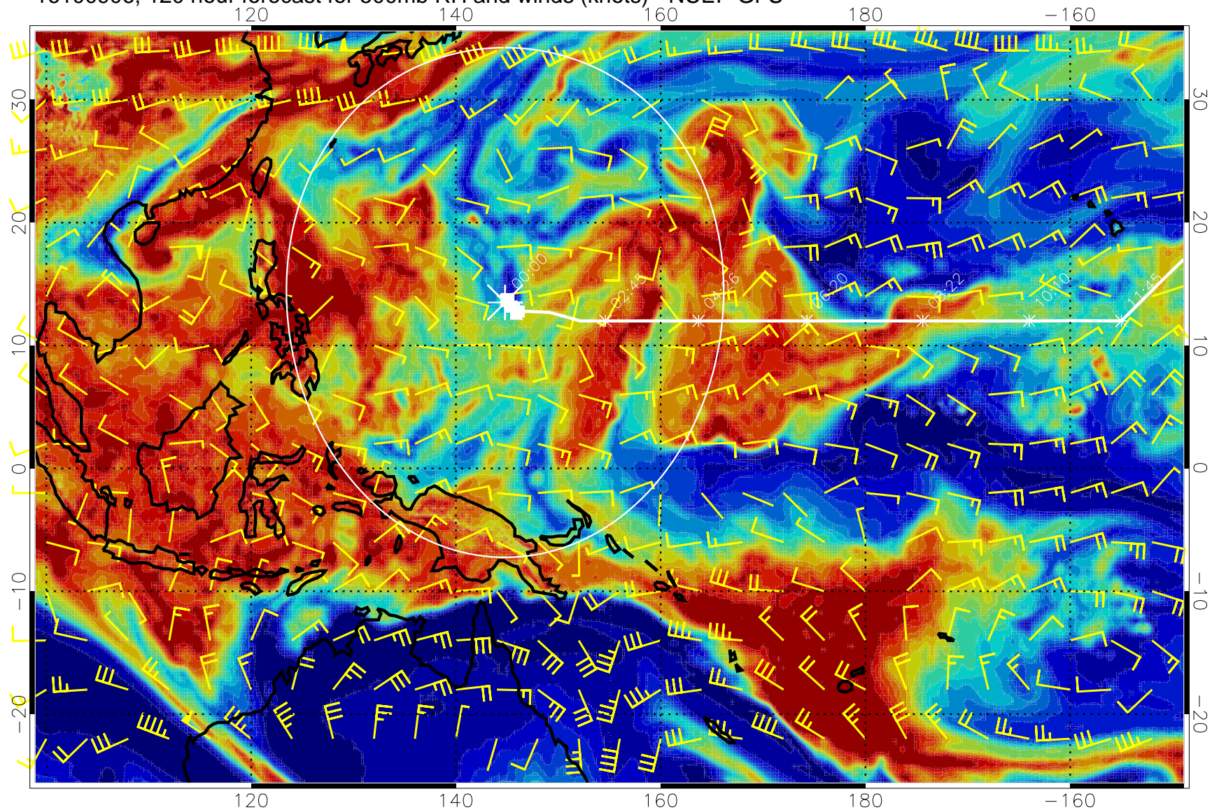
16100906, 120 hour forecast for 500mb RH and winds (knots) - NCEP GFS
