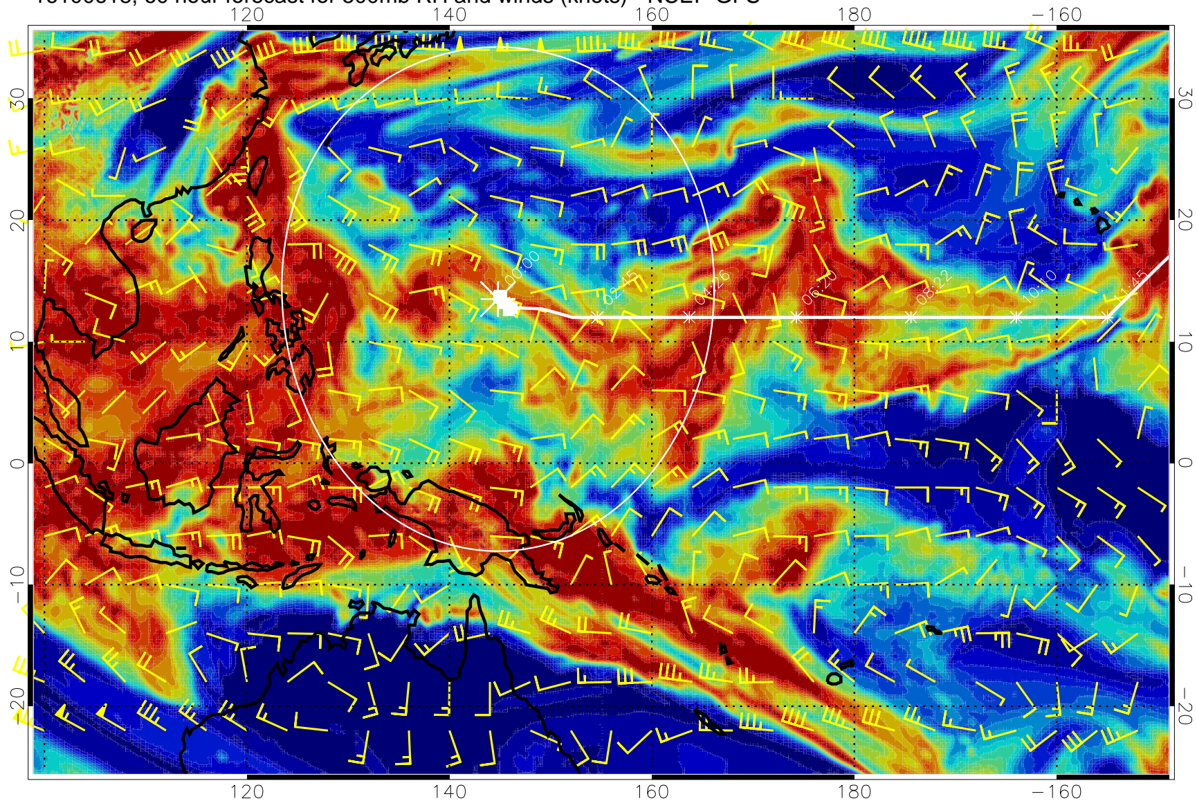
16100618, 60 hour forecast for 500mb RH and winds (knots) - NCEP GFS
