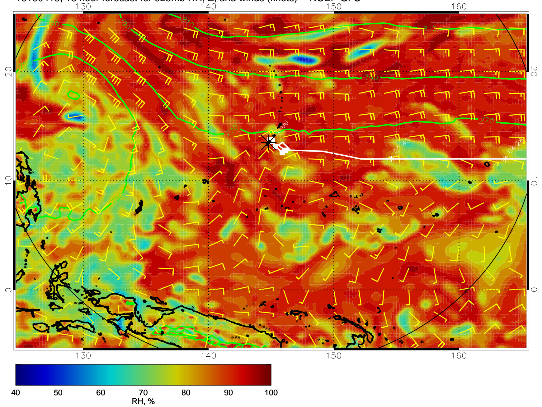
16100418, 18 hour forecast for 925mb RH, Z, and winds (knots) -- NCEP GFS
