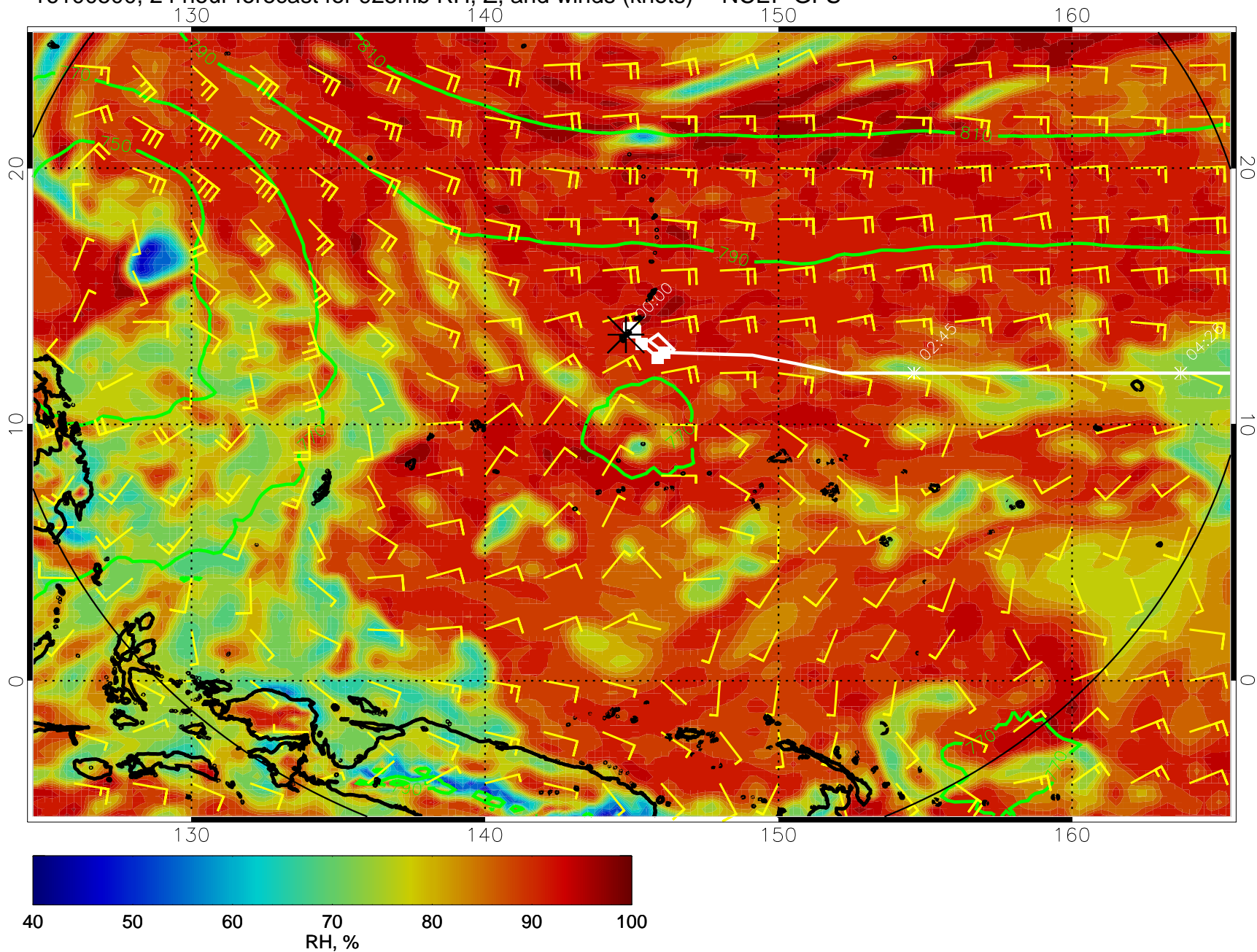
16100500, 24 hour forecast for 925mb RH, Z, and winds (knots) -- NCEP GFS
