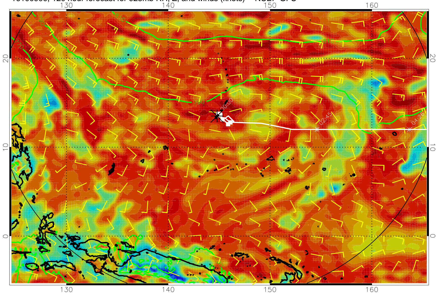
16100900, 120 hour forecast for 925mb RH, Z, and winds (knots) -- NCEP GFS
