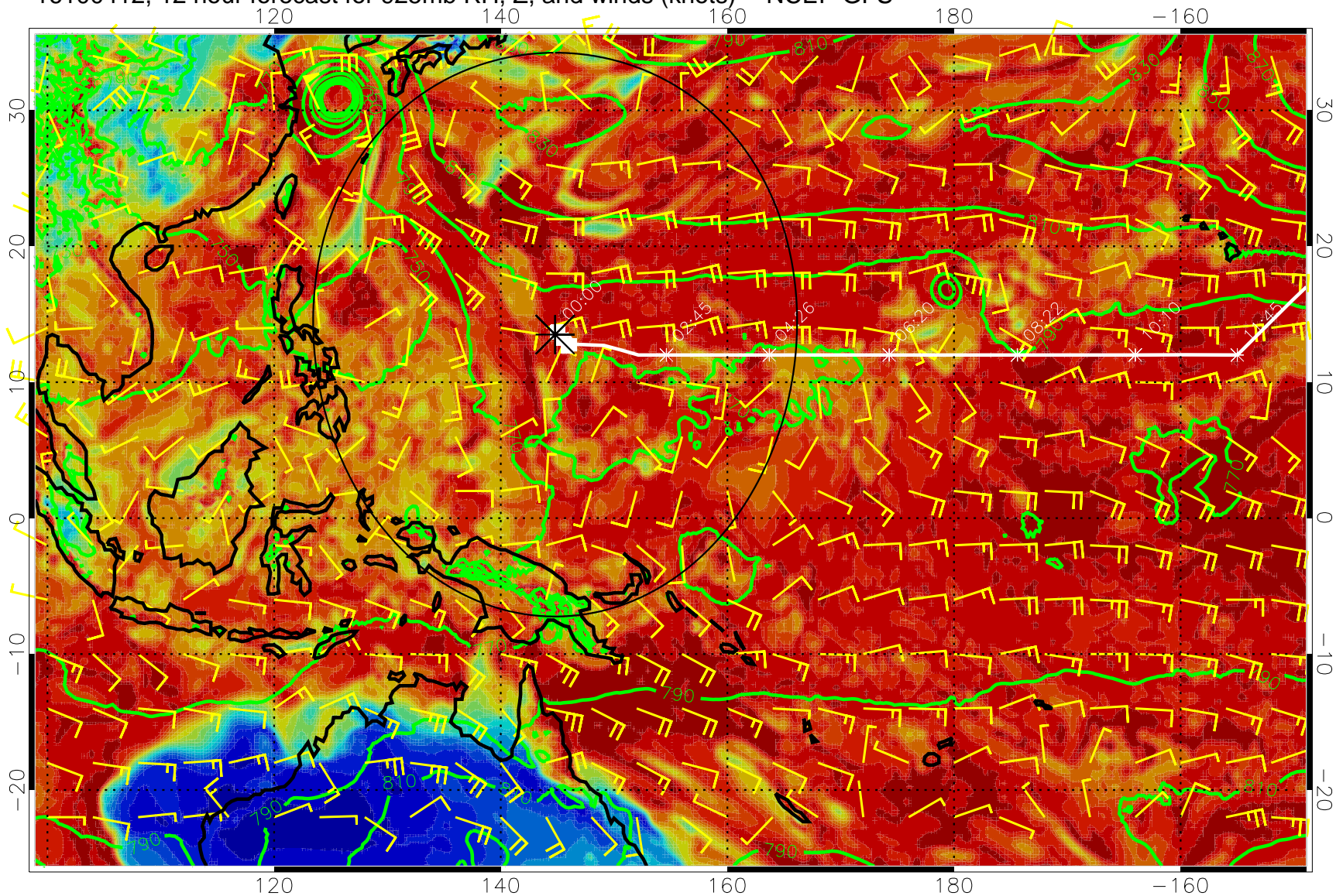
16100412, 12 hour forecast for 925mb RH, Z, and winds (knots) -- NCEP GFS
