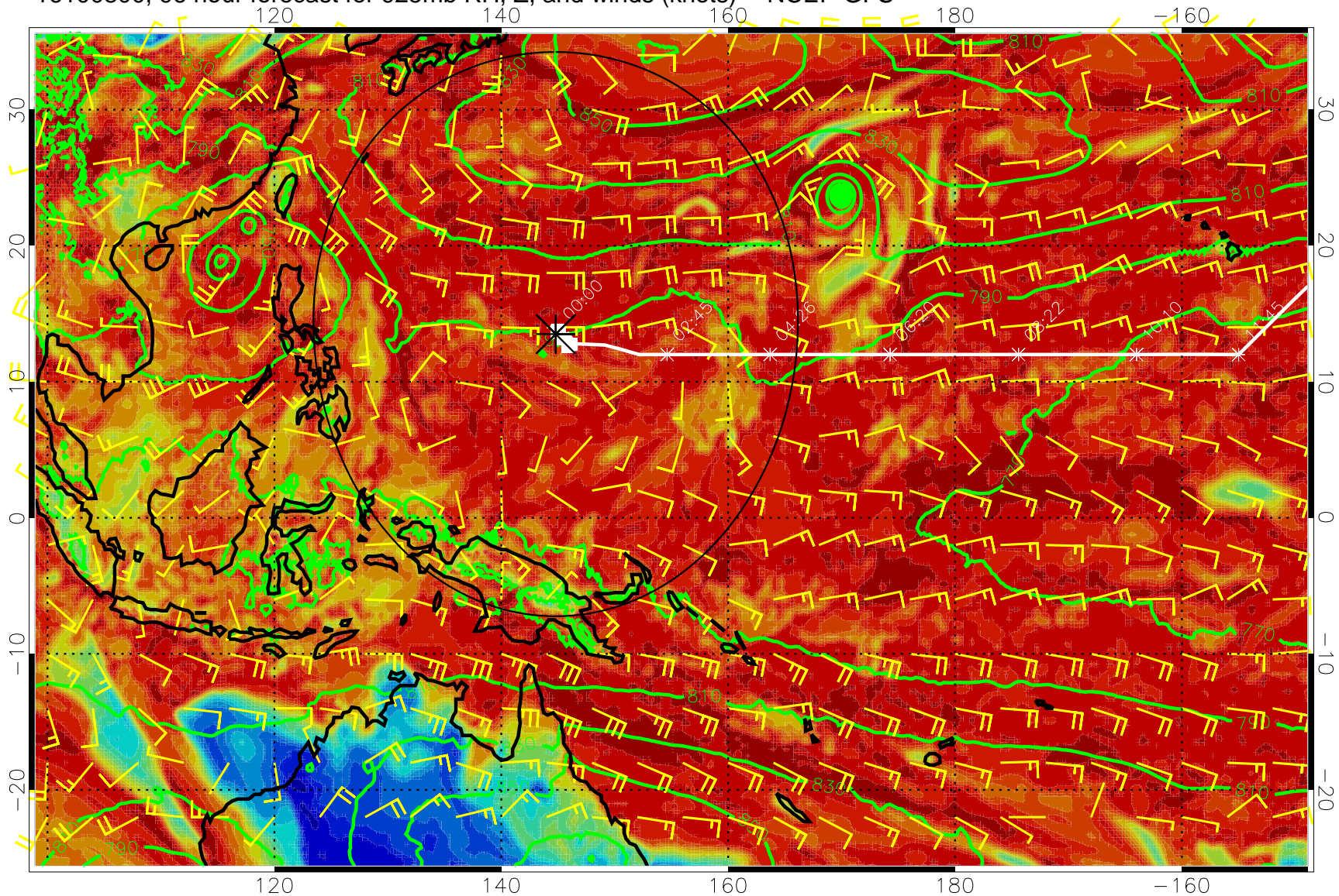
16100800, 96 hour forecast for 925mb RH, Z, and winds (knots) -- NCEP GFS
