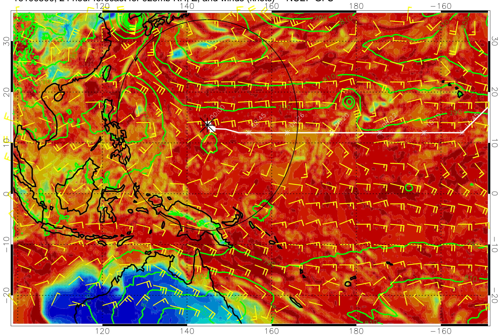
16100500, 24 hour forecast for 925mb RH, Z, and winds (knots) -- NCEP GFS
