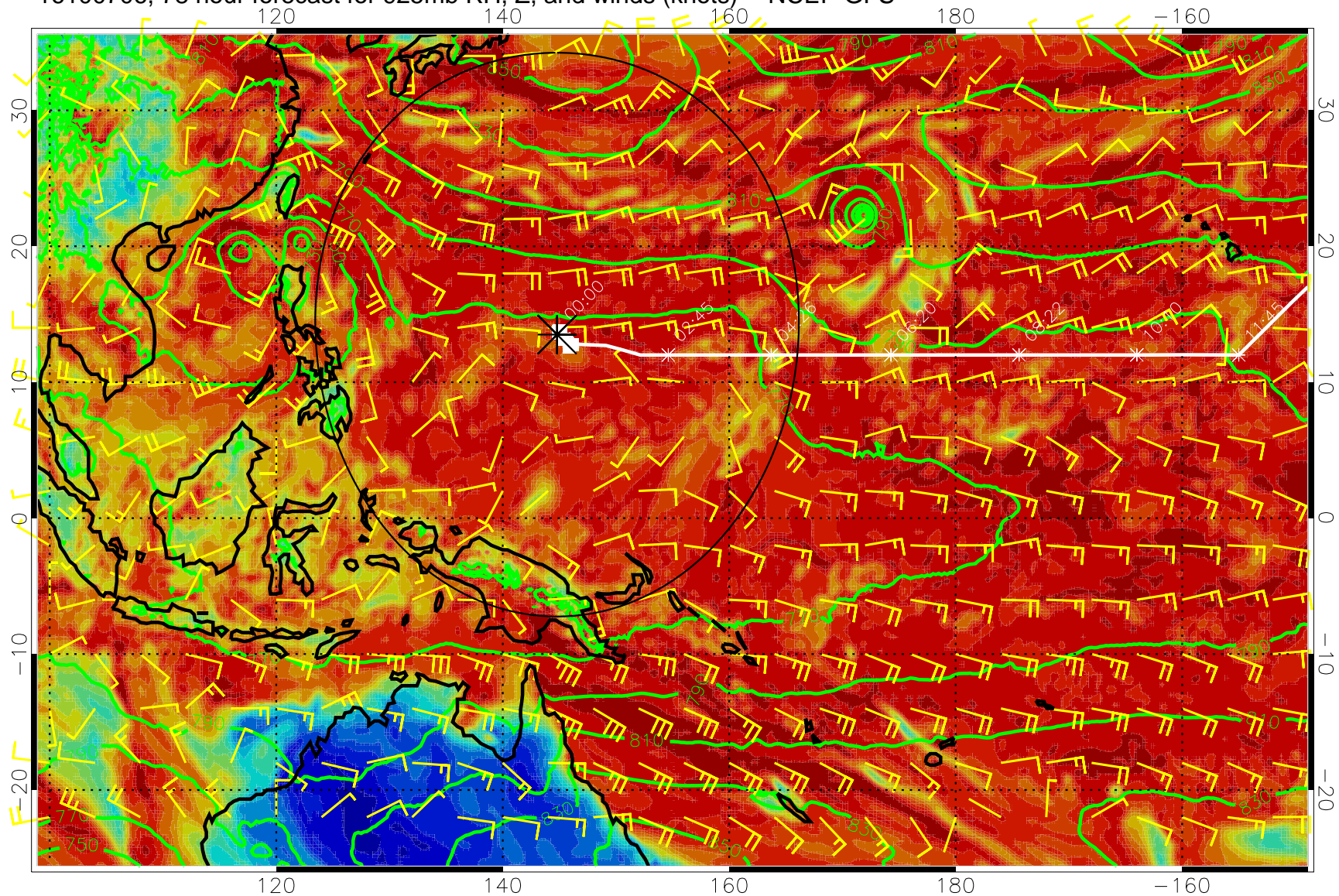
16100706, 78 hour forecast for 925mb RH, Z, and winds (knots) -- NCEP GFS
