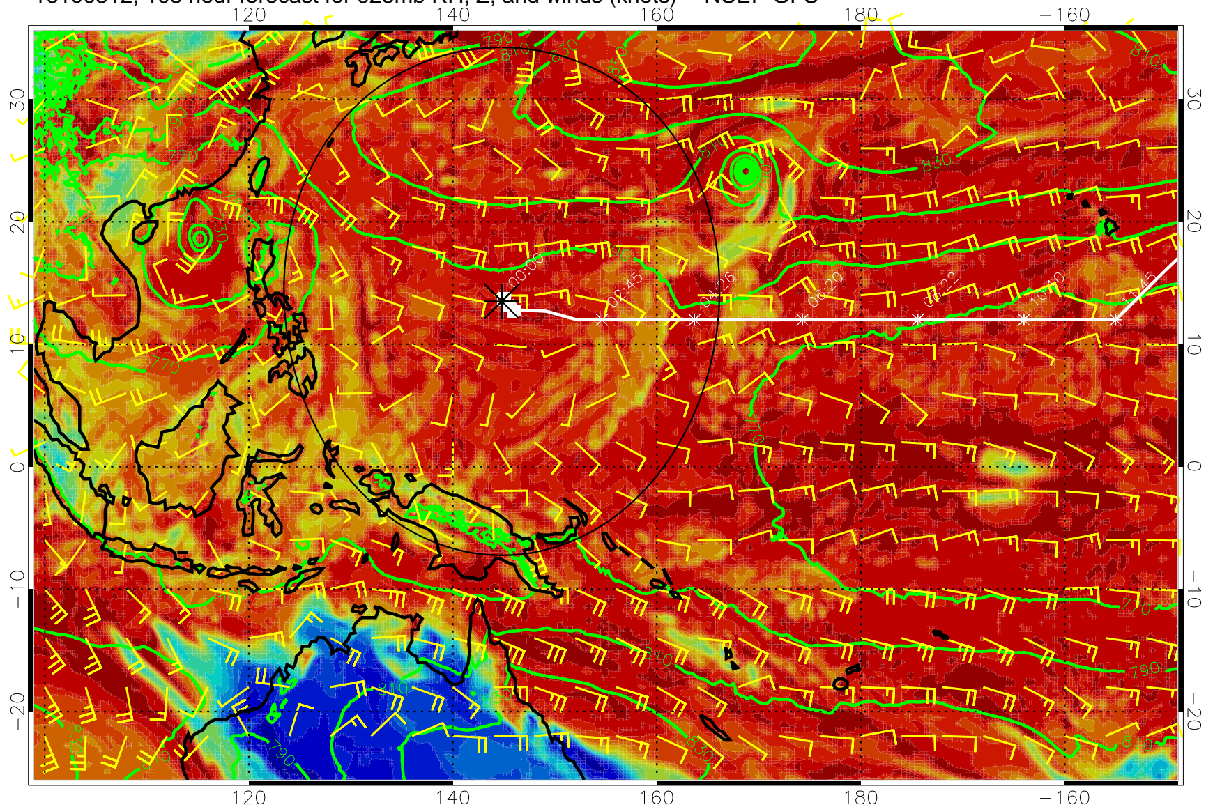
16100812, 108 hour forecast for 925mb RH, Z, and winds (knots) -- NCEP GFS
