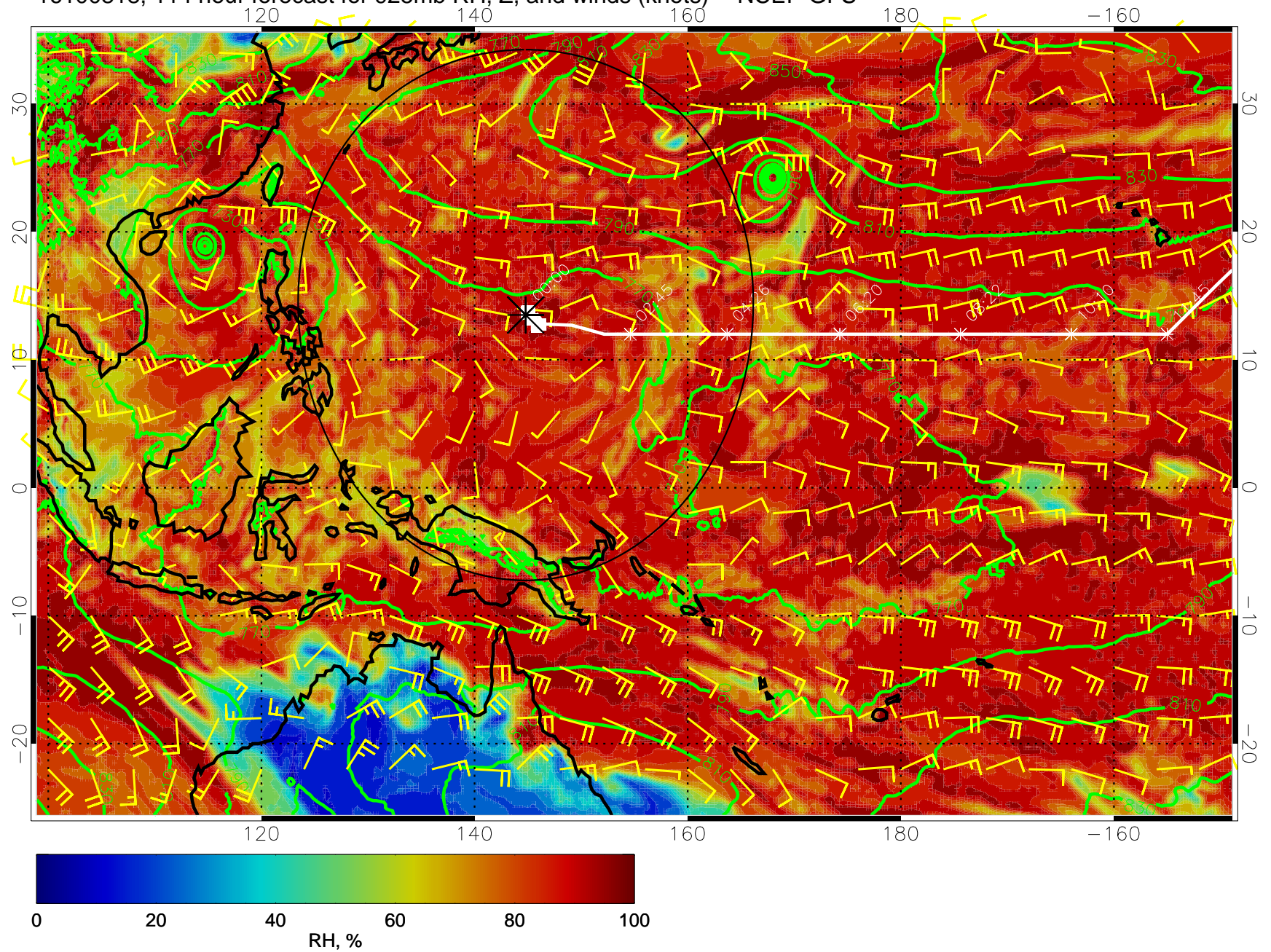
16100818, 114 hour forecast for 925mb RH, Z, and winds (knots) -- NCEP GFS
