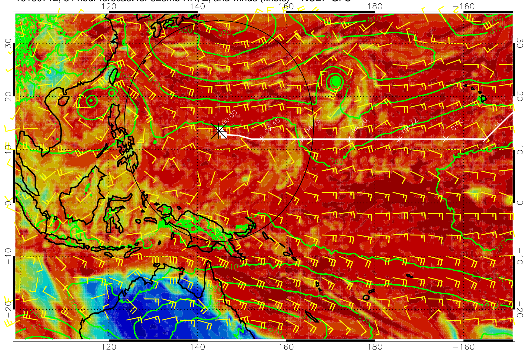
16100712, 84 hour forecast for 925mb RH, Z, and winds (knots) -- NCEP GFS
