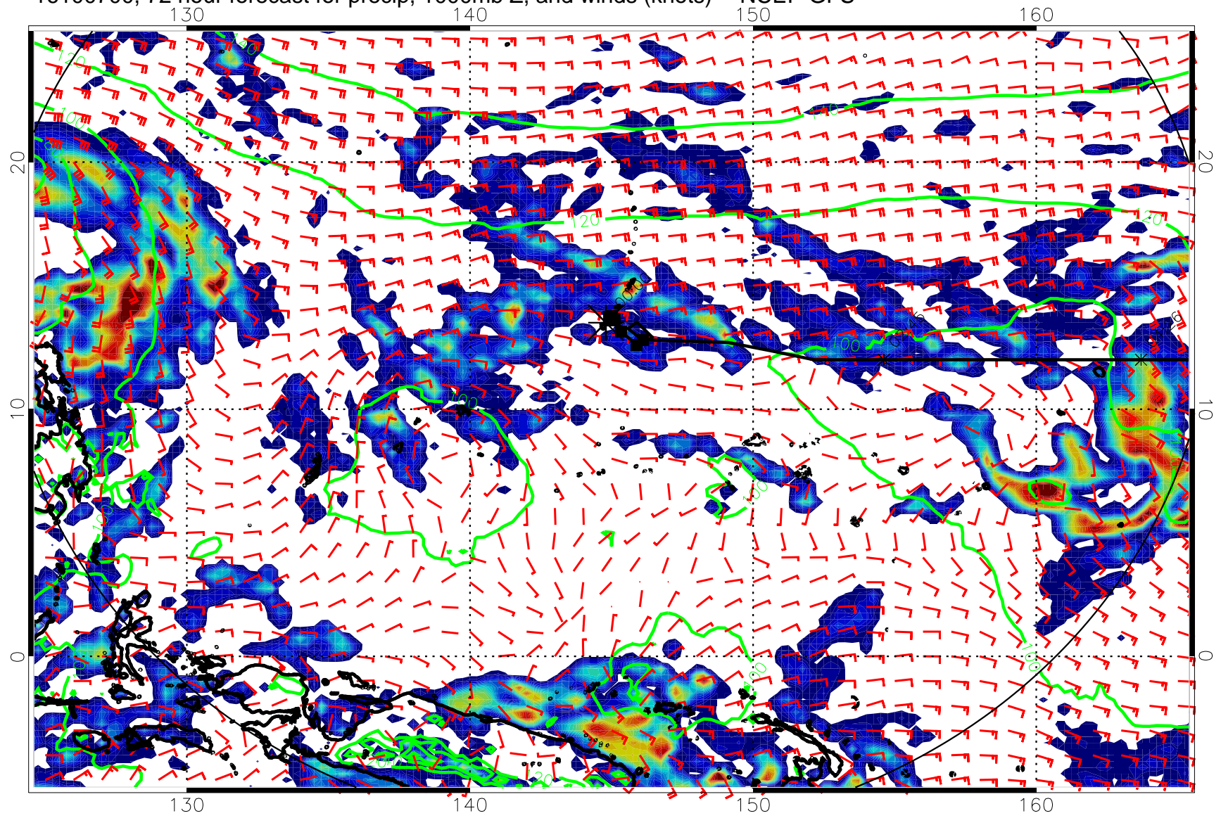
16100700, 72 hour forecast for precip, 1000mb Z, and winds (knots) -- NCEP GFS
