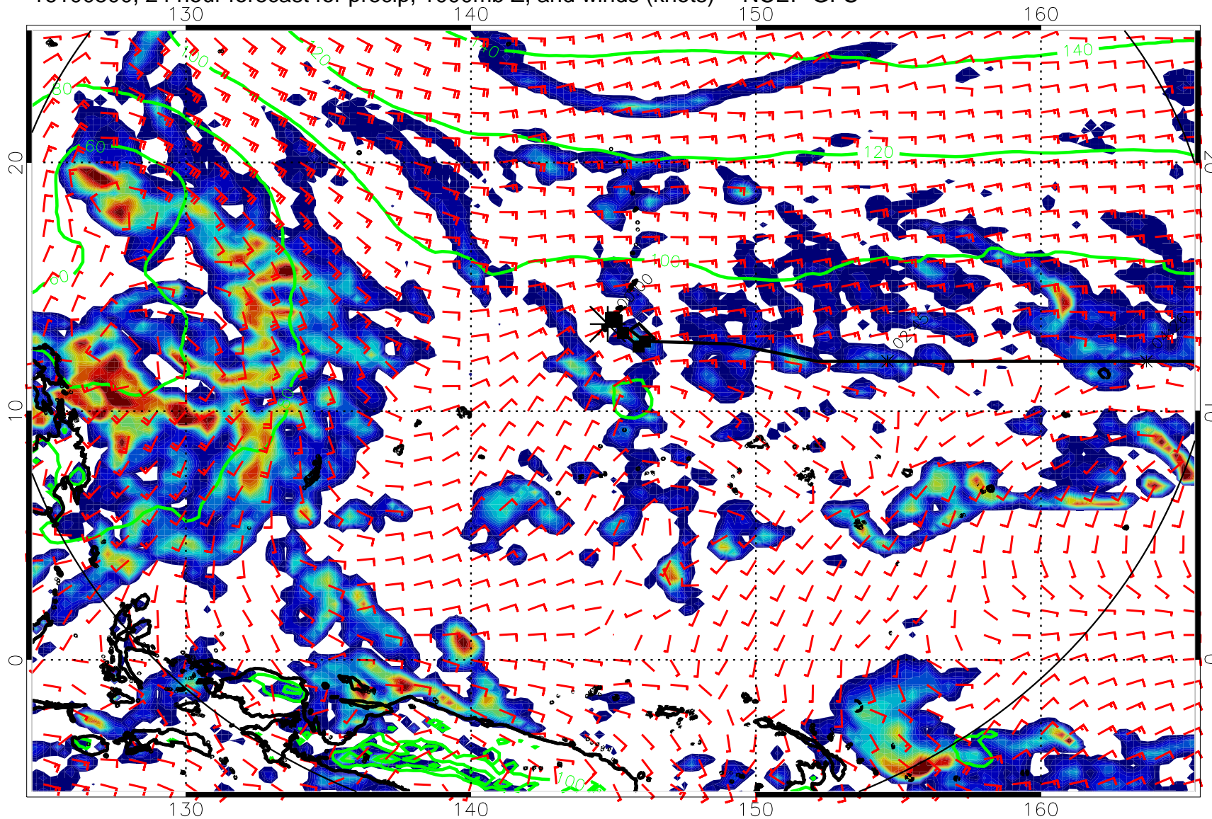
16100500, 24 hour forecast for precip, 1000mb Z, and winds (knots) -- NCEP GFS
