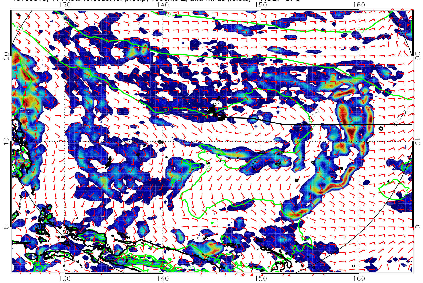
16100818, 114 hour forecast for precip, 1000mb Z, and winds (knots) -- NCEP GFS
