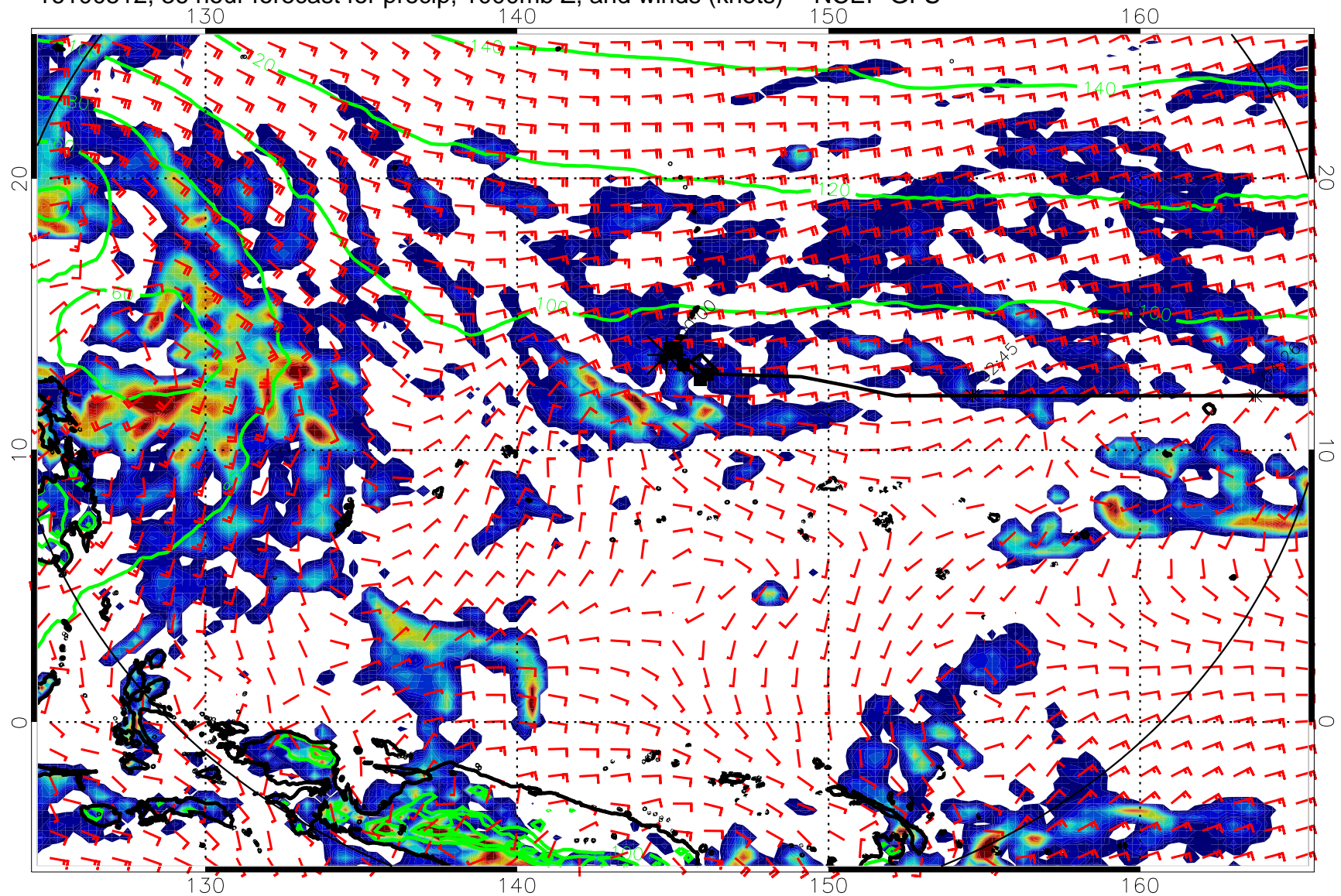
16100512, 36 hour forecast for precip, 1000mb Z, and winds (knots) -- NCEP GFS
