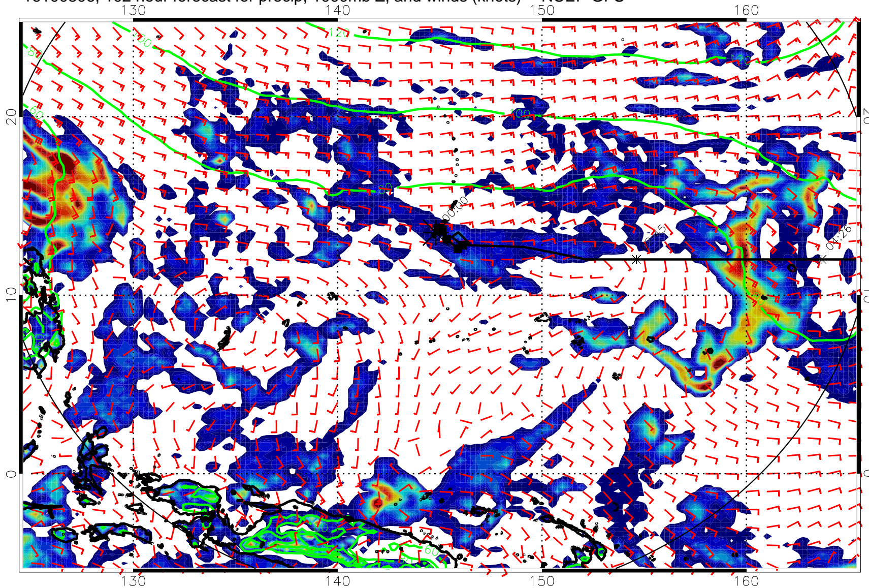
16100806, 102 hour forecast for precip, 1000mb Z, and winds (knots) -- NCEP GFS
