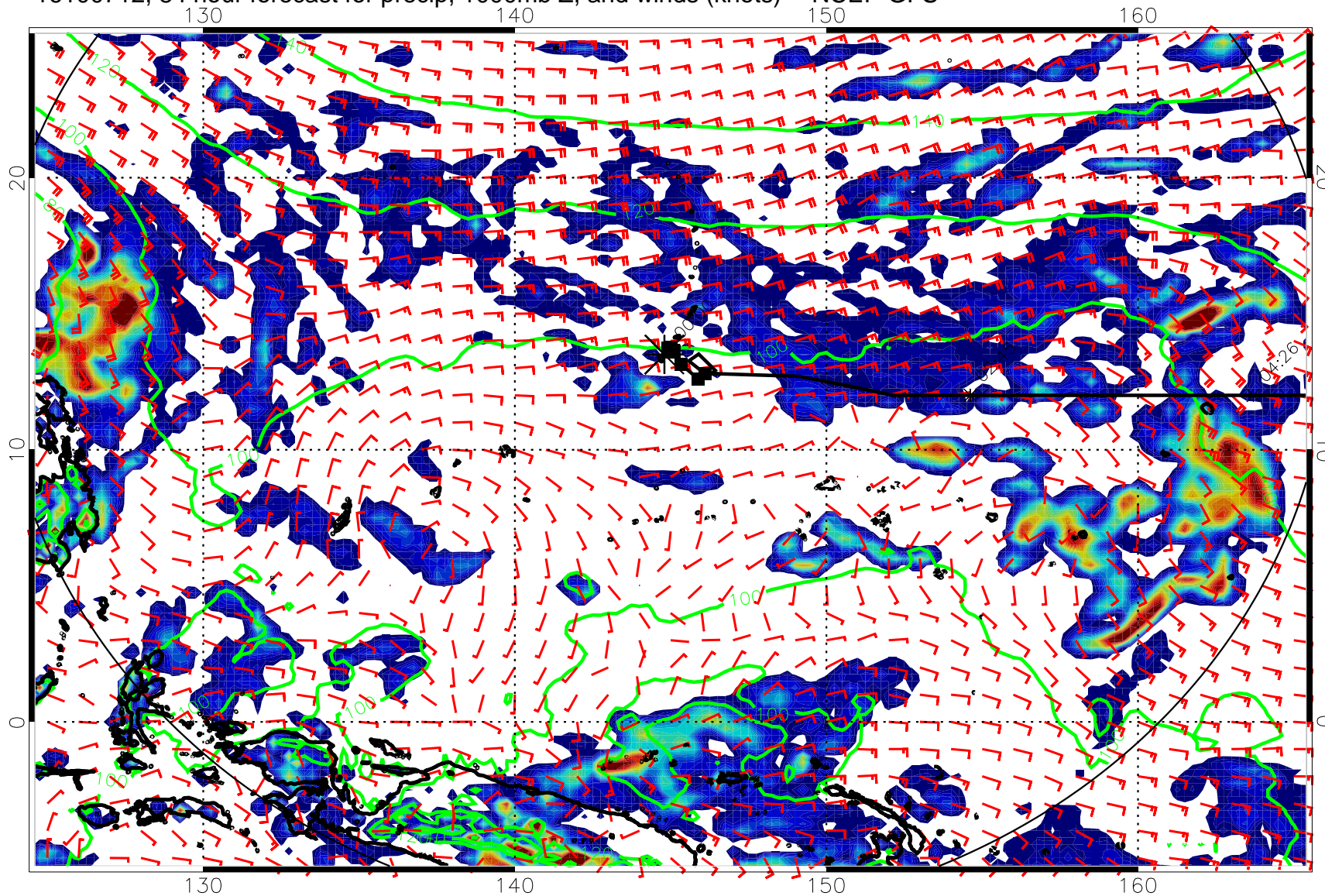
16100712, 84 hour forecast for precip, 1000mb Z, and winds (knots) -- NCEP GFS
