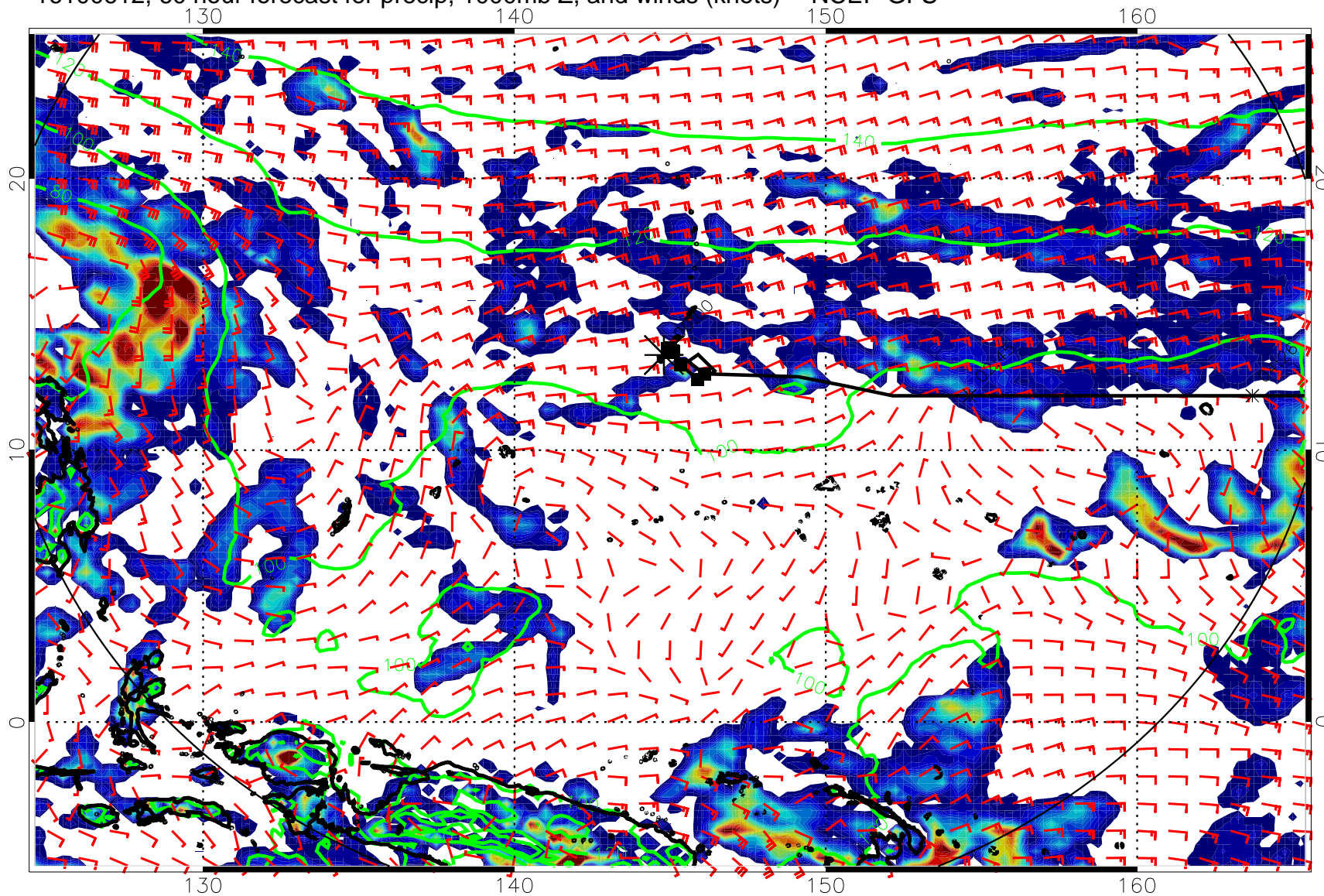
16100612, 60 hour forecast for precip, 1000mb Z, and winds (knots) -- NCEP GFS
