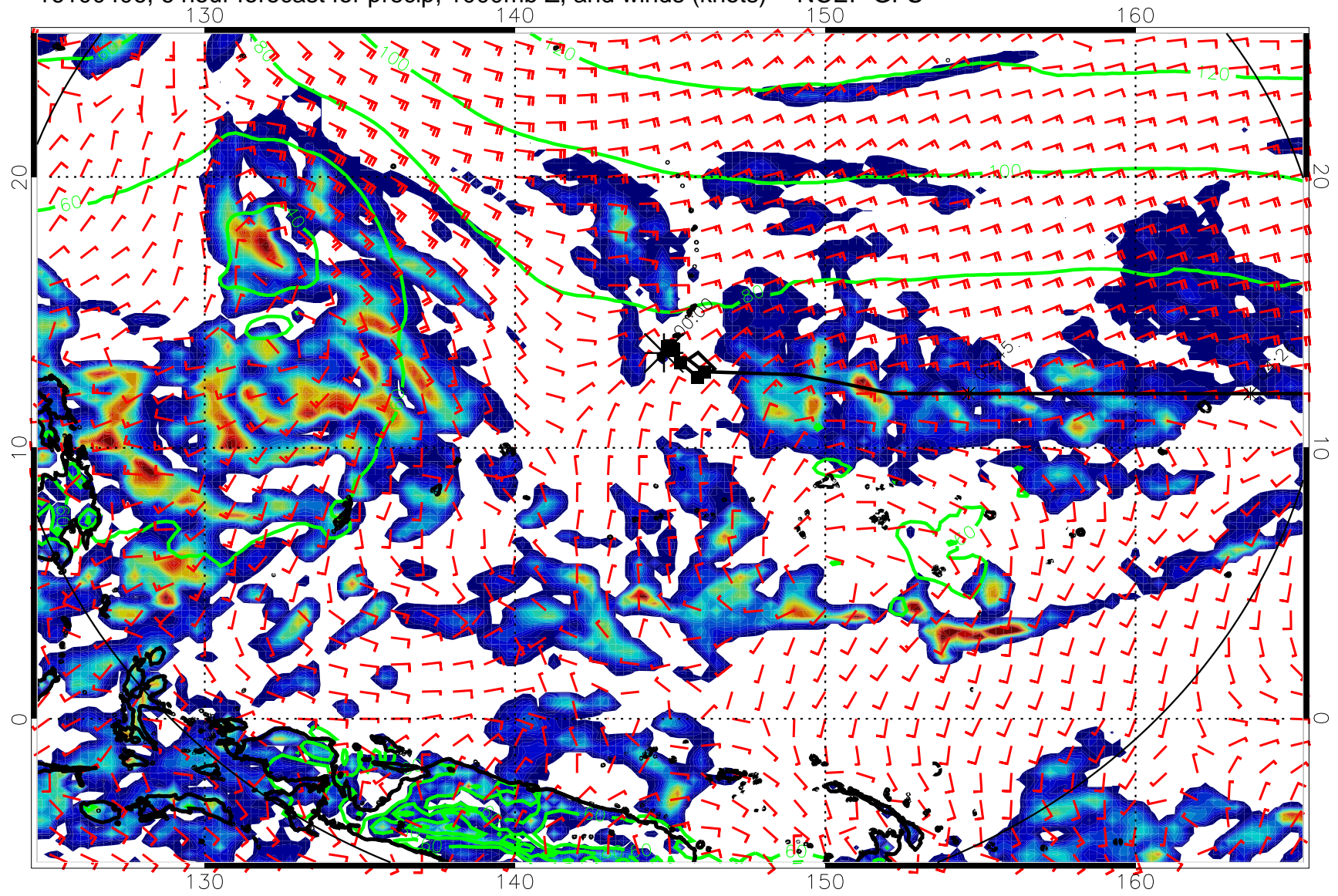
16100406, 6 hour forecast for precip, 1000mb Z, and winds (knots) -- NCEP GFS
