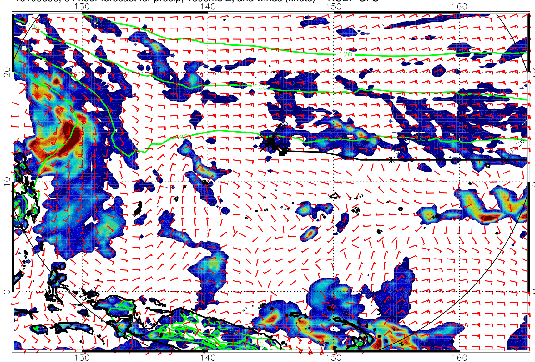
16100606, 54 hour forecast for precip, 1000mb Z, and winds (knots) -- NCEP GFS
