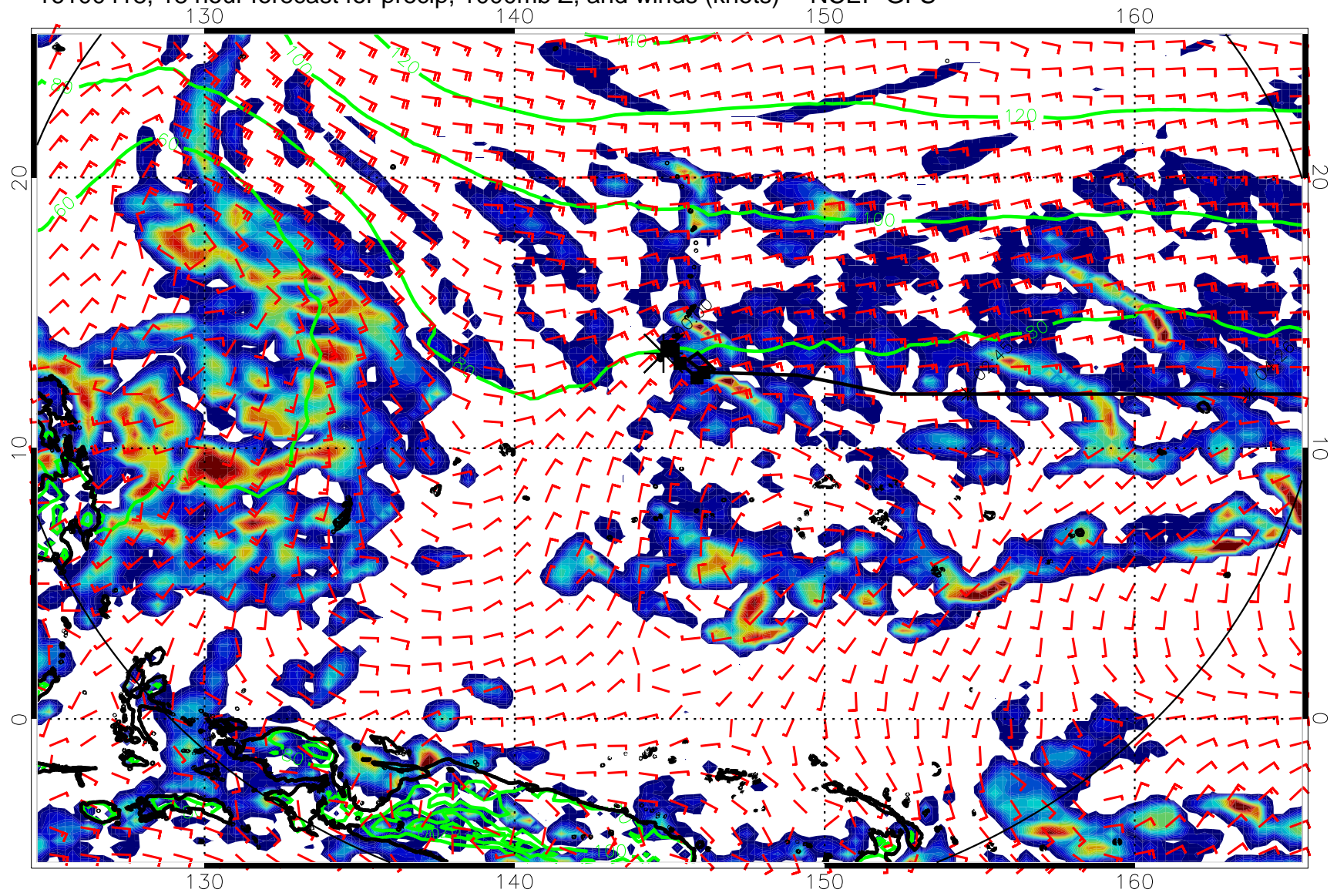
16100418, 18 hour forecast for precip, 1000mb Z, and winds (knots) -- NCEP GFS
