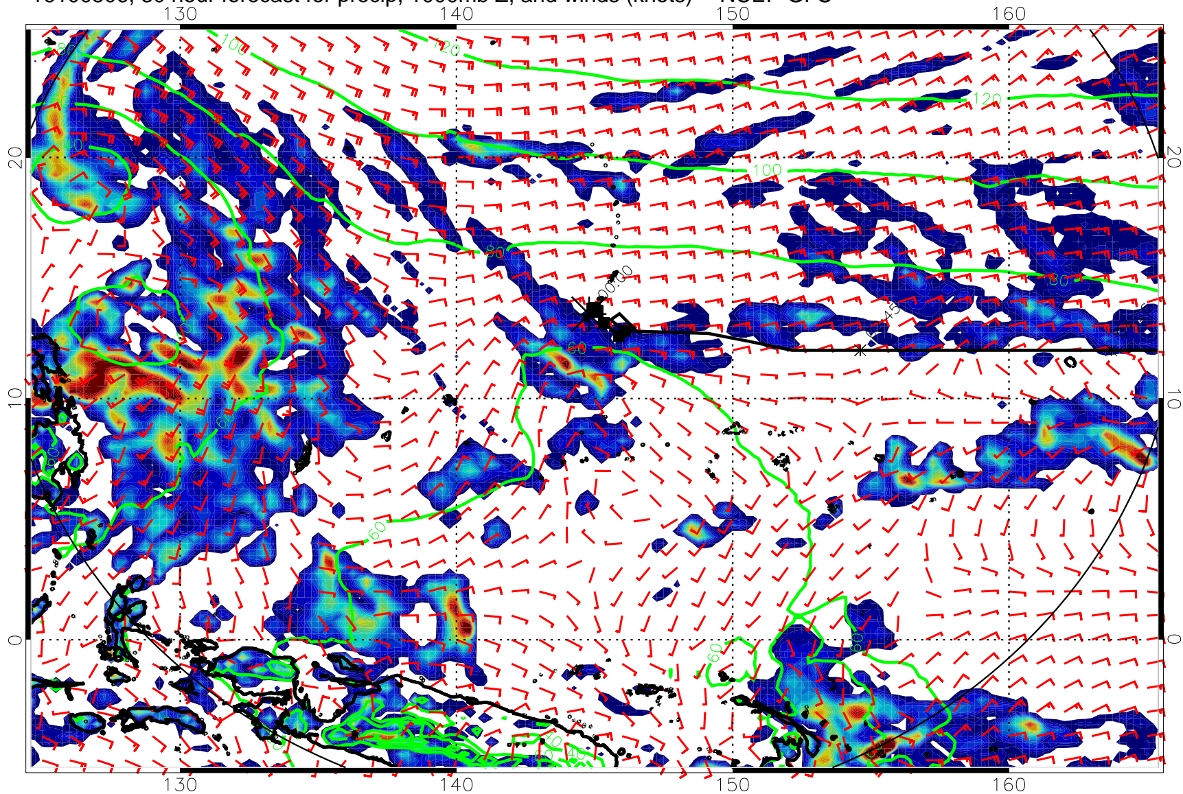
16100506, 30 hour forecast for precip, 1000mb Z, and winds (knots) -- NCEP GFS
