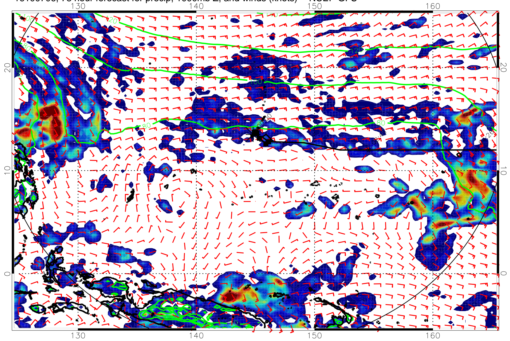
16100706, 78 hour forecast for precip, 1000mb Z, and winds (knots) -- NCEP GFS
