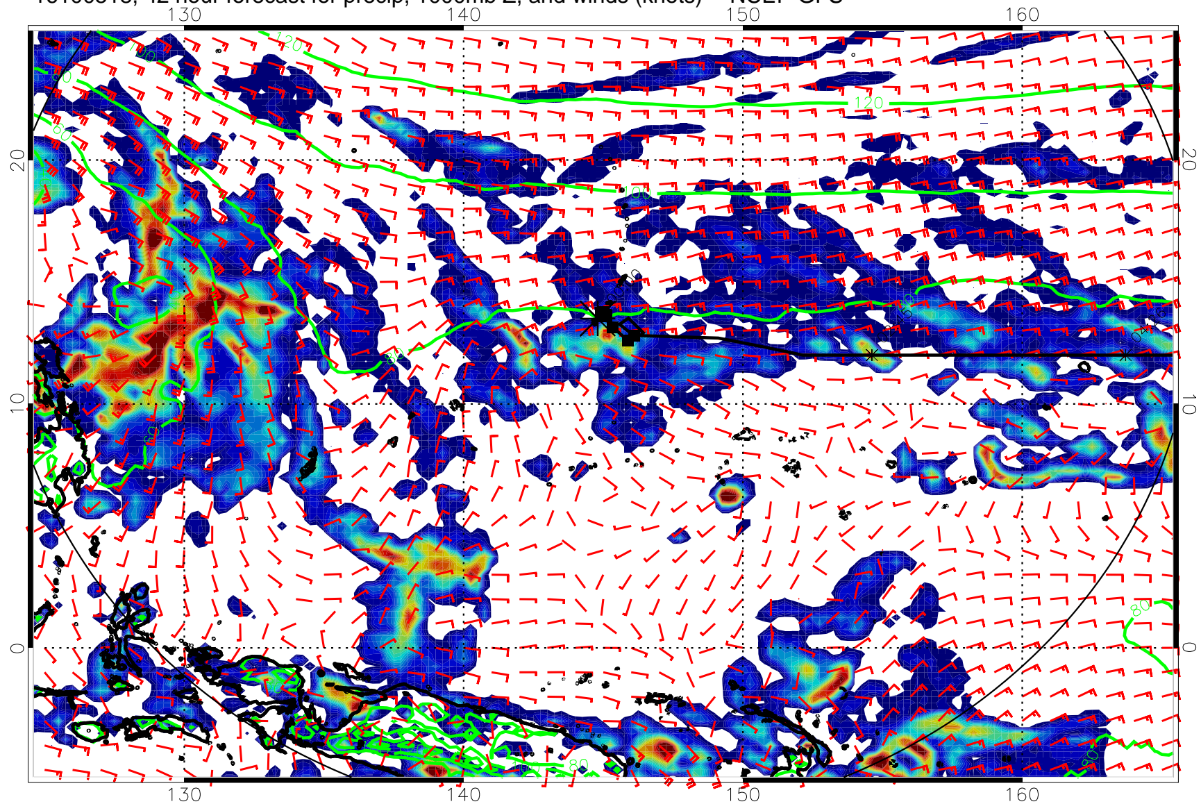
16100518, 42 hour forecast for precip, 1000mb Z, and winds (knots) -- NCEP GFS
