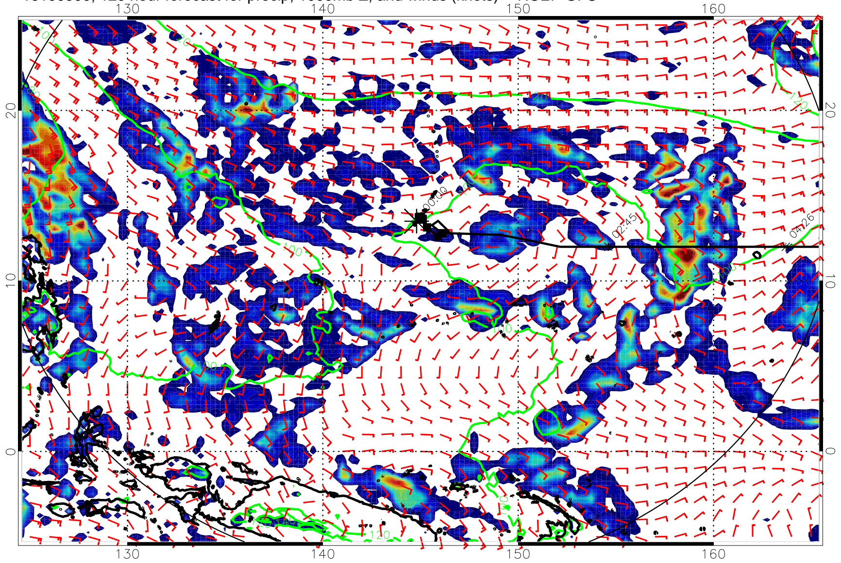
16100900, 120 hour forecast for precip, 1000mb Z, and winds (knots) -- NCEP GFS
