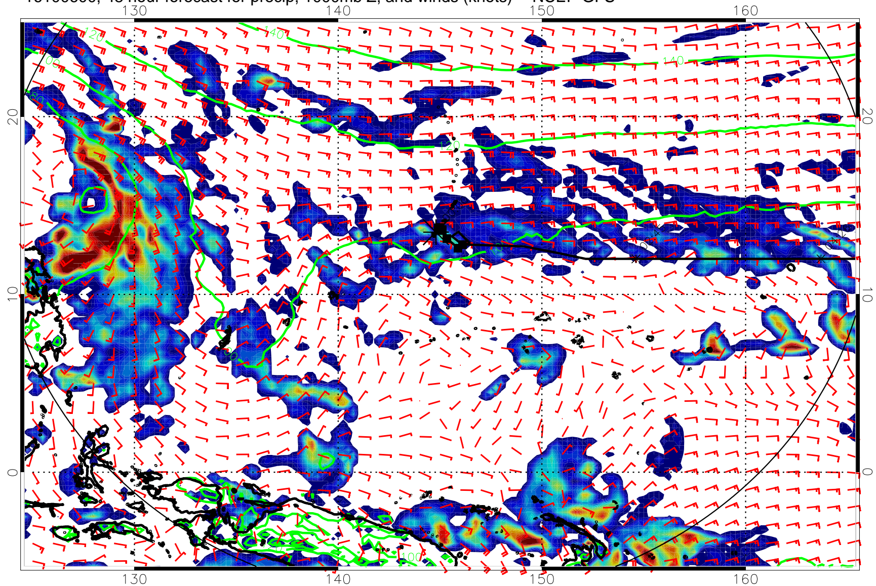
16100600, 48 hour forecast for precip, 1000mb Z, and winds (knots) -- NCEP GFS
