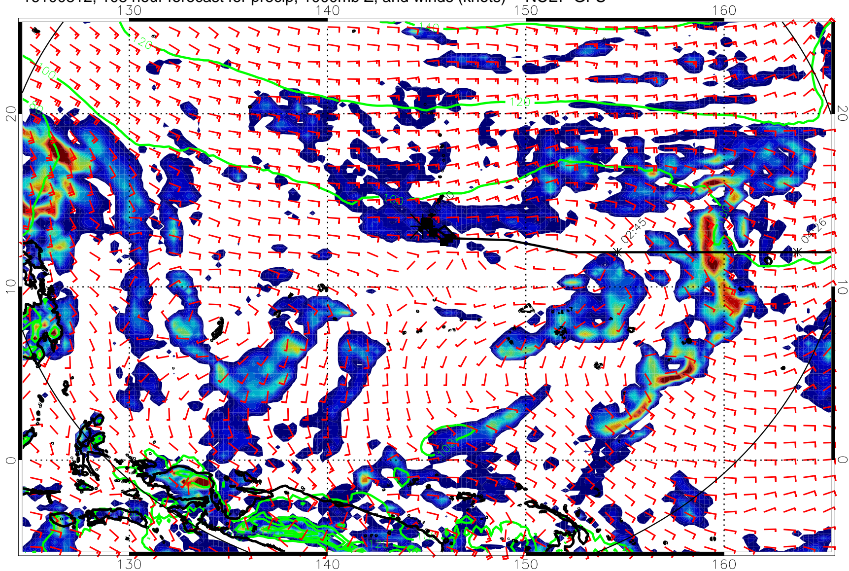
16100812, 108 hour forecast for precip, 1000mb Z, and winds (knots) -- NCEP GFS
