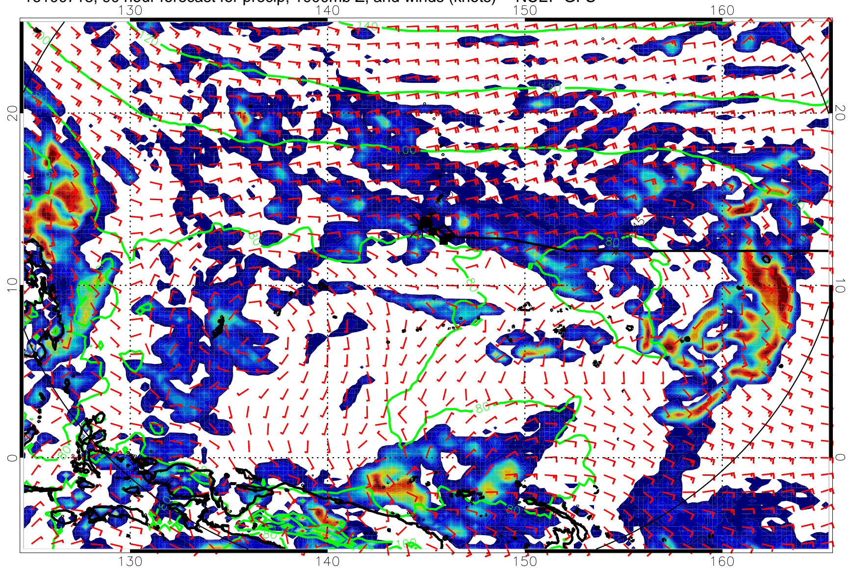
16100718, 90 hour forecast for precip, 1000mb Z, and winds (knots) -- NCEP GFS
