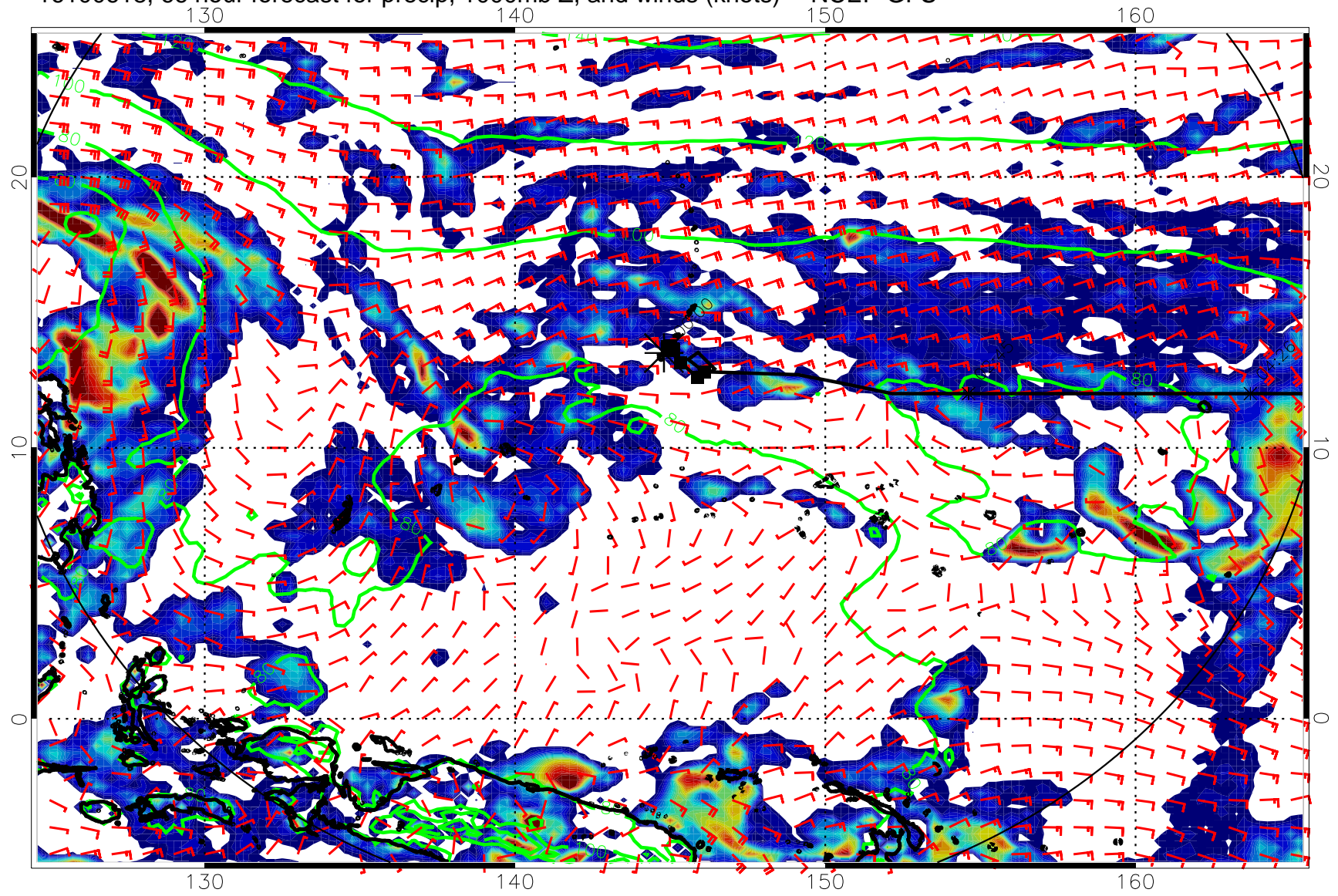
16100618, 66 hour forecast for precip, 1000mb Z, and winds (knots) -- NCEP GFS
