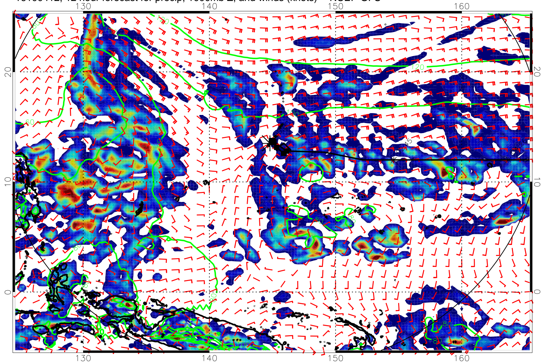
16100412, 12 hour forecast for precip, 1000mb Z, and winds (knots) -- NCEP GFS
