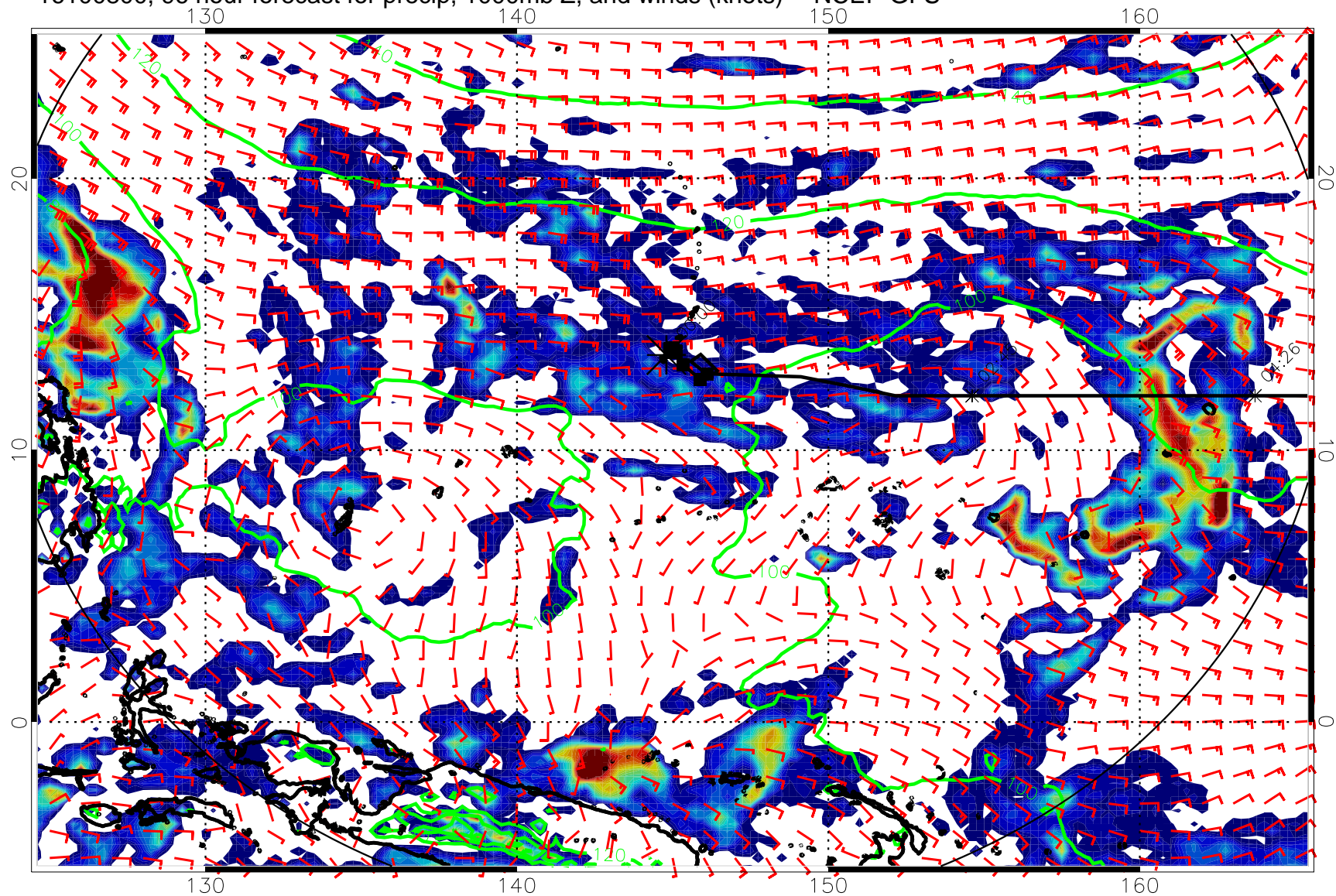
16100800, 96 hour forecast for precip, 1000mb Z, and winds (knots) -- NCEP GFS
