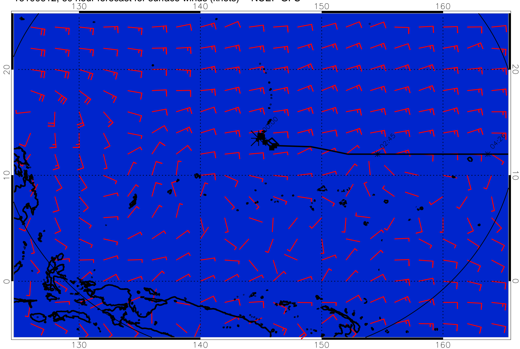
16100612, 60 hour forecast for surface winds (knots) -- NCEP GFS
