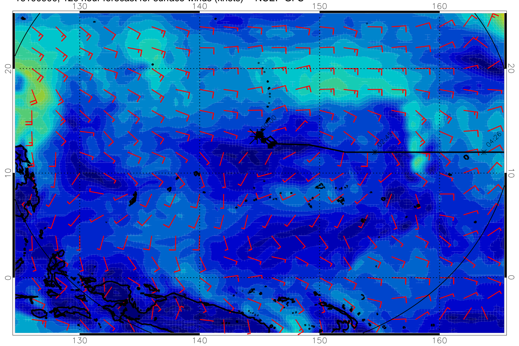
16100900, 120 hour forecast for surface winds (knots) -- NCEP GFS
