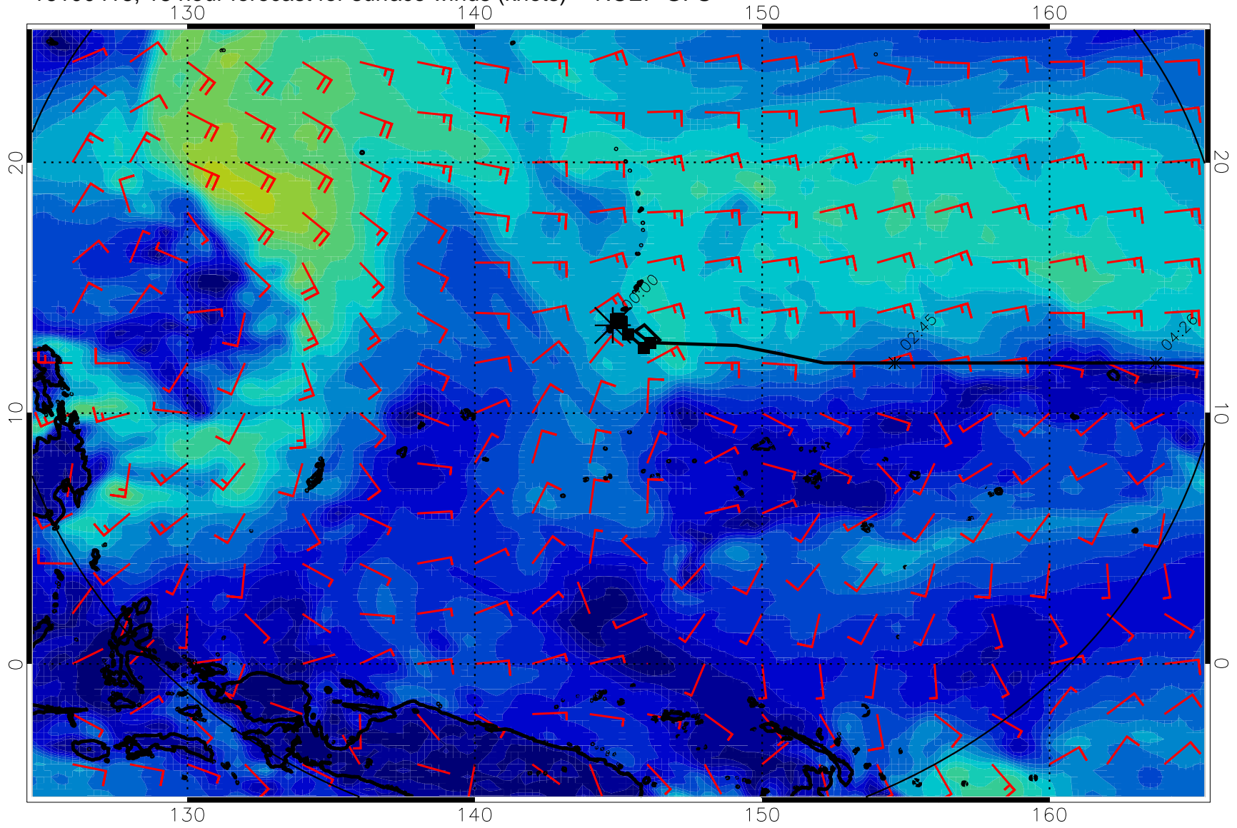
16100418, 18 hour forecast for surface winds (knots) -- NCEP GFS
