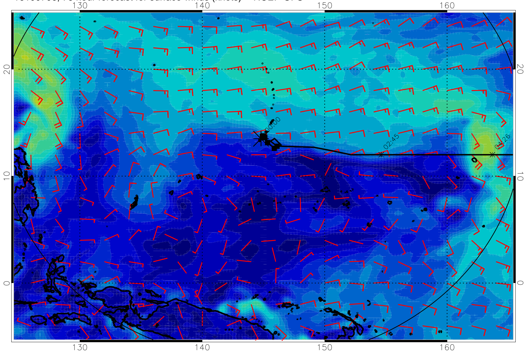
16100706, 78 hour forecast for surface winds (knots) -- NCEP GFS
