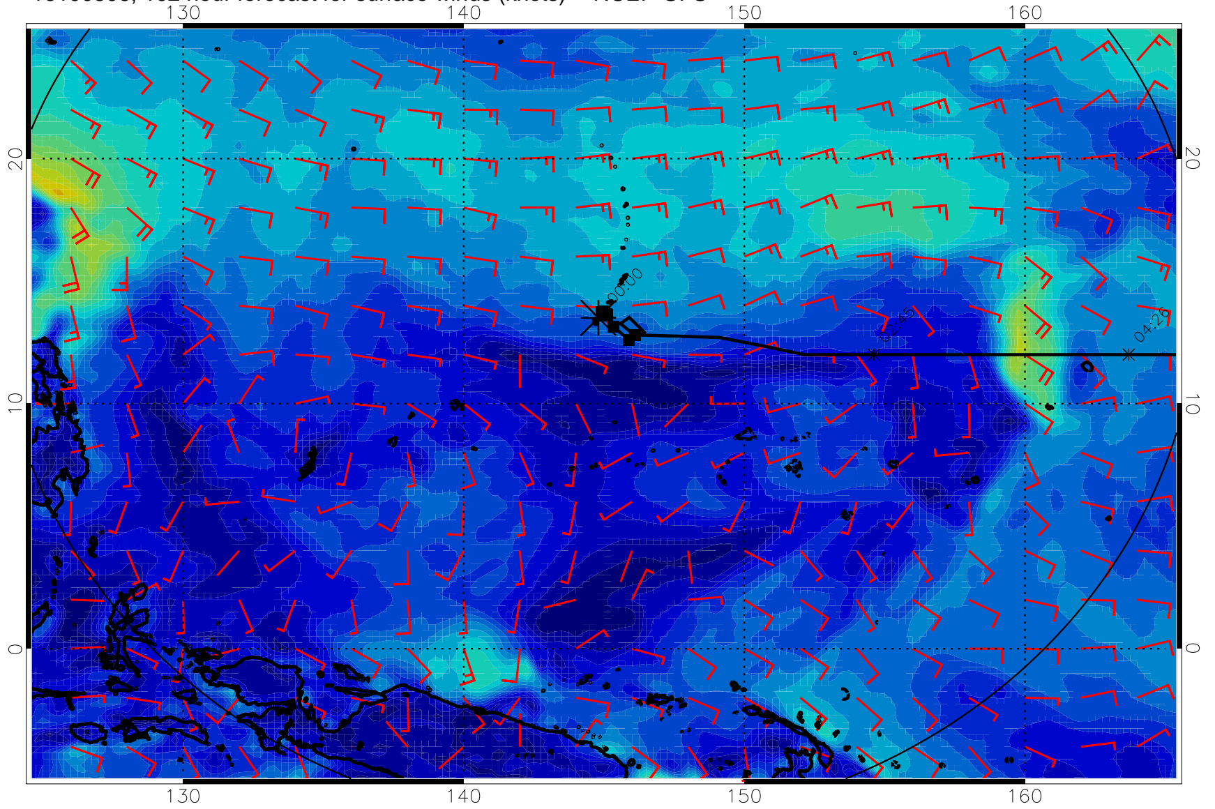
16100806, 102 hour forecast for surface winds (knots) -- NCEP GFS
