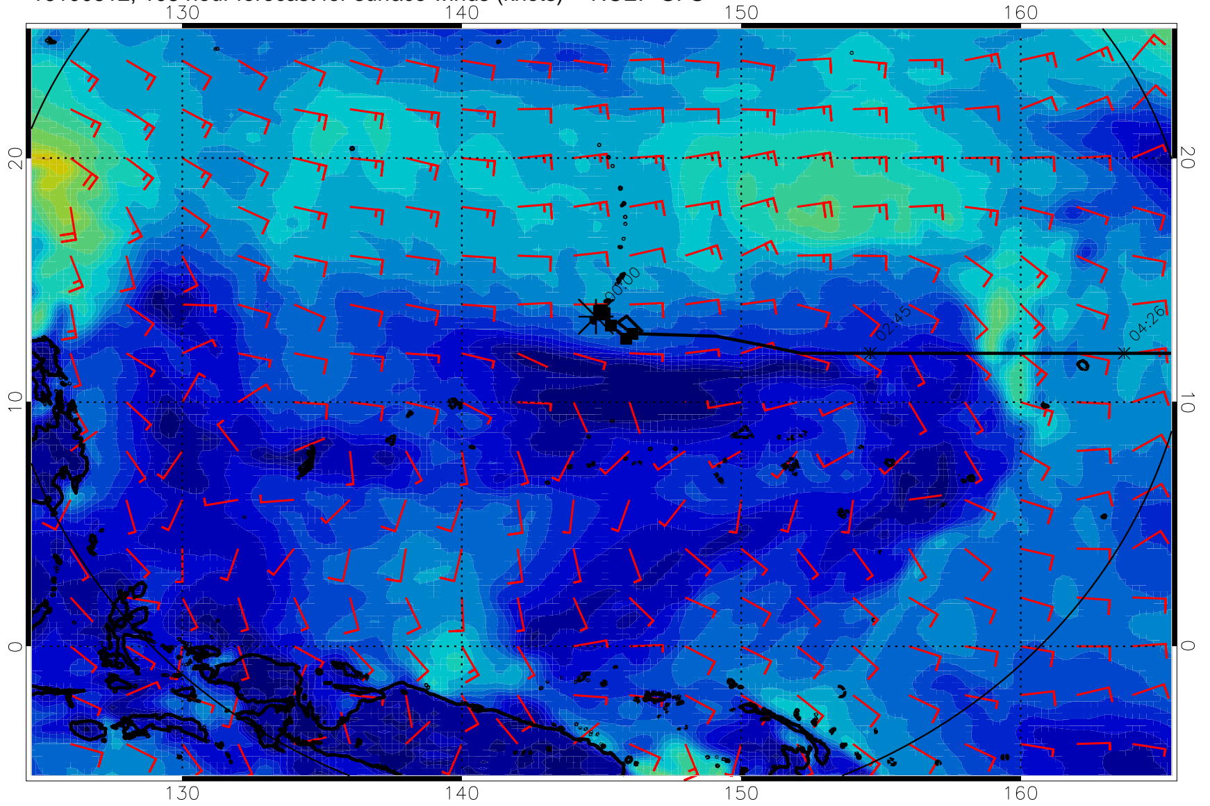
16100812, 108 hour forecast for surface winds (knots) -- NCEP GFS
