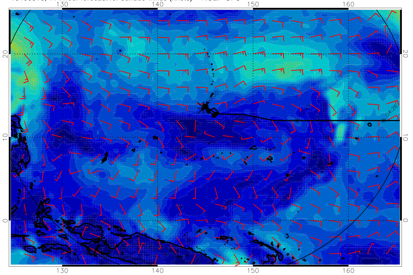
16100818, 114 hour forecast for surface winds (knots) -- NCEP GFS
