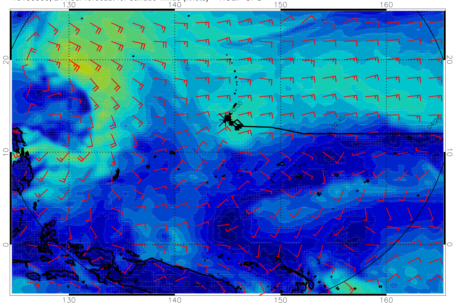
16100500, 24 hour forecast for surface winds (knots) -- NCEP GFS
