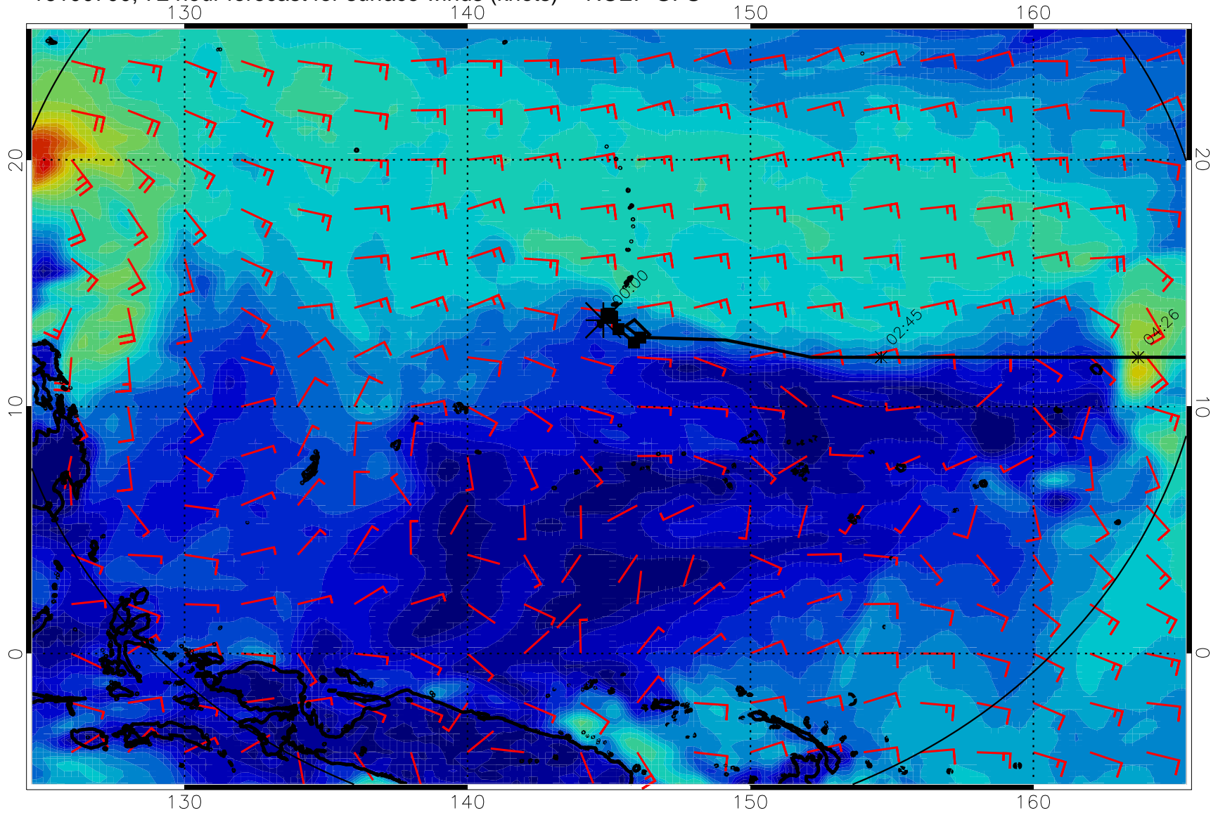
16100700, 72 hour forecast for surface winds (knots) -- NCEP GFS
