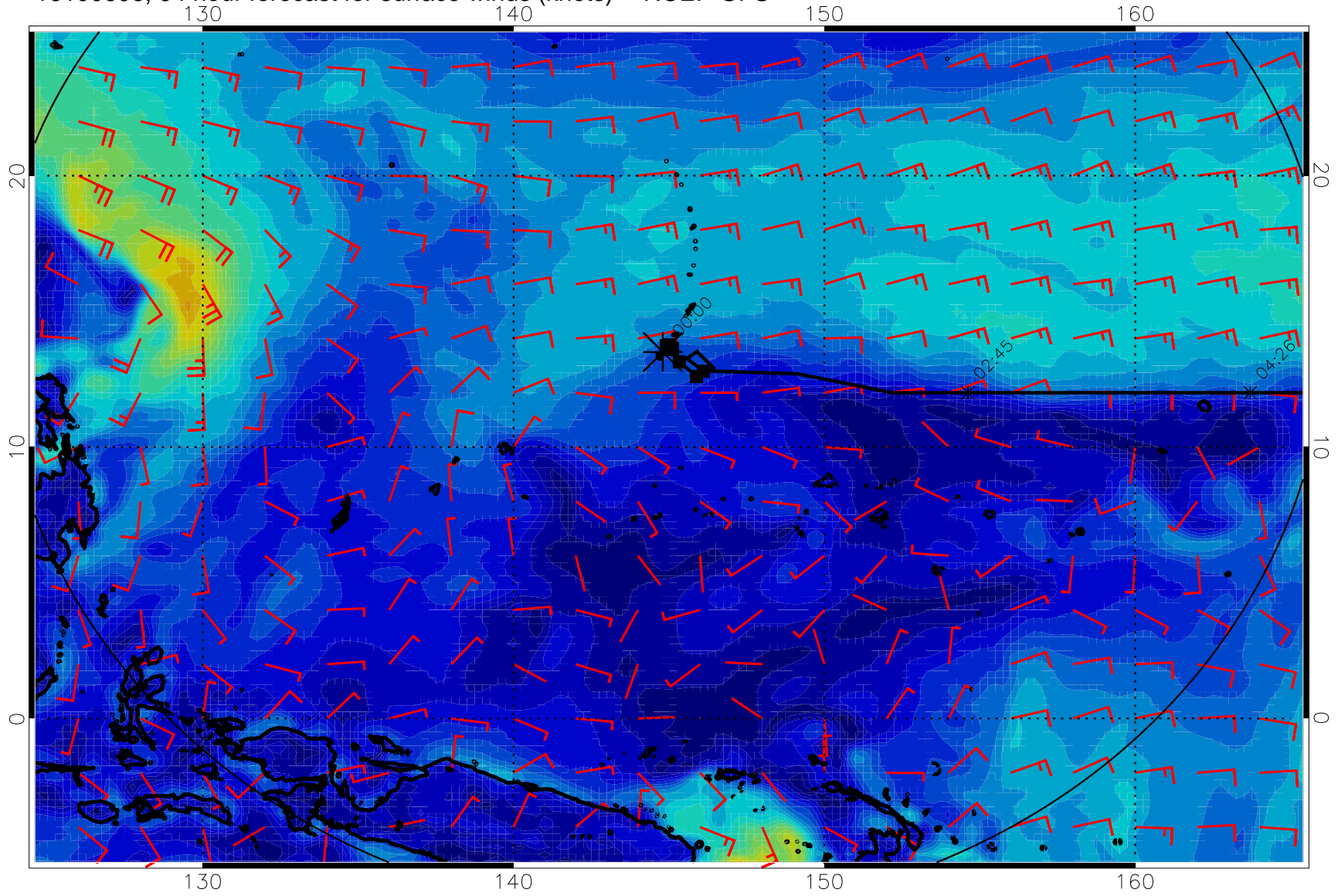
16100606, 54 hour forecast for surface winds (knots) -- NCEP GFS
