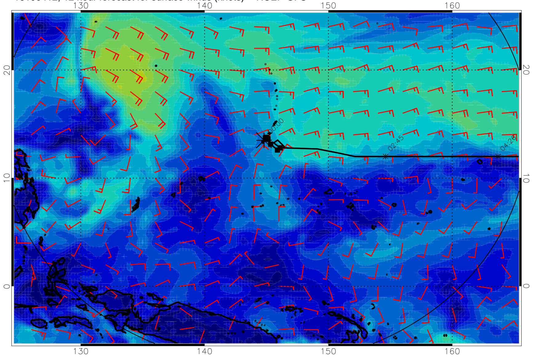
16100412, 12 hour forecast for surface winds (knots) -- NCEP GFS
