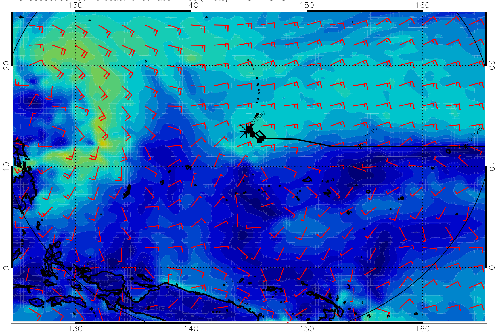
16100506, 30 hour forecast for surface winds (knots) -- NCEP GFS
