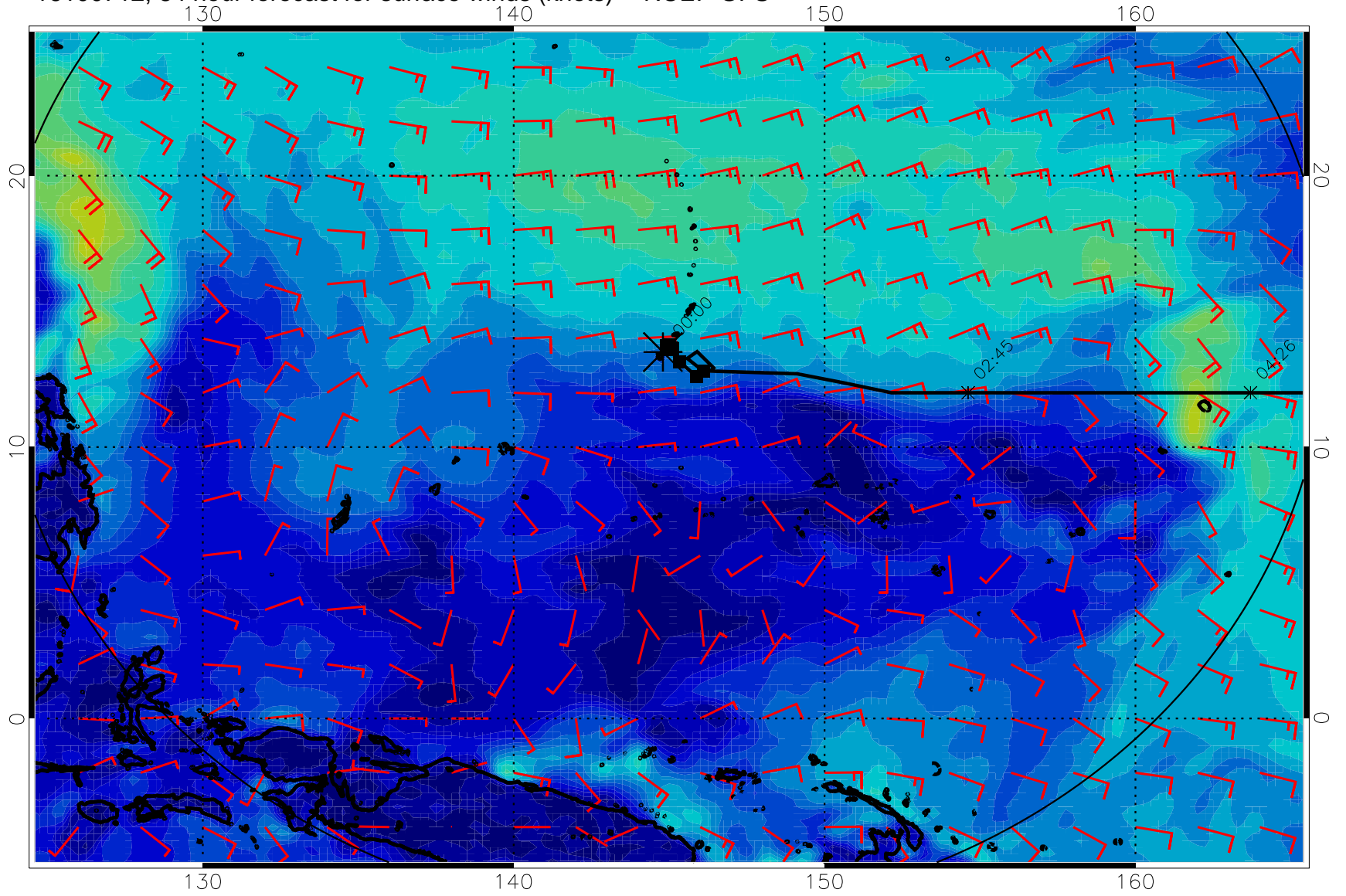
16100712, 84 hour forecast for surface winds (knots) -- NCEP GFS
