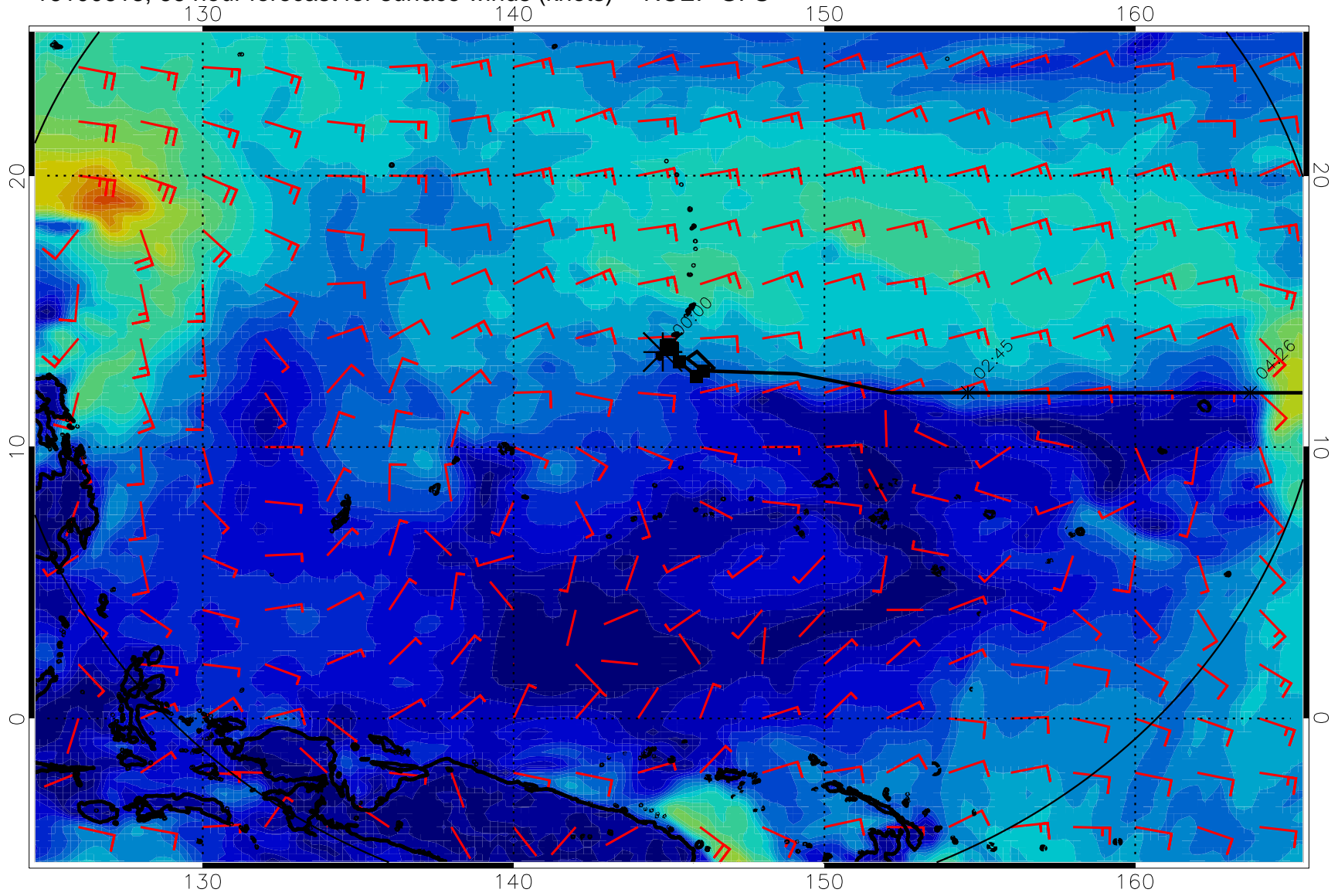
16100618, 66 hour forecast for surface winds (knots) -- NCEP GFS
