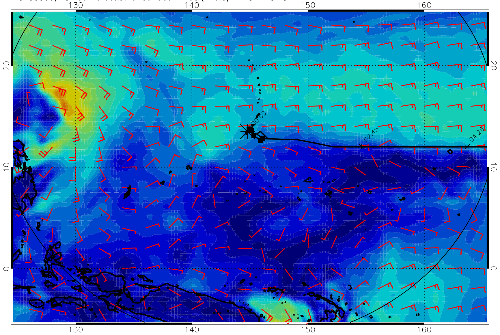
16100600, 48 hour forecast for surface winds (knots) -- NCEP GFS
