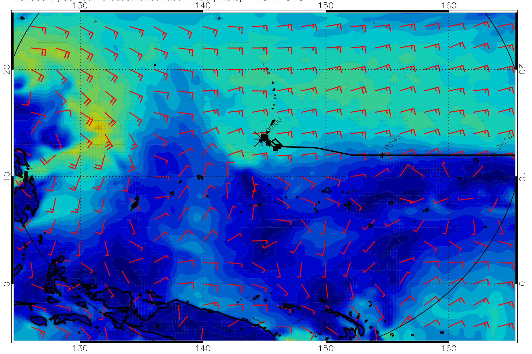
16100512, 36 hour forecast for surface winds (knots) -- NCEP GFS
