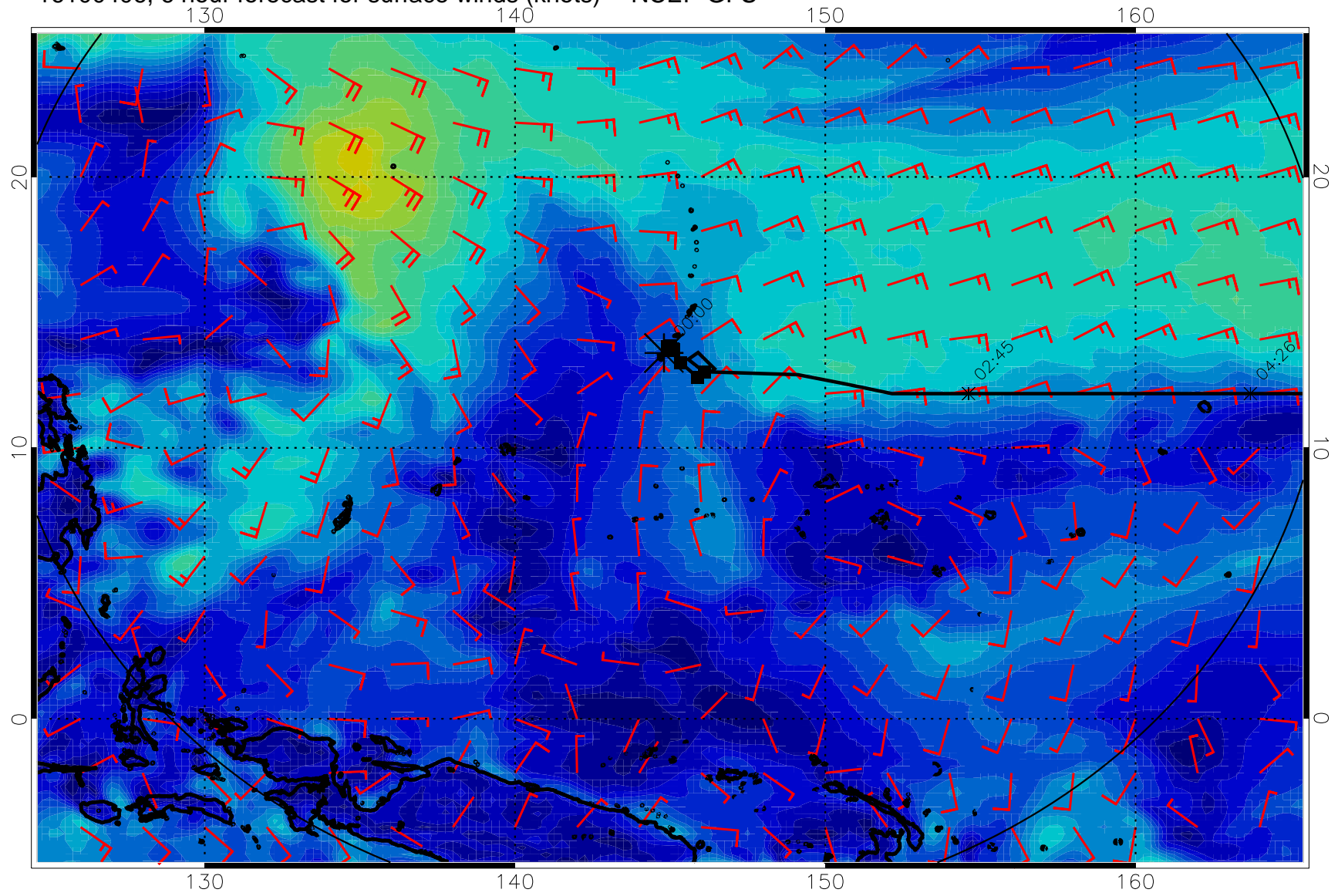
16100406, 6 hour forecast for surface winds (knots) -- NCEP GFS
