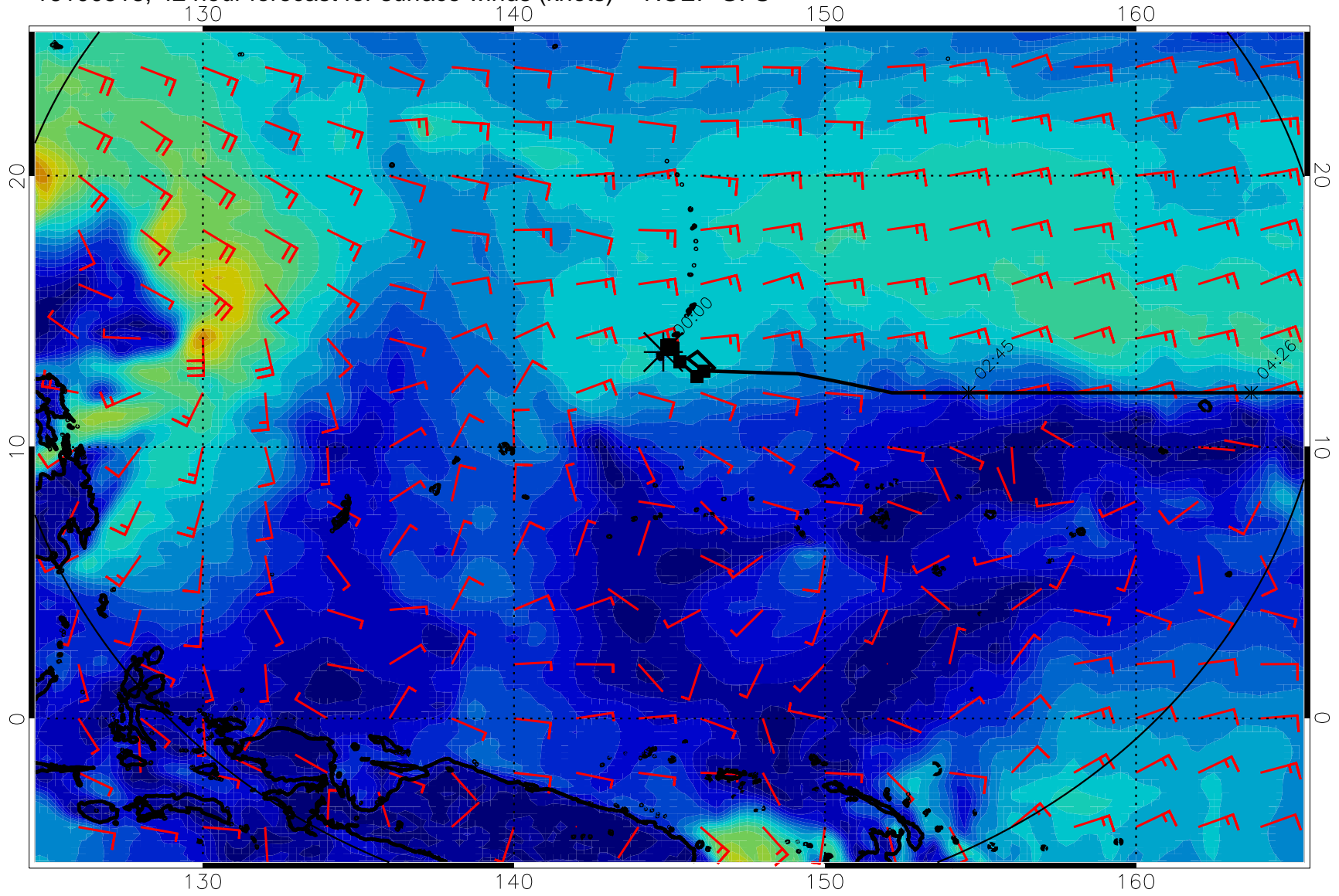
16100518, 42 hour forecast for surface winds (knots) -- NCEP GFS
