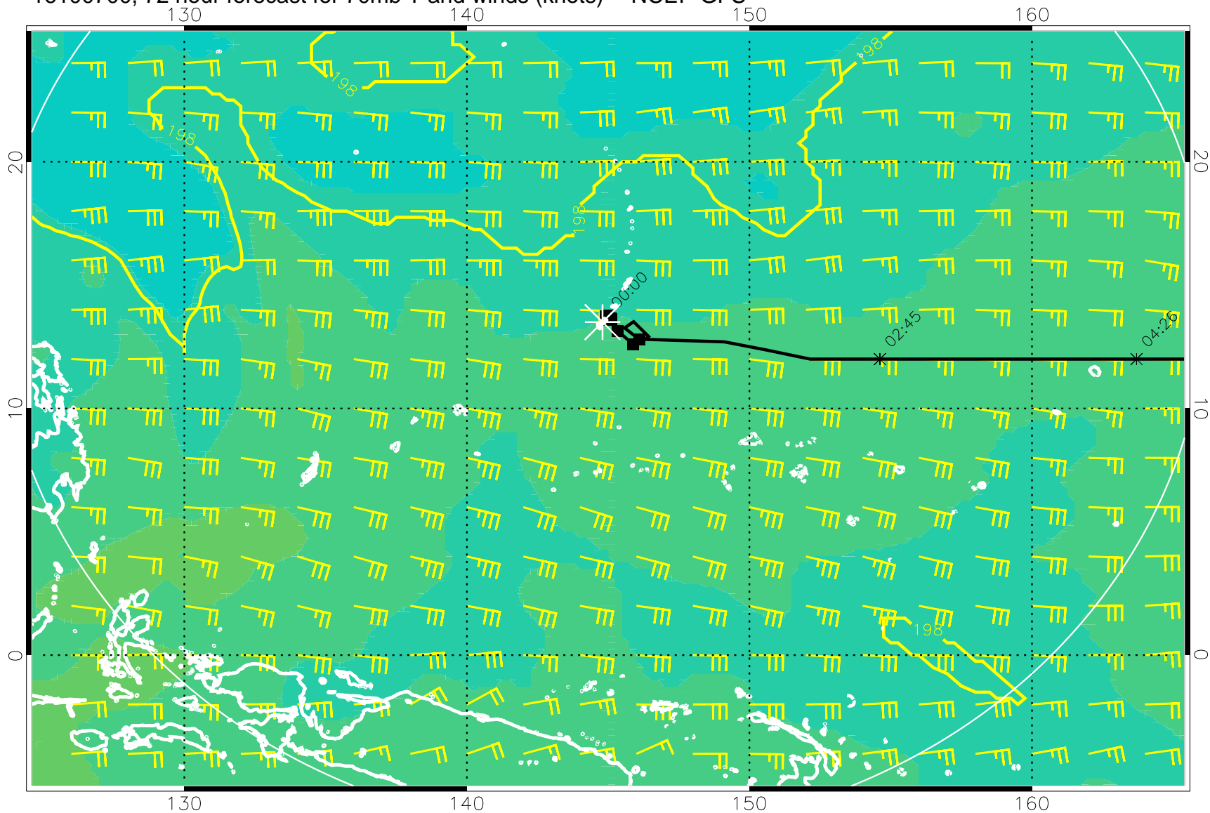
16100700, 72 hour forecast for 70mb T and winds (knots) -- NCEP GFS
