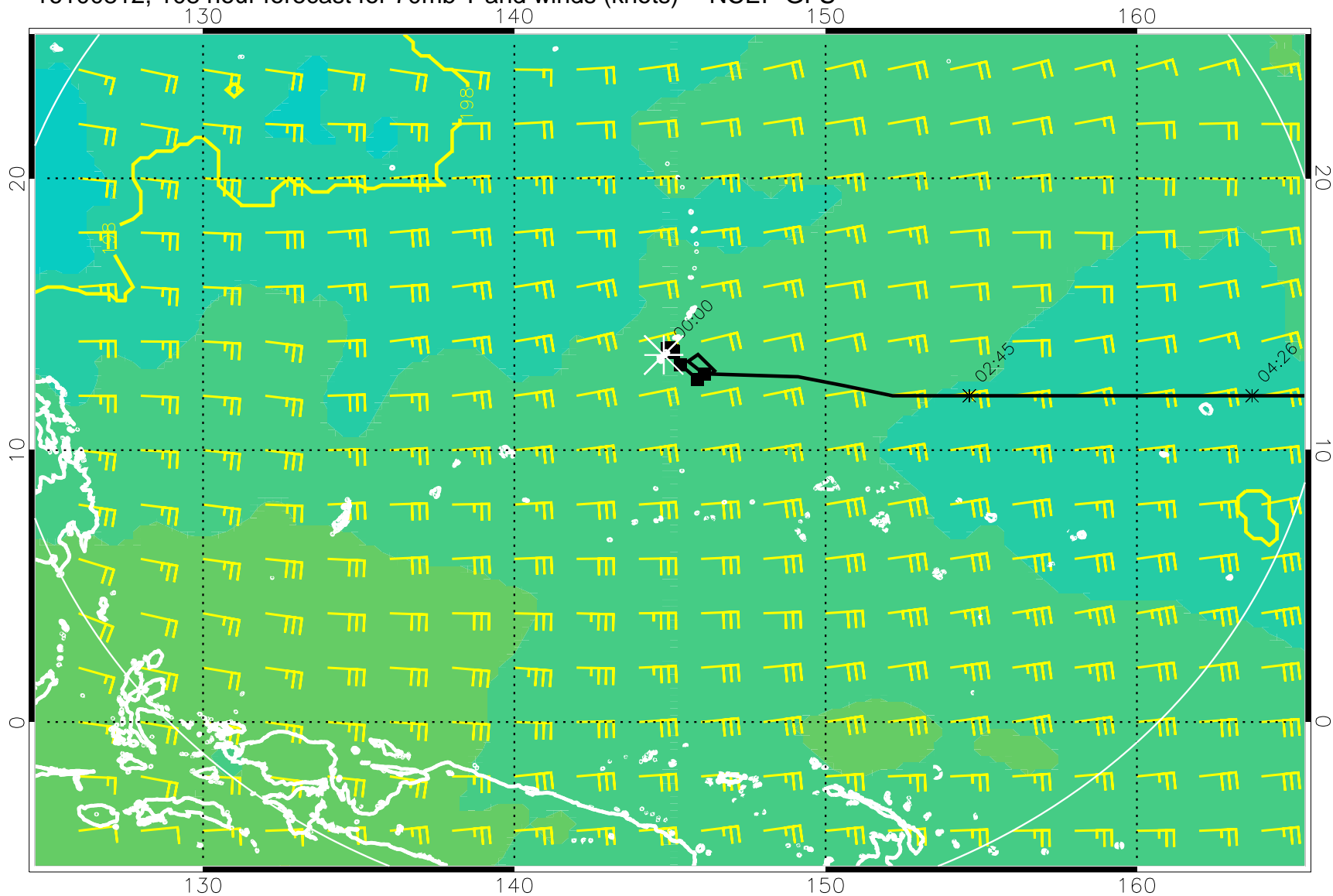
16100812, 108 hour forecast for 70mb T and winds (knots) -- NCEP GFS
