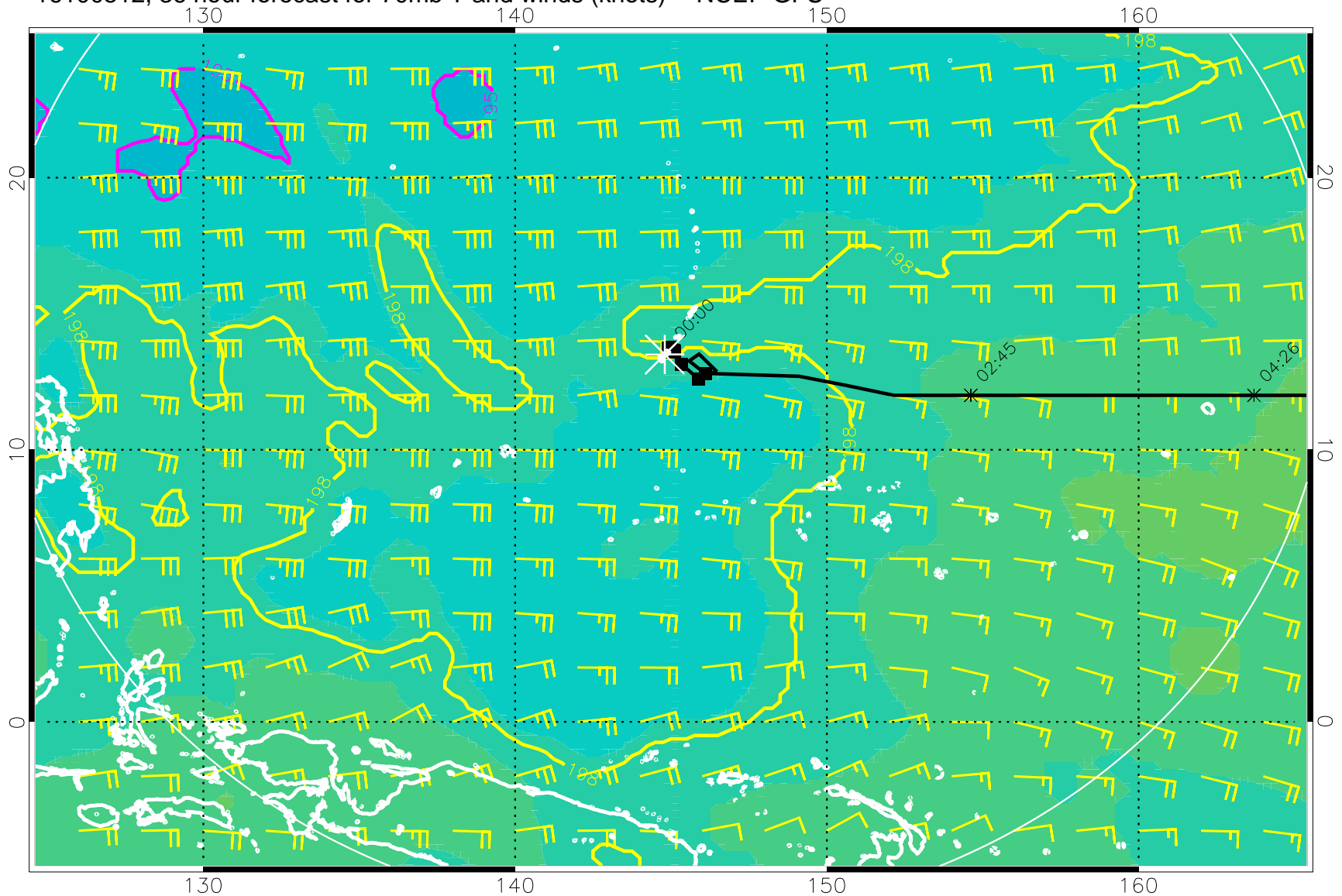
16100512, 36 hour forecast for 70mb T and winds (knots) -- NCEP GFS
