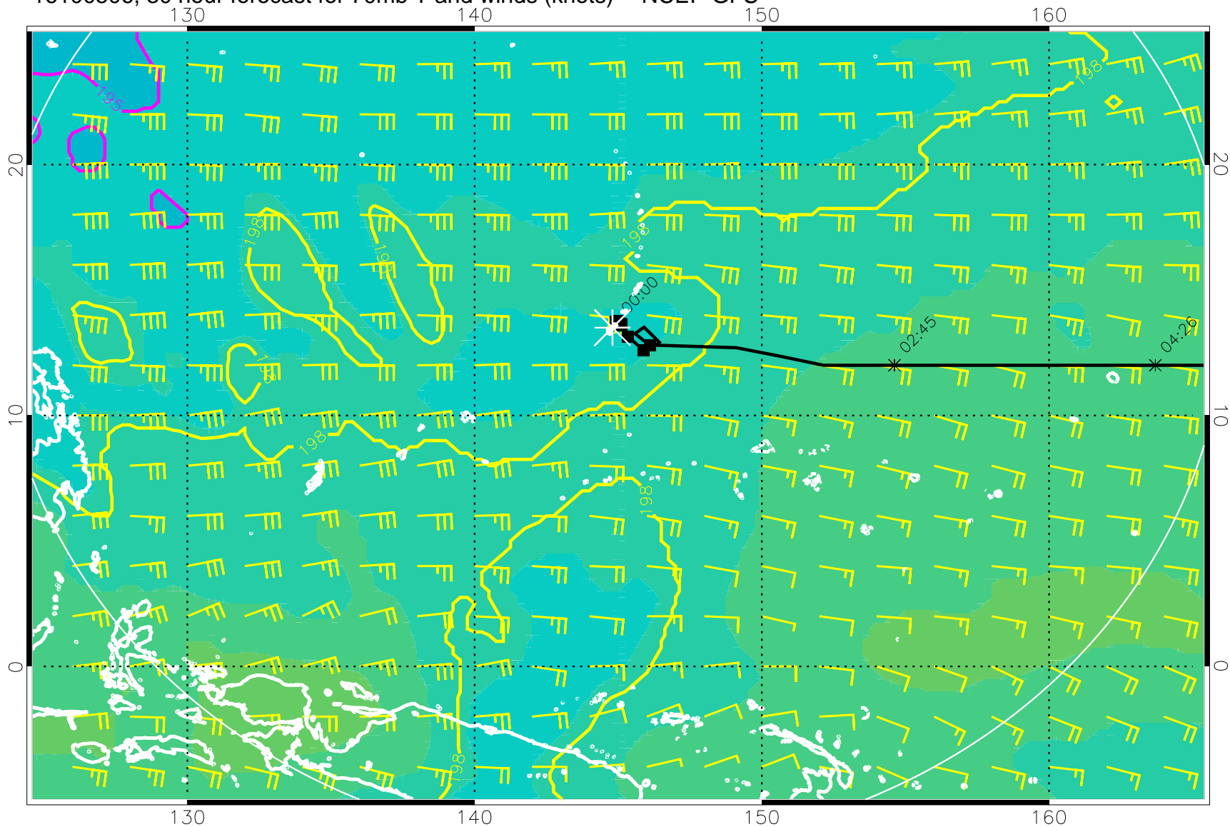
16100506, 30 hour forecast for 70mb T and winds (knots) -- NCEP GFS
