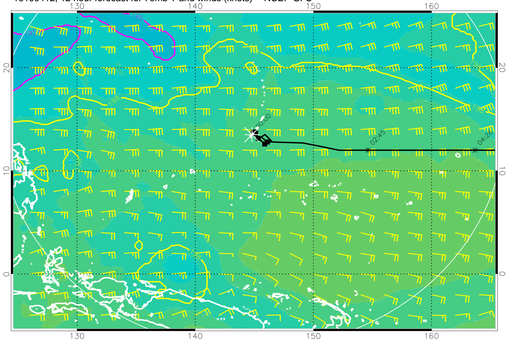
16100412, 12 hour forecast for 70mb T and winds (knots) -- NCEP GFS
