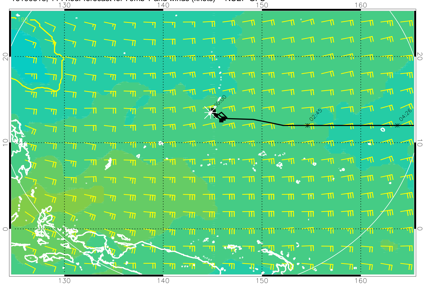
16100818, 114 hour forecast for 70mb T and winds (knots) -- NCEP GFS
