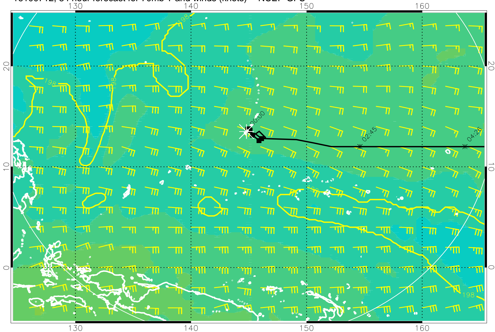
16100712, 84 hour forecast for 70mb T and winds (knots) -- NCEP GFS
