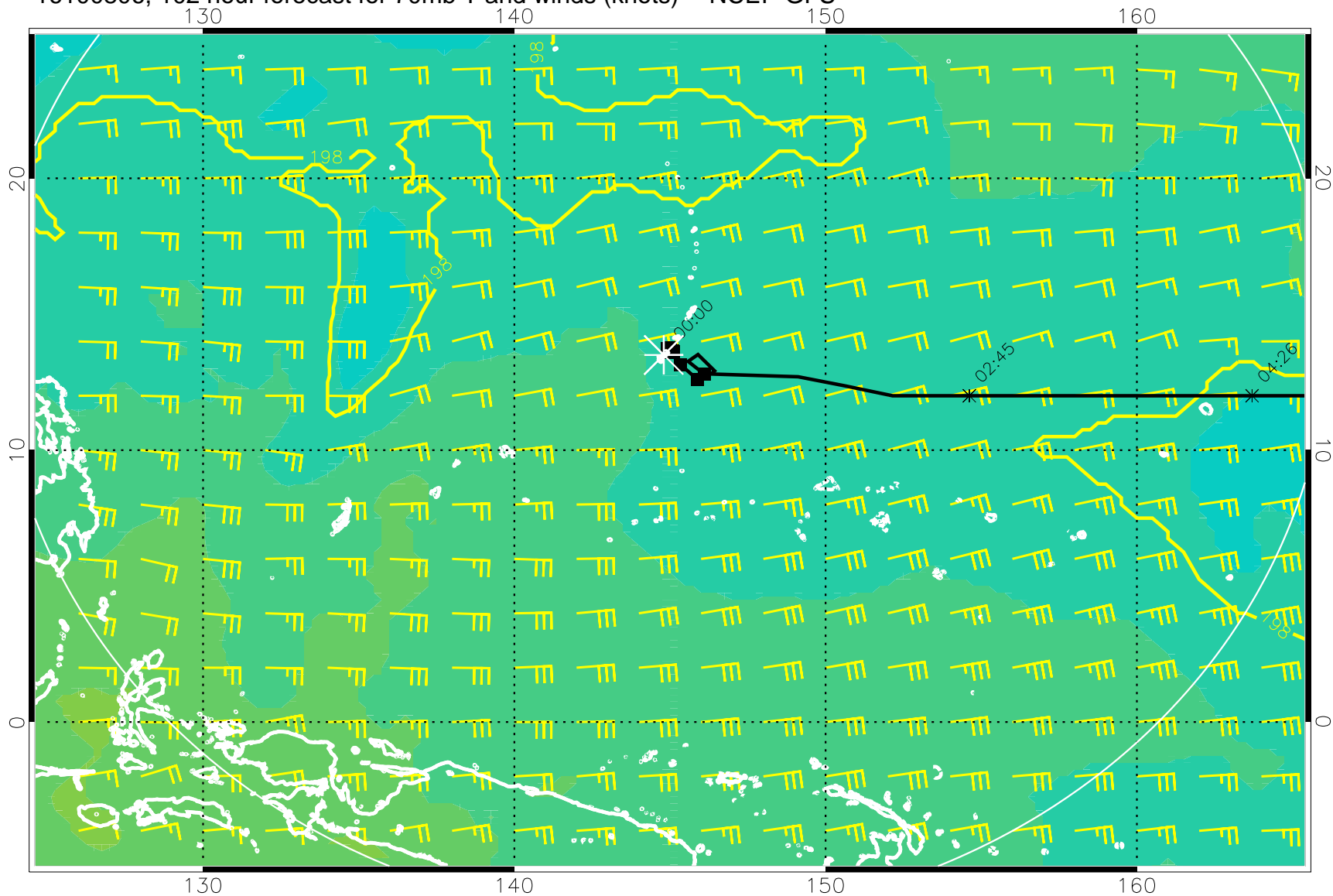
16100806, 102 hour forecast for 70mb T and winds (knots) -- NCEP GFS
