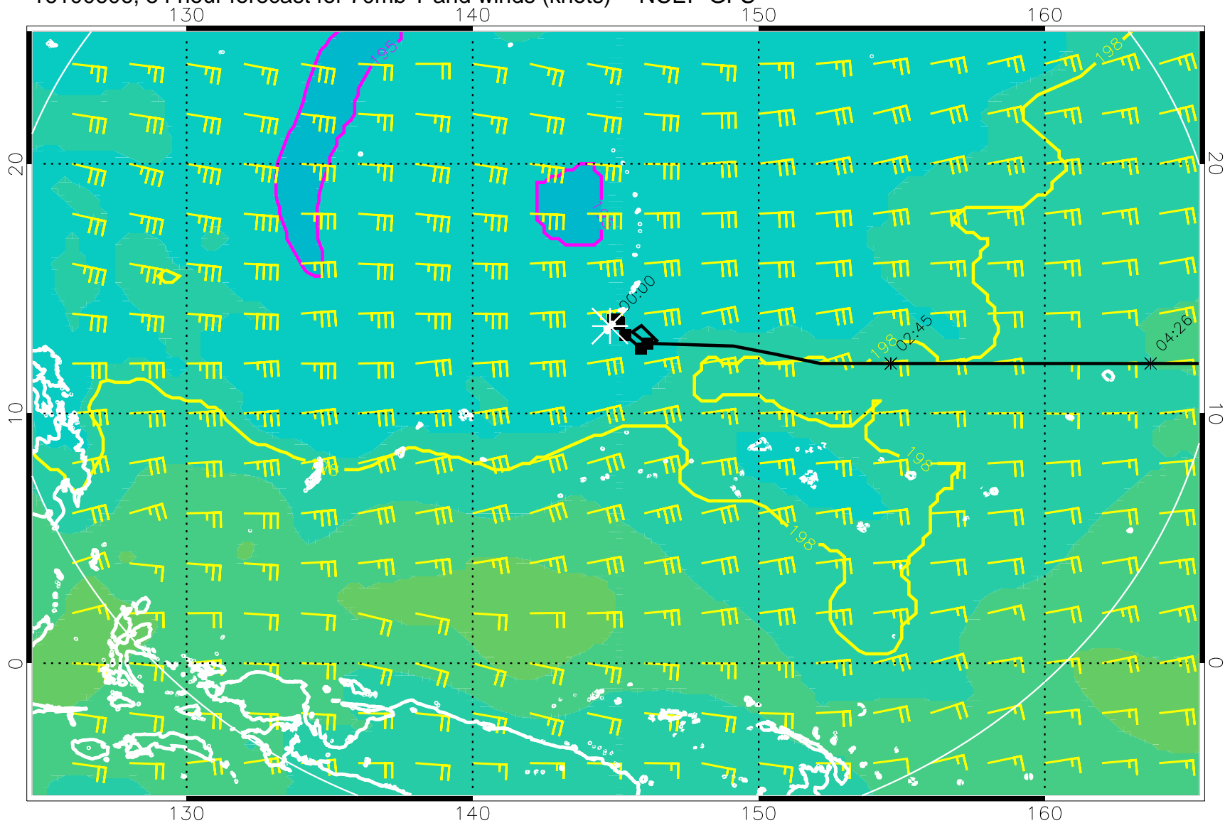
16100606, 54 hour forecast for 70mb T and winds (knots) -- NCEP GFS
