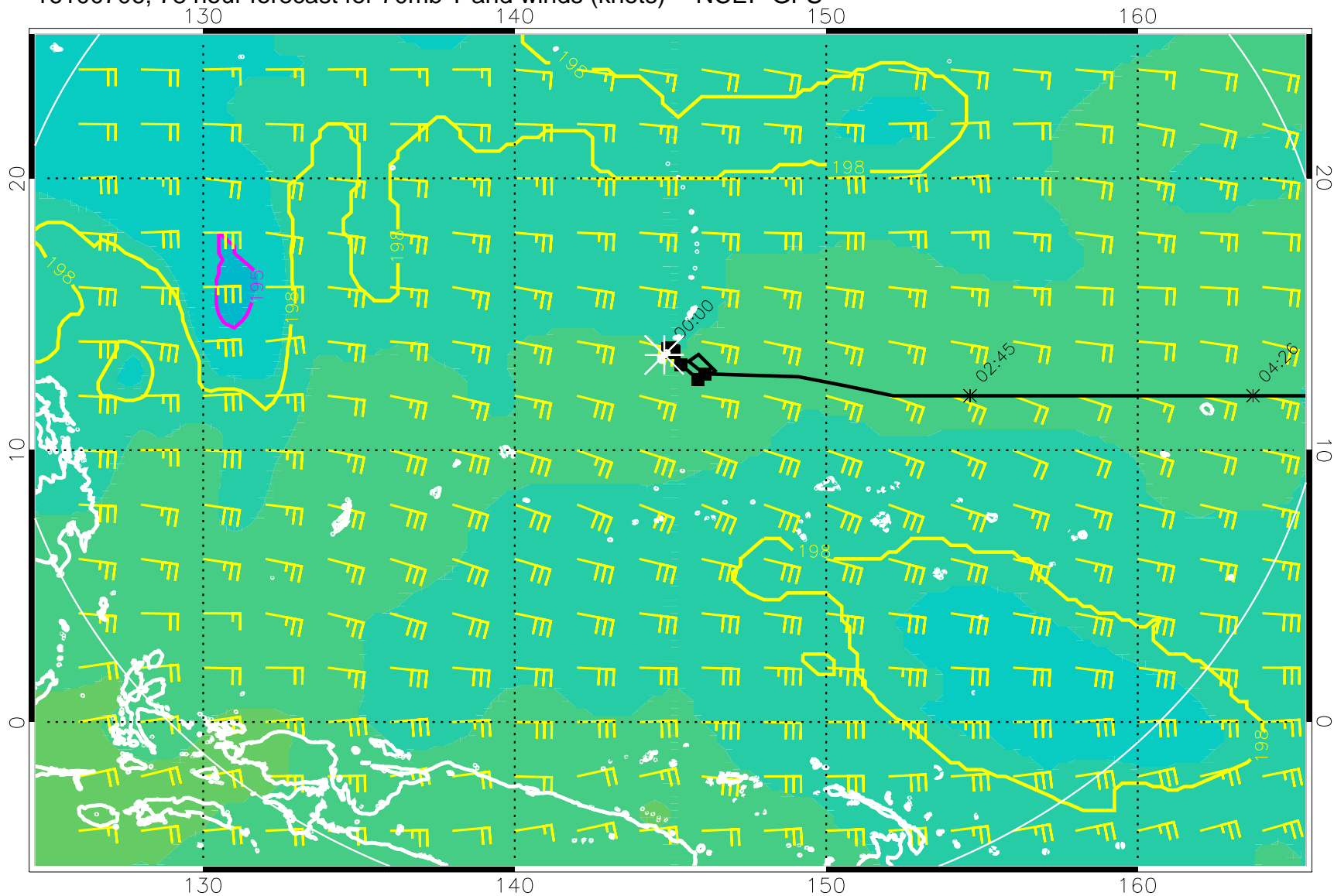
16100706, 78 hour forecast for 70mb T and winds (knots) -- NCEP GFS
