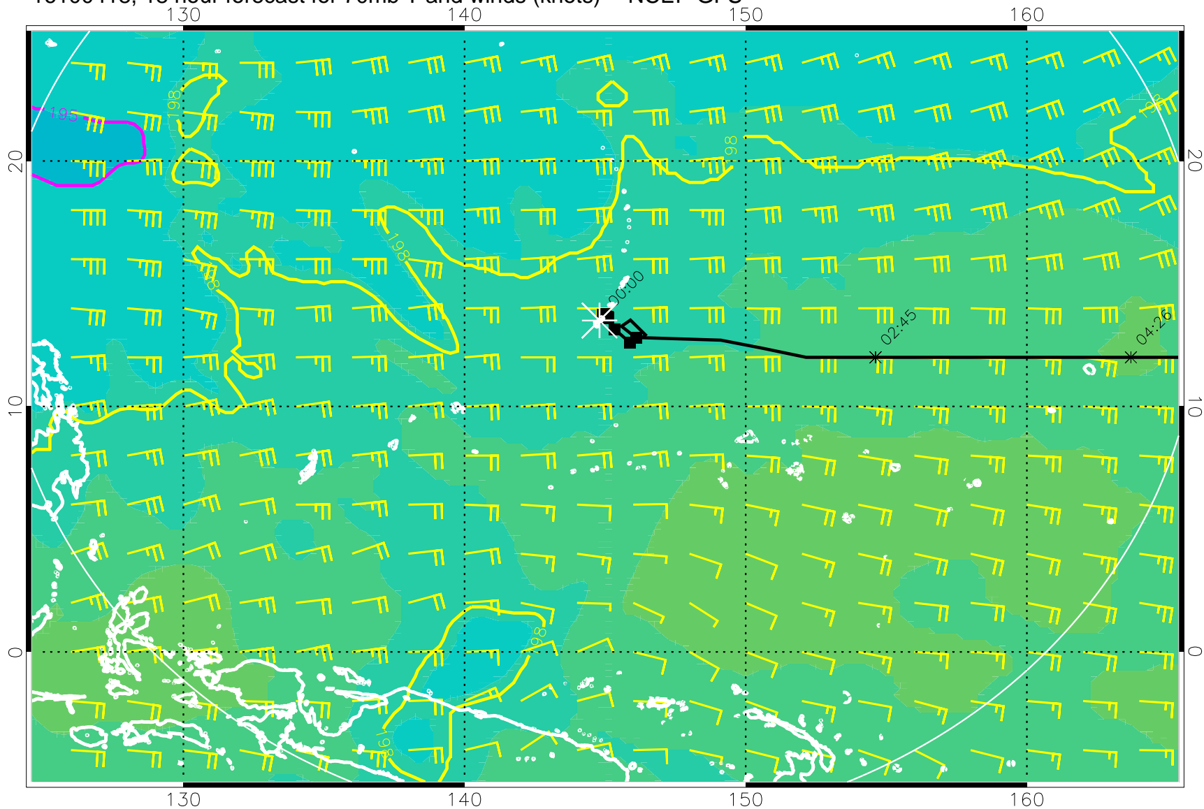
16100418, 18 hour forecast for 70mb T and winds (knots) -- NCEP GFS
