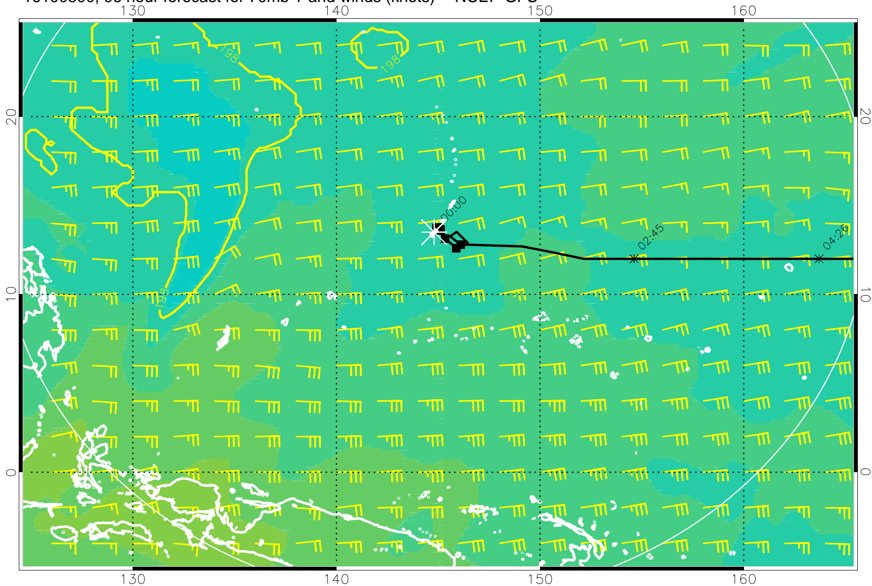
16100800, 96 hour forecast for 70mb T and winds (knots) -- NCEP GFS
