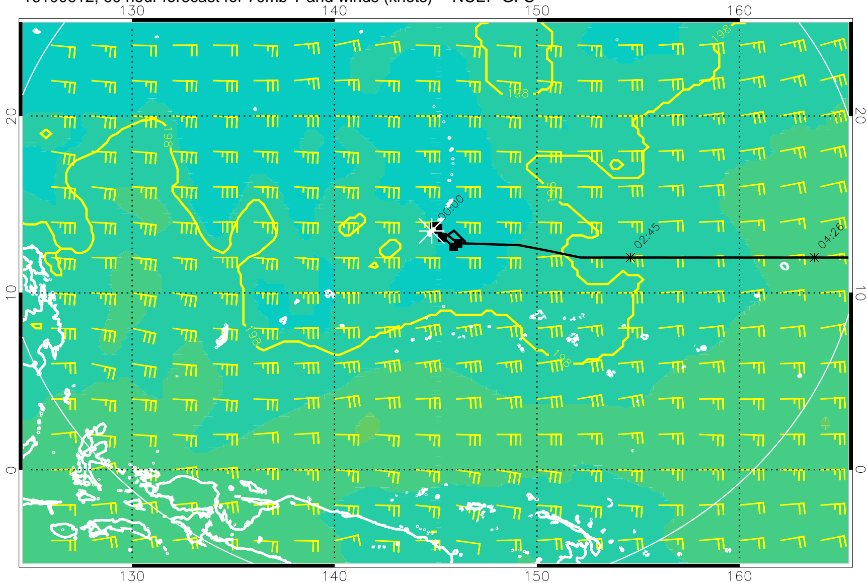
16100612, 60 hour forecast for 70mb T and winds (knots) -- NCEP GFS
