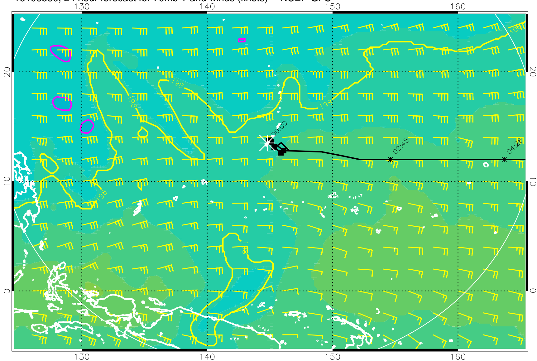
16100500, 24 hour forecast for 70mb T and winds (knots) -- NCEP GFS
