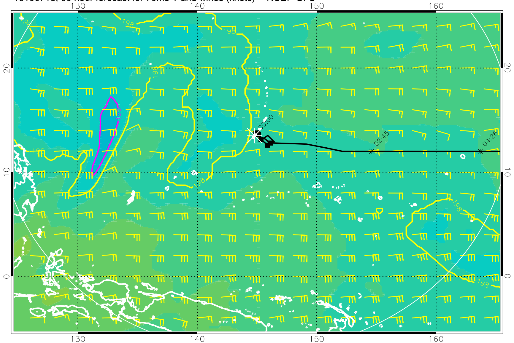
16100718, 90 hour forecast for 70mb T and winds (knots) -- NCEP GFS
