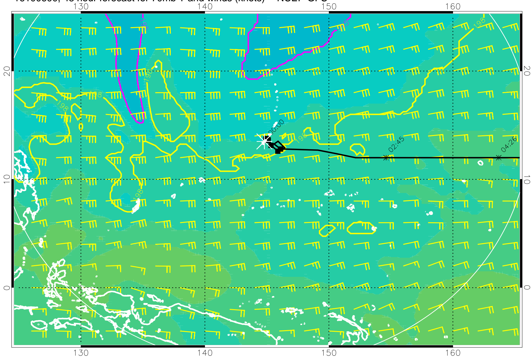
16100600, 48 hour forecast for 70mb T and winds (knots) -- NCEP GFS
