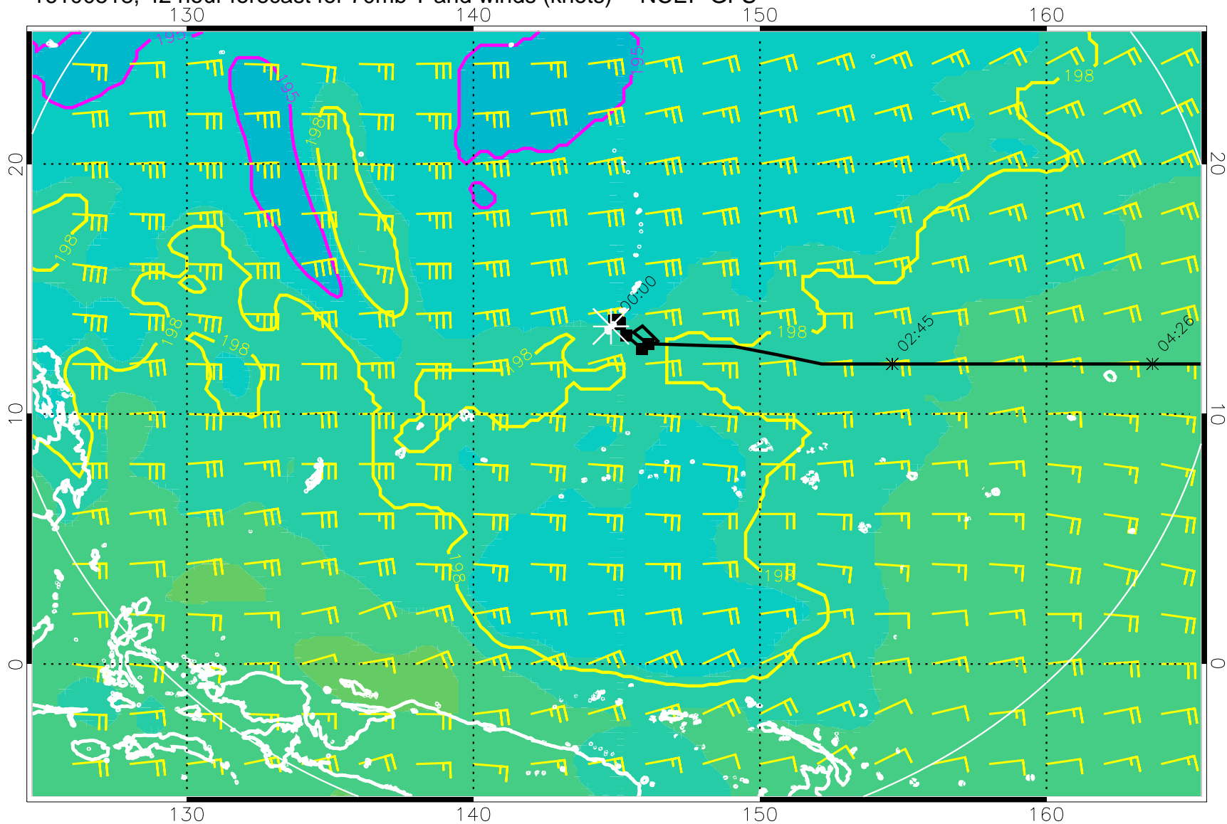
16100518, 42 hour forecast for 70mb T and winds (knots) -- NCEP GFS
