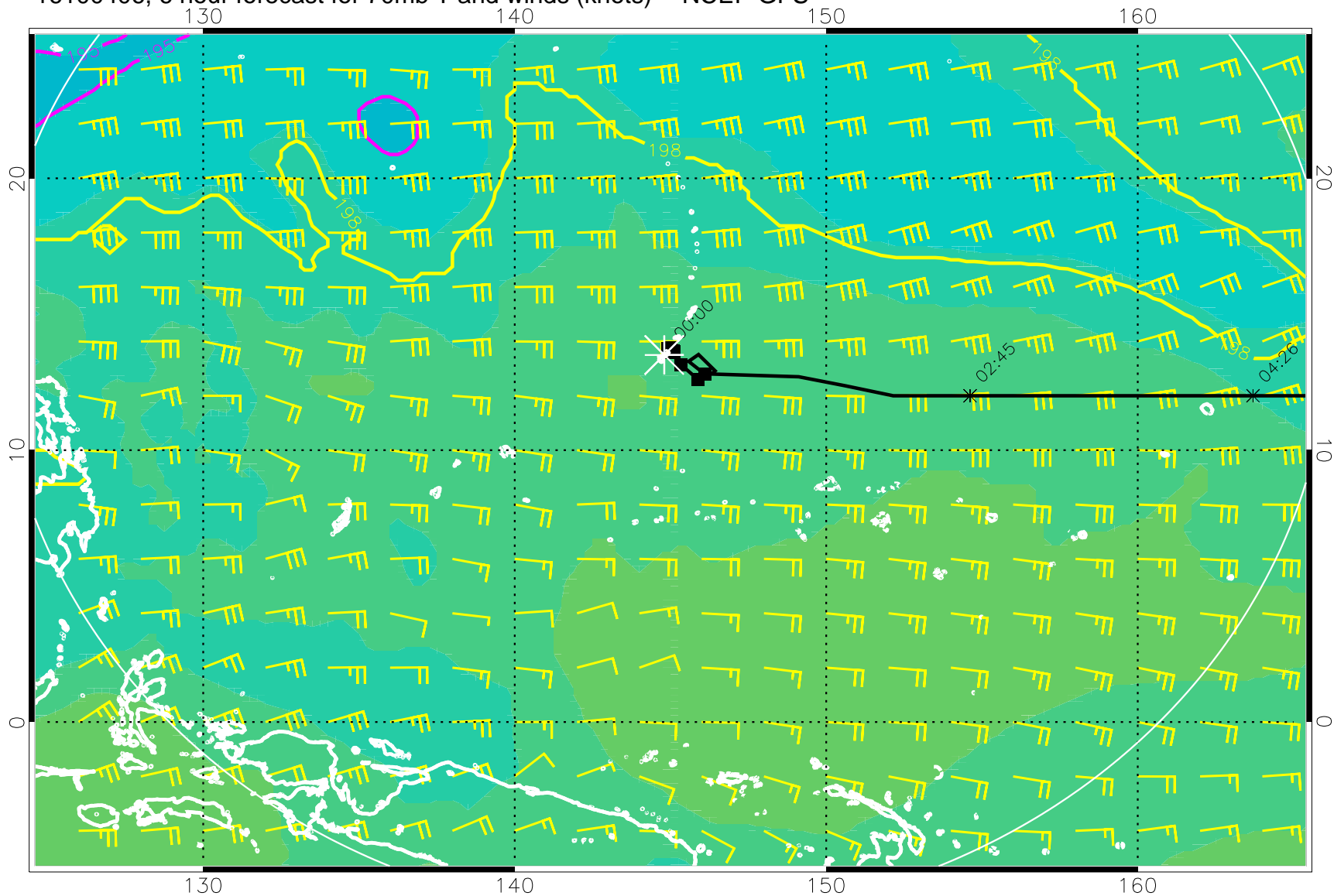
16100406, 6 hour forecast for 70mb T and winds (knots) -- NCEP GFS
