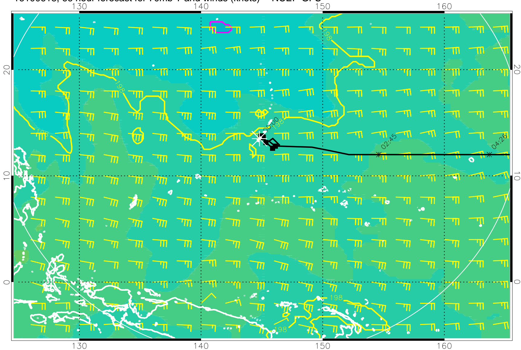
16100618, 66 hour forecast for 70mb T and winds (knots) -- NCEP GFS
