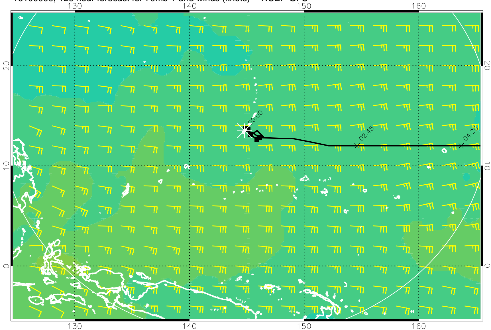
161100900, 120 hour forecast for 70mb T and winds (knots) -- NCEP GFS
