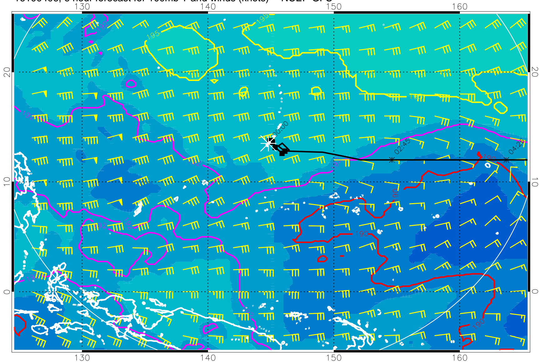
16100406, 6 hour forecast for 100mb T and winds (knots) -- NCEP GFS
