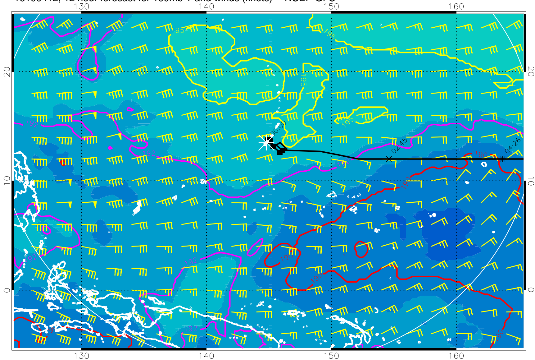
16100412, 12 hour forecast for 100mb T and winds (knots) -- NCEP GFS
