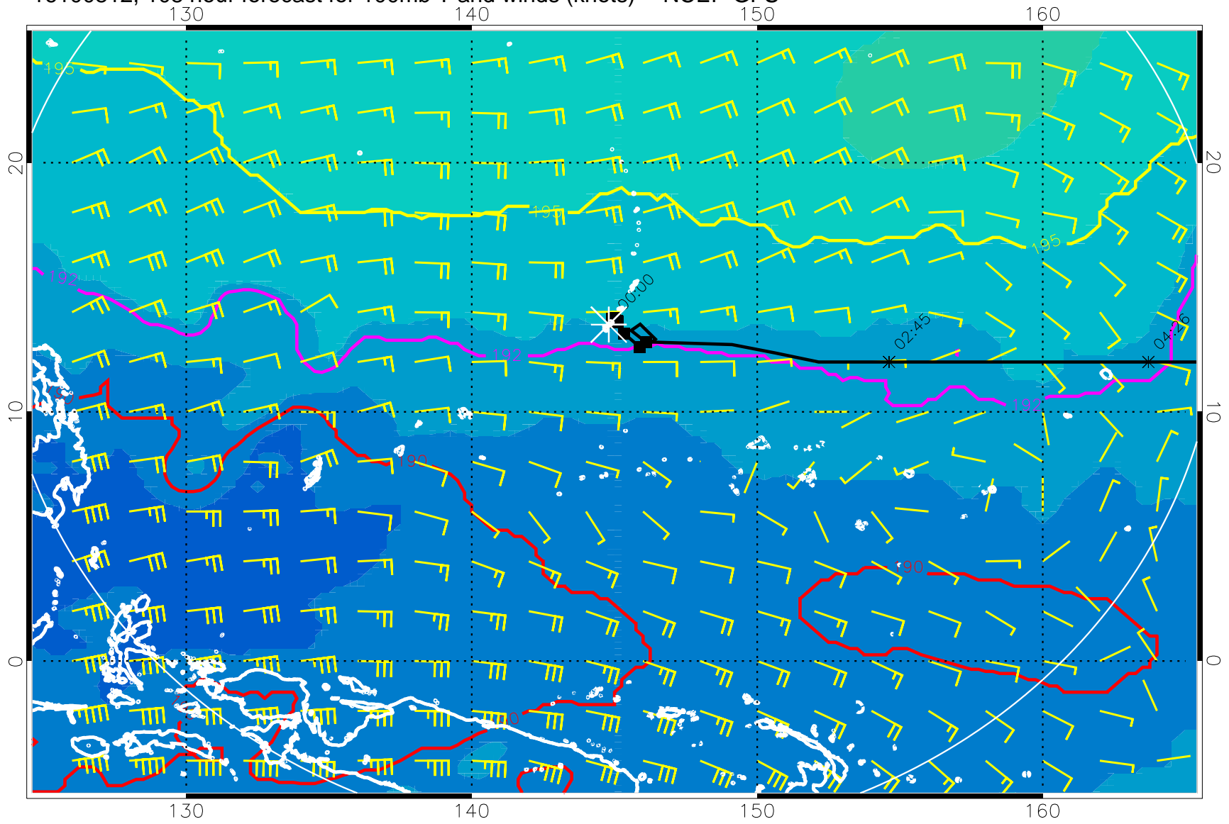
16100812, 108 hour forecast for 100mb T and winds (knots) -- NCEP GFS
