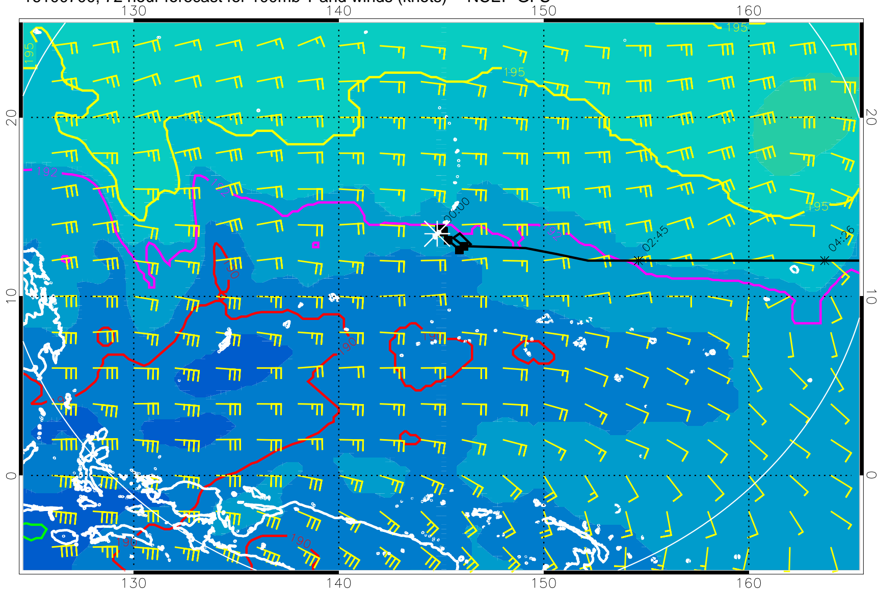
16100700, 72 hour forecast for 100mb T and winds (knots) -- NCEP GFS
