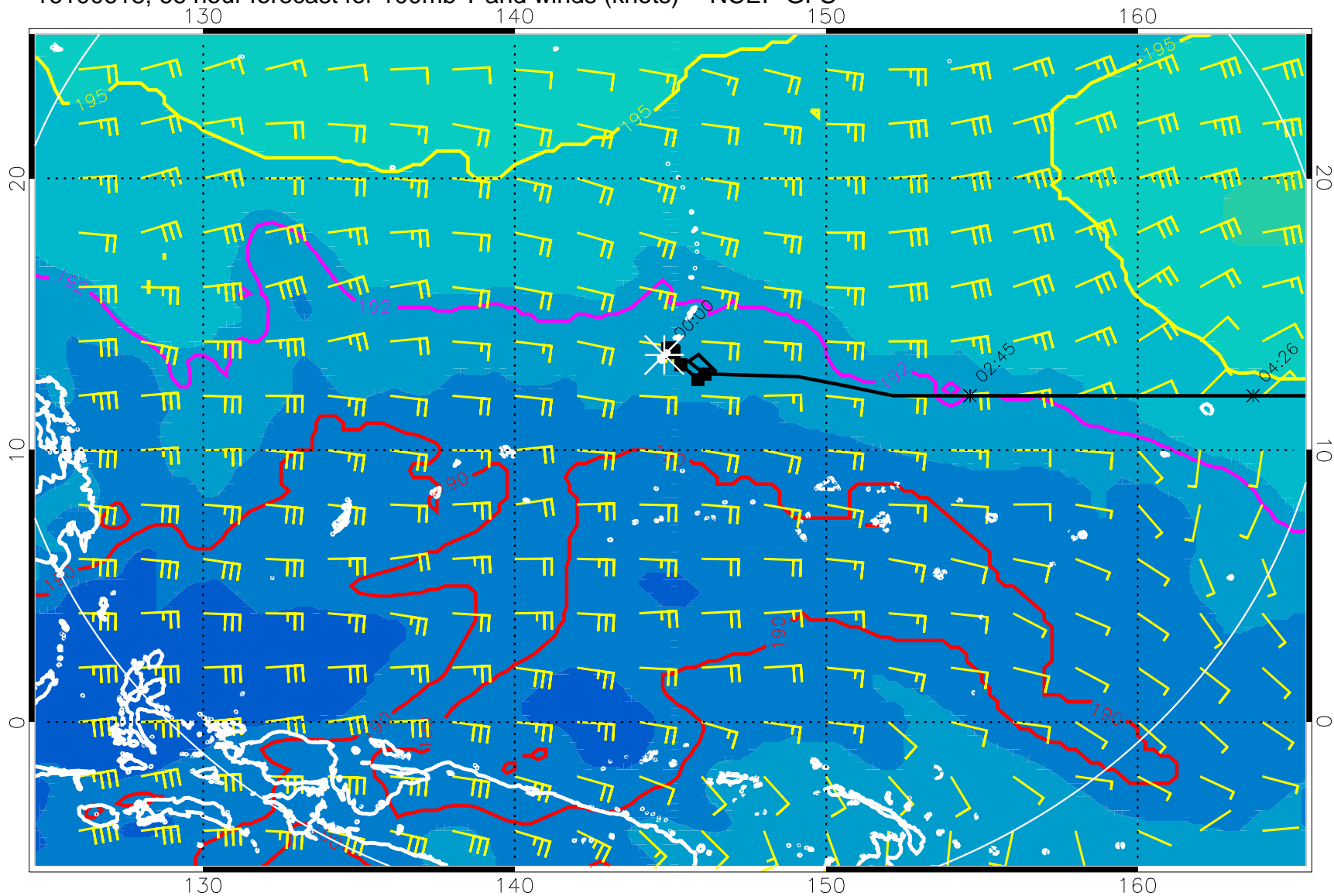
16100618, 66 hour forecast for 100mb T and winds (knots) -- NCEP GFS
