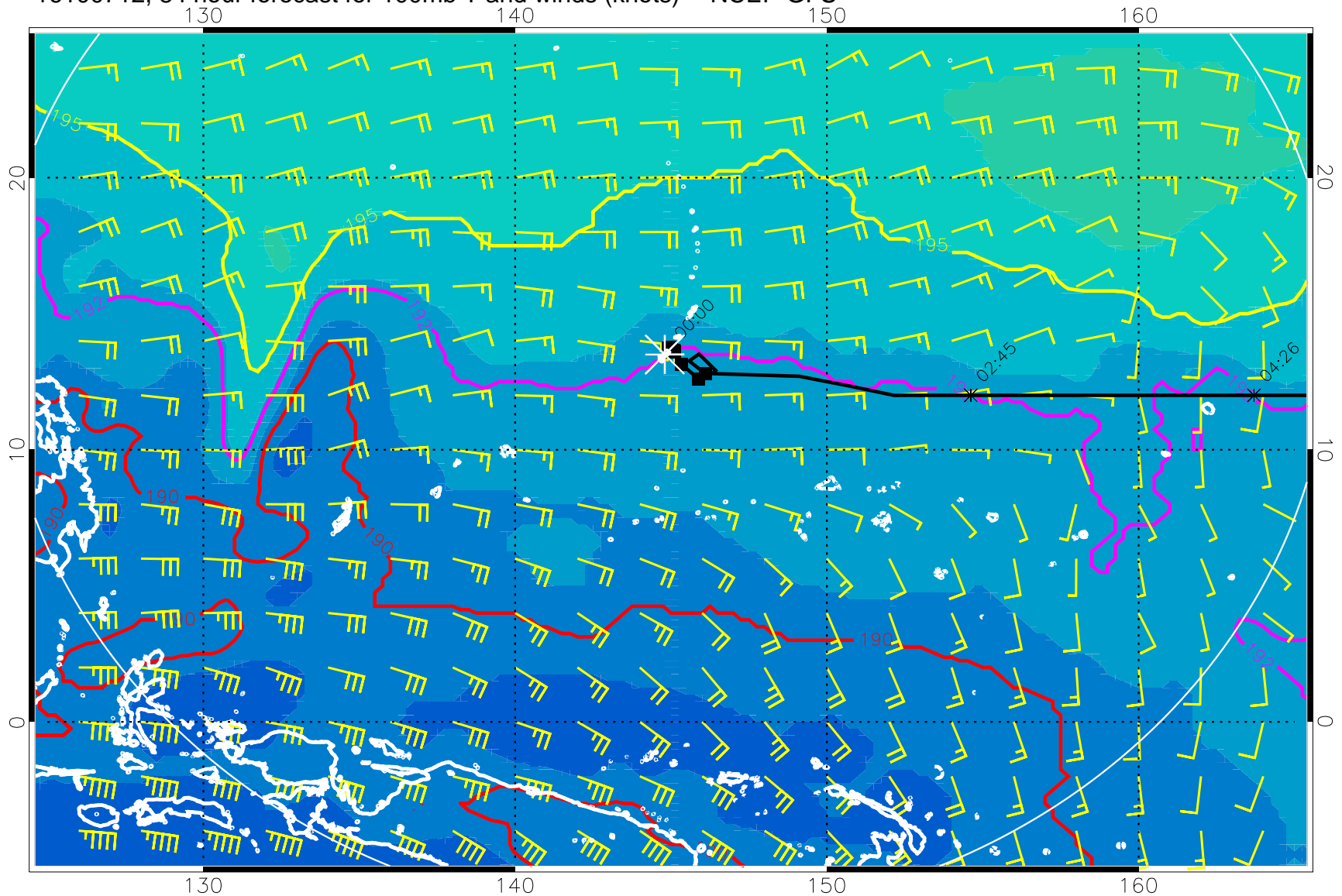
16100712, 84 hour forecast for 100mb T and winds (knots) -- NCEP GFS
