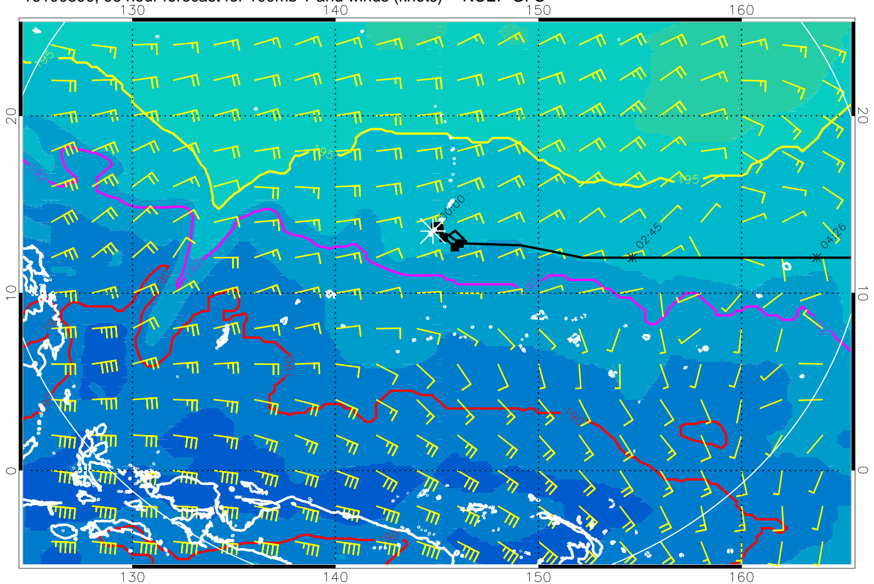
16100800, 96 hour forecast for 100mb T and winds (knots) -- NCEP GFS
