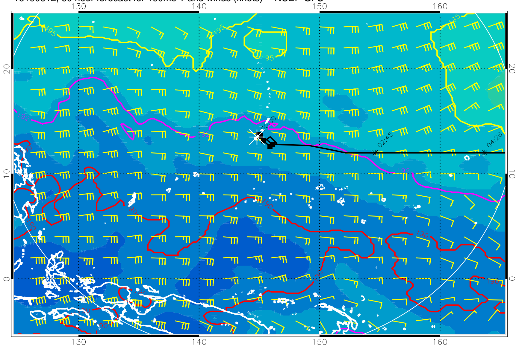
16100612, 60 hour forecast for 100mb T and winds (knots) -- NCEP GFS
