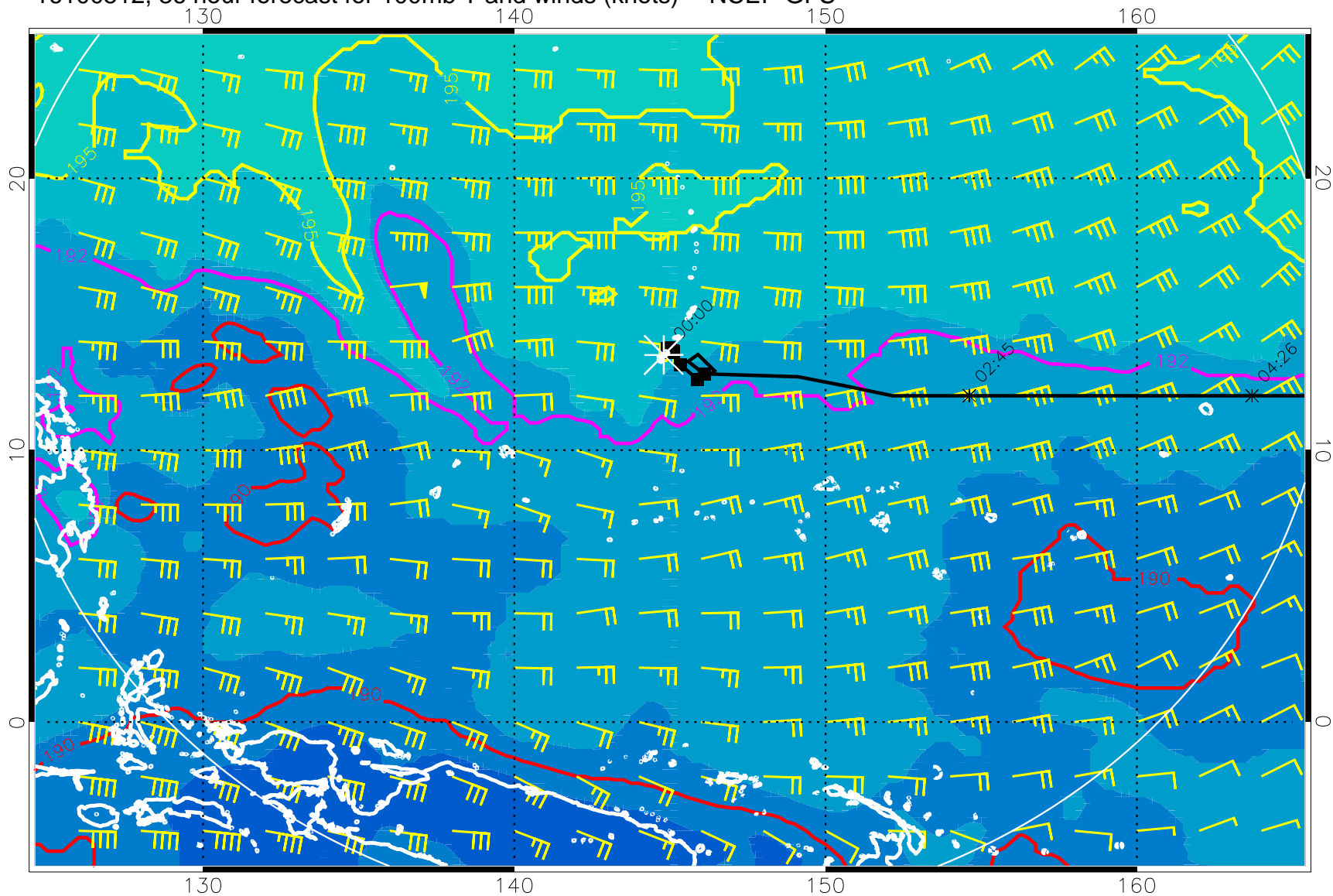
16100512, 36 hour forecast for 100mb T and winds (knots) -- NCEP GFS
