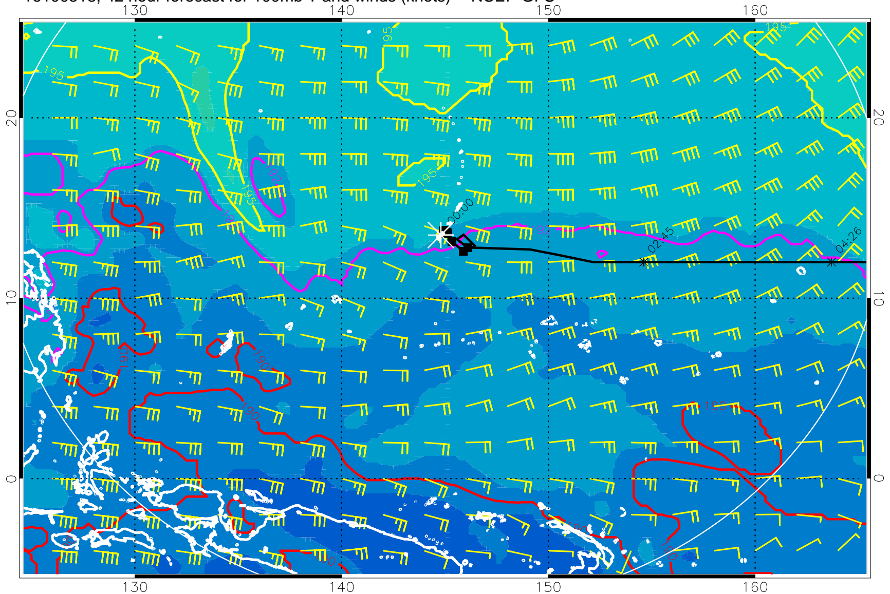
16100518, 42 hour forecast for 100mb T and winds (knots) -- NCEP GFS
