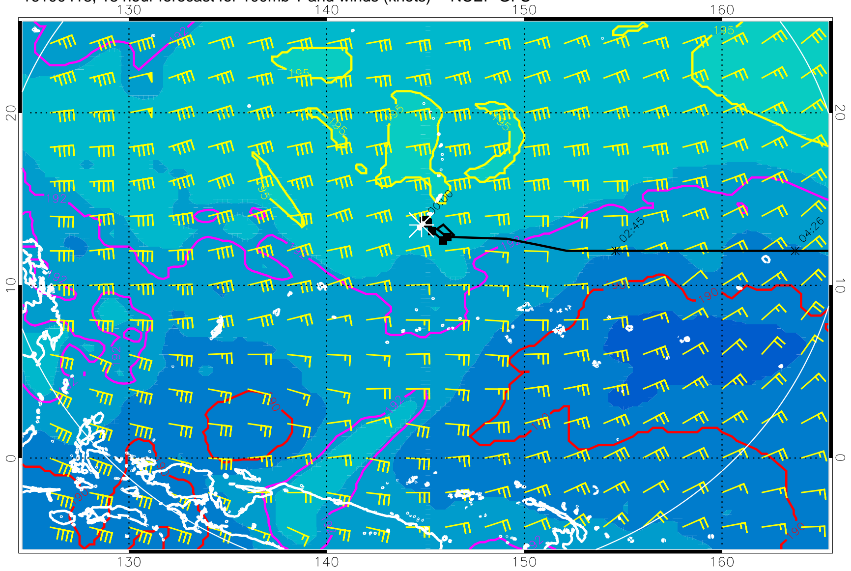
16100418, 18 hour forecast for 100mb T and winds (knots) -- NCEP GFS
