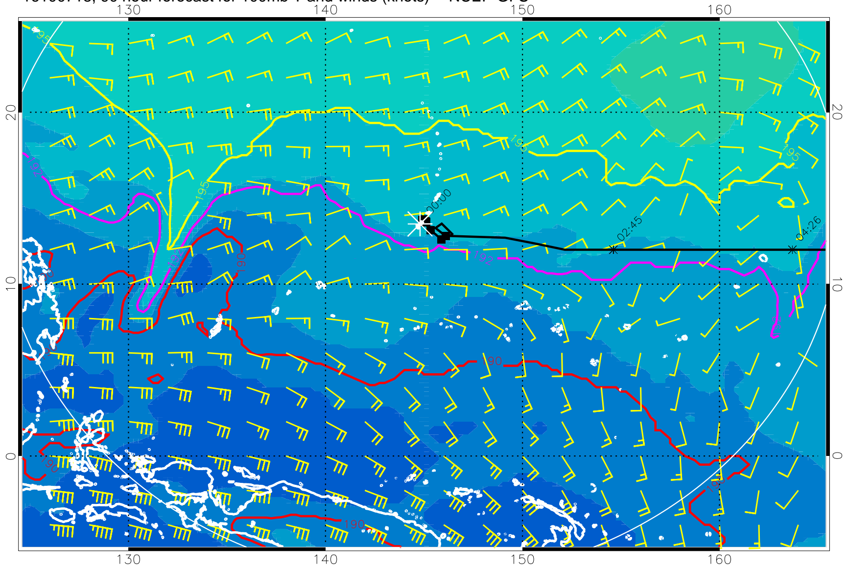
16100718, 90 hour forecast for 100mb T and winds (knots) -- NCEP GFS
