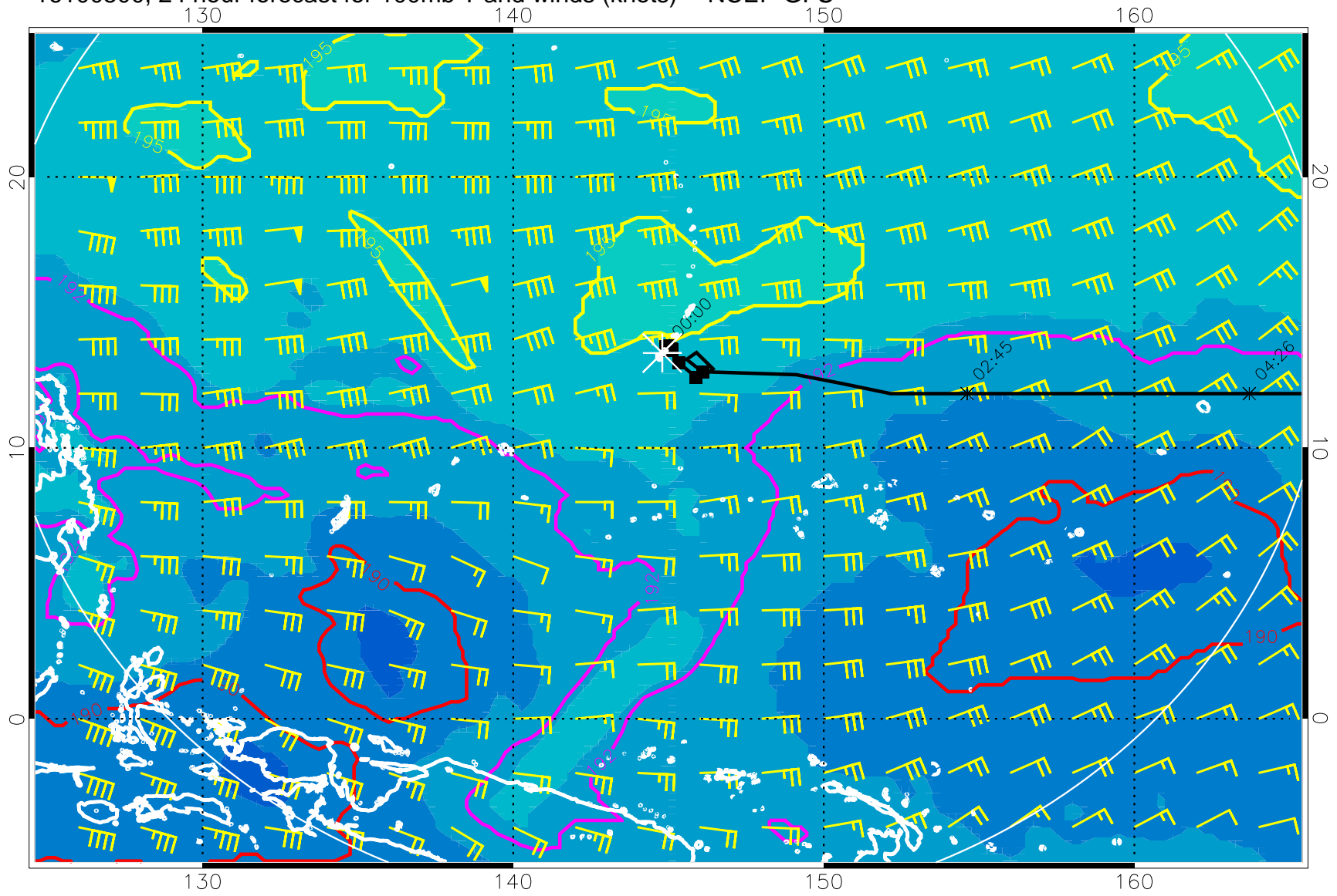
16100500, 24 hour forecast for 100mb T and winds (knots) -- NCEP GFS
