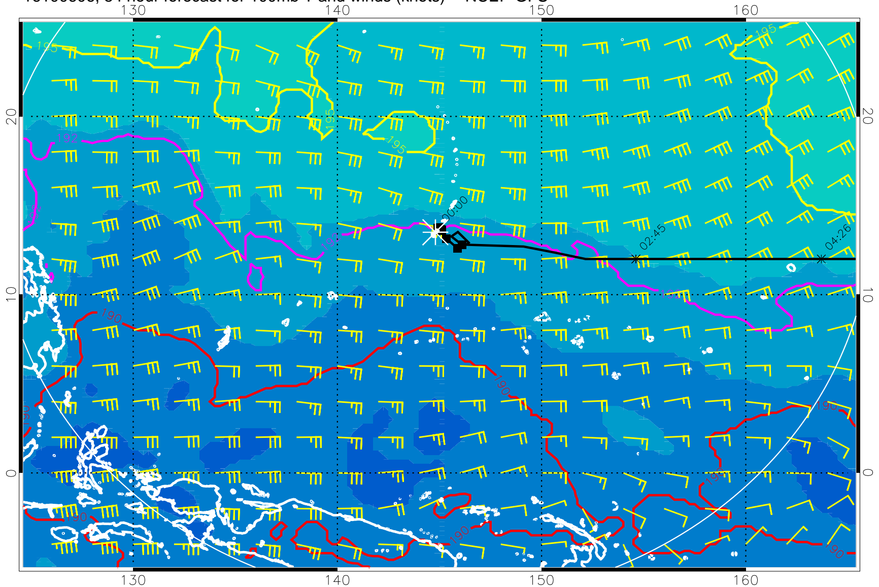
16100606, 54 hour forecast for 100mb T and winds (knots) -- NCEP GFS
