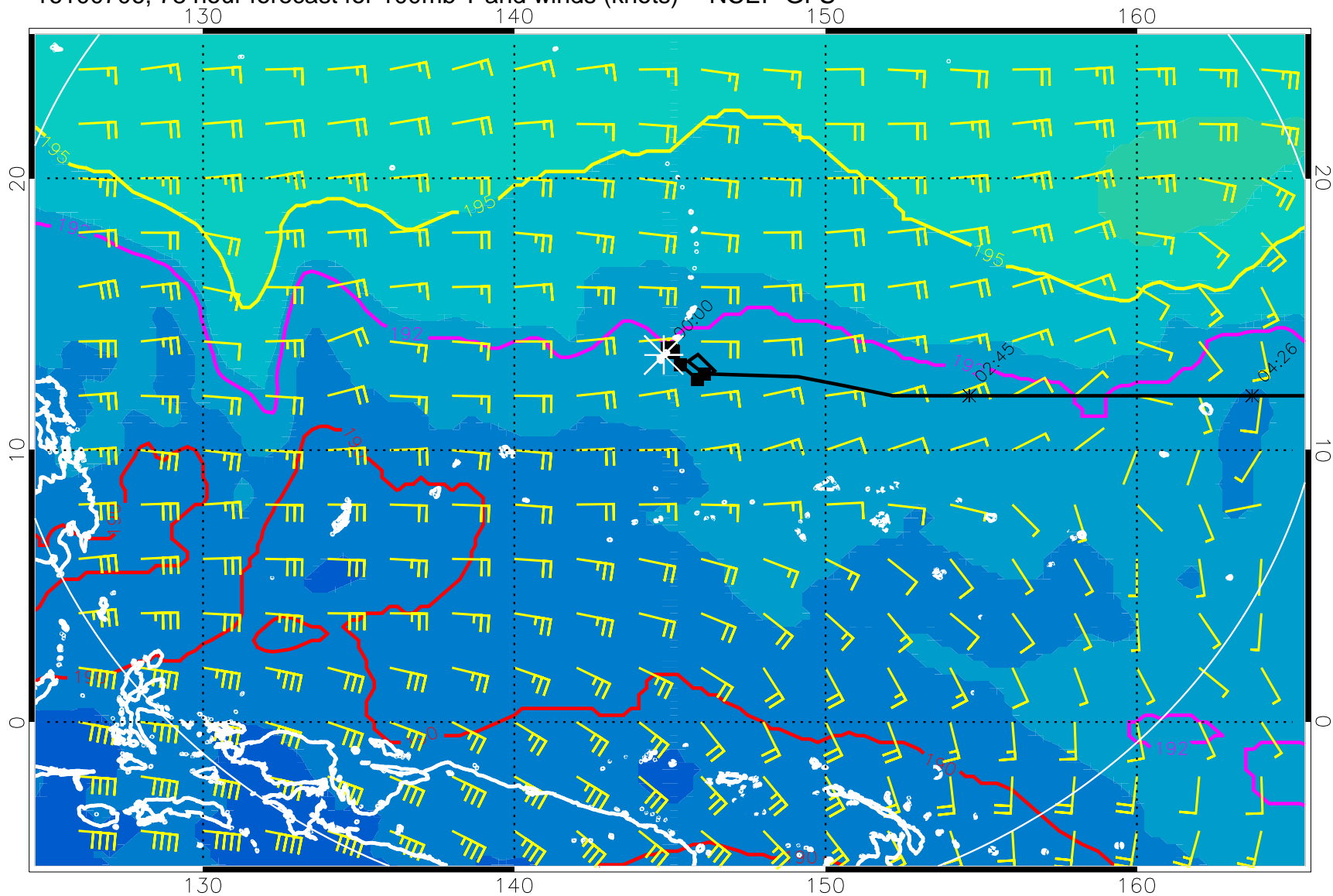
16100706, 78 hour forecast for 100mb T and winds (knots) -- NCEP GFS
