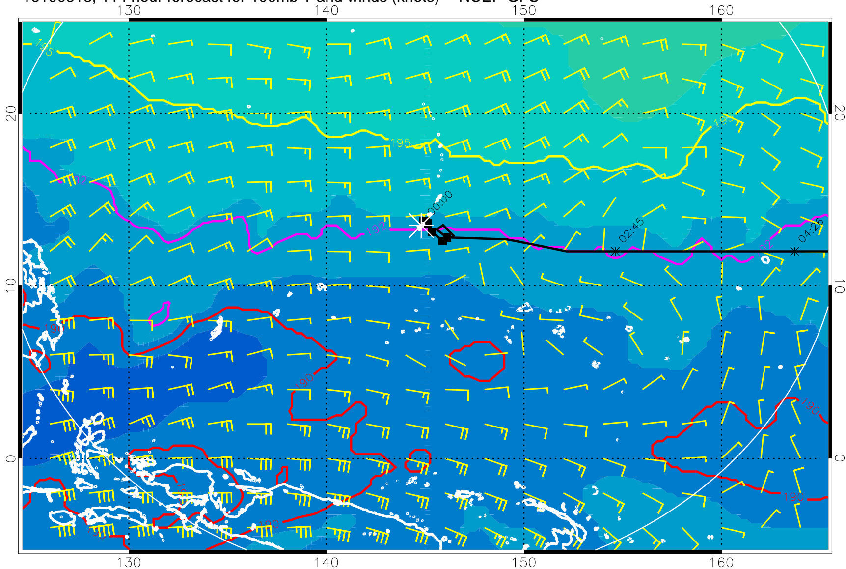
16100818, 114 hour forecast for 100mb T and winds (knots) -- NCEP GFS
