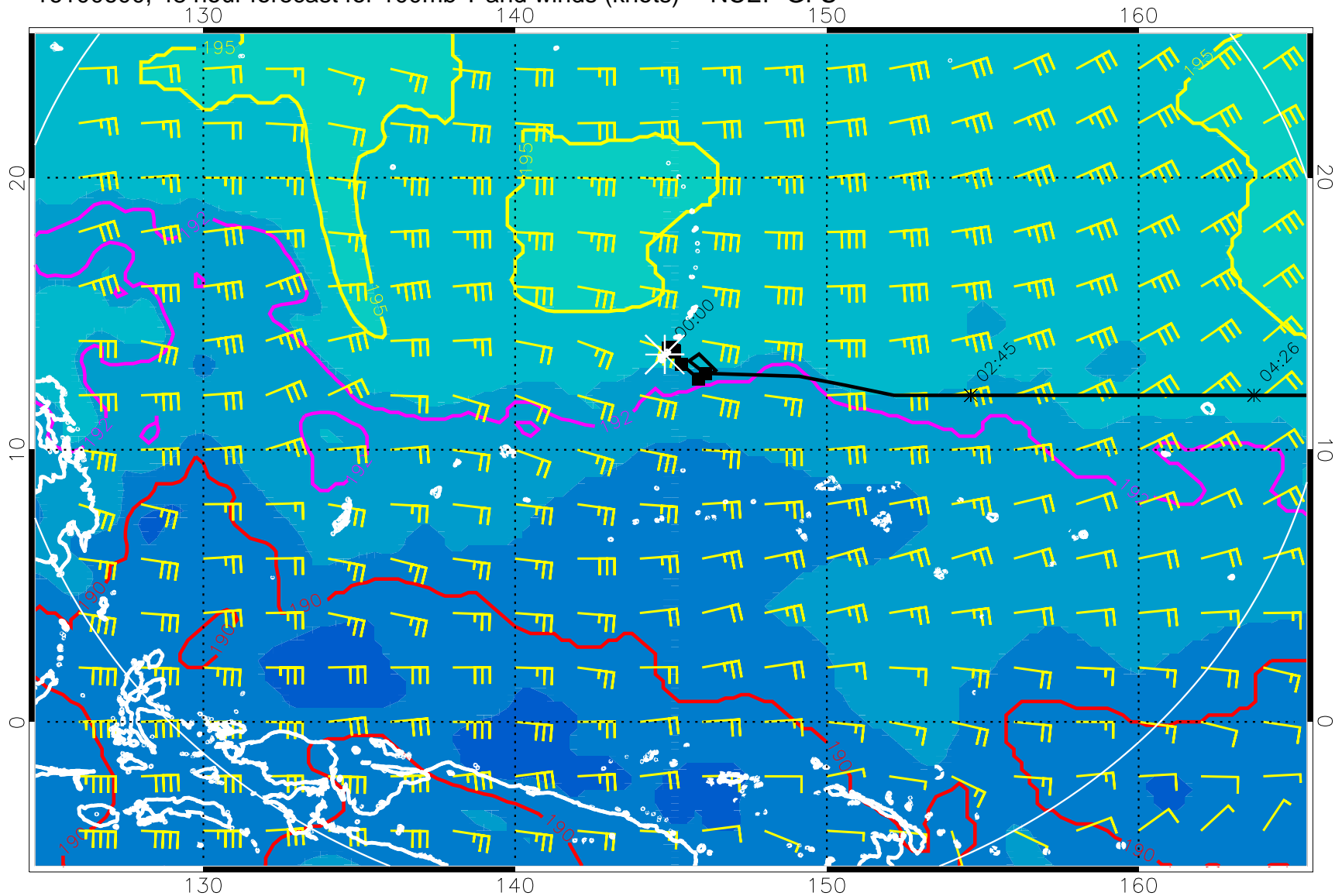
16100600, 48 hour forecast for 100mb T and winds (knots) -- NCEP GFS
