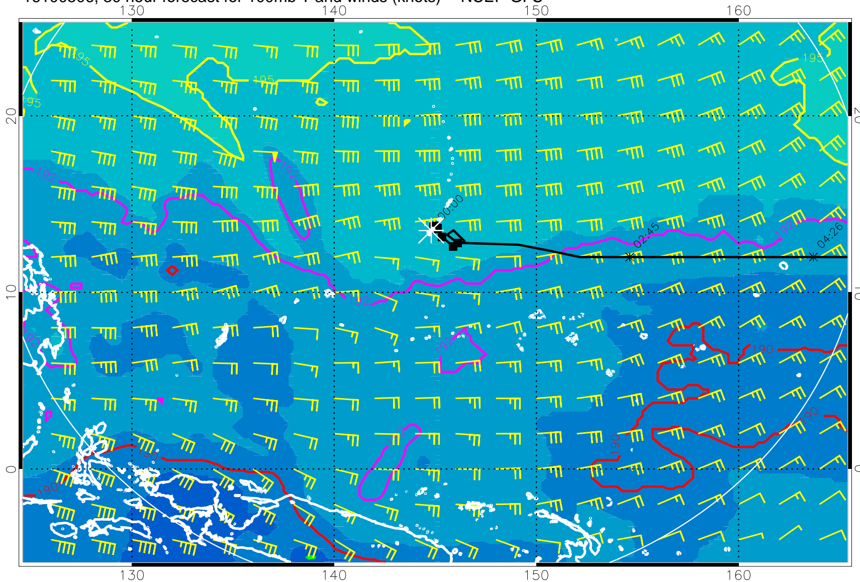
16100506, 30 hour forecast for 100mb T and winds (knots) -- NCEP GFS
