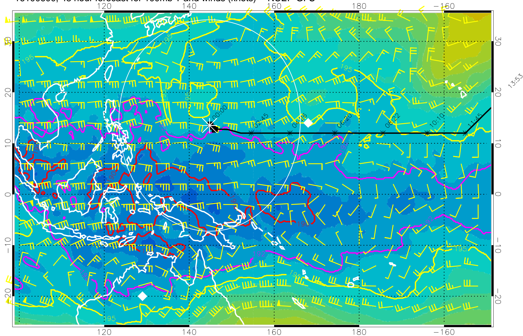
16100600, 48 hour forecast for 100mb T and winds (knots) -- NCEP GFS
