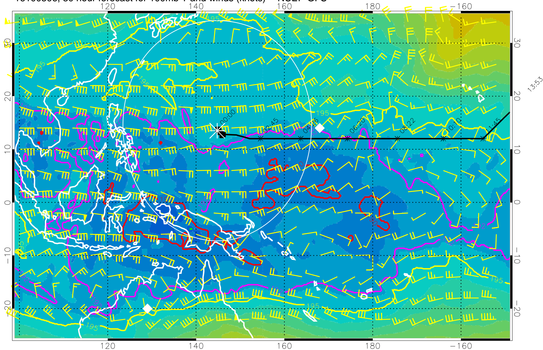
16100506, 30 hour forecast for 100mb T and winds (knots) -- NCEP GFS
