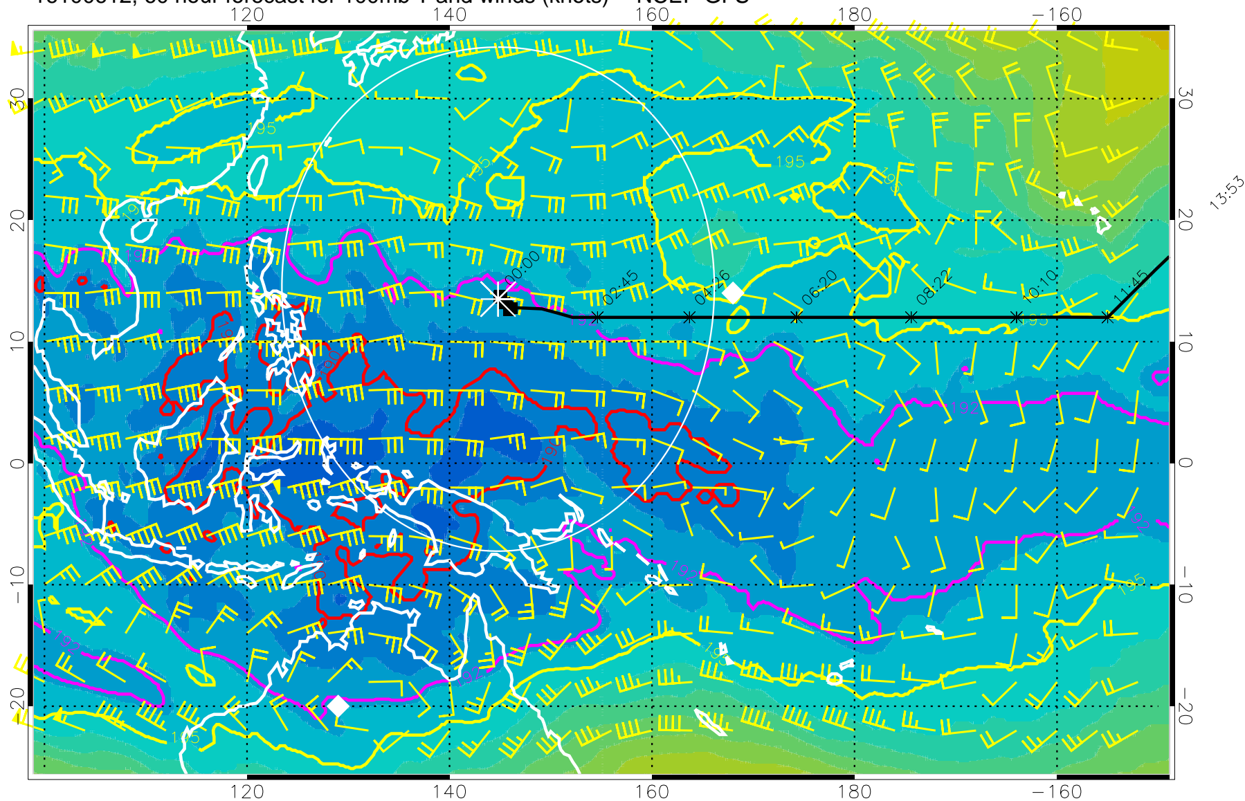
16100612, 60 hour forecast for 100mb T and winds (knots) -- NCEP GFS
