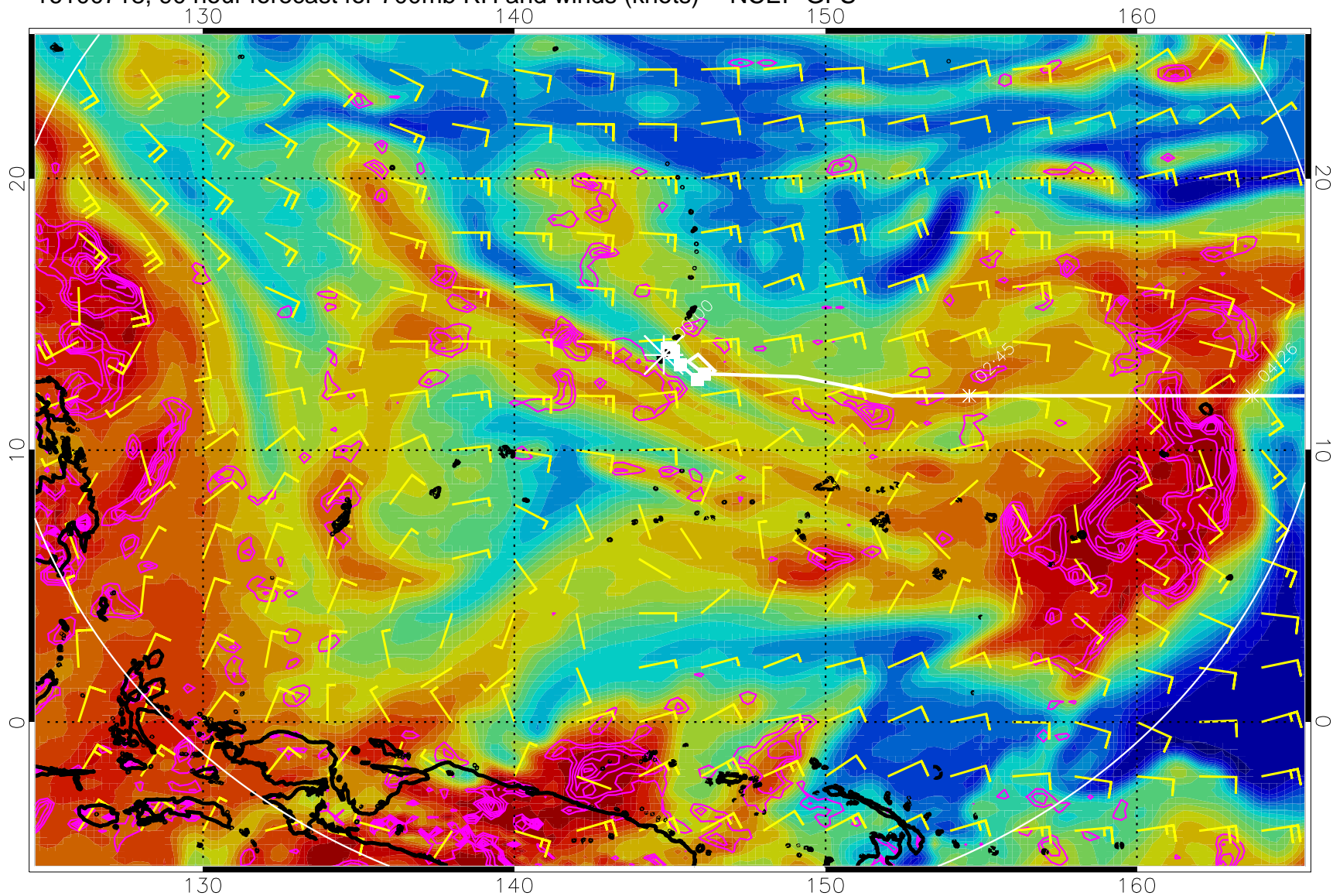
16100718, 90 hour forecast for 700mb RH and winds (knots) -- NCEP GFS
