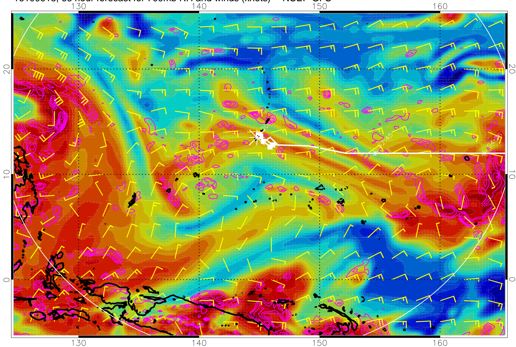
16100618, 66 hour forecast for 700mb RH and winds (knots) -- NCEP GFS
