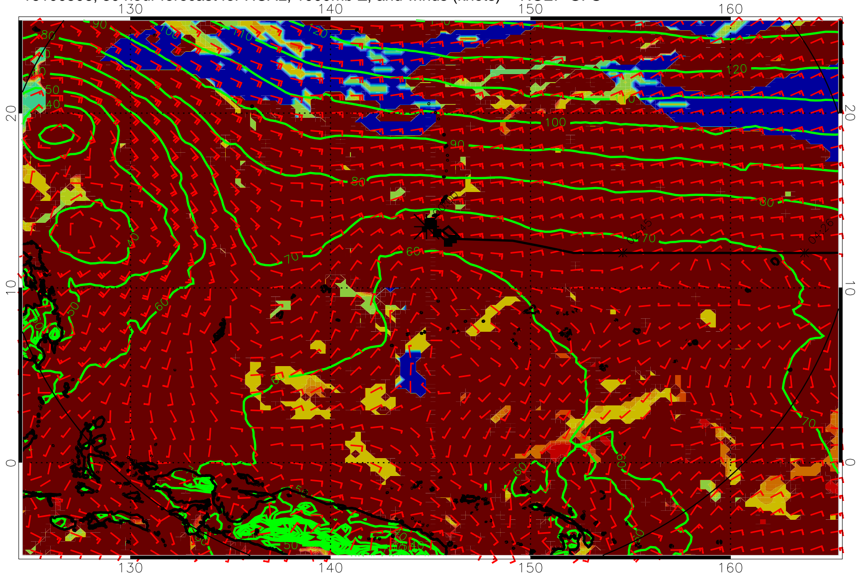
16100506, 30 hour forecast for HCAL, 1000mb Z, and winds (knots) -- NCEP GFS
