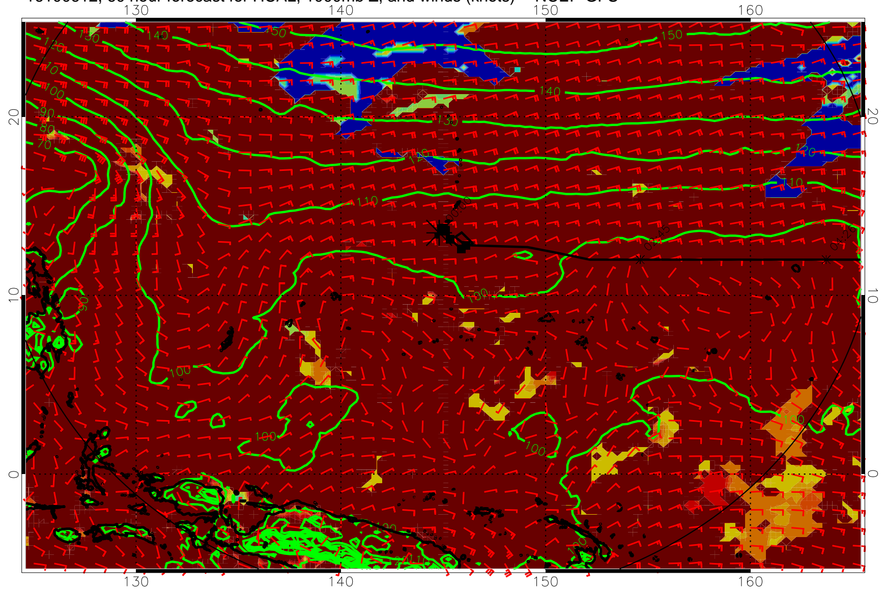
16100612, 60 hour forecast for HCAL, 1000mb Z, and winds (knots) -- NCEP GFS
