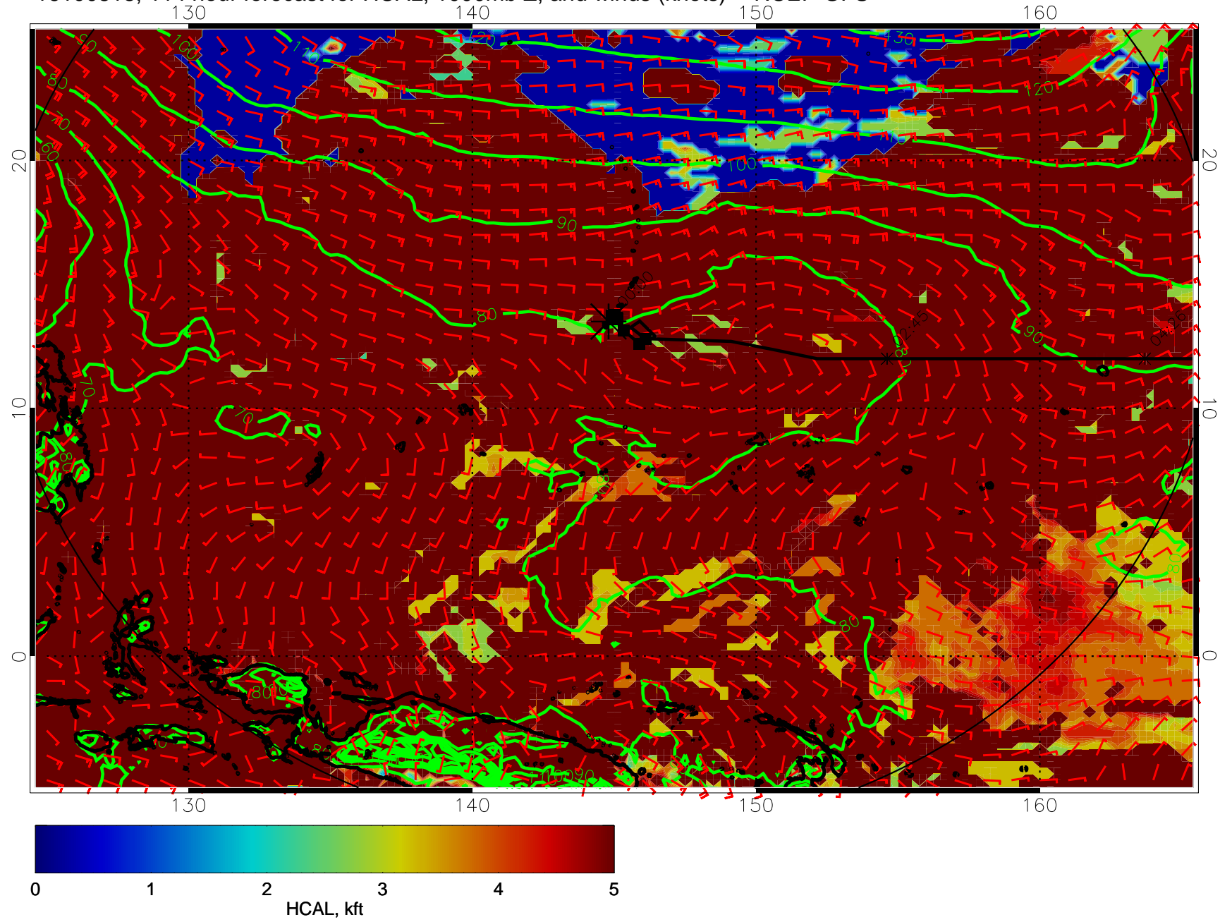
16100818, 114 hour forecast for HCAL, 1000mb Z, and winds (knots) -- NCEP GFS
