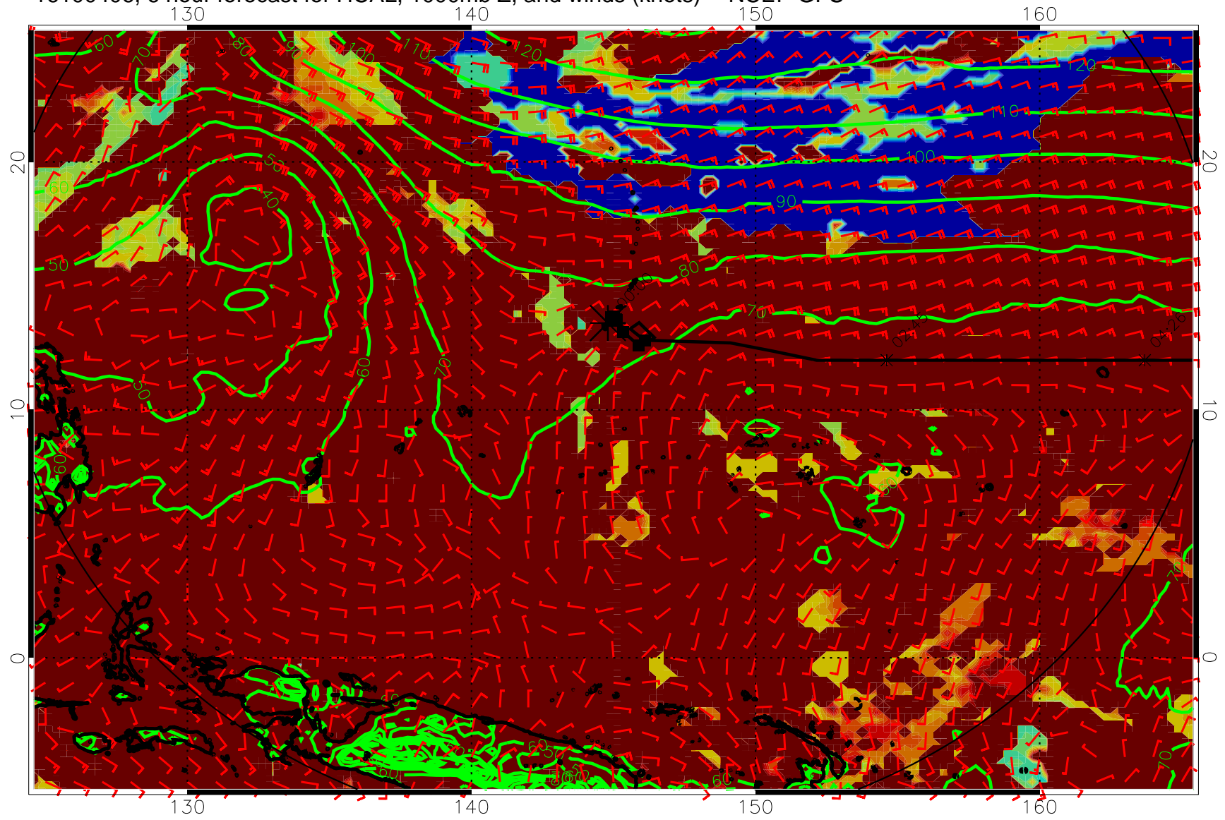
16100406, 6 hour forecast for HCAL, 1000mb Z, and winds (knots) -- NCEP GFS
