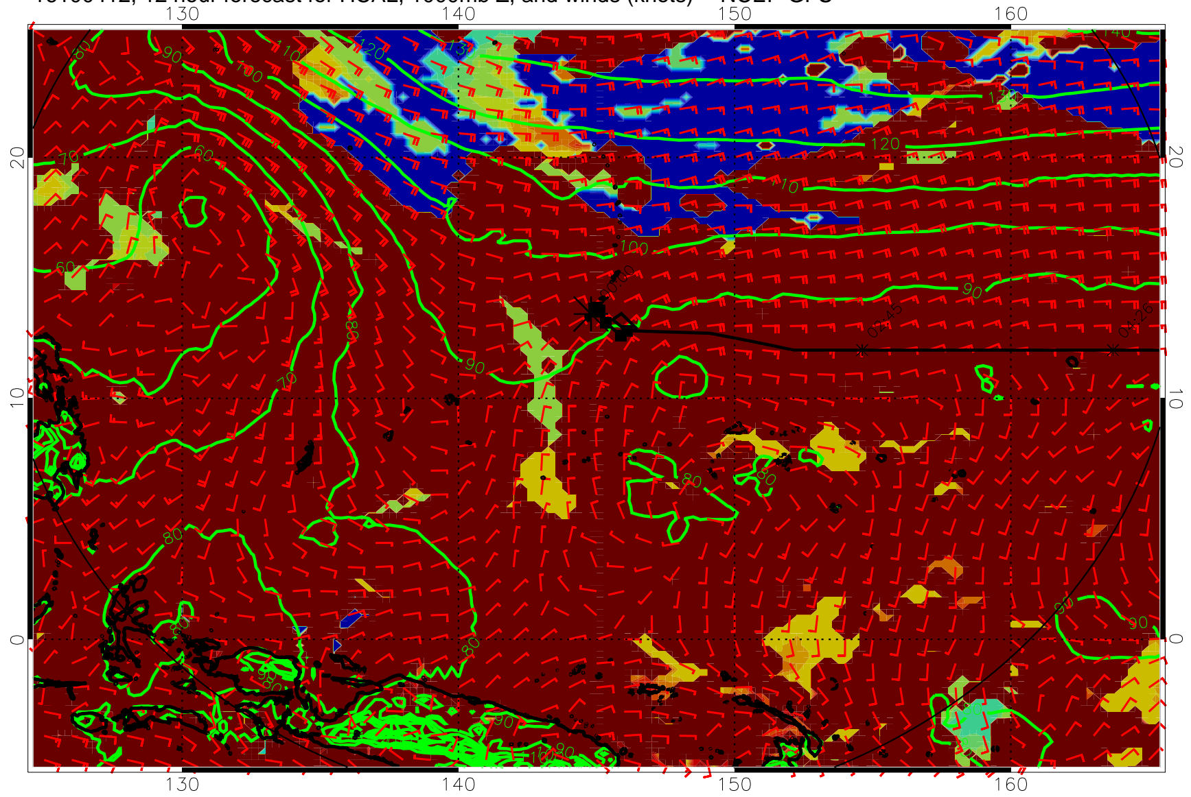
16100412, 12 hour forecast for HCAL, 1000mb Z, and winds (knots) -- NCEP GFS
