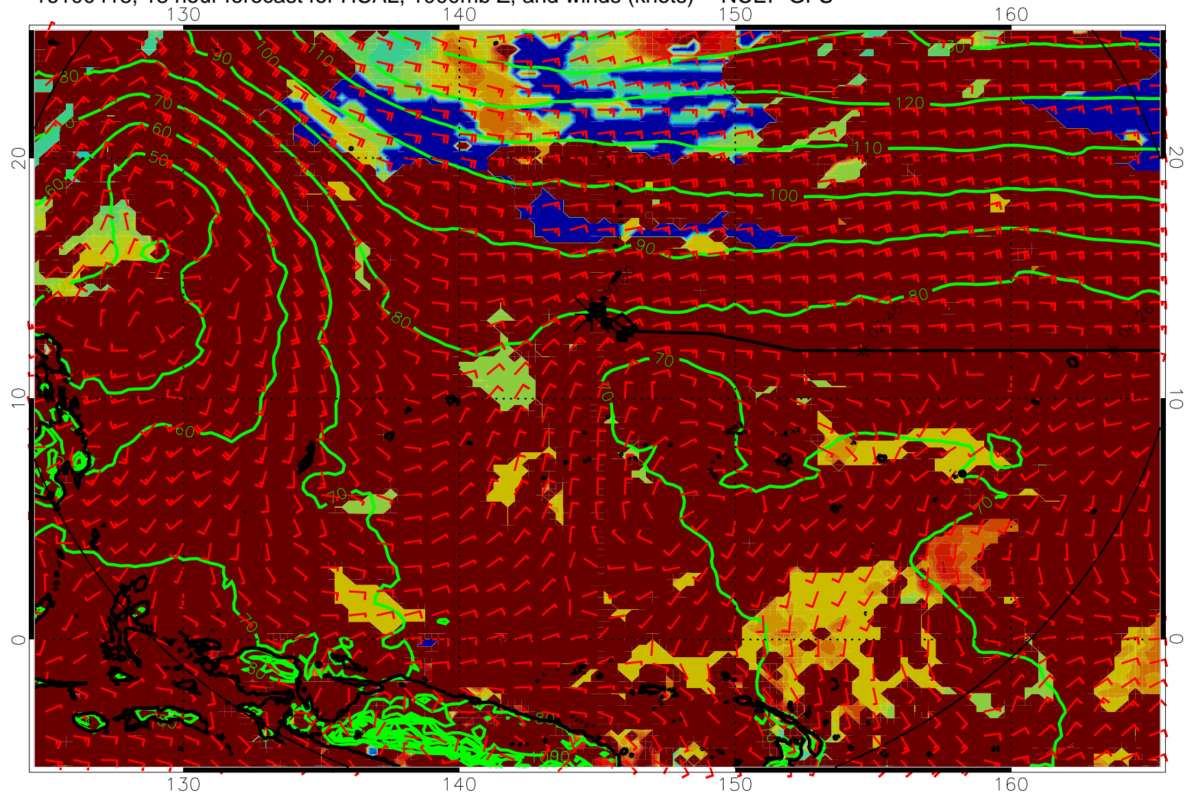
16100418, 18 hour forecast for HCAL, 1000mb Z, and winds (knots) -- NCEP GFS
