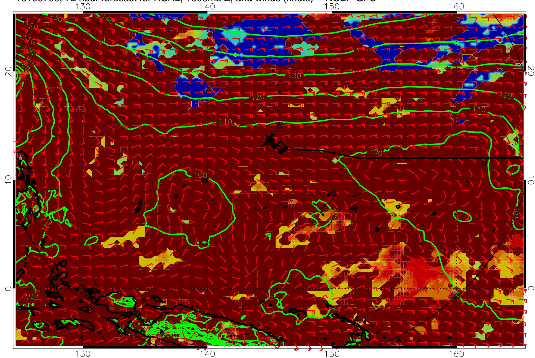
16100700, 72 hour forecast for HCAL, 1000mb Z, and winds (knots) -- NCEP GFS
