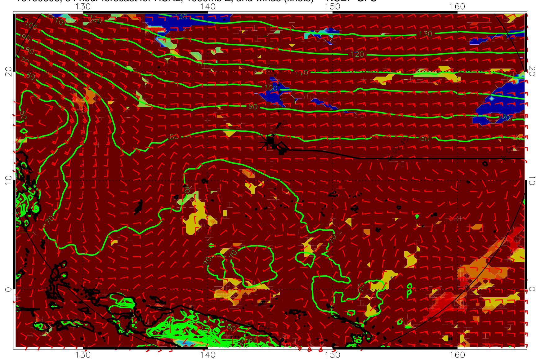
16100606, 54 hour forecast for HCAL, 1000mb Z, and winds (knots) -- NCEP GFS
