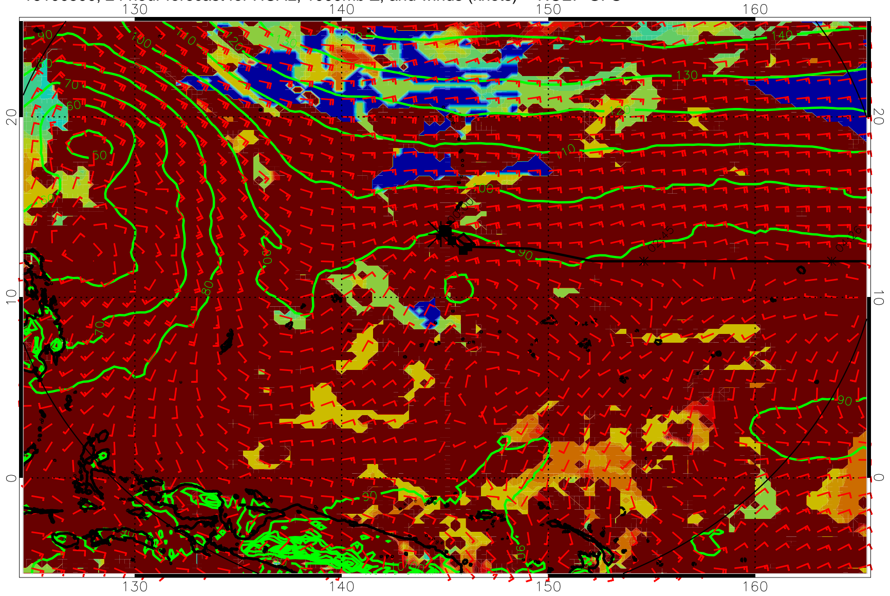
16100500, 24 hour forecast for HCAL, 1000mb Z, and winds (knots) -- NCEP GFS
