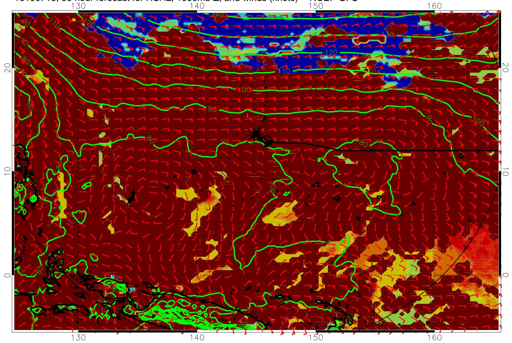
16100718, 90 hour forecast for HCAL, 1000mb Z, and winds (knots) -- NCEP GFS
