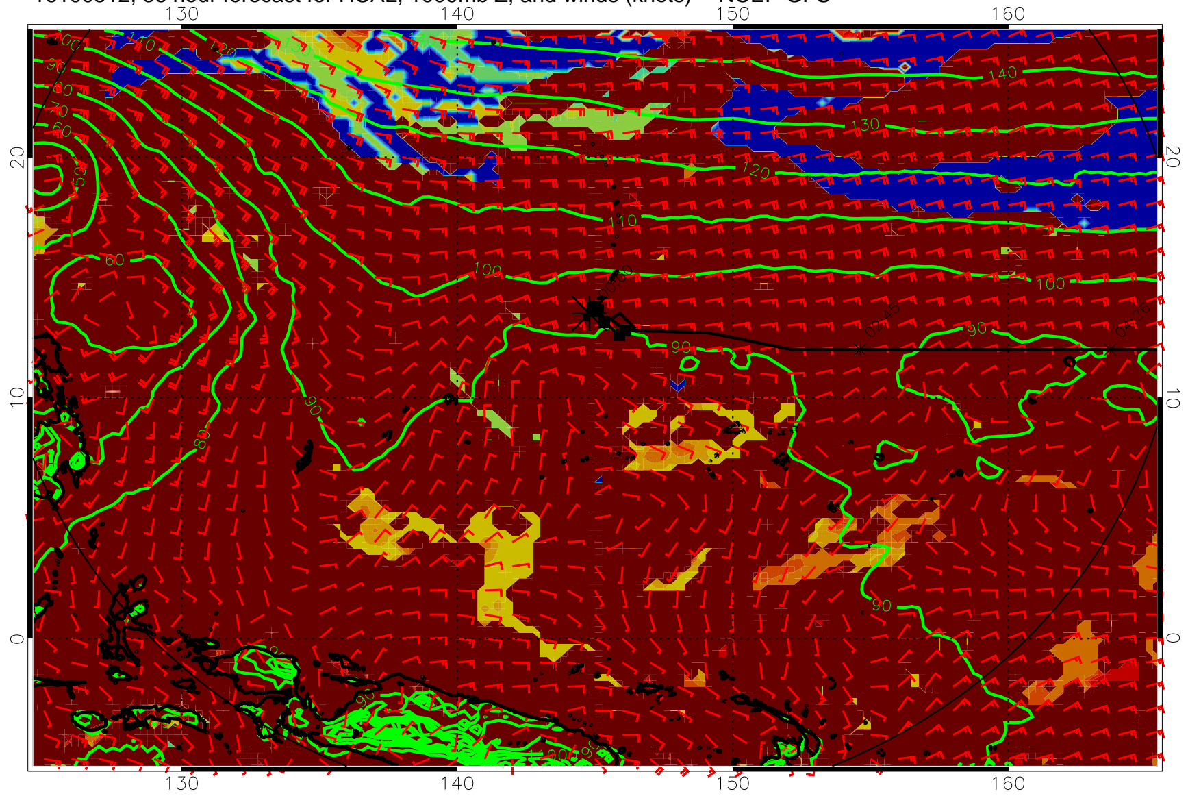
16100512, 36 hour forecast for HCAL, 1000mb Z, and winds (knots) -- NCEP GFS
