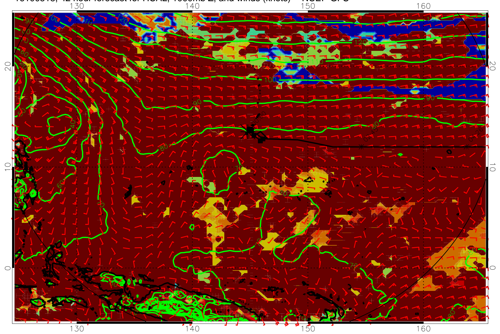
16100518, 42 hour forecast for HCAL, 1000mb Z, and winds (knots) -- NCEP GFS
