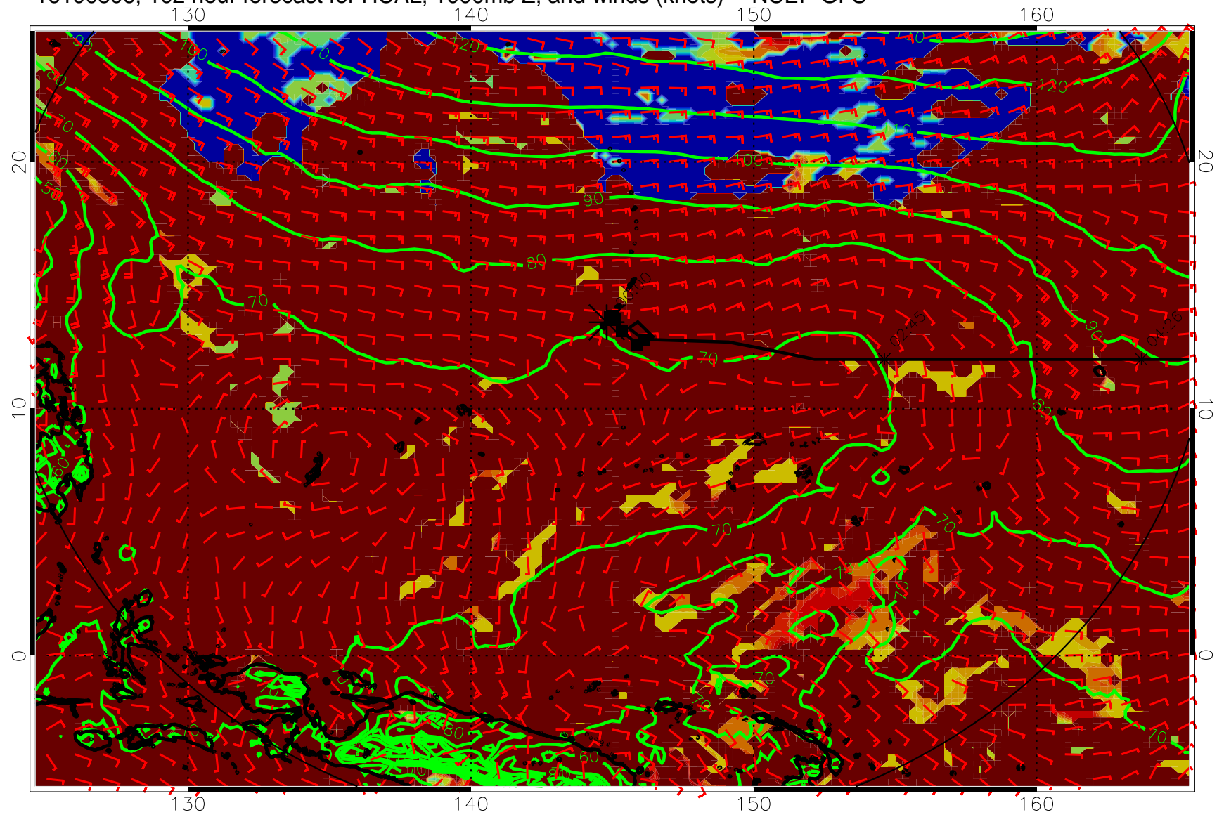
16100806, 102 hour forecast for HCAL, 1000mb Z, and winds (knots) -- NCEP GFS
