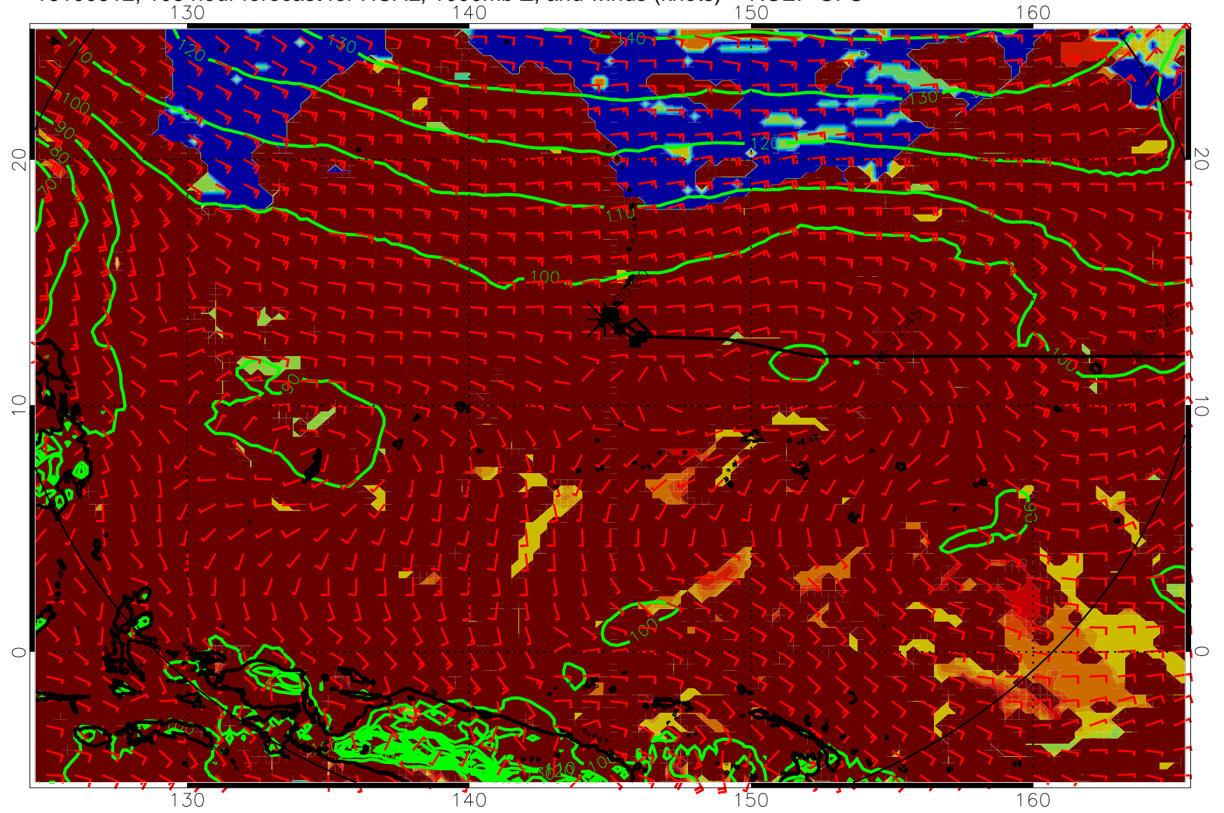
16100812, 108 hour forecast for HCAL, 1000mb Z, and winds (knots) -- NCEP GFS
