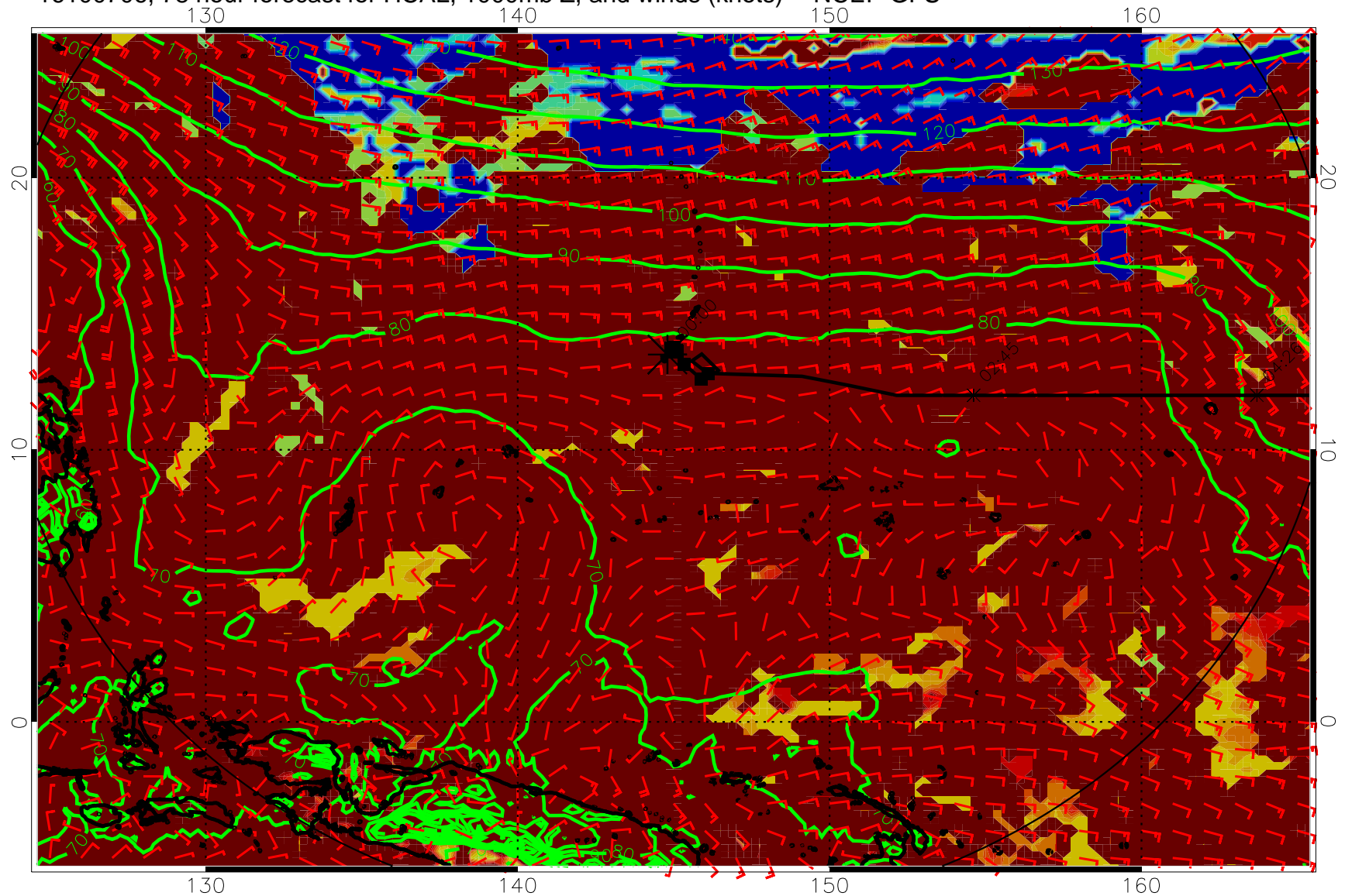
16100706, 78 hour forecast for HCAL, 1000mb Z, and winds (knots) -- NCEP GFS
