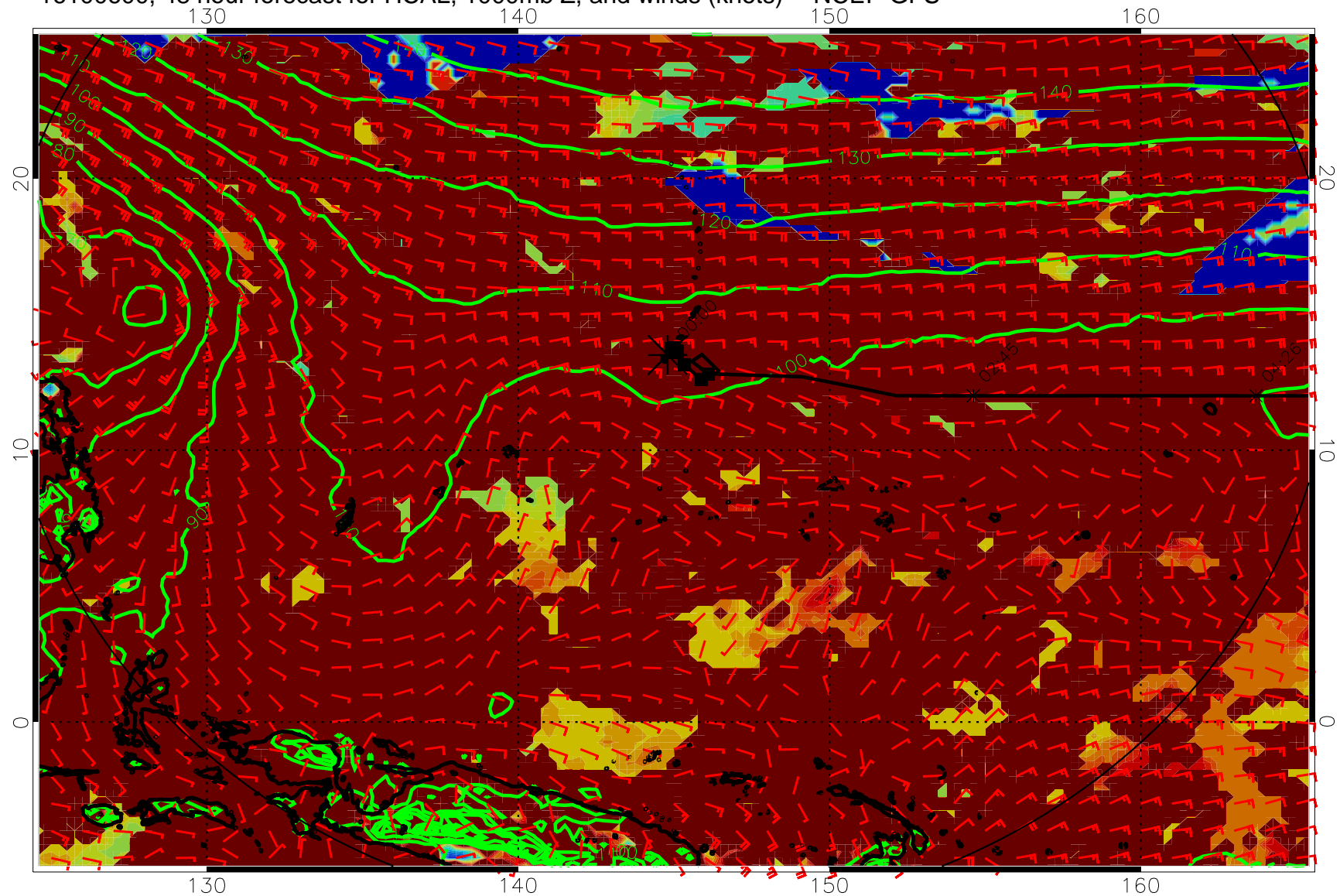
16100600, 48 hour forecast for HCAL, 1000mb Z, and winds (knots) -- NCEP GFS
