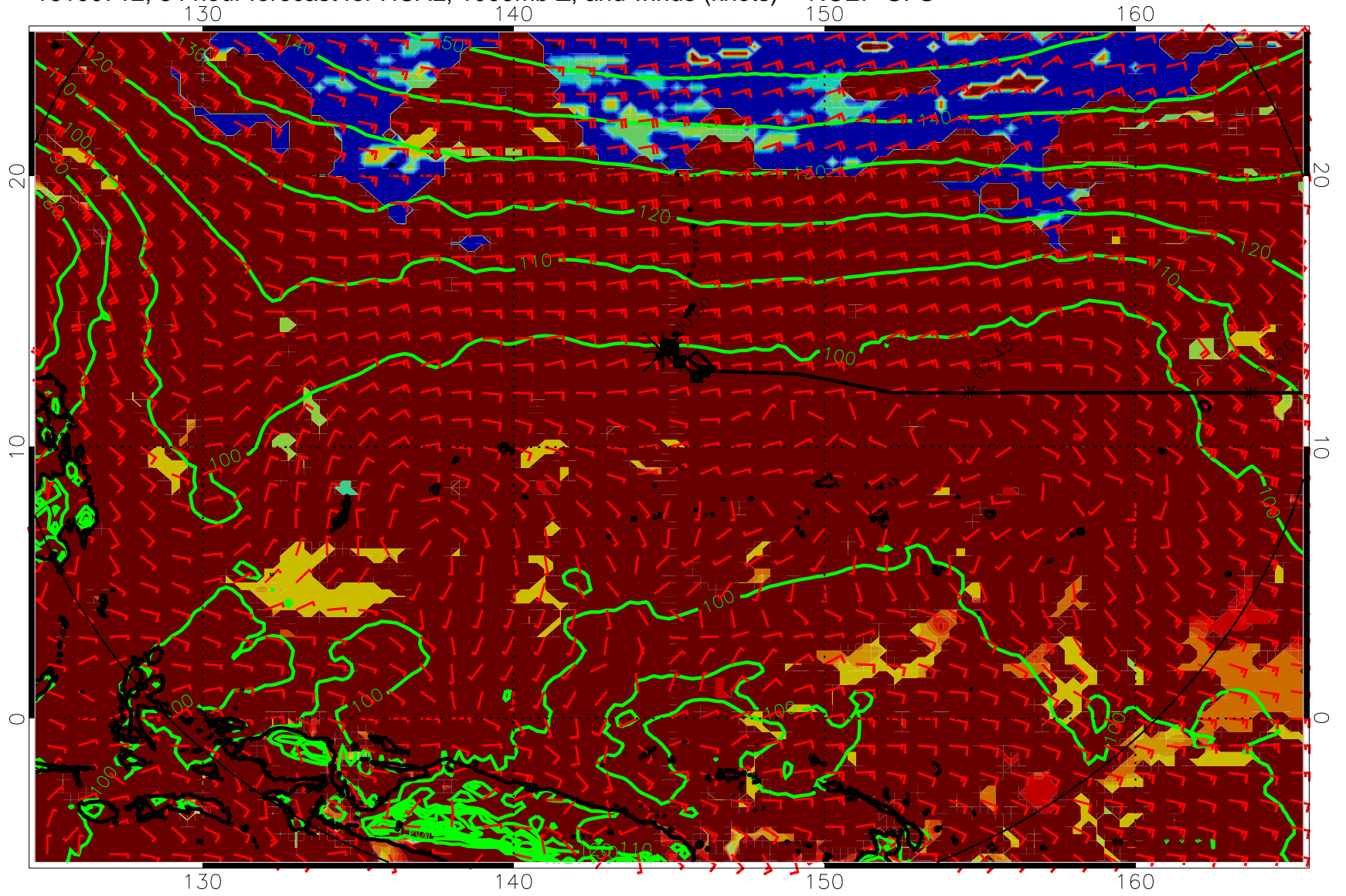
16100712, 84 hour forecast for HCAL, 1000mb Z, and winds (knots) -- NCEP GFS
