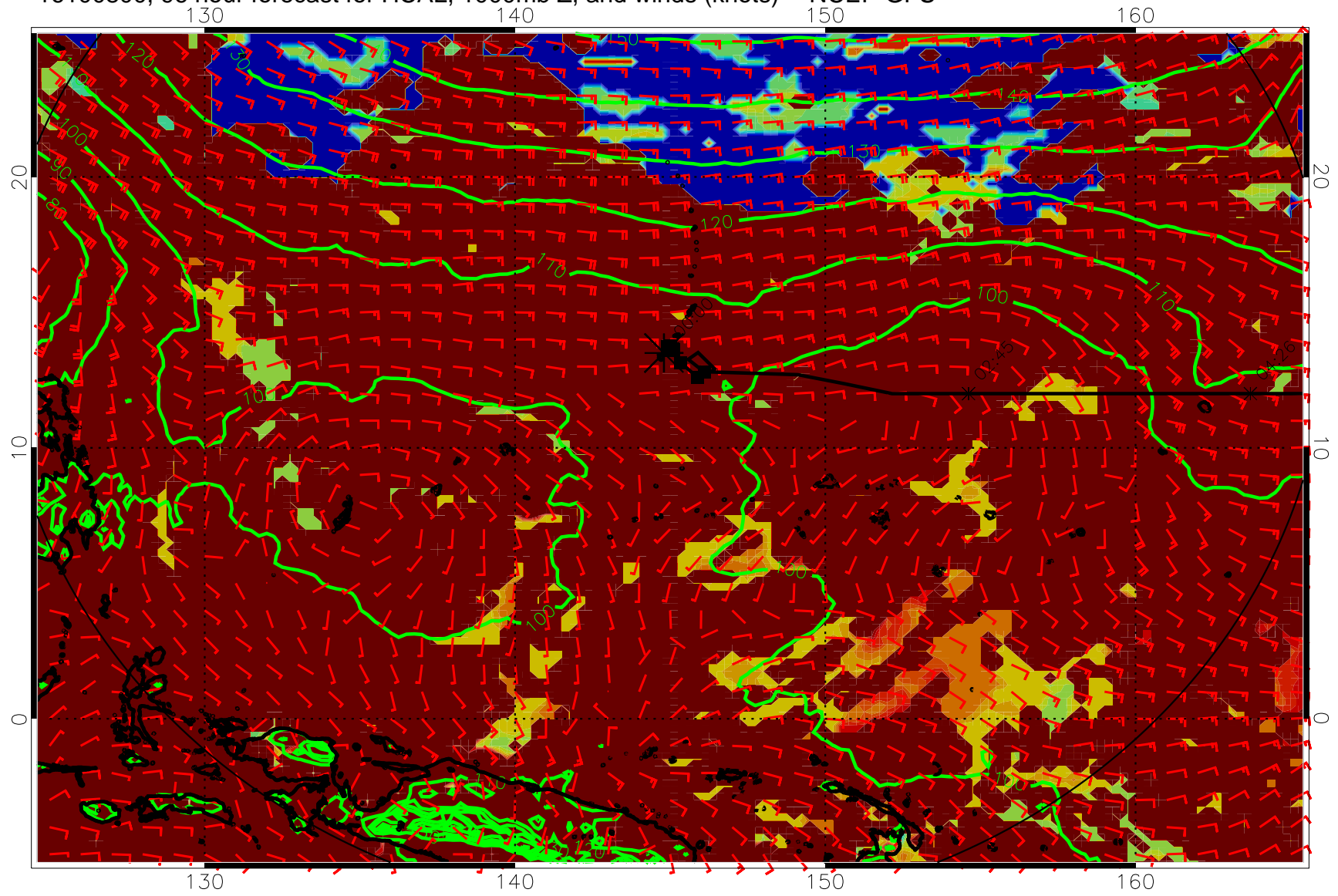
16100800, 96 hour forecast for HCAL, 1000mb Z, and winds (knots) -- NCEP GFS
