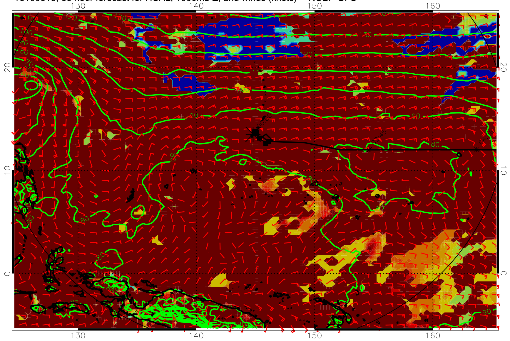
16100618, 66 hour forecast for HCAL, 1000mb Z, and winds (knots) -- NCEP GFS
