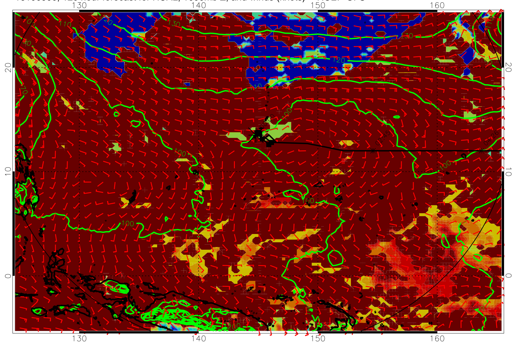
16100900, 120 hour forecast for HCAL, 1000mb Z, and winds (knots) -- NCEP GFS
