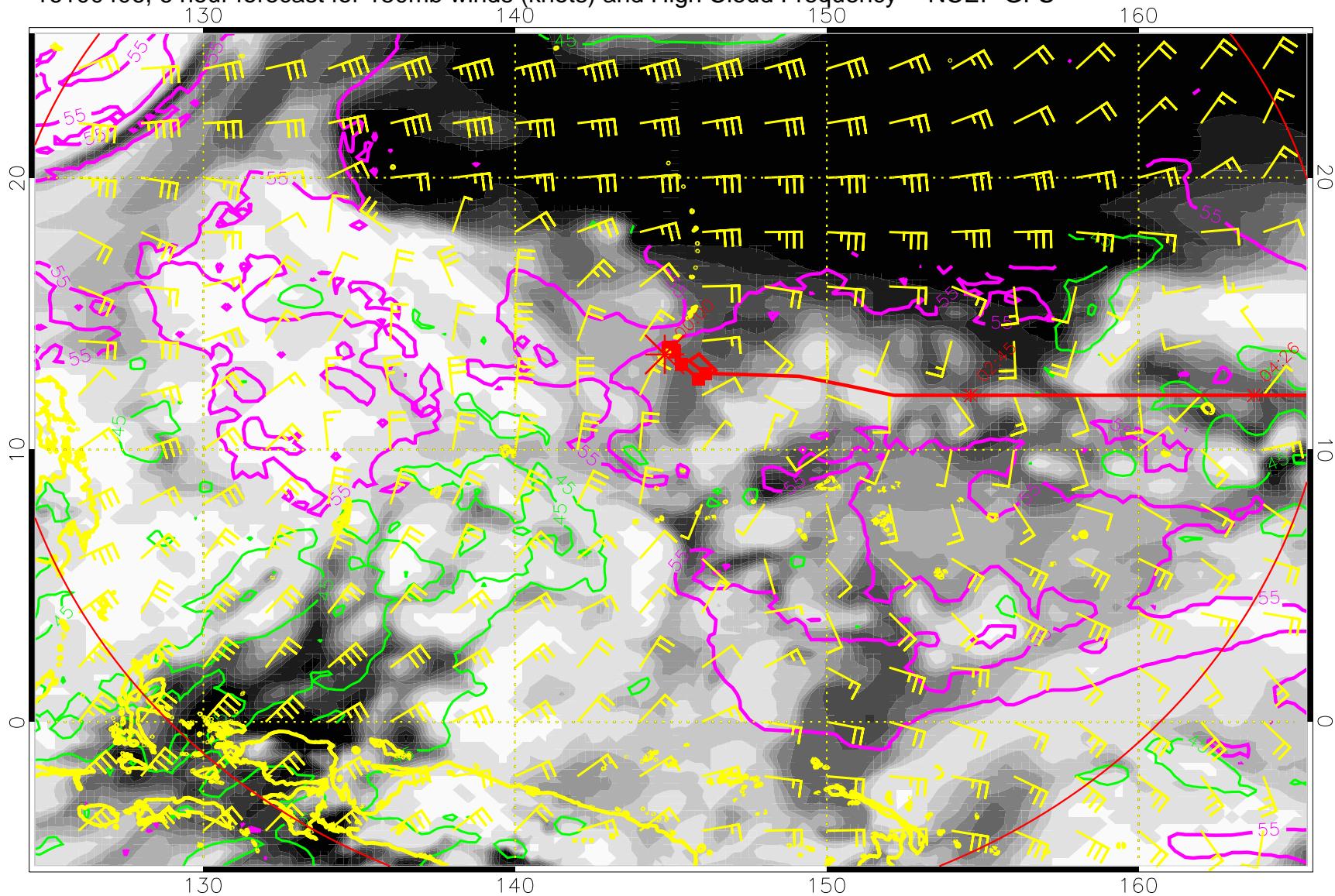
16100406, 6 hour forecast for 150mb winds (knots) and High Cloud Frequency -- NCEP GFS
