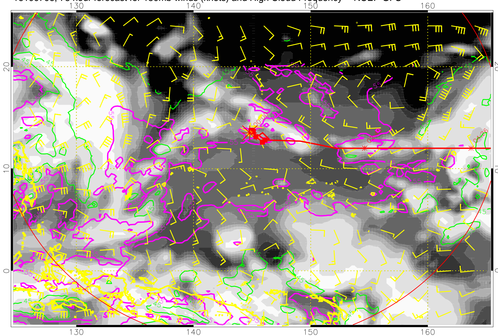
16100706, 78 hour forecast for 150mb winds (knots) and High Cloud Frequency -- NCEP GFS
