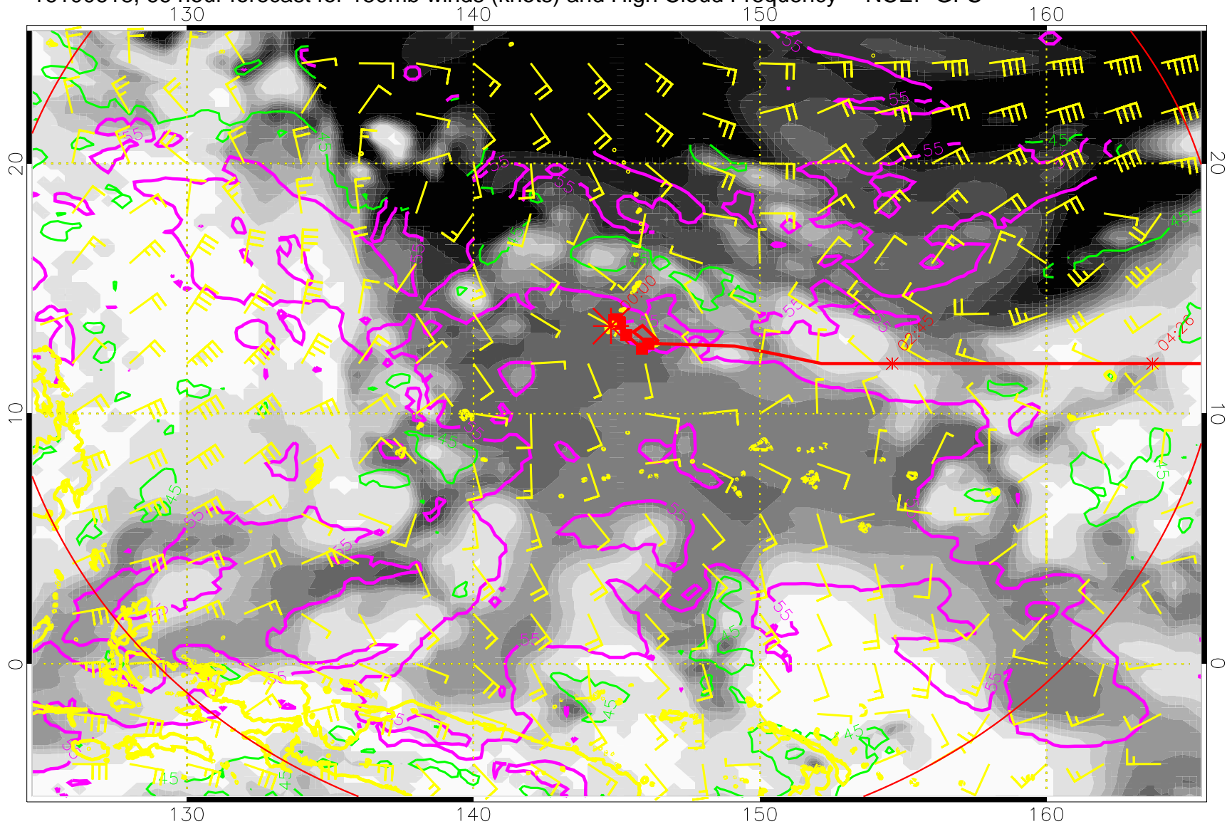
16100618, 66 hour forecast for 150mb winds (knots) and High Cloud Frequency -- NCEP GFS
