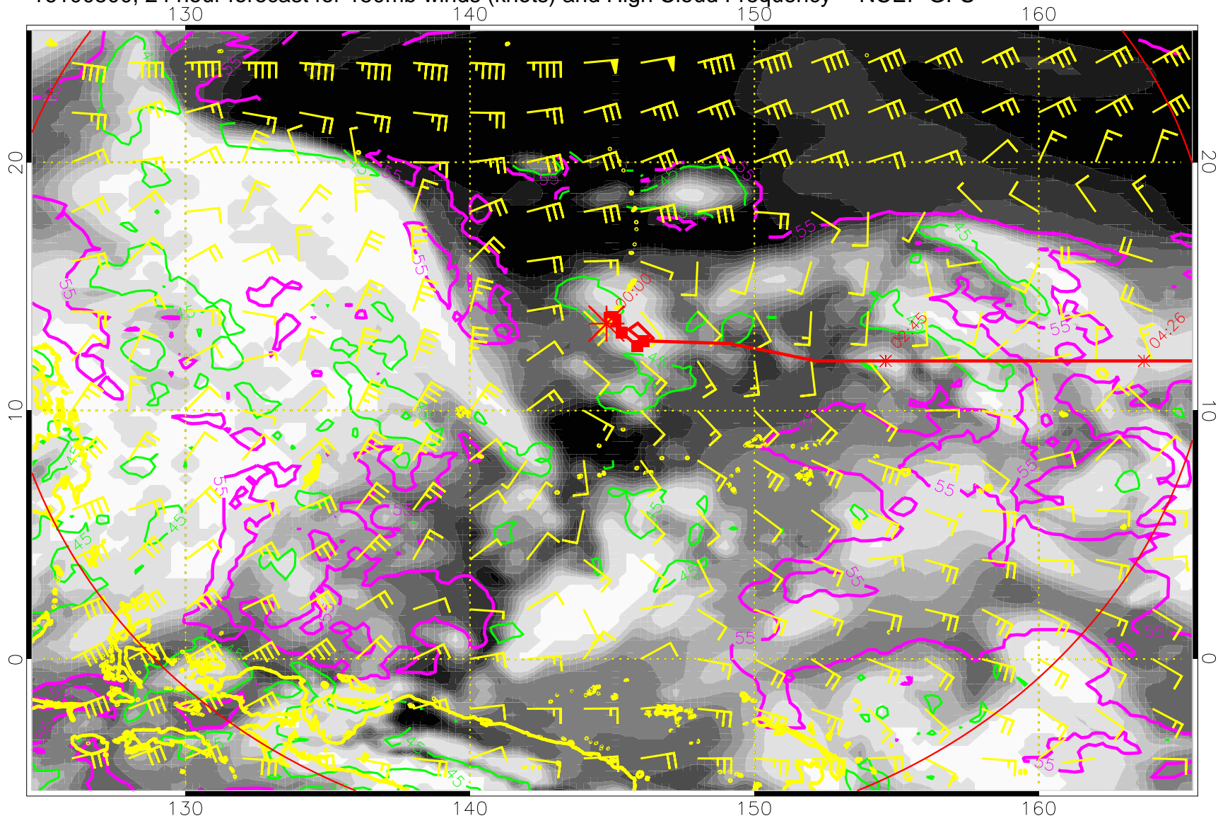
16100500, 24 hour forecast for 150mb winds (knots) and High Cloud Frequency -- NCEP GFS
