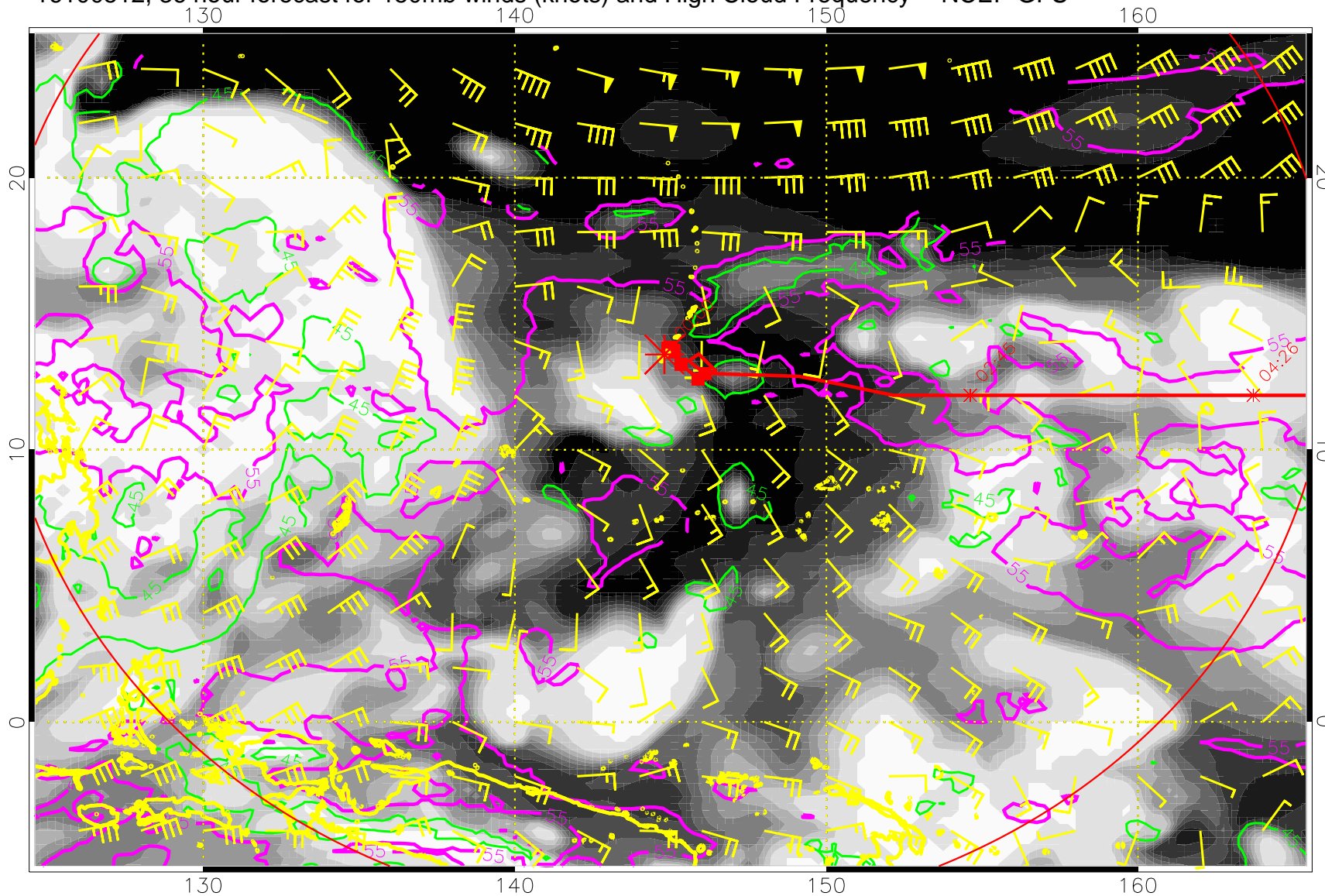
16100512, 36 hour forecast for 150mb winds (knots) and High Cloud Frequency -- NCEP GFS
