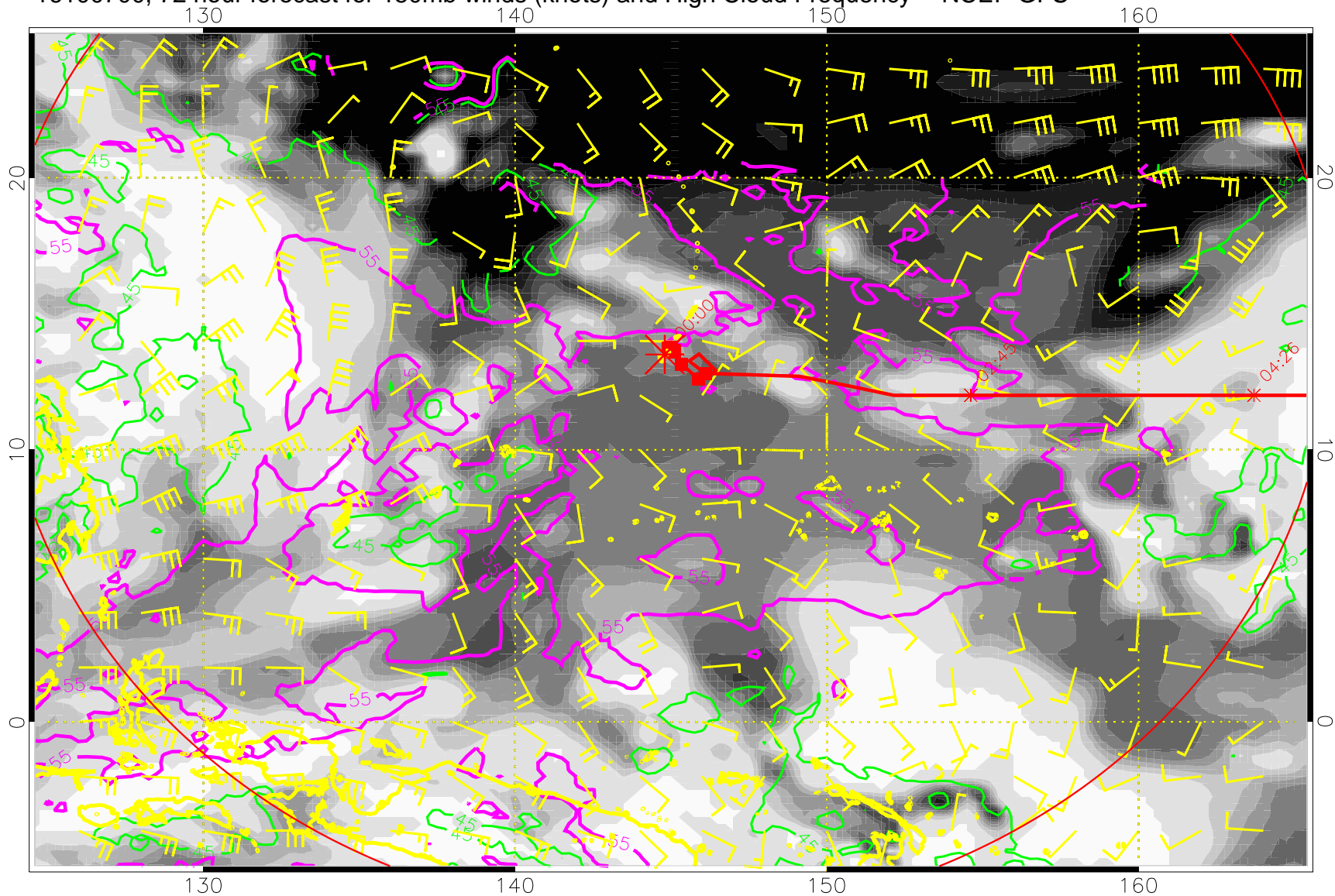
16100700, 72 hour forecast for 150mb winds (knots) and High Cloud Frequency -- NCEP GFS
