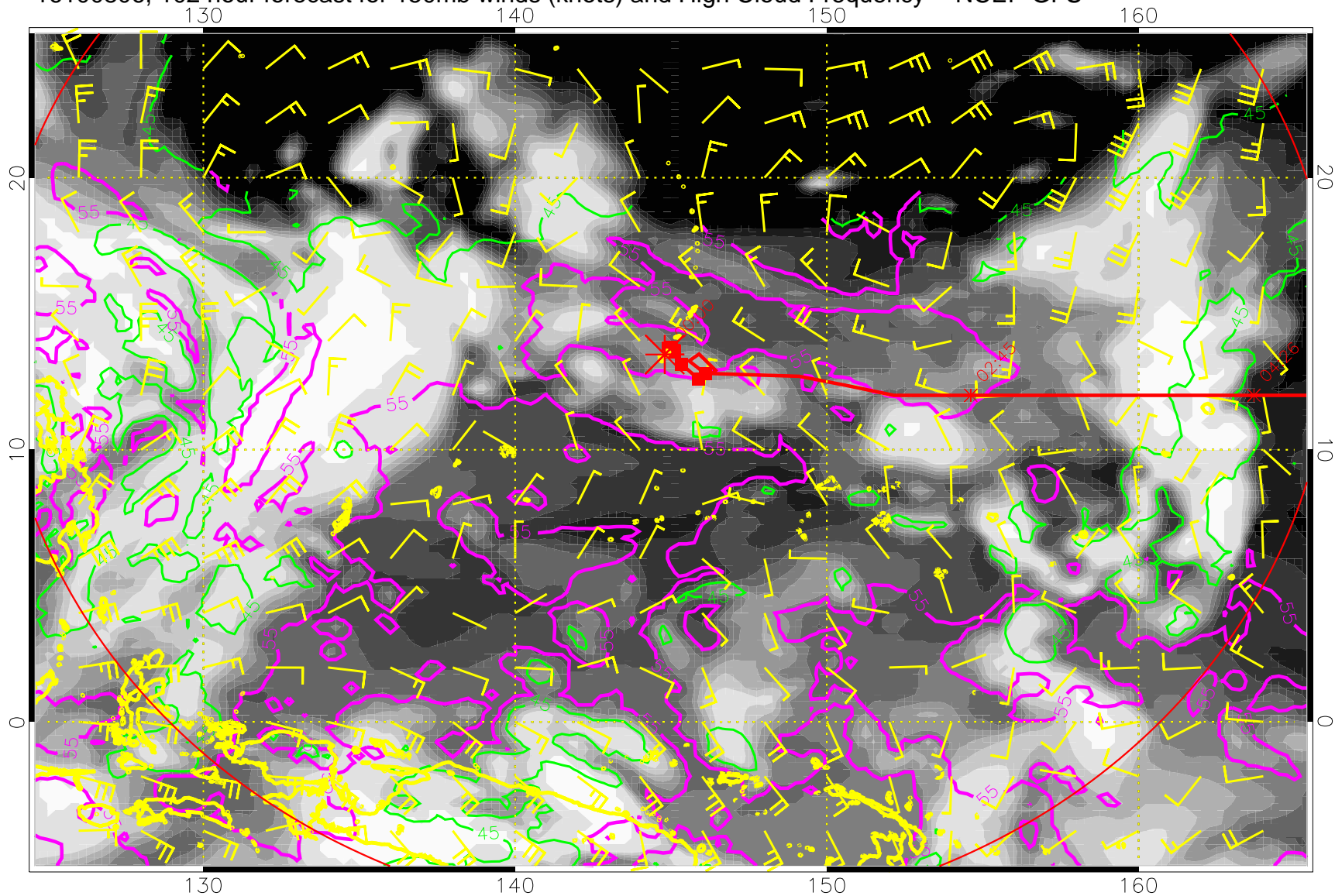
16100806, 102 hour forecast for 150mb winds (knots) and High Cloud Frequency -- NCEP GFS
