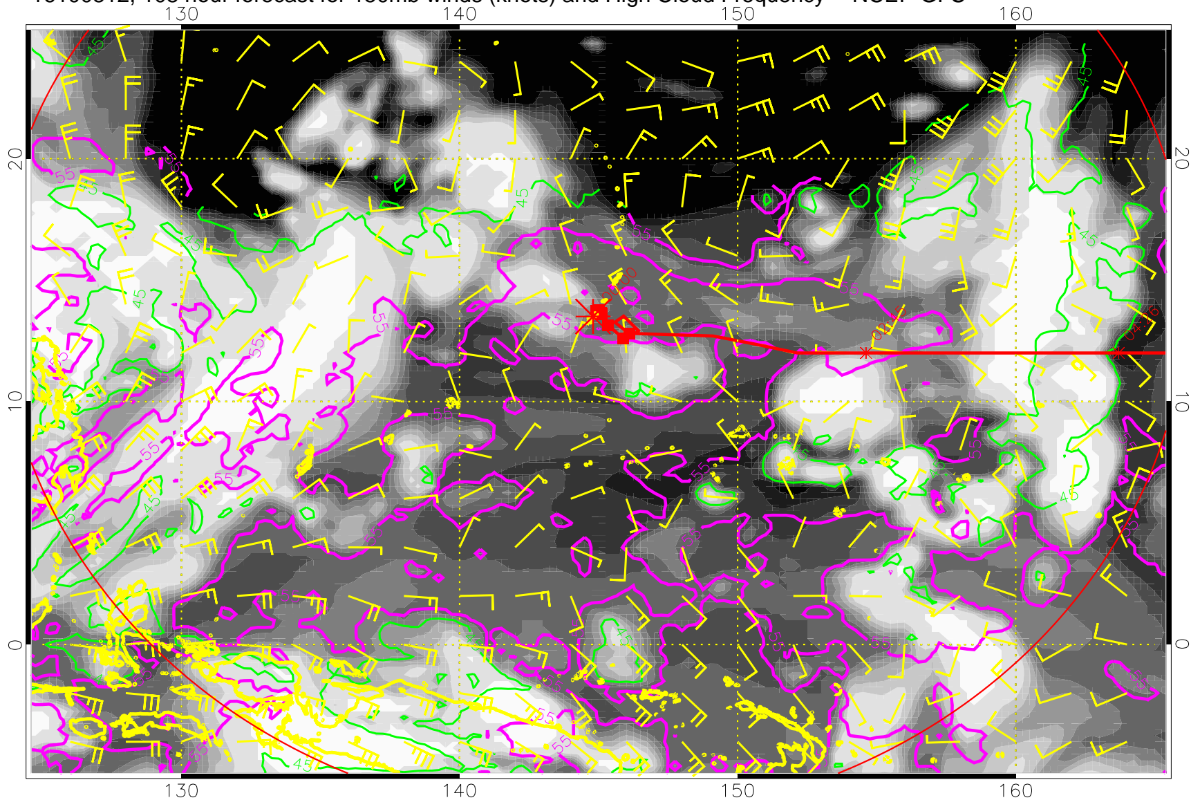
16100812, 108 hour forecast for 150mb winds (knots) and High Cloud Frequency -- NCEP GFS
