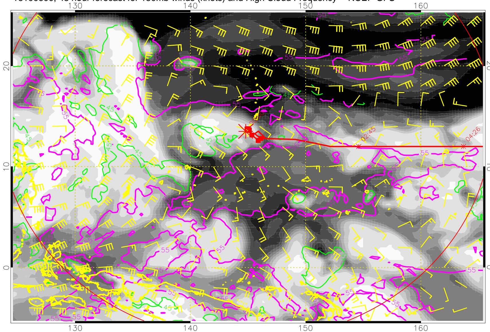
16100600, 48 hour forecast for 150mb winds (knots) and High Cloud Frequency -- NCEP GFS
