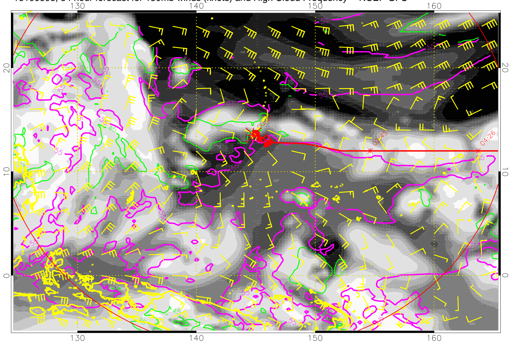
16100606, 54 hour forecast for 150mb winds (knots) and High Cloud Frequency -- NCEP GFS
