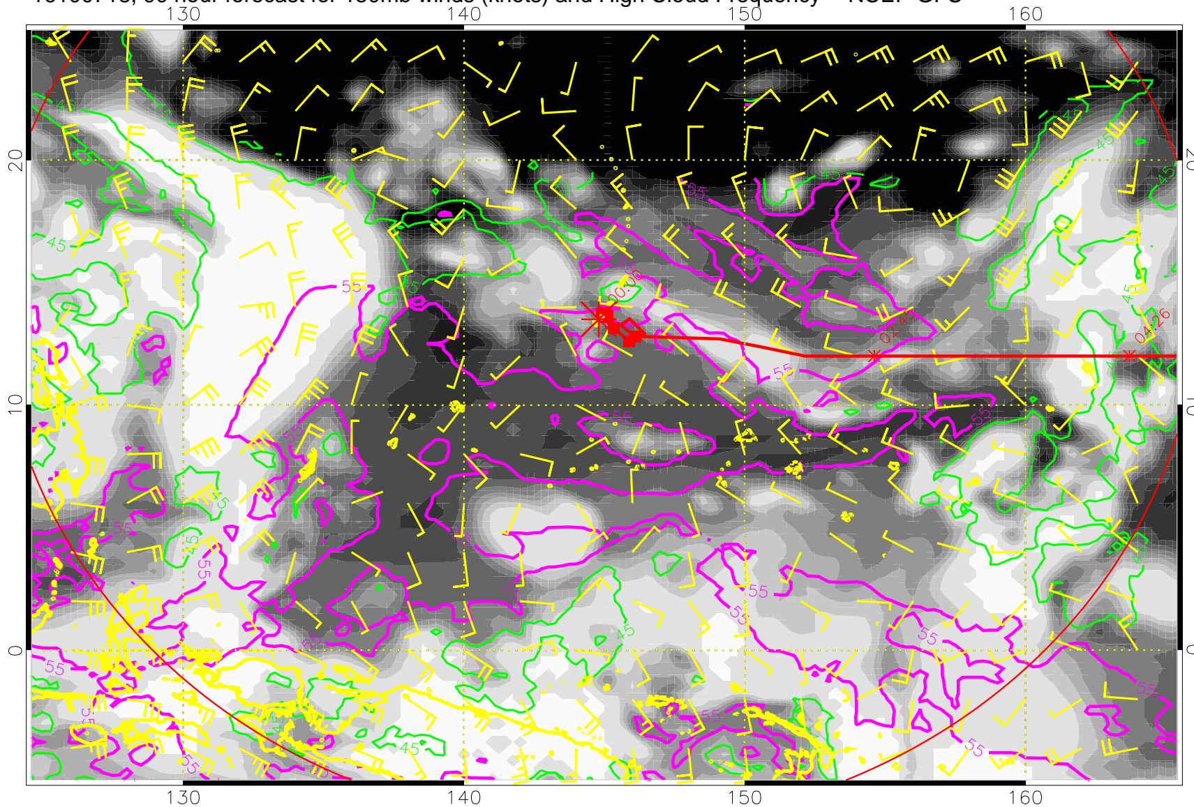
16100718, 90 hour forecast for 150mb winds (knots) and High Cloud Frequency -- NCEP GFS
