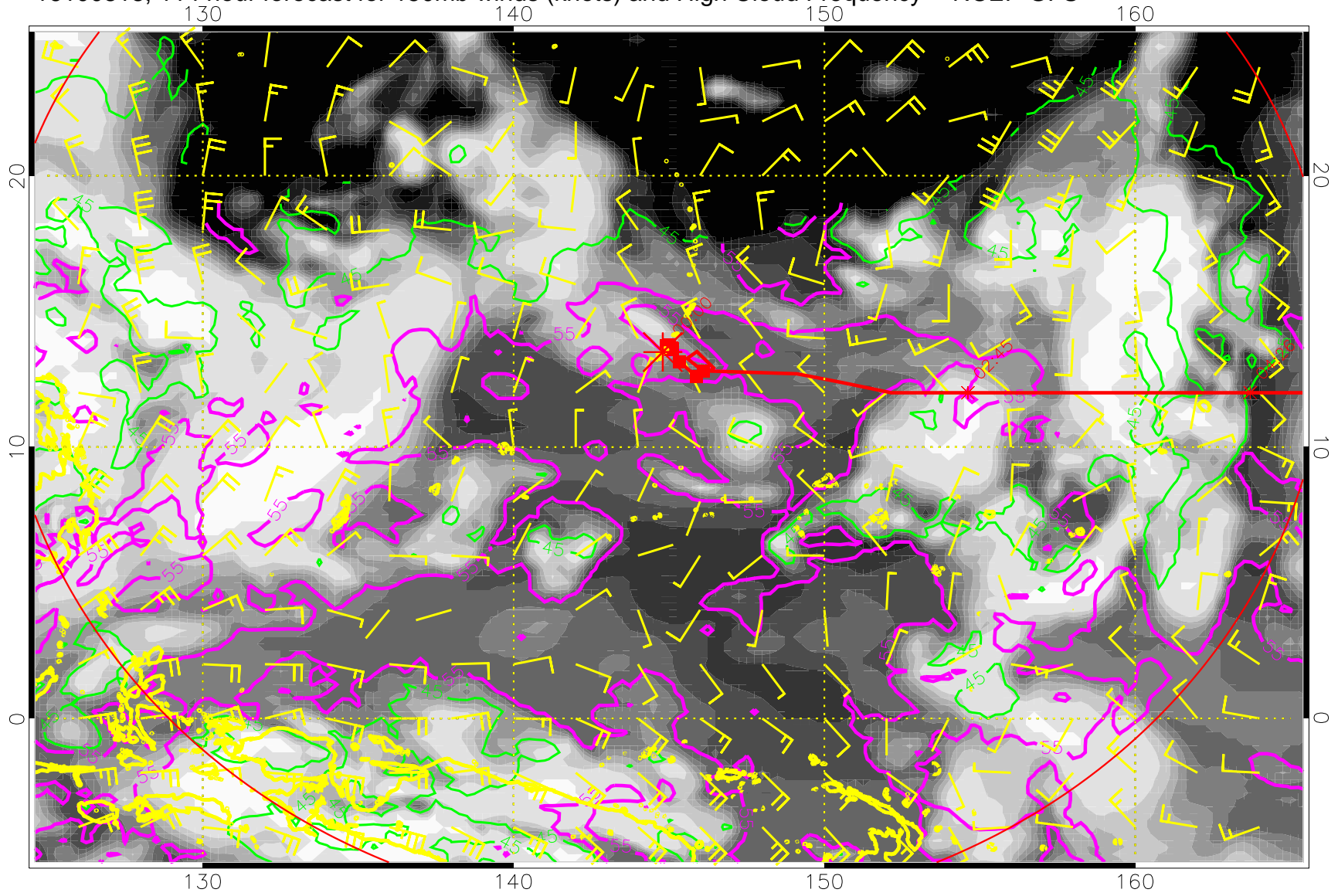
16100818, 114 hour forecast for 150mb winds (knots) and High Cloud Frequency -- NCEP GFS
