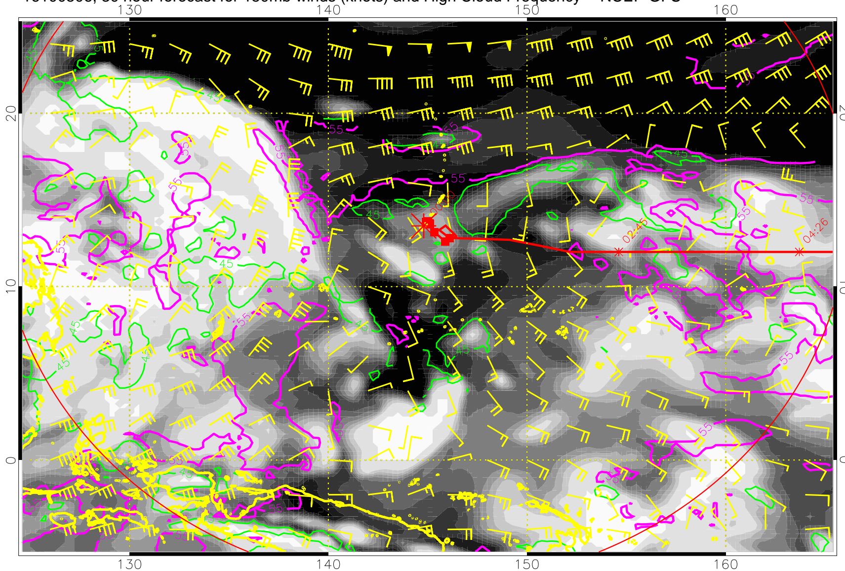
16100506, 30 hour forecast for 150mb winds (knots) and High Cloud Frequency -- NCEP GFS
