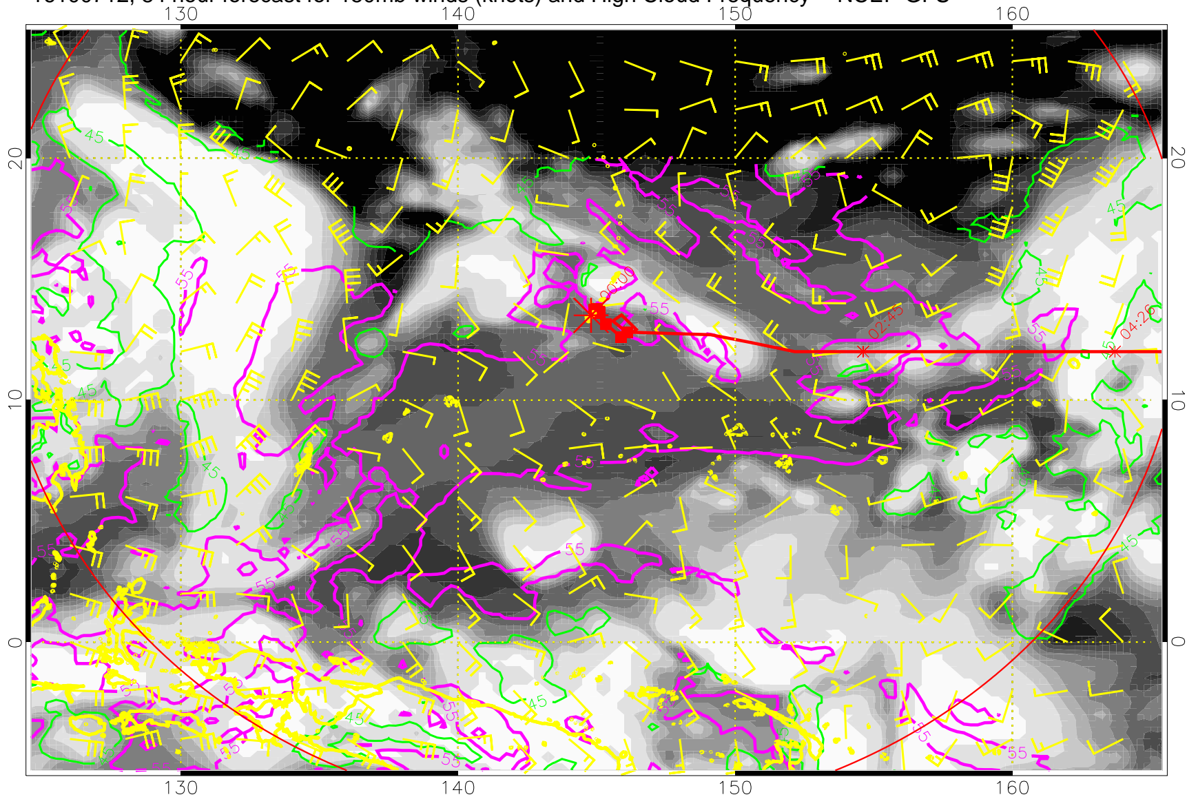
16100712, 84 hour forecast for 150mb winds (knots) and High Cloud Frequency -- NCEP GFS
