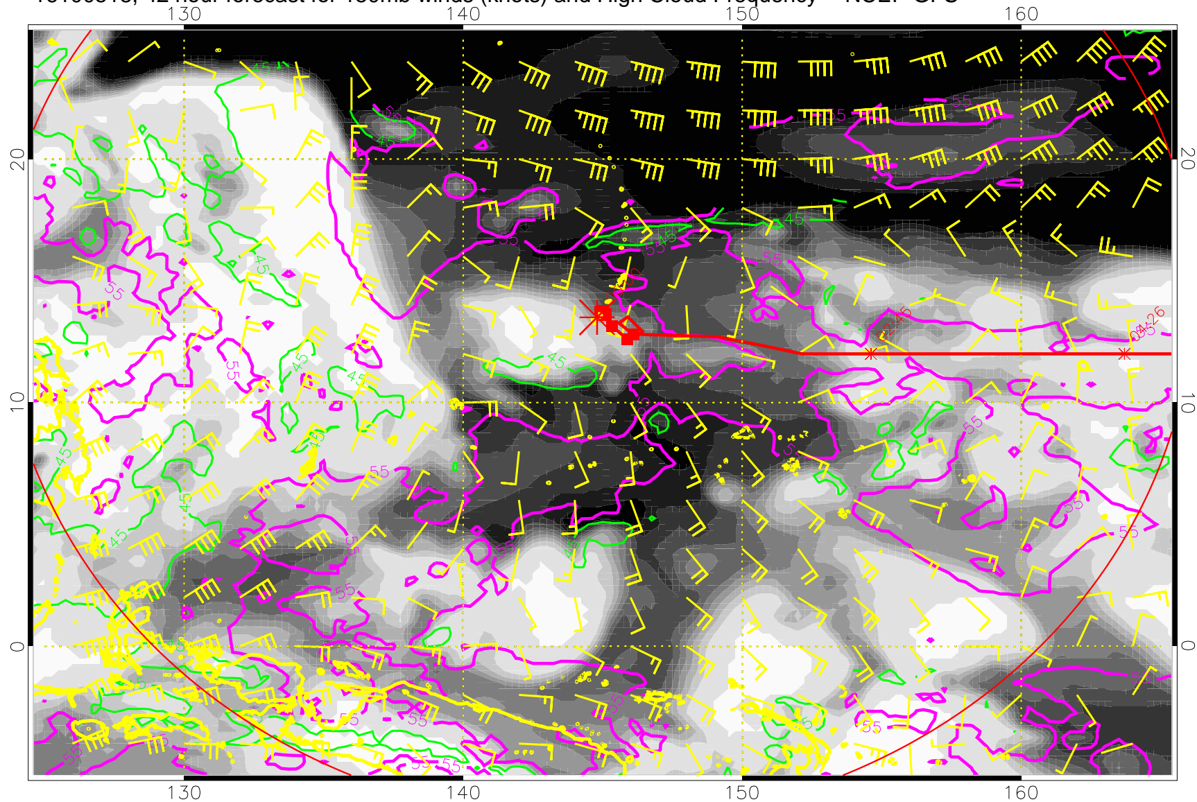
16100518, 42 hour forecast for 150mb winds (knots) and High Cloud Frequency -- NCEP GFS
