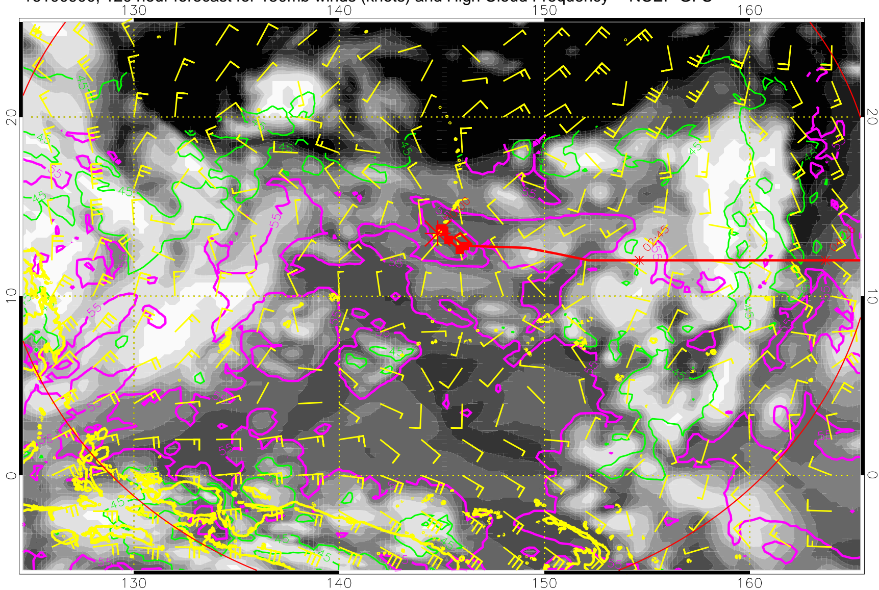
16100900, 120 hour forecast for 150mb winds (knots) and High Cloud Frequency -- NCEP GFS
