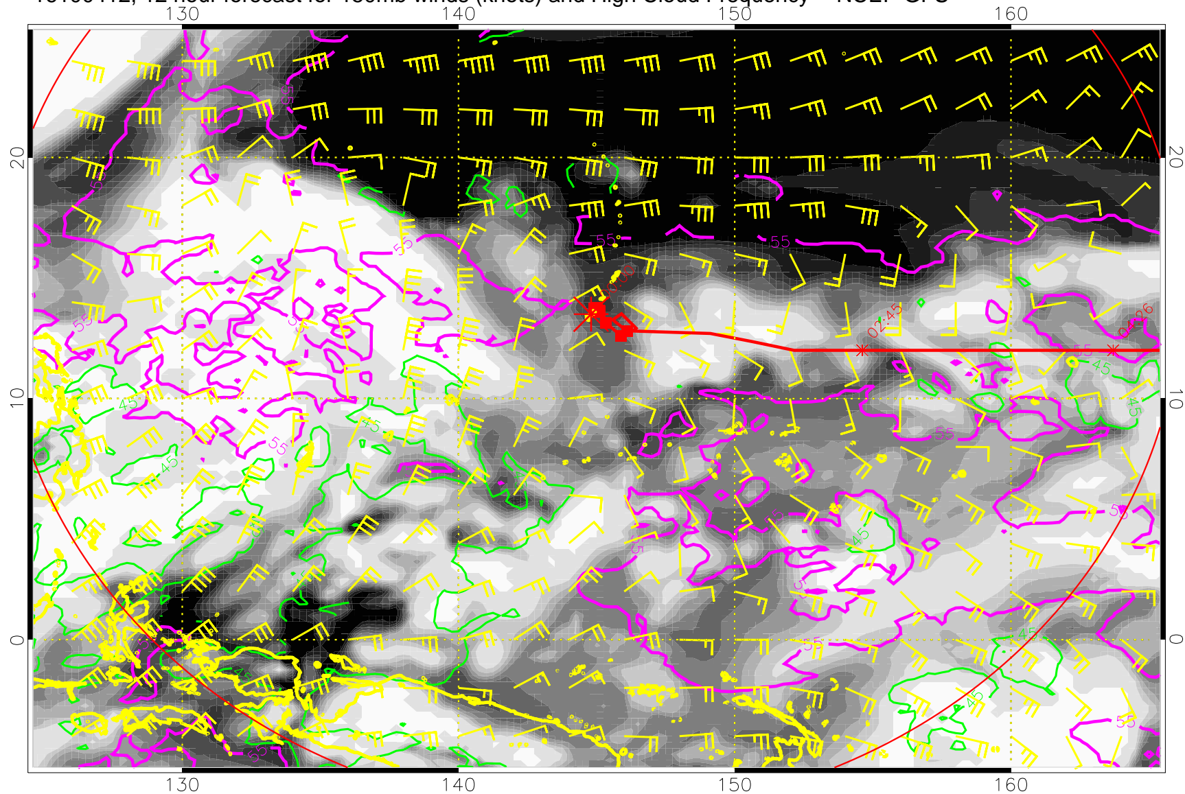
16100412, 12 hour forecast for 150mb winds (knots) and High Cloud Frequency -- NCEP GFS
